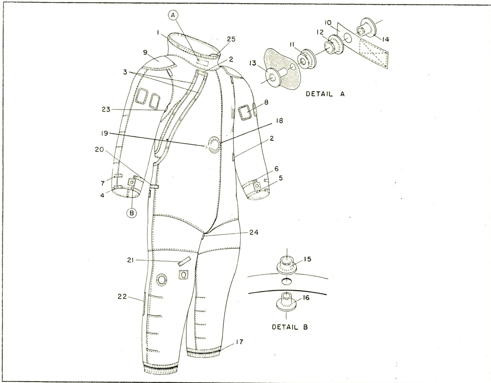
Figure 4 EV TISA Liner Assembly
