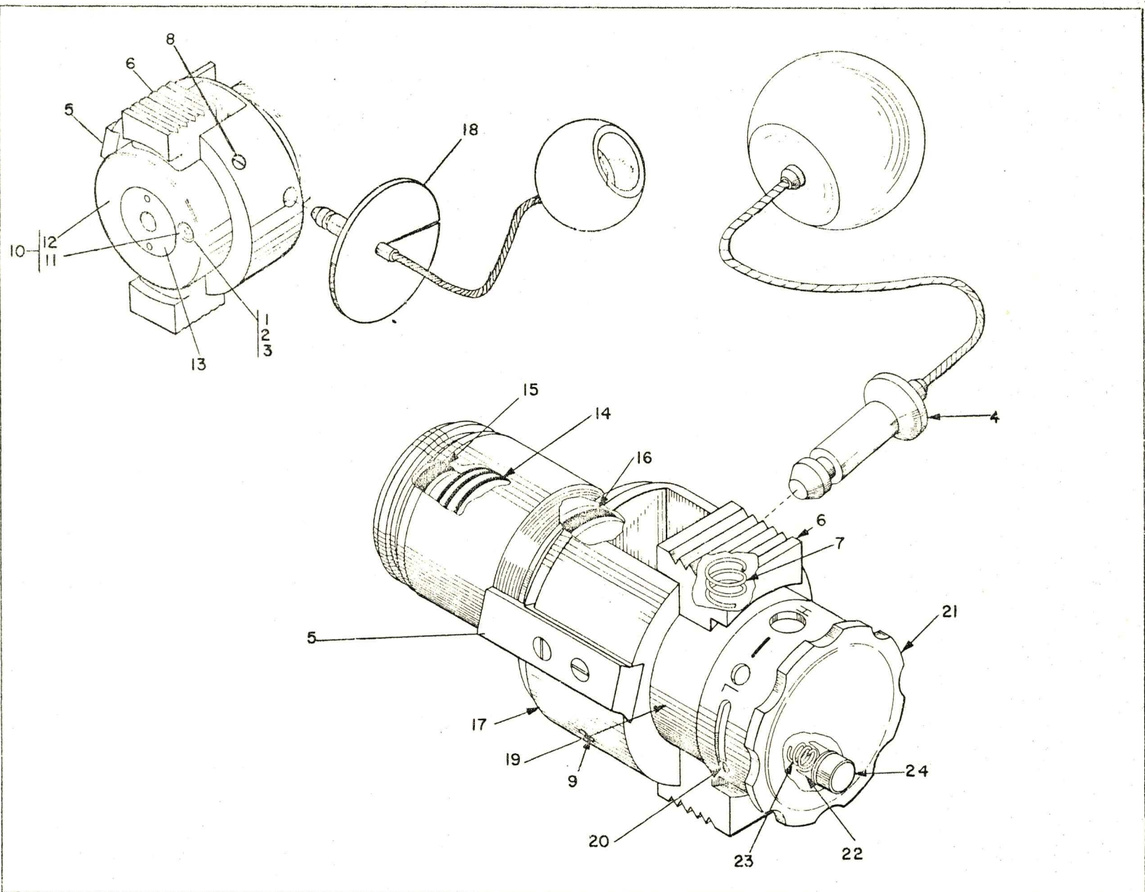
Figure 47 Purge Valve Assembly
