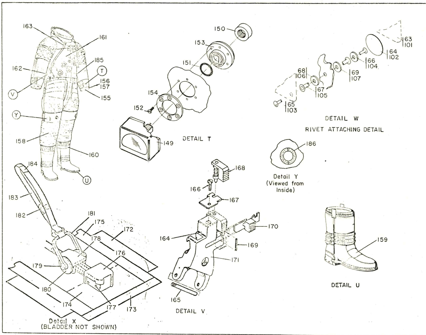
Figure 36 (Sheet 6 of 6) Skylab Torso Limb Suit Assembly
