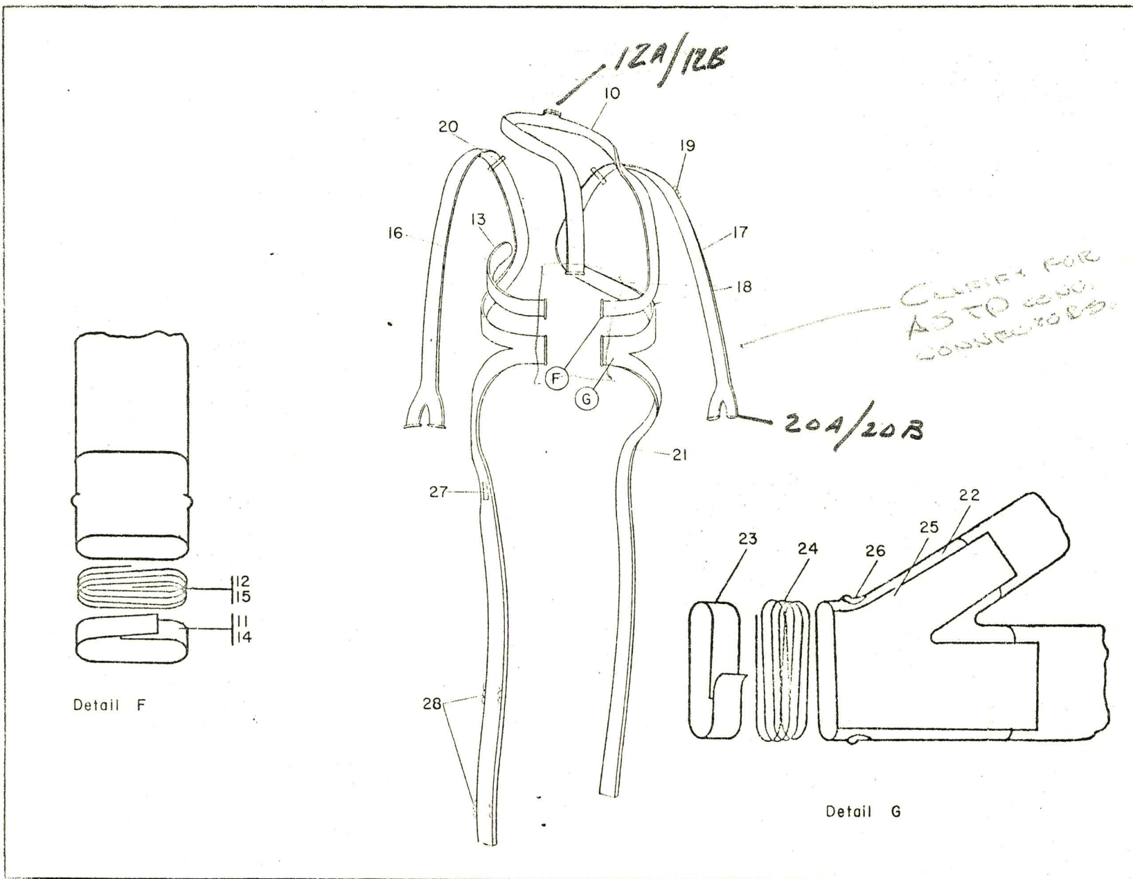
Figure 41 (Sheet 2 of 5) Torso Limb Suit Assembly, ASTP
