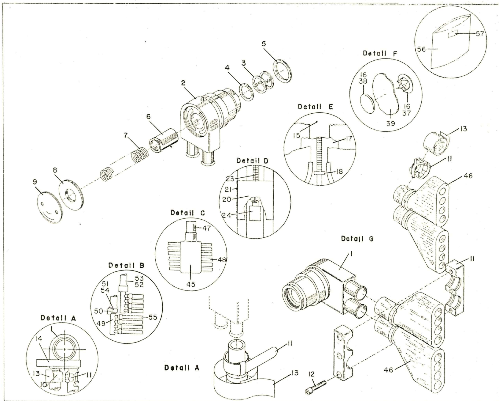
Figure 43 (Sheet 2 of 2) Liquid Cooling Garment Assembly
