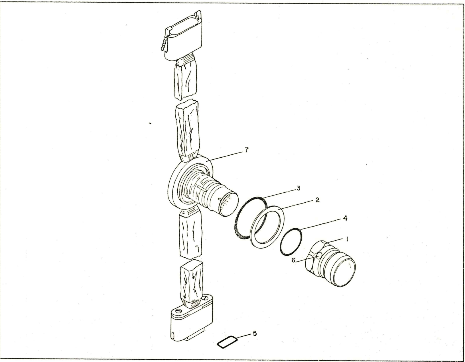
Figure 55 CWG Electrical Harness
