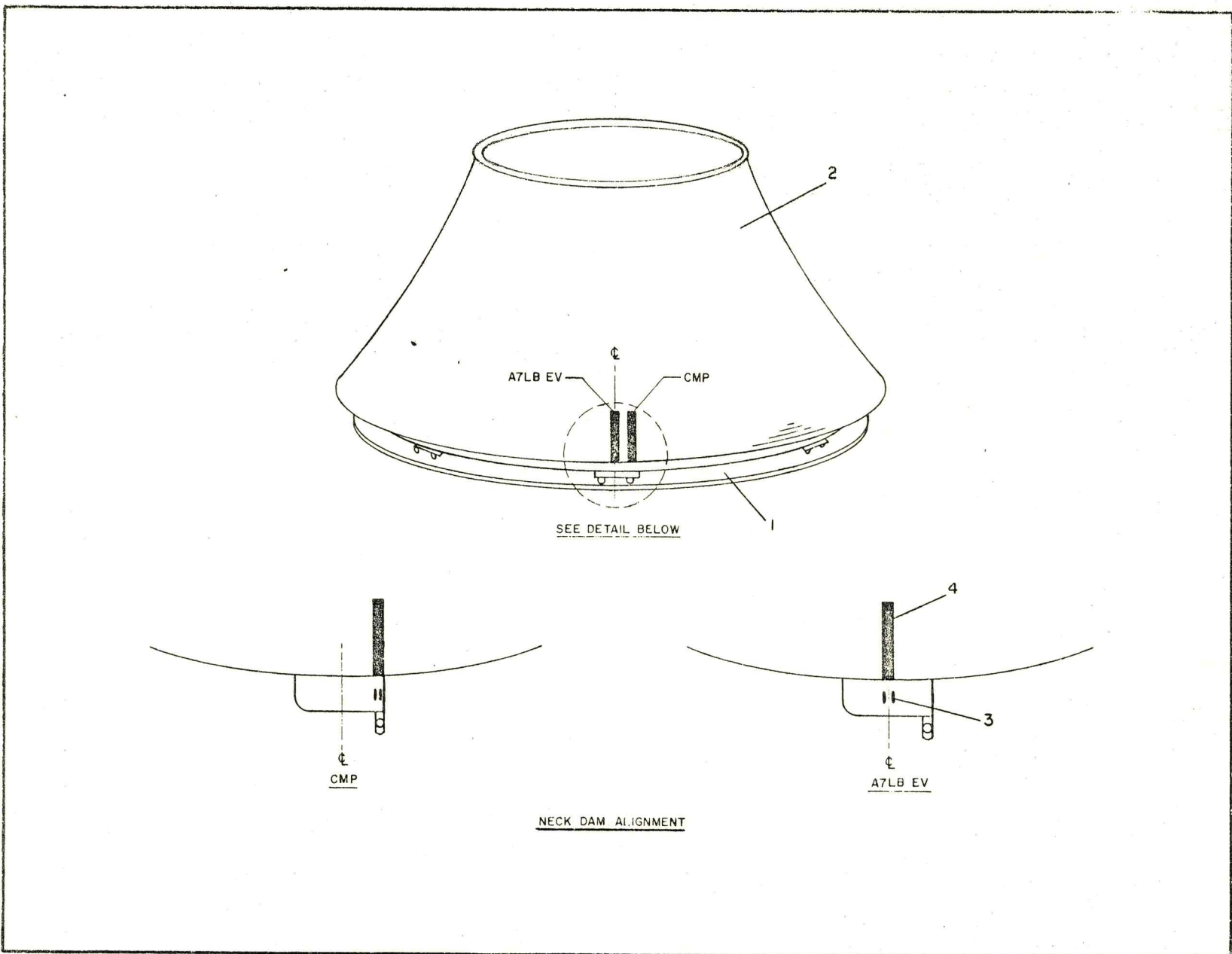
Figure 50 Neck Dam Assembly
