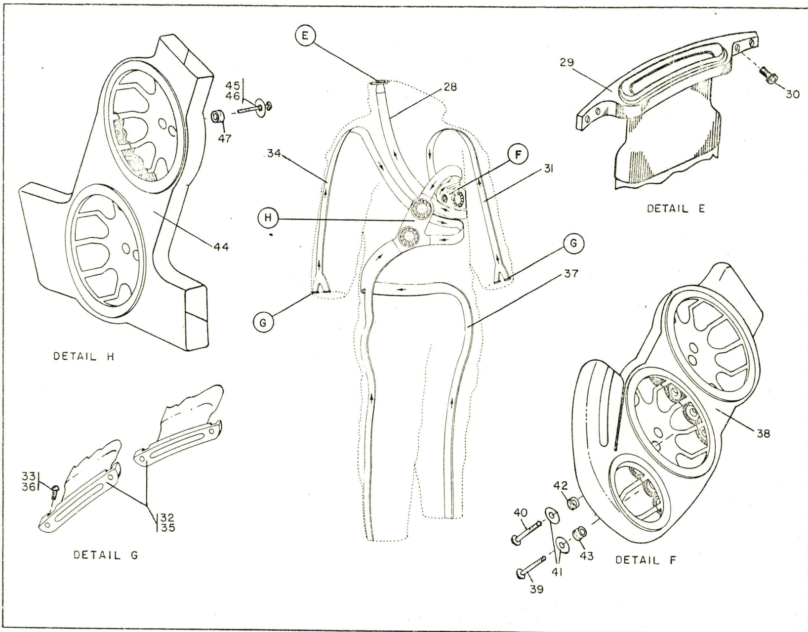
Figure 36 (Sheet 2 of 6) Skylab Torso Limb Suit Assembly
