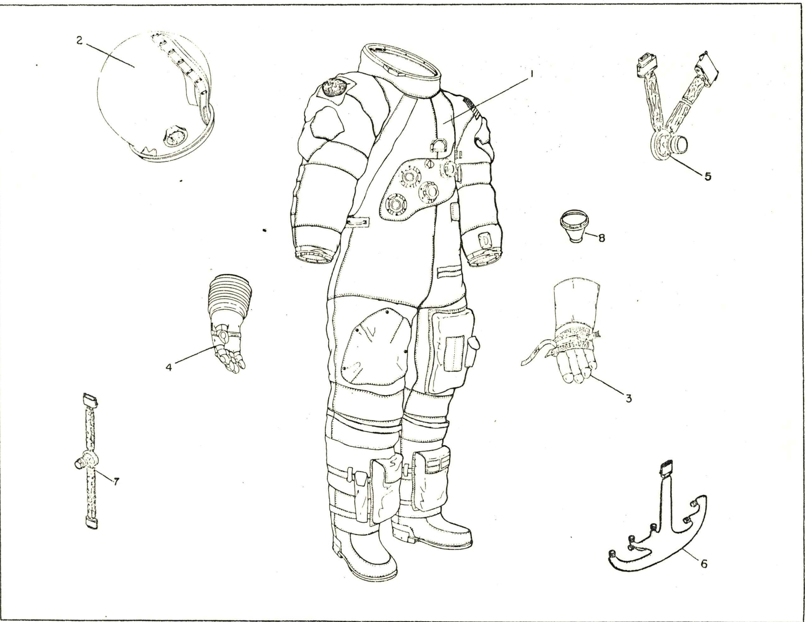
Figure 34 Skylab Separable Components
