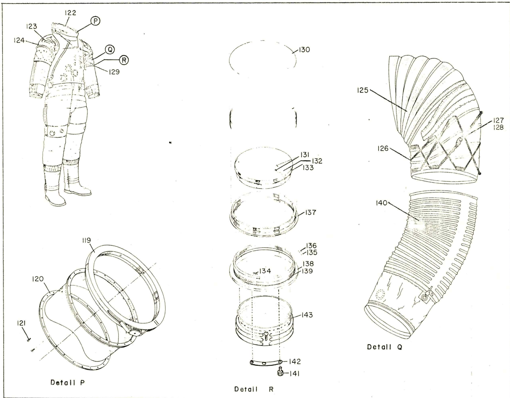
Figure 3 (Sheet 5 of 6) A7LB EV Torso Limb Suit Assembly
