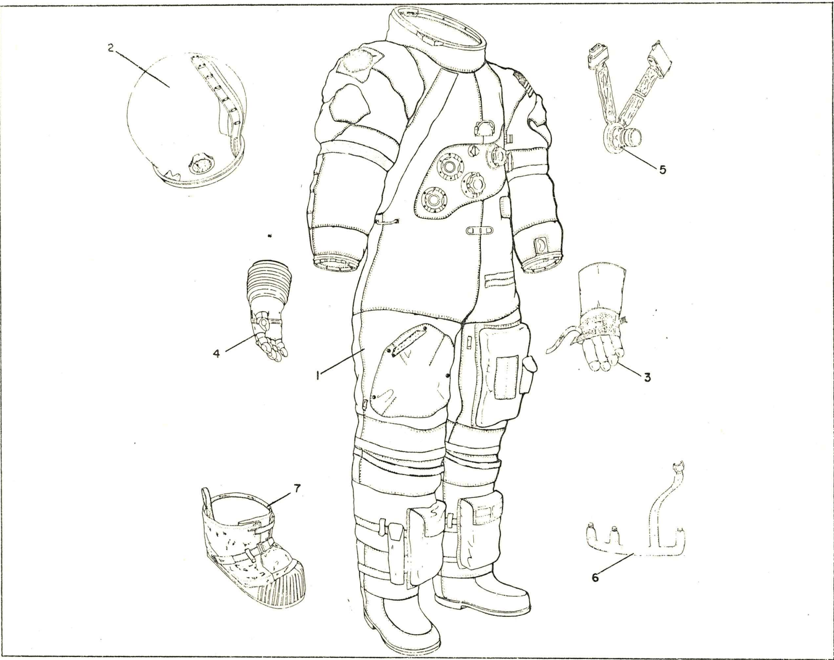
Figure 1 A7LB EV Separable Components
