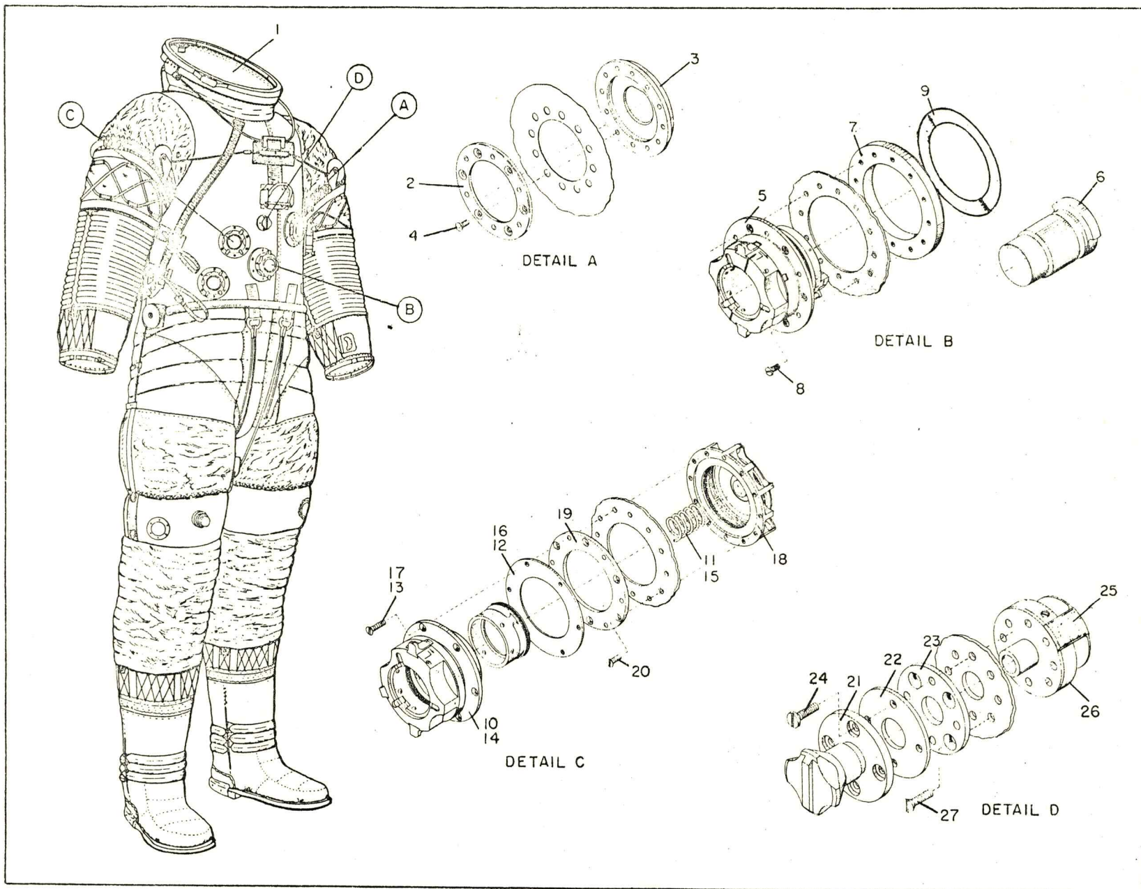
Figure 36 (Sheet 1 of 6) Skylab Torso Limb Suit Assembly
