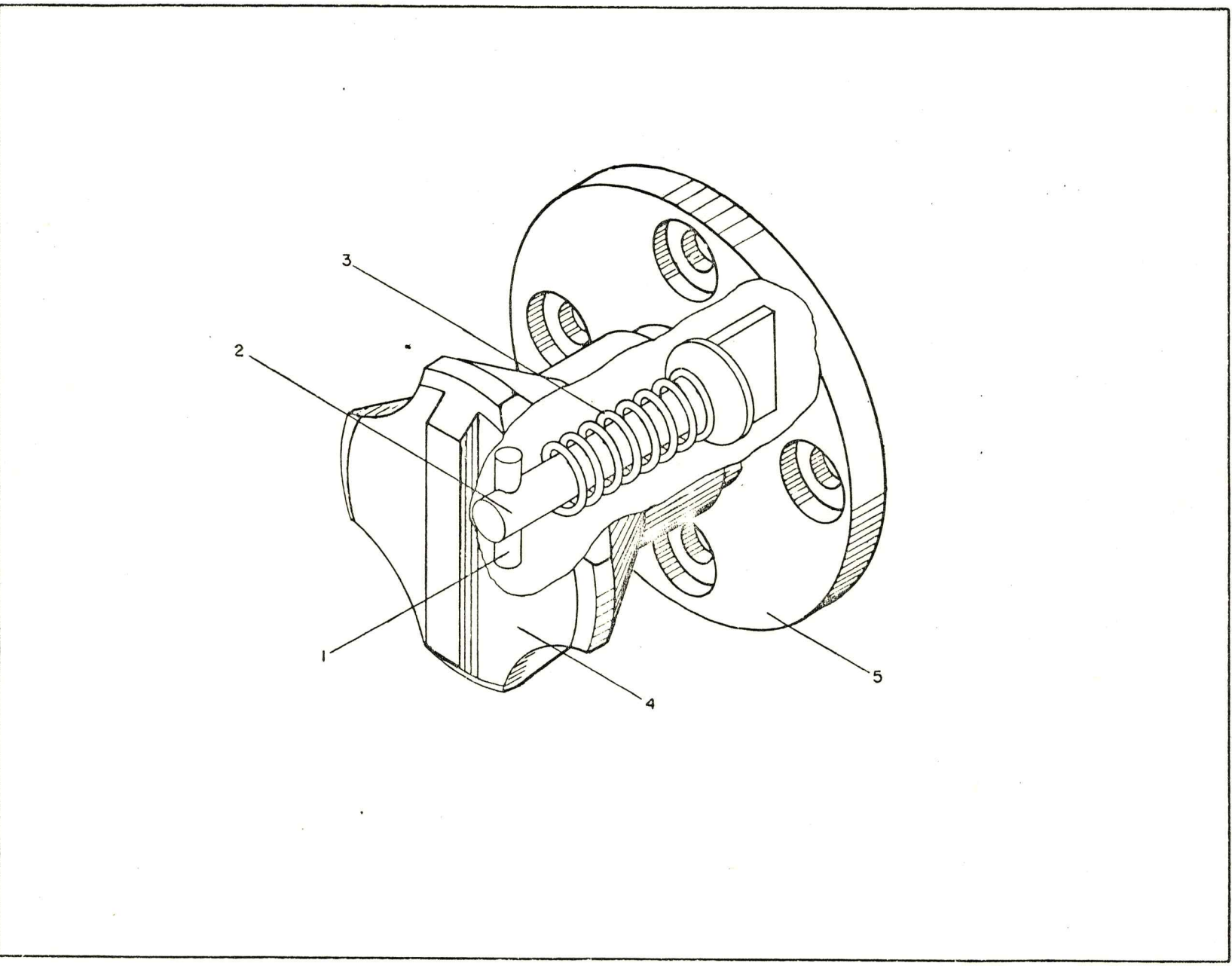
Figure 12 Diverter Valve Knob and Shaft Assy
