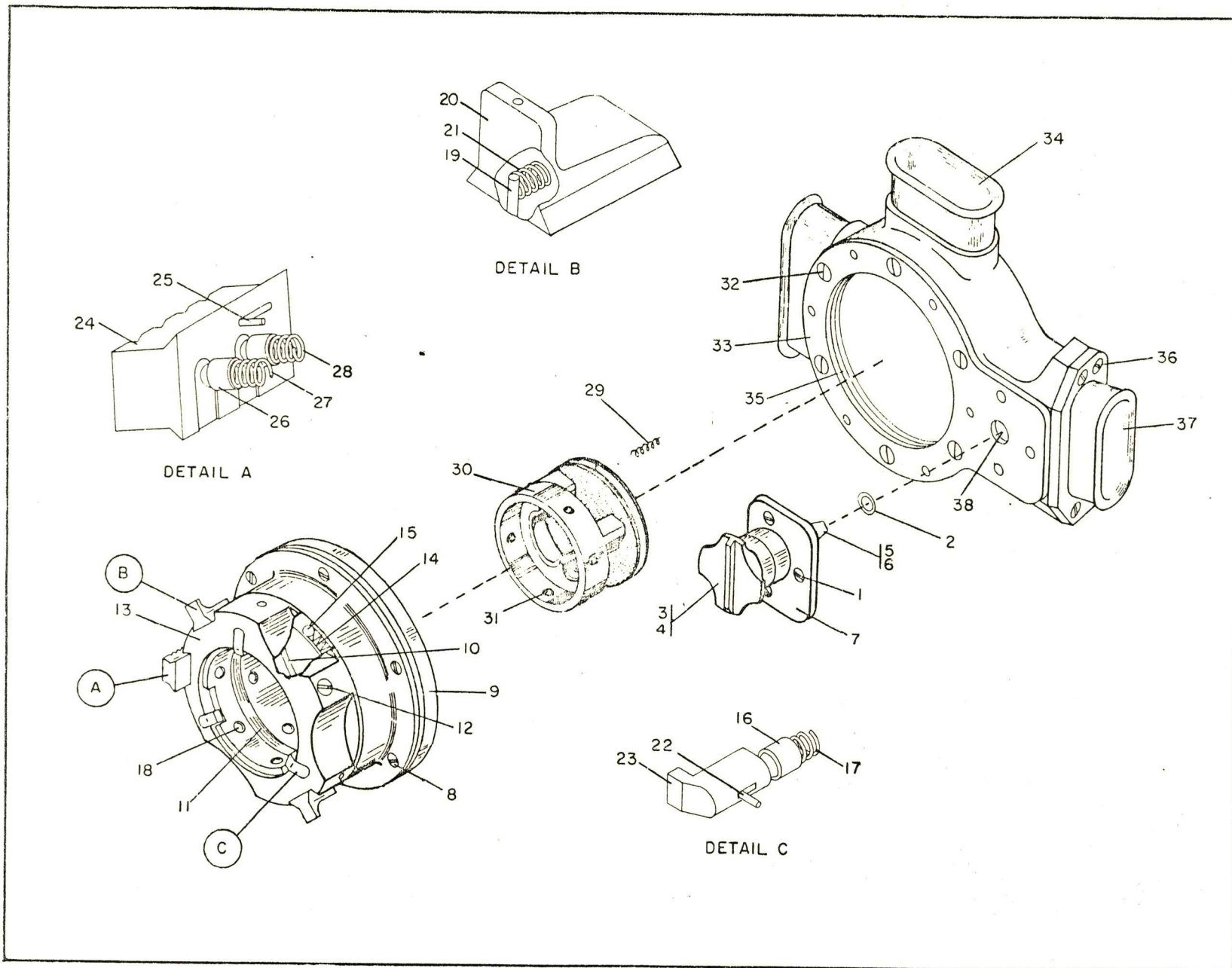
Figure 30 Upper Gas Connector
