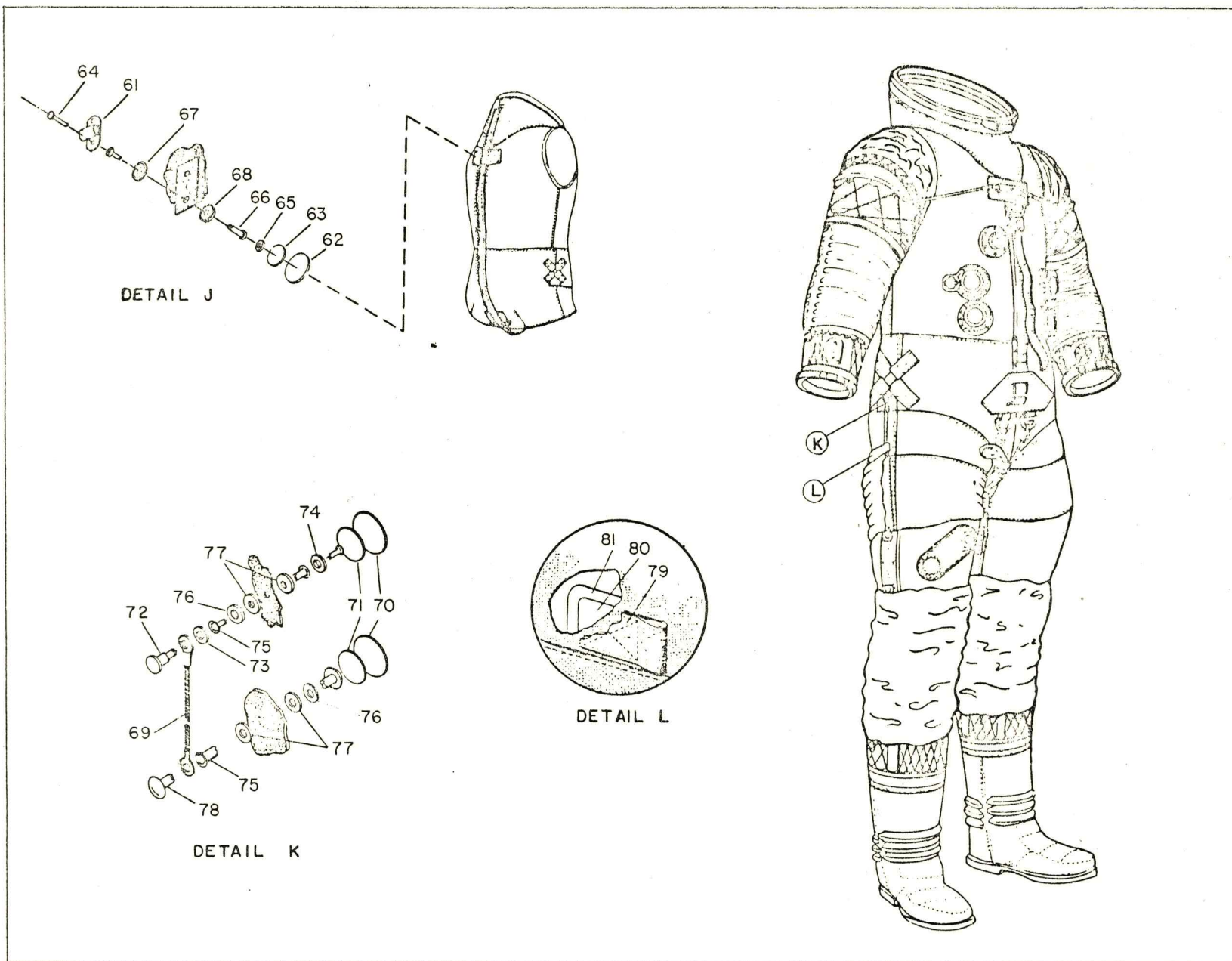
Figure 25 (Sheet 3 of 5) Torso Limb Suit Assembly, CMP
