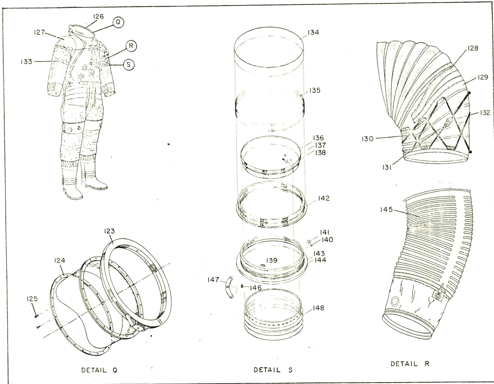
Figure 36 (Sheet 5 of 6) Skylab Torso Limb Suit Assembly
