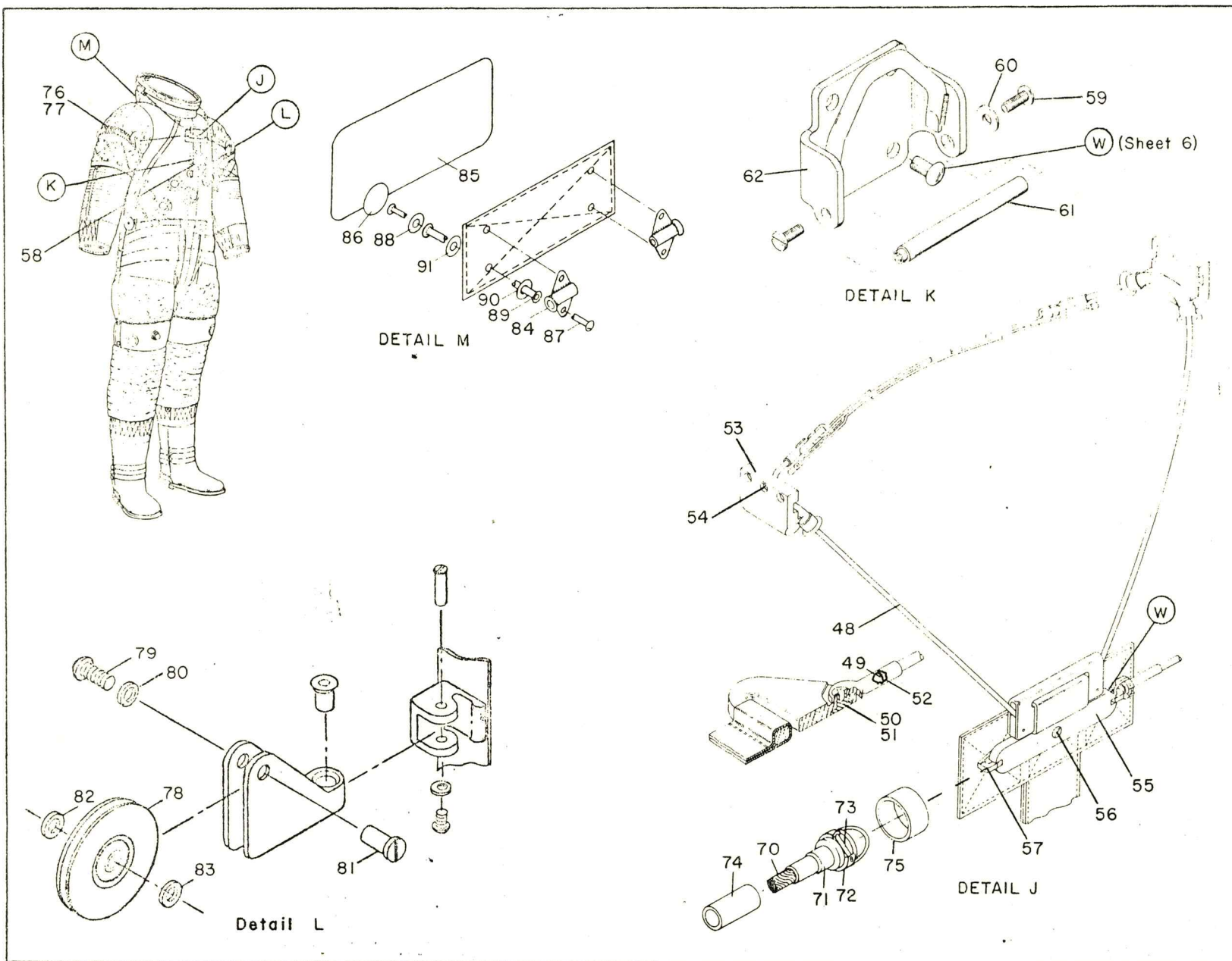
Figure 36 (Sheet 3 of 6) Skylab Torso Limb Suit Assembly
