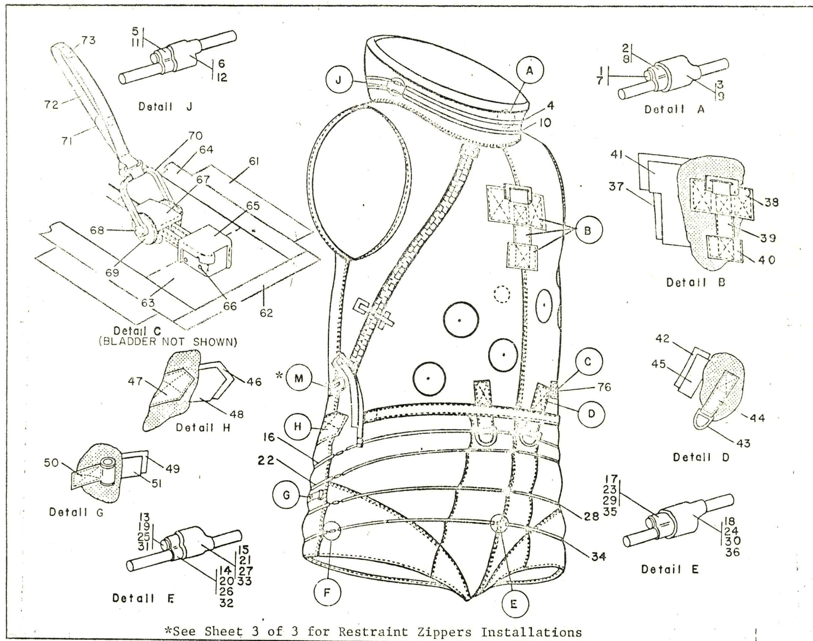
Figure 5 (Sheet 1 of 3) EV TUSA Torso Assembly
