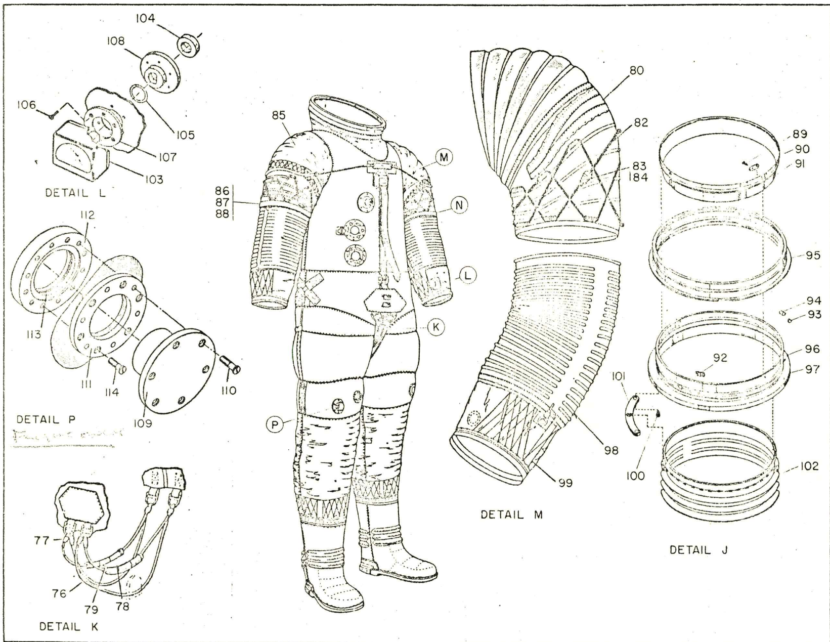
Figure 41 (Sheet 4 of 5) Torso Limb Suit Assembly, ASTP
