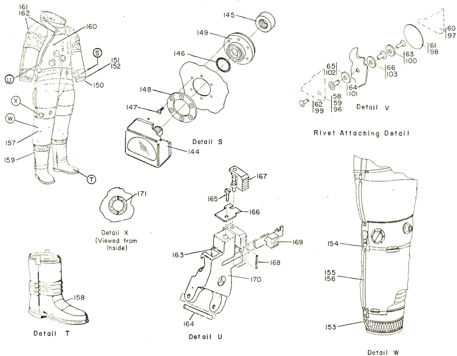
Figure 3 (Sheet 6 of 6) A7LB EV Torso Limb Suit Assembly
