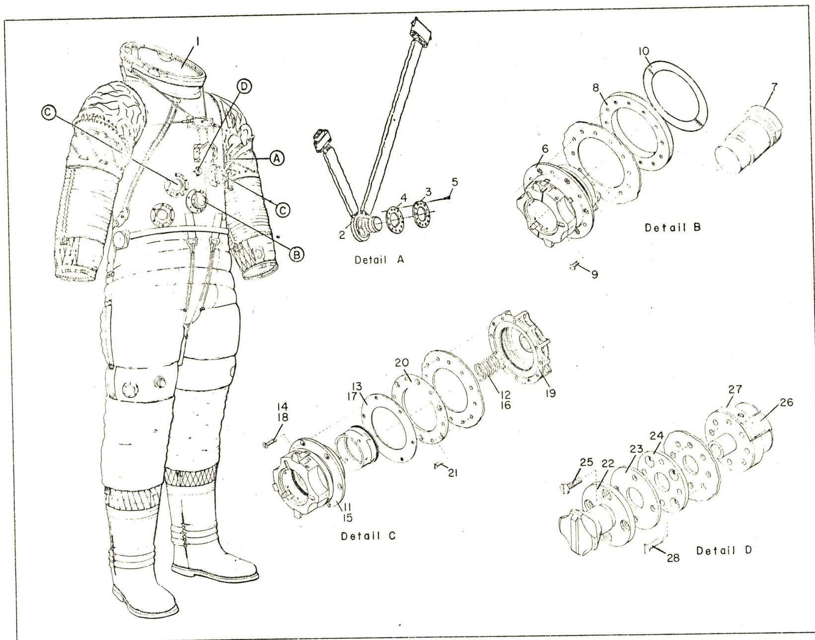
Figure 3 (Sheet 1 of 6) A7LB EV Torso Limb Suit Assembly
