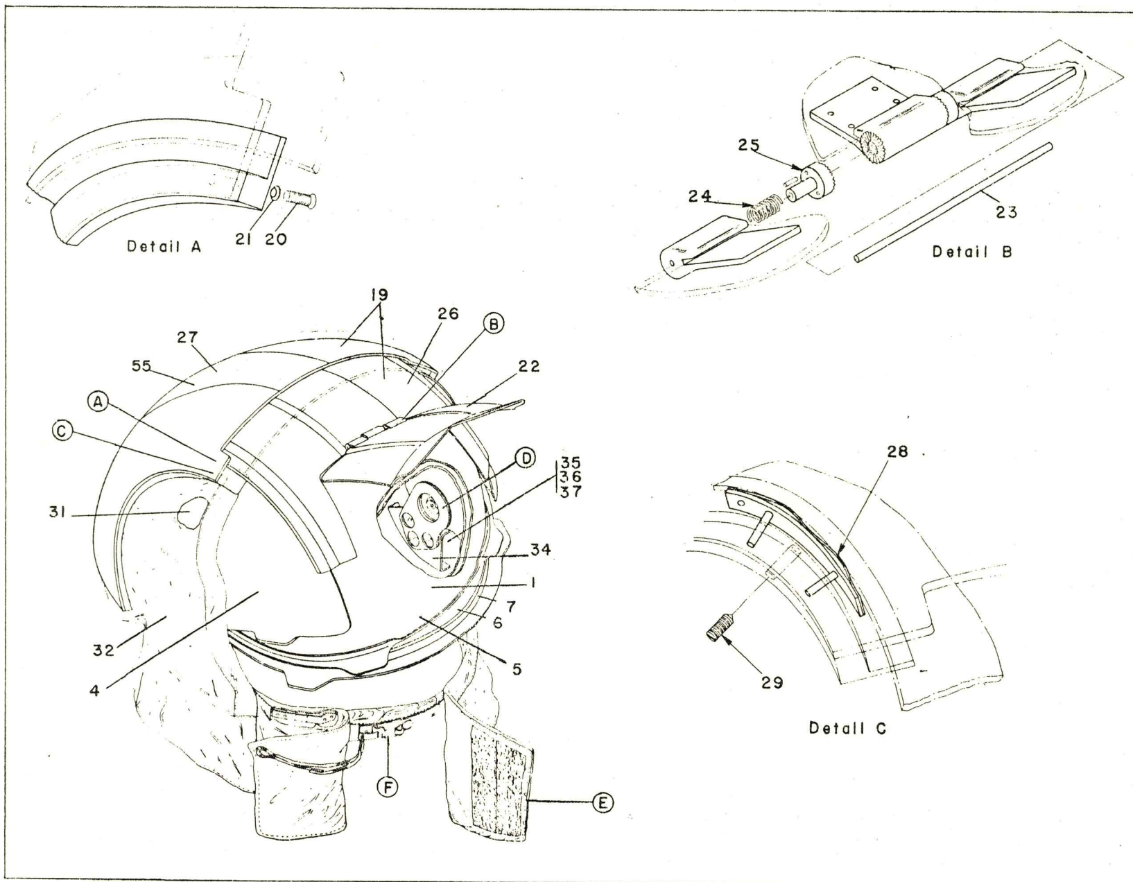
Figure 45 (Sheet 1 of 2) Lunar Extravehicular Visor Assembly
