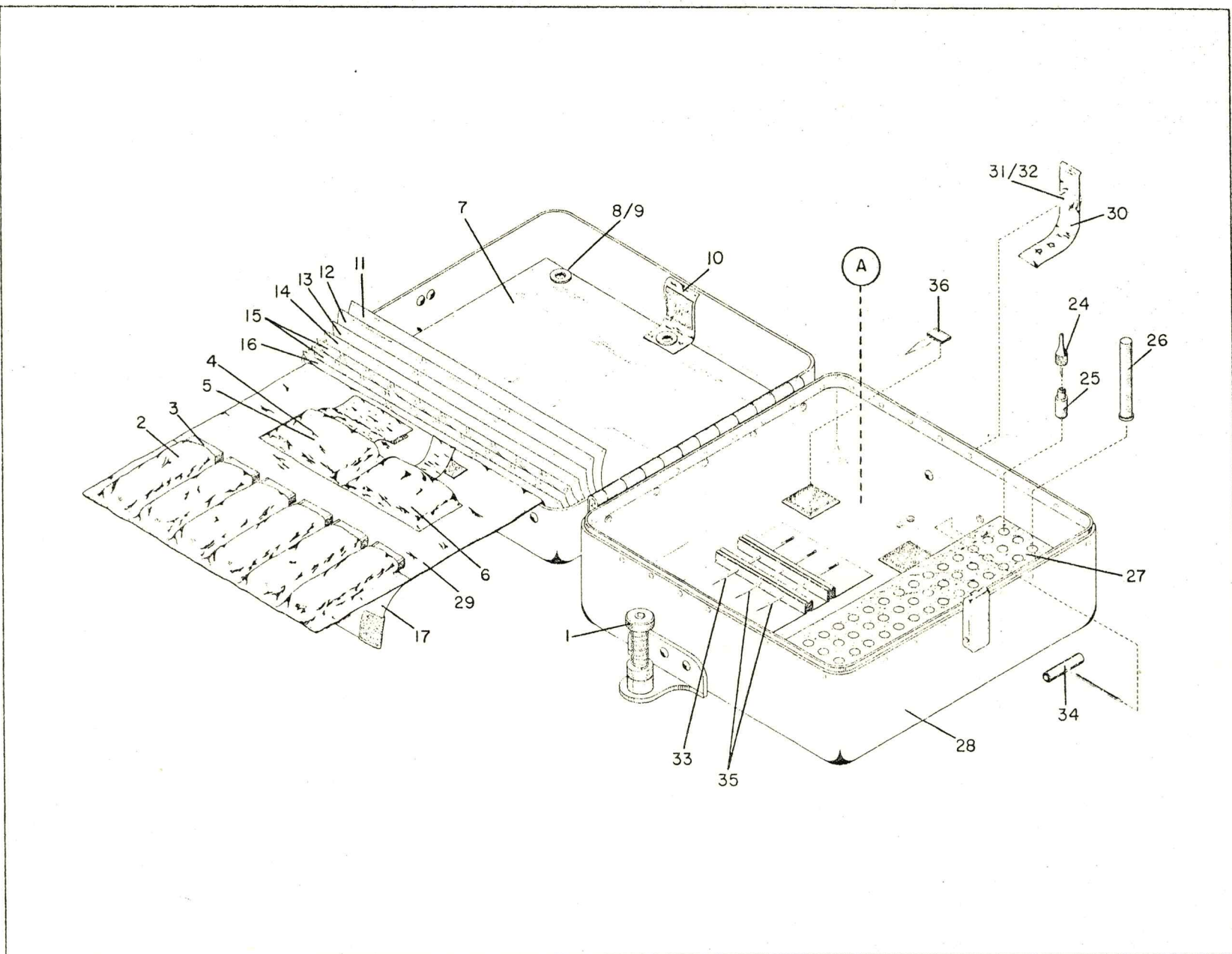
Figure 59 (Sheet 1 of 2) OMS Maintenance Kit
