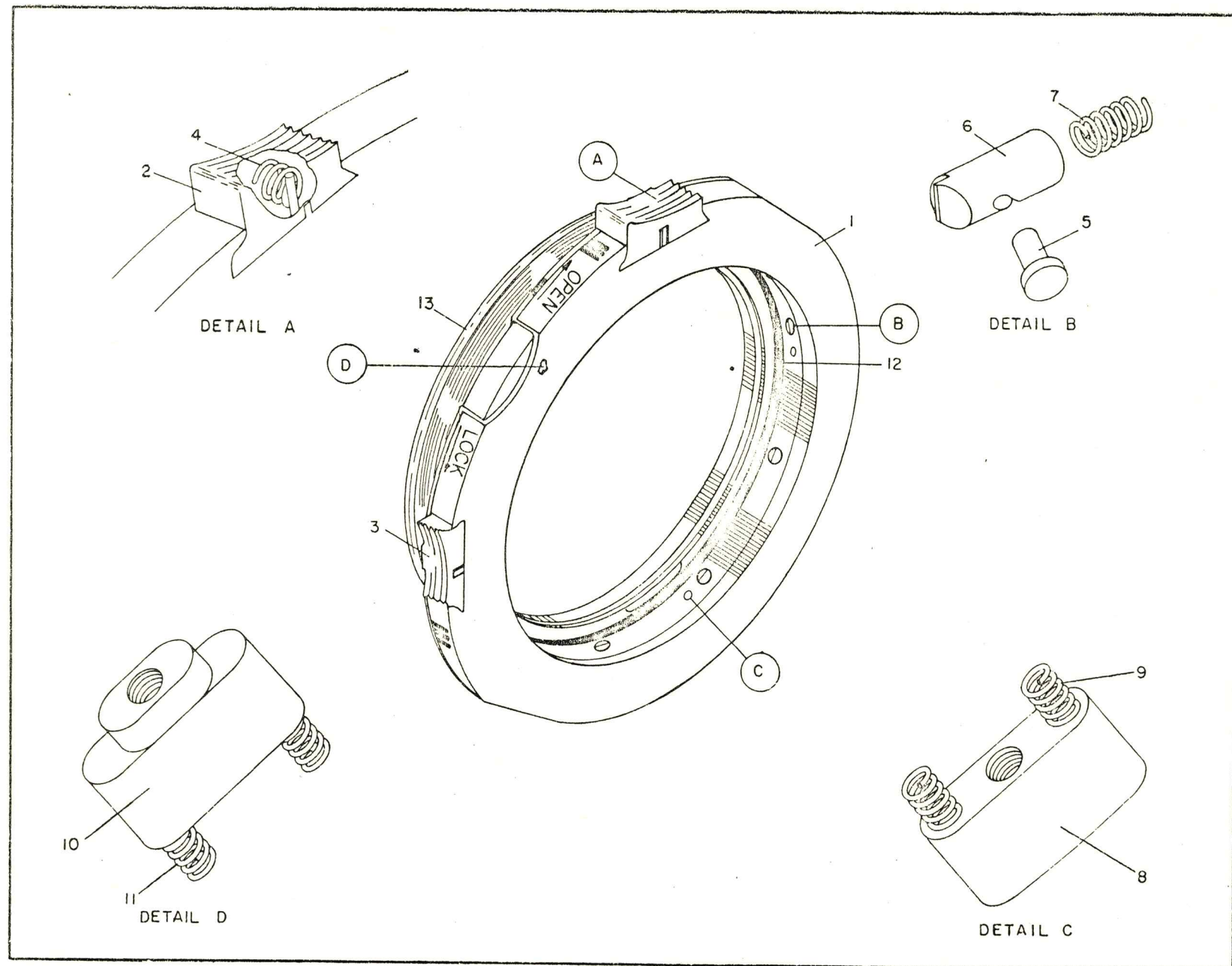
Figure 17 Suit Side Wrist Disconnect
