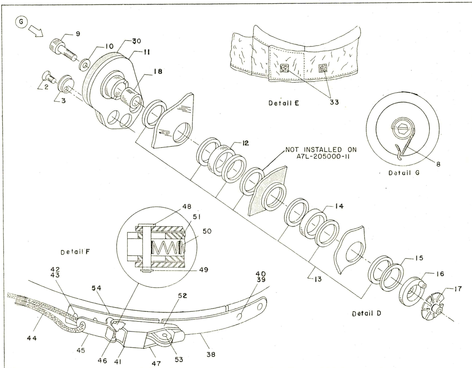
Figure 45 (Sheet 2 of 2) Lunar Extravehicular Visor Assembly
