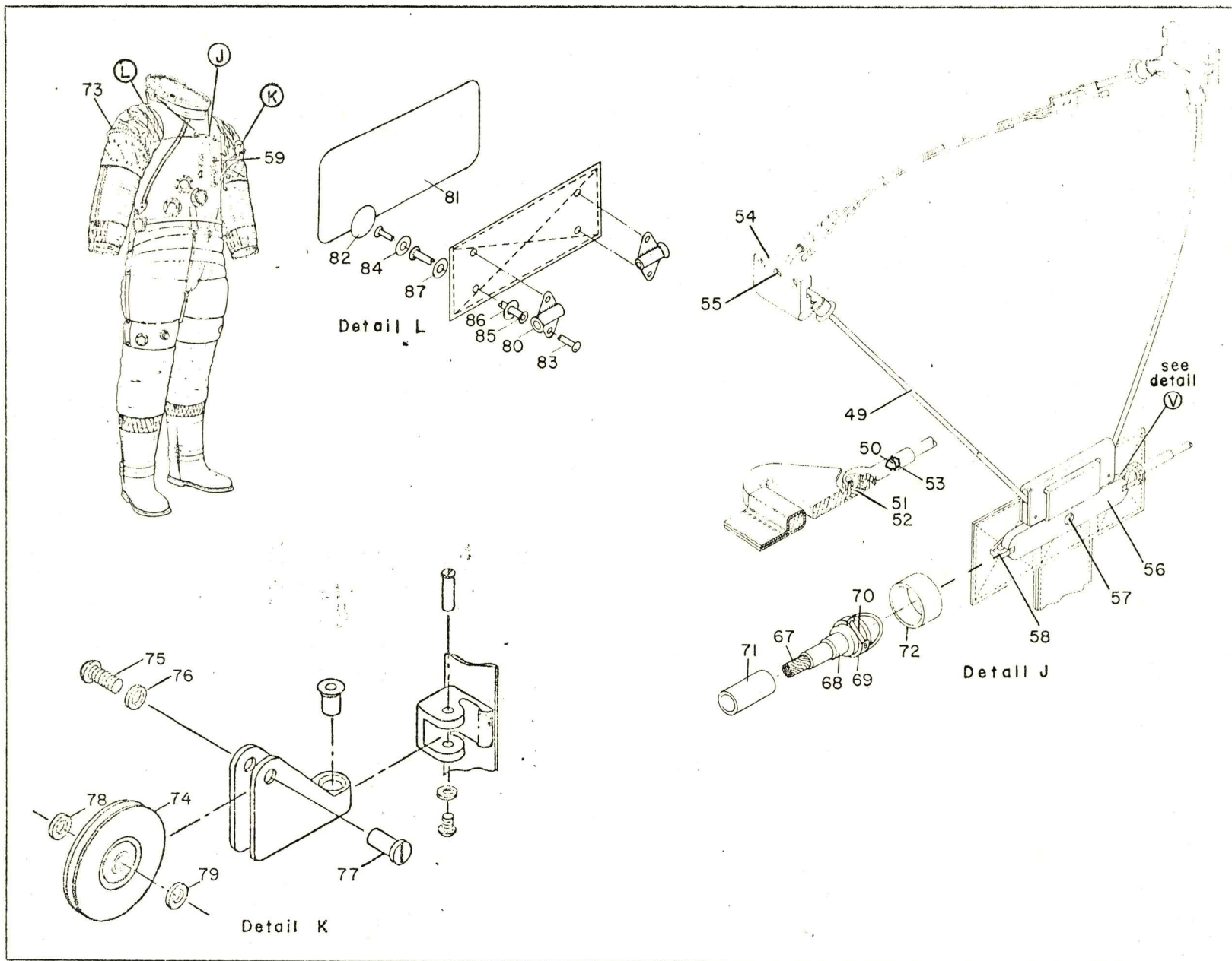
Figure 3 (Sheet 3 of 6) A7LB EV Torso Limb Suit Assembly
