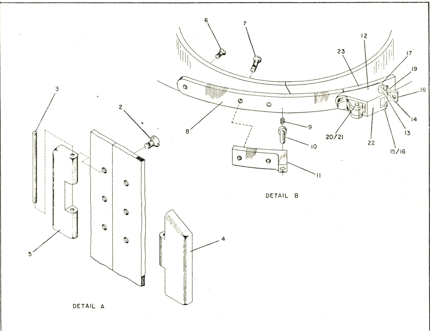
Figure 46 (Sheet 2 of 5) Skylab Extravehicular Visor Assembly
