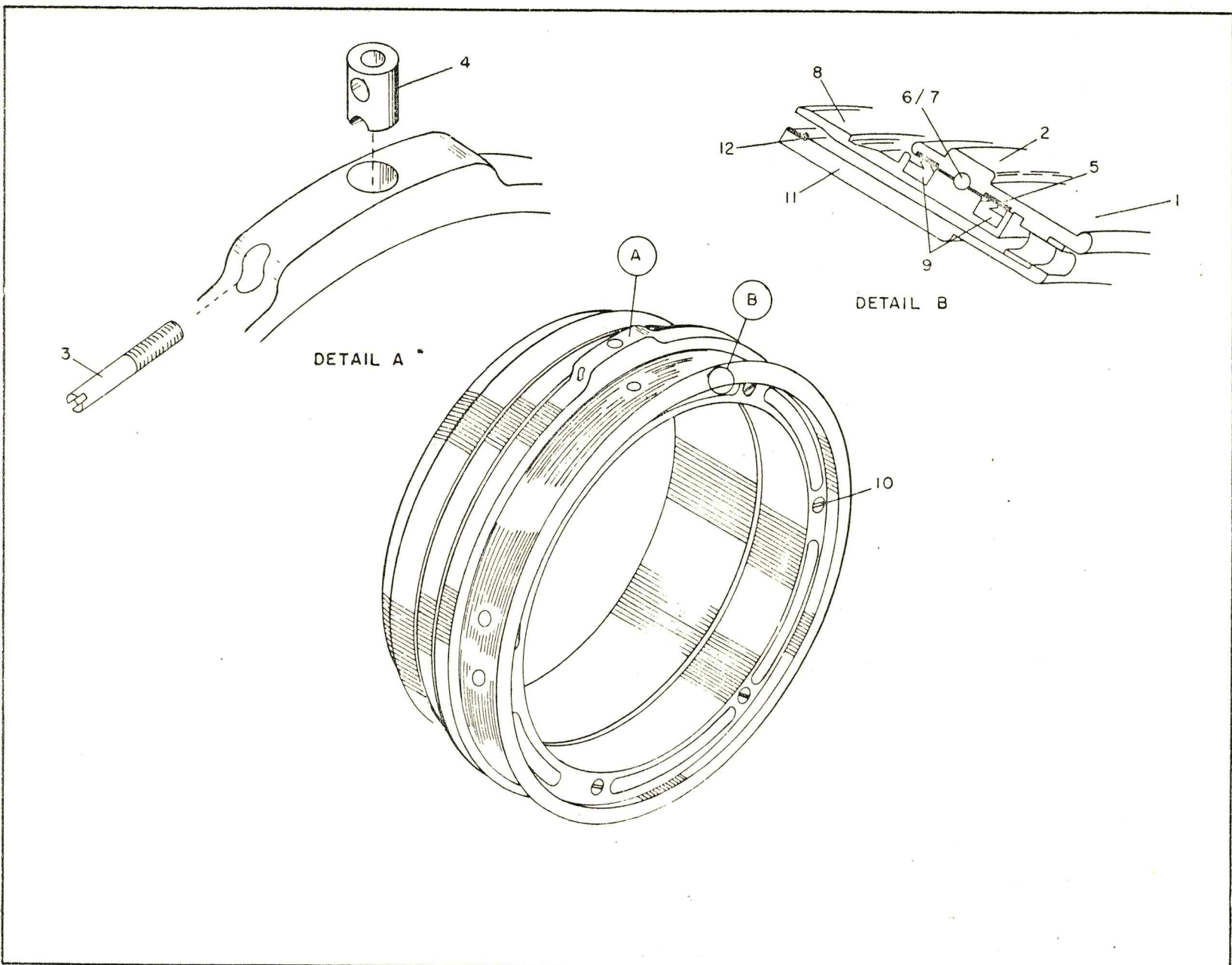
Figure 18 Glove Side Wrist Disconnect
