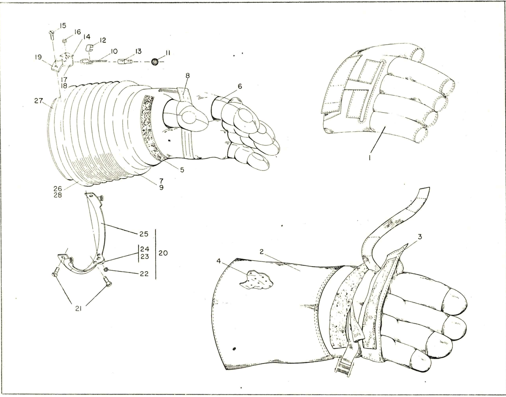
Figure 19 A7LB EV Glove Assembly
