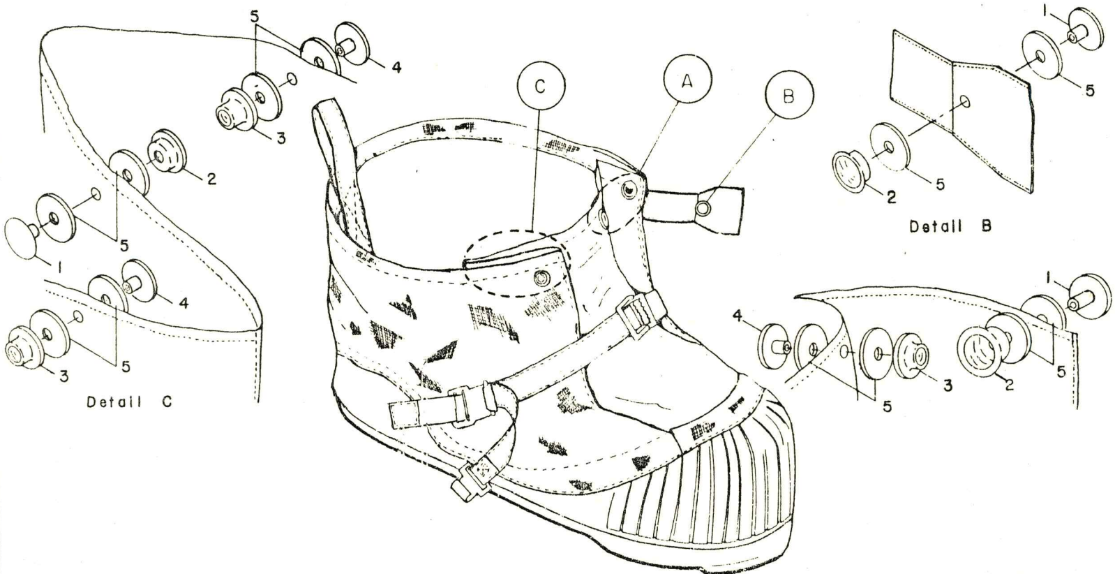
Figure 49 Lunar Boot Assembly
