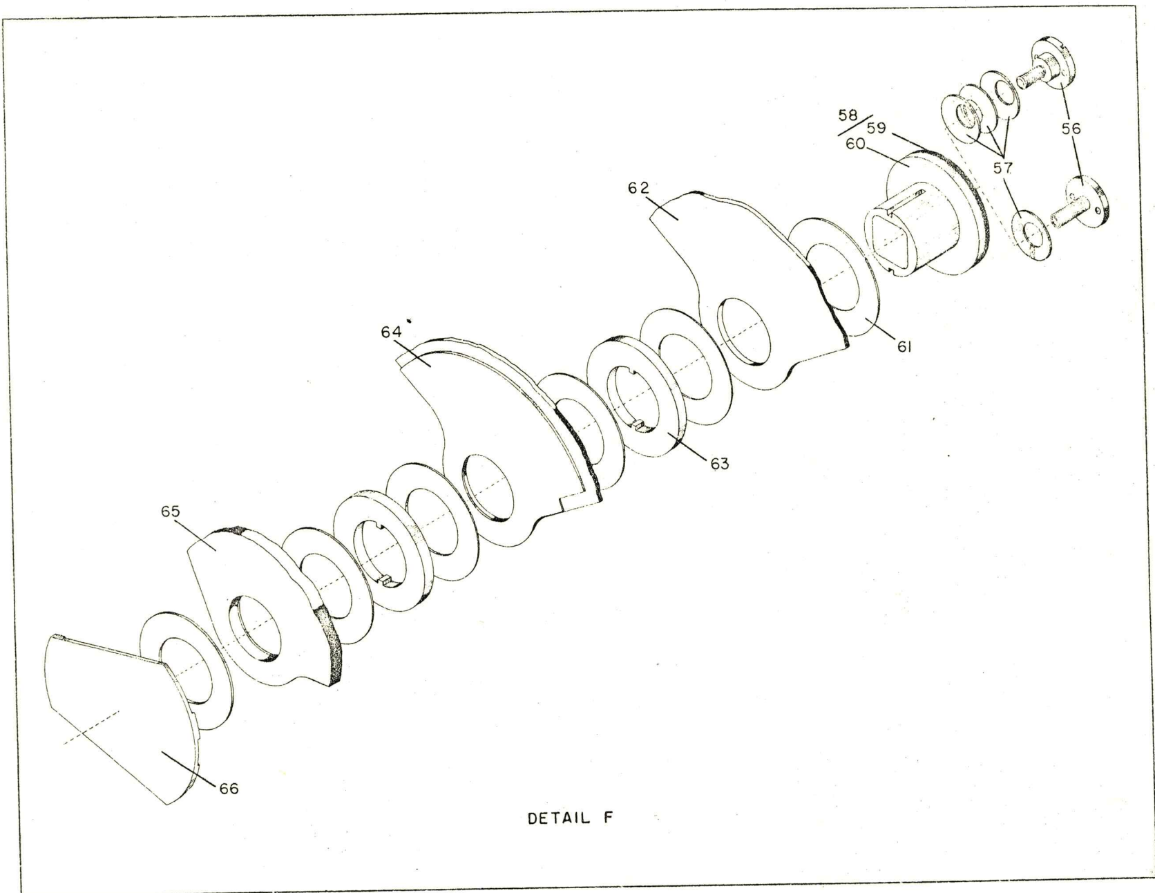
Figure 46 (Sheet 5 of 5) Skylab Extravehicular Visor Assembly
