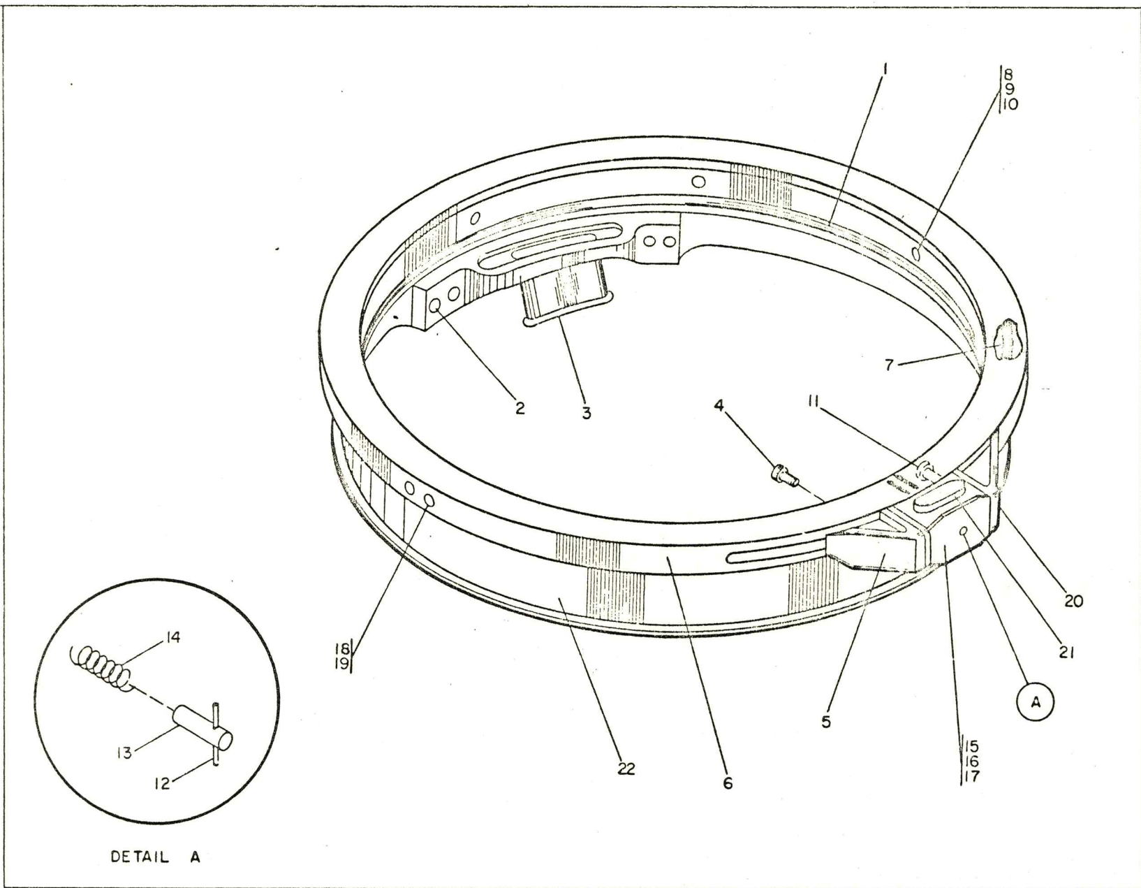
Figure 32 Neck Ring Assembly, PGA
