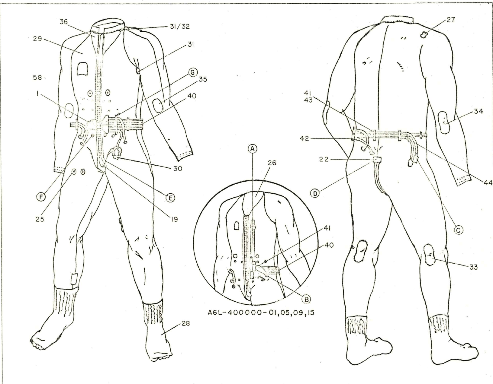
Figure 43 (Sheet 1 of 2) Liquid Cooling Garment Assembly
