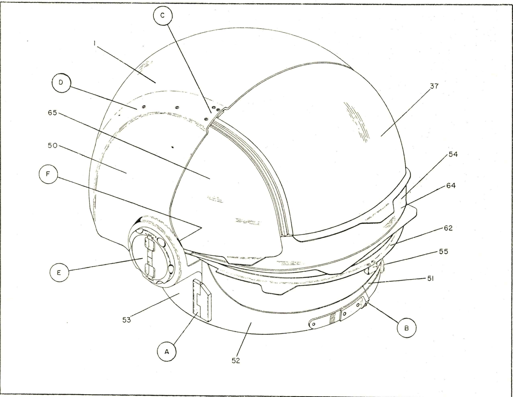
Figure 46 (Sheet 1 of 5) Skylab Extravehicular Visor Assembly
