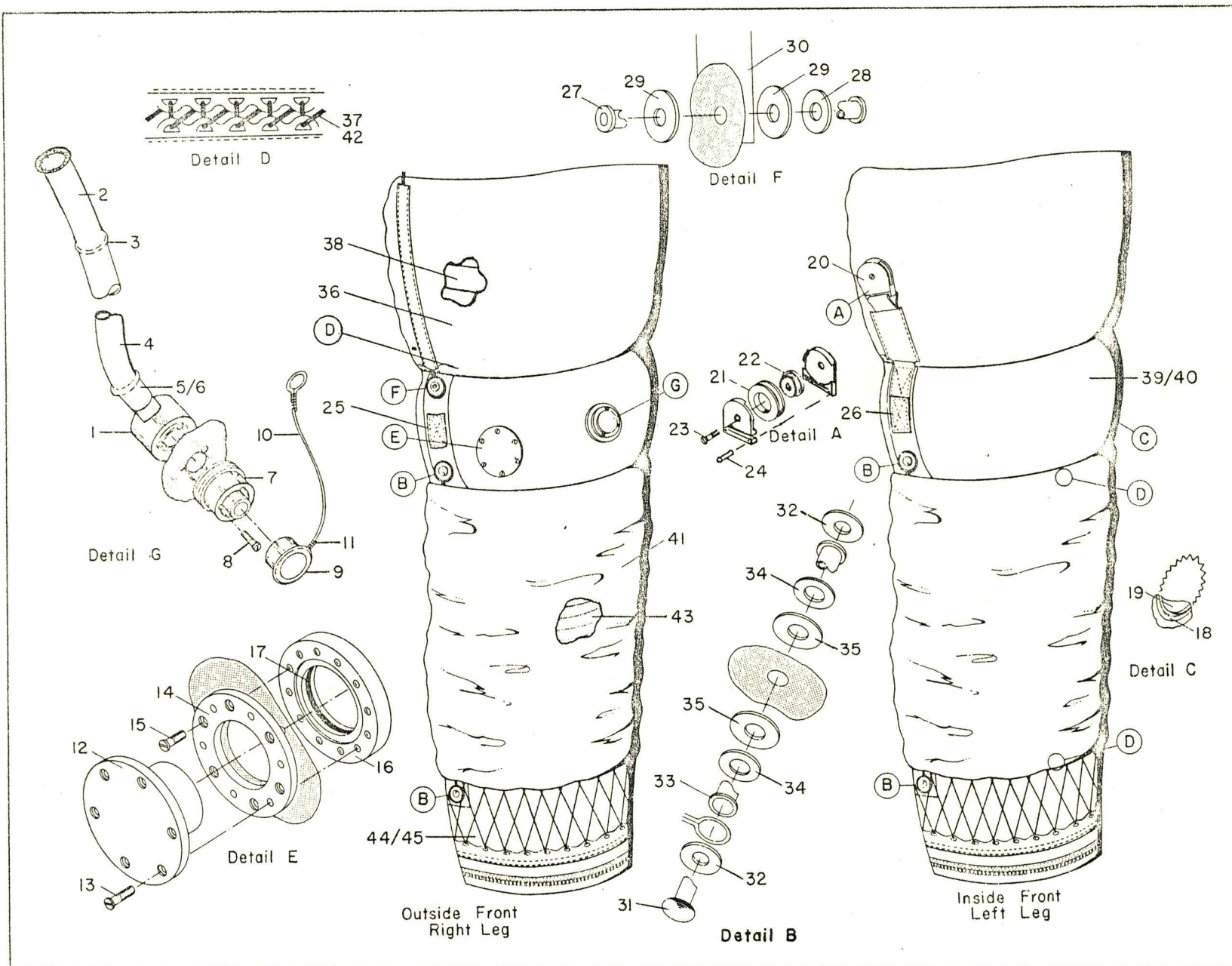
Figure 8 EV TUSA Leg Assembly
