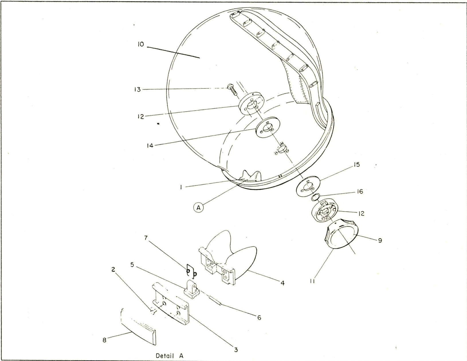
Figure 21 Pressure Helmet Assembly
