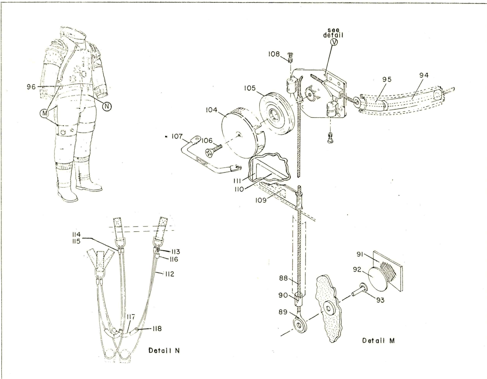
Figure 3 (Sheet 4 of 6) A7LB EV Torso Limb Suit Assembly
