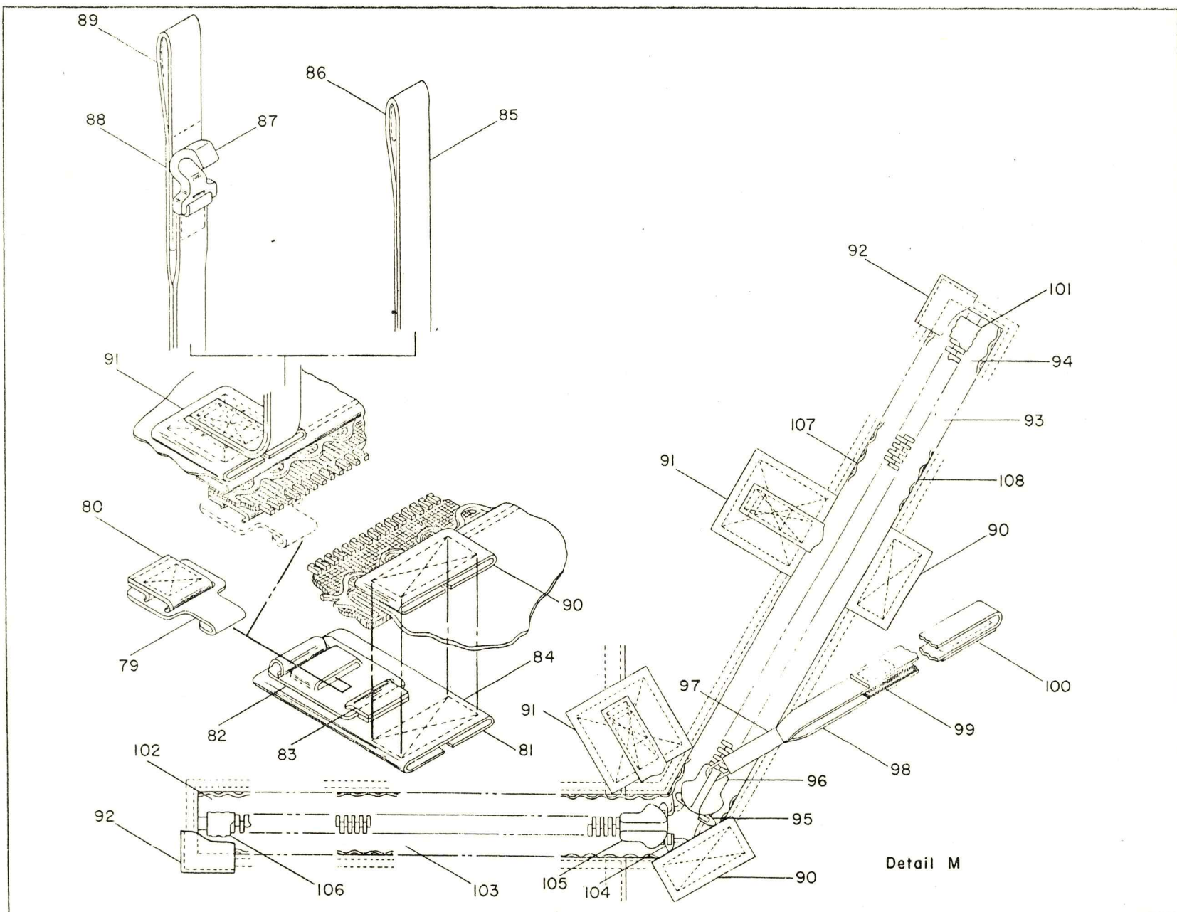
Figure 5 (Sheet 3 of 3) EV TL5A Torso Assembly
