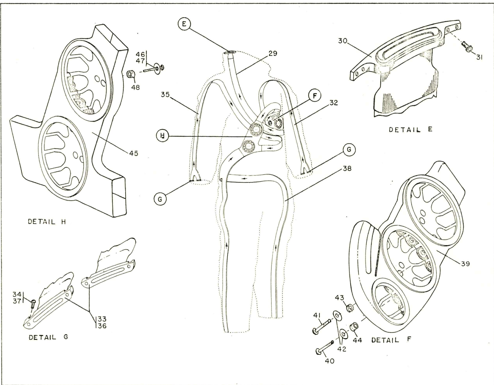
Figure 3 (Sheet 2 of 6) A7LB EV Torso Limb Suit Assembly
