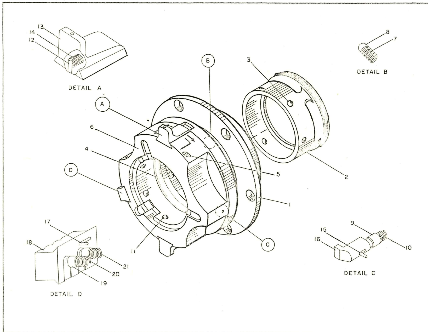
Figure 10 Outer Gas Connector Housing
