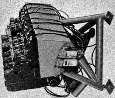
PROJECTOR ASSEMBLY, UNIT 6 PHO - OAI552 (TYPICAL)
