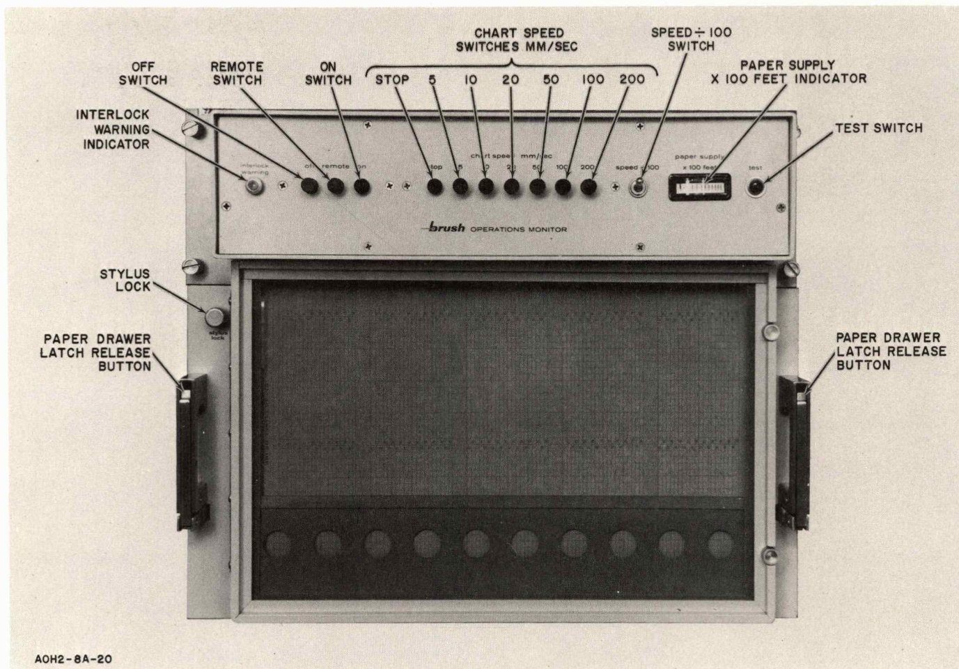
Figure 3-17. 100-Channel Event Recorder
