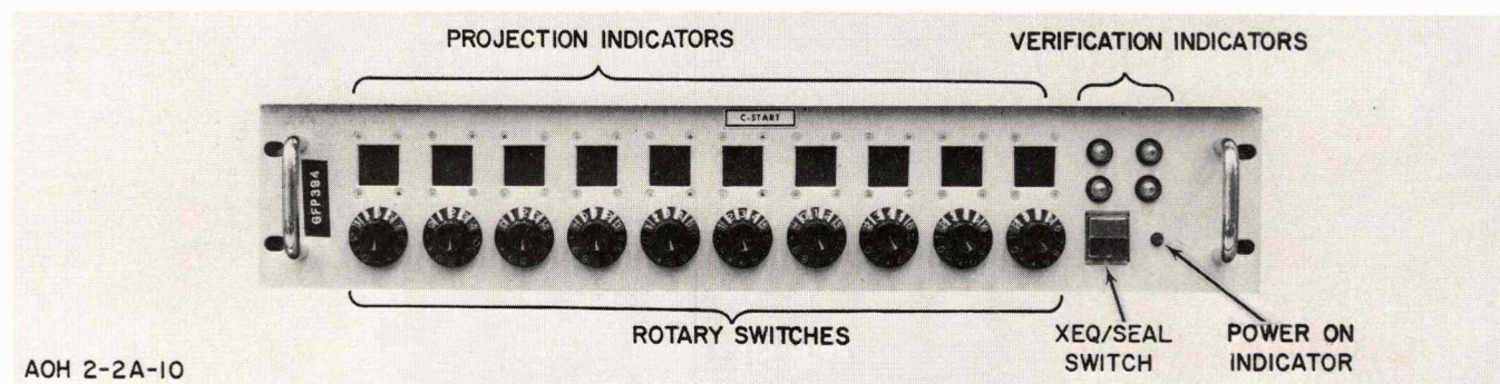
Figure 3-3. C START Panel
