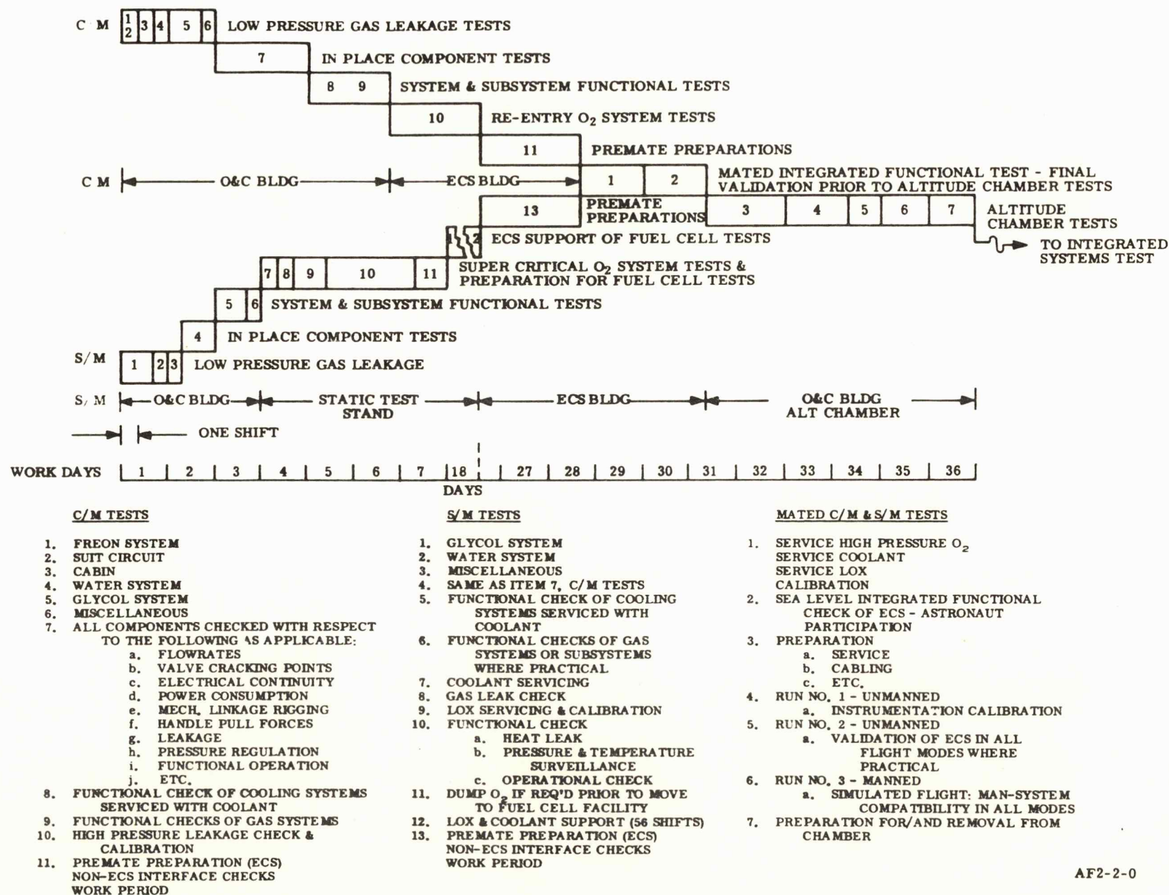
Figure 2-2. Spacecraft Environmental Control System (ECS) Checkout Cycle at MILA
