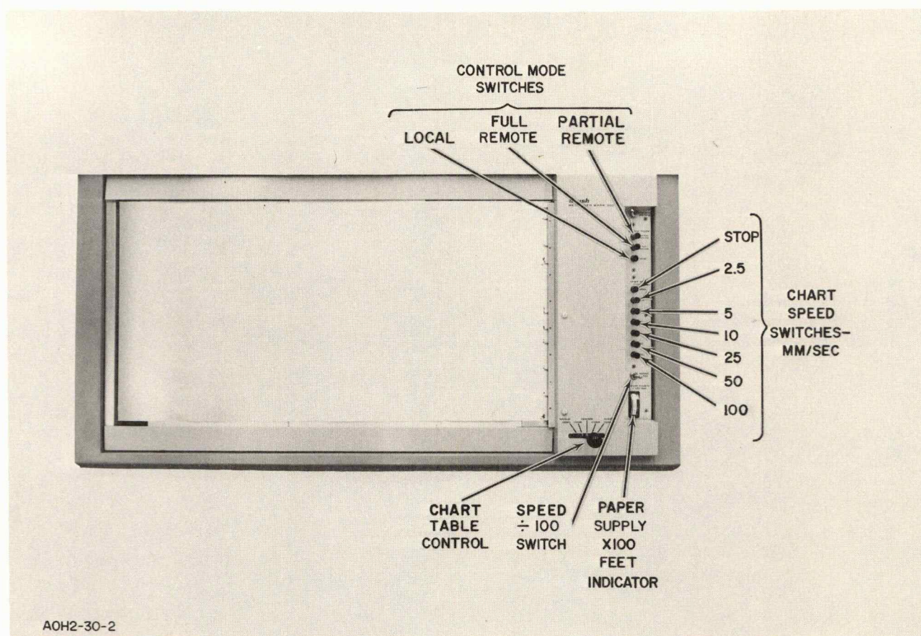
Figure 3-13. 8-Channel Horizontal Analog Recorder
