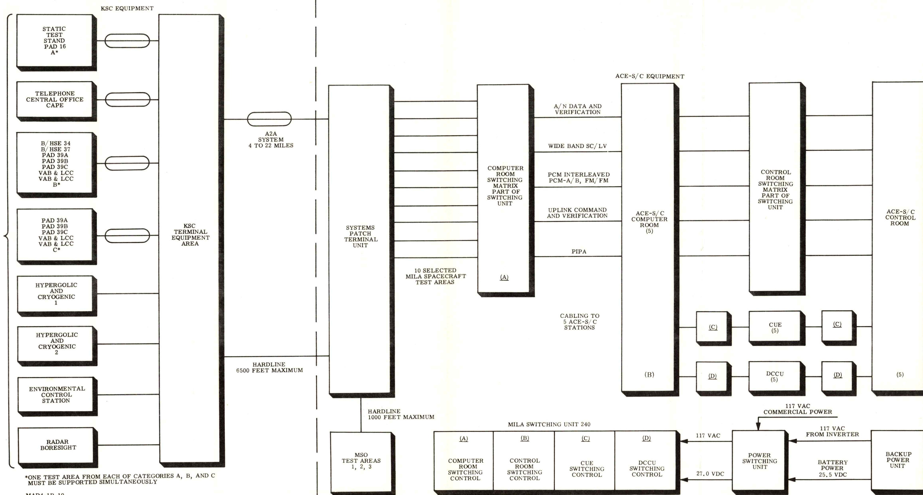
Figure 1-2. ACE-S/C MILA Switching Equipment Block Diagram
