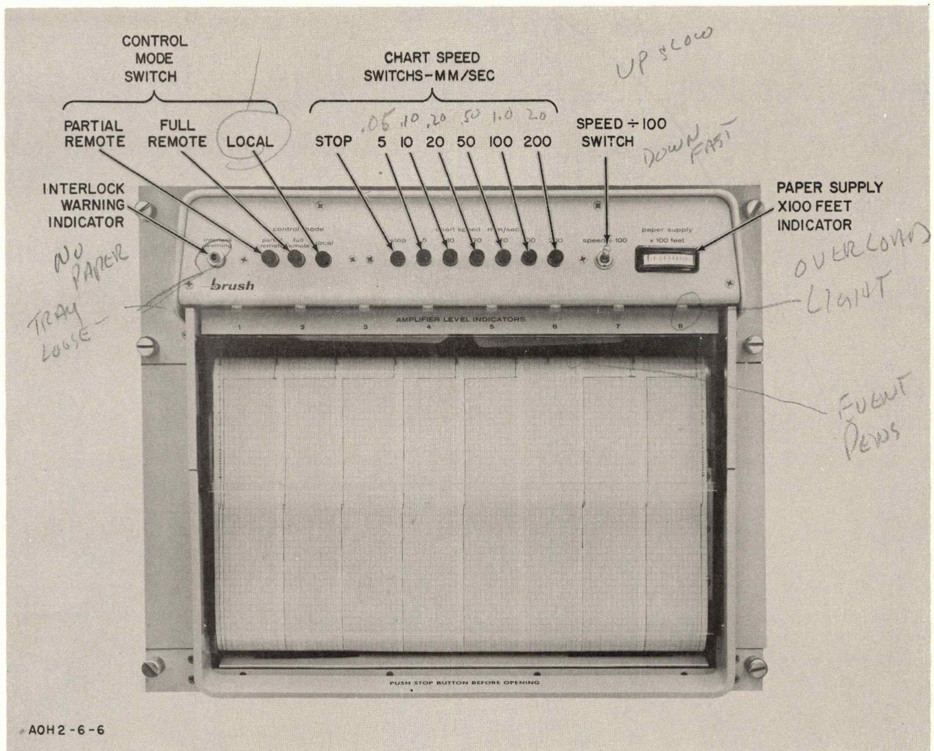
Figure 3-9. Eight-Channel Analog Recorder
