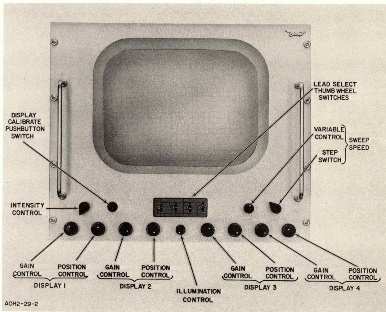
Figure 3-14. Cardioscope Display
