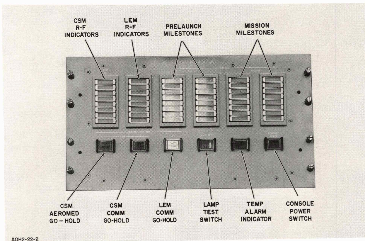
Figure 3-33. Astronaut Communicator Display Panel
