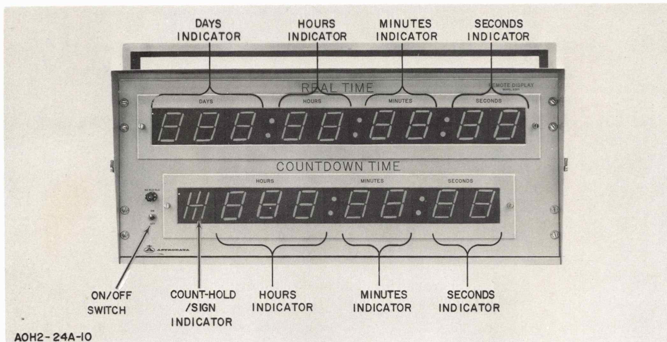
Figure 3-25. Wall Clock Display Unit
