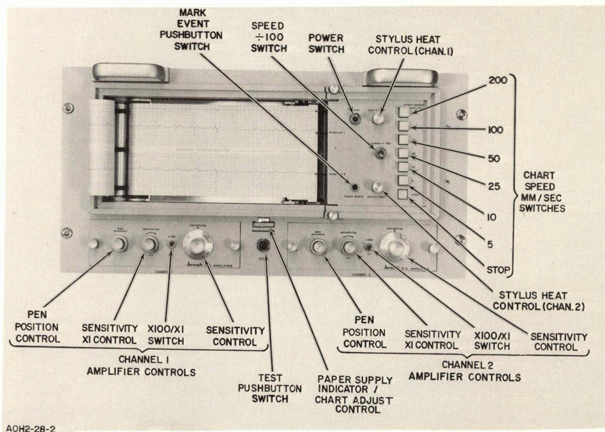
Figure 3-29. Two-Channel Cardiograph Recorder
