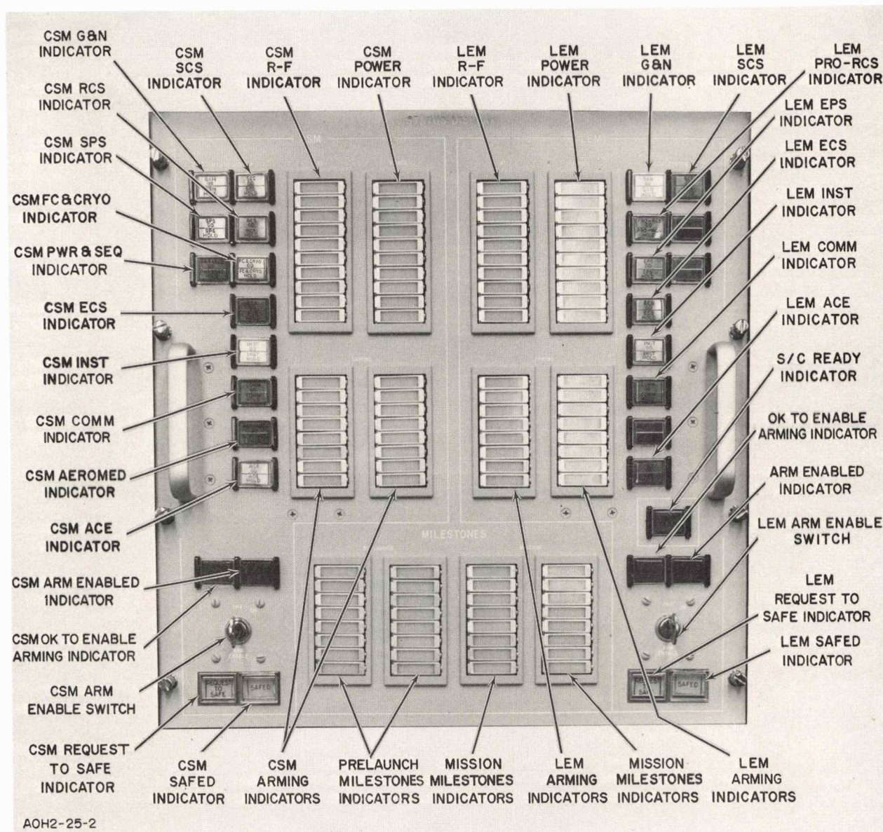
Figure 3-28. Test Conductor Status Display Panel (MILA Peripheral)
