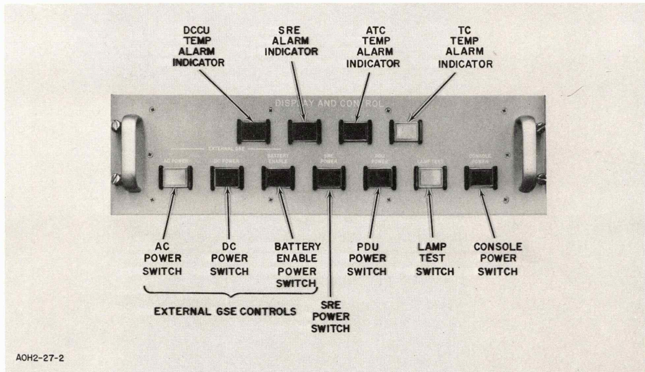
Figure 3-32. Power Status and Control Panel
