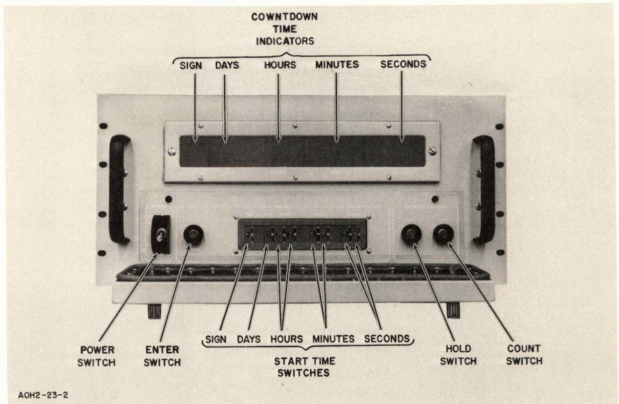
Figure 3-31. Independent Clock
