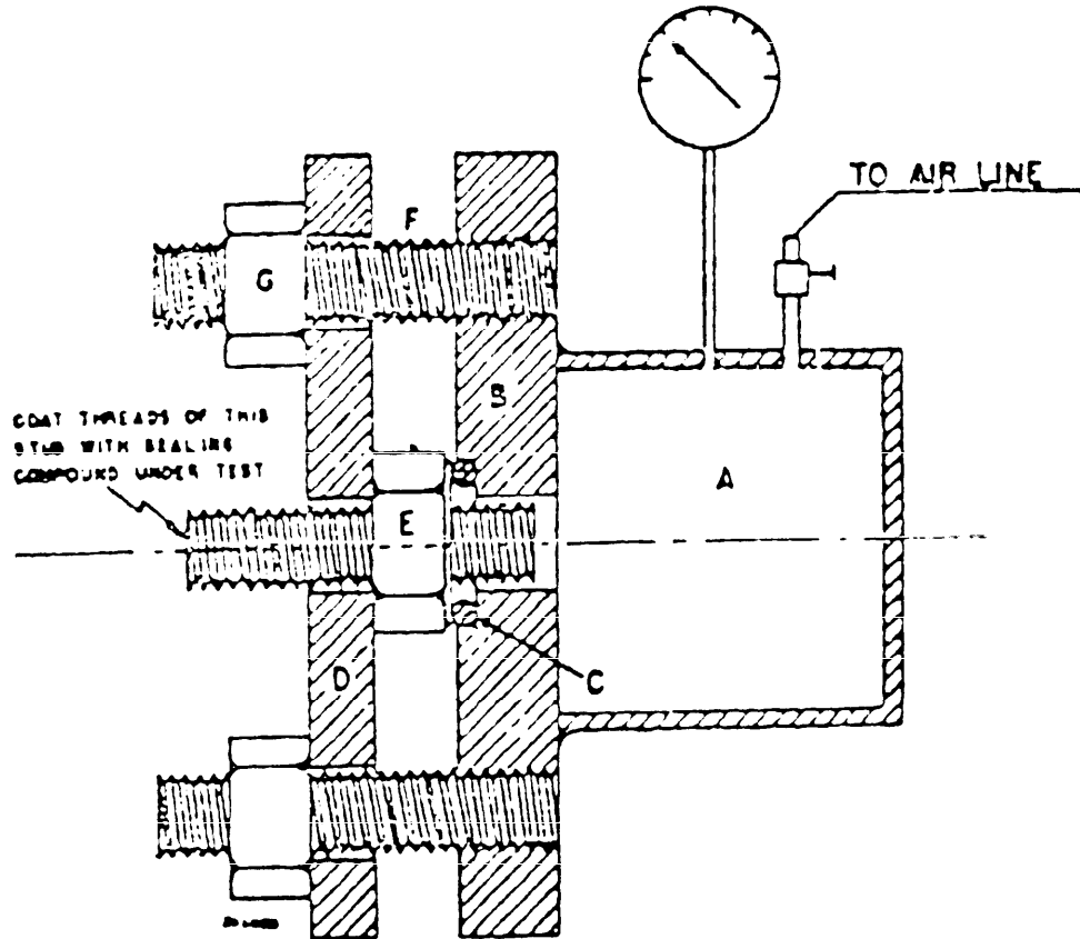
FIGURE 1. Fluid tightness test jig.
