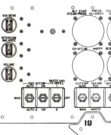
PANEL 108 CLOCK AND TIMER PANEL, FORWARD LEFT HAND EQUIPMENT BAY
