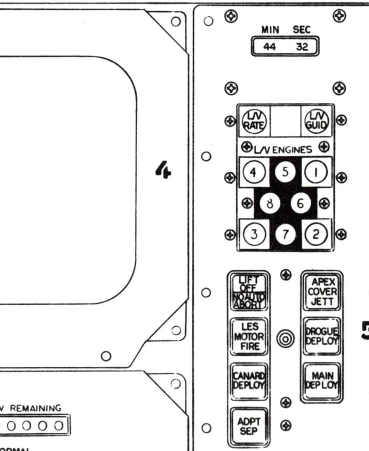
PANEL 105 CLOCK AND TIMER PANEL, FORWARD LEFT HAND EQUIPMENT BAY
