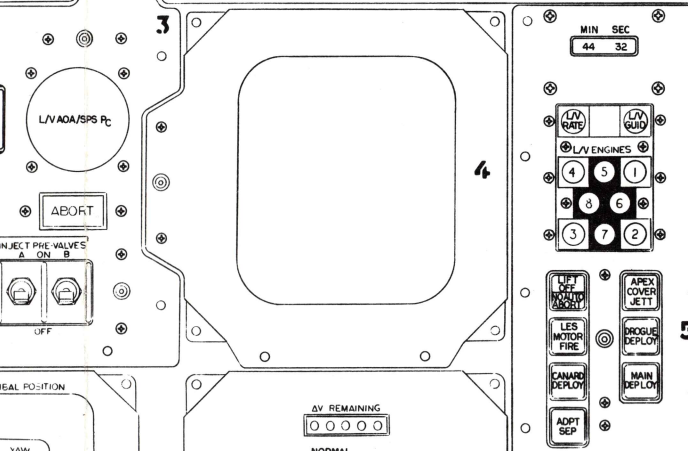
PANEL 104 CLOCK AND TIMER PANEL, FORWARD LEFT HAND EQUIPMENT BAY
