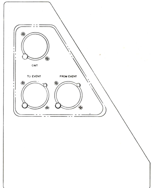
PANEL 100 CLOCK AND TIMER PANEL, FORWARD LEFT HAND EQUIPMENT BAY
