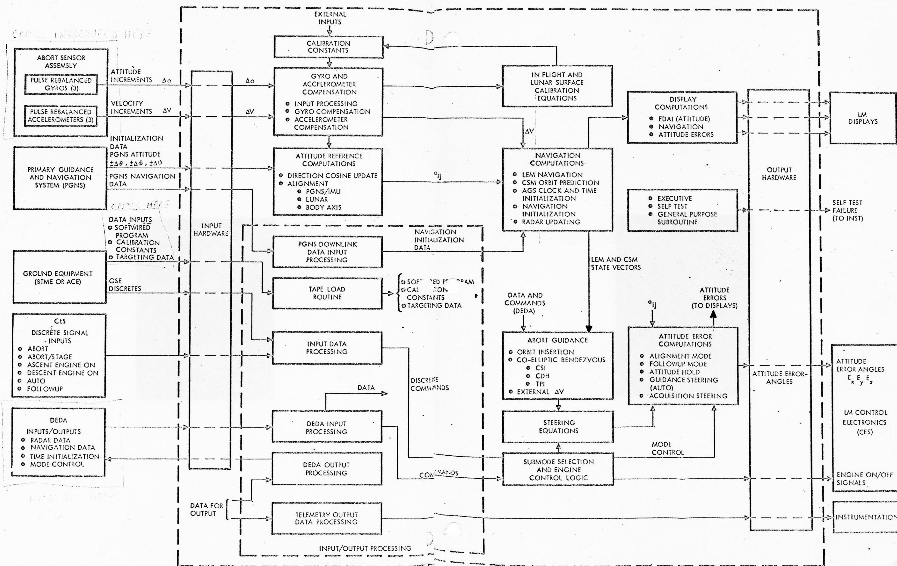
Figure 2.2 AGS Functional Block Diagram
