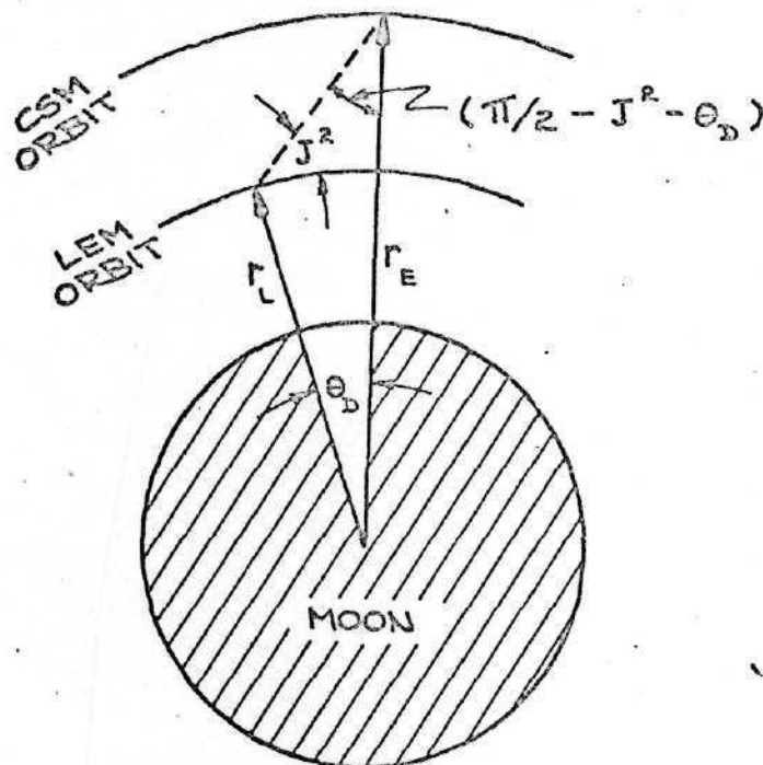
FIGURE 7.4 TPI GEOMETRY
