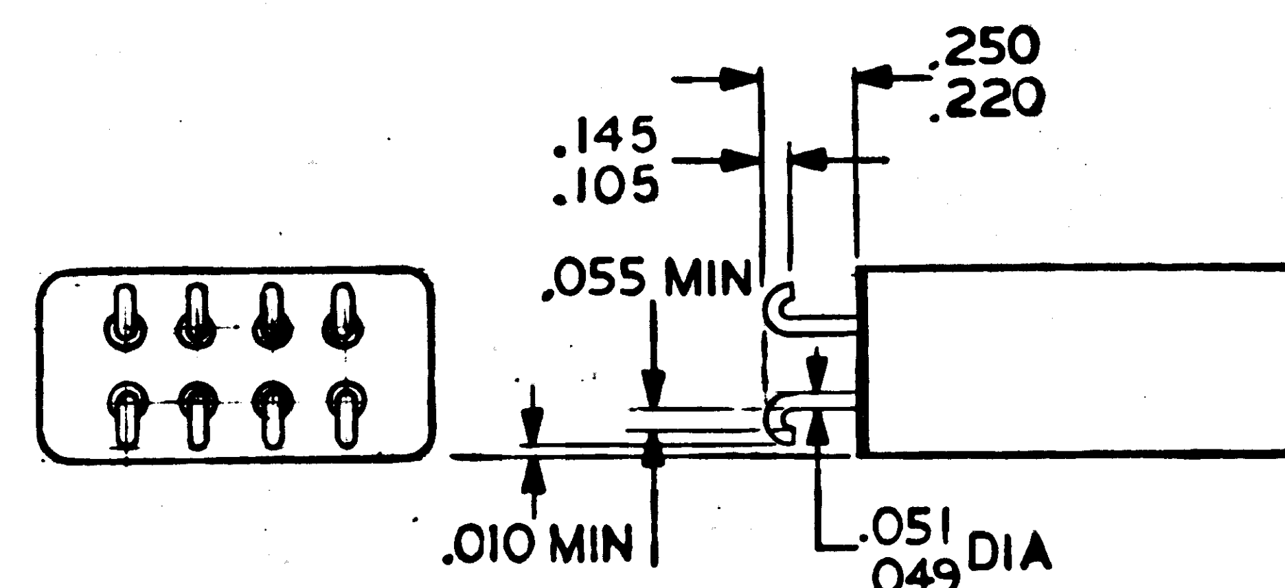
-002 LEAD CONFIGURATION
