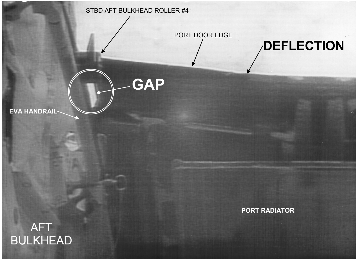
Figure 9-2.- Port aft centerline viewed by camera C.
