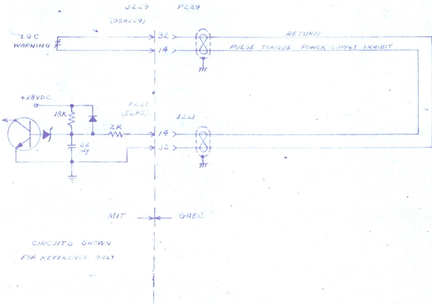
FIG. 45 PULSE TORQUE PWR SUPPLY INHIBIT
