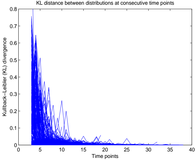
Figure 7: Relative Entropy (i.e. KL divergence) between tag frequency distributions at consecutive time-steps
