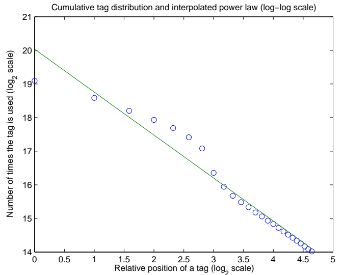
Figure 5: Cumulative number of tag usage frequency, based on their relative position. The plot is on a log-log scale: the horizontal axis shows the logarithm of the relative position, while the vertical axis shows the logarithm of the cumulative frequency of tags in that relative position. The best fit linear regression (using the least-squares method) is also shown.
