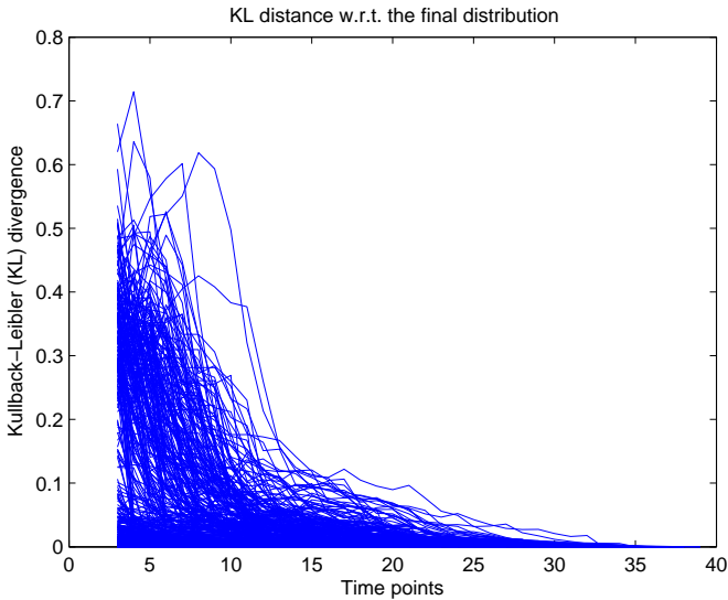
Figure 8: Relative Entropy (KL divergence) of tag frequency distribution at each time step, with respect to the final distribution
