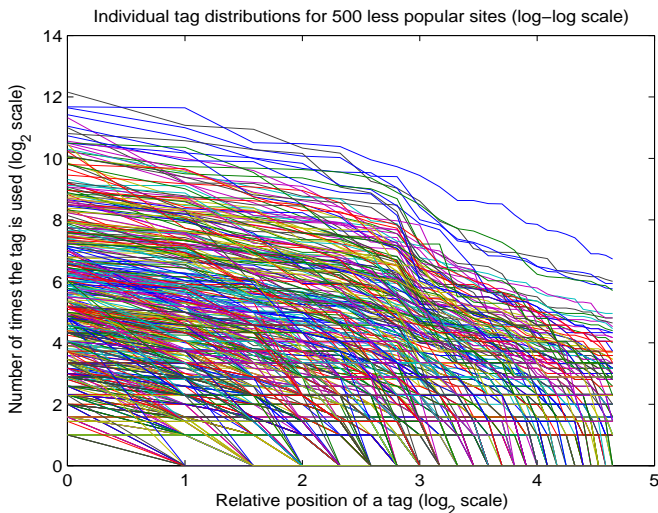
Figure 6: Frequency of tag usage based on relative position for a dataset consisting of 500 less-heavily tagged sites (with the 25 most frequently used tags considered for each).
