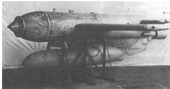
Illustration 17 (Hs 293)
