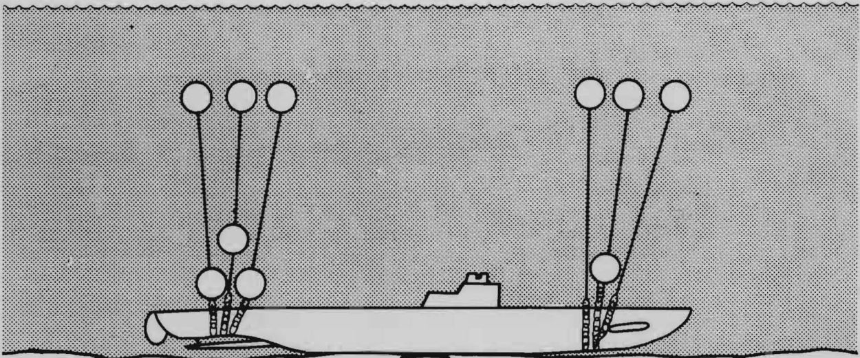
TEN-PONTOON ARRANGEMENT FOR SUCCESSFUL FIRST LIFT. FIGURE E-4
