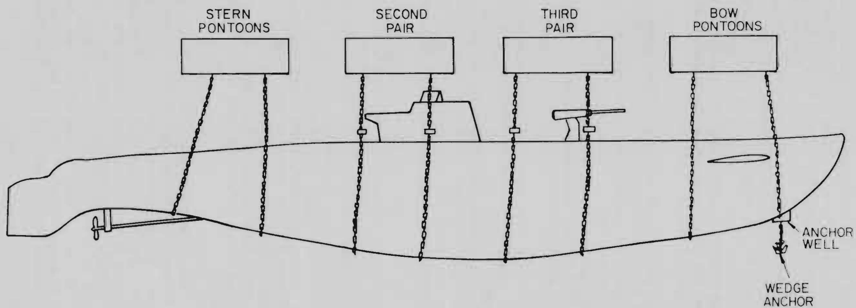
ARRANGEMENT OF PONTOONS AND SLINGS ON S-51 LIFT. FIGURE C-1
