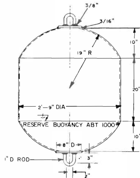
ROEBLING BUOY (18)
