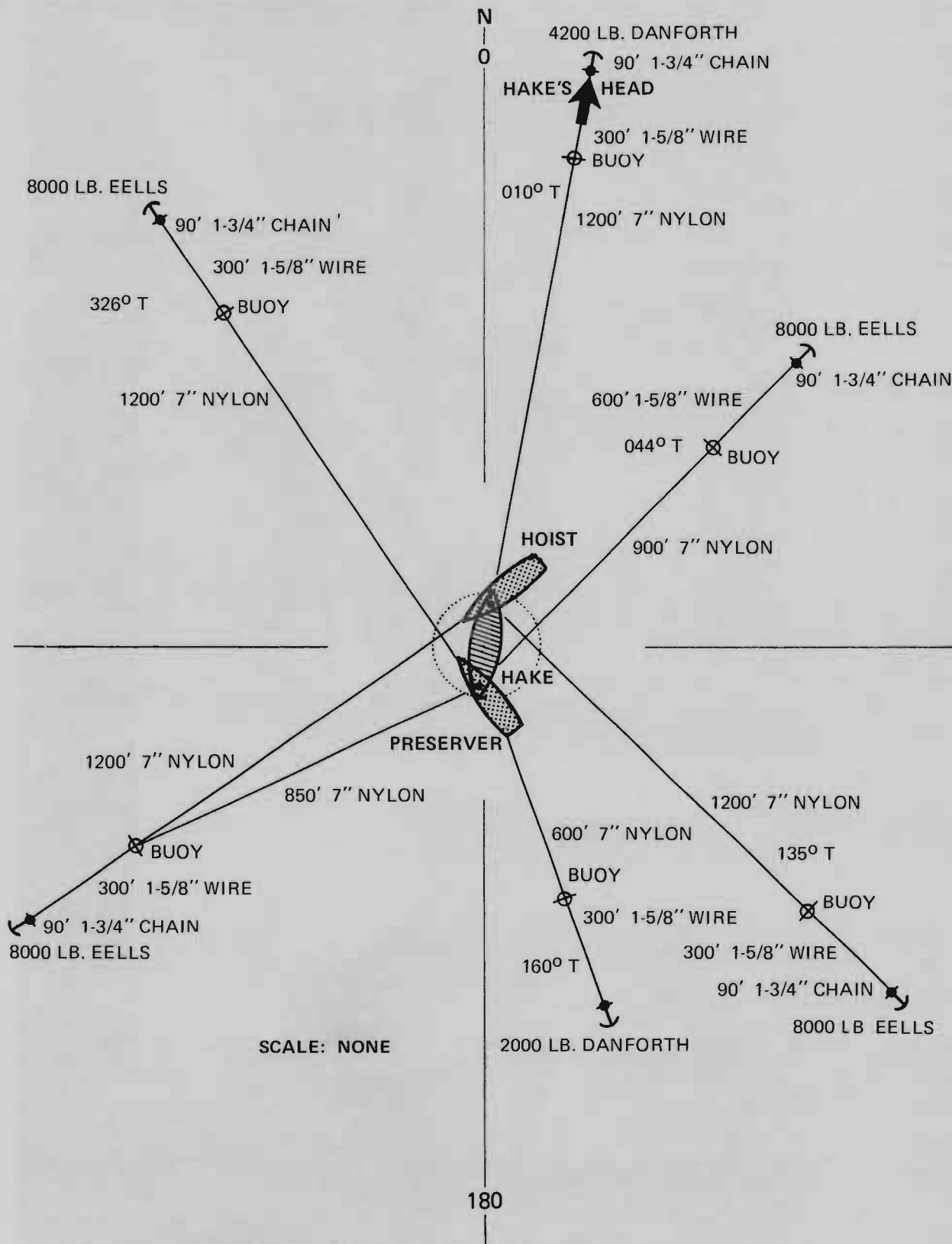
WORKING MOOR FOR THE FIRST LIFT. HOIST AND PRESERVER MOORED OVER EX-HAKE.
