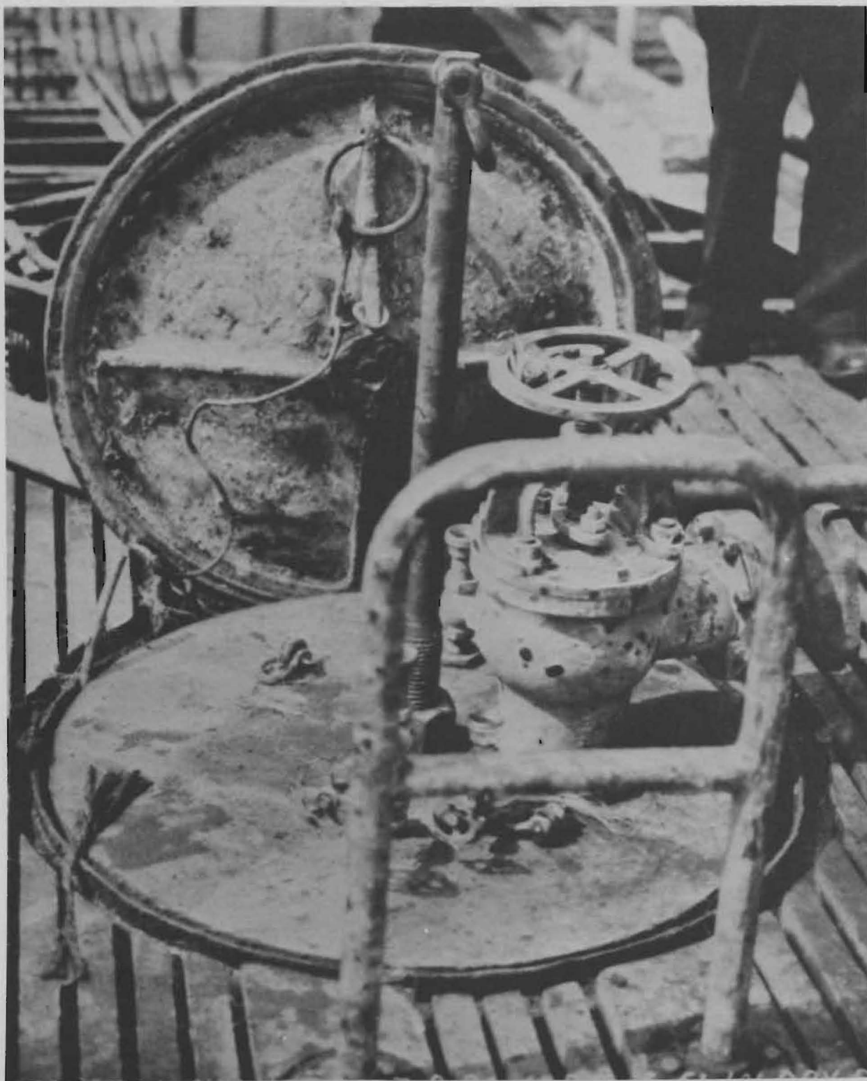
ENGINE ROOM SALVAGE HATCH IN POSITION, S-51. FIGURE C-5
