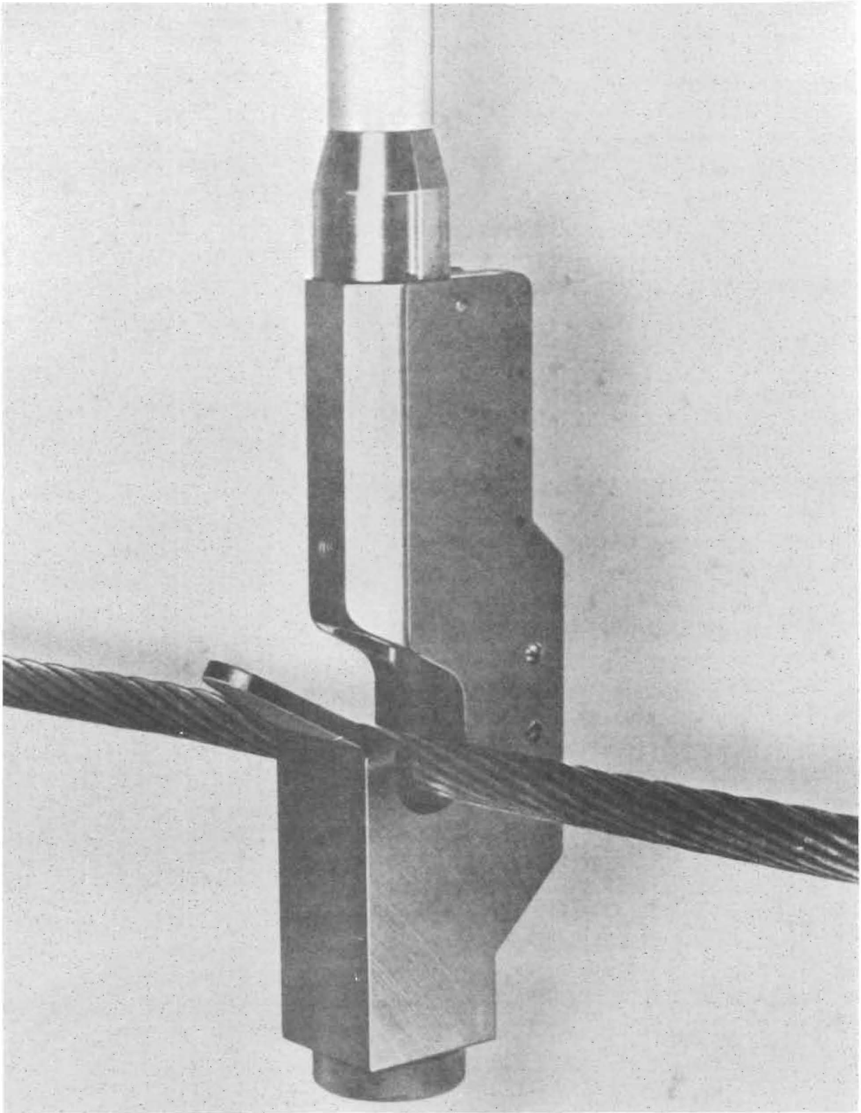
POLE C FRAME CABLE CUTTER. FIGURE 2-14
