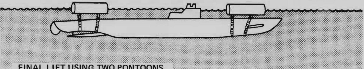
FINAL LIFT USING TWO PONTOONS AT BOW AND STERN. FIGURE E-6
