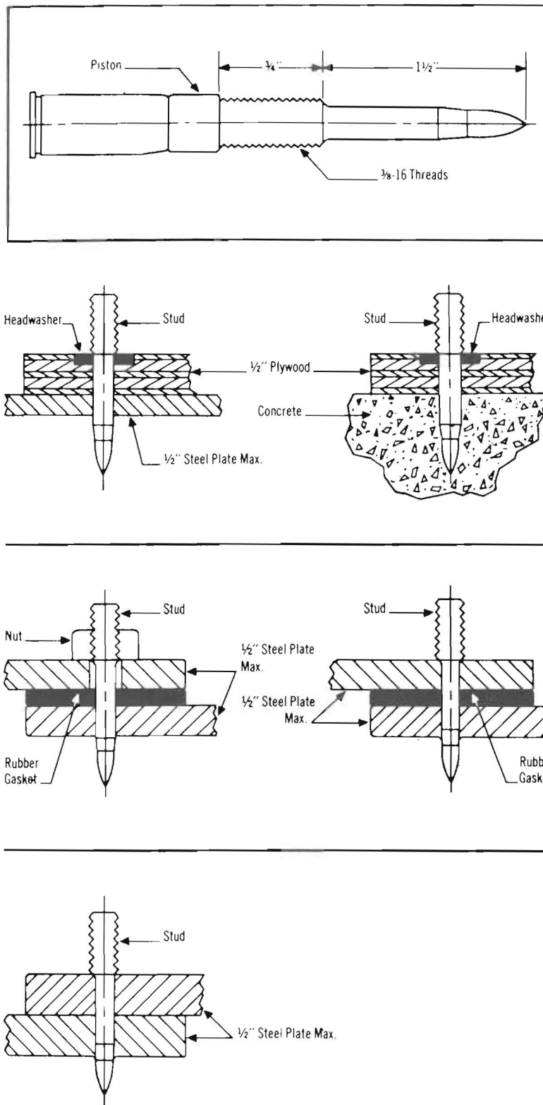
STUD CHART FOR NUD 38 DRIVER.
