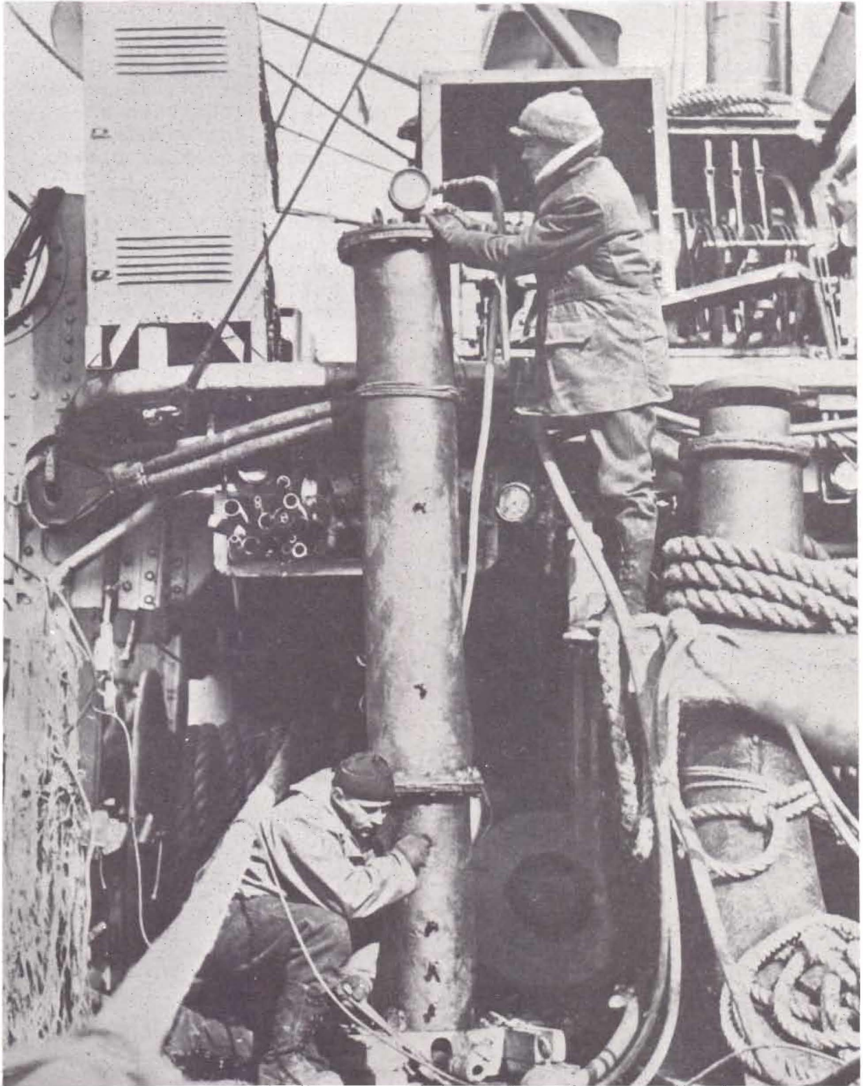
CEMENT GUN ON BOARD FALCON AS USED IN S-4 SALVAGE. FIGURE 2-28
