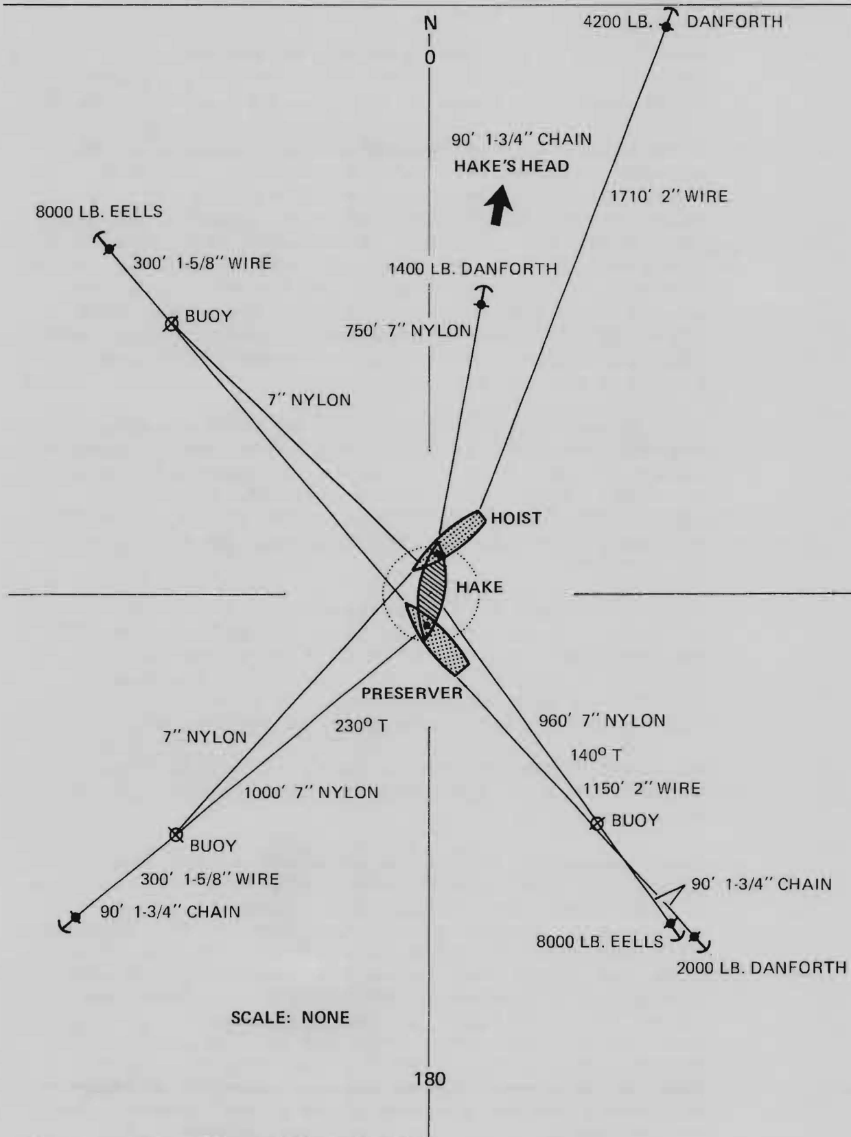
HOIST AND PRESERVER IN THE SECOND LIFT WORKING MOOR.
