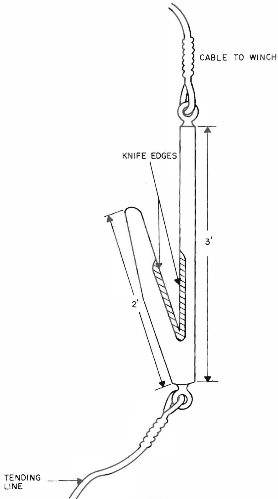
HOOK CUTTER 1/2-INCH STEEL STOCK. FIGURE 2-13
