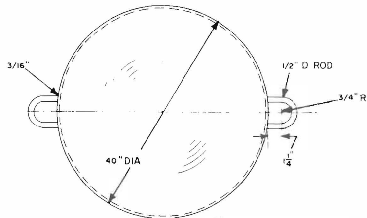
SPHERICAL BUOY (20)
