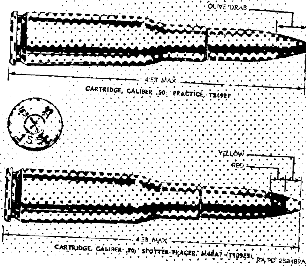
Figure 17. Cartridges for caliber .50 spotting rifle M27.
