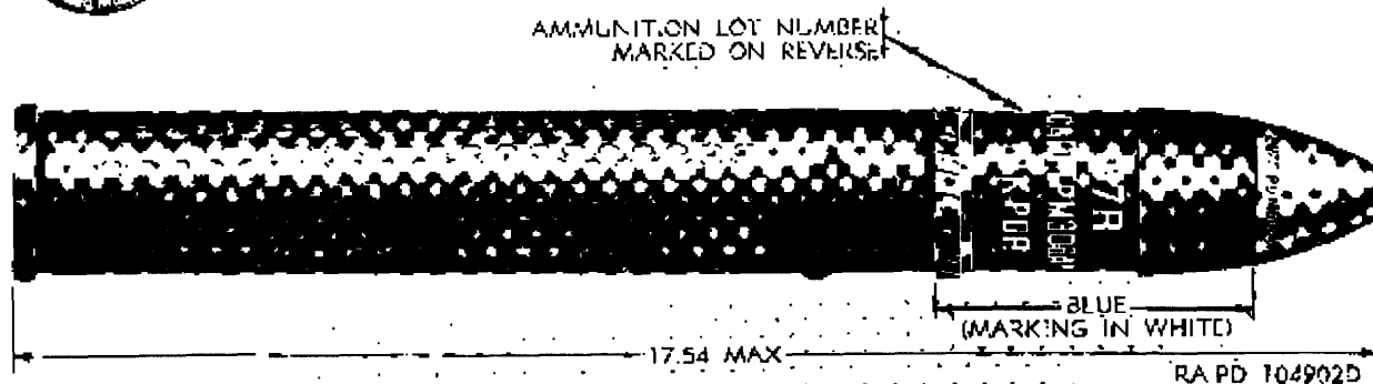
Figure 8. Cartridge, 57 millimeter: TP, MS06A1, w/face, PD, M503 or M503A1.
