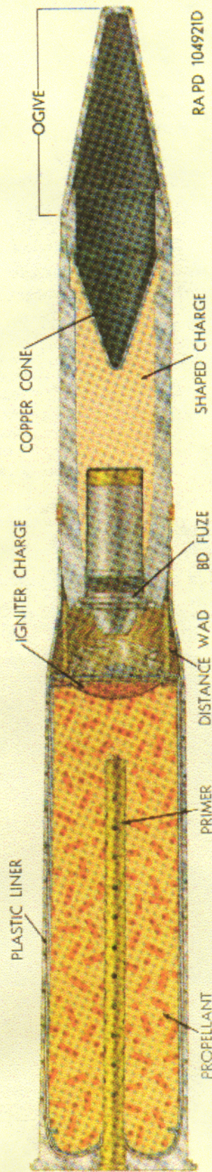
Figure 10. Cartridge, 75 millimeter: HE, AT-T, M91A1, w/fuze, BD, M91A1.
