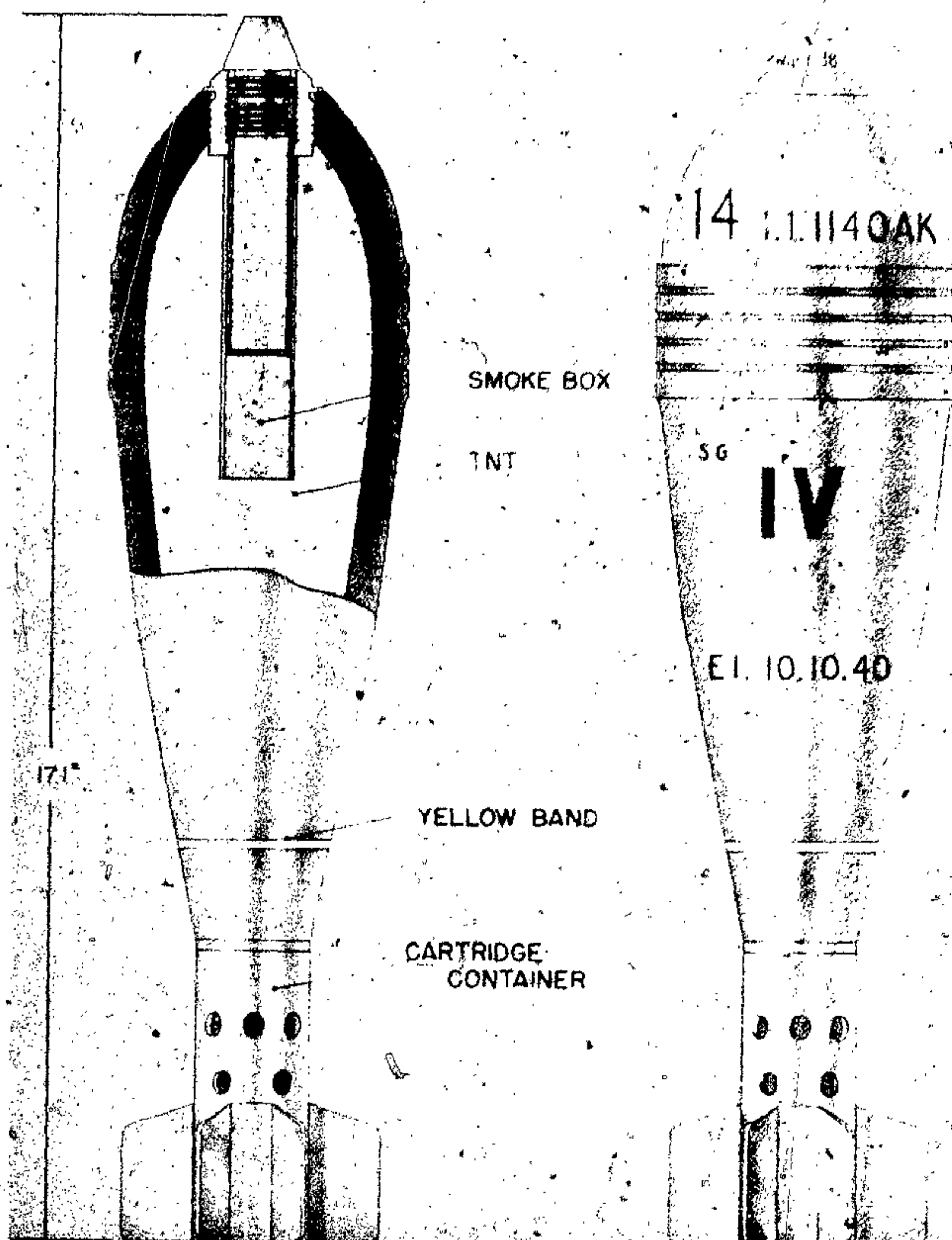
Figure 547—H. E. Mortar Projectile, 100-mm, 10-cm Wgr. 37
