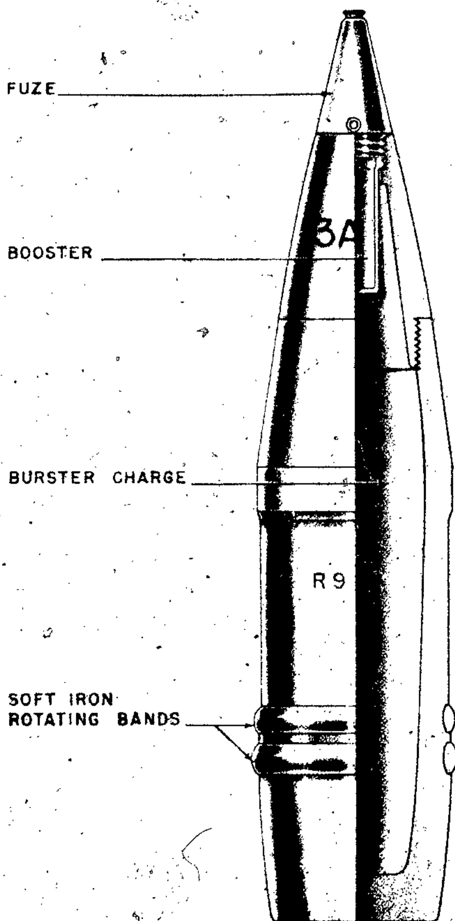
Figure 485—H. E. Projectile, 150-mm, 15-cm K. Gr. 42
