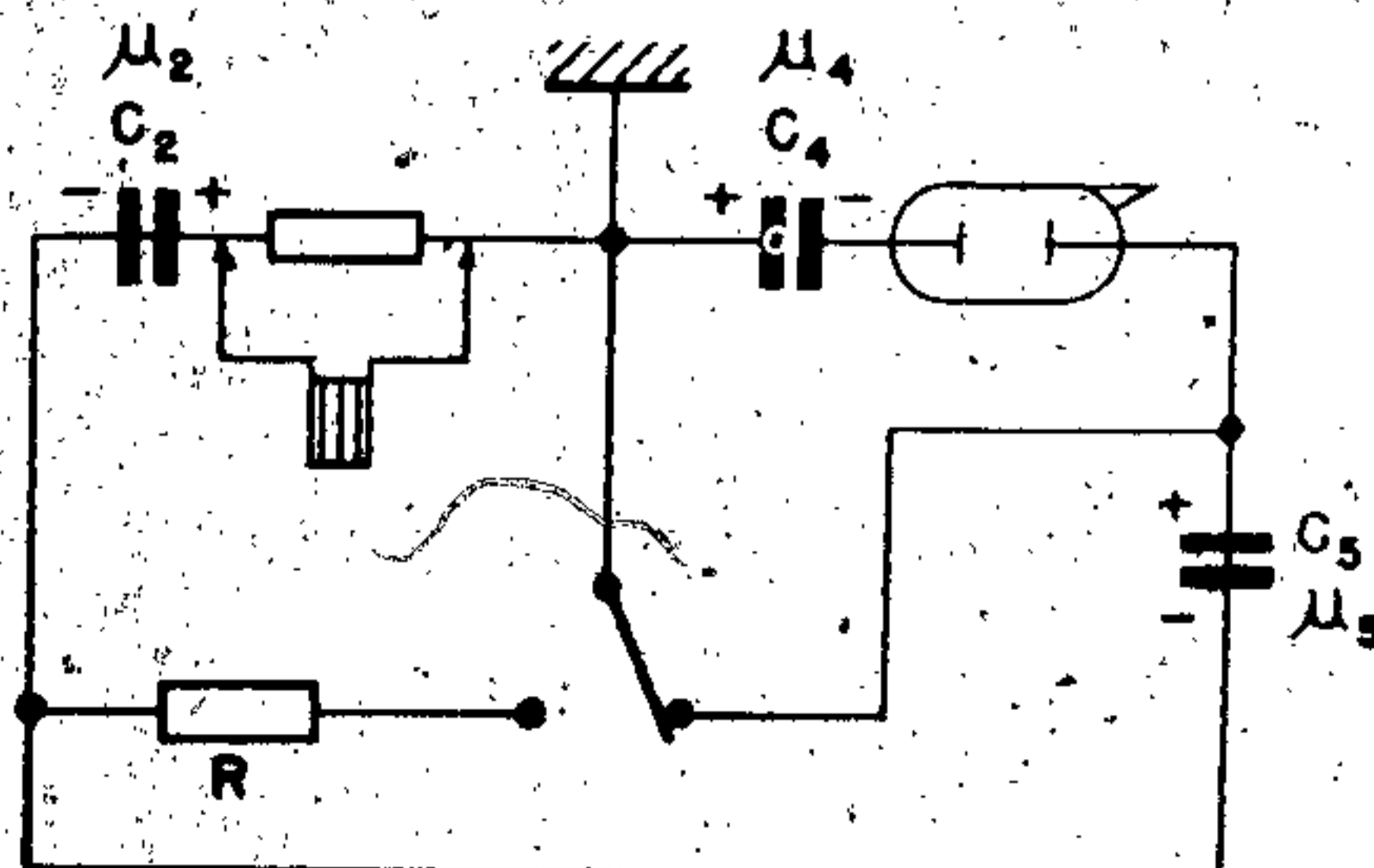
Figure 597B—Wiring Diagram
