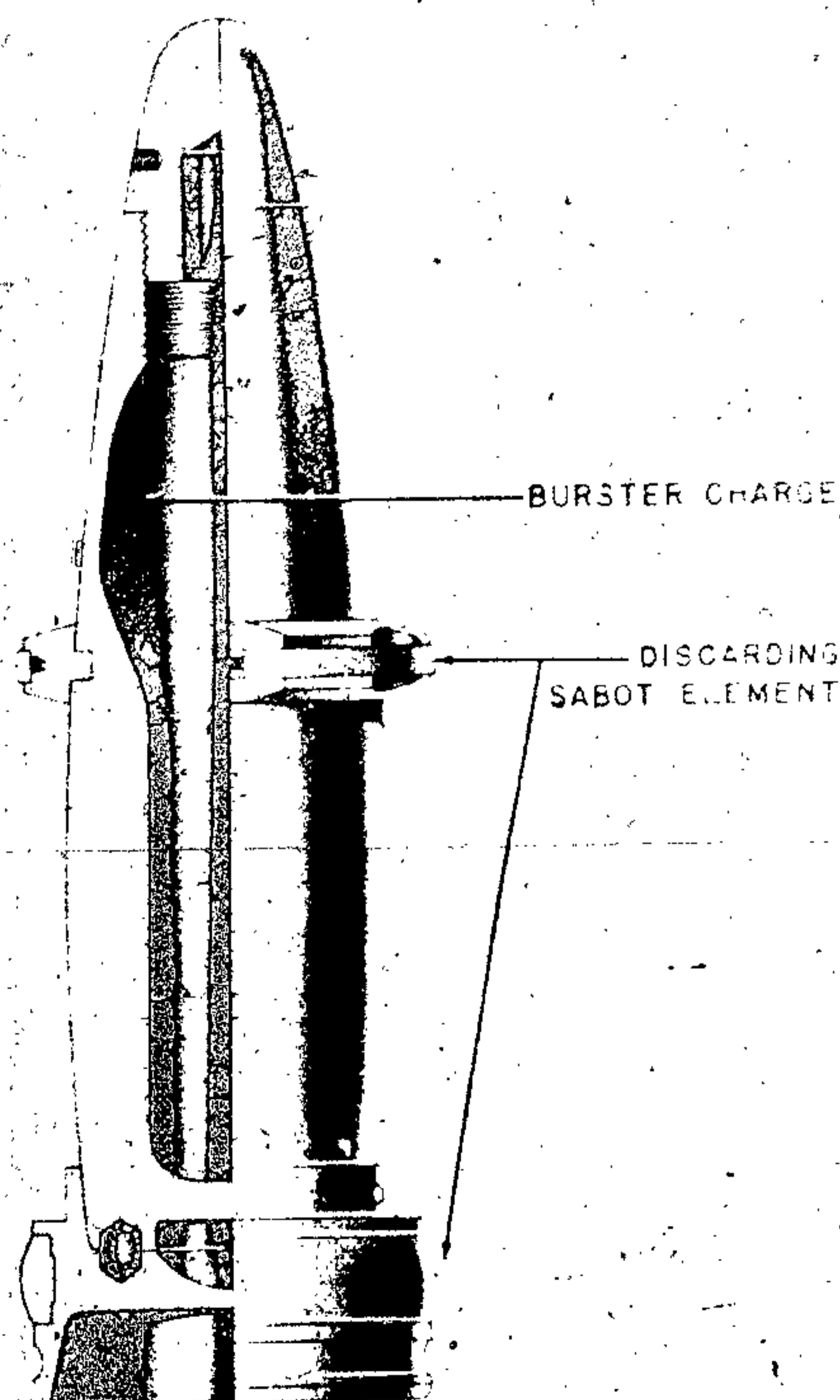
Figure 326A—Sabot Projectile Type A
