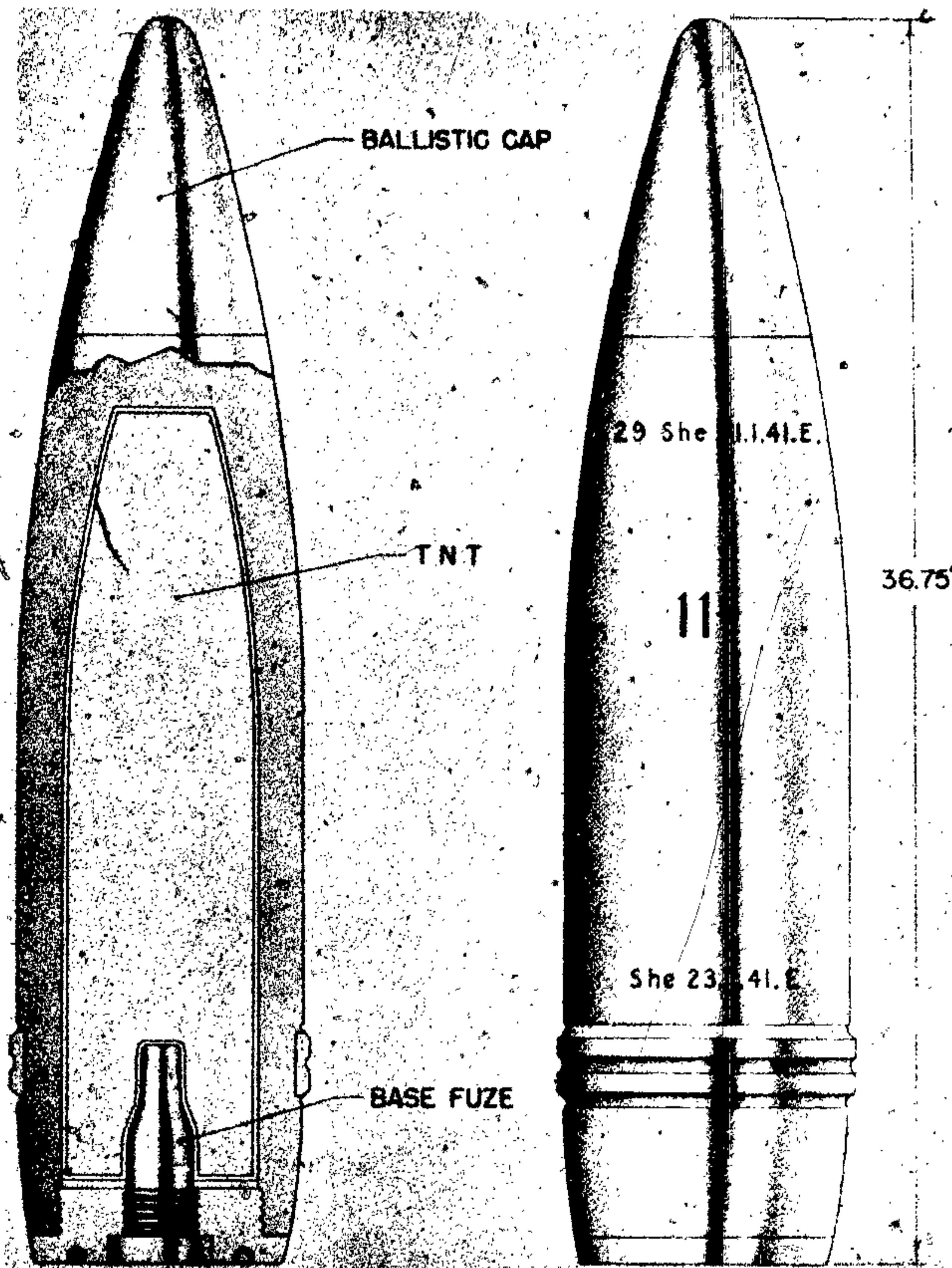
Figure 532—Anticoncrete Projectile, Type 18, 210-mm, 21-cm Gr. 18 Be.
