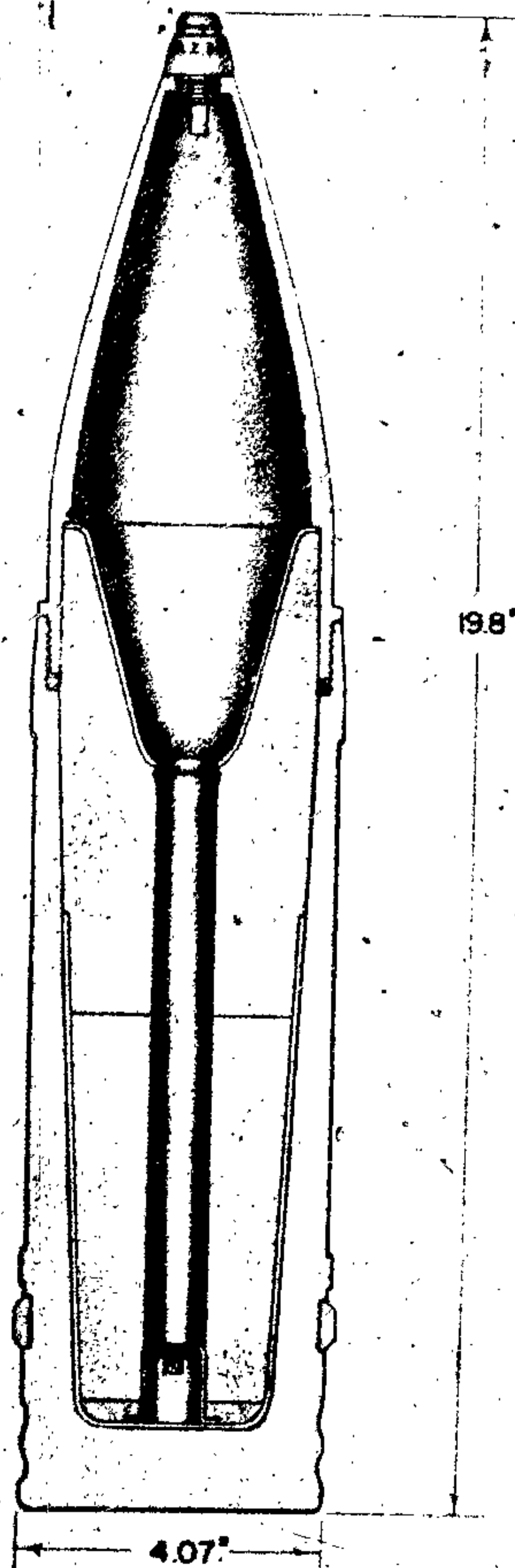
Figure 472—Hollow Charge Projectile, Type A, 105-mm, 10-cm Gr. 39 Rot HL/A
