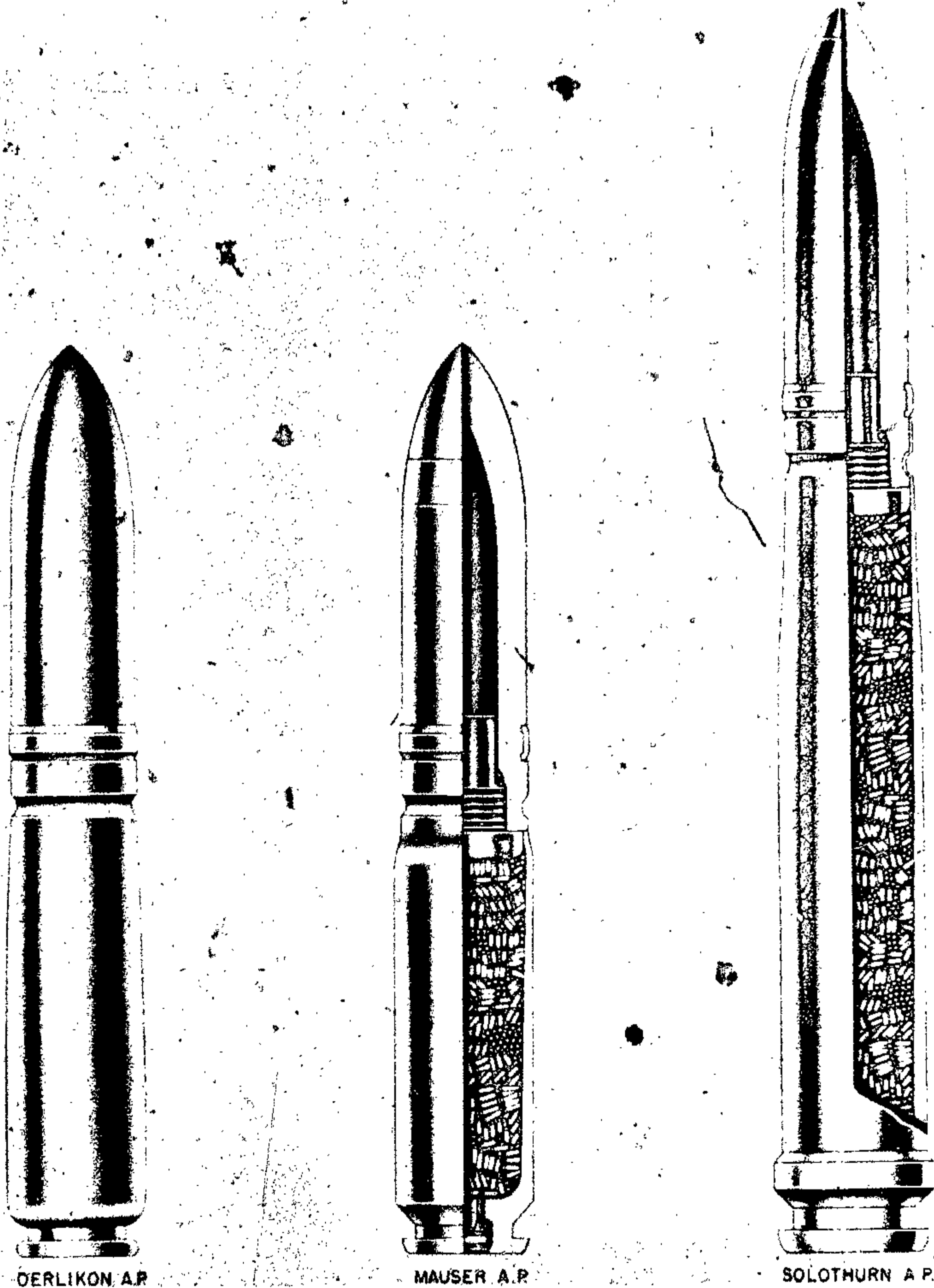
Figure 324A—20-mm Ammunition
