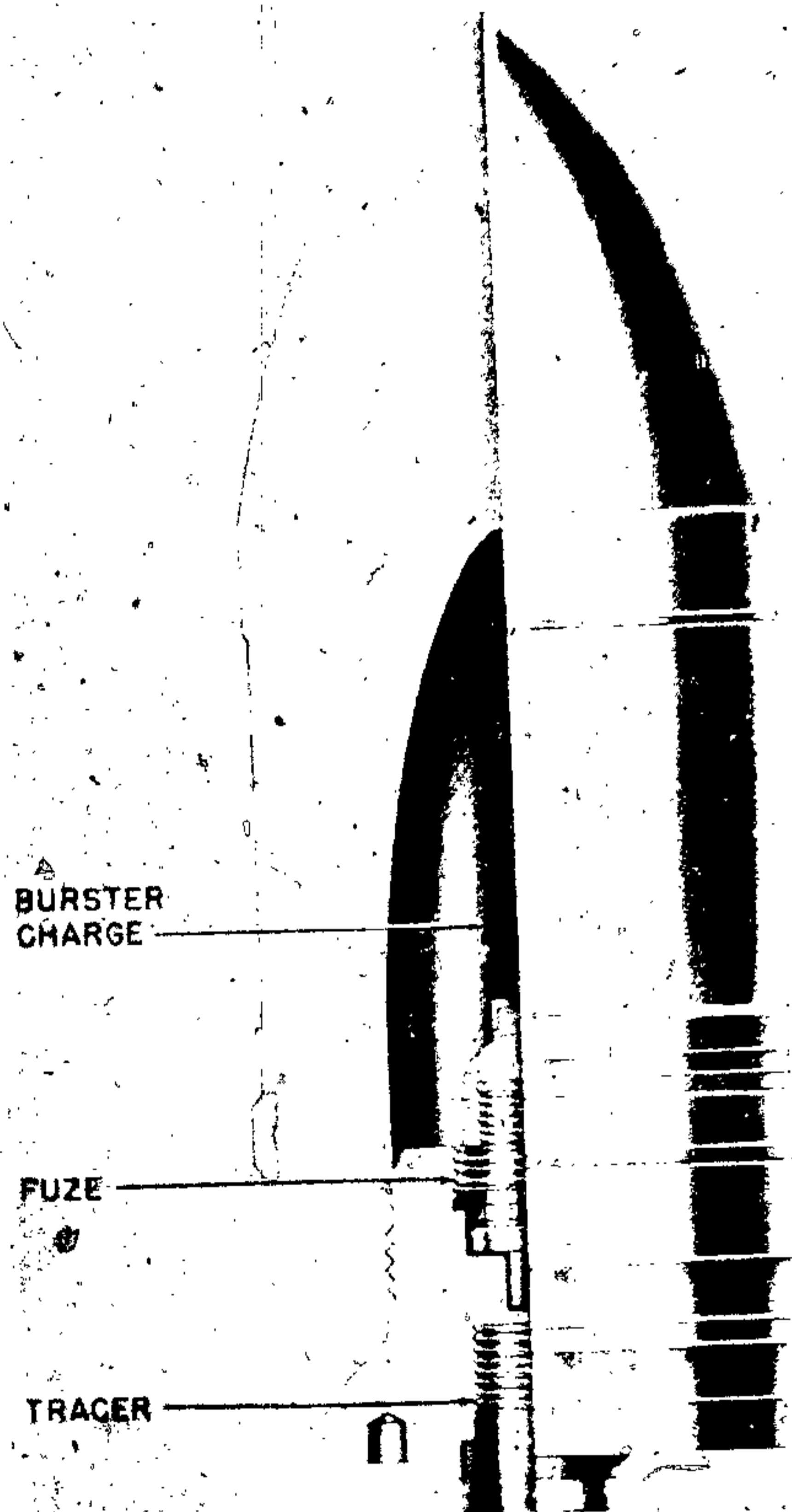
Figure 453—A. P. Projectile, 105-mm, 10-cm Pzgr. (f)
