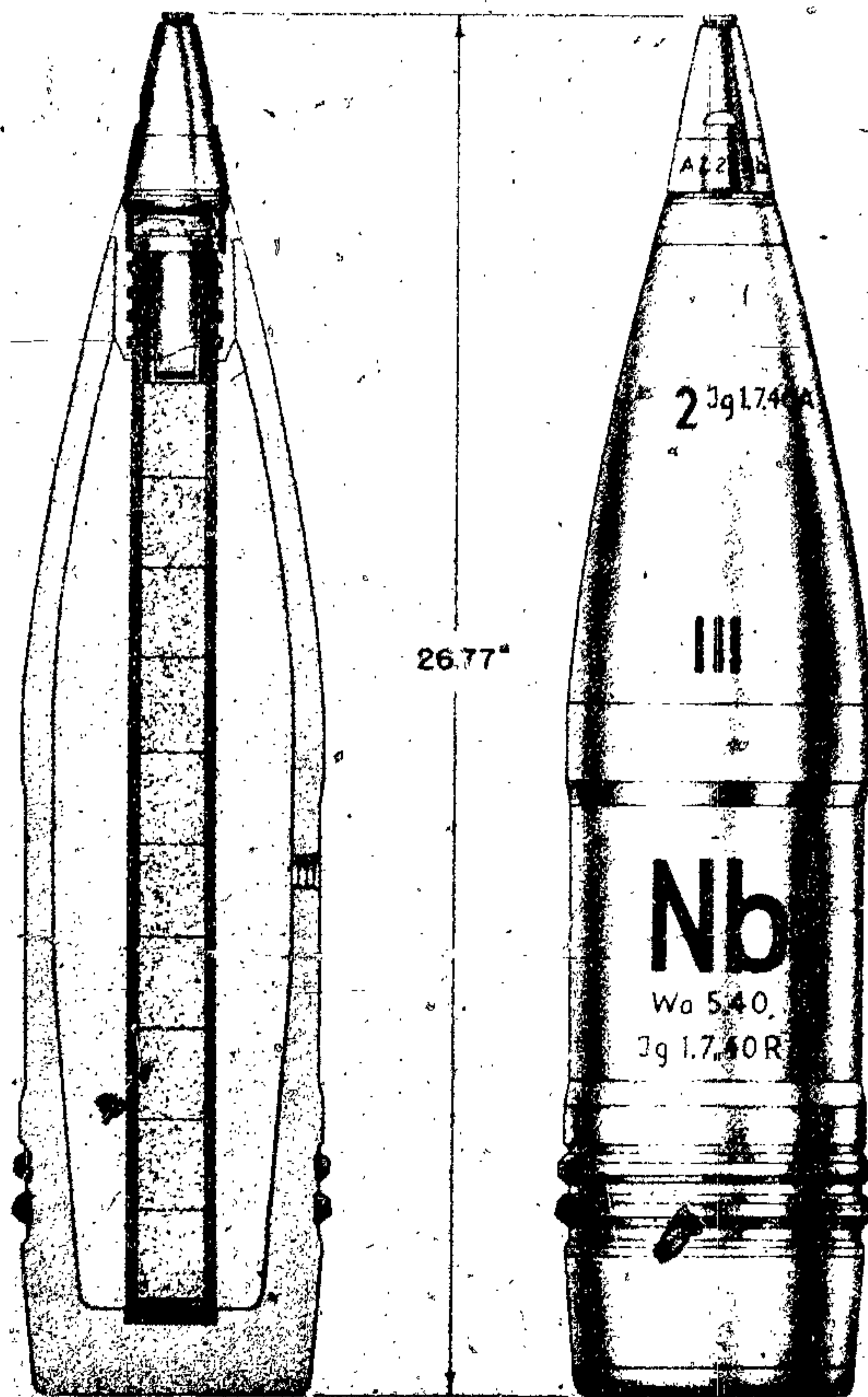
Figure 499—Smoke Projectile, Type 19, 150-mm, 15-cm Gr. 19 Nb.
