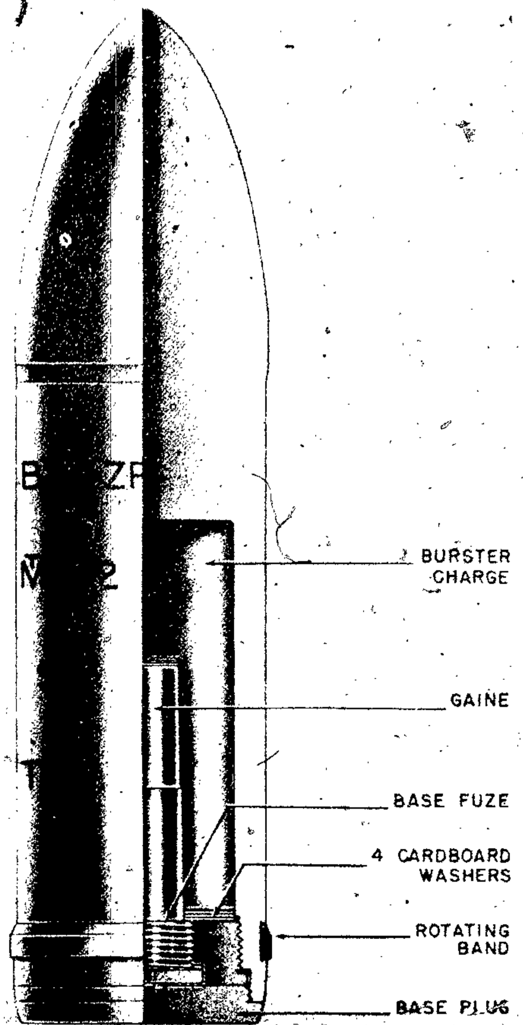
Figure 490—H. E. Projectile for 150-mm Howitzer, 15-cm Min. Gr. M. 13/19 (t)
