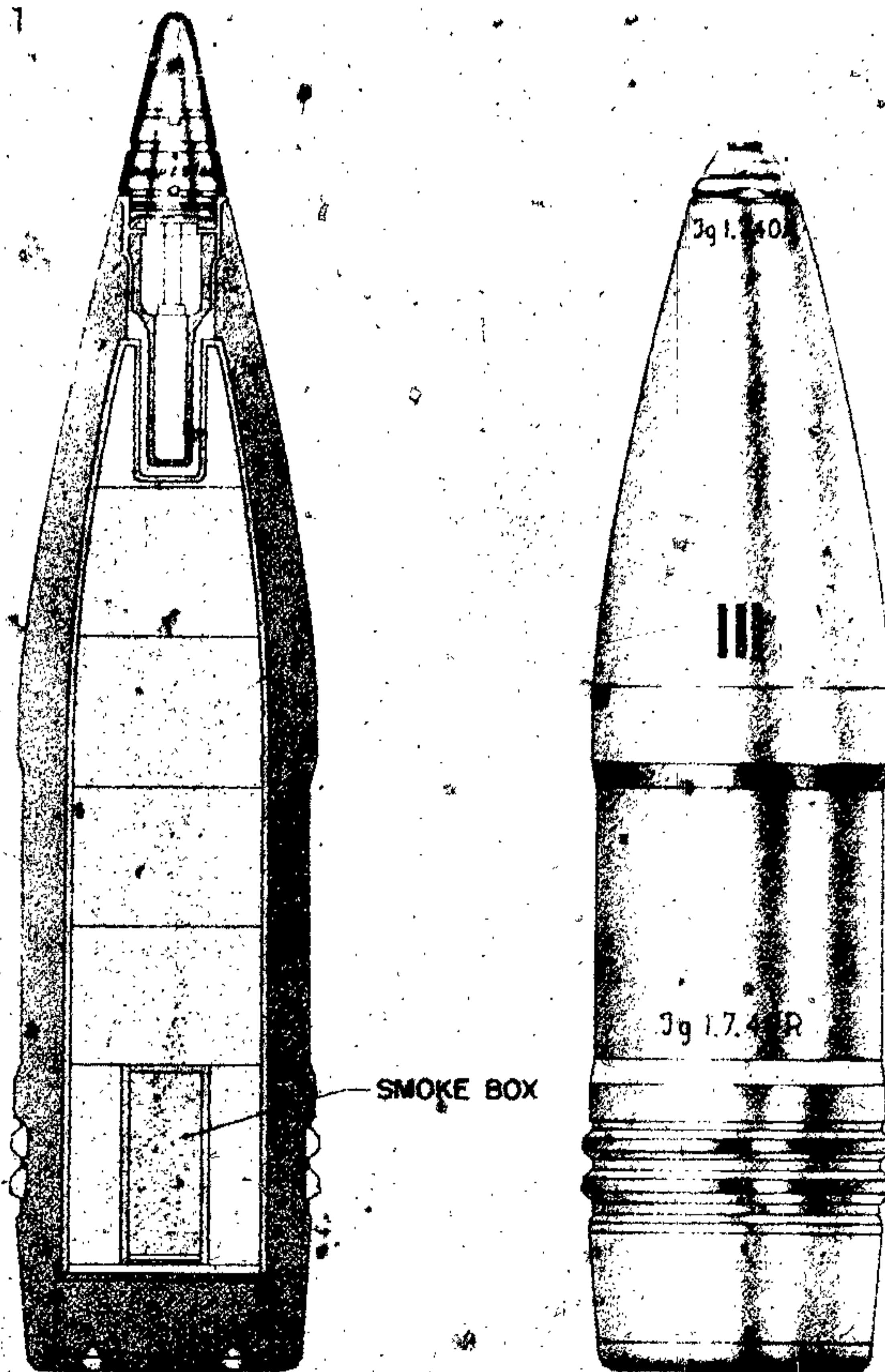
Figure 504—H. E. Projectile, Type 19, 150-mm, 15-cm Gr. 19
