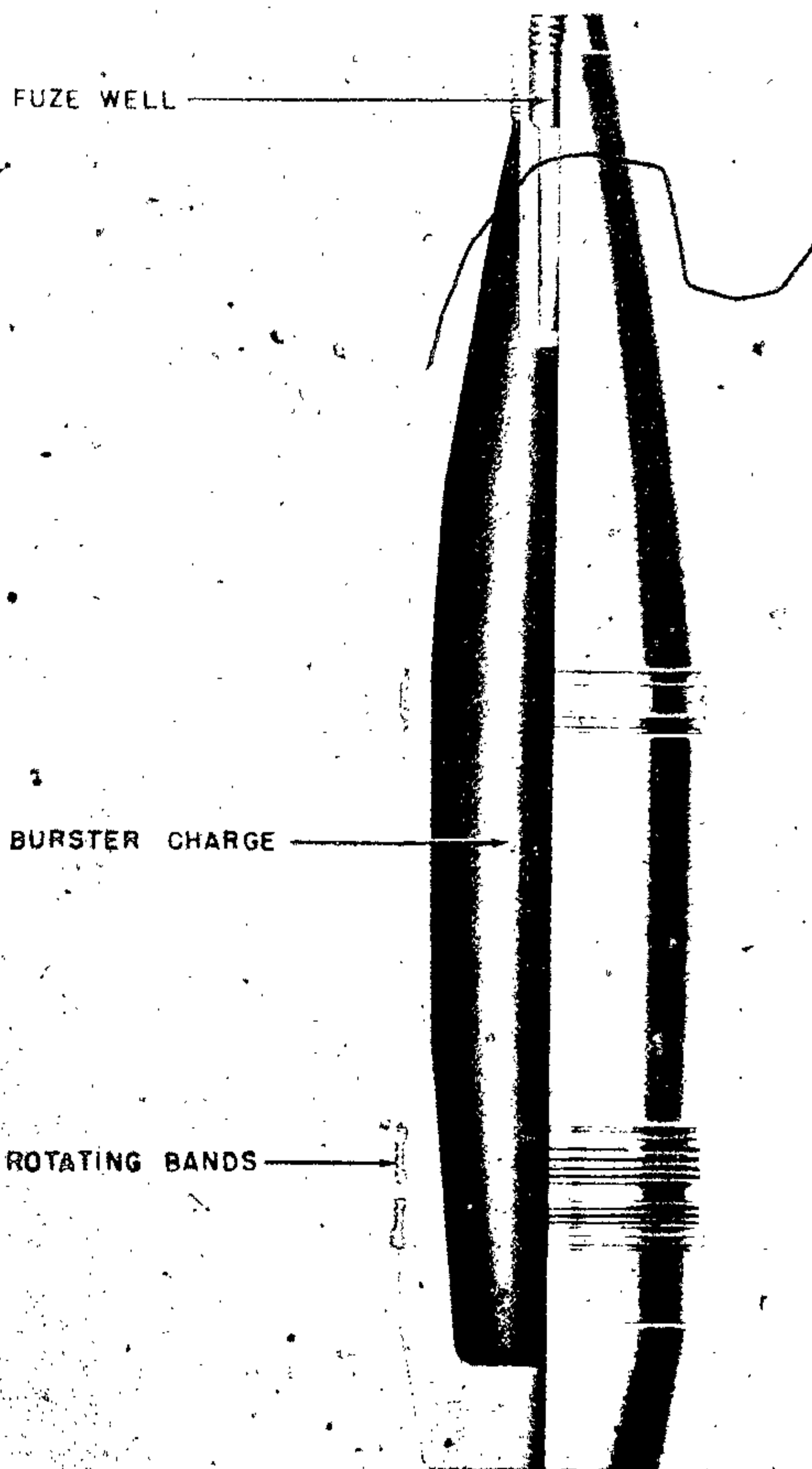
Figure 459—H. E. Projectile, 105-mm, 10.5-cm Sprgr. 348 (f) (French 36)
