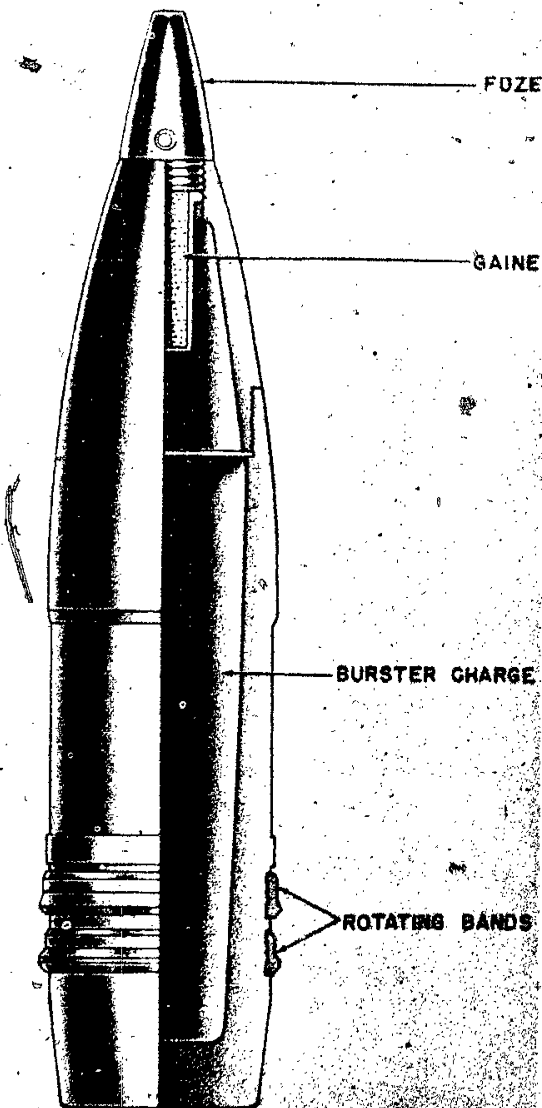
Figure 501—H. E. Projectile, Type 18, 150-mm, 15-cm K. Gr. 18
