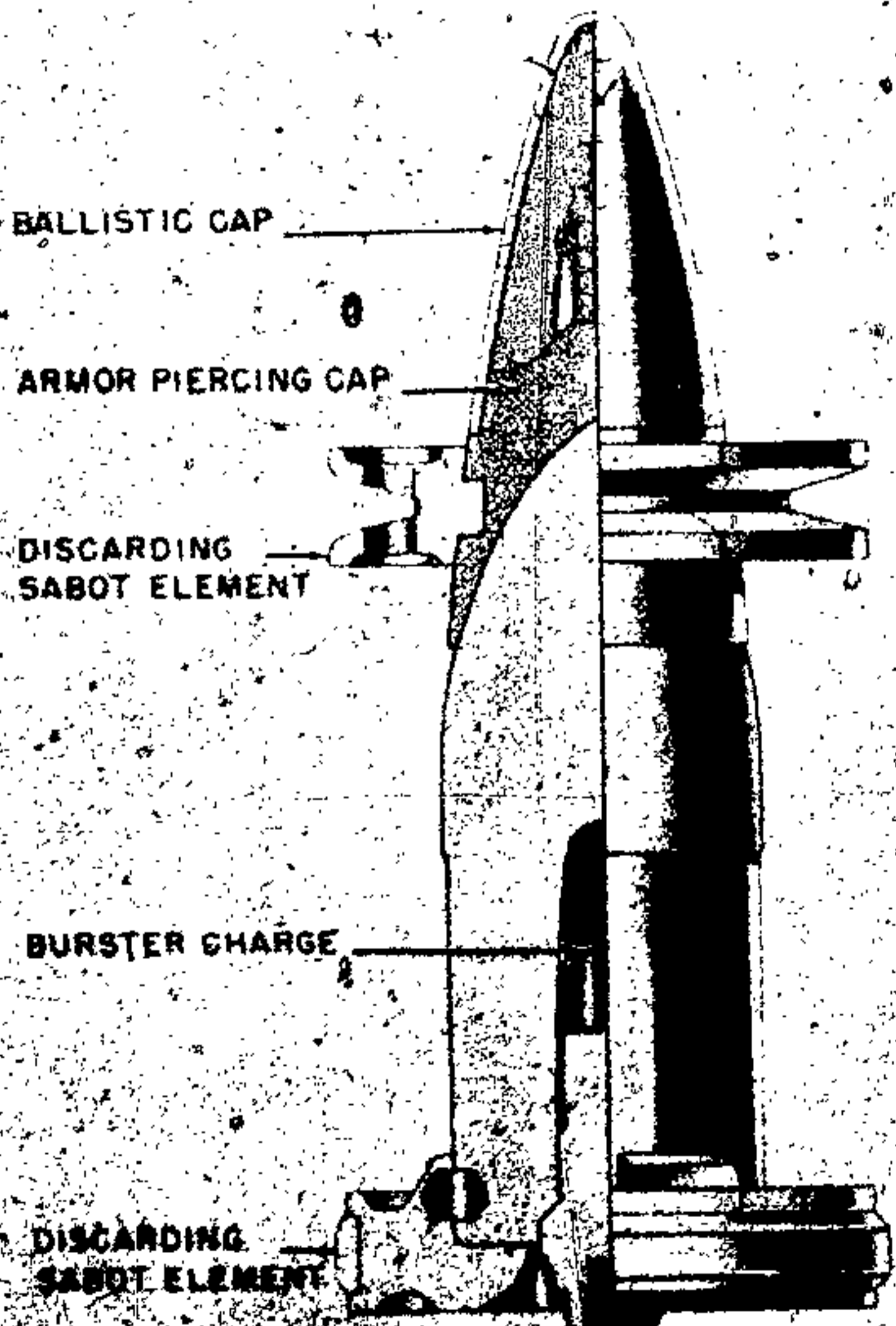
Figure 332—Sabot Projectile Type G
