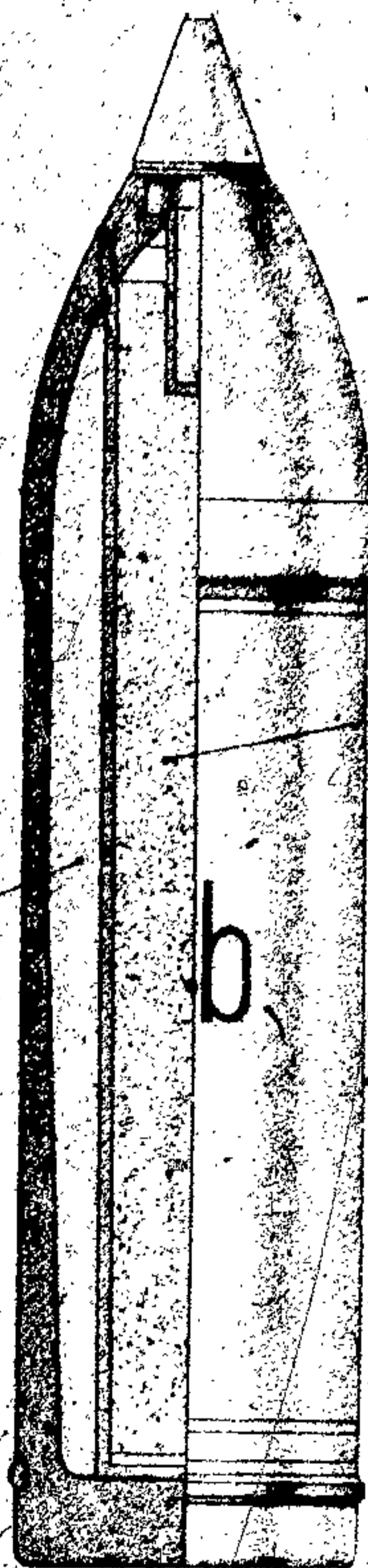
Figure 500—Smoke Projectile for Heavy Infantry Gun, 150-mm, 15-cm Jgr. 38 Nb.
