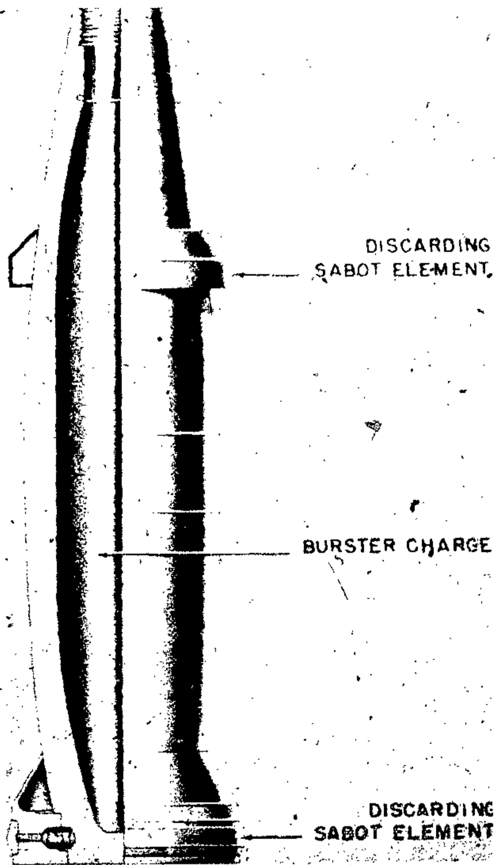
Figure 330—Sabot Projectile Type E
