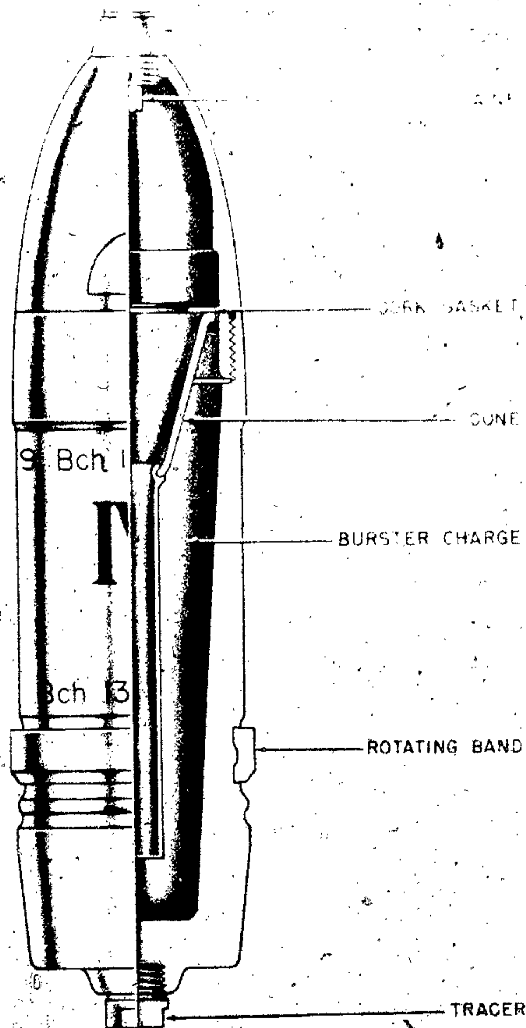
Figure 414—Hollow Charge Projectile for Howitzer, 76.2-mm, 7.62-cm Gr. 38/2 HL/B
