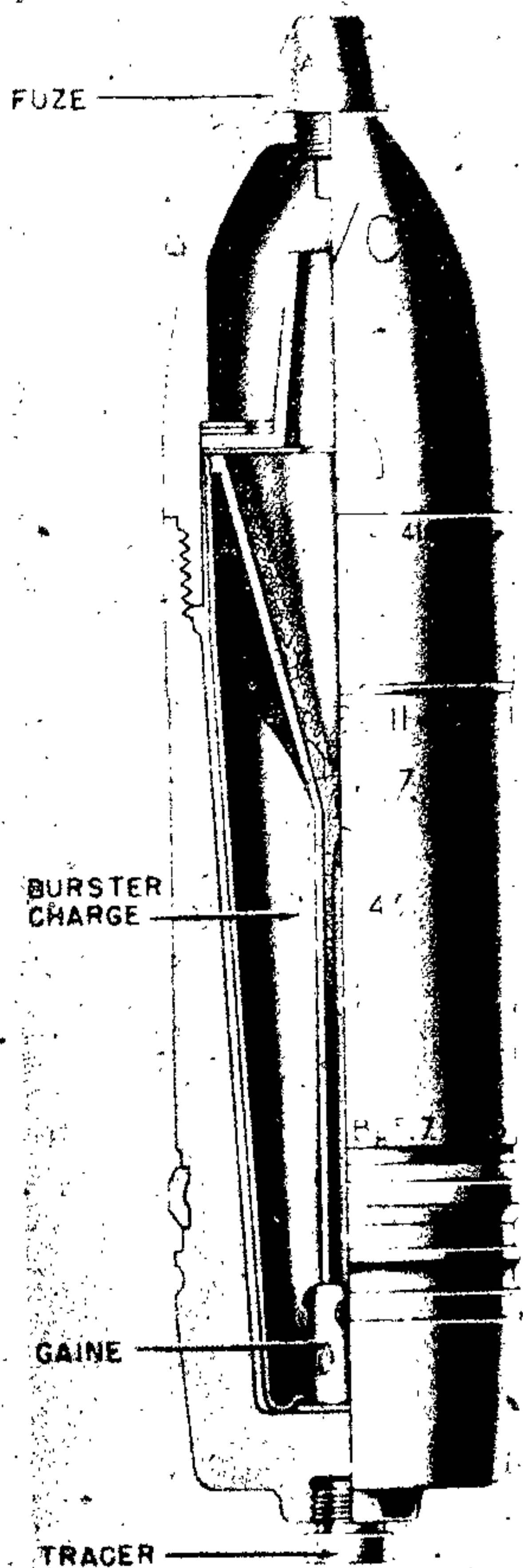
Figure 398—Hollow Charge Projectile 75-mm, 7.5-cm Gr. 38/97 H1/C (f)
