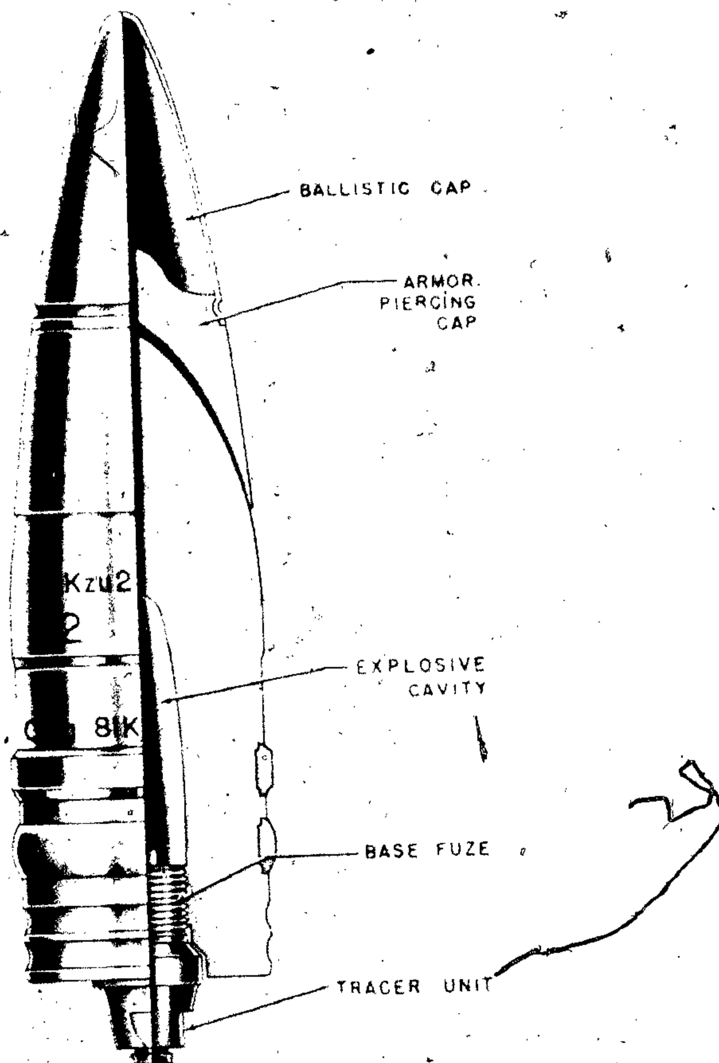
Figure 437—A. P. Projectile for 88-mm Gun, 8.8-cm Pzgr. 39/1
