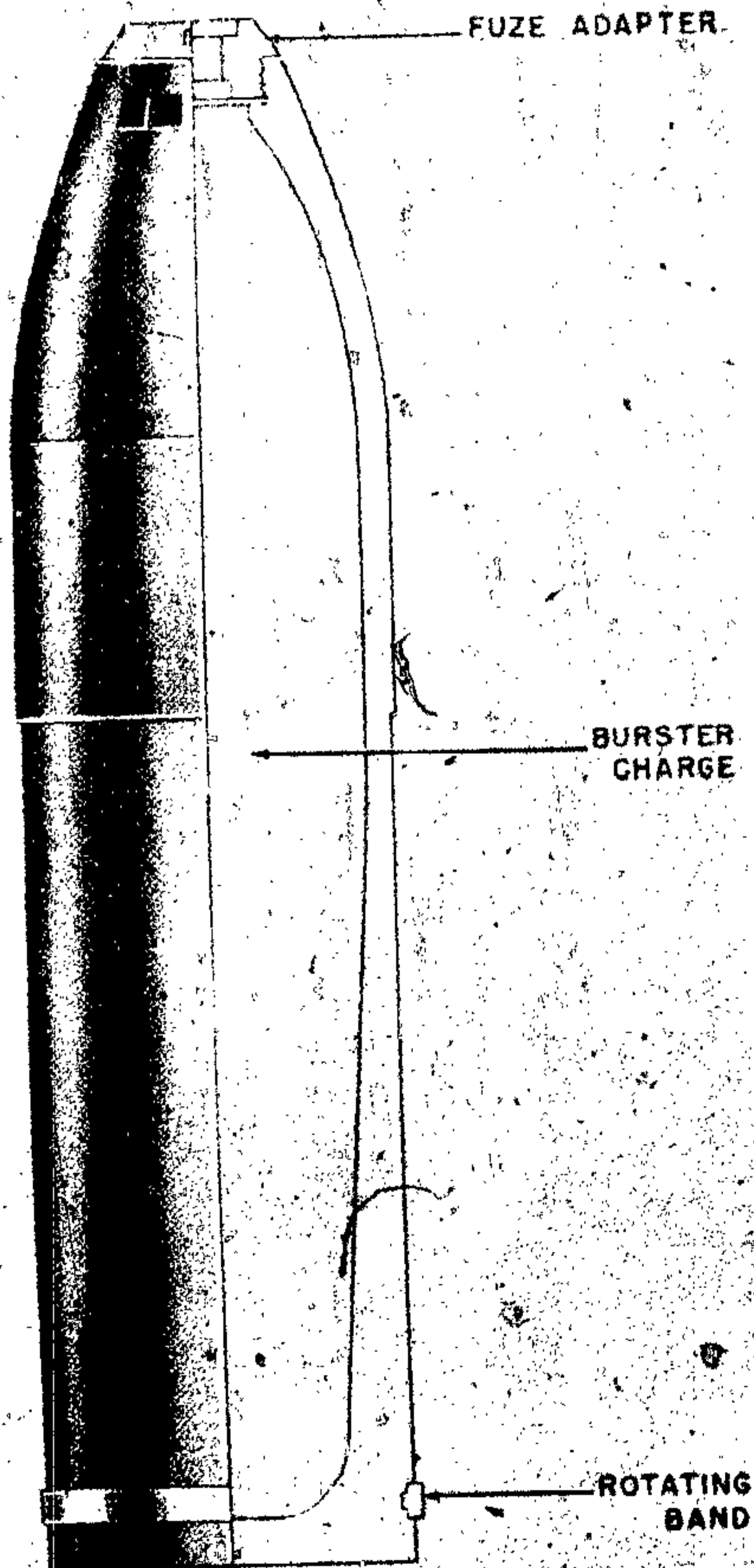
Figure 521—H. E. Projectile, 155-mm, 15.5-cm Langgr. 415 (f)
