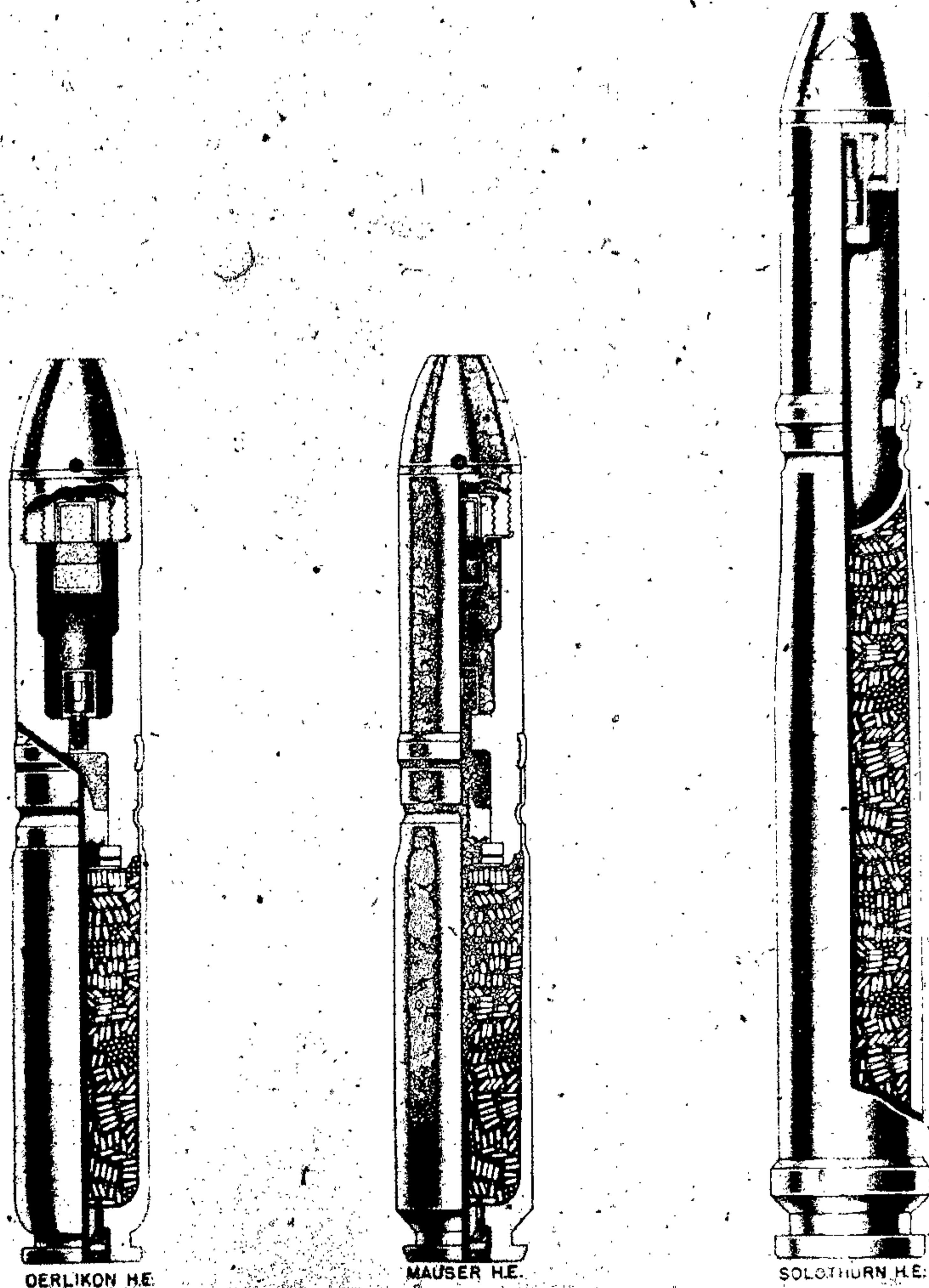
Figure 324B—20-mm Ammunition
