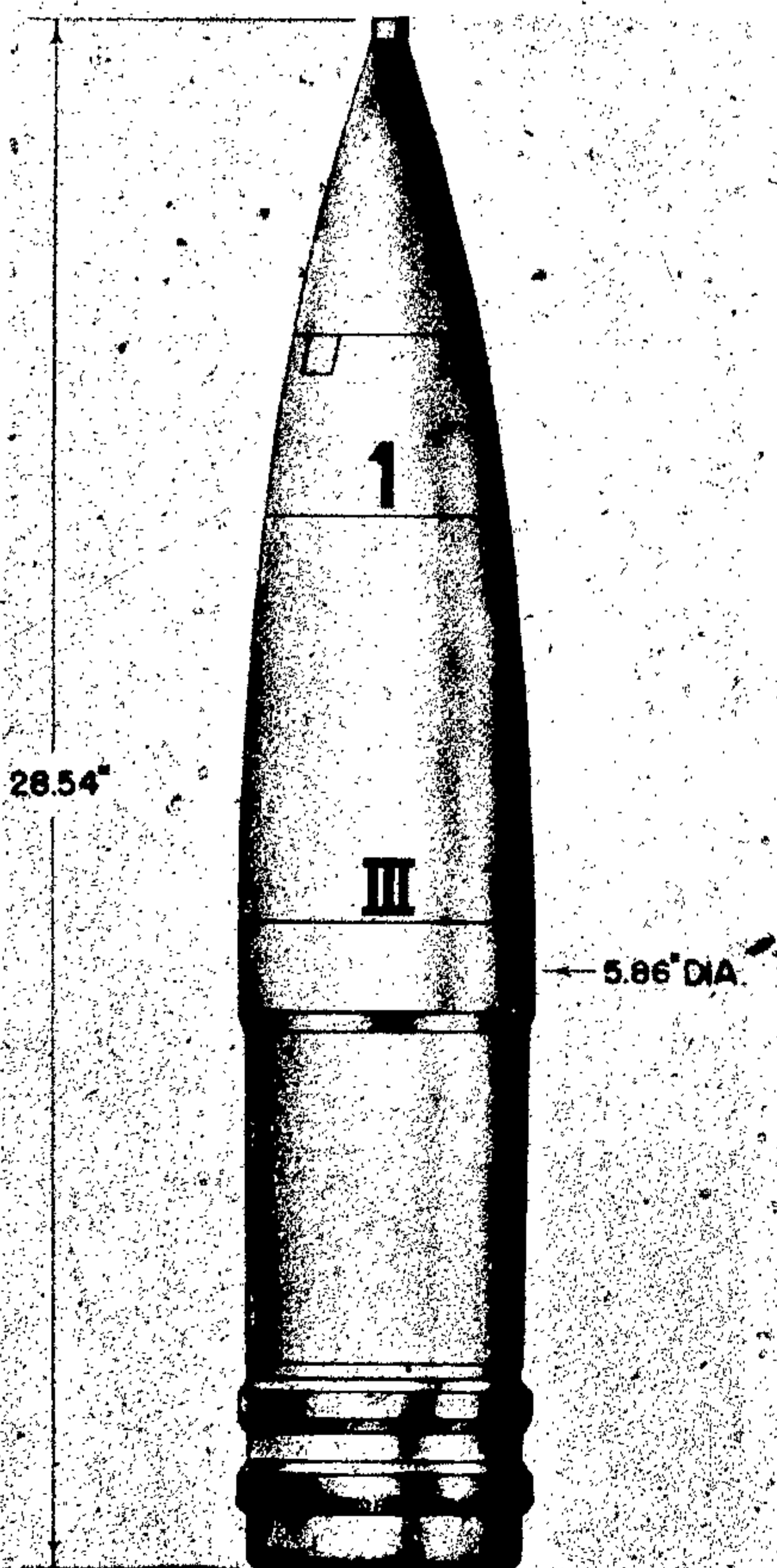
Figure 505—H. E. Projectile for Gun 16, 150-mm, 15-cm Hbgr. 16
