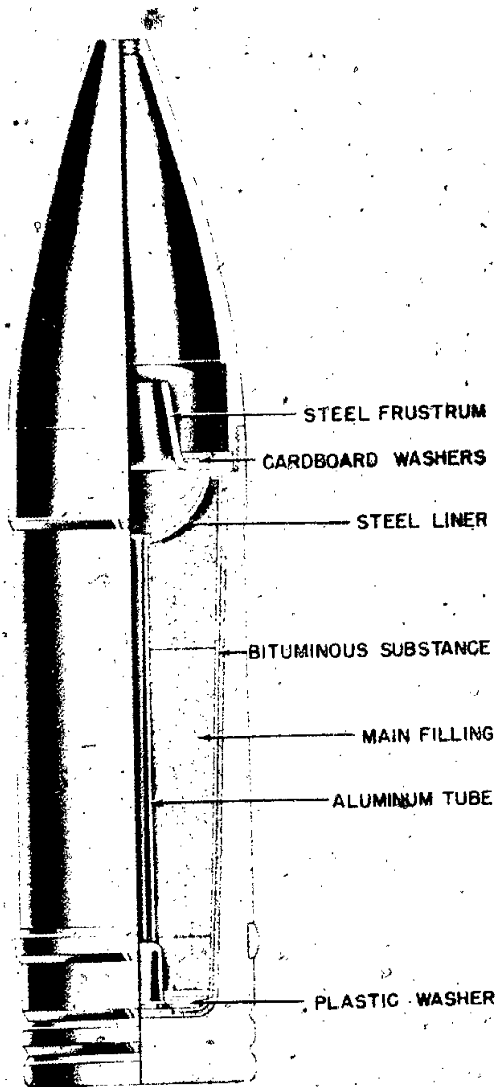
Figure 441—H. E. Hollow Charge Projectile, 100-mm, 10-cm 39 Rot H1/C 1FH 18
