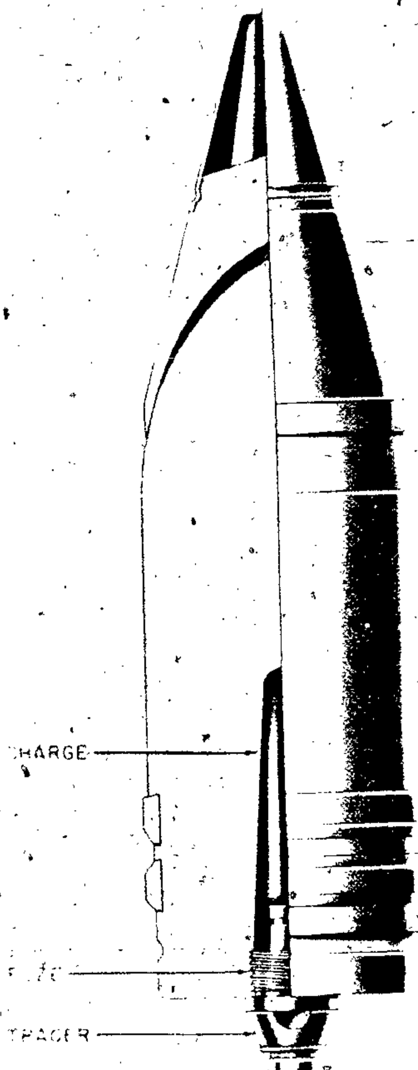
Figure 404—A. P. Projectile, 75-mm, 7.5-cm Pzgr. 39/42
