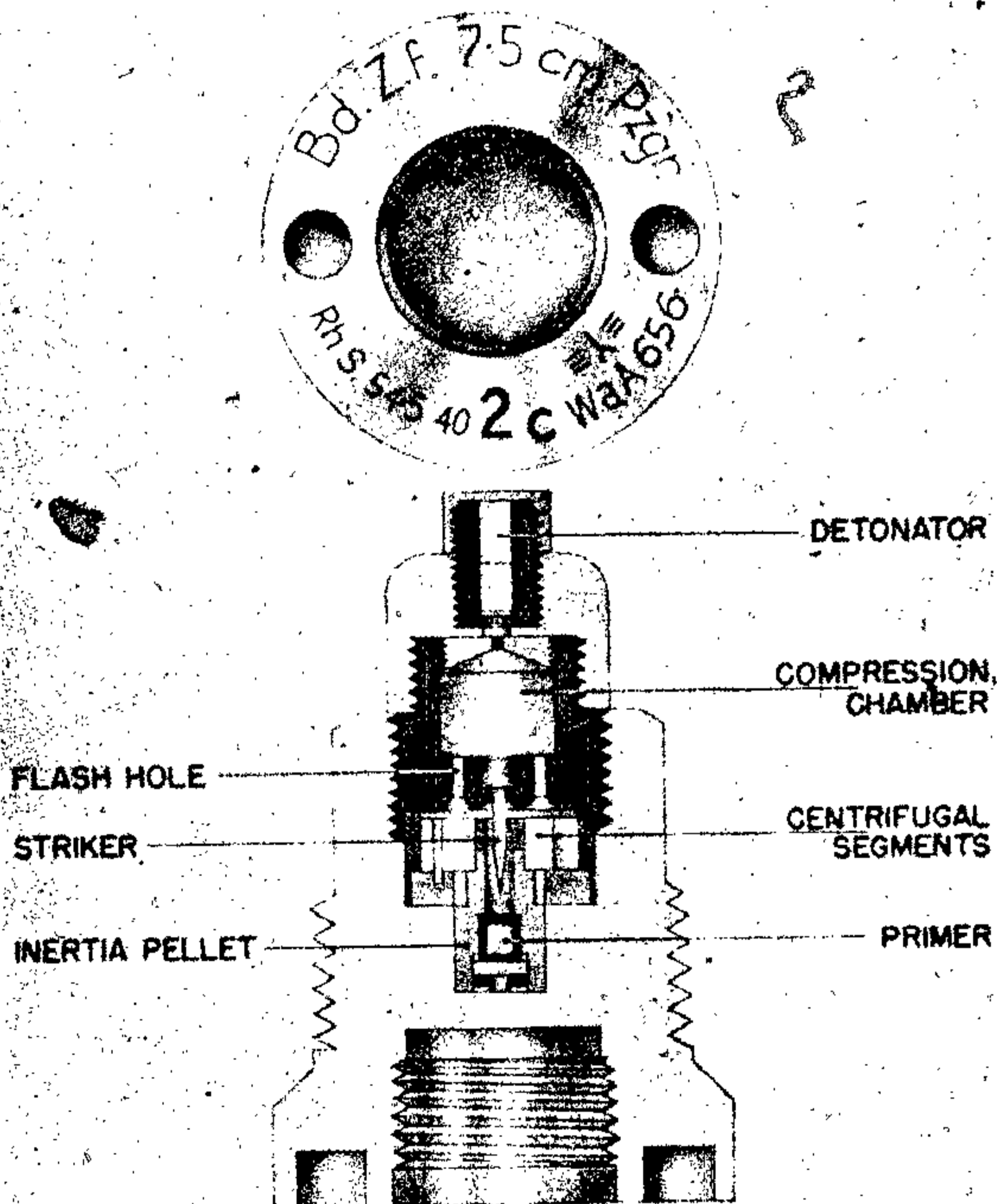
PLAN WITH GAIN ADAPTER REMOVED SHOWING CENTRIFUGAL SEGMENTS
