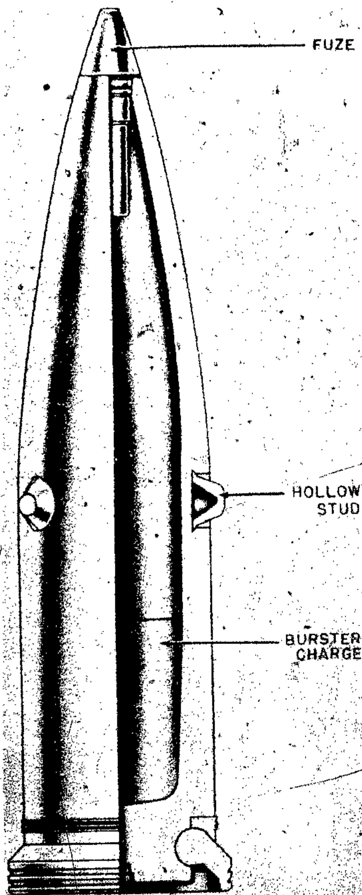
Figure 325A—German Flange Geschoss
