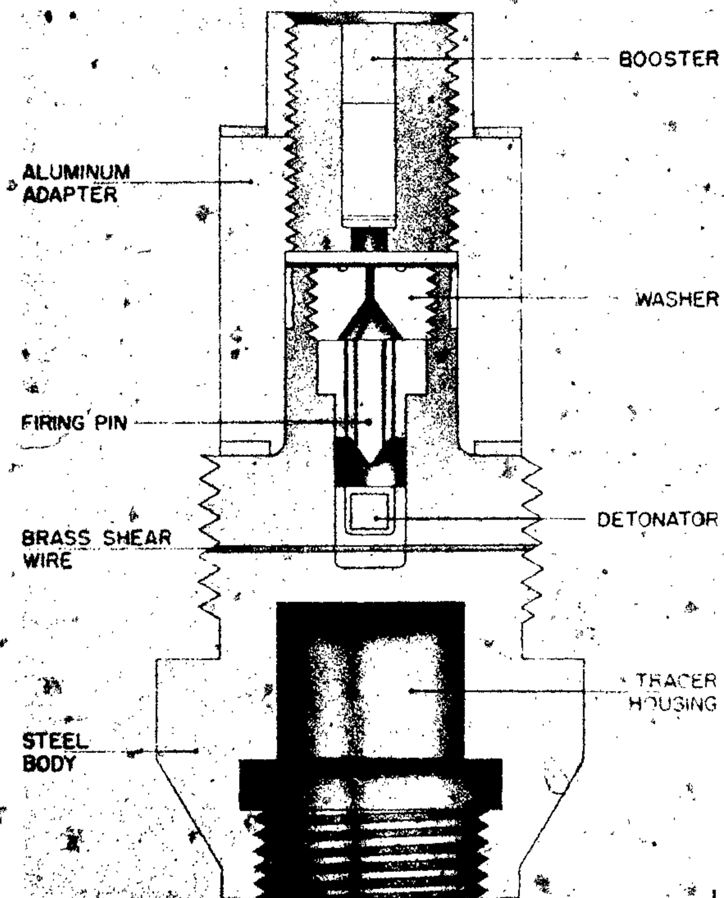
Figure 607—Fuze for 7.5-cm Projectiles (Small Cavity)
