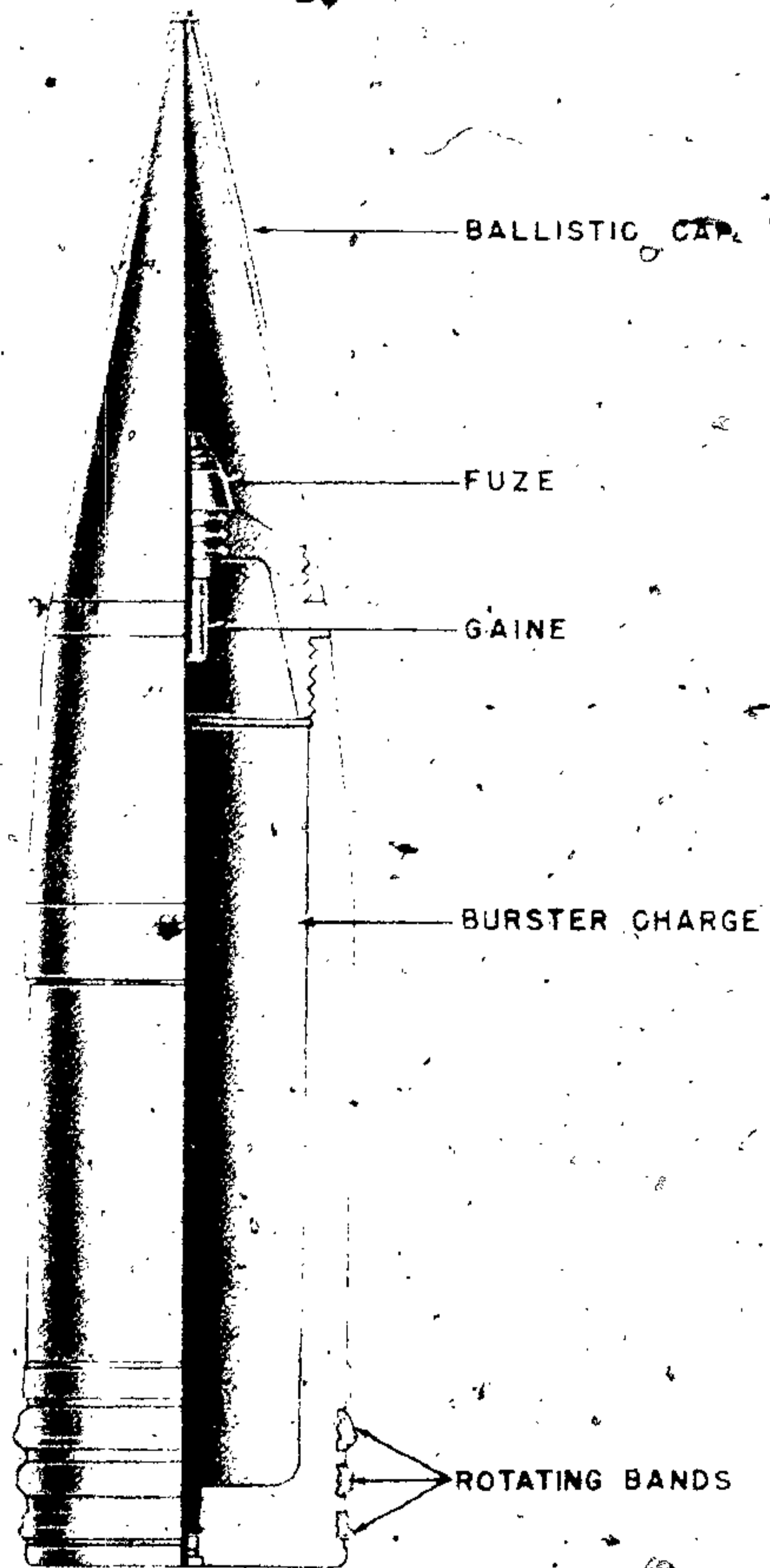
Figure 539—H. E. Projectile for 280-mm Railway Gun, 28-cm Gr. 39 m. Hbgr. Z.
