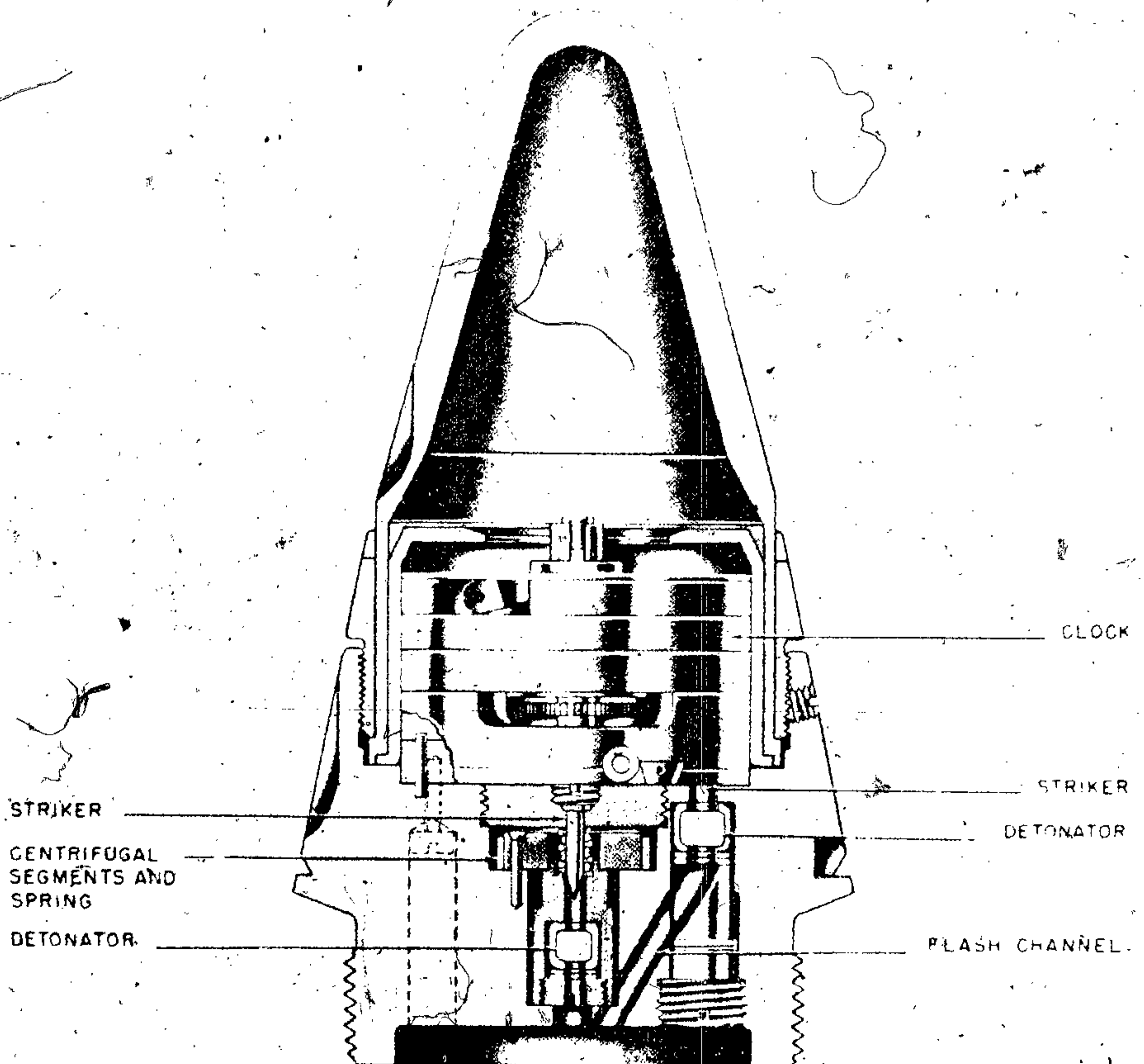
Figure 593B—Dopp. Z. S/90
