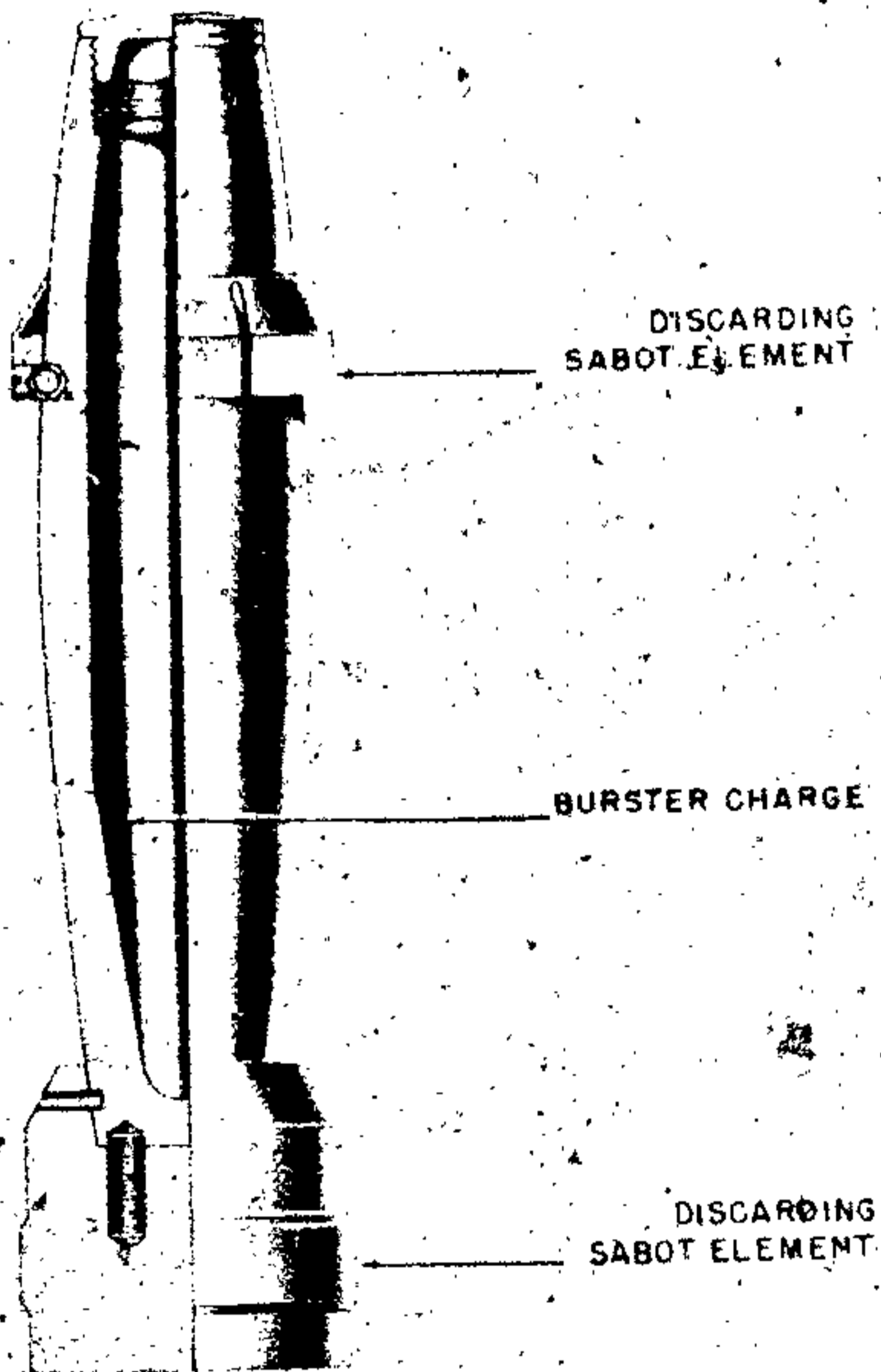
Figure 331B—Sabot Projectile Type F-2
