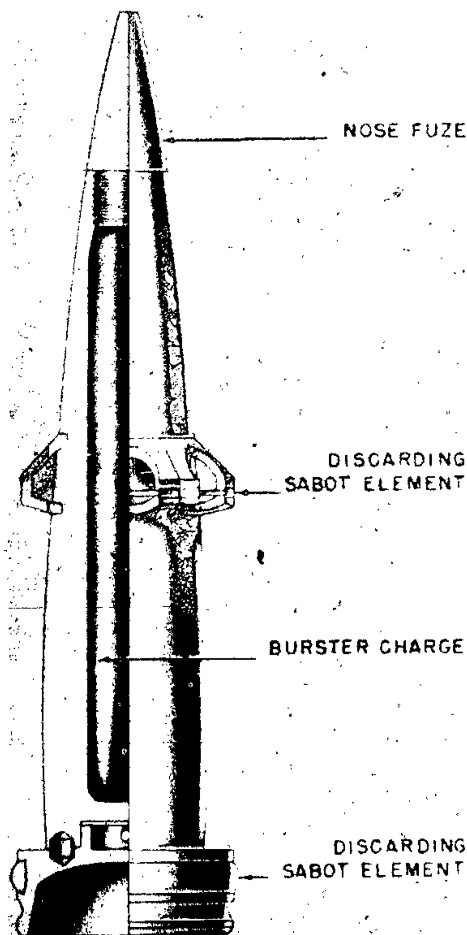
Figure 327—Sabot Projectile Type B
