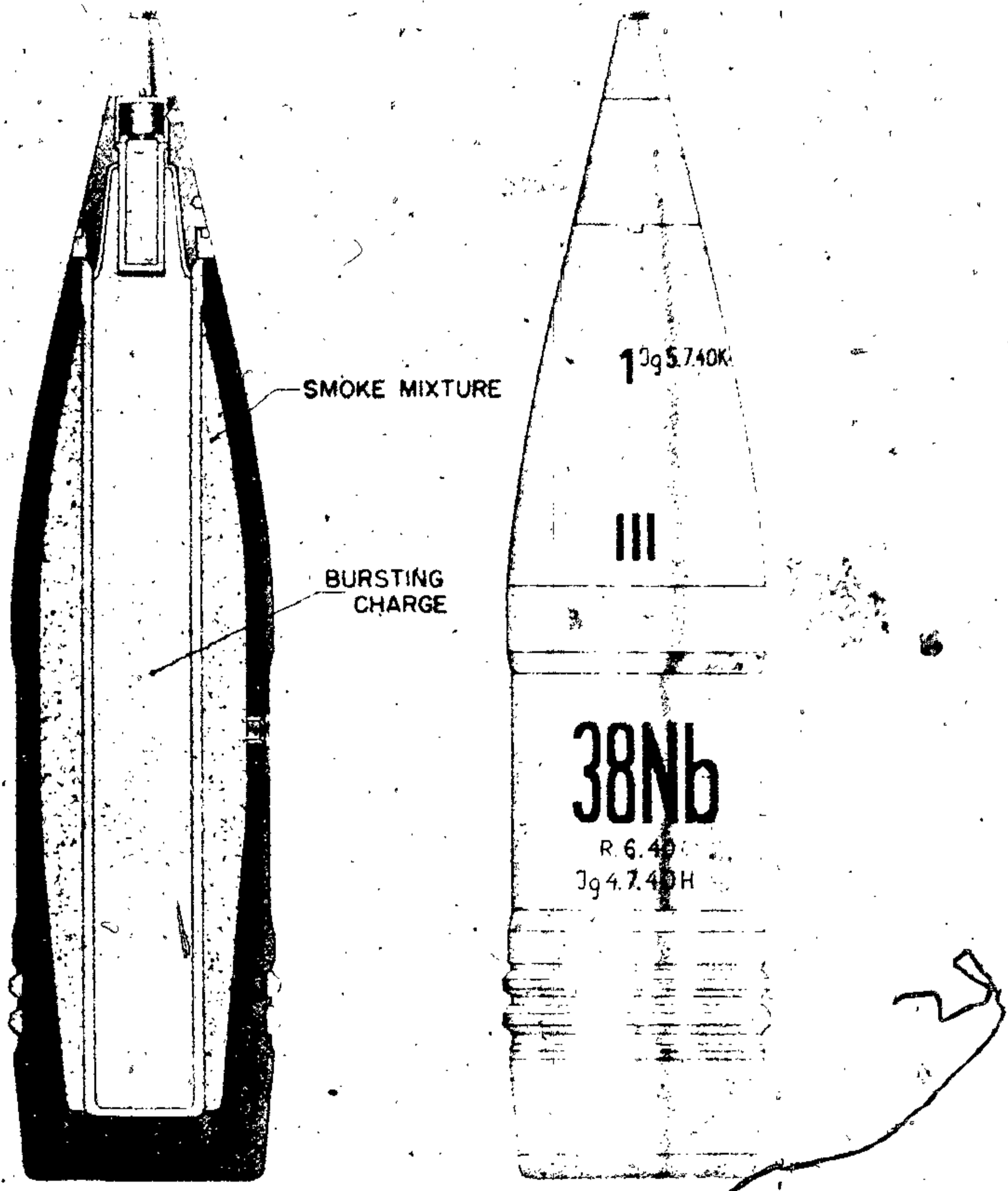
Figure 511—Smoke Projectile, Type 38, 150-mm, 15-cm Gr. 38 Nb.
