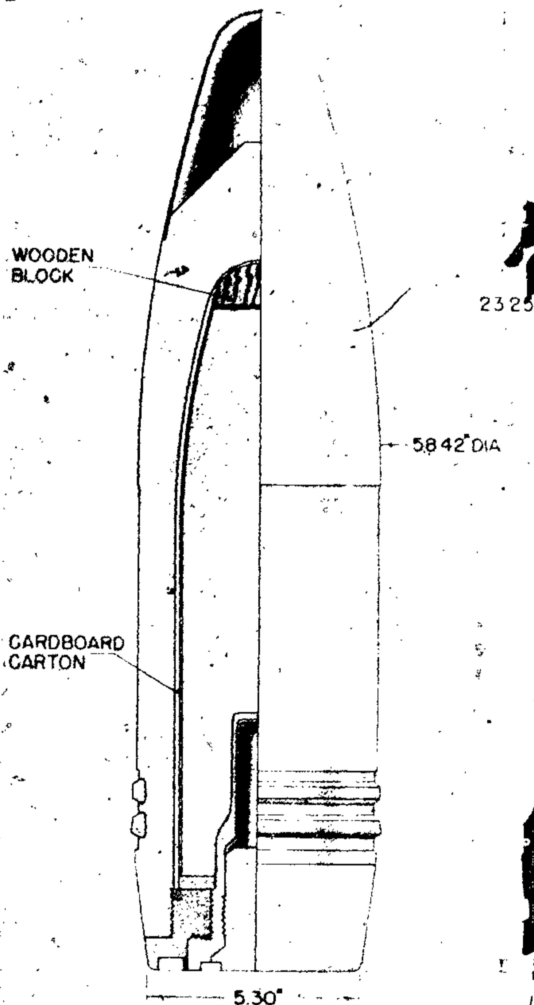
Figure 496—Anticoncrete Projectile, 150-mm Tracer, 15-cm Gr. 19 Rot Be.
