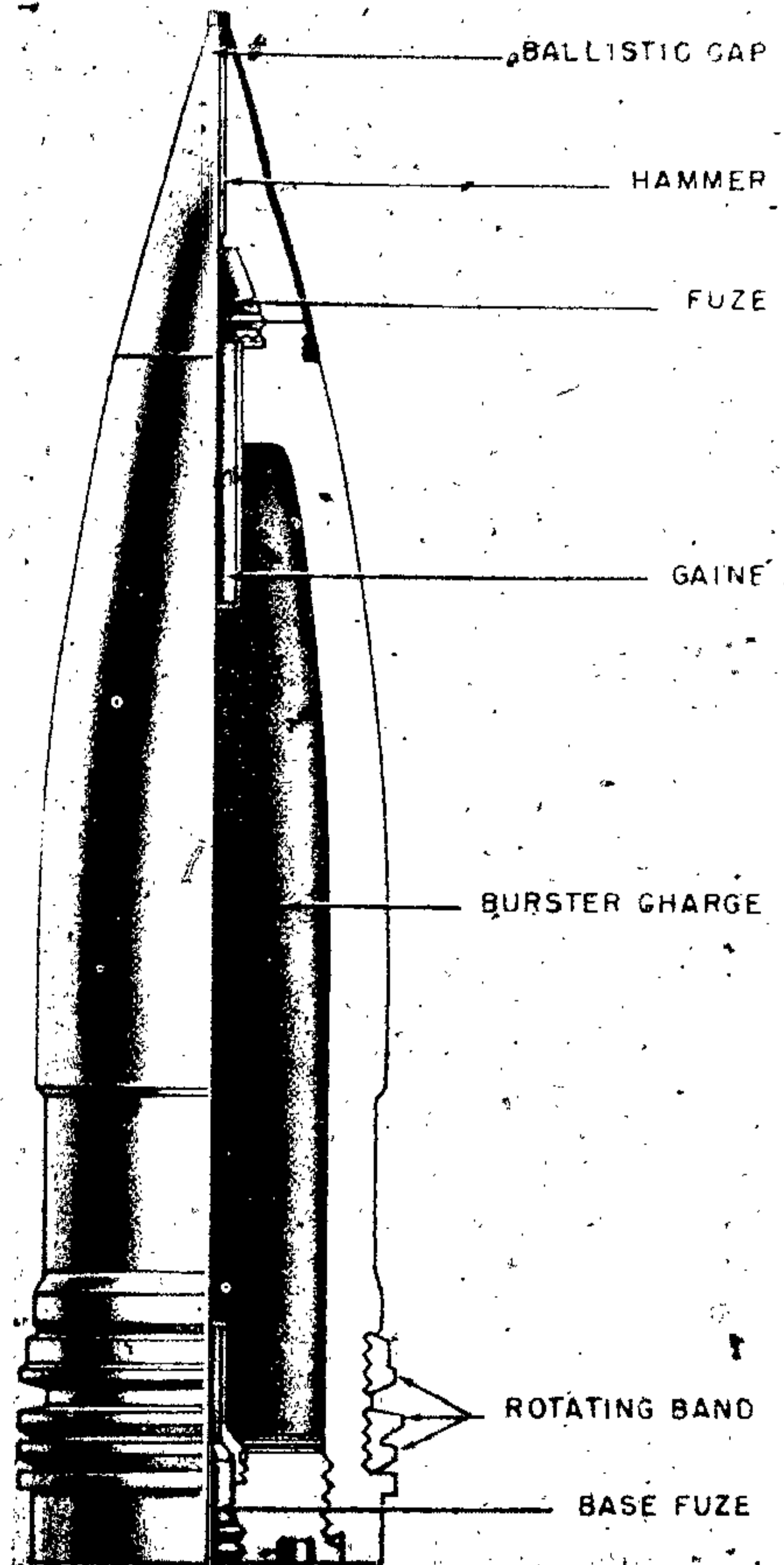
Figure 534—H. E. Shell for 240-mm Gun, 24-cm Sprgr. L/4.2 m. lb.
