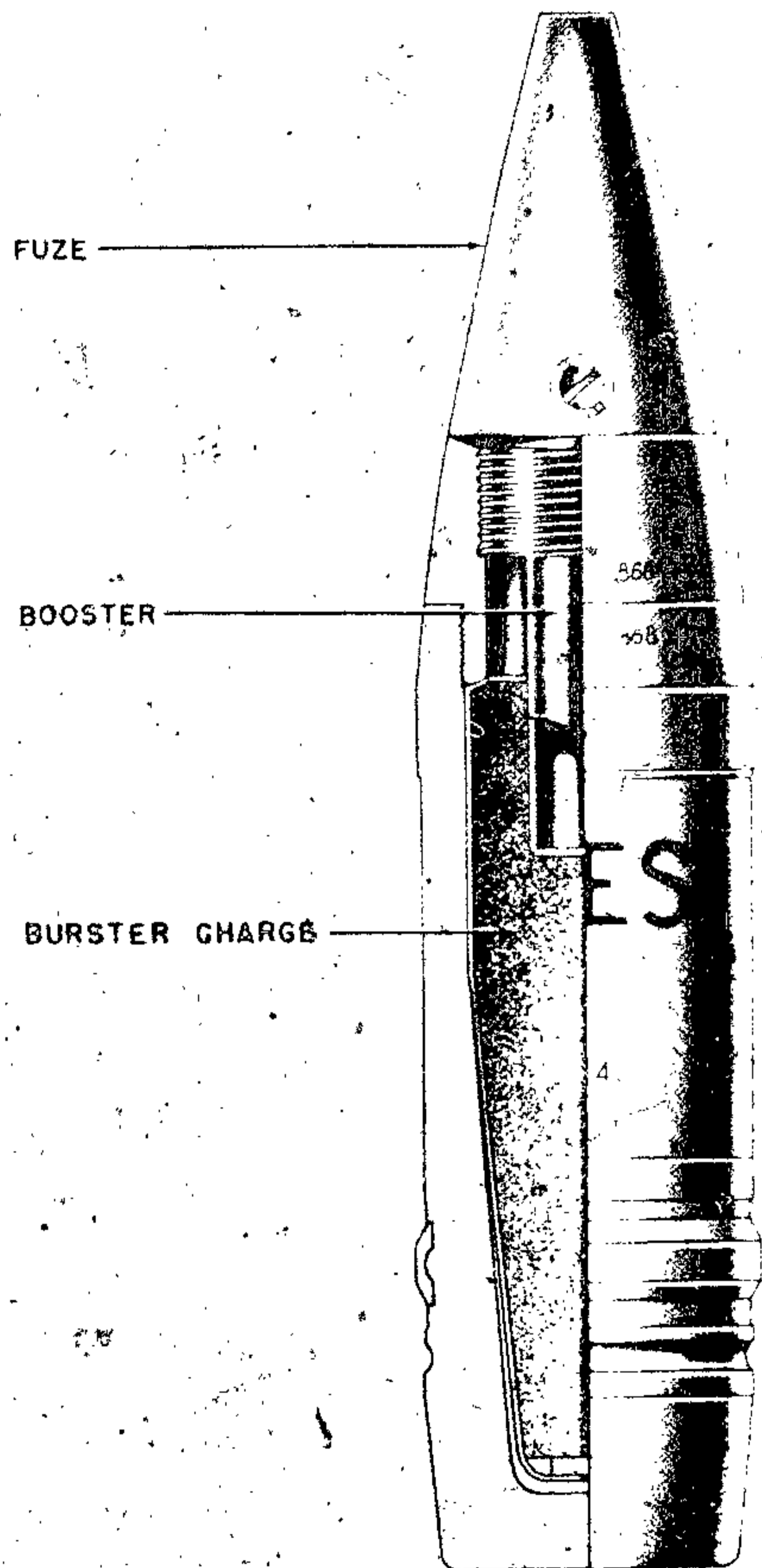
Figure 392—H. E. Shell for 75-mm Field Gun, 7.5-cm K. Gr. Rot FES
