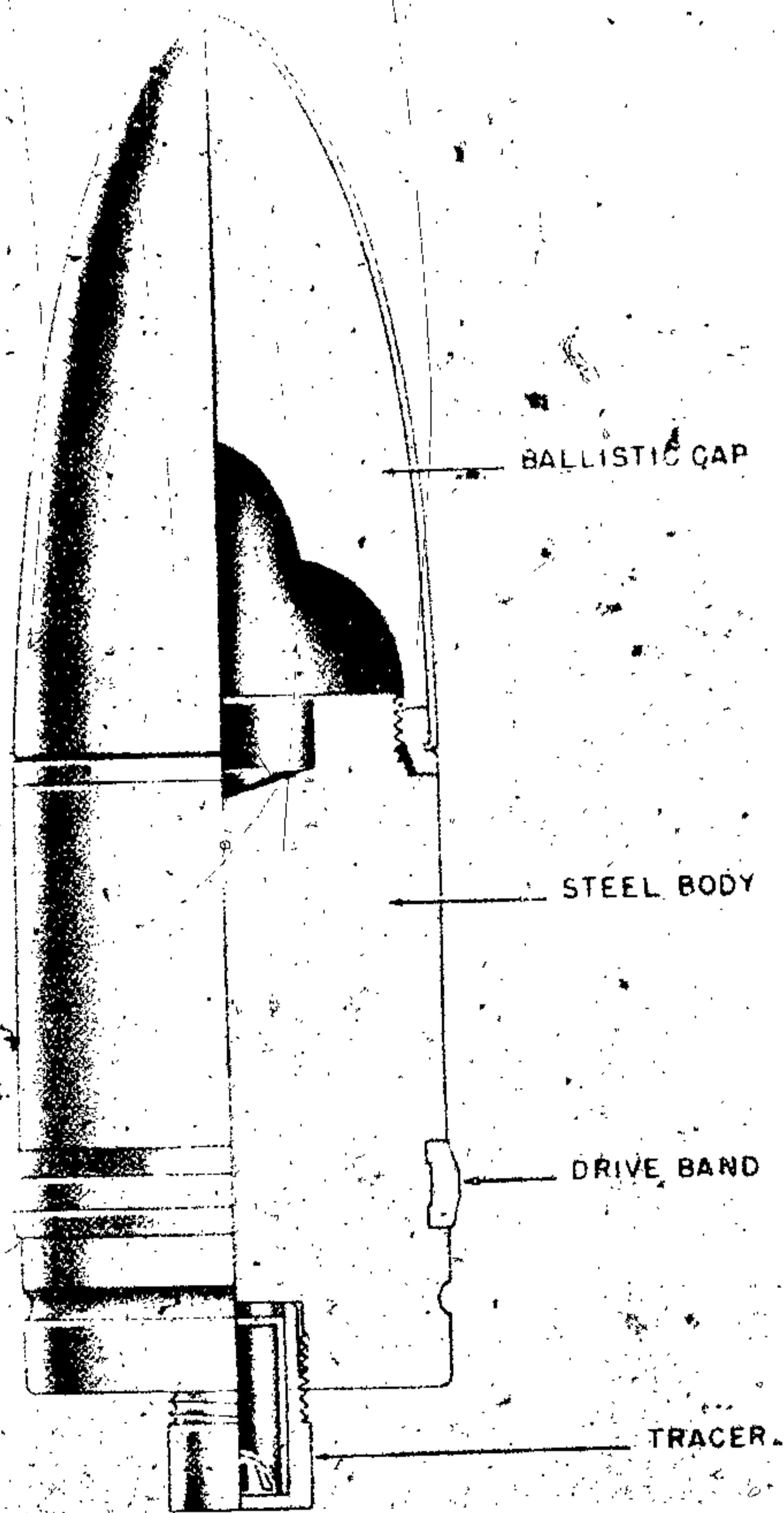
Figure 382—A. P. Projectile 75-mm, 7.5-cm Pzgr. 40 (W) Pack. 40
