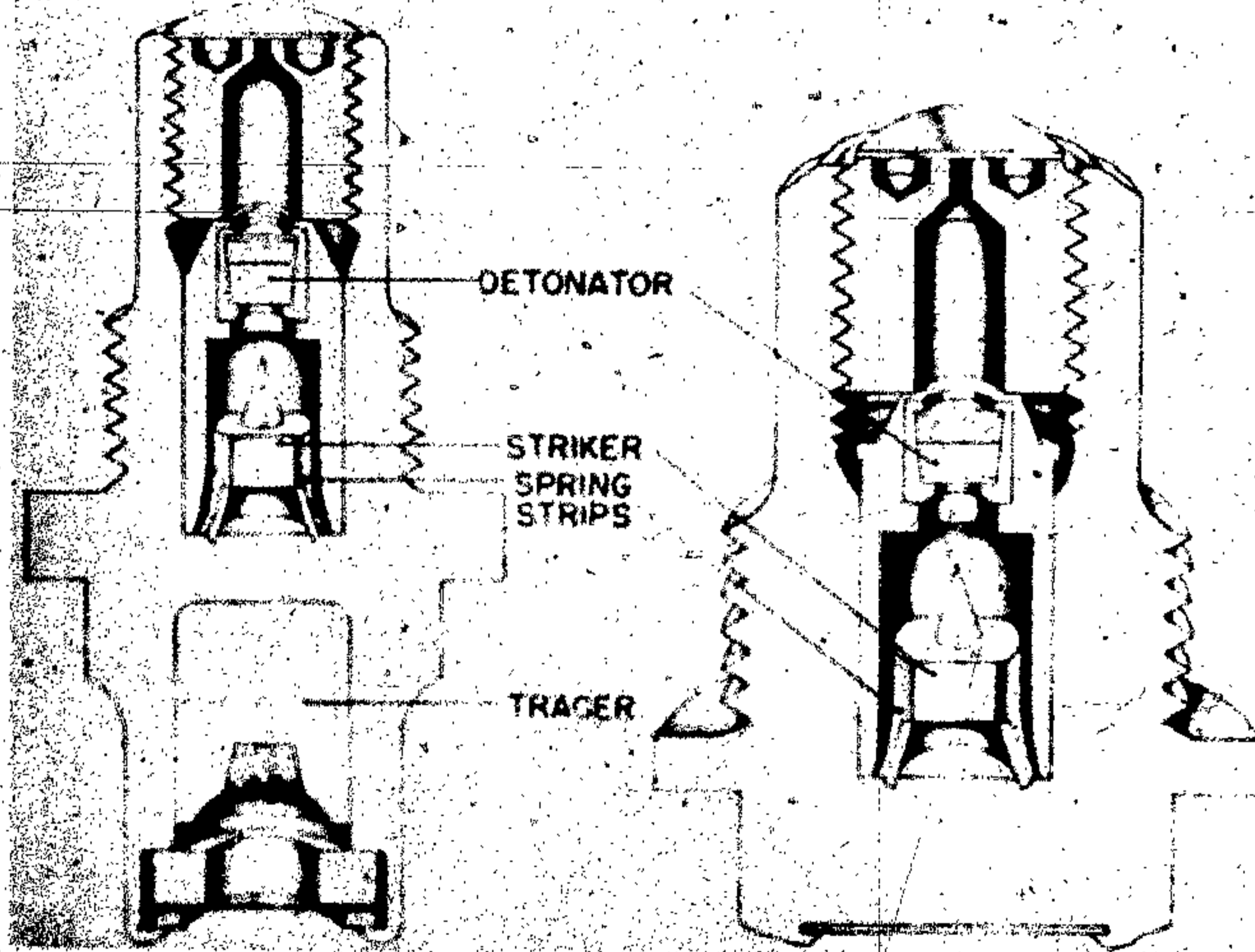
Figure 599—Bd. Z. 1511 and Bd. Z. 1512
