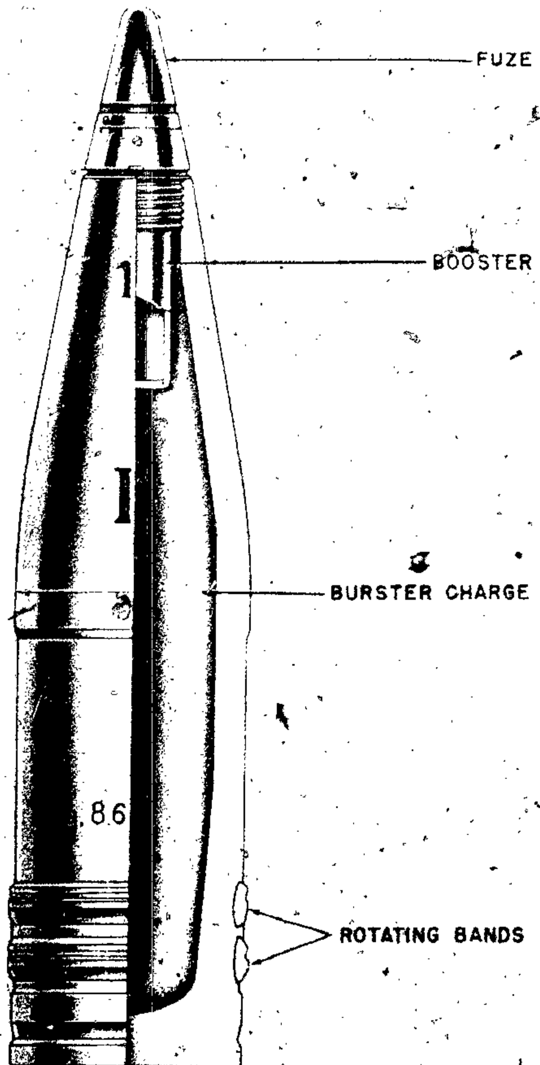
Figure 480—H. E. Projectile, 128-mm, 12.8-cm Sprgr. Patr. 1/4.5
