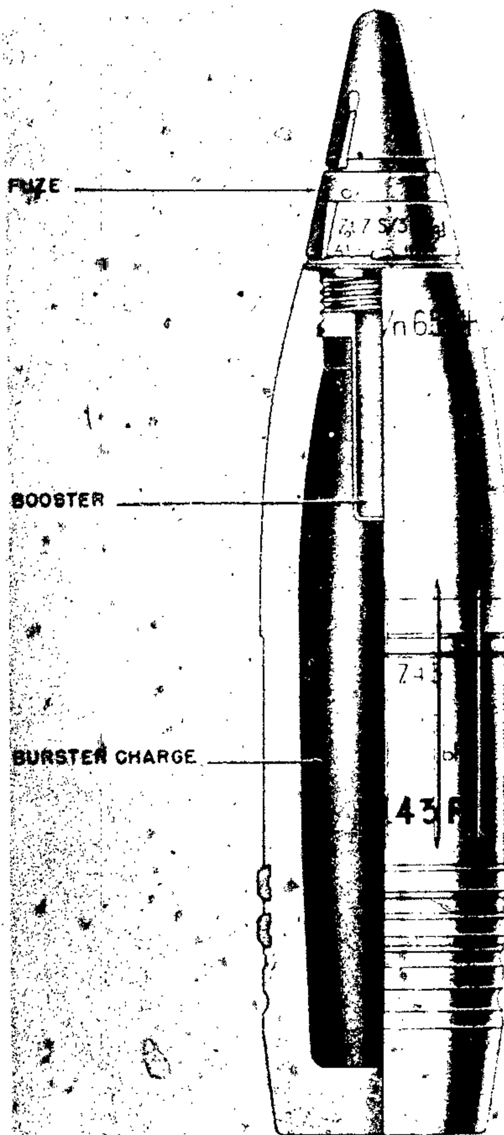
Figure 432—H. E. Projectile for 88-mm Gun, 8.8-cm Sprgr. Flak 41
