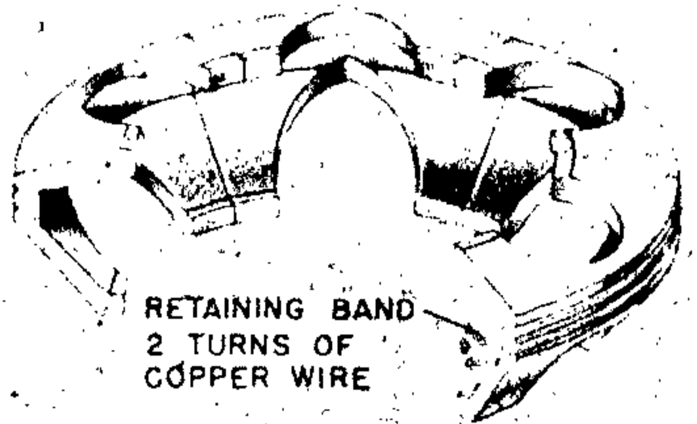
FORWARD DISCARDING SABOT ELEMENT (4 SEGMENTS OF 6)
