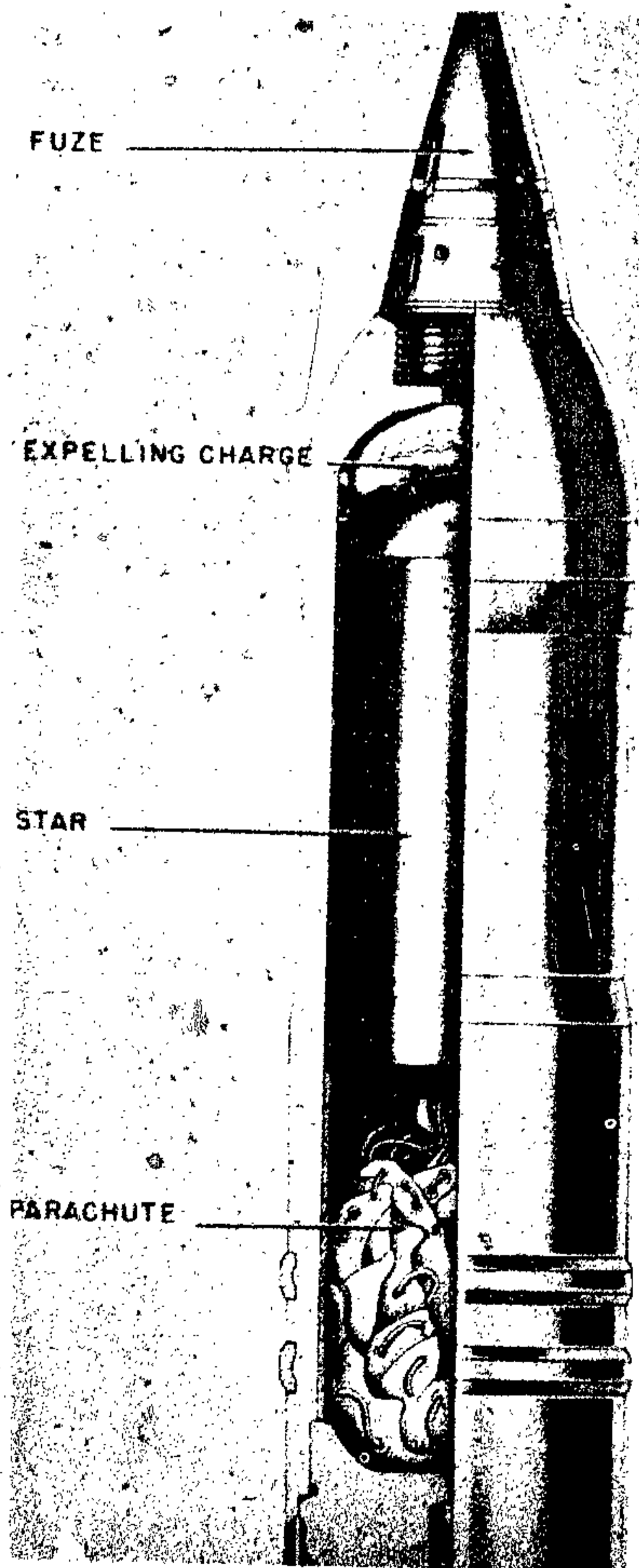
Figure 460—Star Shell, 105-mm, 10.5-cm Lt. Gs. FES
