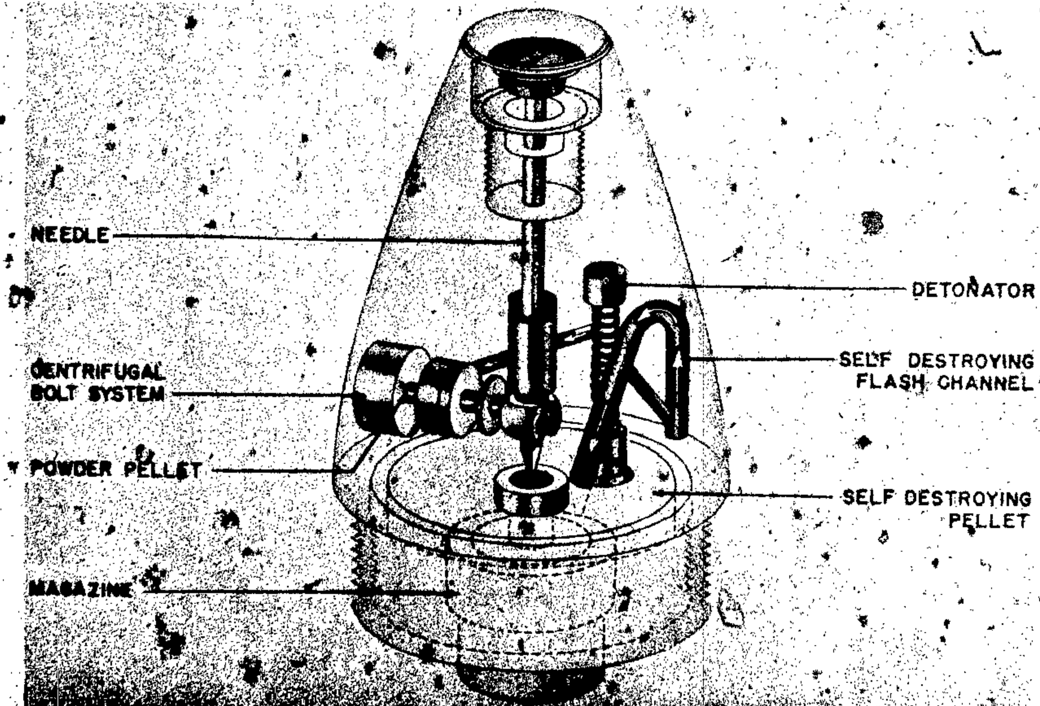
Figure 566—3.7-cm Kopfzunder Zerl. P.
