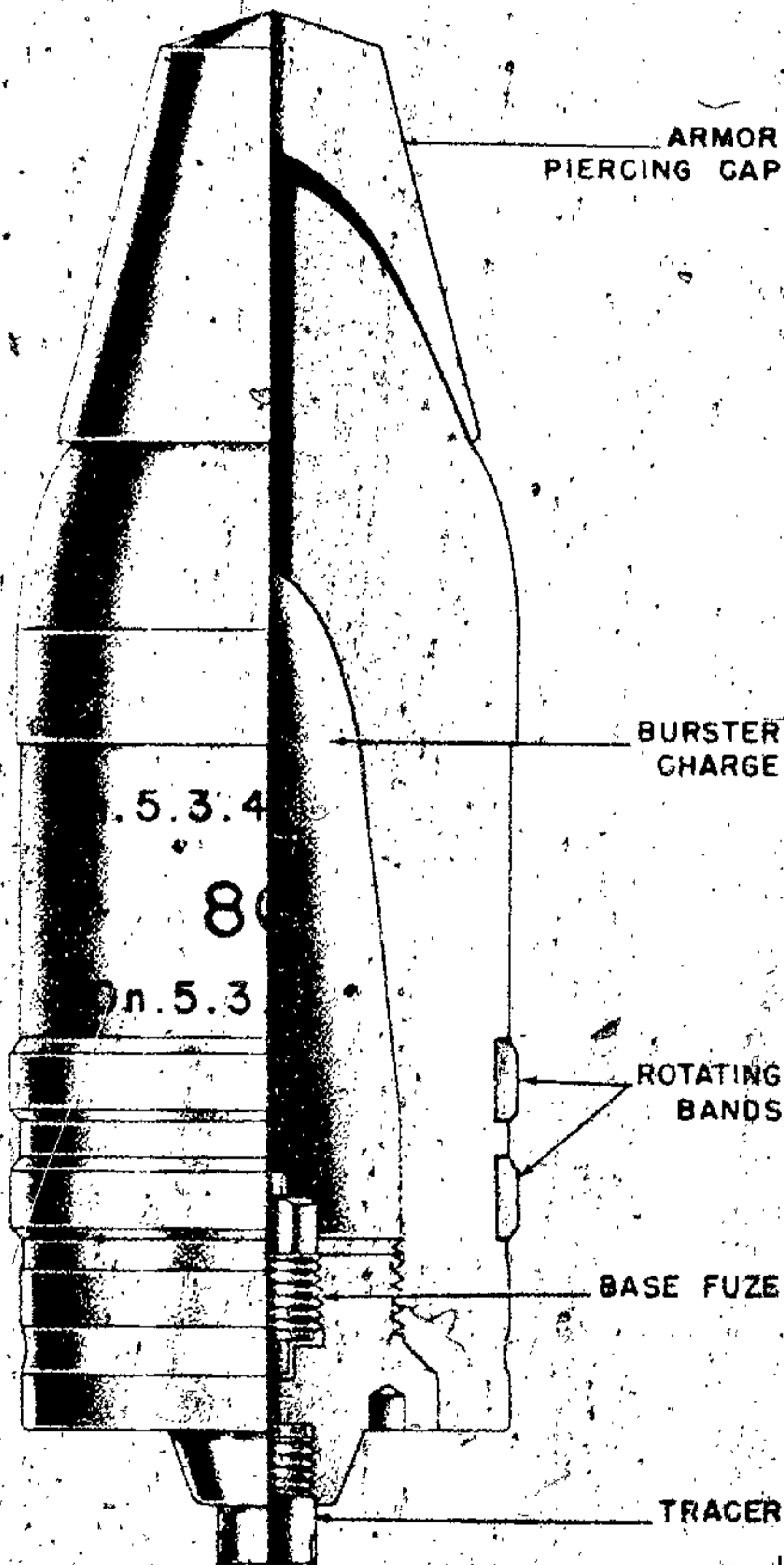
Figure 482—A. P. Projectile, 128-mm, 12.8-cm Pzgr. KPS
