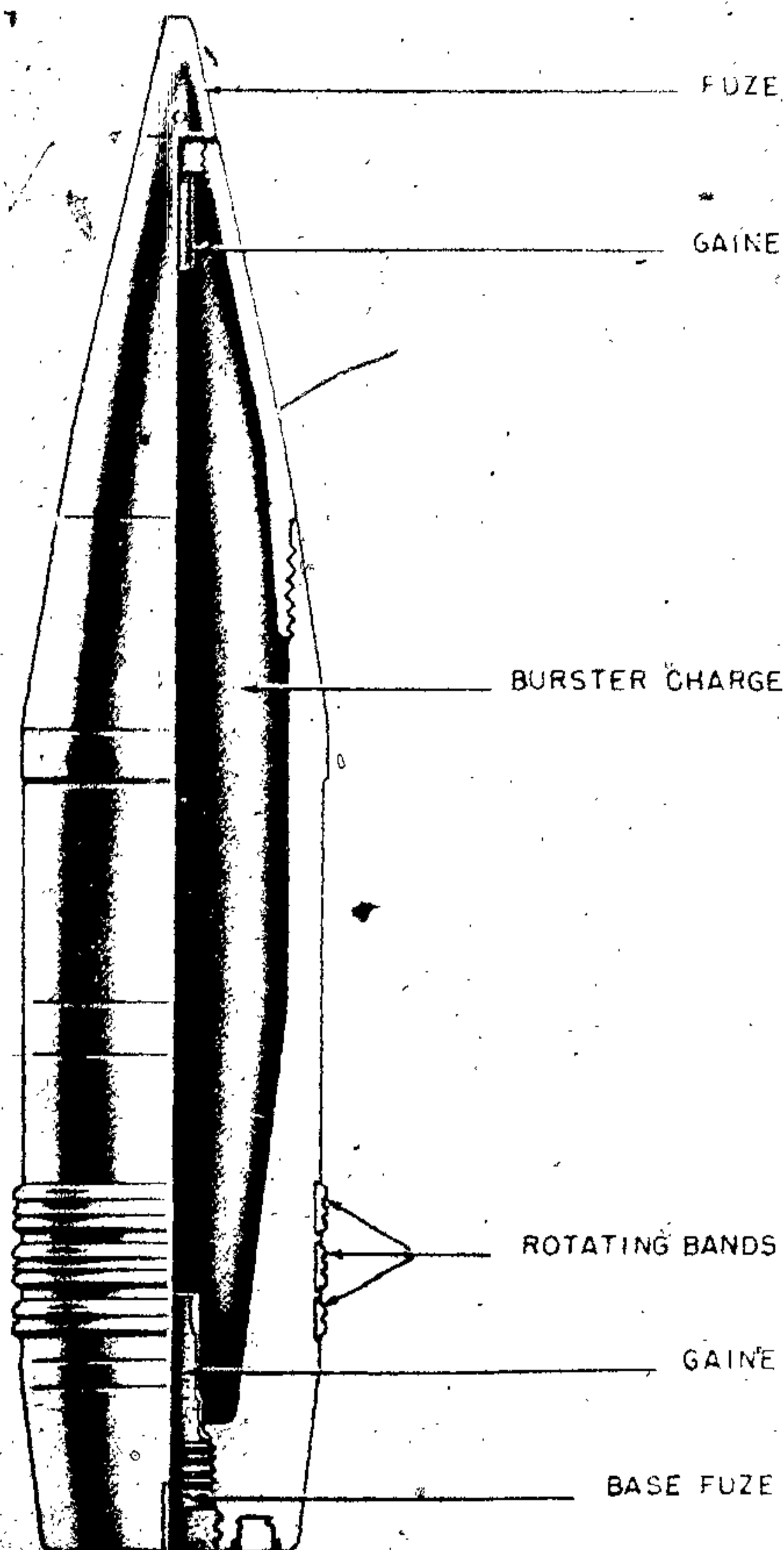
Figure 535—H. E. Projectile for 240-mm Czech Heavy Gun, 24-cm Gr. 40 (t)
