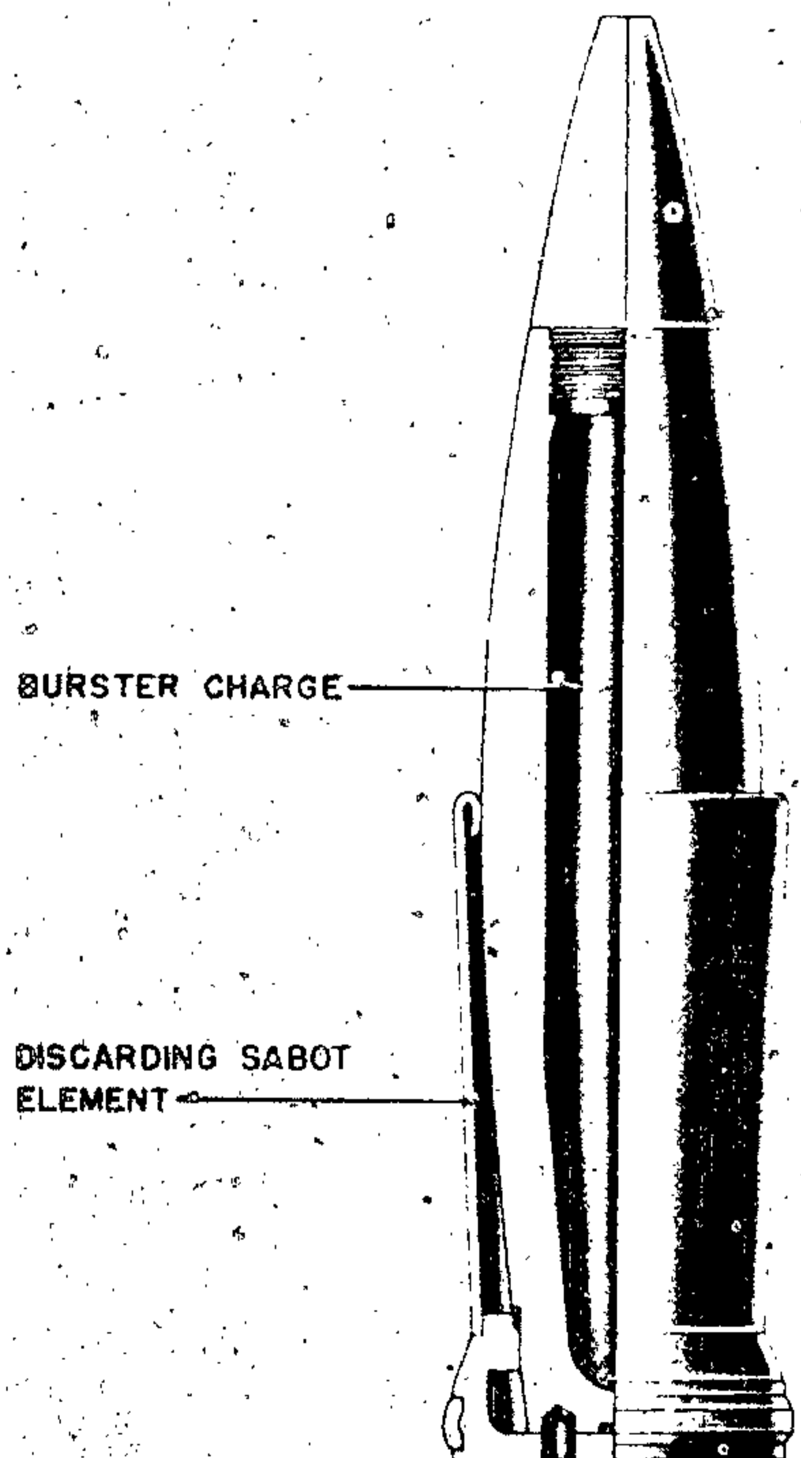
Figure 334—Sabot Projectile Type J
