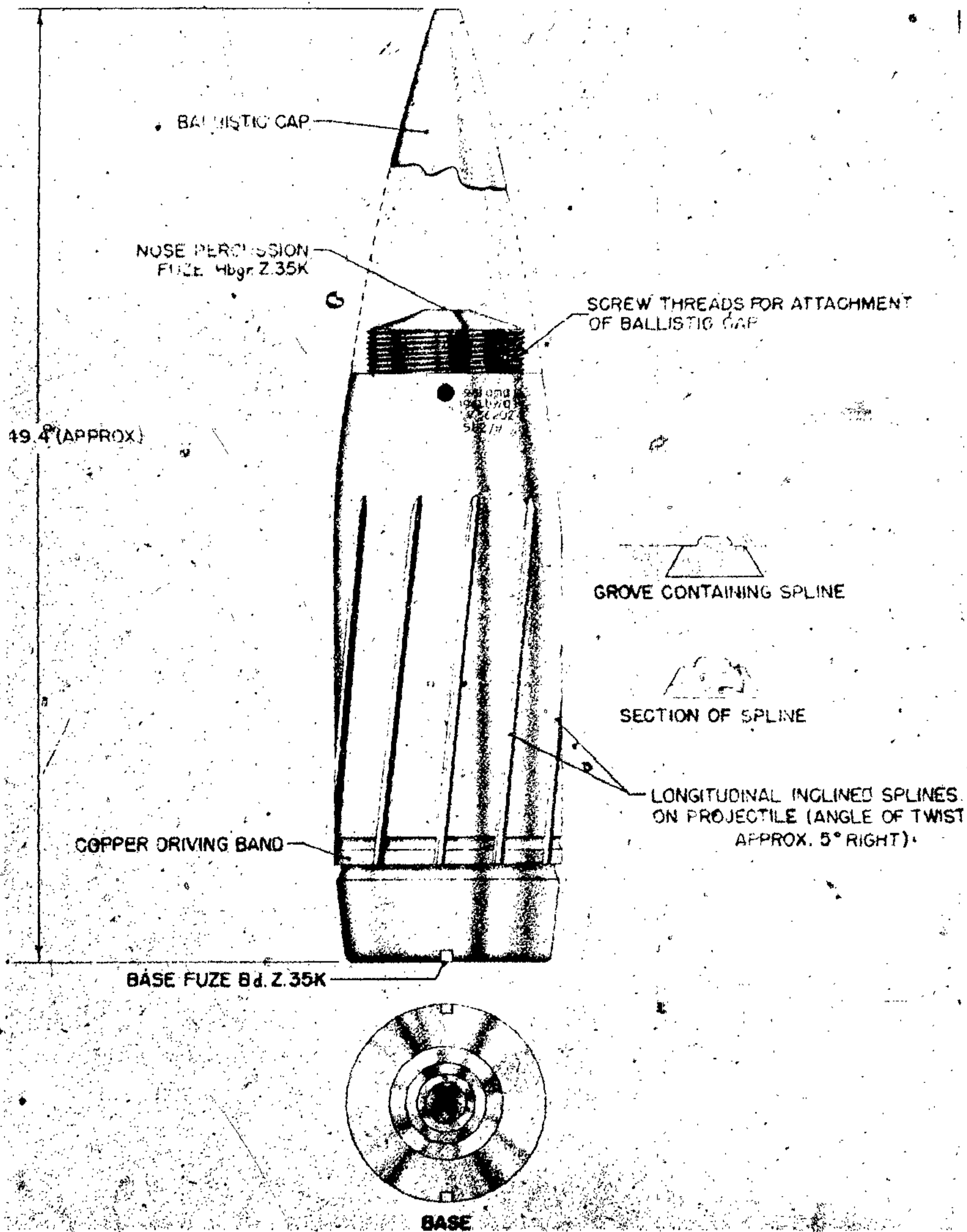
Figure 536—H. E. Projectile, Rifled, 280-mm, 28-cm
