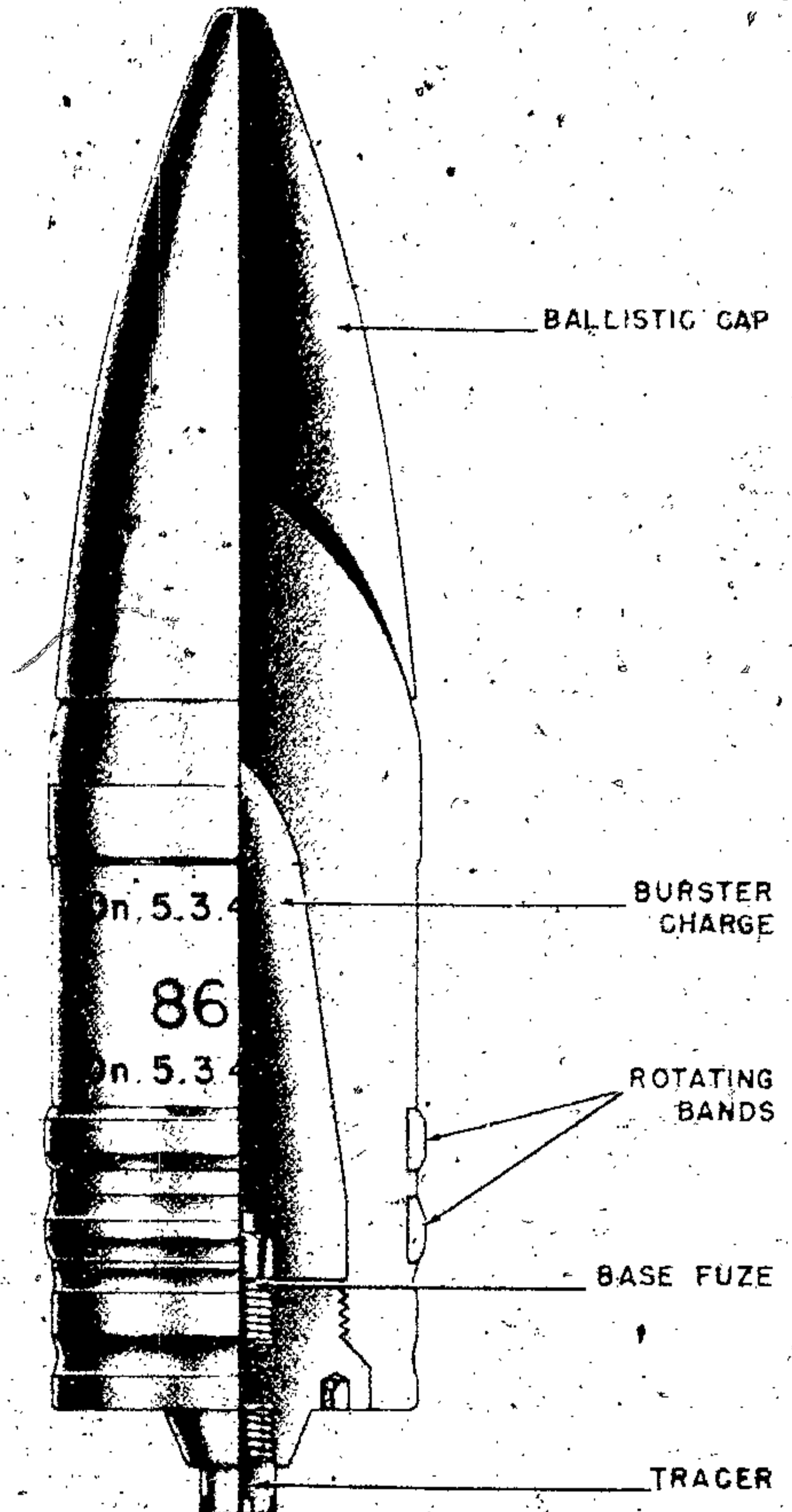
Figure 483—A. P. Projectile, 128-mm, 12.8-cm Pzgr. 43
