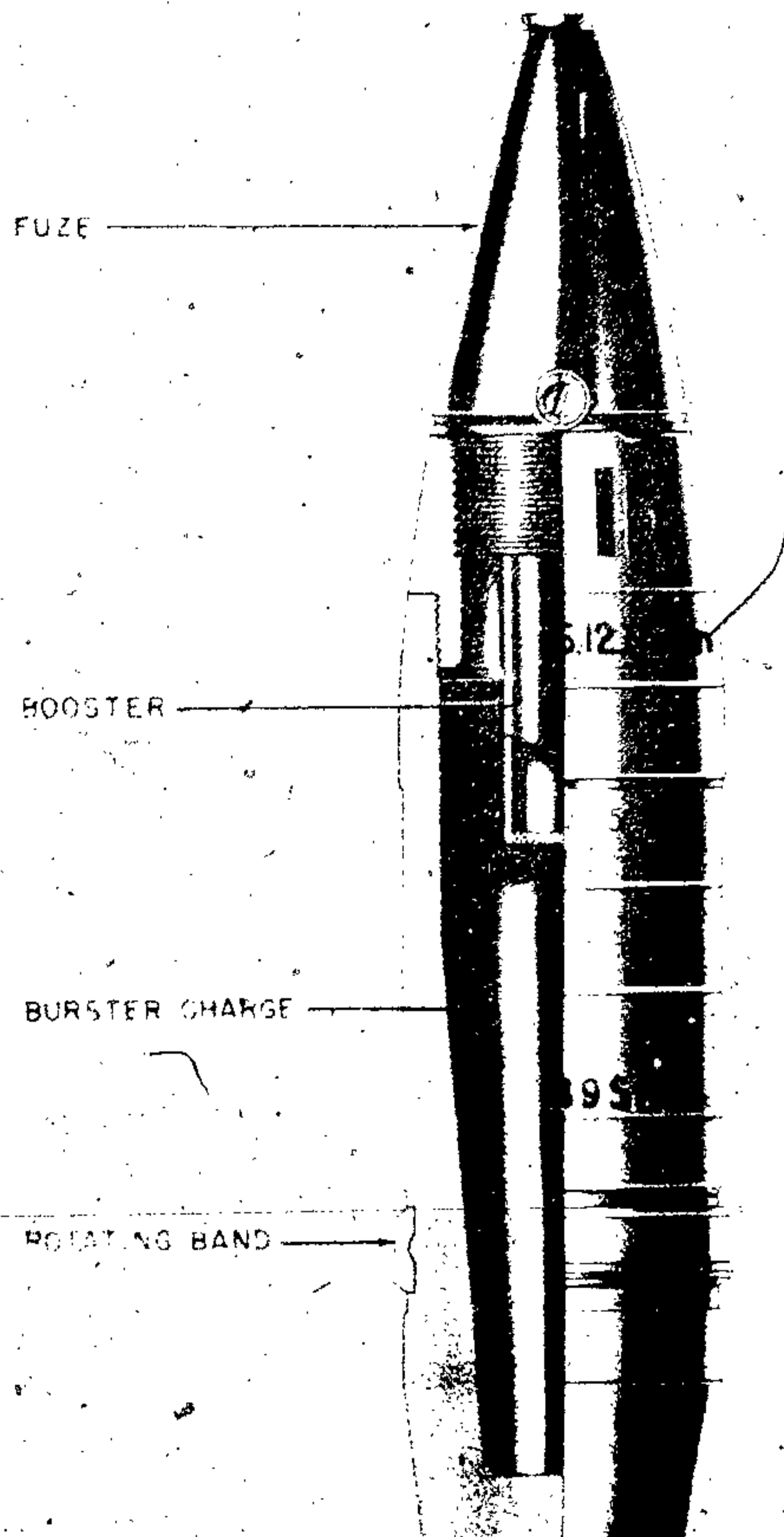
Figure 401—H. E. Projectile, 75-mm, 7.5-cm. K. Gr. Rot KPS
