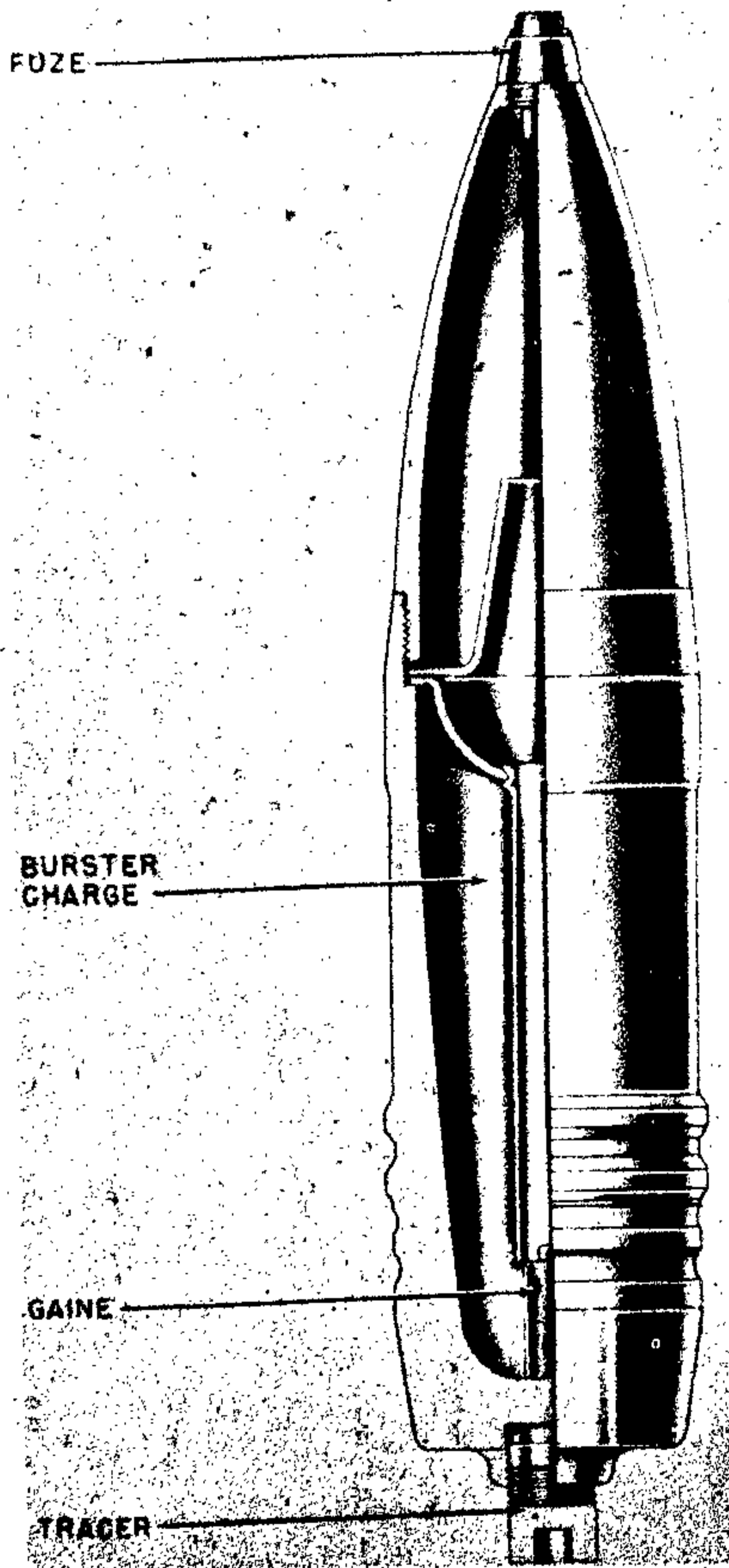
Figure 433—Hollow Charge Projectile for 88-mm Tank Gun, 8.8-cm Gr. 39 H.L.
