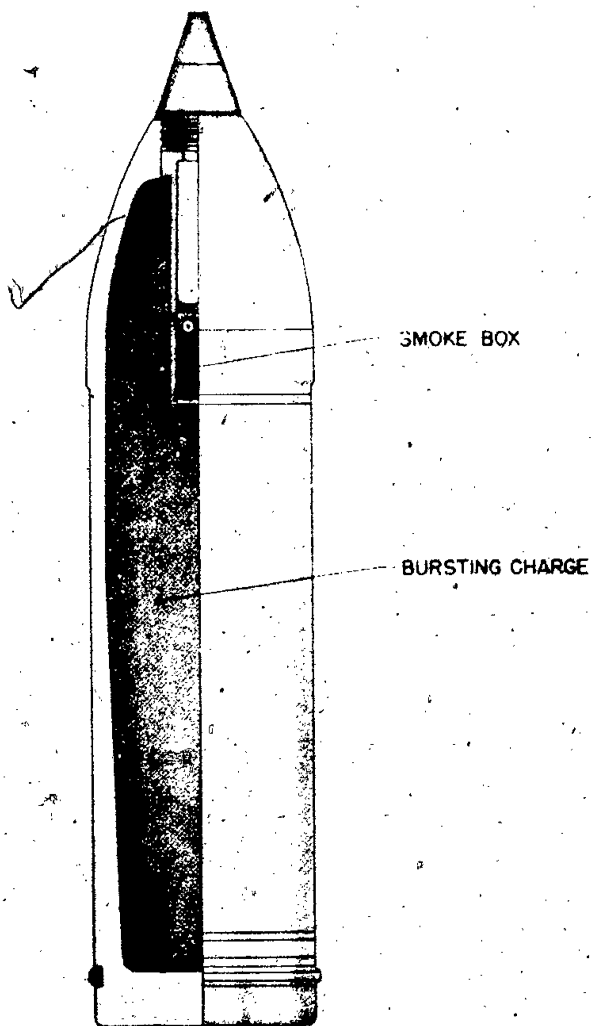
Figure 506—H. E. Projectile for Heavy Infantry Gun, 150-mm, 15-cm Jgr. 38
