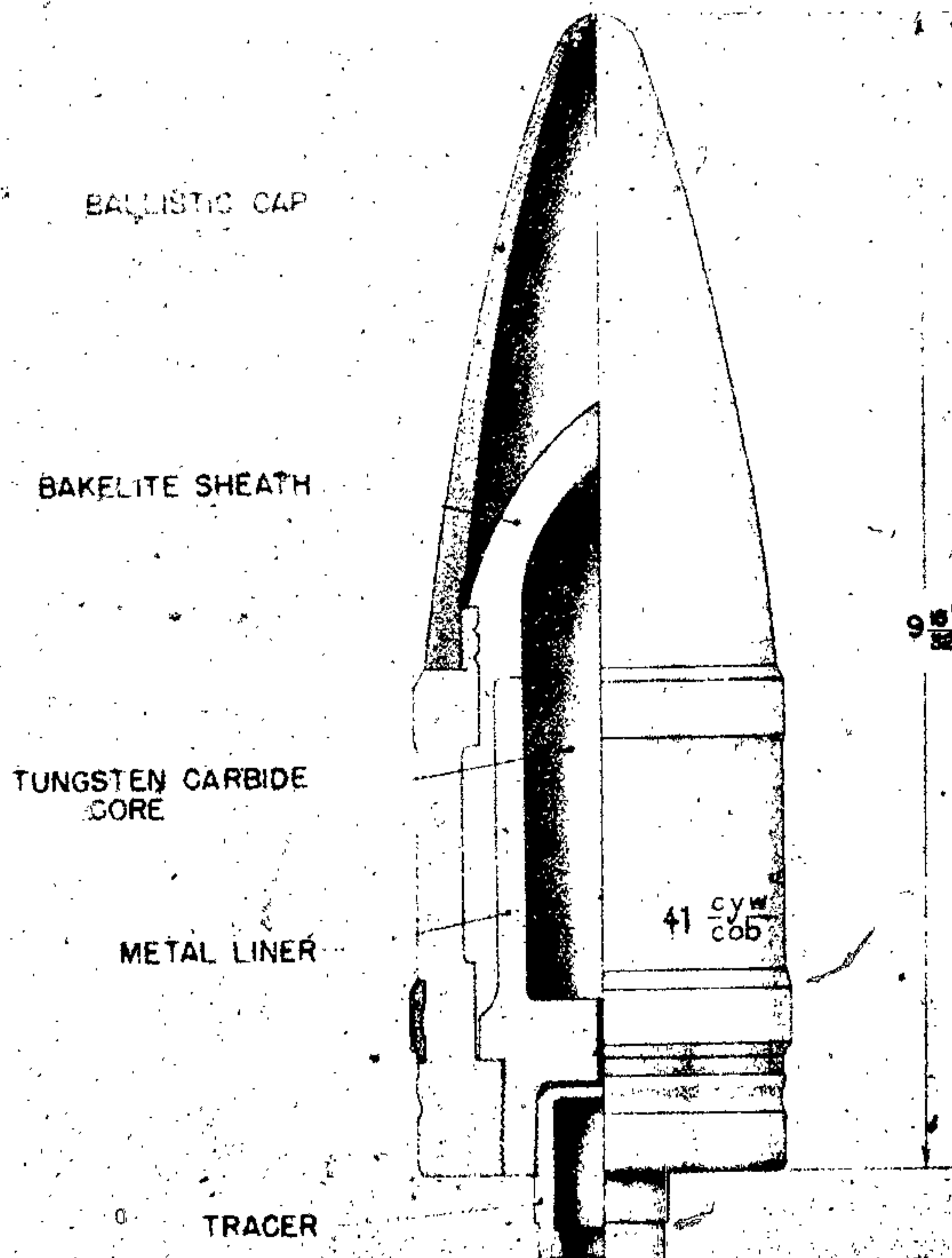
Figure 410—A. P. Projectile With Tungsten Carbide Core, 76.2-mm. 7.62-cm. Pzgr. Patr. 40 (r)
