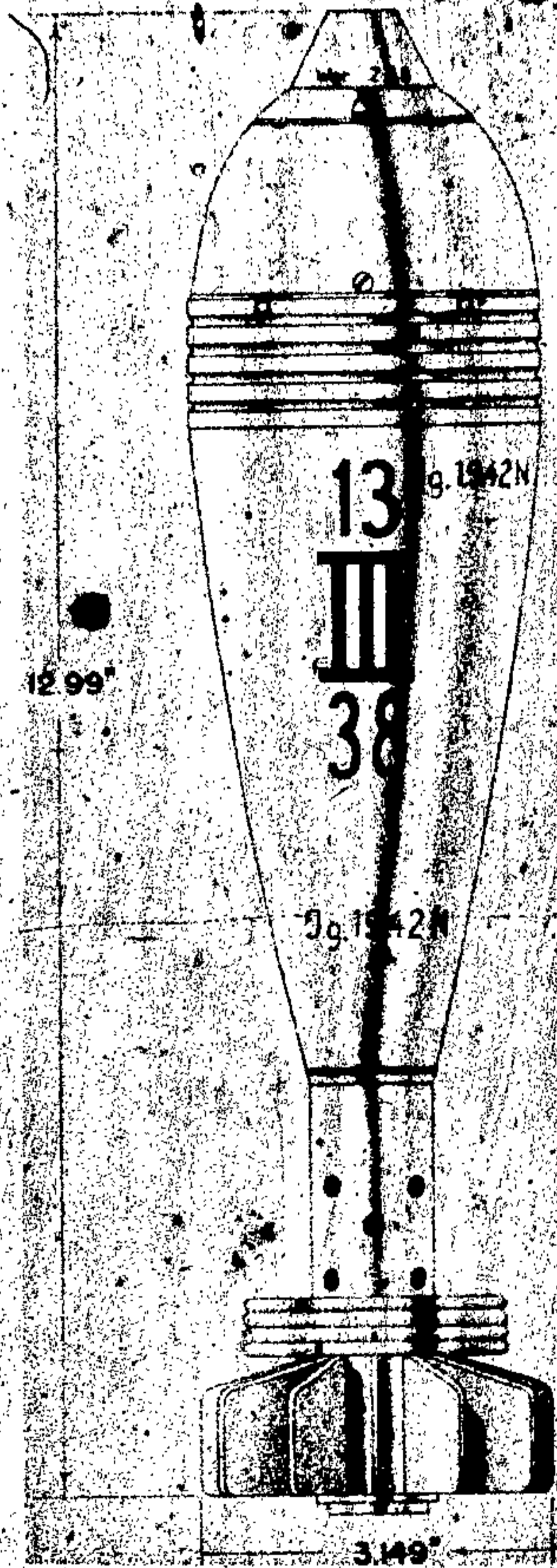
Figure 541—H. E. Mortar Projectile, Type 38, 80-mm, 8-cm Wgr. 38
