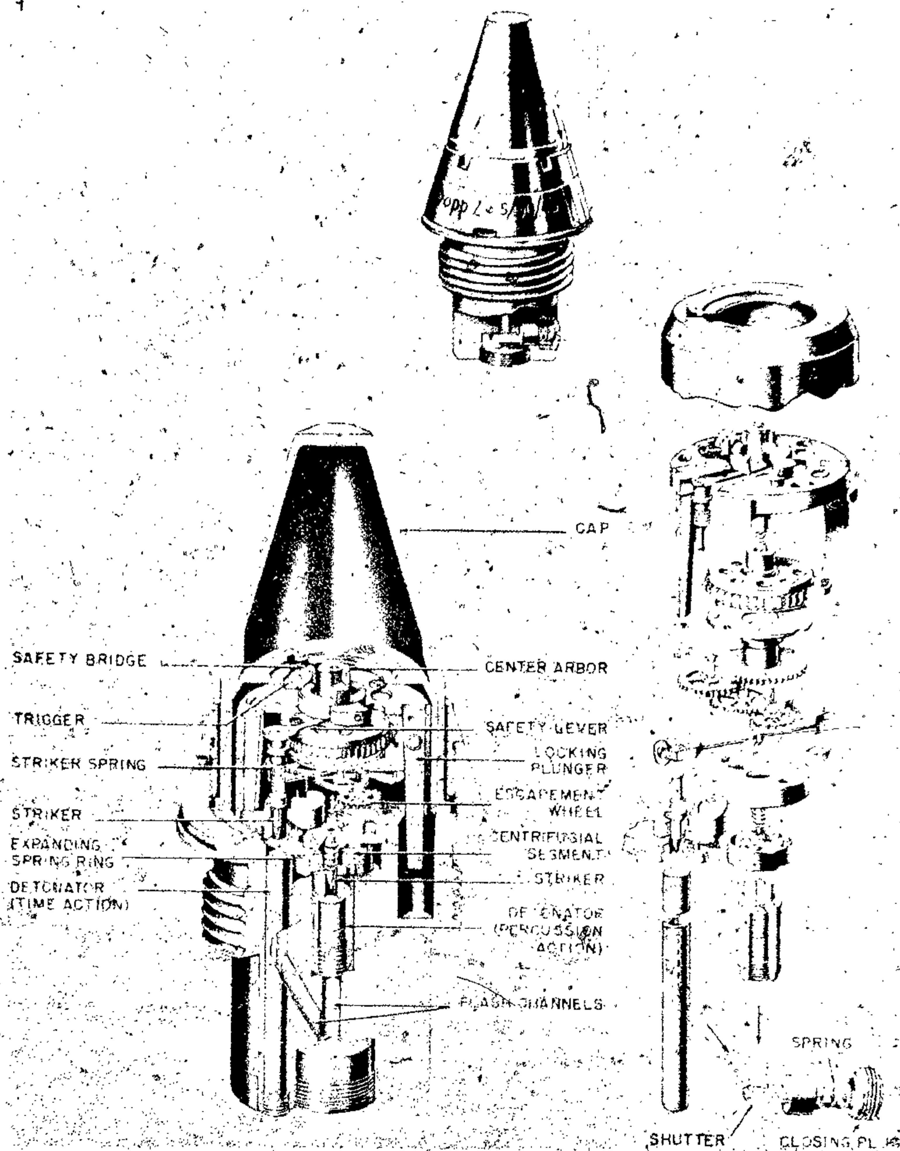
Figure 595A—Dopp. Z. S/90/45
