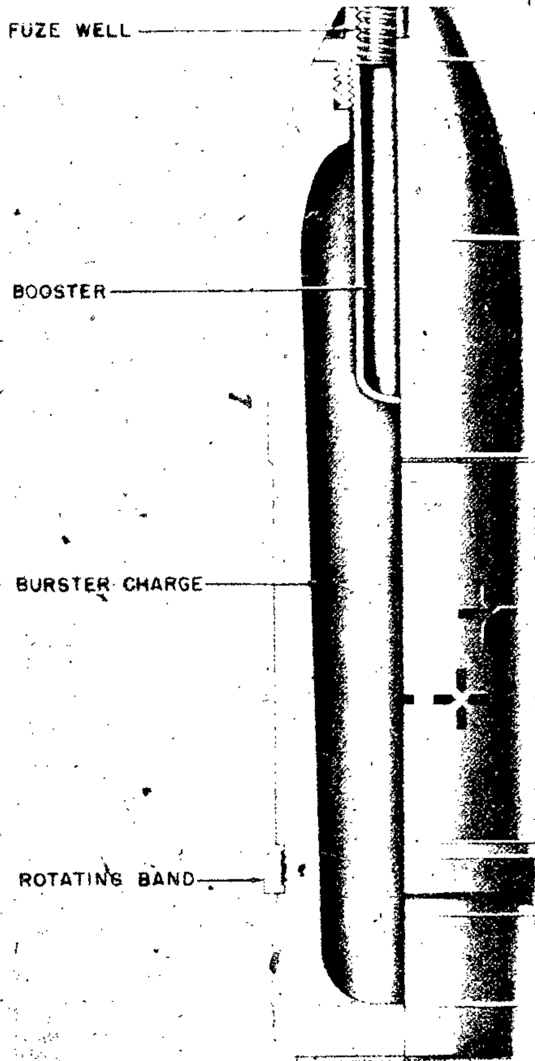
Figure 403—H. E. Projectile, 75-mm, 7.5-cm Sprgr. 264 (j)
