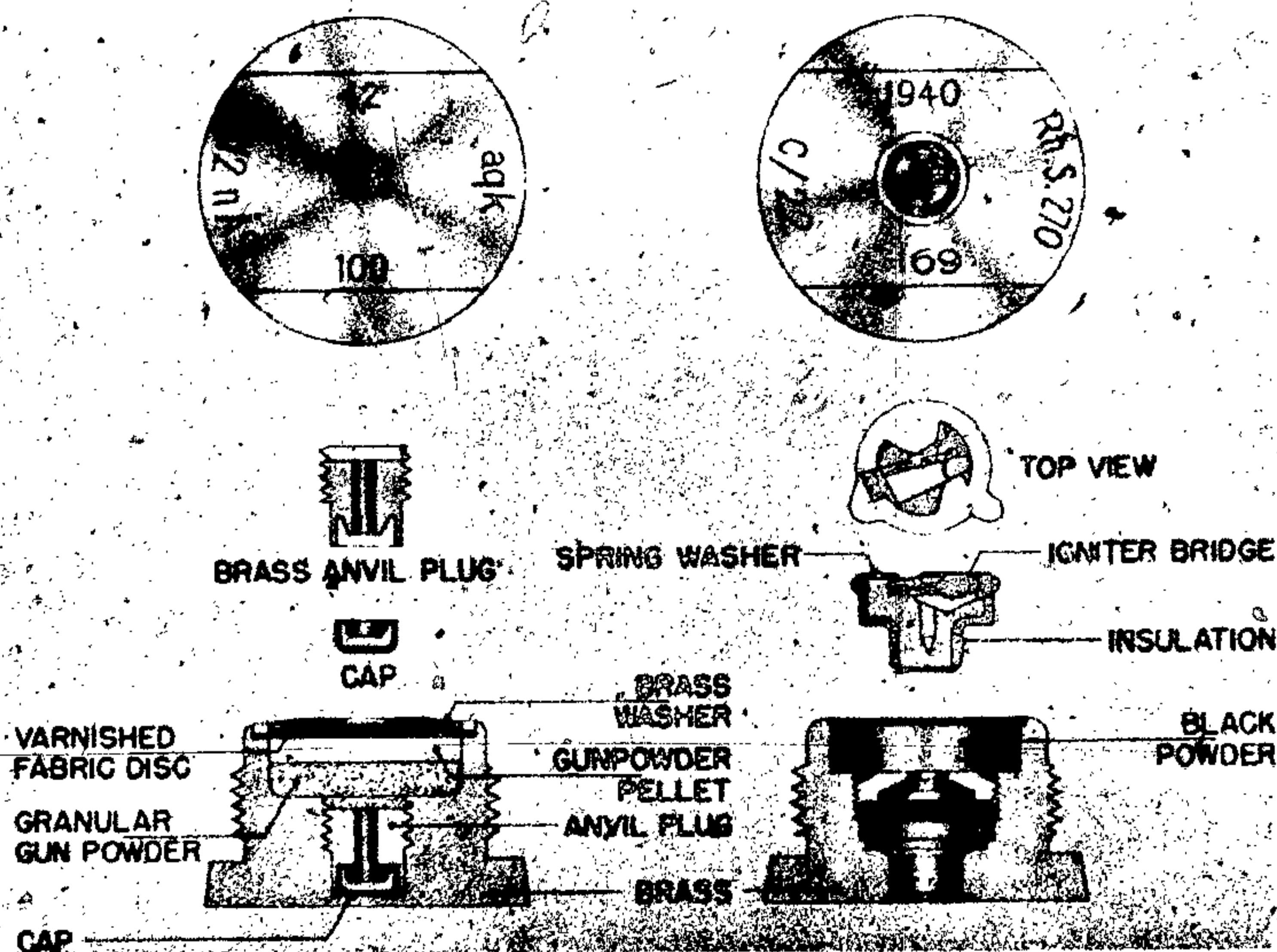
Figure 320—Electric Primers c/12nA and c/22
