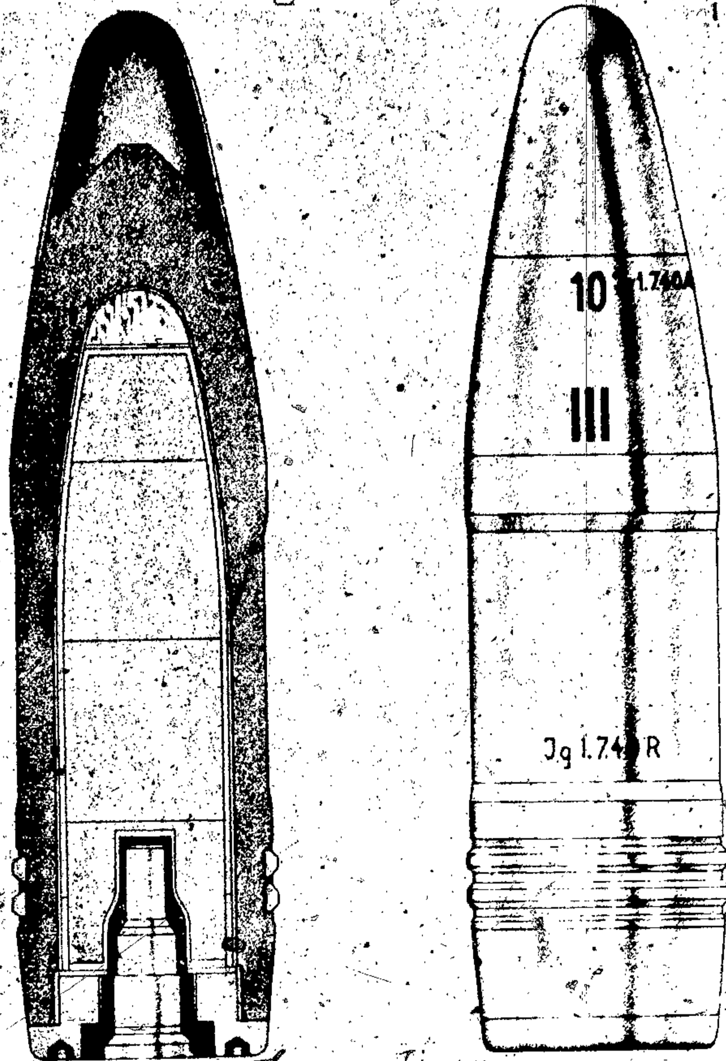
Figure 512—Anticoncrete Projectile, Type 19, 150-mm, 75-cm Gr. 19 Be.
