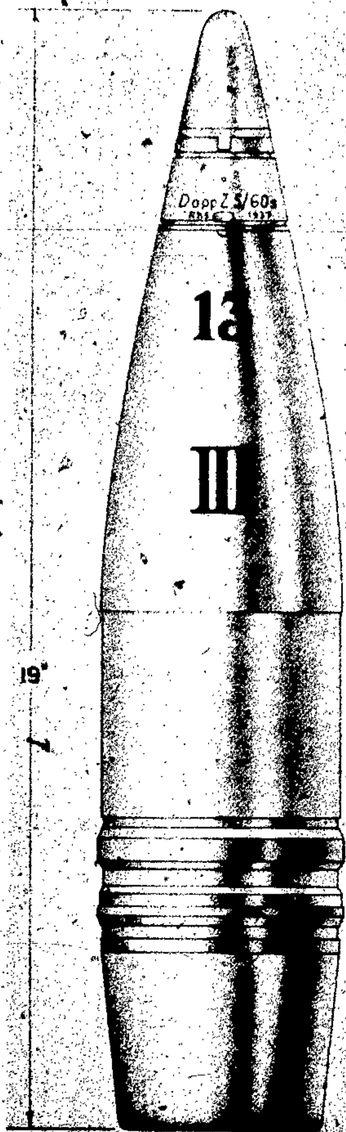
Figure 478—H. E. Projectile, Type 19, 105-mm Gr., 19 Kz. 13
