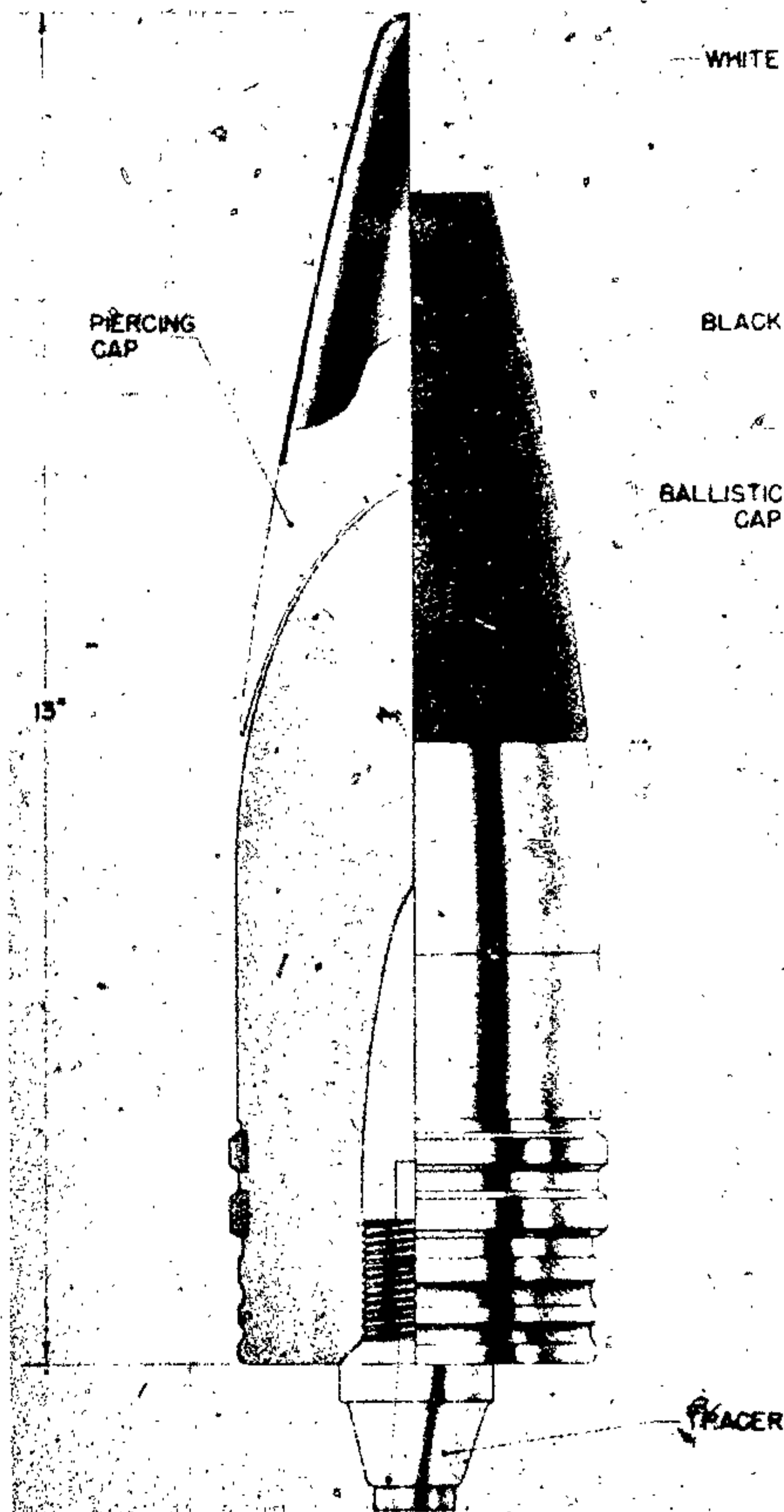
Figure 426—A. P. Projectile for 88-mm Antitank Gun, 8.8-cm Pzgr. Patr. 41
