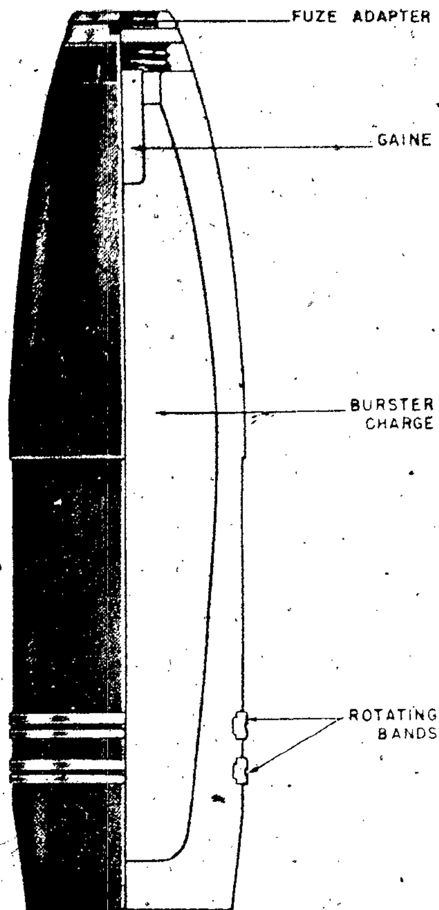
Figure 523—H. E. Projectile, 155-mm, 15.5-cm Gr. 421 (f)
