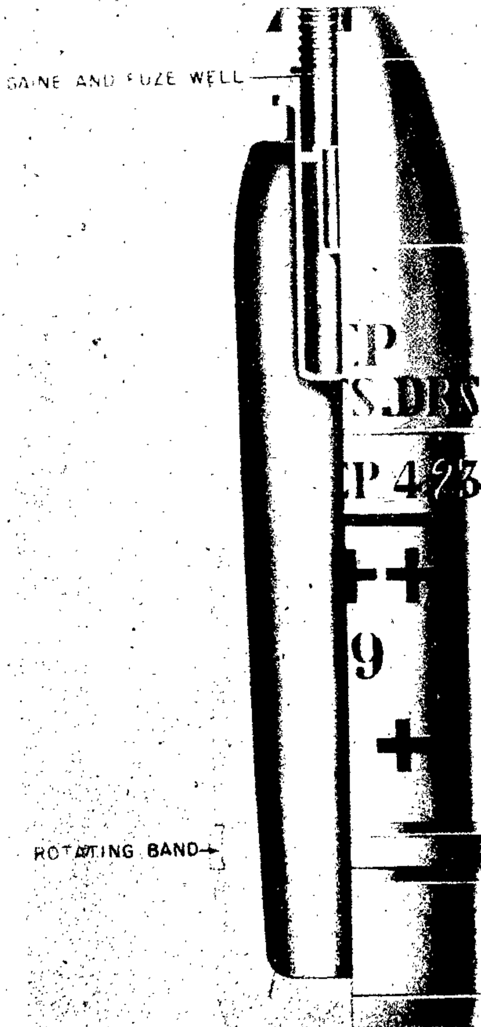
Figure 400—H. E. Shell for 75-mm Gun, 7.5-cm Sprgr. 1900/15 (f)
