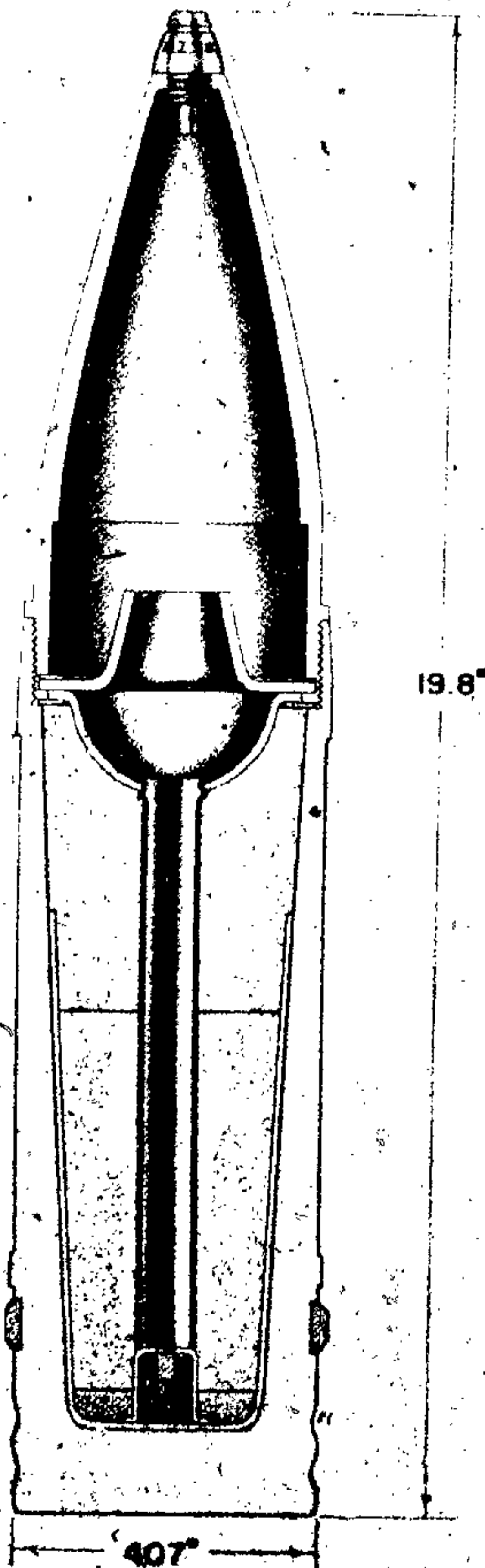
Figure 474.—Hollow Charge Projectile, Type C, 105-mm, 10-cm Gr. 39 Rot HL/C
