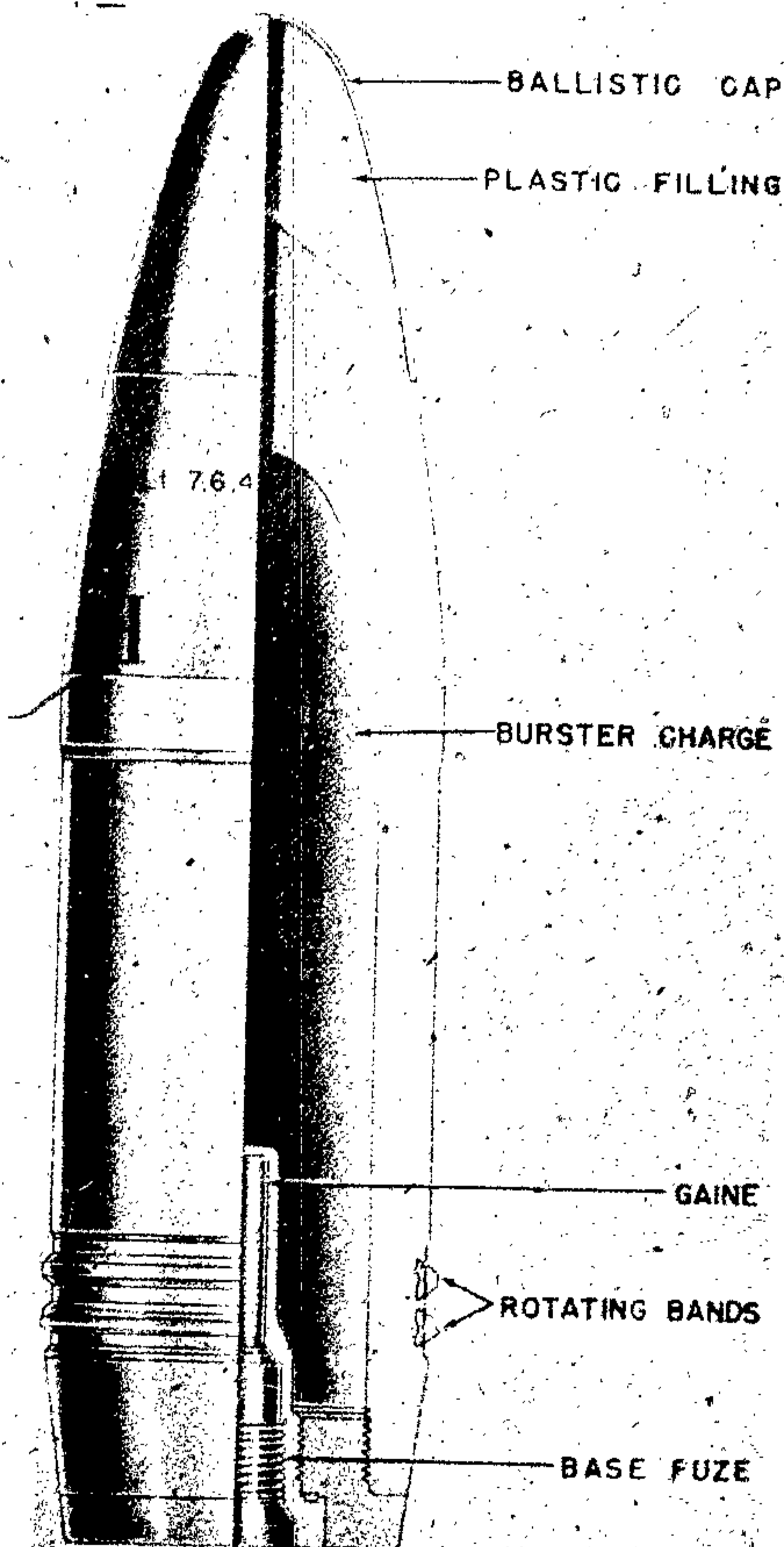
Figure 487—Anticoncrete Projectile for 150-mm Gun, 15-cm Gr. 19 Rot Be.
