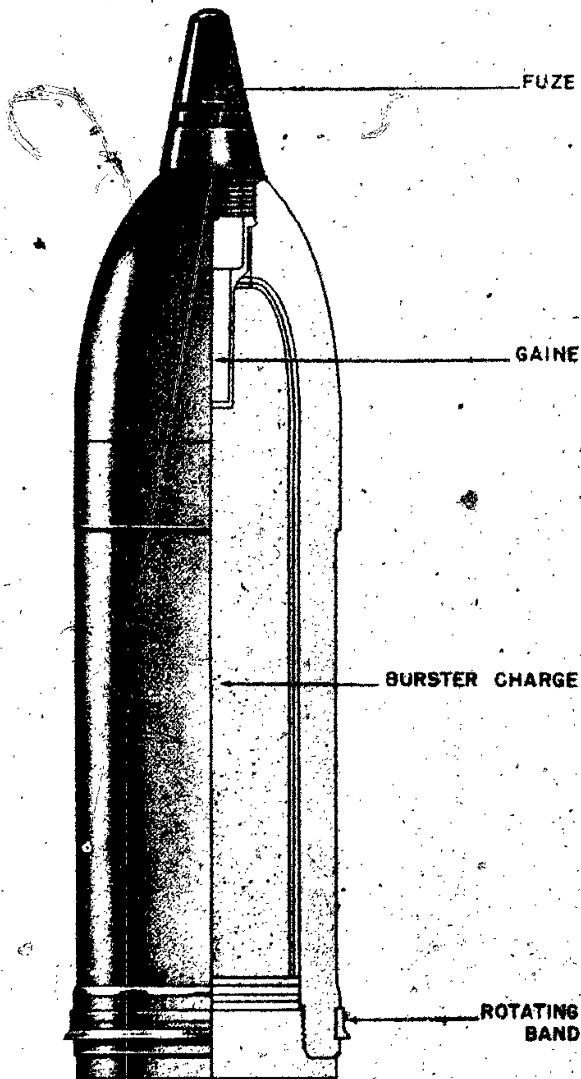
Figure 503—H. E. Projectile, Type 18, 150-mm, 15-cm Gr. 18
