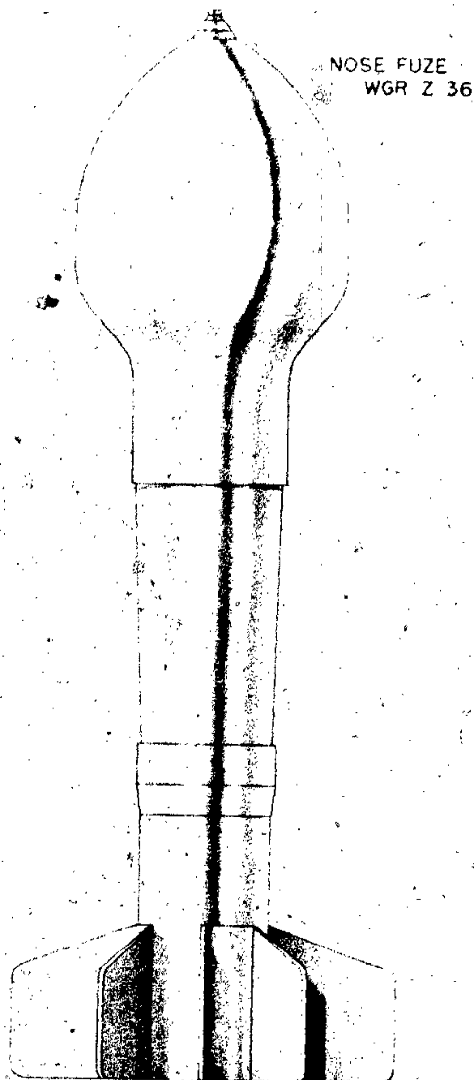
Figure 549—H. E. Mortar Projectile, 380-mm, 38-cm Wgr. 40
