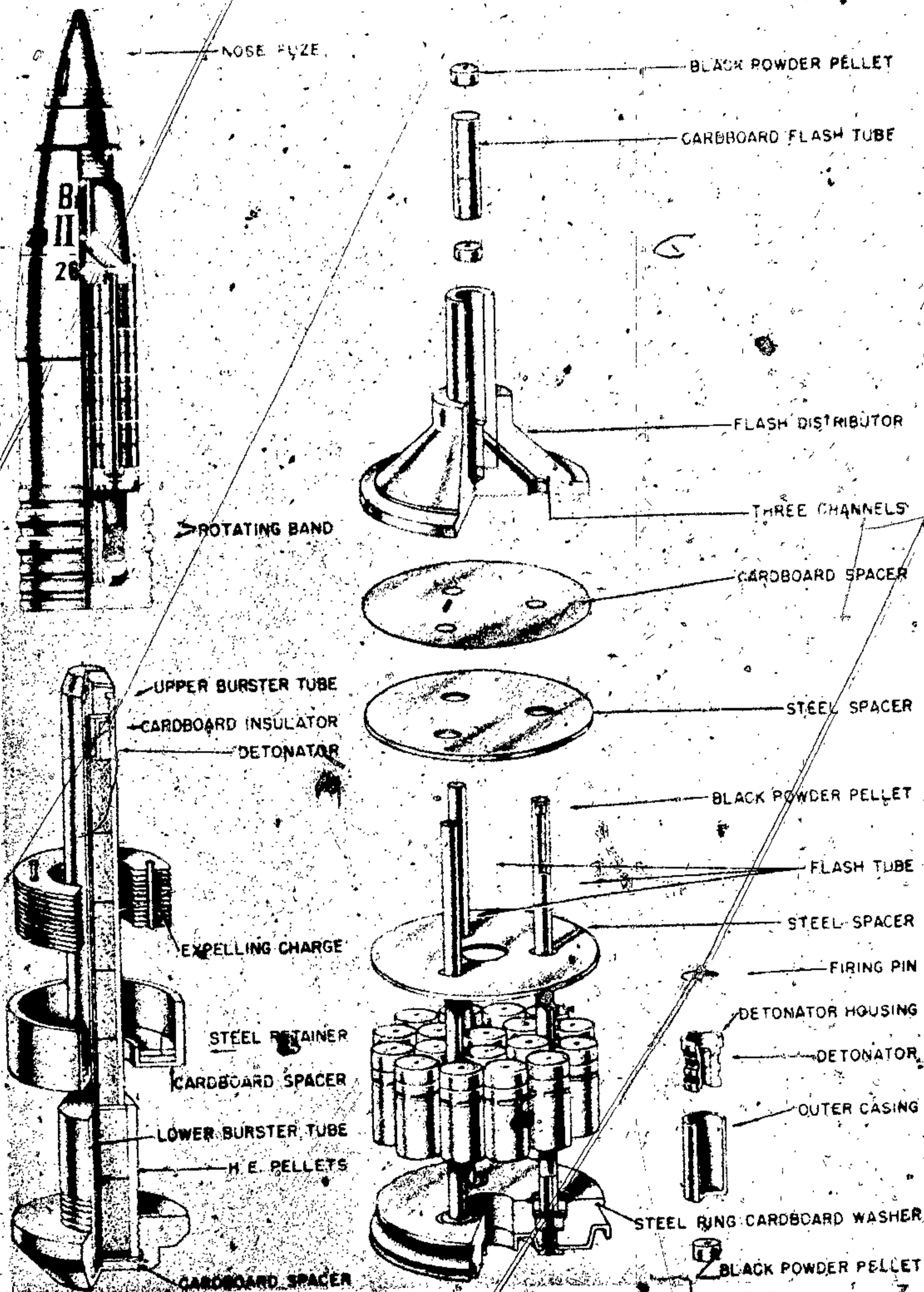
Figure 439—Incendiary Shrapnel Shell for 88-mm A. A. G. H. 8.8-cm Gr. Br. Schr. Flak
