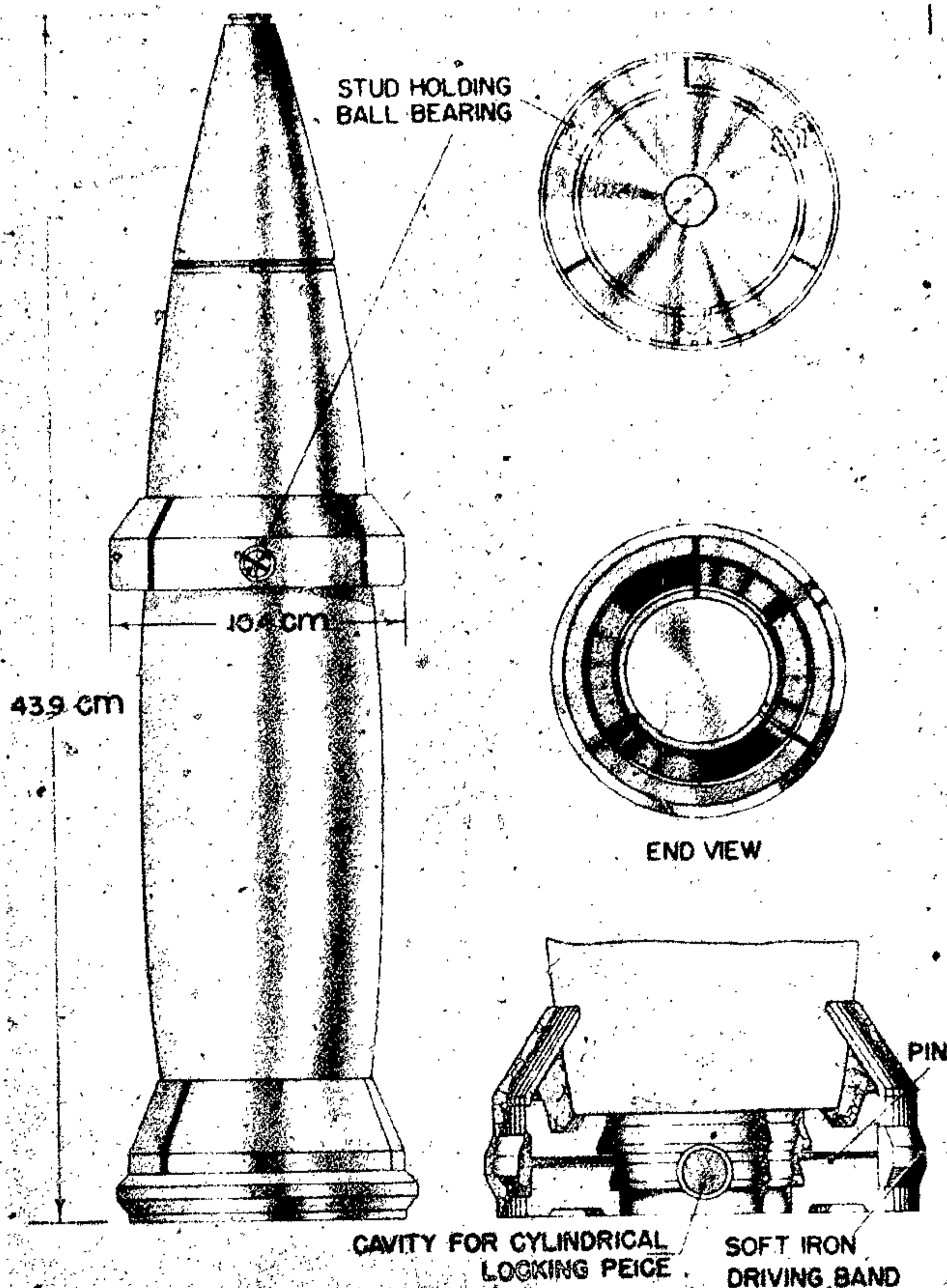
Figure 336—H. E. Projectile with Disintegrating Bands, 105-mm
