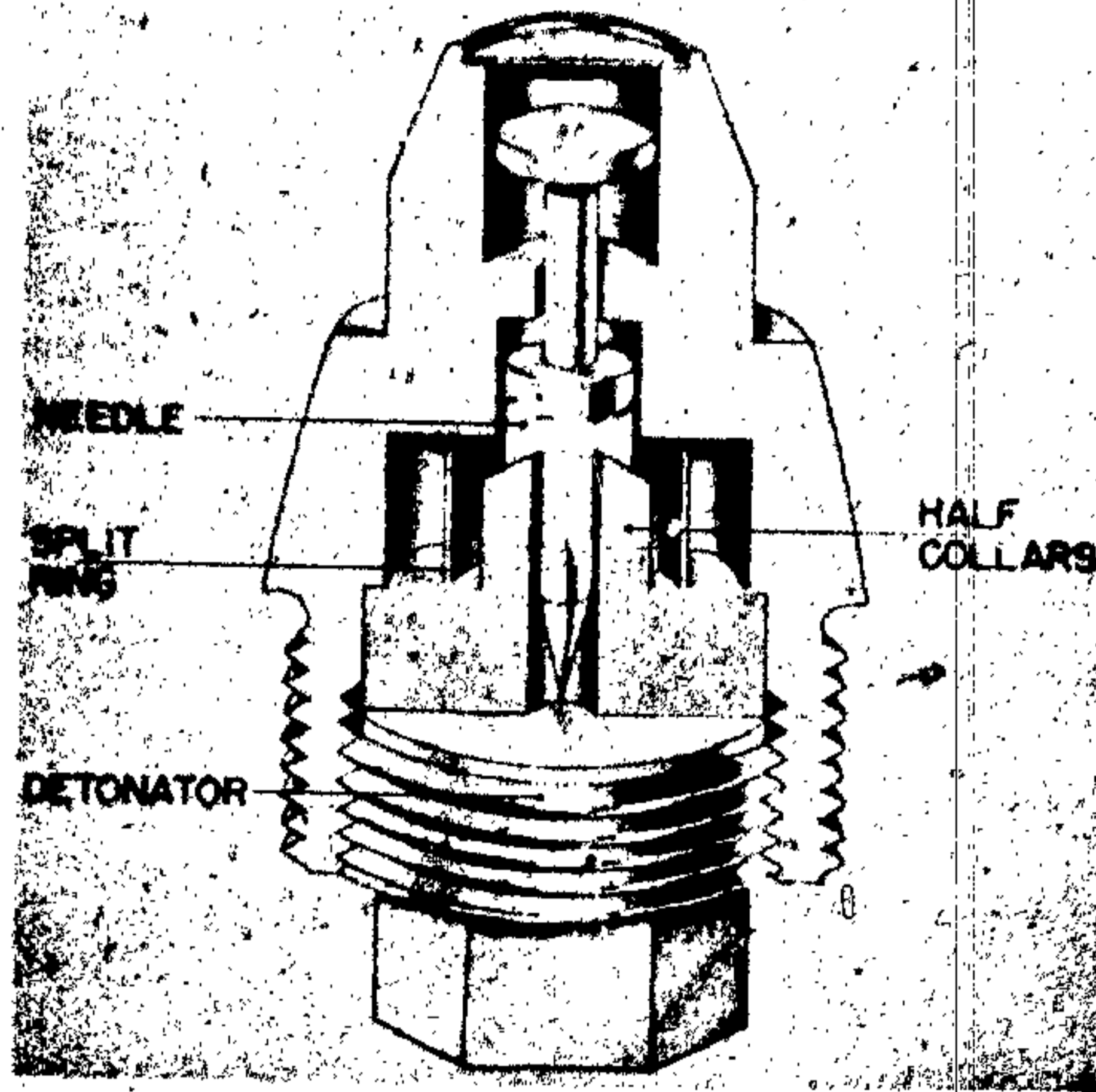
Figure 557—A. Z. 1551 and 1552
