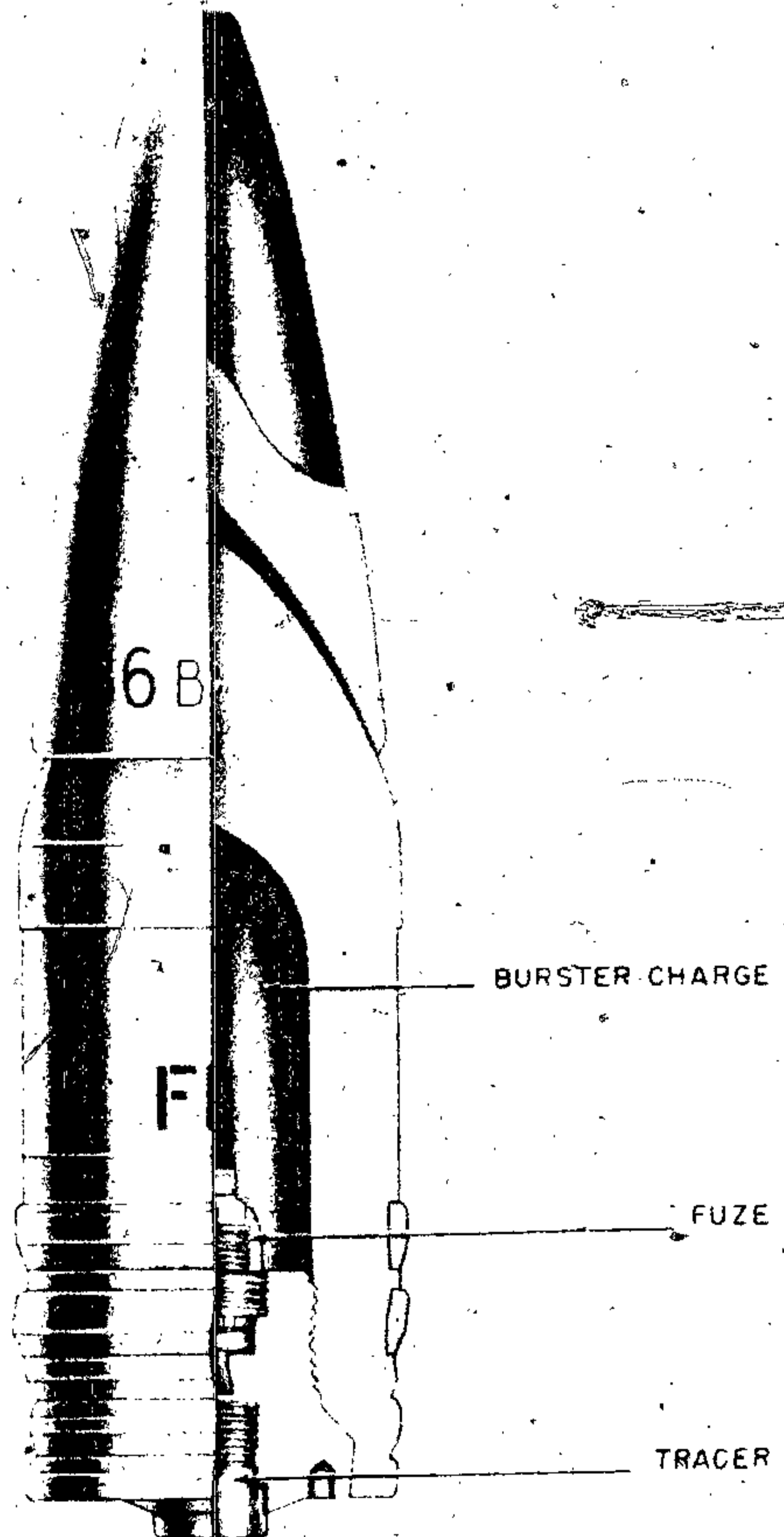
Figure 452—A. P. Projectile, 105-mm, 10-cm Pxgr. Rot FES
