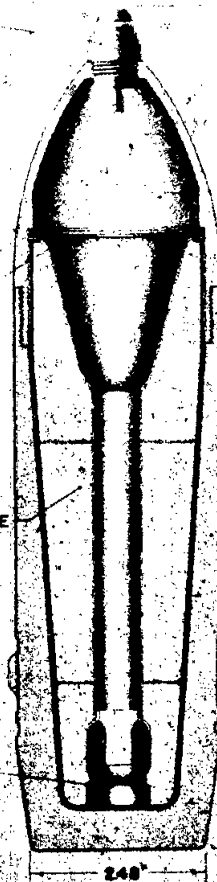
Figure 374—Hollow Charge Projectile for Tank Gun, Type B, 75-mm, 7.5-cm Gr. Patr. KwK. (H.L/B)
