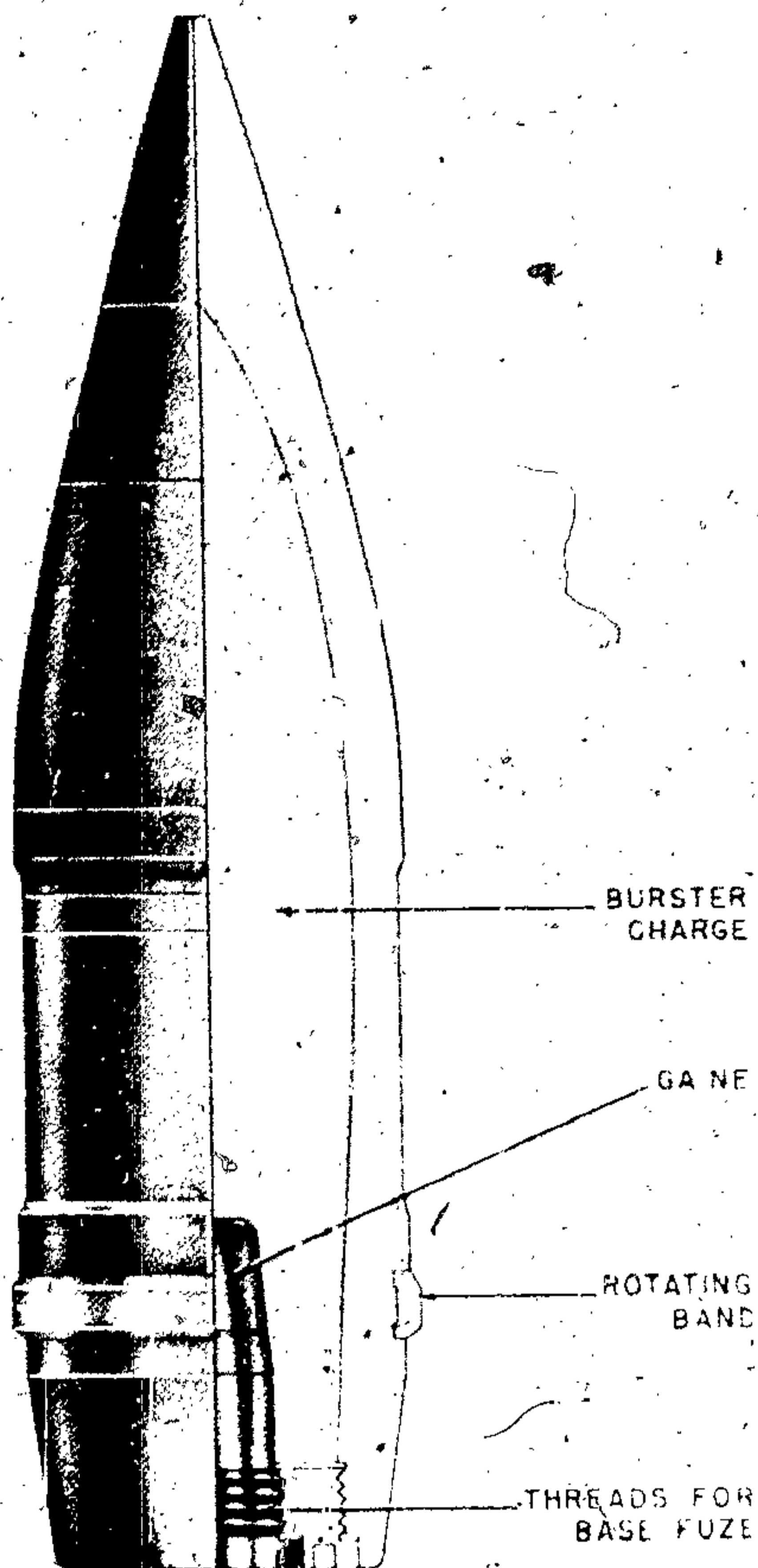
Figure 517—Anticoncrete (H. E.) Projectile 152-mm, 15.2-cm Gr. 434 Be. (r)
