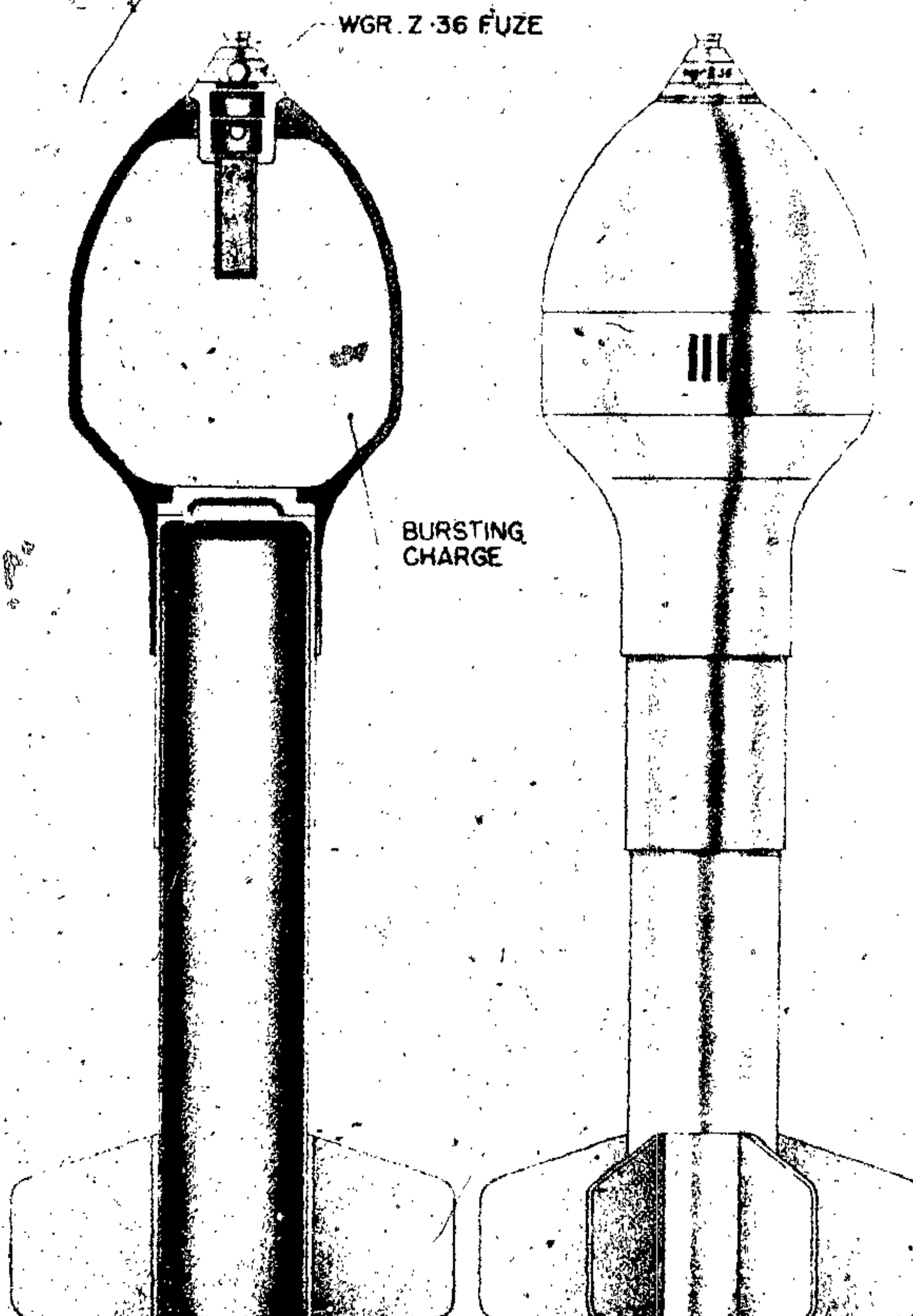
Figure 548—H. E. Mortar Projectile, 200-mm, 20-cm Wgr. 40
