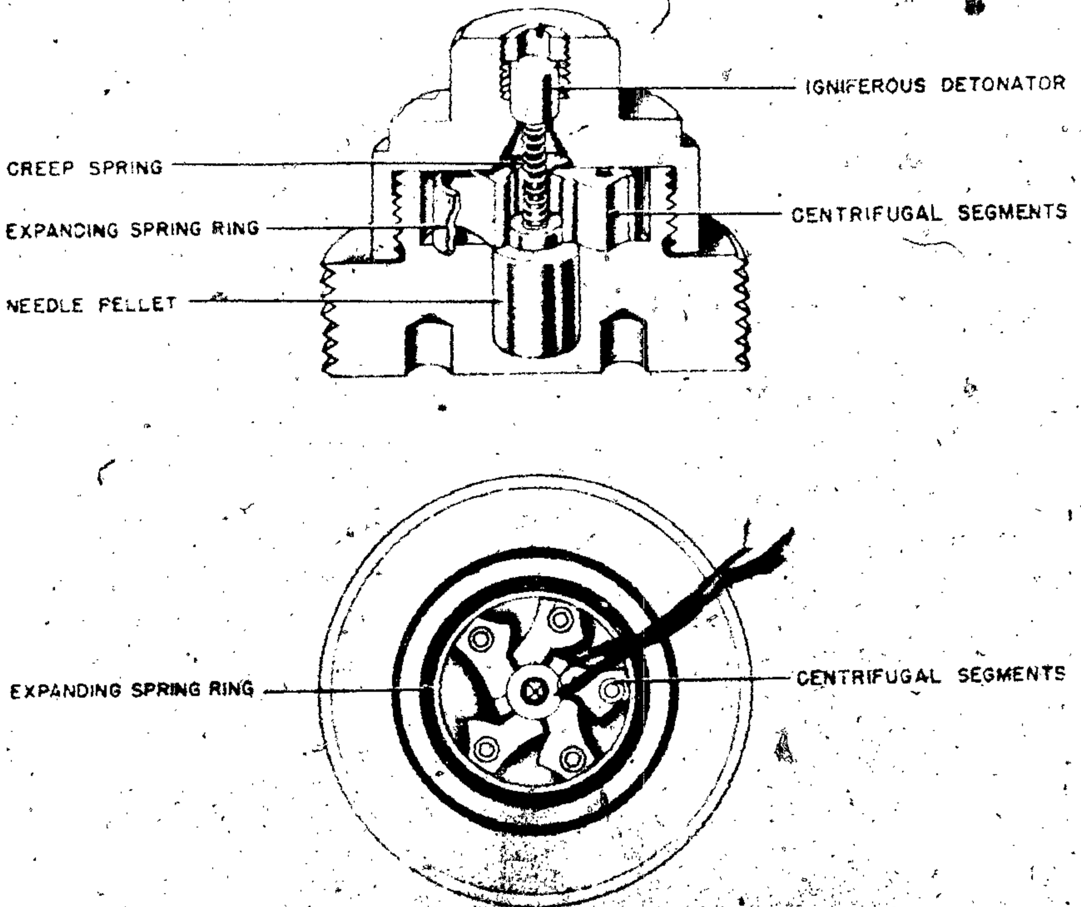
Figure 612—Bd. Z. DOV
