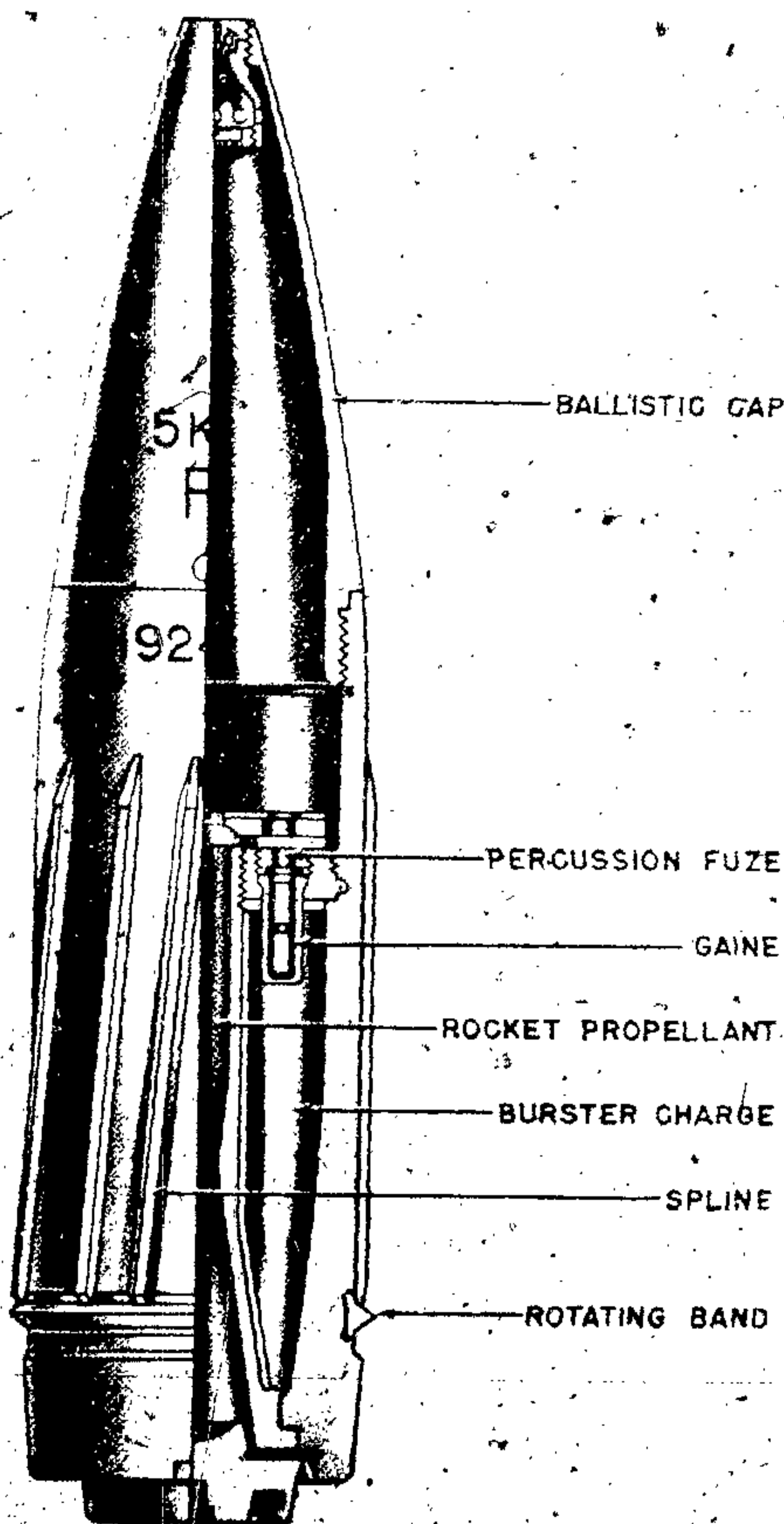
Figure 537—H. E. Rocket Assisted Projectile for 280-mm R. R. Gun, 28-cm R. G. 4331
