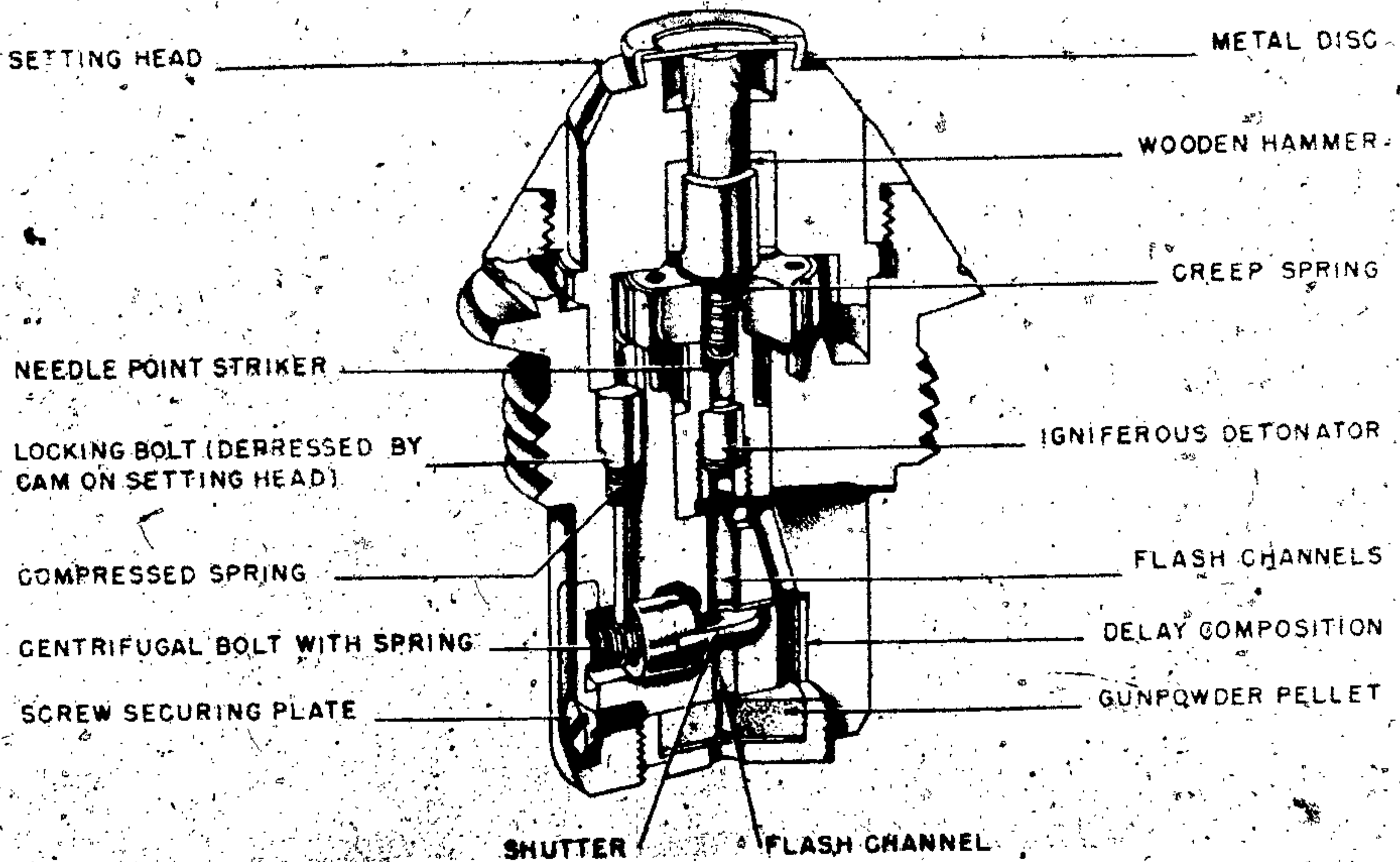
Figure 578—A. Z. 23 umg
