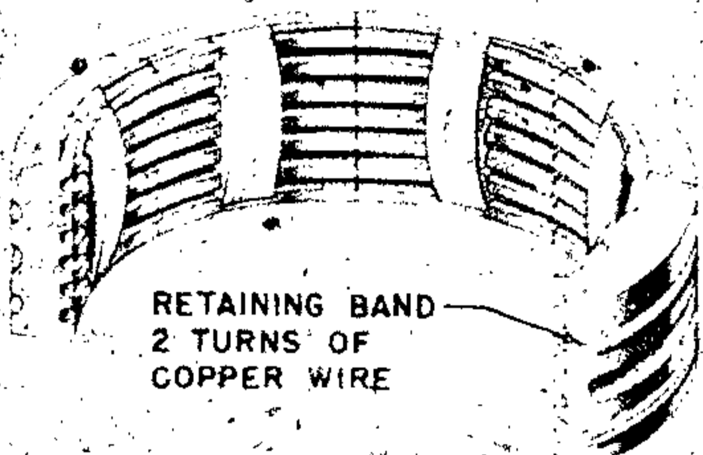
REAR DISCARDING SABOT ELEMENT (5 SEGMENTS OF 8)
