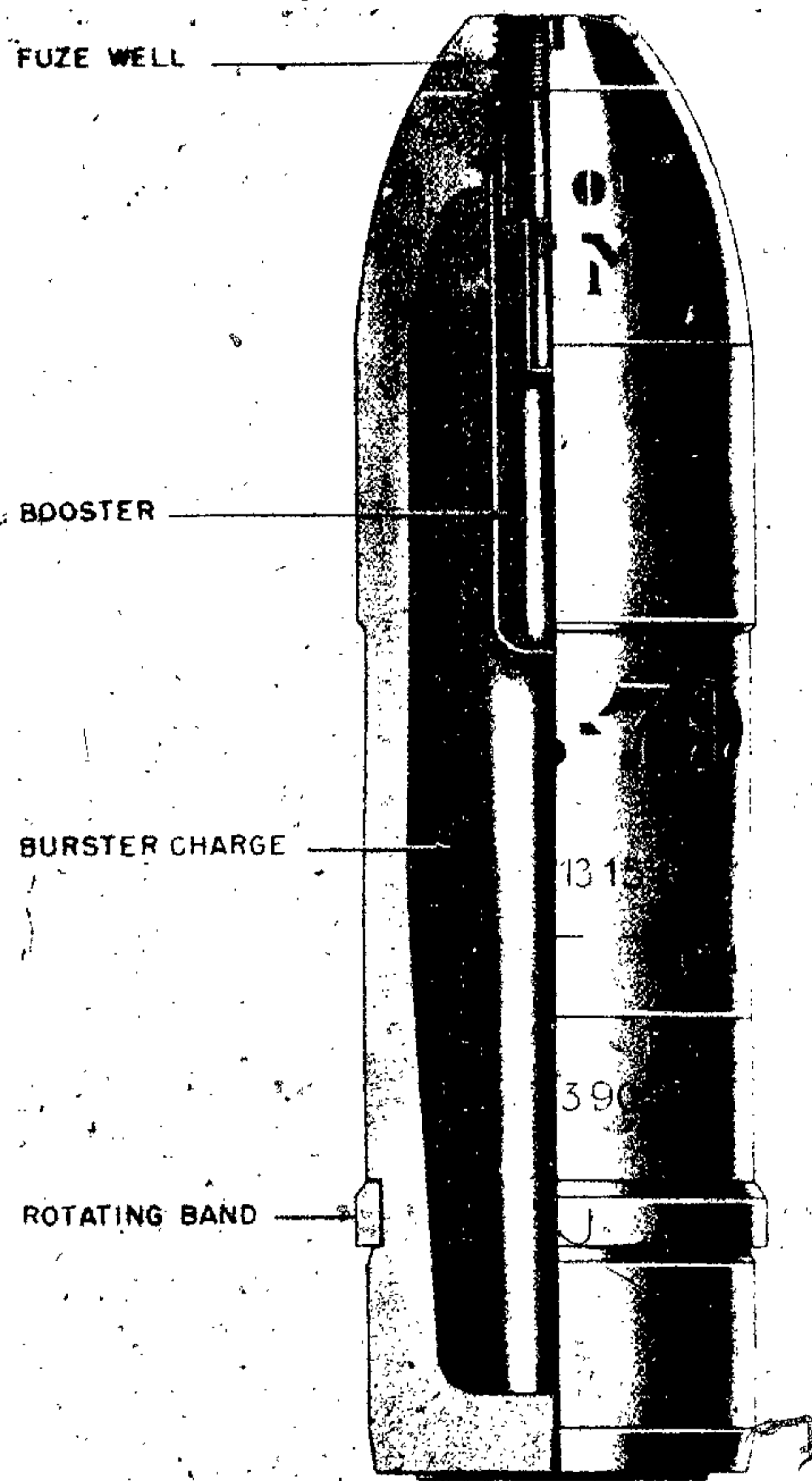
Figure 402—H. E. Projectile, 75-mm, 7.5-cm Sprgr. 240/2 (b)
