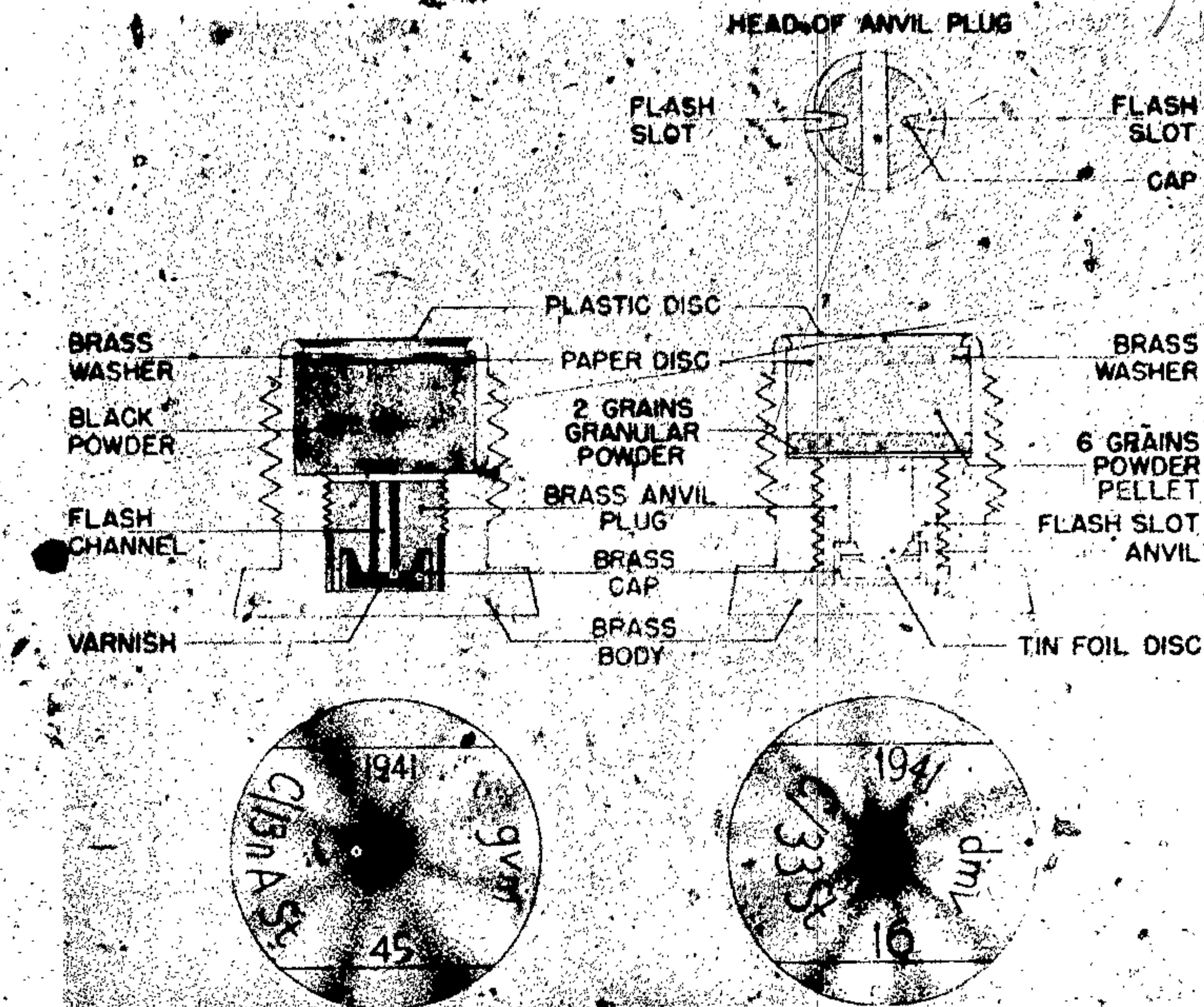
Figure 321—Percussion Primers c/13nA and c/33
