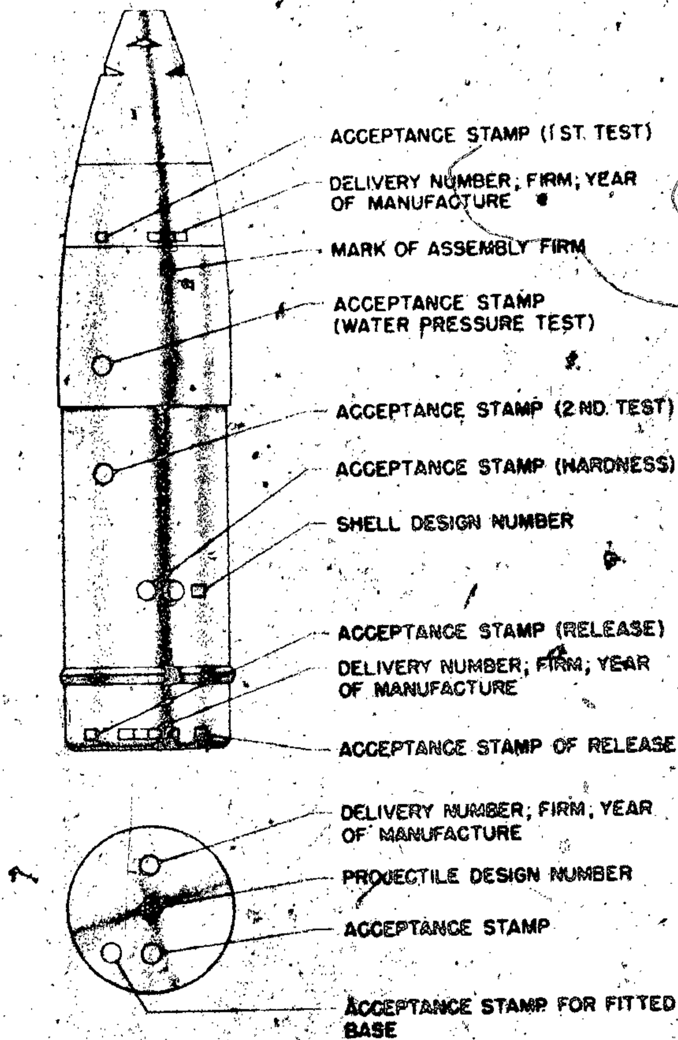
Figure 317—Projectile Stampings
