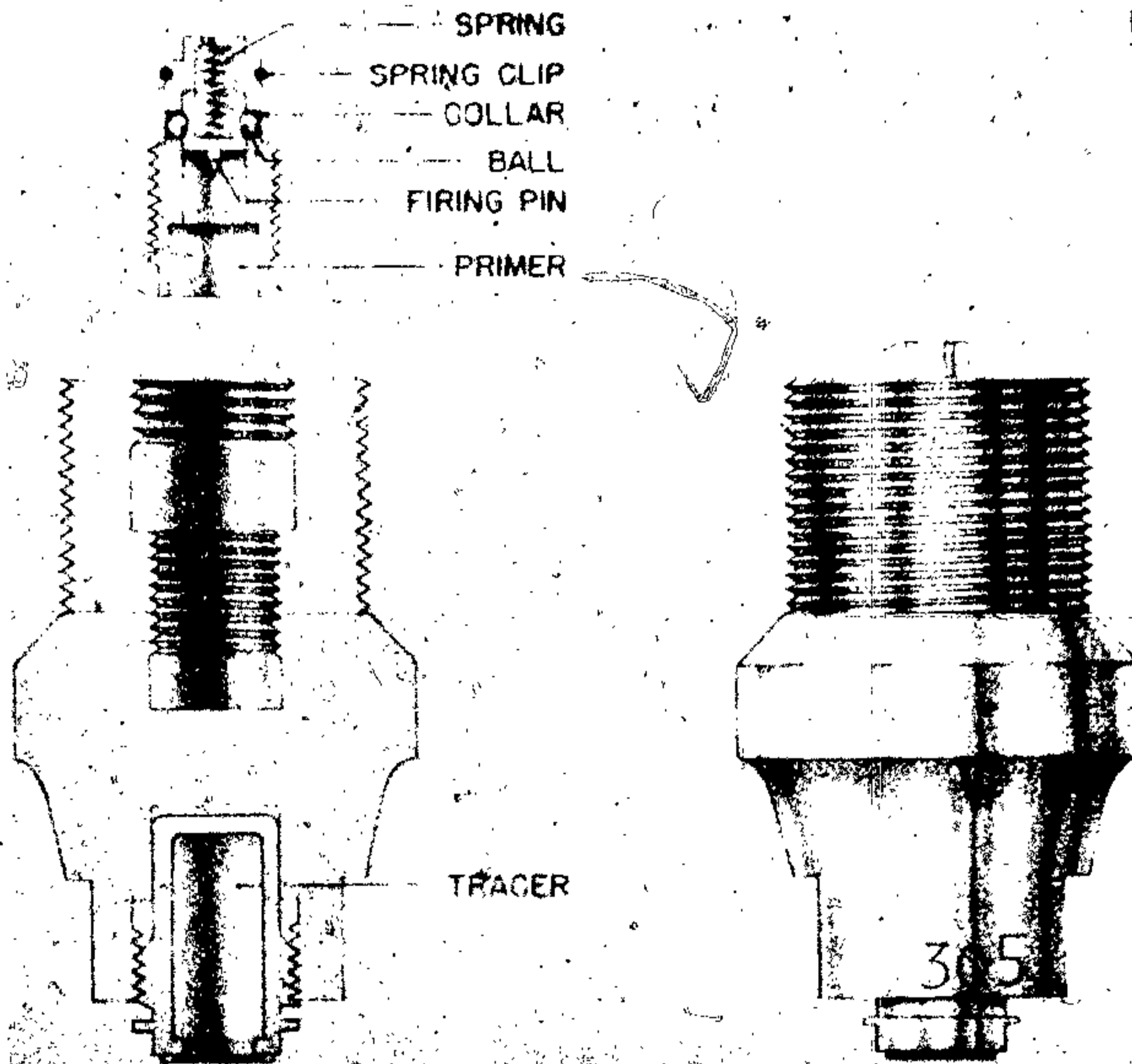
Figure 609—Bd. Z. for 8.8-cm Pzgr.
