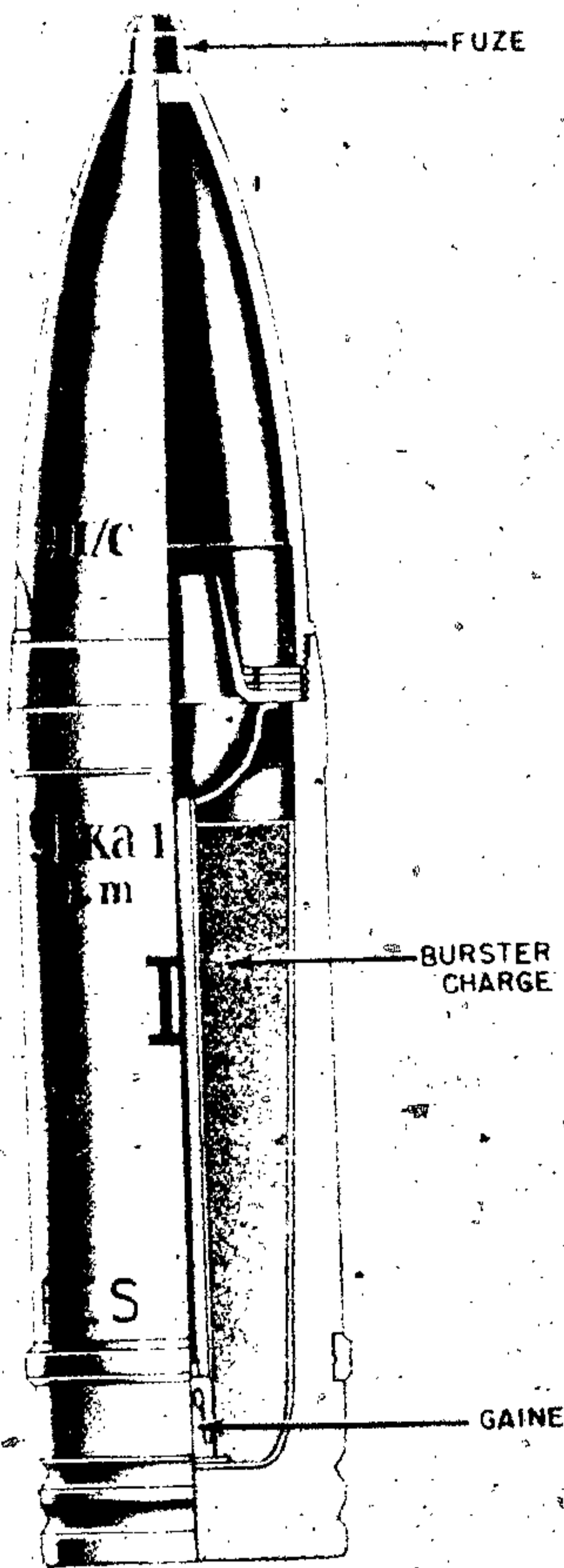
Figure 451—Hollow Charge Projectile for 105-mm Howitzer, 10.5-cm K. HL/C Granate 39 FES
