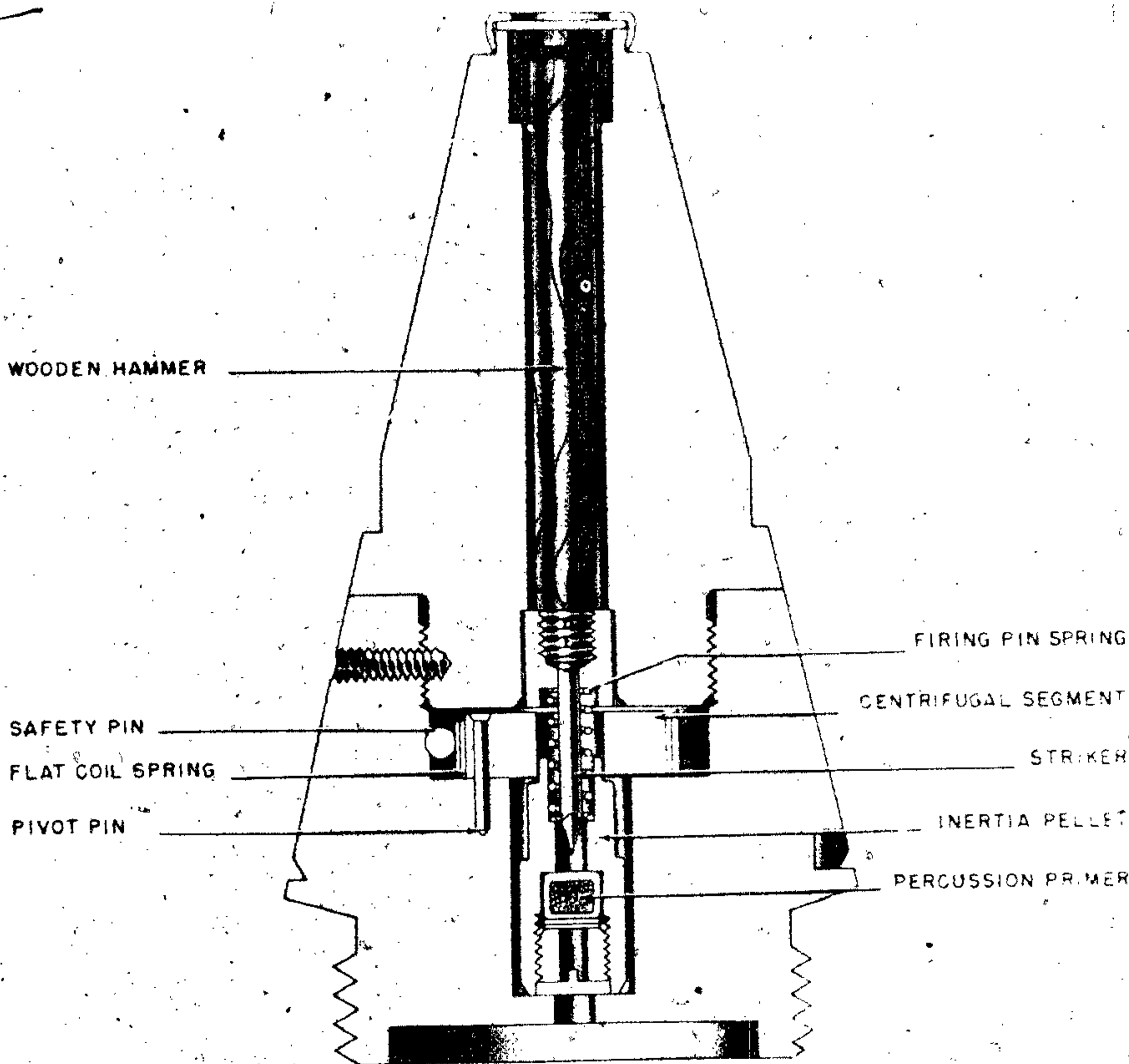
Figure 577C—A. Z. 23 Nb
