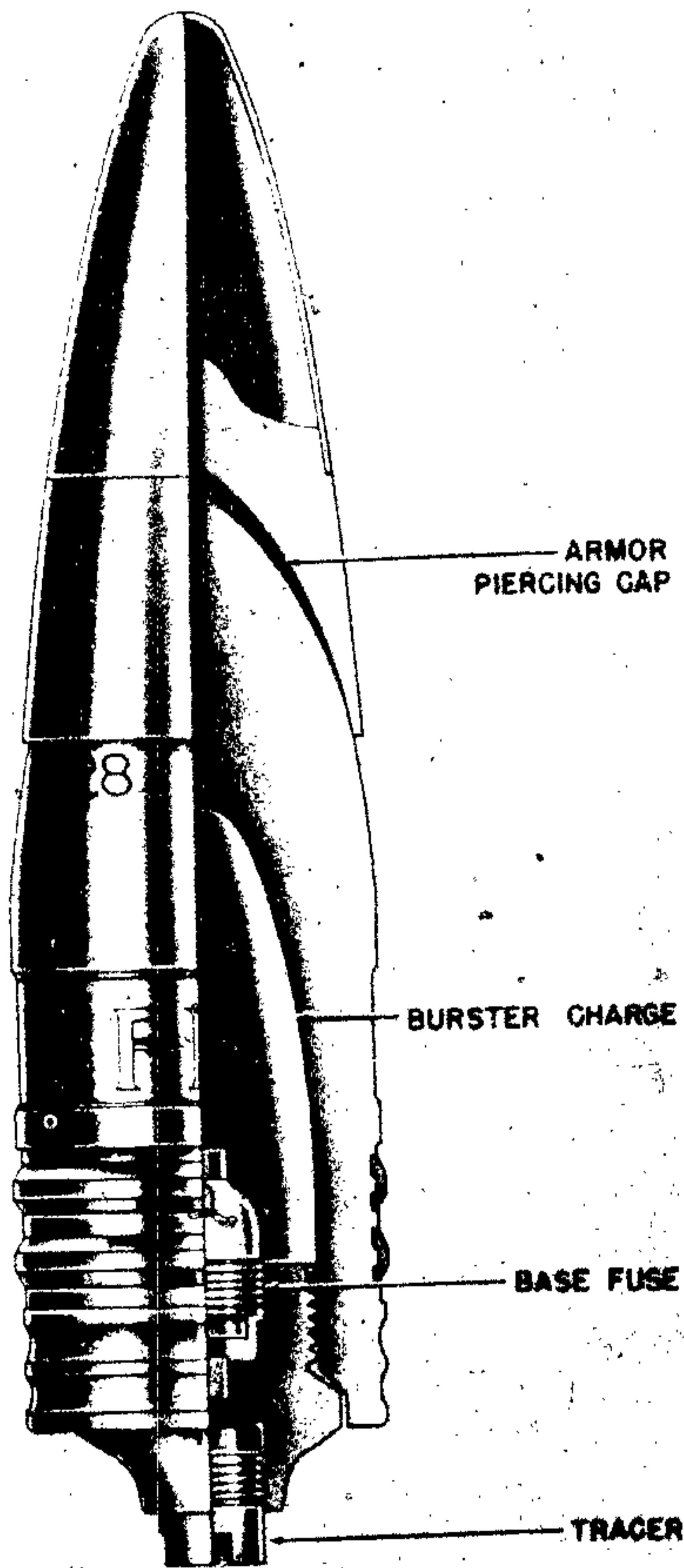
Figure 436—Armor-Piercing Projectile for 88-mm Gun, 8.8-cm Pzgr.
