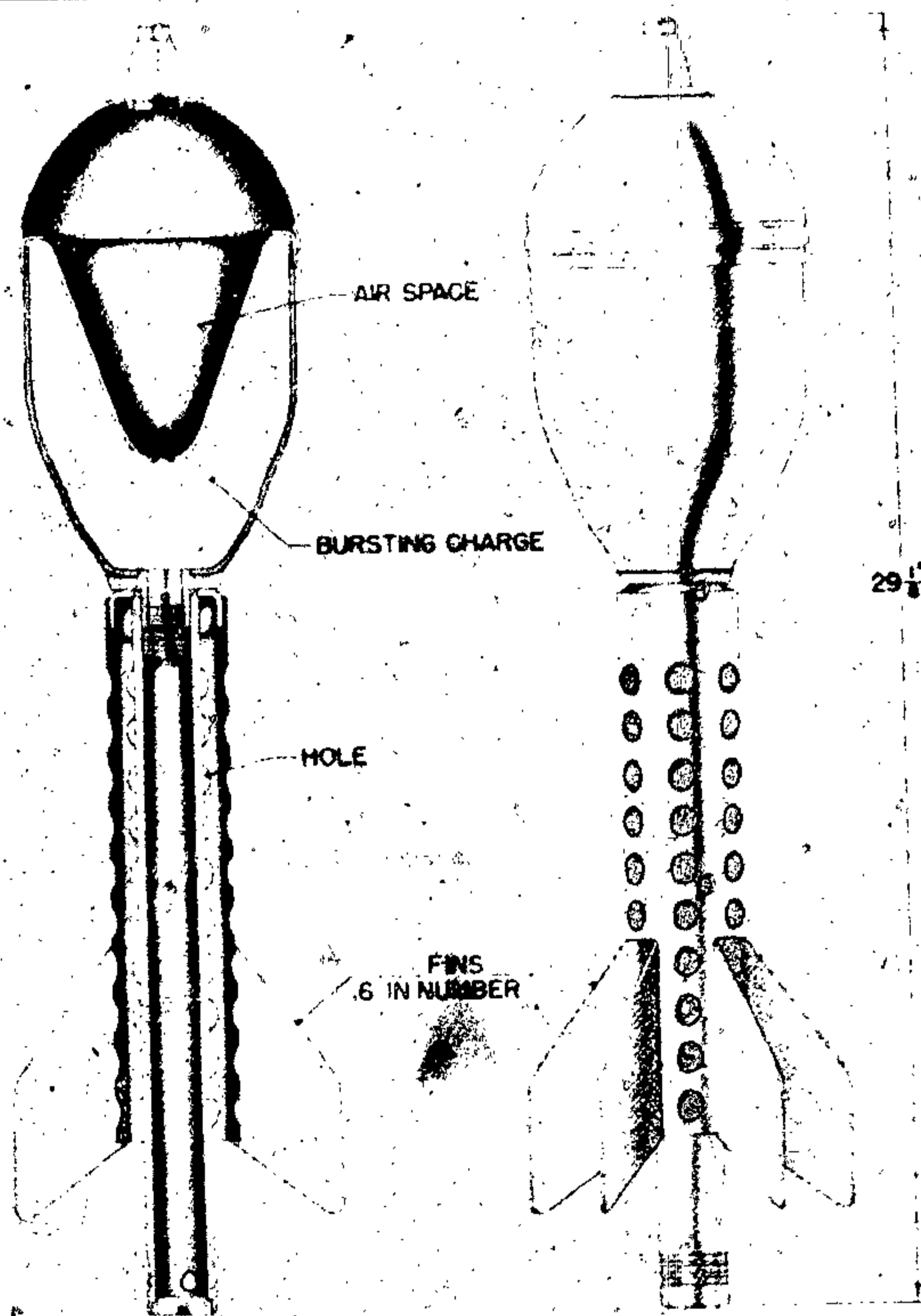
Figure 353—Redded Bomb for A. T. Gun 41, 37-mm, 3.7-cm Pak. 41
