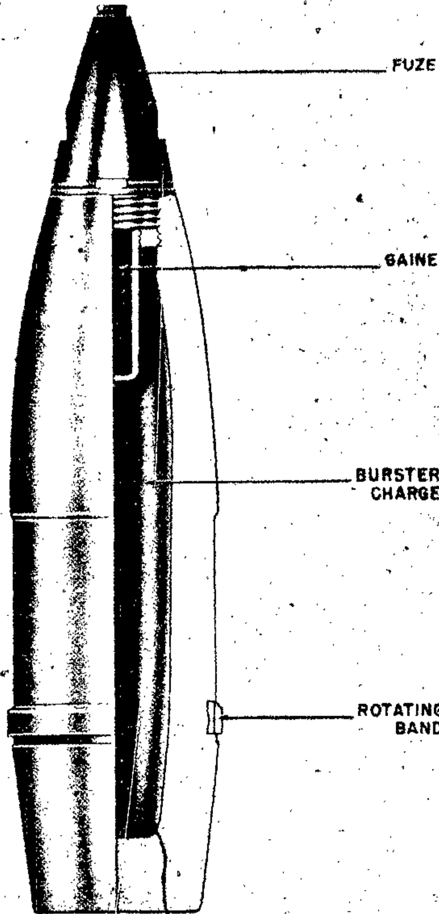
Figure 550—H. E. Projectile for 105-mm Howitzer
