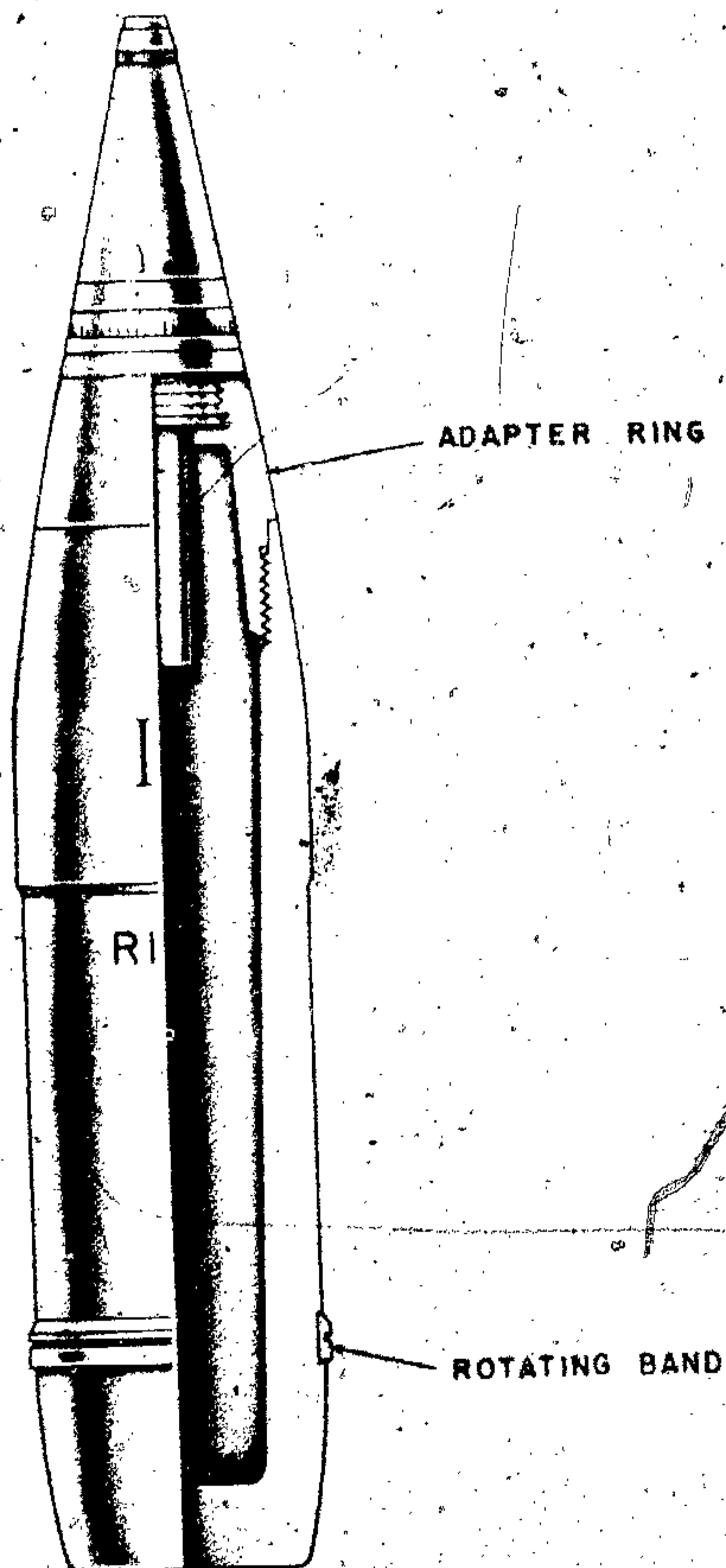
Figure 445—H. E. Projectile for 100-mm Howitzer, 10-cm Dopp. Z. Gr. 30 (f)
