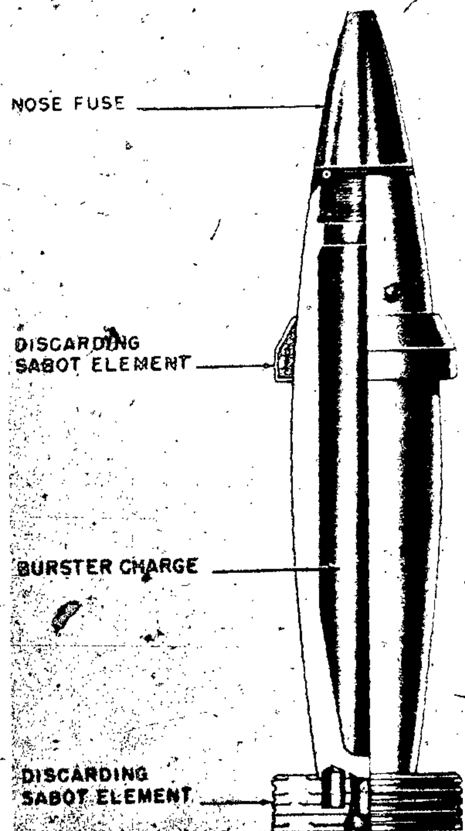
Figure 331A—Sabot Projectile Type F-1
