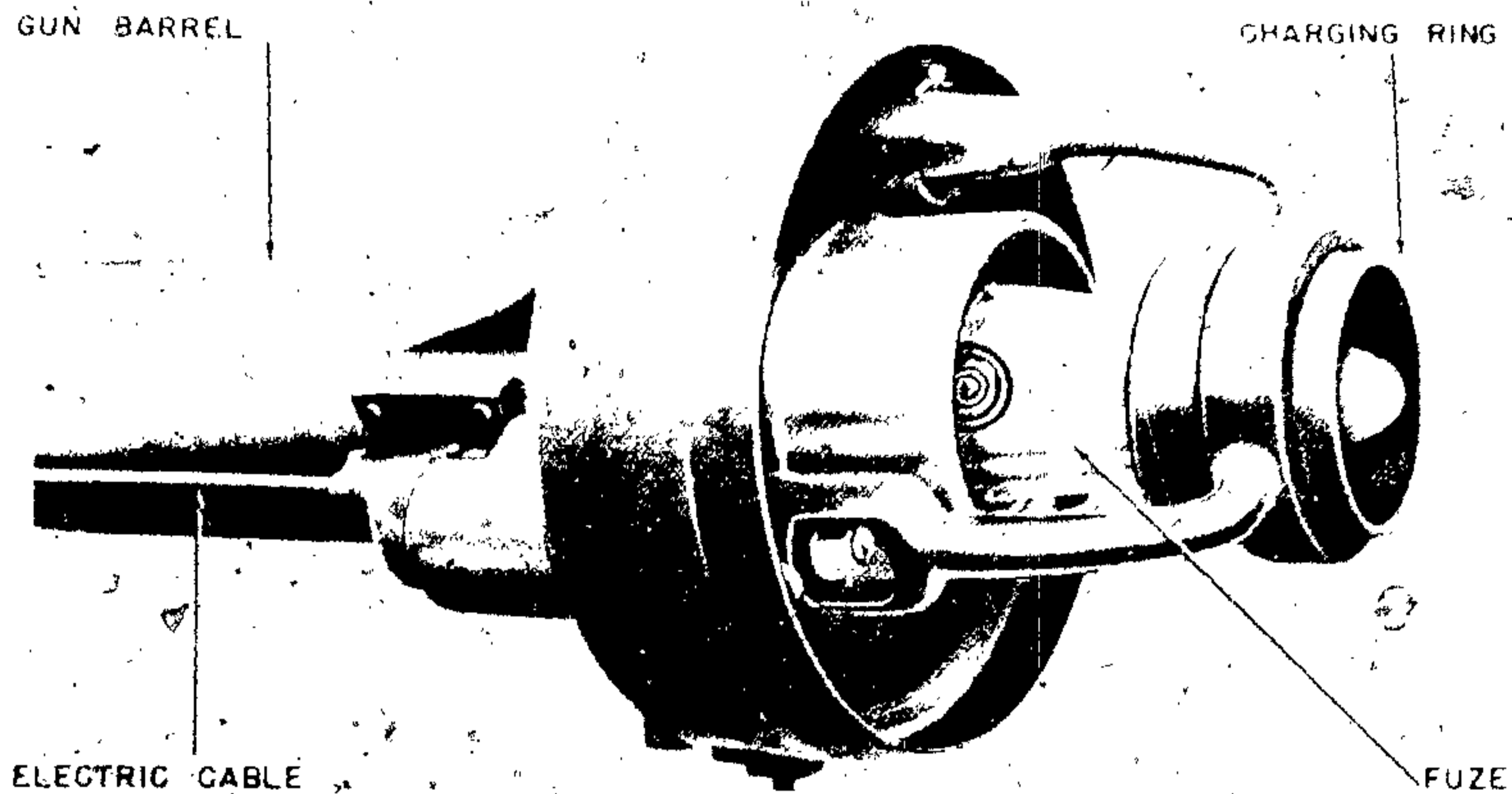
Figure 597C—Muzzle Charging Ring
