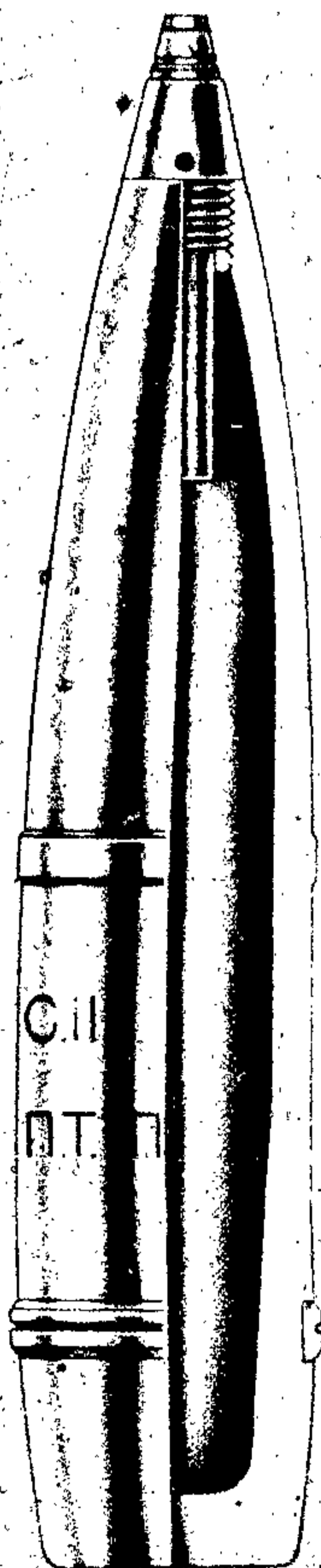
Figure 444—H. E. Projectile for 100-mm Howitzer, 10-cm Sprgr. (A. Z.) 310 (j)
