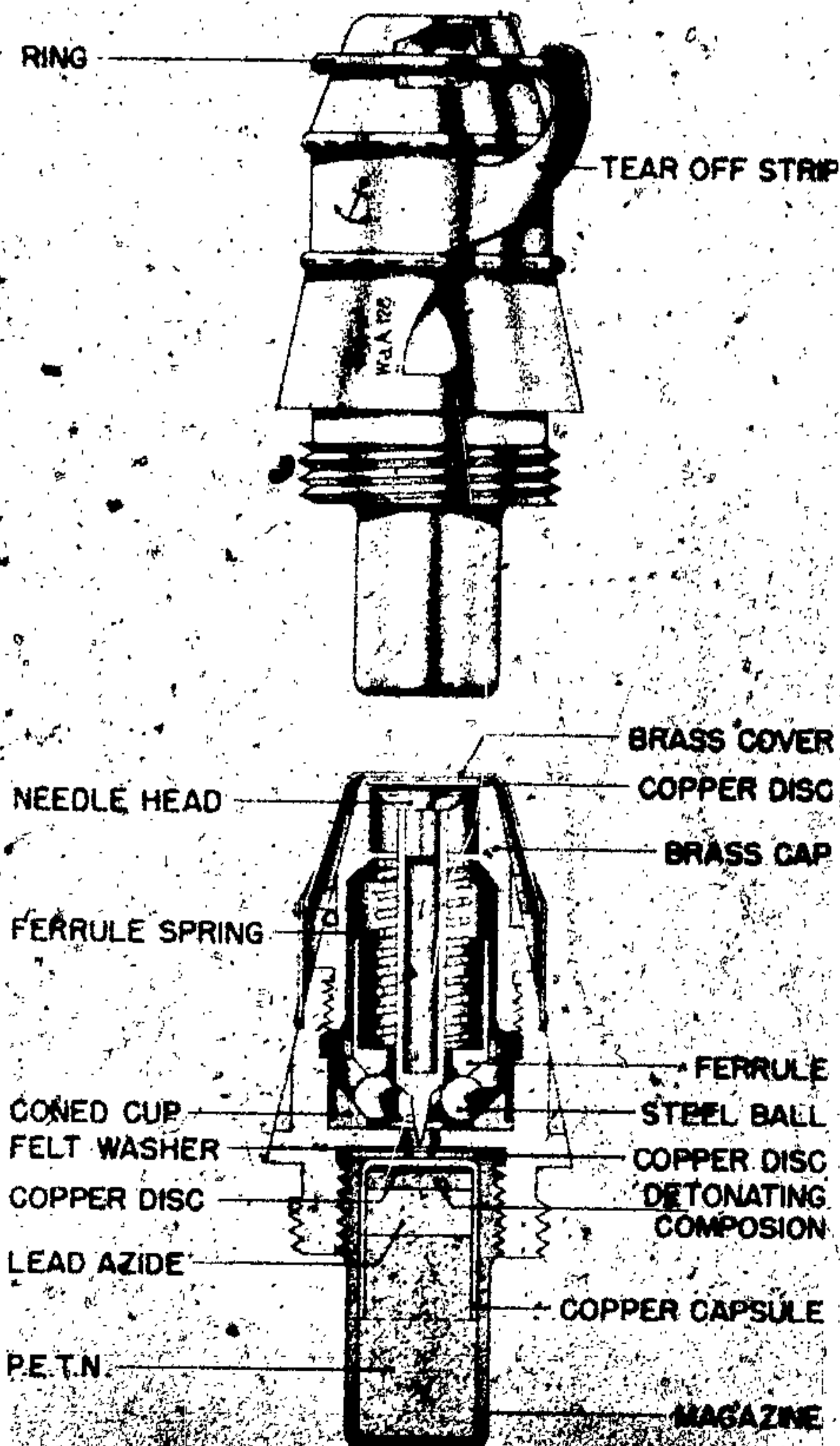
Figure 572—Fuze for 4.7-cm Pak. Spgr.
