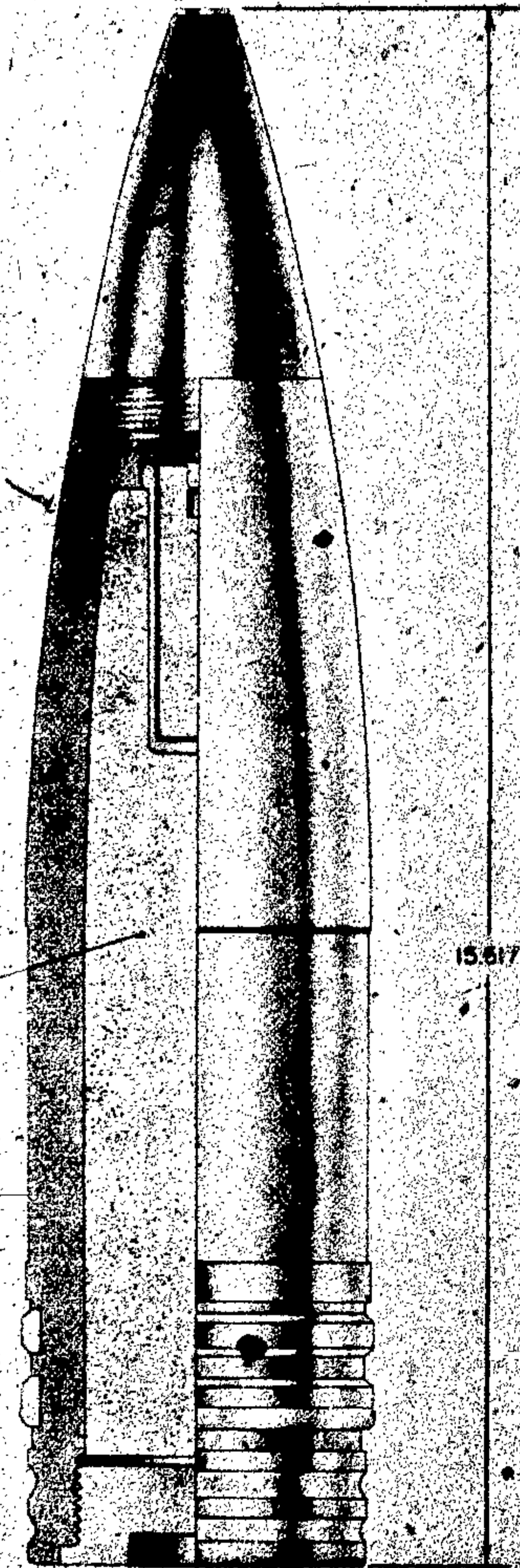
Figure 425—H. E. Projectile, Type L/4.5, 88-mm Sprgr. Patr. L/4.5 (Kz.)
