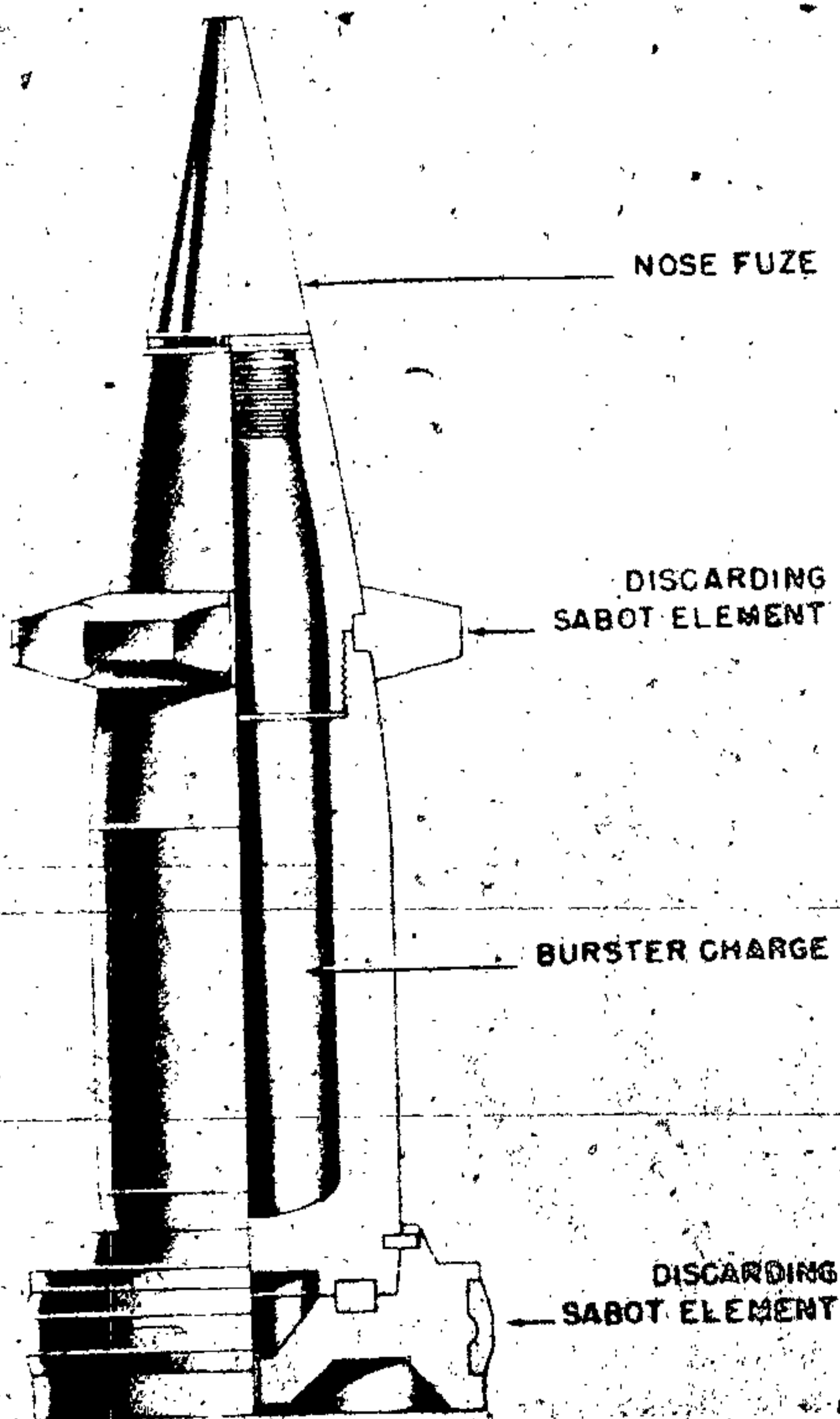
Figure 328—Sabot Projectile Type C
