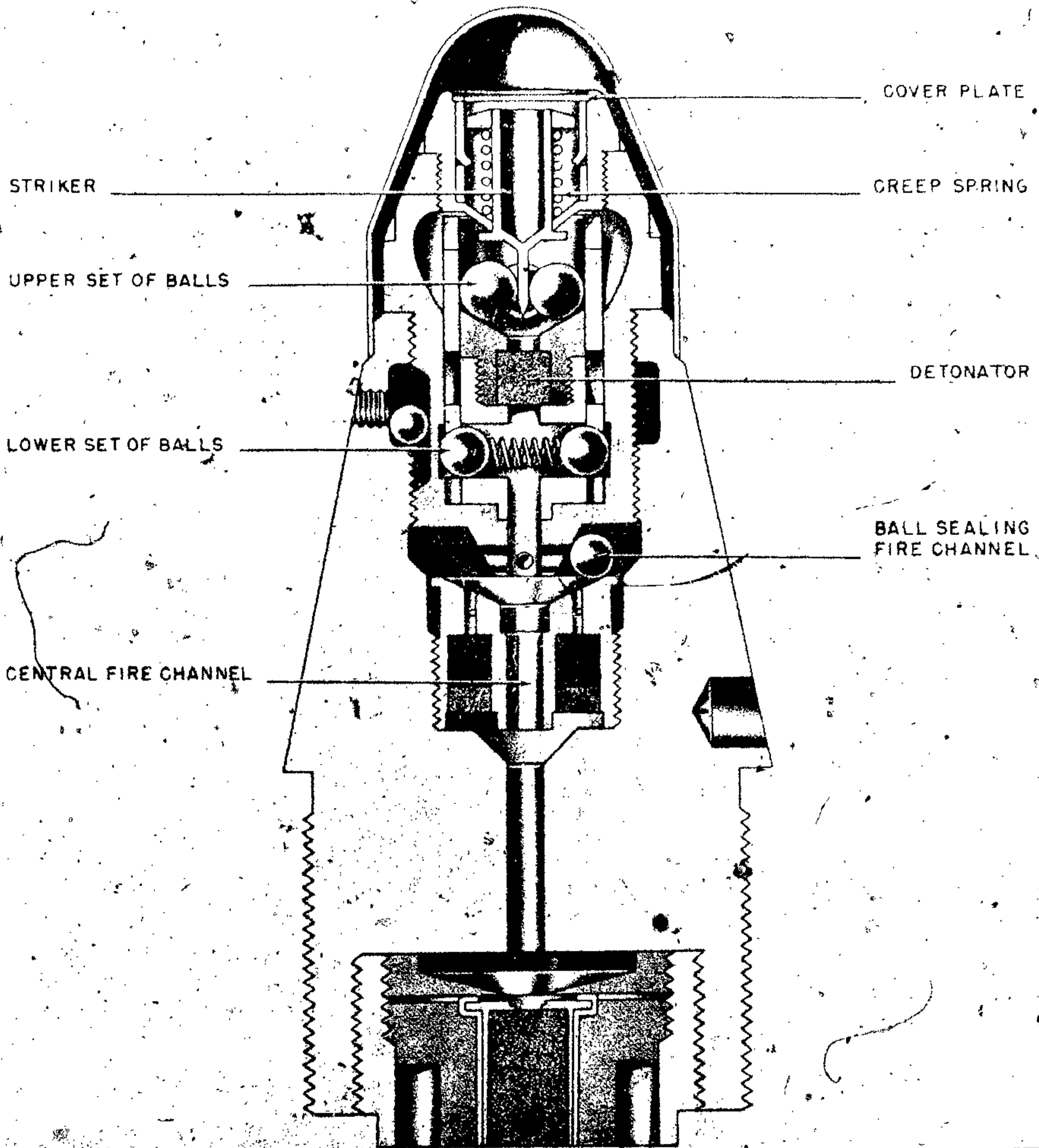
Figure 589—Skoda Percussion Fuze
