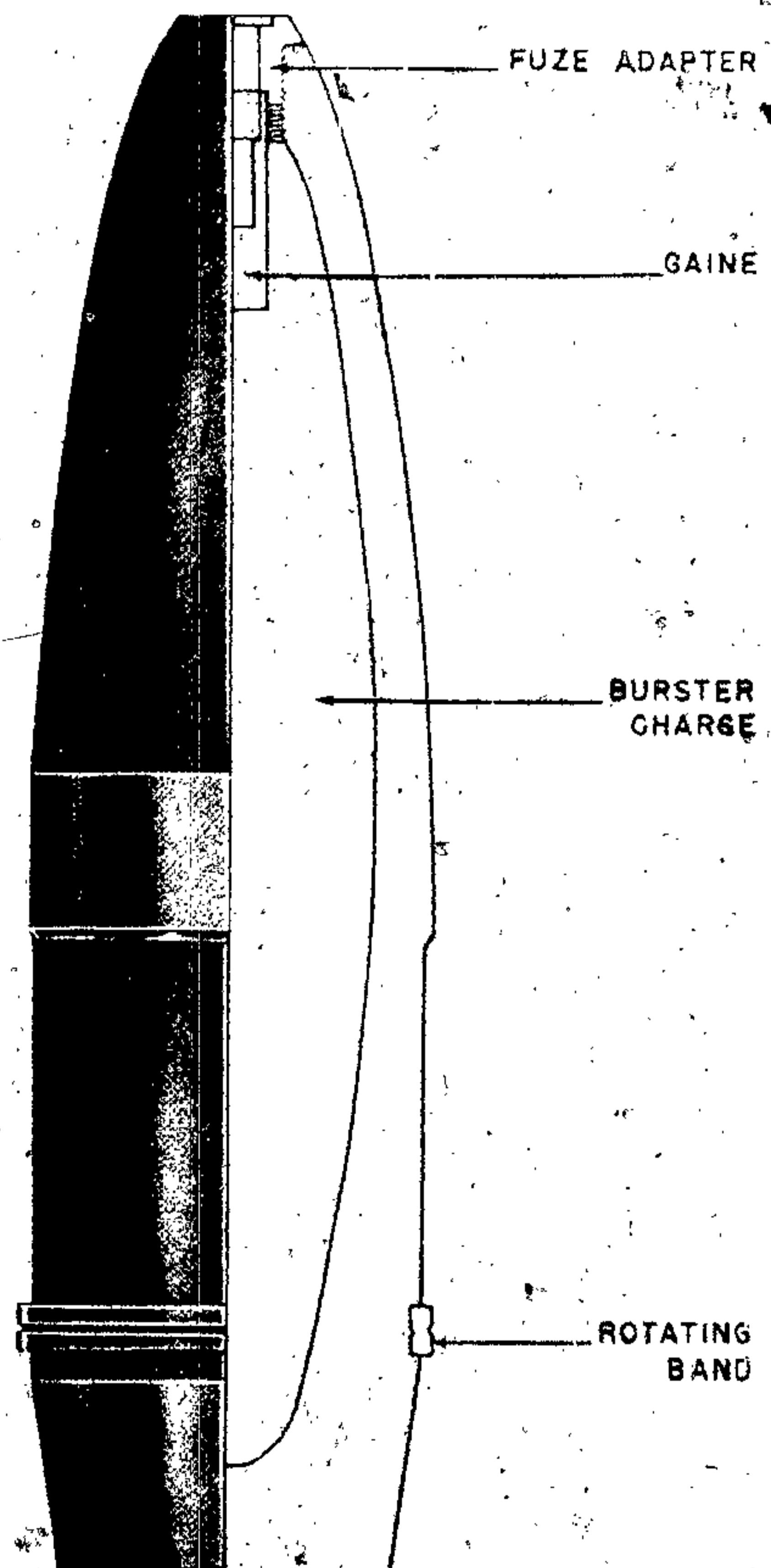
Figure 520—H. E. Projectile, 155-mm, 15.5-cm Gr. 417 (f)
