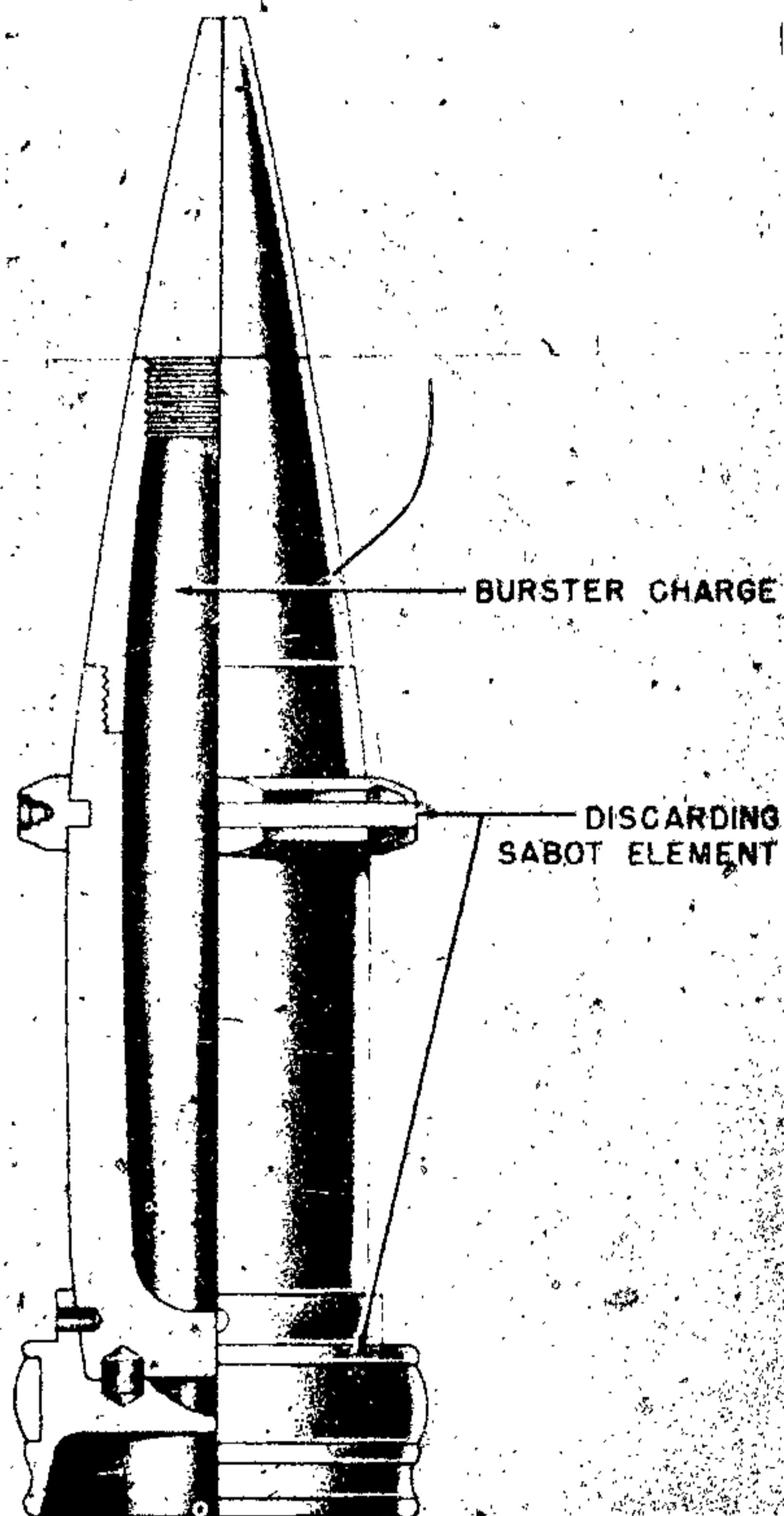
Figure 326B—Sabot Projectile Type A
