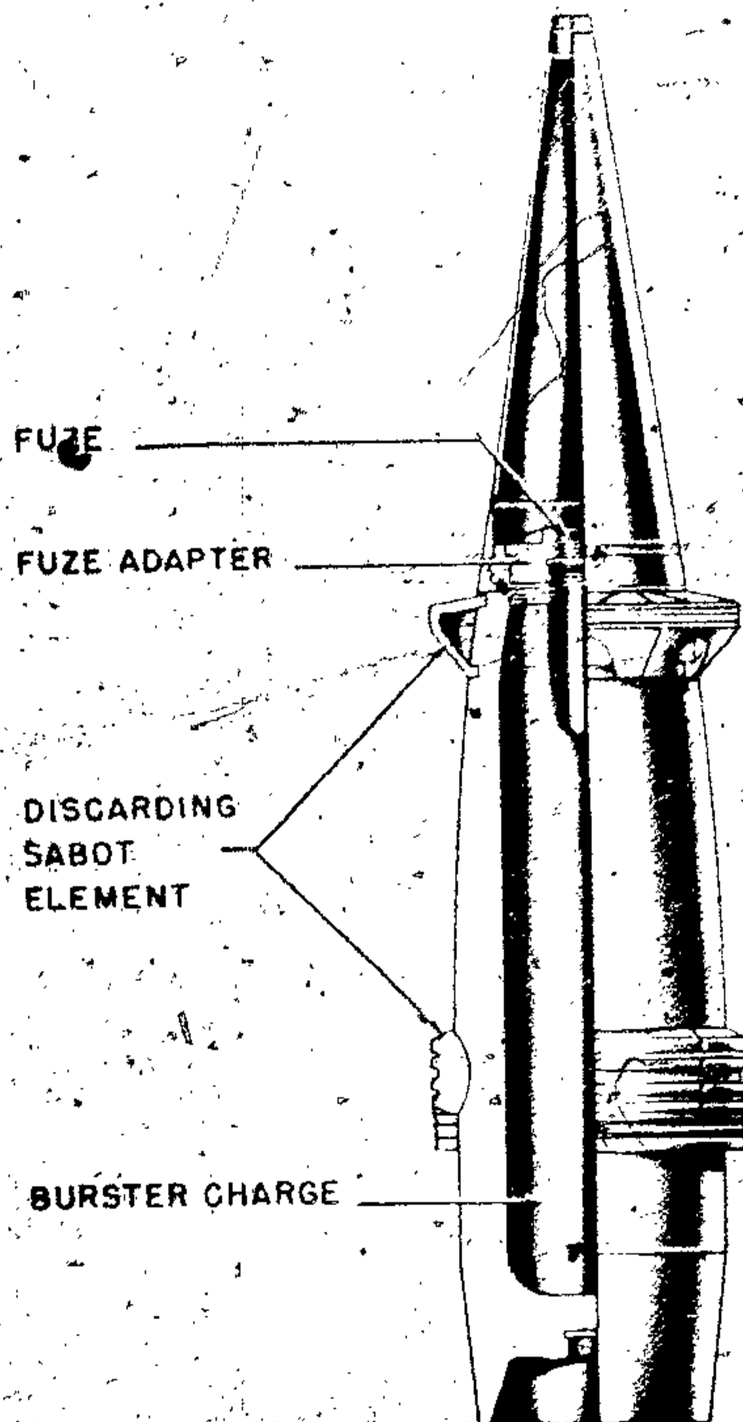
Figure 333A—Sabot Projectile Type H
