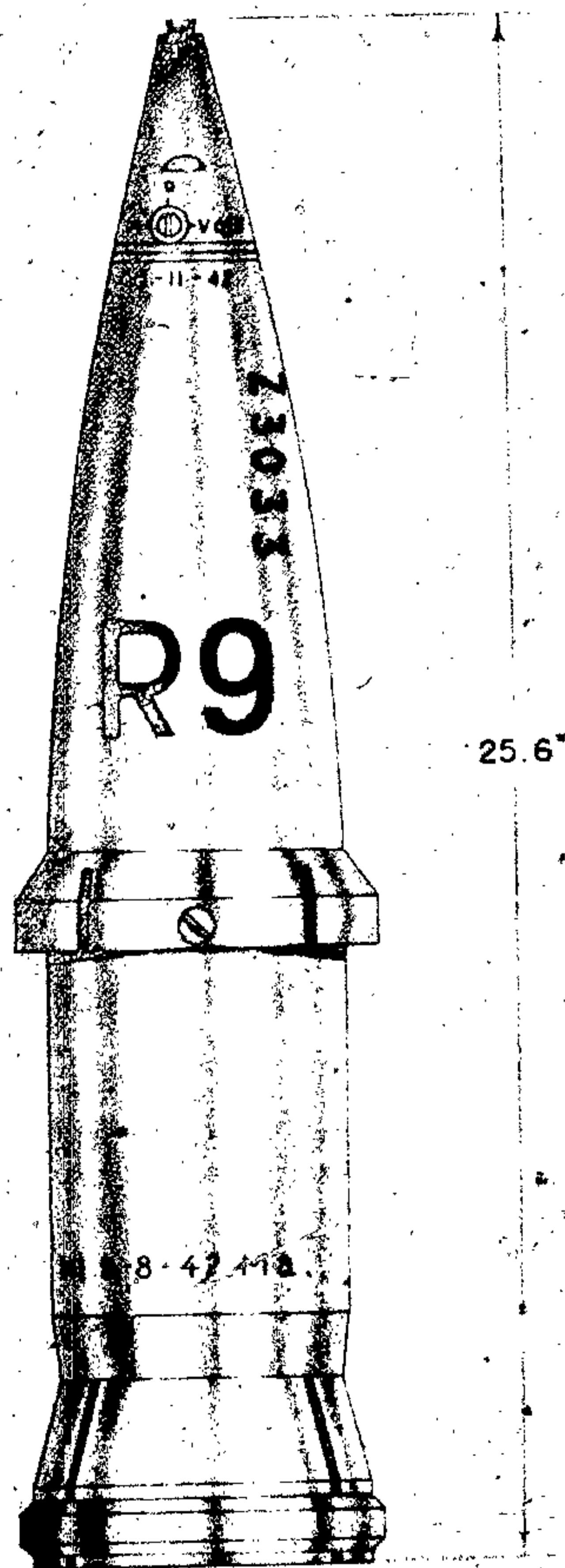
Figure 337—H. E. Projectile (Sabot Type), 150-mm
