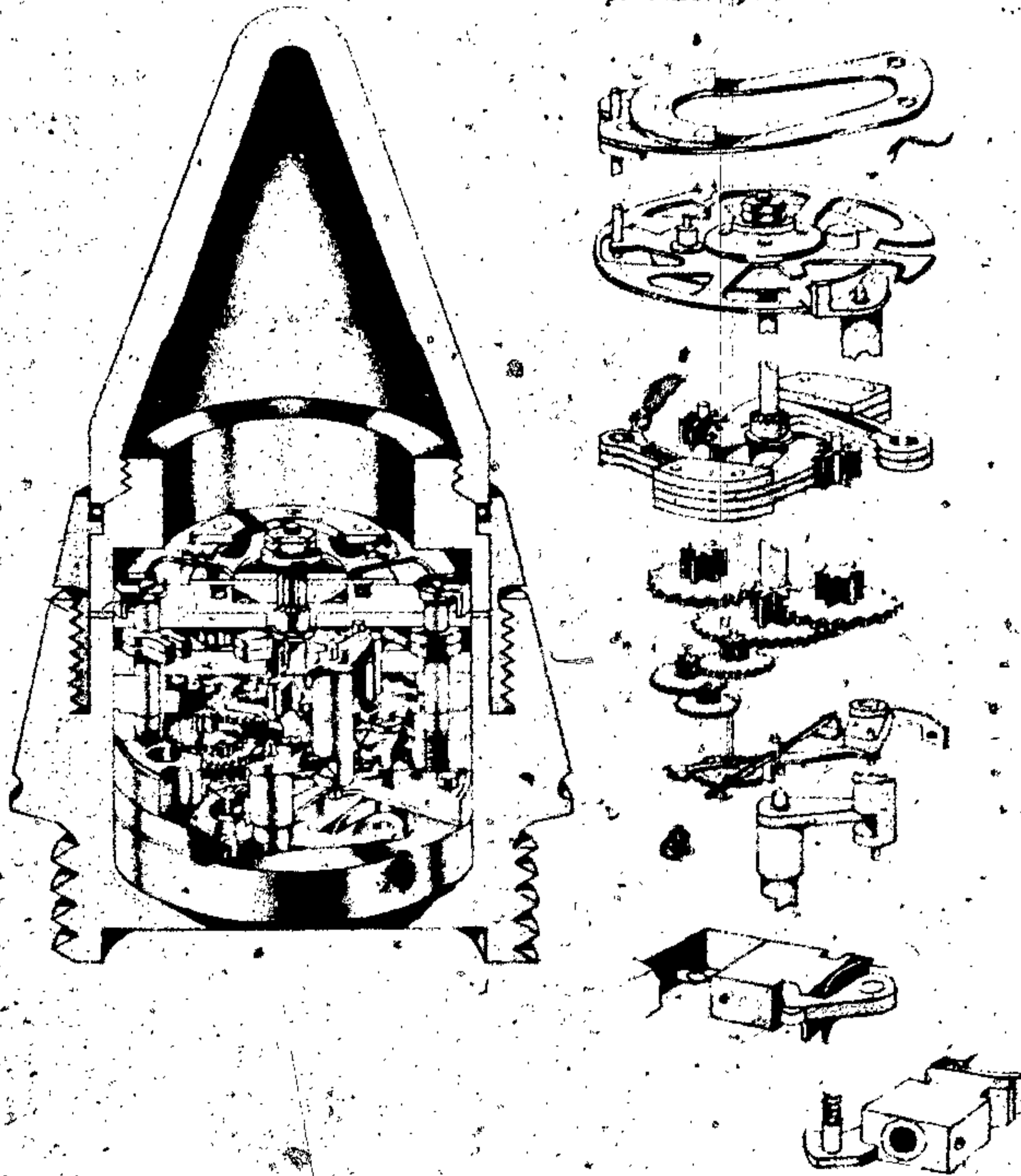
DIAGRAMMATIC ARRANGEMENT OF MECHANISM
