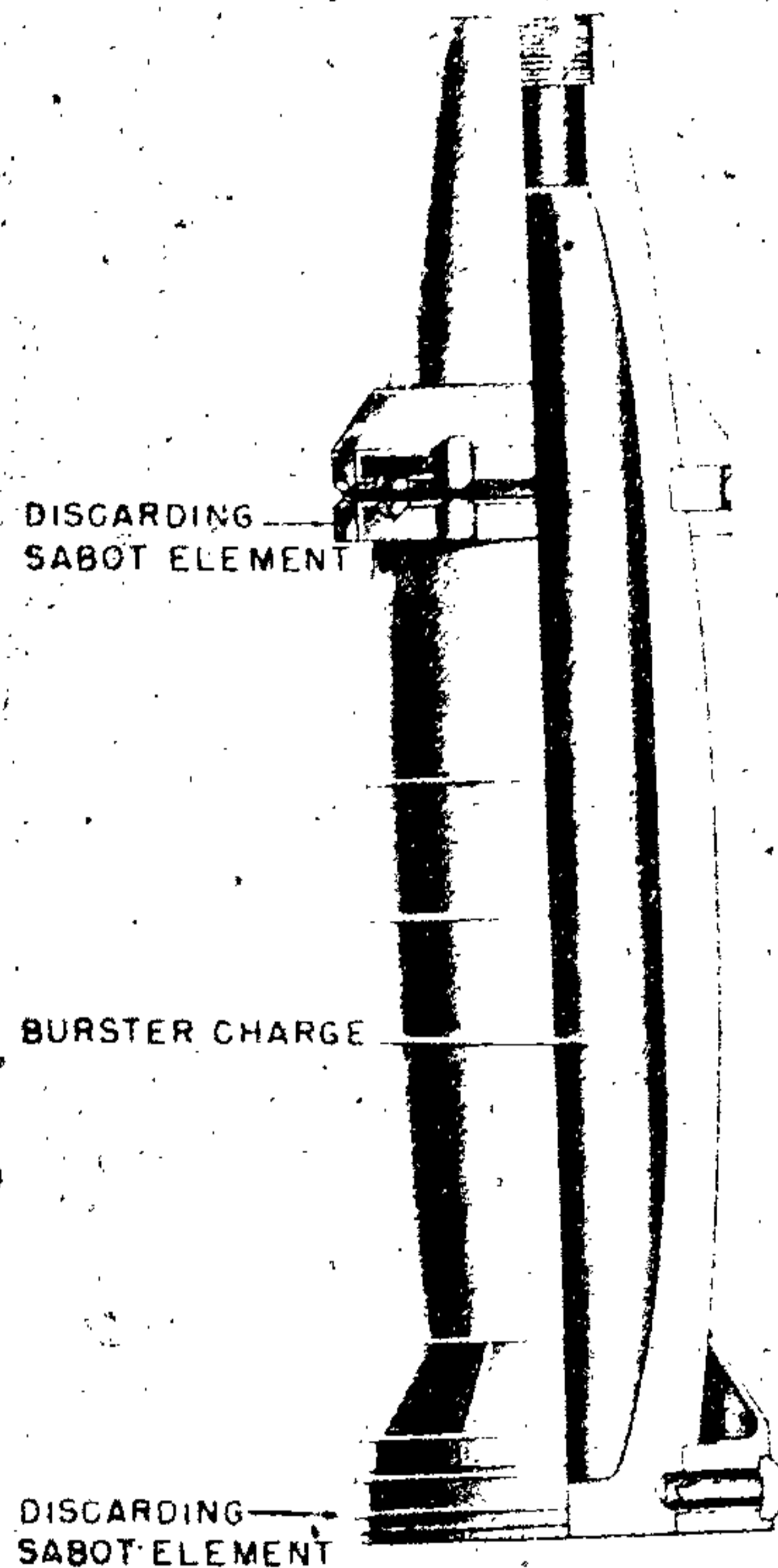
Figure 329—Sabot Projectile Type D
