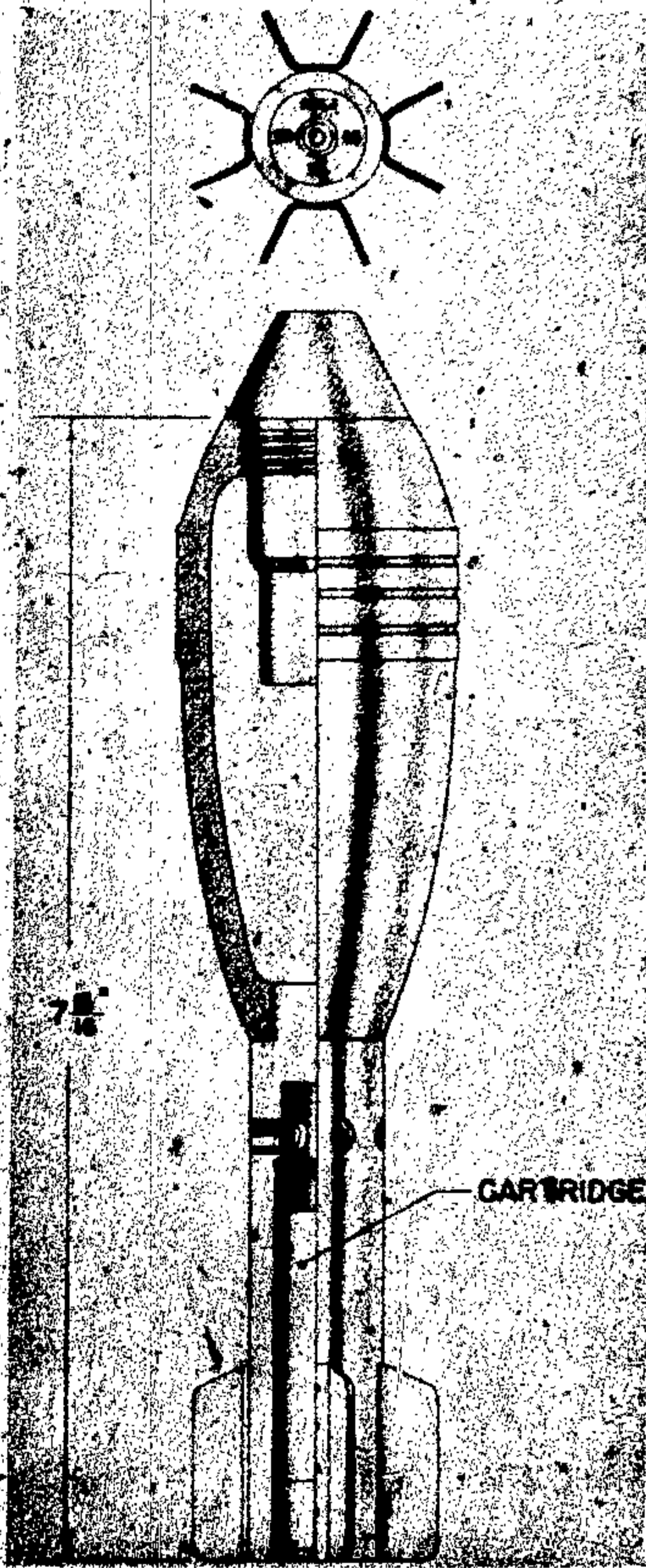
Figure 542—H. E. Mortar Projectile, 50-mm, 5-cm H. E. Bomb
