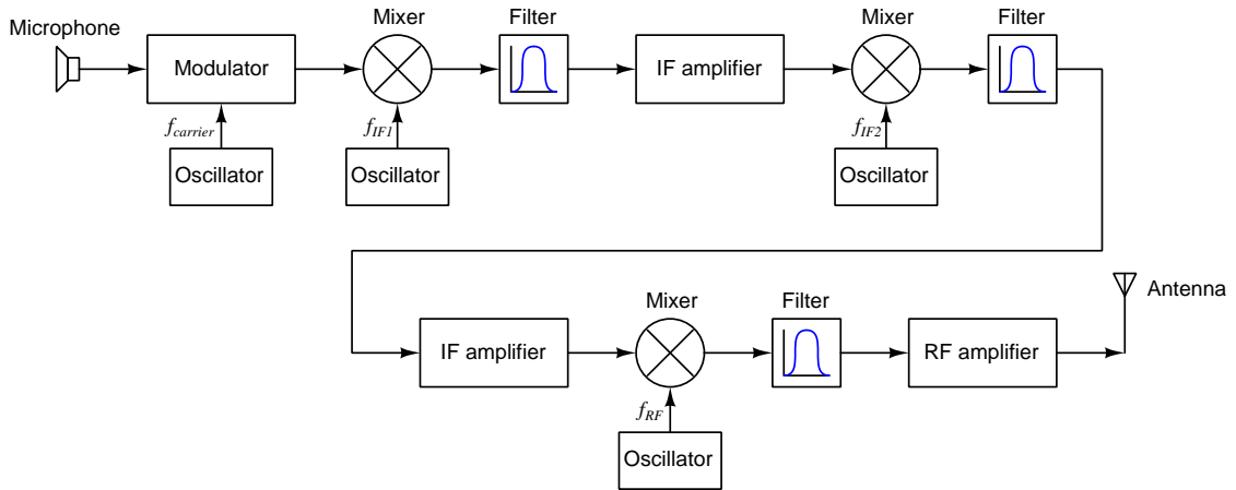
Radio transmitter with intermediate-frequency (IF) stages
