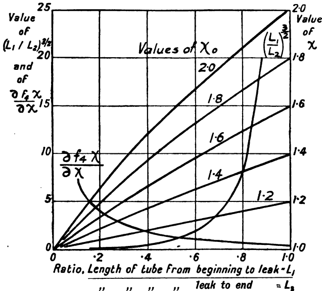
FIG. 6'2.—Effect of leaks on transit time. The lines marked 2.0, 1.8, etc., give the ratio of initial pressure to the pressure at points along the tube, viz. \chi = P_1/P , when the ratio P_1/P_2 = 2.0, 1.8 , etc.
