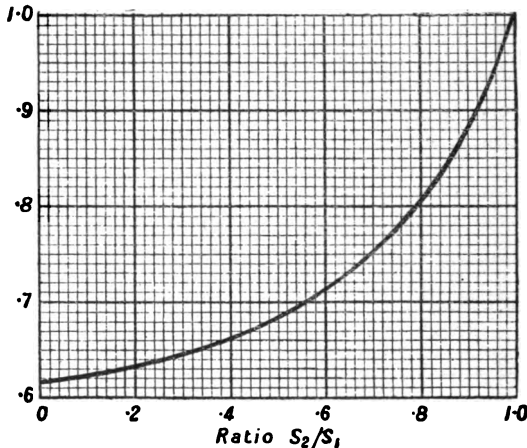
FIG. 8'9.—Coefficient of contraction as given by Gaskell.
