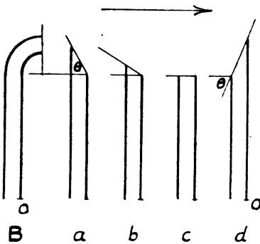
FIG. 9'5.—Pitot tubes as used by Anderson.
