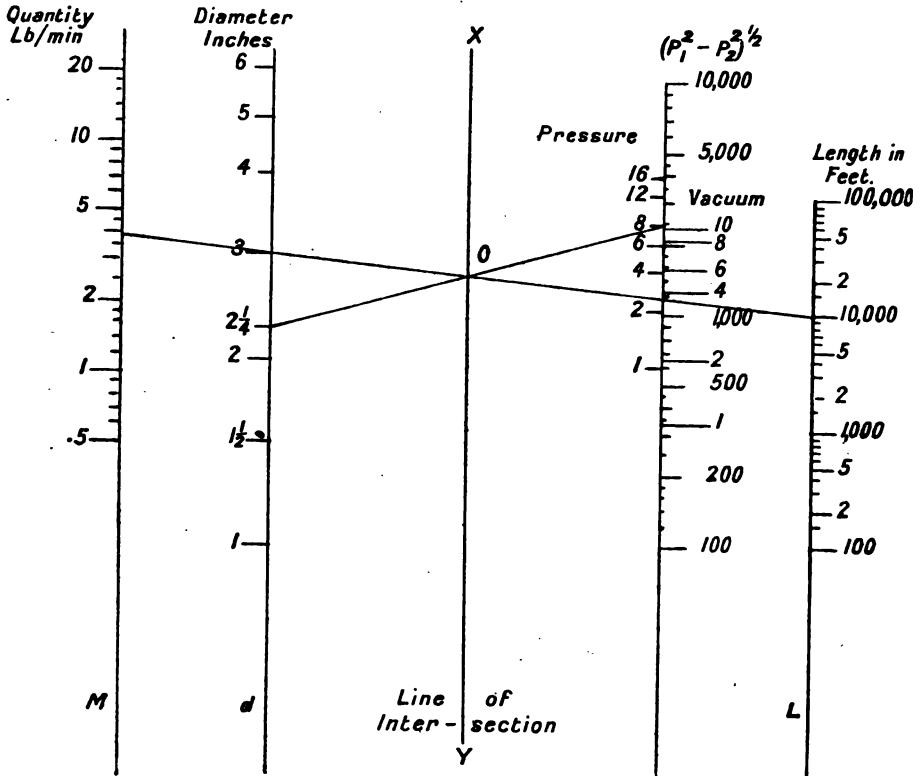
FIG. 27.—Typical abacus, for giving the quantity of flow in pneumatic tubes, 100 to 100,000 ft. long, 1 in. to 6 in. diam., when working at various pressures or vacuum. To find the quantity of air used per minute, join the given diameter to the given pressure, intersecting the XY line at O. Join the given length to O, and produce this line to meet the quantity line; where this cuts the quantity line gives the quantity flowing in lb/min. The figures under pressure and vacuum are gauge pressures in lb/in 2 . The fig. is drawn up from the equation (P_1^2 - P_2^2)^{1/2} D^{2.654} = 4.52ML^{1/2} . Lorenz's value of friction is used. P is lb/ft 2 , D is diam. in ft., M is quantity in lb/sec, L is length in ft.
