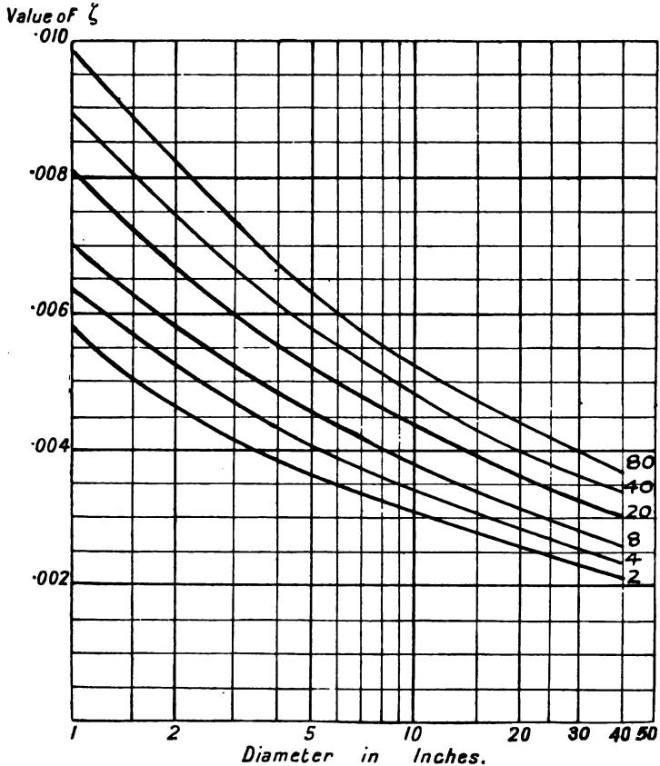
FIG. 23.—Coefficient of friction, \zeta , depending on \frac{T}{\rho u} , or \frac{144S}{MC} , and on diameter. Given by Fritzsche. The numbers against the curves are values of T/(\rho u) in metric units. When using English units, viz. T absolute Fahrenheit, p lb/in 2 , u ft/sec, multiply the value of T/(\rho u) by 26 to bring to the metric value.
