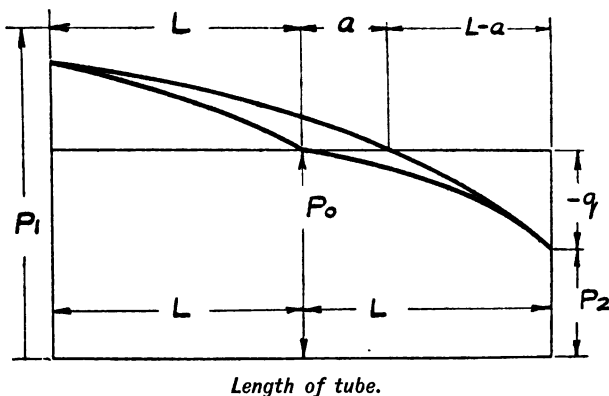
Fig. 4.5.—Theory of looped tubes. P_0 =atmospheric pressure.
