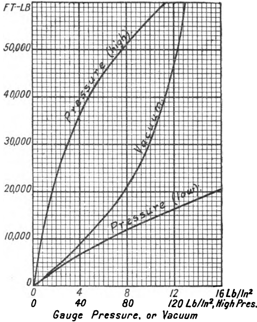
FIG. 4.8.—Work done in isothermal compression per lb. of air, when compressing from atmospheric pressure, 14.7 lb/in 2 , and 60° F.
