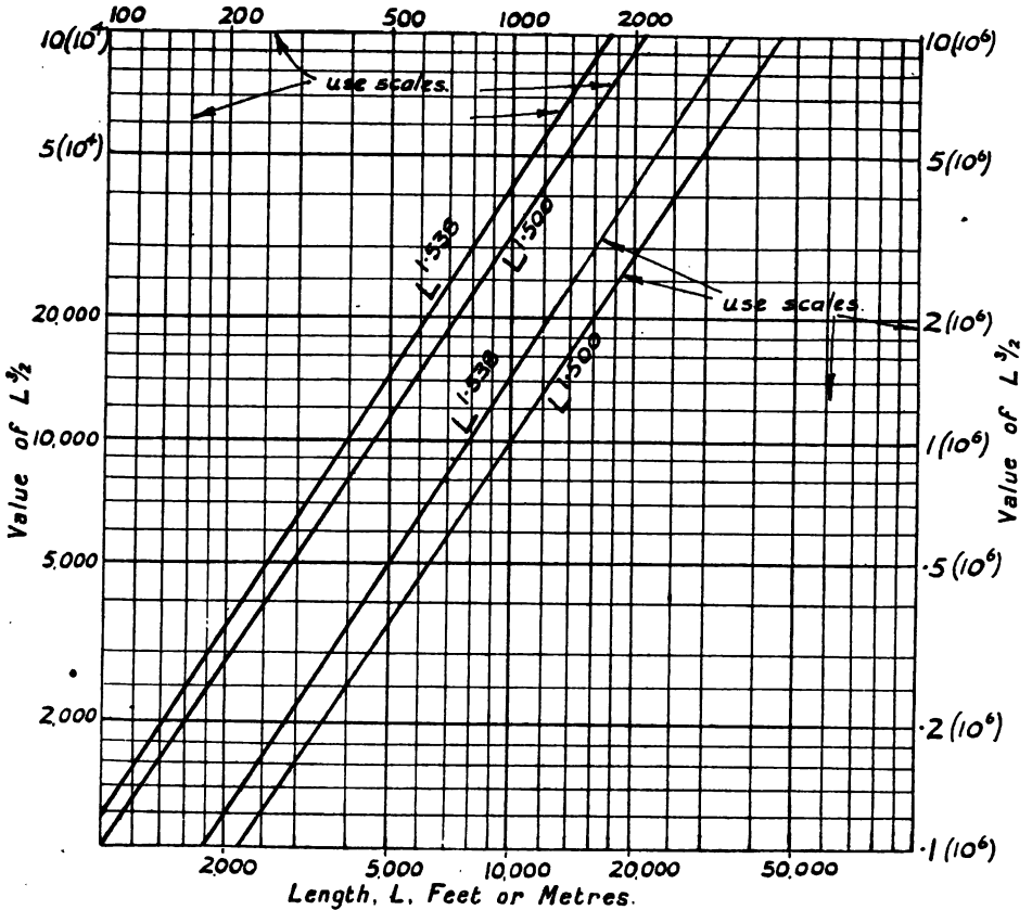
FIG. 4.4.—Functions of L for use in finding transit time.
