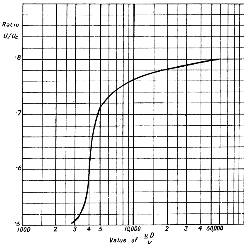
FIG. 9'3.—Ratio of mean velocity, U , to the velocity at the centre of the pipe, U_c , for various values of uD/\nu ; u in cm/sec, D in cm, \nu is the kinematical viscosity in dyne/cm 2 . Given by Stanton.
