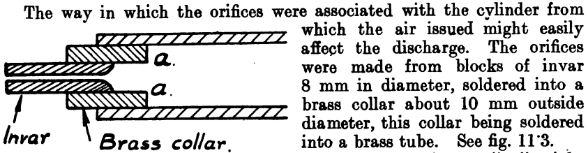
FIG. 11'3.—Hartshorn's orifice.
