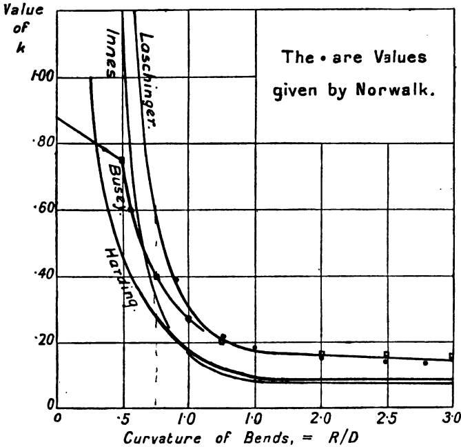
Fig. 3.2.—Coefficient k for the resistance of bends of various curvature.
