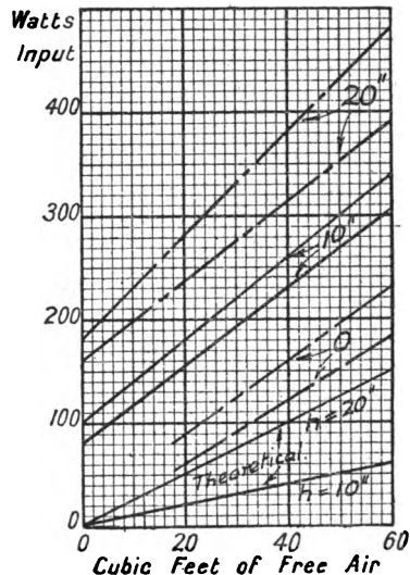
FIG. 14'2.—Electrical energy required to deliver air at various pressures. The energy will lie between the upper and lower lines, depending on the type of blower used.
