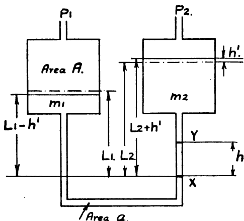
FIG. 9'6.—Theory of the differential multiplying manometer.
