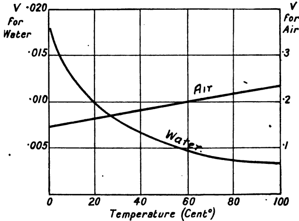
FIG. 2'5.—Variation of kinematical viscosity with temperature. \nu = \eta/m , in \text{cm}^2/\text{sec}^2 . From Blasius ( Mitt. über Forsch. Ver. Deut. Ingr. , 131/35/1913).
