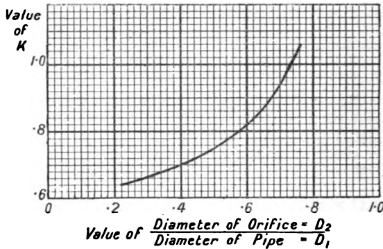
FIG. 8.7.—Coefficient of delivery for orifices in a pipe line. Given by Hickstein, p. 217.
