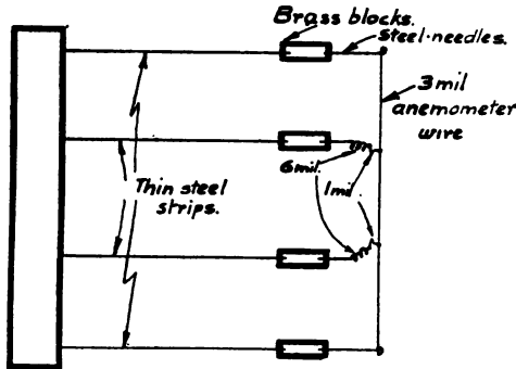
FIG. 10'1.—Hot-wire anemometer.
