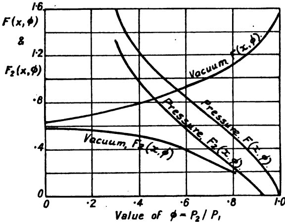
FIG. 7.4.—Functions giving the time for unsteady flow after the cock is turned off. F(x, \phi) assists in determining t4 ; see Eq. 7.29, 7.30. F_2(x, \phi) is the time taken for the pressure in the tube to reach 1 lb/in 2 above or below atmospheric pressure. See Eq. 7.40, 7.41.
