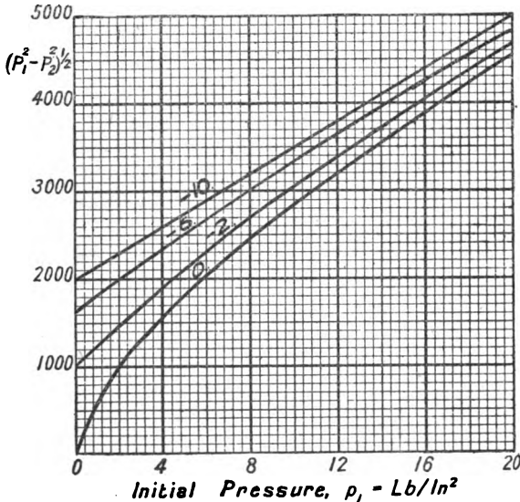
FIG. 4'3.—Function for giving the quantities of air circulating in looped tubes: using English units. The figures on the curves give the final pressure in lb/in 2 gauge. The function is (P_1^2 - P_2^2)^{1/2} , P in lb/ft 2 .
