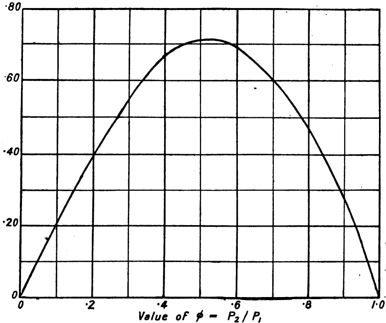
FIG. 11.2.—Value of the function \phi^{1.41} - \phi^{1.71} for use in orifice flow.
