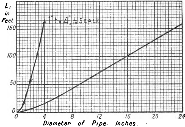
FIG. 3'1.—Length of pipe in which the velocity head is lost. Length = L_1 = D/(4\zeta) , using Unwin's \zeta .
