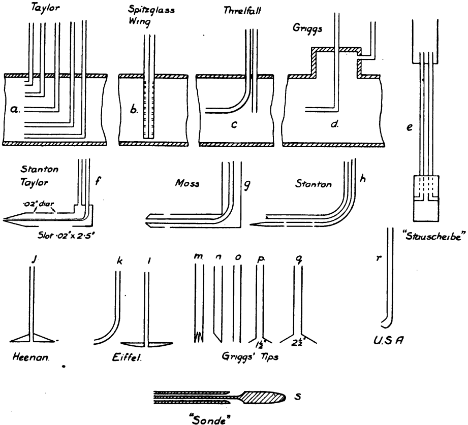
FIG. 9'2.—Forms of Pitot tubes.
