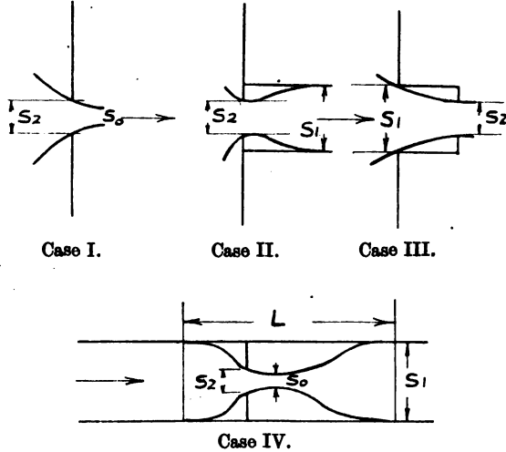
FIG. 8.5.—Orifice flow : Müller's theory.
