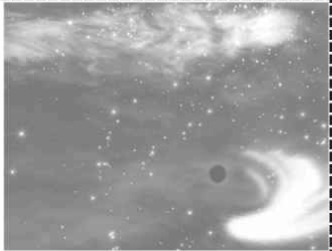
Artist's impression illustrates the tremendous gravitational pull of a giant black hole on a passing star. The supermassive black holes that dot outer space are the "most fuel efficient engines" in the universe, according to the findings of a new US study that used a powerful NASA X-ray observatory to observe nine vast black holes.—INTERNET
