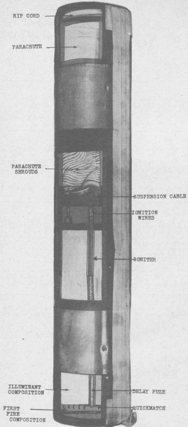
AIRCRAFT PARACHUTE FLARE AN-MK 8, MOD. 1
