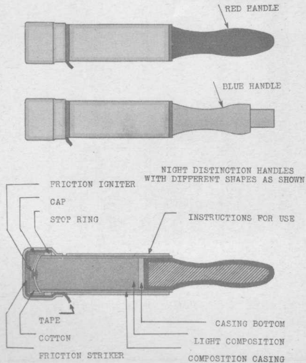
NAVY RED LIGHT, MK I & NAVY BLUE LIGHT, MK I, MOD I
