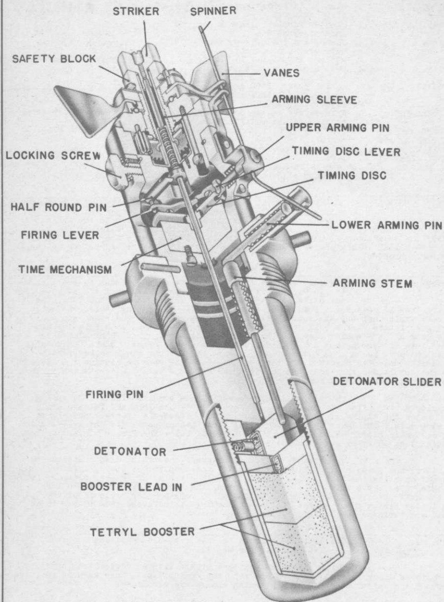
MI35AI, MI36AI MECHANICAL TIME FUZE (NOSE)
