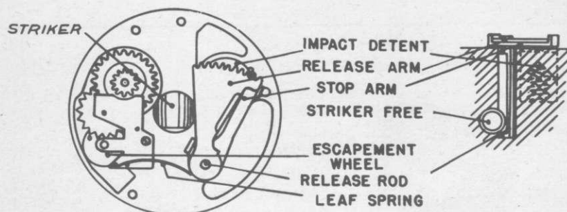
FIGURE 8 (FIRING POSITION)
