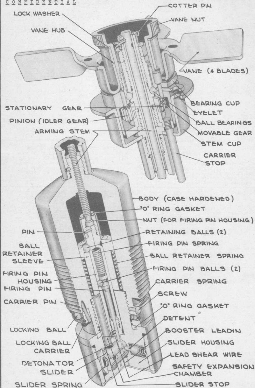
BOMB TAIL FUZE MK 237 MOD 0 & MK 238 MOD 0 (LEAD SHEAR WIRE - LONG DELAY TIME)
