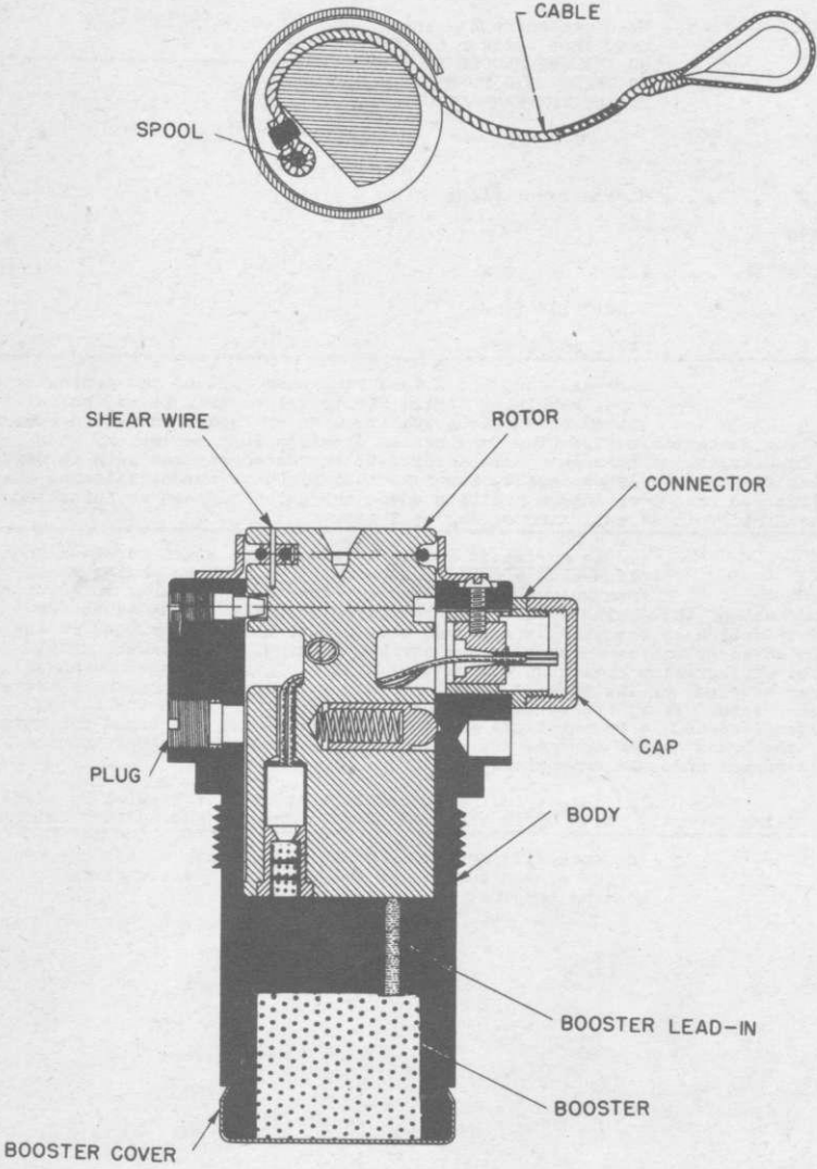
U.S. NAVY MK.233 NOSE FUZE
