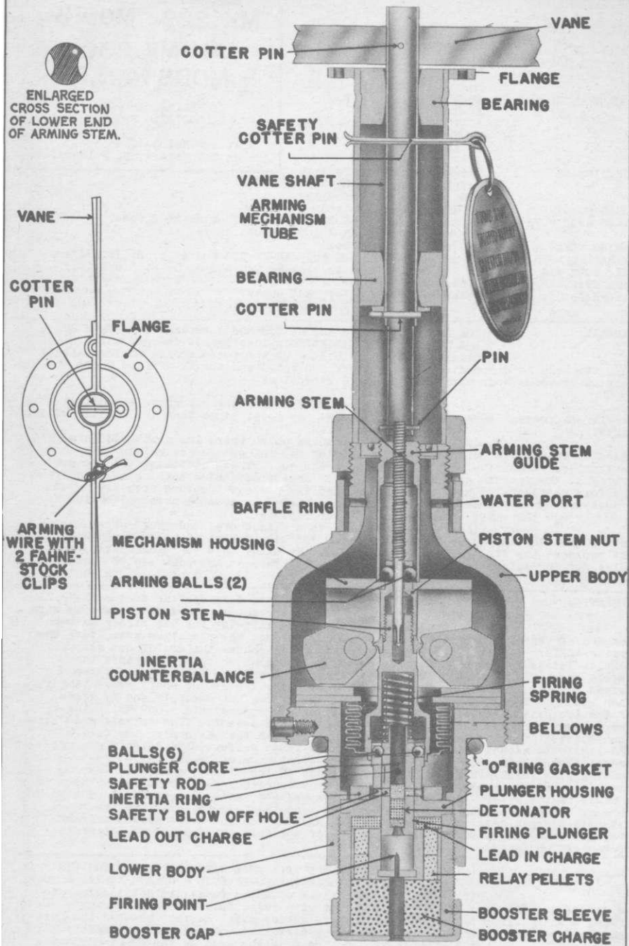
BOMB TAIL FUZE MK. 231 MOD. 0 (HYDROSTATIC)
