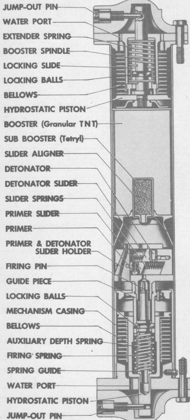
BOOSTER EXTENDER
