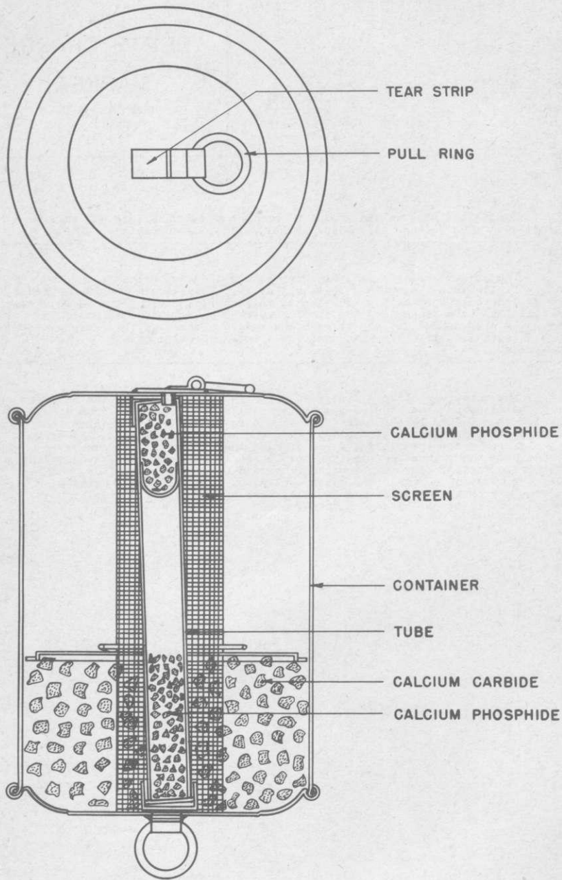
DEPTH CHARGE MARKER (NIGHT) MK 2
