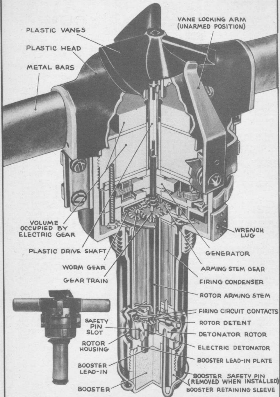
M 166(T5IEI) VT BOMB FUZE (ARMED)
