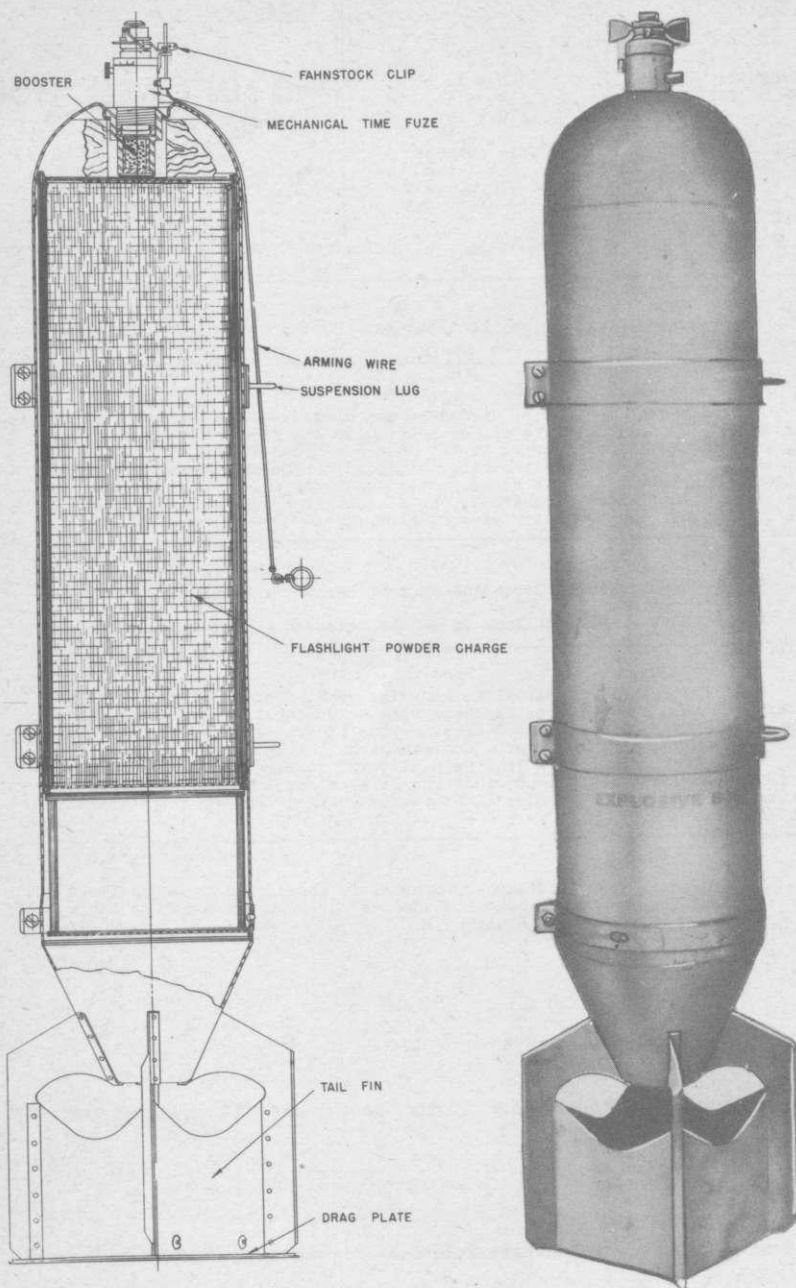
100 LB. PHOTOFLASH BOMB, AN-M46
