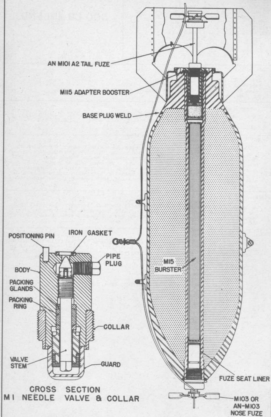
AN-M78 500 LB. CHEMICAL BOMB
