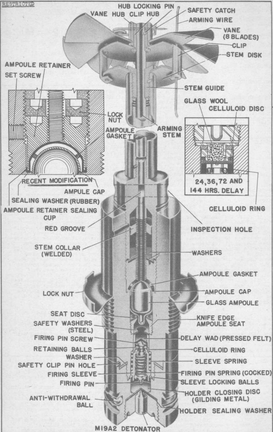
U.S. 123 A1 SERIES LONG DELAY TAIL FUZE (1, 2, 6 & 12 HOURS DELAY)
