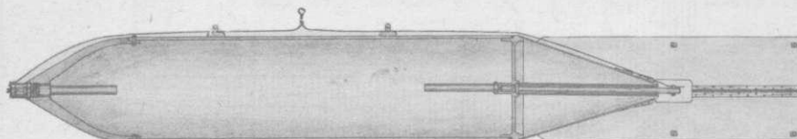
2000 LB. MK. I M3 (135"8 LONG)
