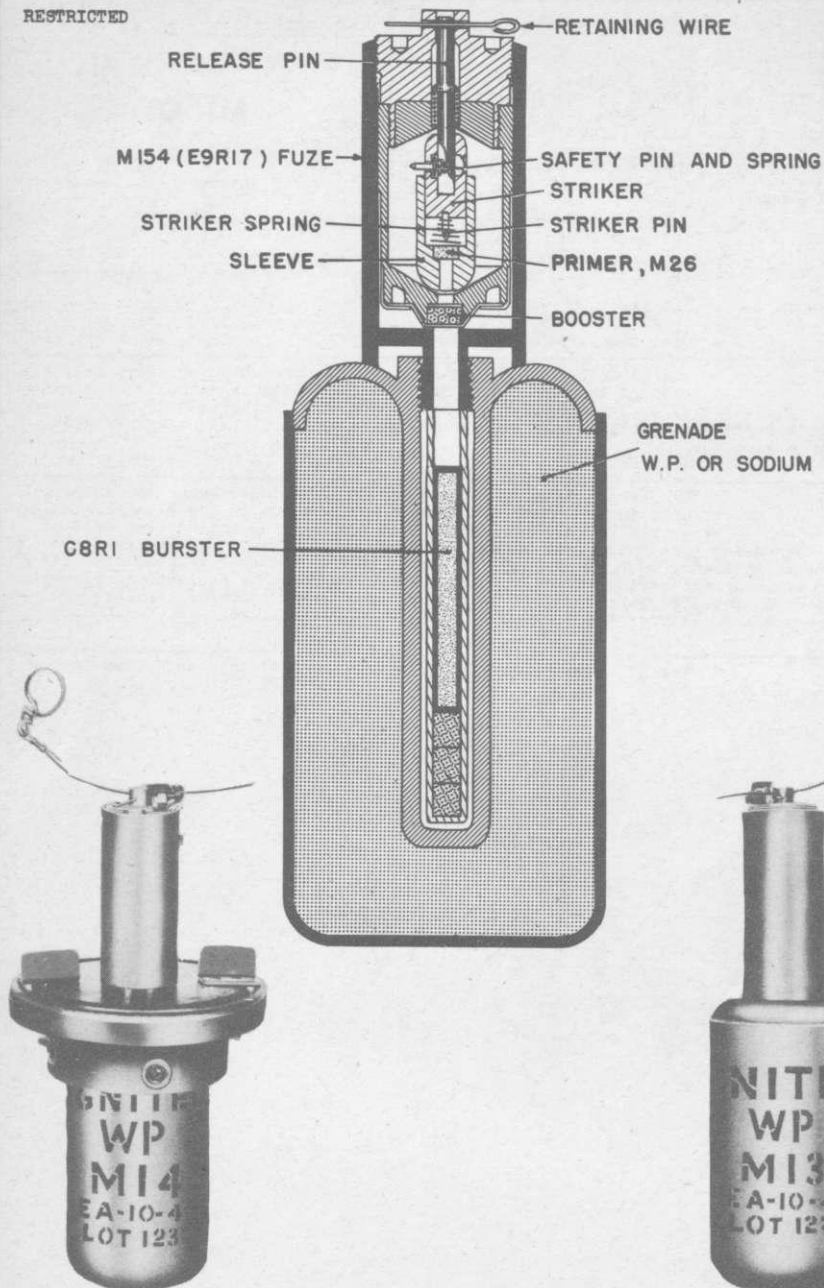
M154 FUZE M13 AND M14 IGNITERS
