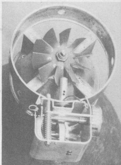
MI (T2E1) AIR TRAVEL ARMING DELAY
