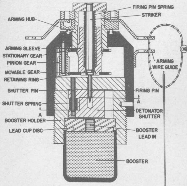
MI58 NOSE IMPACT FUZE
