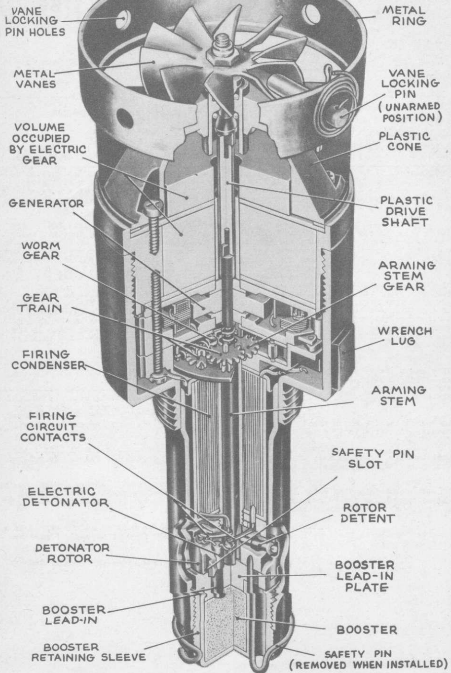
T91-T92 VT BOMB NOSE FUZE (ARMED)
