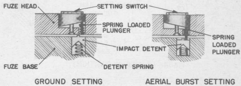
FIG. 5 SETTING SWITCH
