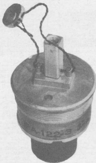
FIG. 2 M 130 FUZE - TIME
