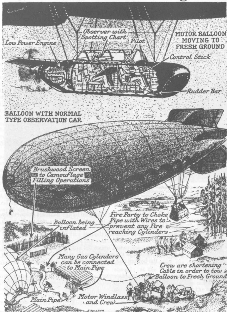
This diagram of a new French dual-purpose balloon shows the features which make it so much more serviceable than the ordinary observation balloon. A power-driven nacelle for driving the balloon from place to place obviates the necessity of repeated deflation and inflation close to the enemy lines.
