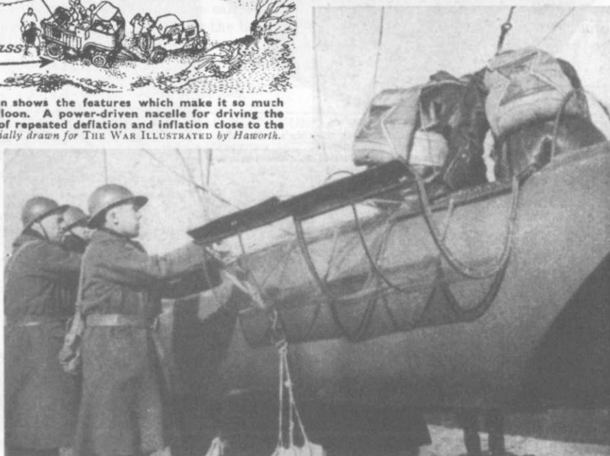
The pilot and observer climb into the power-driven nacelle of an observation balloon, whilst the ground staff steady it for them. The clean aerodynamic lines of the nacelle show a marked improvement on the cars of the older types of power-driven balloons.
