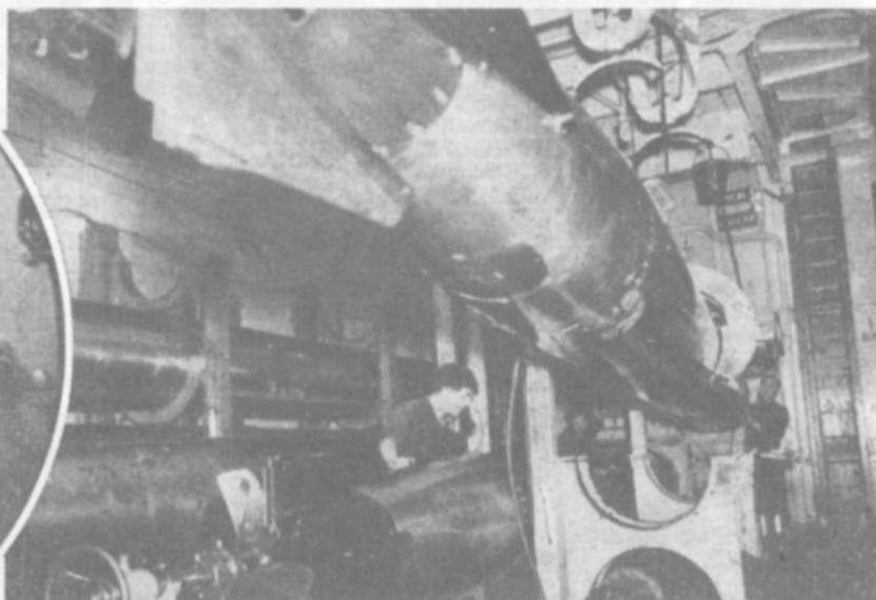
Practically all the ships of the Royal Navy from battleships to destroyers, except the very newest battleships, carry torpedo tubes. The torpedo-room in which the 21-in. "tin fish" are kept is seen in the photograph above. A torpedo is just being placed in the tube, while another is being lowered into position ready to follow it.
