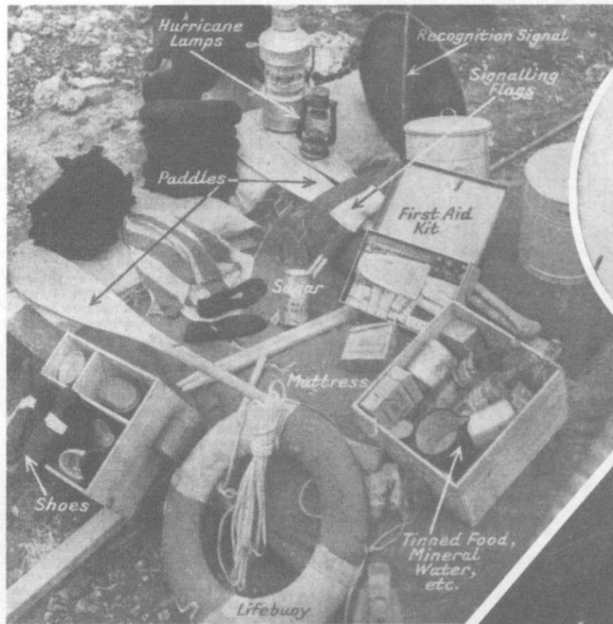
The equipment brought ashore from a refuge buoy which drifted across the Channel is seen, left, with the chief items labelled. Above is the upper part of the buoy, much battered by its involuntary cross-Channel trip.
