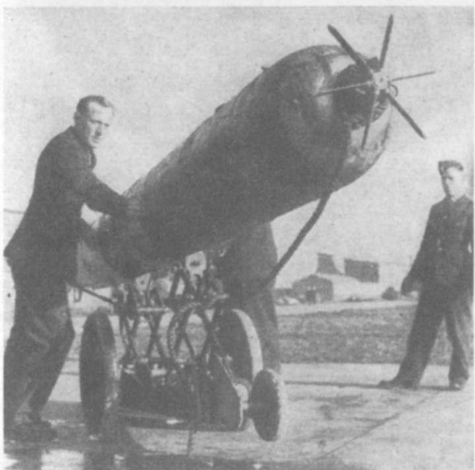
Some idea of the size of the torpedoes carried may be judged from the one above, which is being wheeled to the aircraft. Right, torpedo-carrying Albacores in flight.
