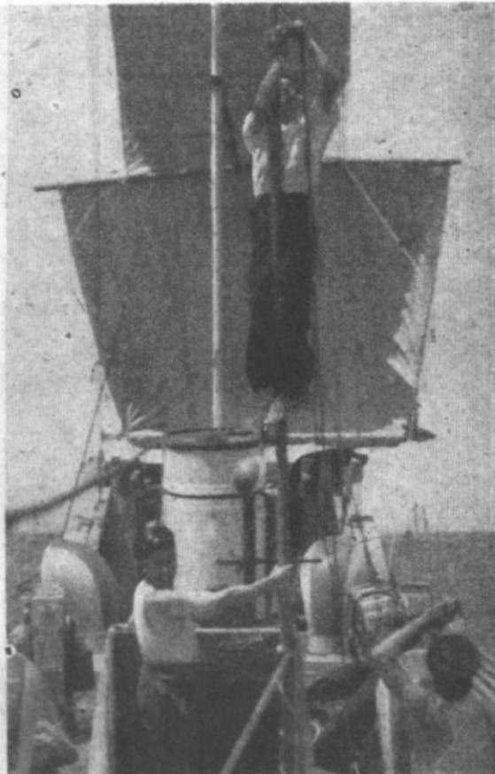
THE WANG-HO MAIN ROYAL tackle being fixed by a rating of the motor-launch. An awning, spars and boathooks went to the construction of this junk-like sail—an example of brilliant naval improvisation in emergency.
