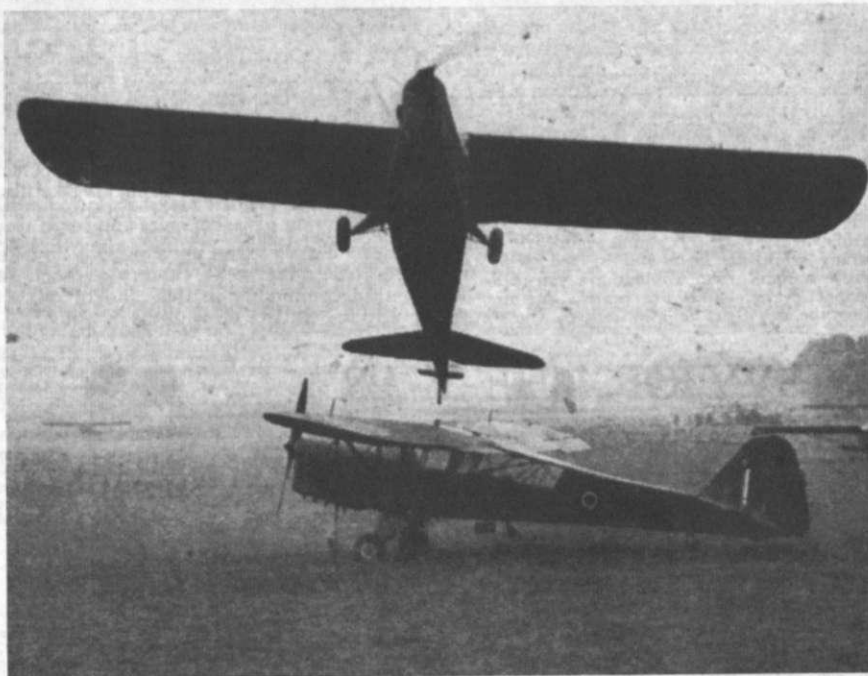
'EYES OF THE ARMY' is the apt nickname of the Taylorcraft Auster III, a two-seater R.A.F. plane able to take off in the astonishingly short distance of 50 yards and to land even in a roadway, a performance which makes it specially useful for military observation work. Its wingspan is only 36 feet, length 23 feet, height just over 6 feet. Top speed is 125 miles per hour. One is shown above in a steep climb over another of the same type. Photo, Keystone
