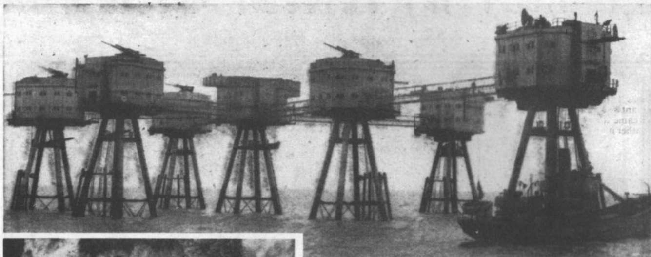
SEA FORTS OF CONCRETE AND STEEL built to guard the Thames Estuary from enemy mine-laying aircraft consist of circular towers each mounted on four concrete legs rising from the river bed, and connected by bridges. Six of these grouped towers carry A.A. guns; the seventh is a control tower. They are linked to the land by telephone, and manned by R.A. and other specialists.
