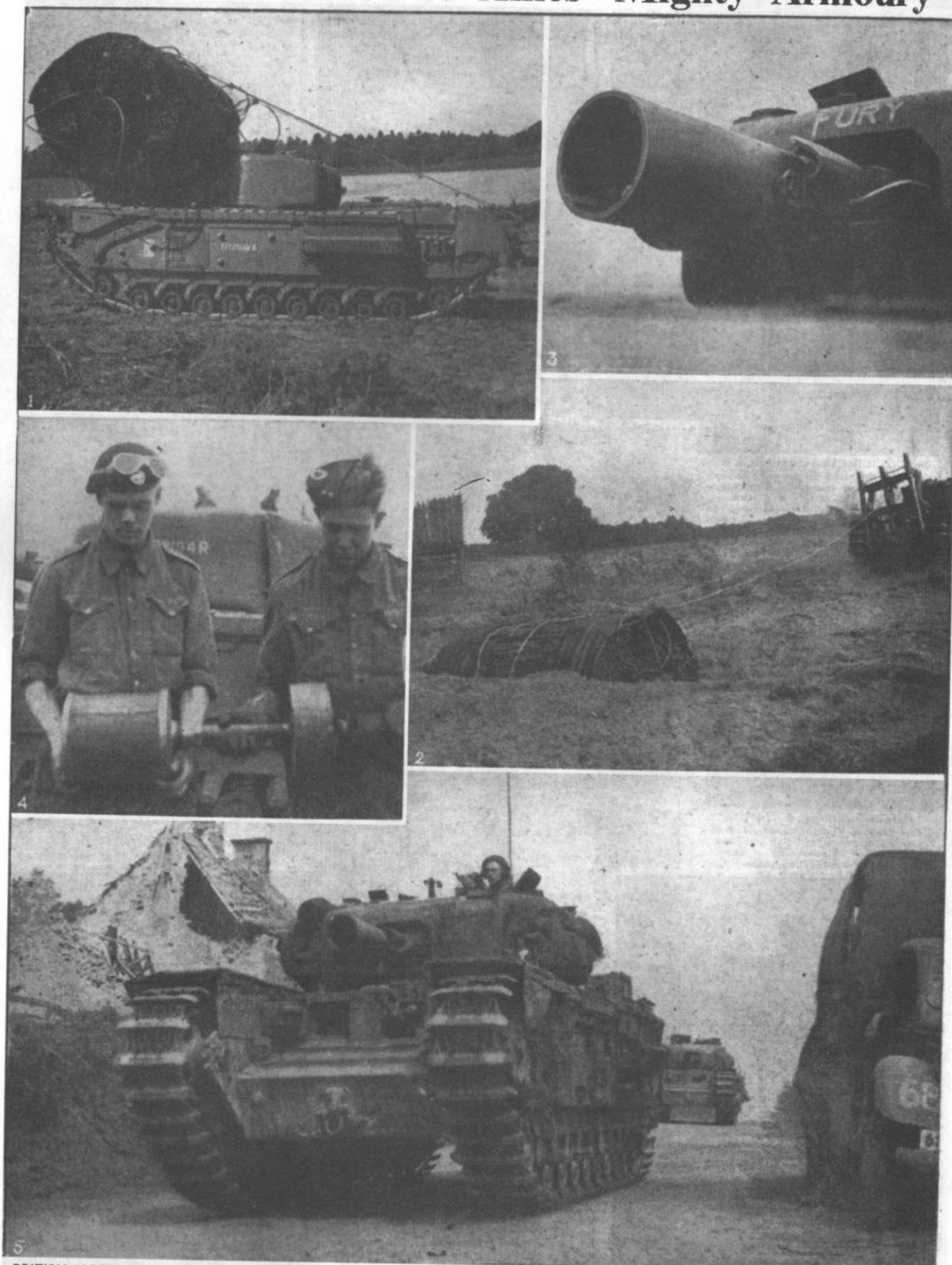
BRITISH MORTAR TANK, THE A.V.R.E. (Armoured Vehicle, Royal Engineers) specialises in the assault of powerful fortifications, such as the Siegfried Line, and the "West Wall" defences through which it smashed on D-Day. Resembling a Churchill, it carries a flexible track for carpeting insecure ground or forming a causeway across a hole, ditch or stream—a fascine or bundle of chestnut palings (1), which is unloaded (2) where required. Main armament is a mortar mounted in the turret (3); this hurls a "flying dustbin" (4) containing a great weight of explosive. A.V.R.E. moving up in France (5).
