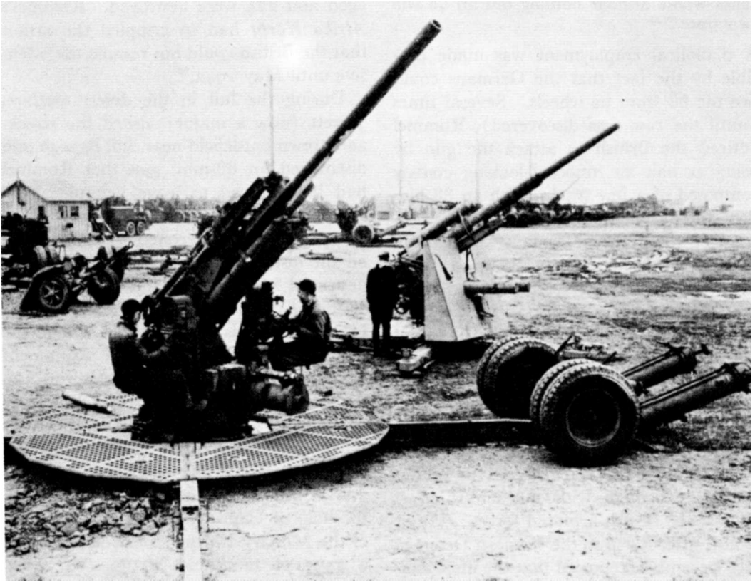
THE U.S. 90-MM. AND THE GERMAN 88-MM. ANTI-AIRCRAFT GUNS ( left and right, respectively ) at Aberdeen Proving Ground, 1943.
