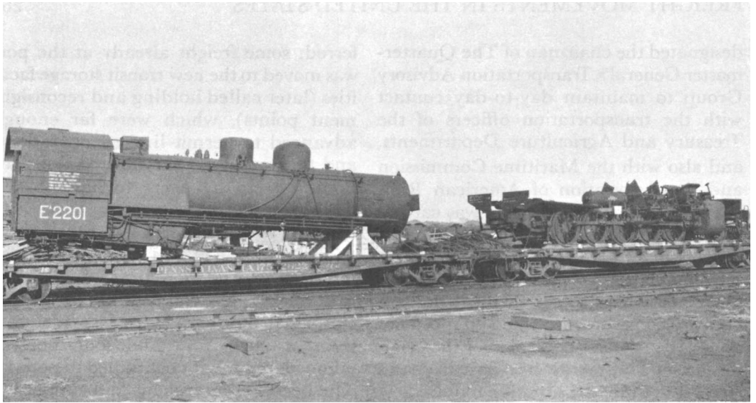
LOCOMOTIVES SHIPPED AS RAILWAY FREIGHT. Broad-gauge locomotives moving to Portland, Oregon, to be assembled and shipped to the Soviet Union (above); boxed diesel locomotives on flatcars (below).
