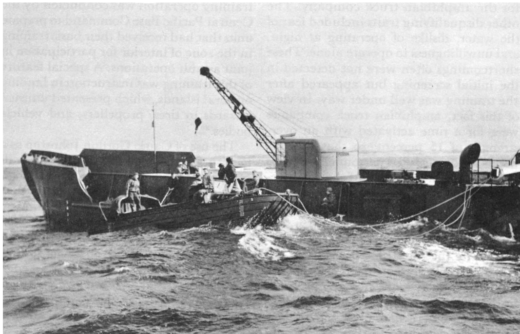
AMPHIBIAN TRUCK COMPANY TROOPS IN TRAINING. DUKW's practice entering a heavy surf (above); a DUKW in choppy water receives cargo over the side of a training barge (below).
