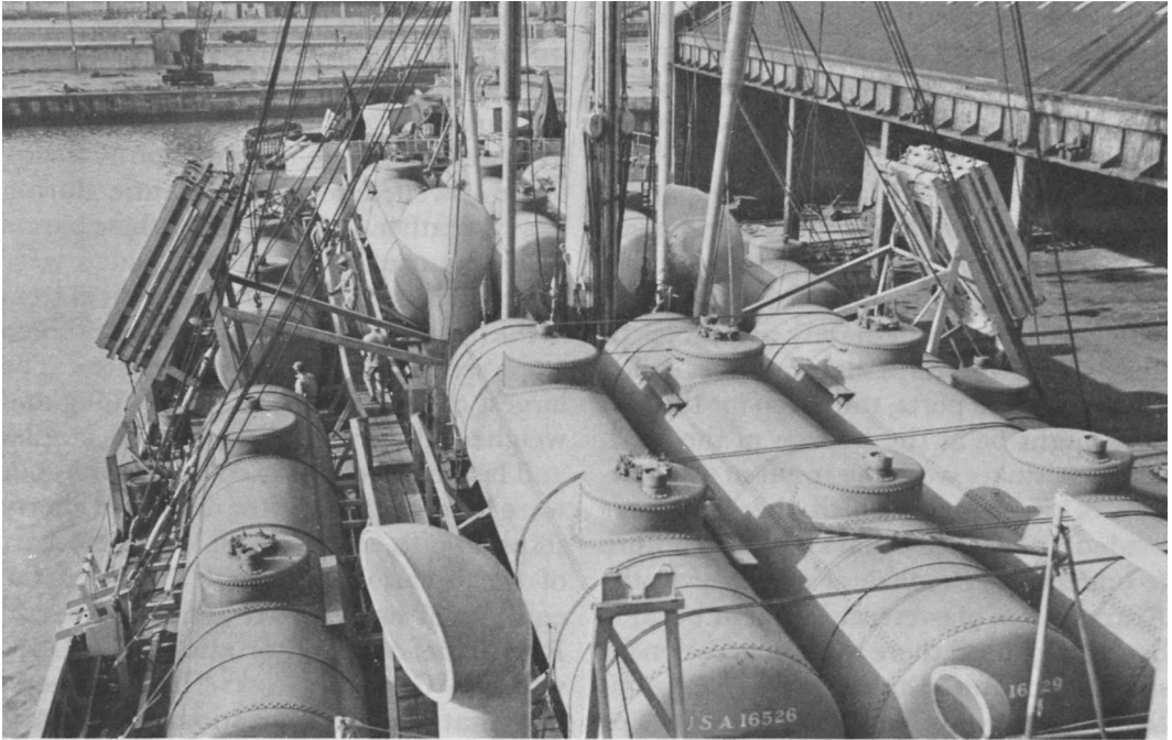
TEN RAILROAD TANK CARS ON THE FORWARD DECK of a Liberty ship; an equal number was carried on the after deck.
