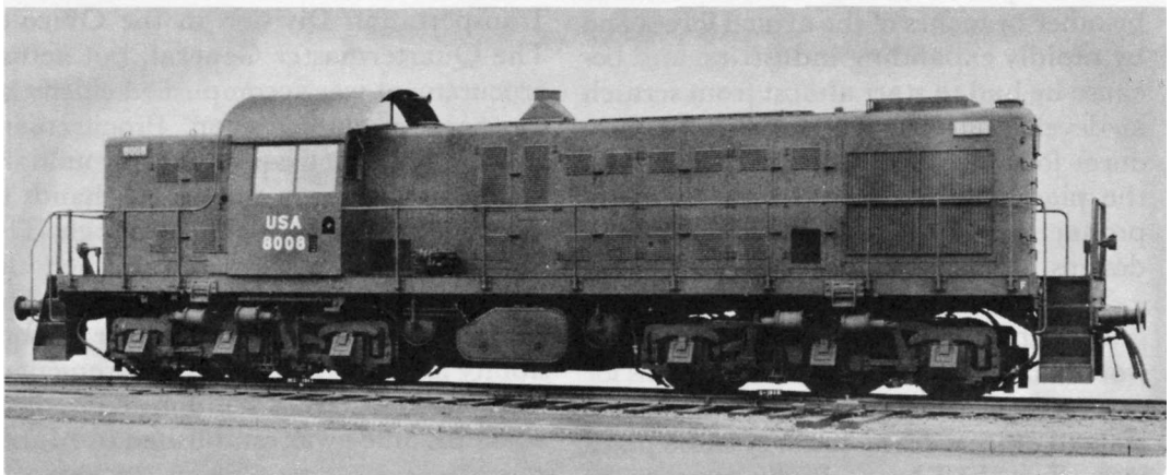
U.S.-BUILT LOCOMOTIVES FOR SERVICE OVERSEAS. The 2-8-0 standard-gauge steam locomotive procured by the Military Railway Service (top); the 2-10-0 broad-gauge steam locomotive procured for shipment to the Soviet Union under lend-lease (middle); the 127-ton diesel locomotive of the type used by the MRS in Italy and Iran (bottom).
