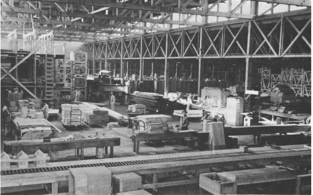
PROCESSING AND CRATING SHOP at the Lathrop, California, Holding and Reconsignment Point.
