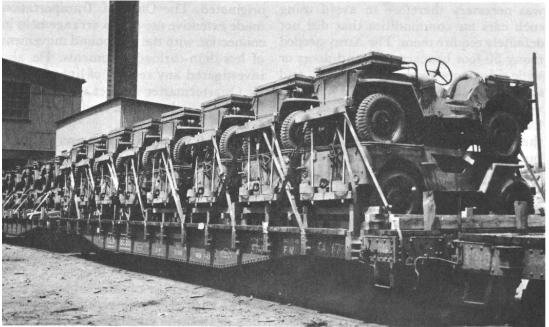
SIXTEEN ¼-TON TRUCKS LOADED ON A FLATCAR by double-decking
