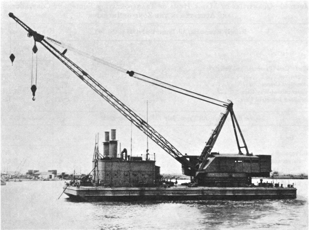
REVOLVING FLOATING CRANE with 60-ton capacity.
