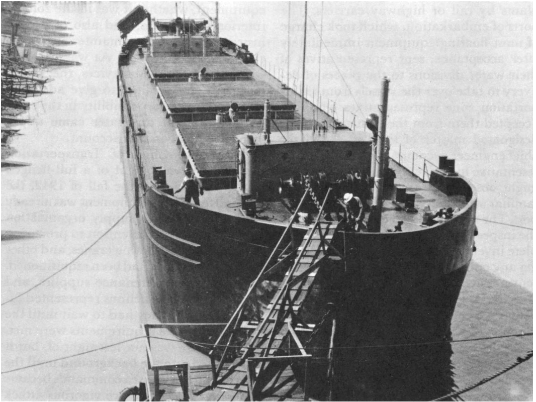
SEAGOING STEEL BARGE UNDER CONSTRUCTION for Transportation Corps
