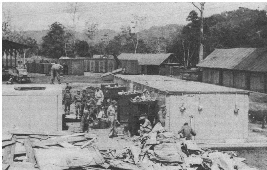
PREFABRICATED REFRIGERATED WAREHOUSES are shown in process of assembly at Oro Bay, New Guinea.
