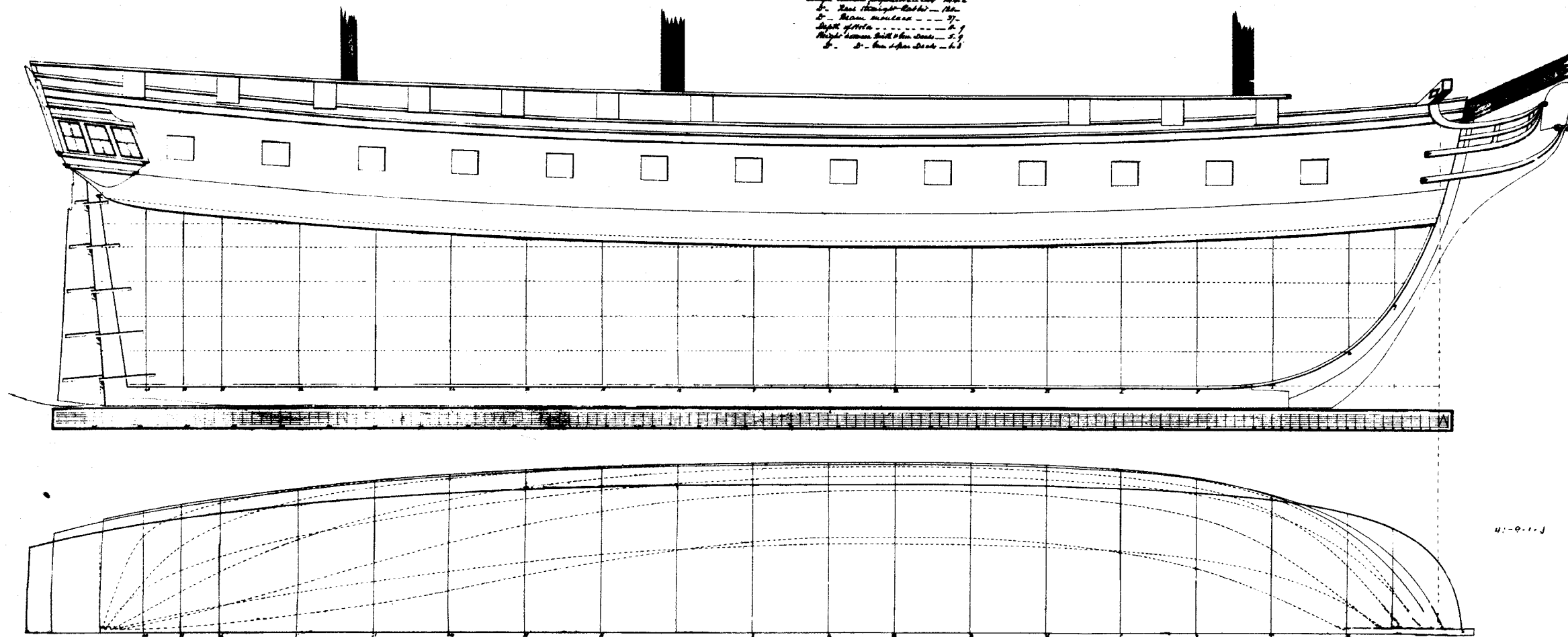
PLATE VI. LINES OF THE UNITED STATES FRIGATE NEW YORK.
