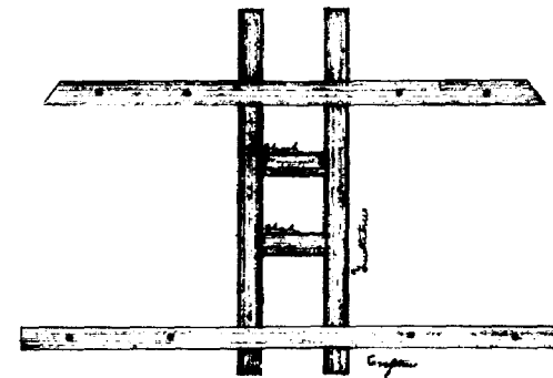
Fore Mast Luff and Cap
