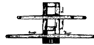
Fore Topmast Luff and Cap
