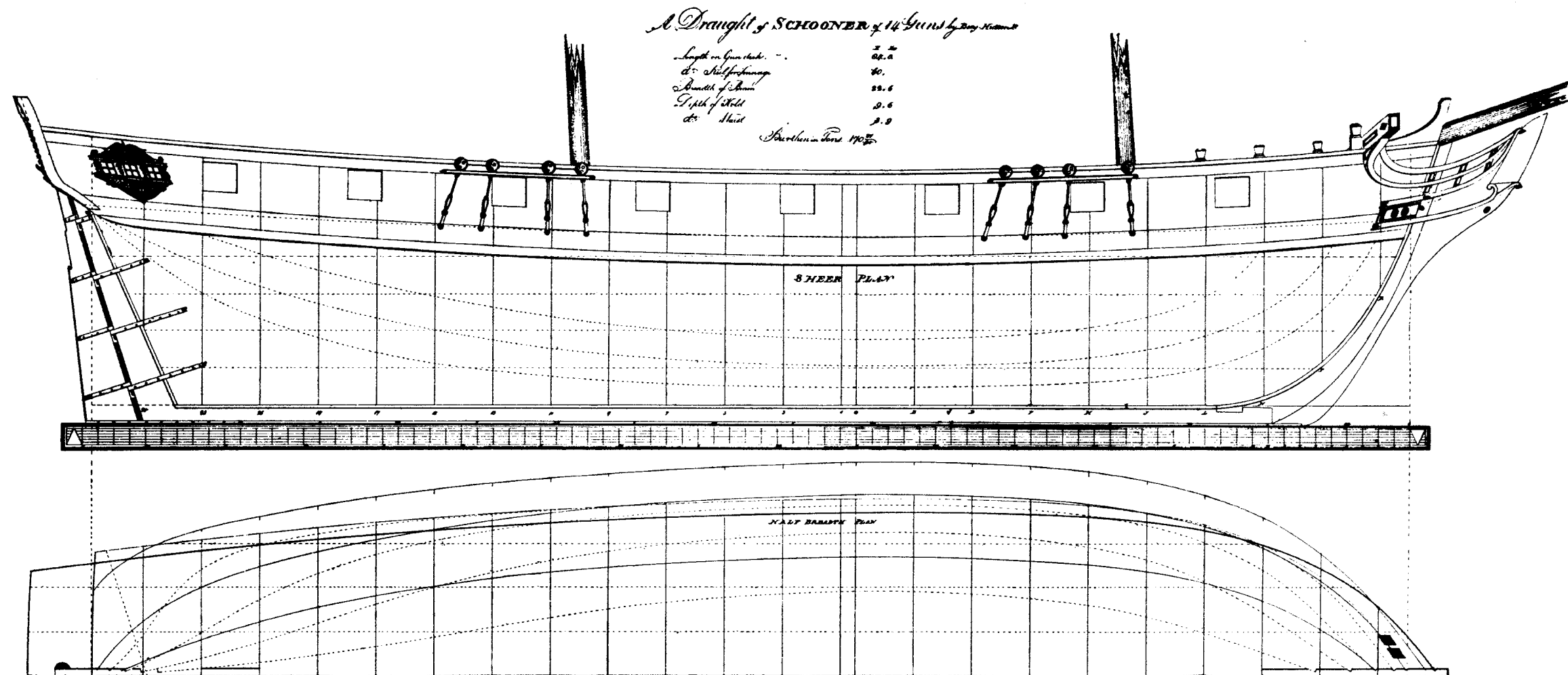
PLATE IX. LINES OF THE UNITED STATES SCHOONER (LATER BRIG) VIXEN
