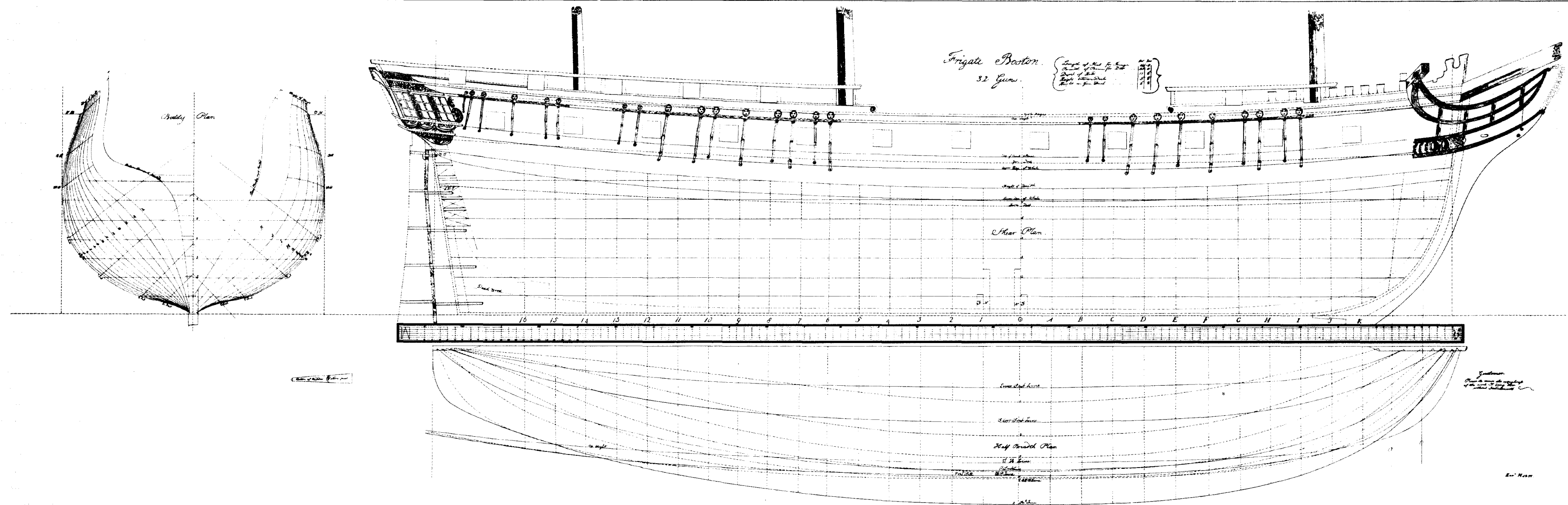
PLATE II. LINES OF THE UNITED STATES FRIGATE BOSTON.
