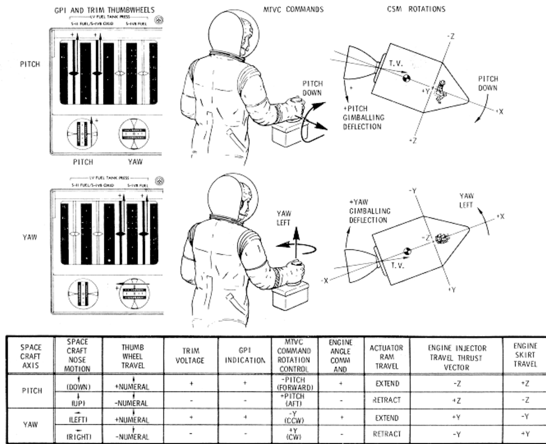
Figure 2.4-11. SPS Gimballing
