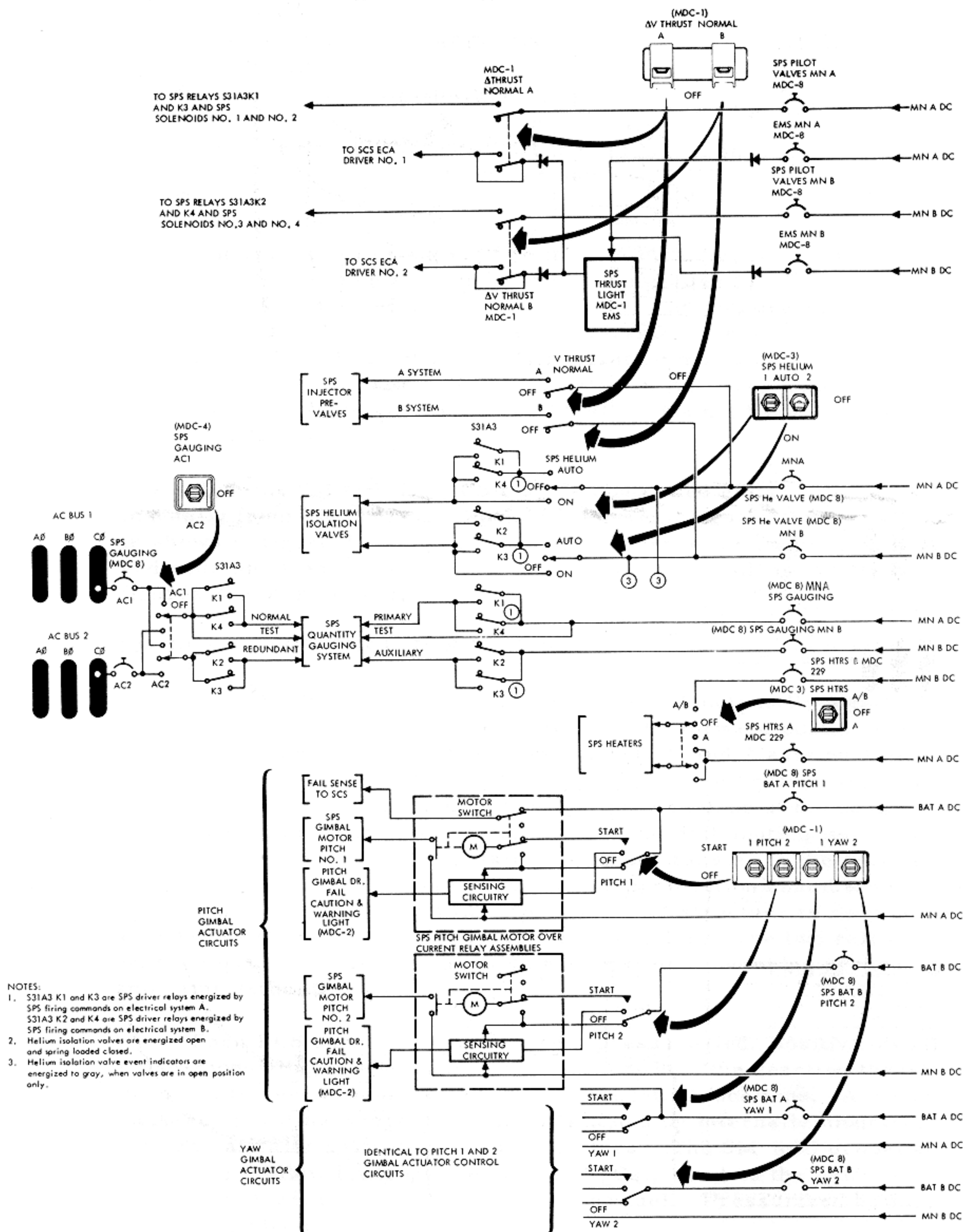
Figure 2.4-18. Electrical Power Distribution (CSM 112 and Subs)
