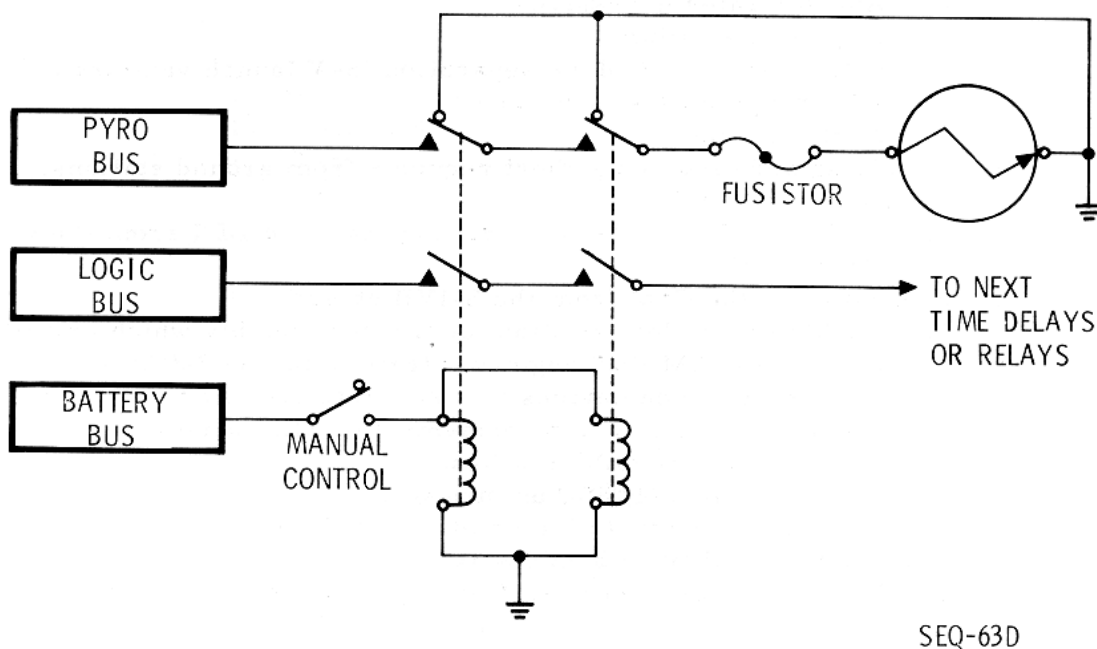
Figure 2.9-18. Circuit Concept
