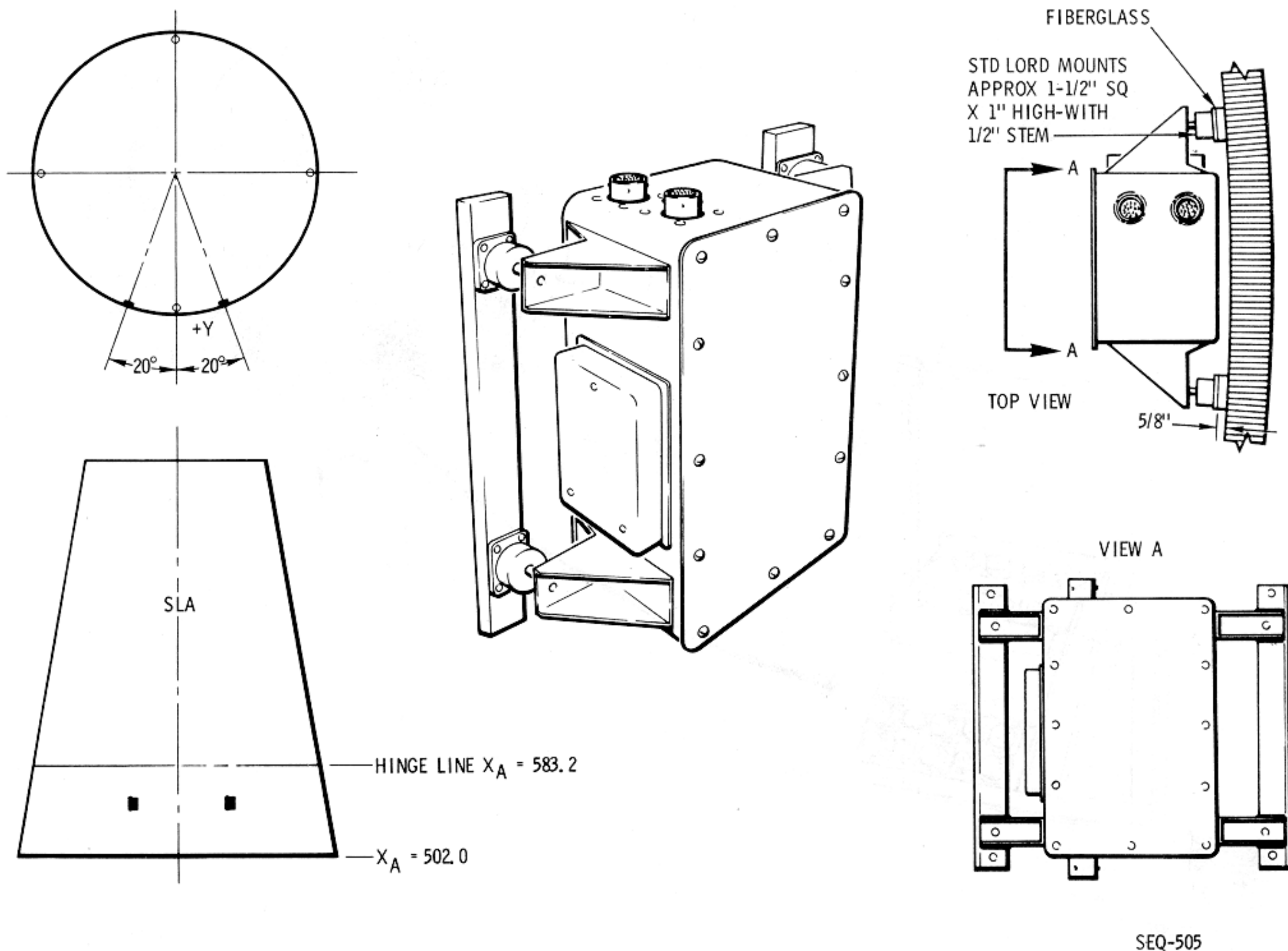
Figure 2.9-6. LSSC Location
