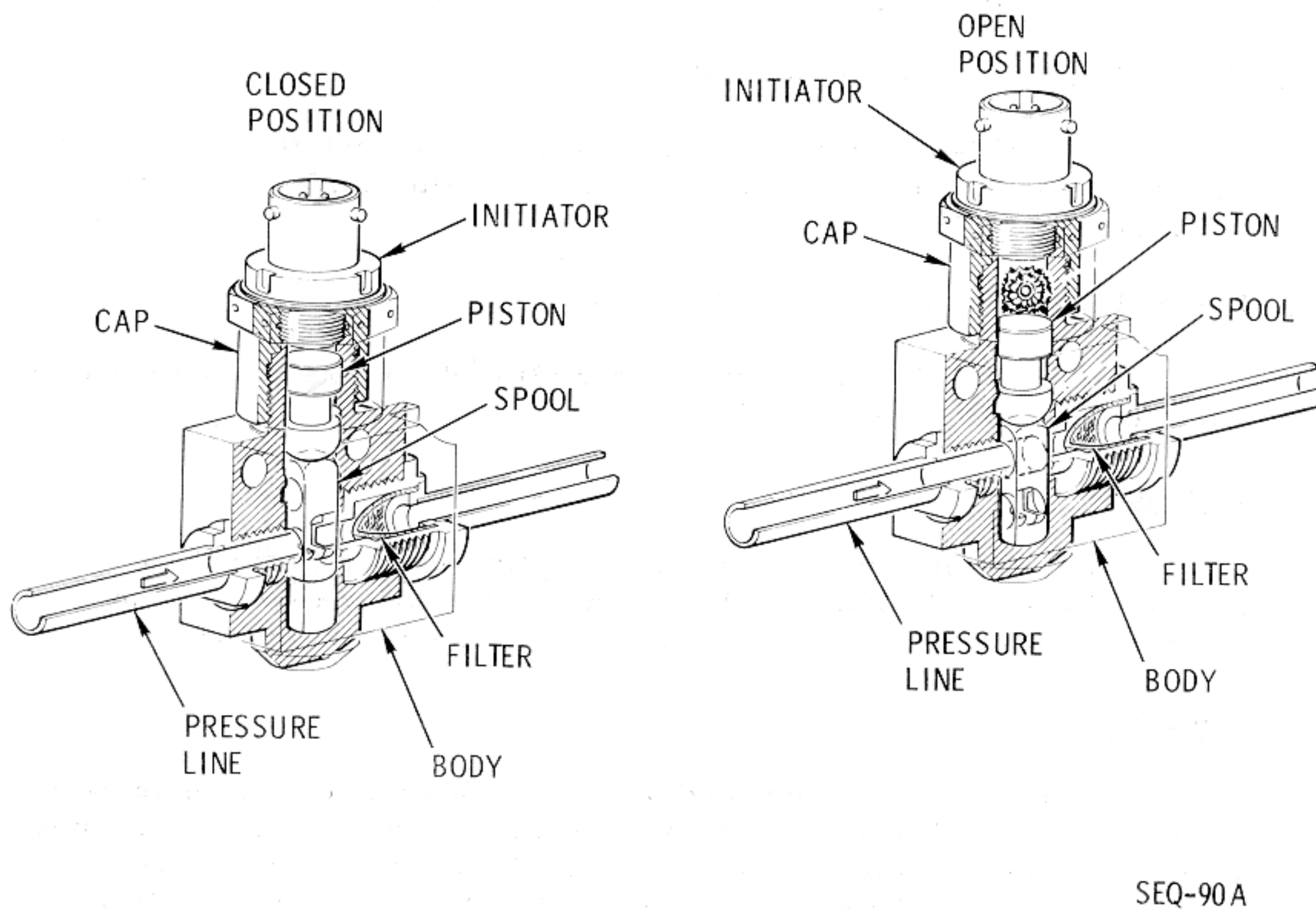
Figure 2.9-44. Squib Valve
