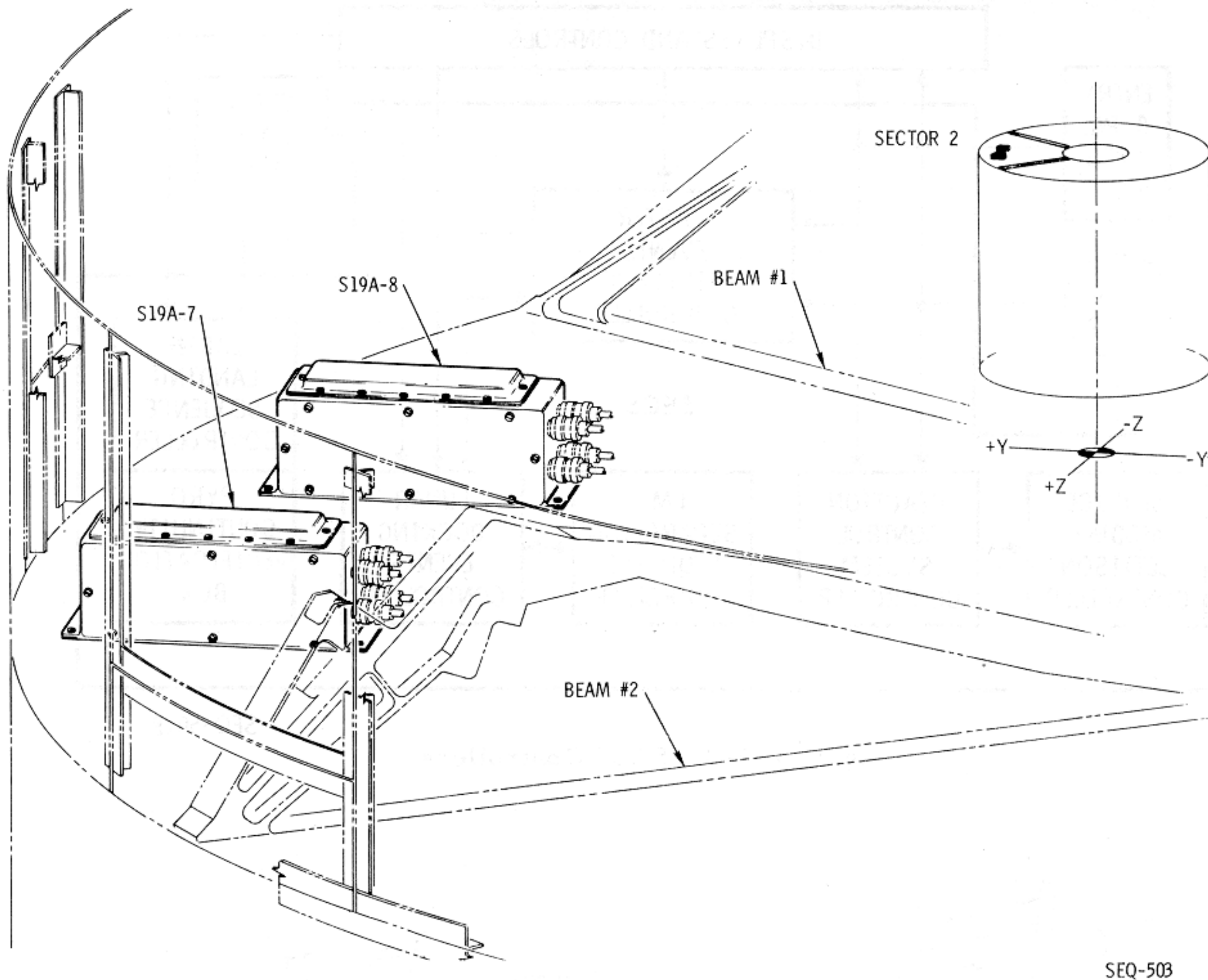
Figure 2.9-4. SMJC Location
