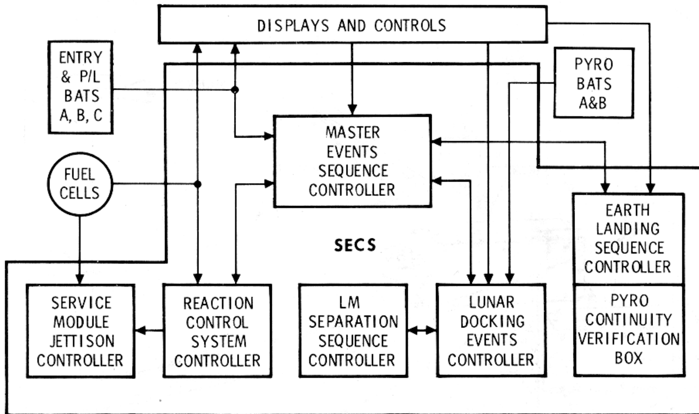
Figure 2.9-2. SECS Controllers
