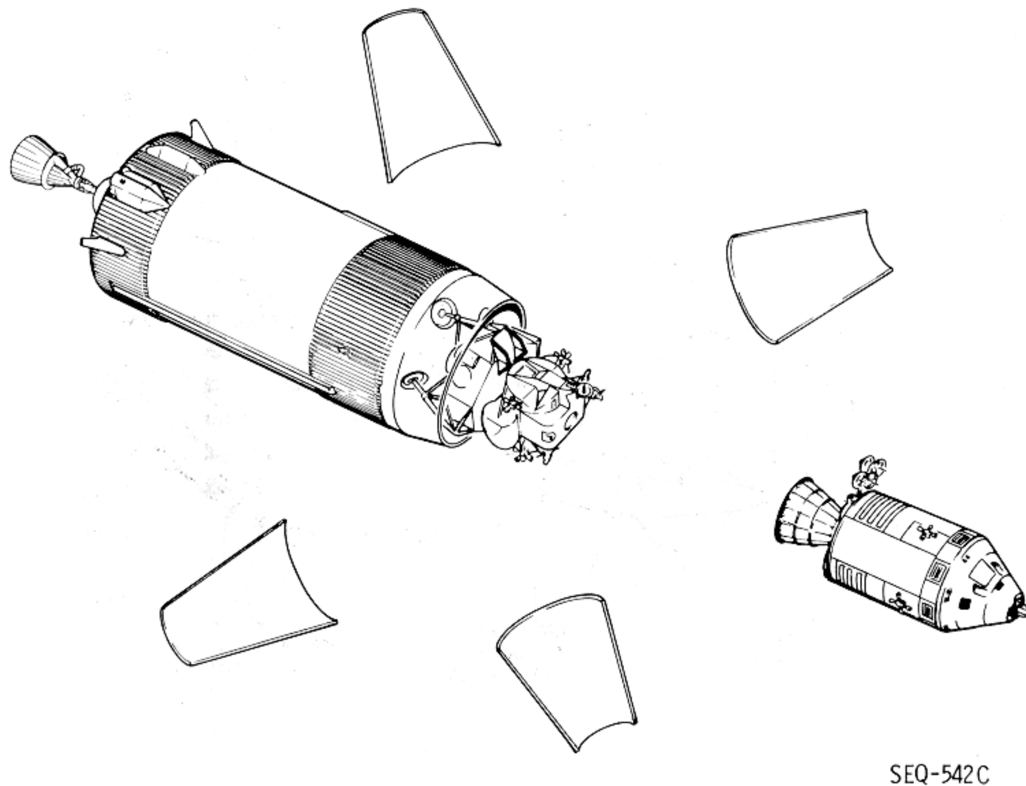
Figure 2.9-9. Normal CSM/LV Separation
