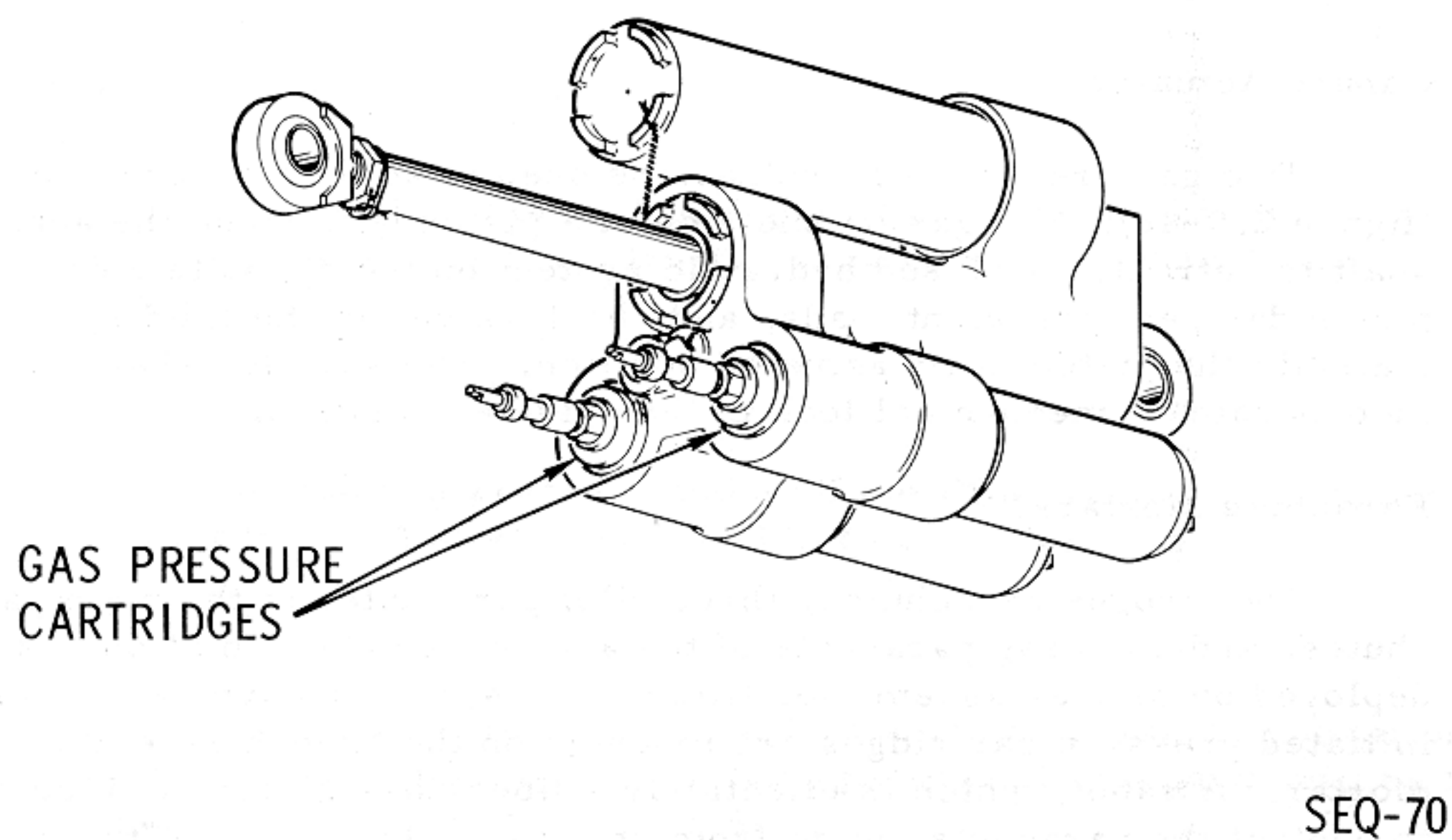
Figure 2.9-48. Canard Actuator
