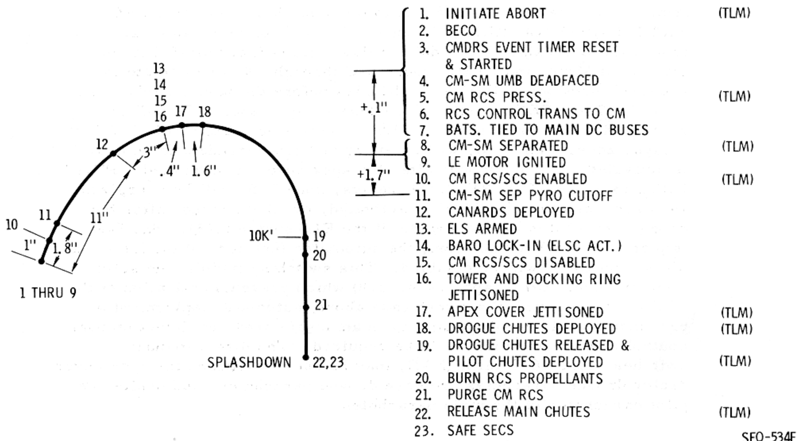
Figure 2.9-34. Event Profile, Mode 1B Abort T + 42 Sec to \approx 30,000 Feet
