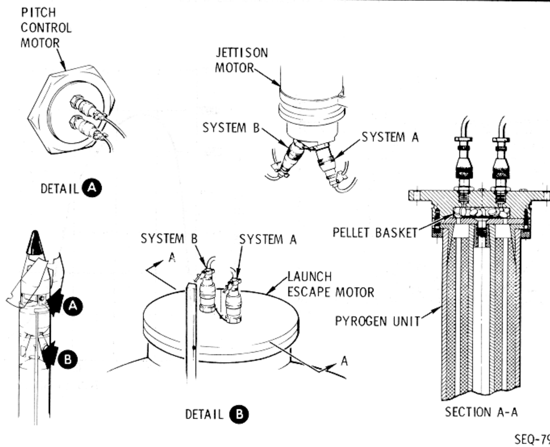
Figure 2.9-43. LES Igniters
