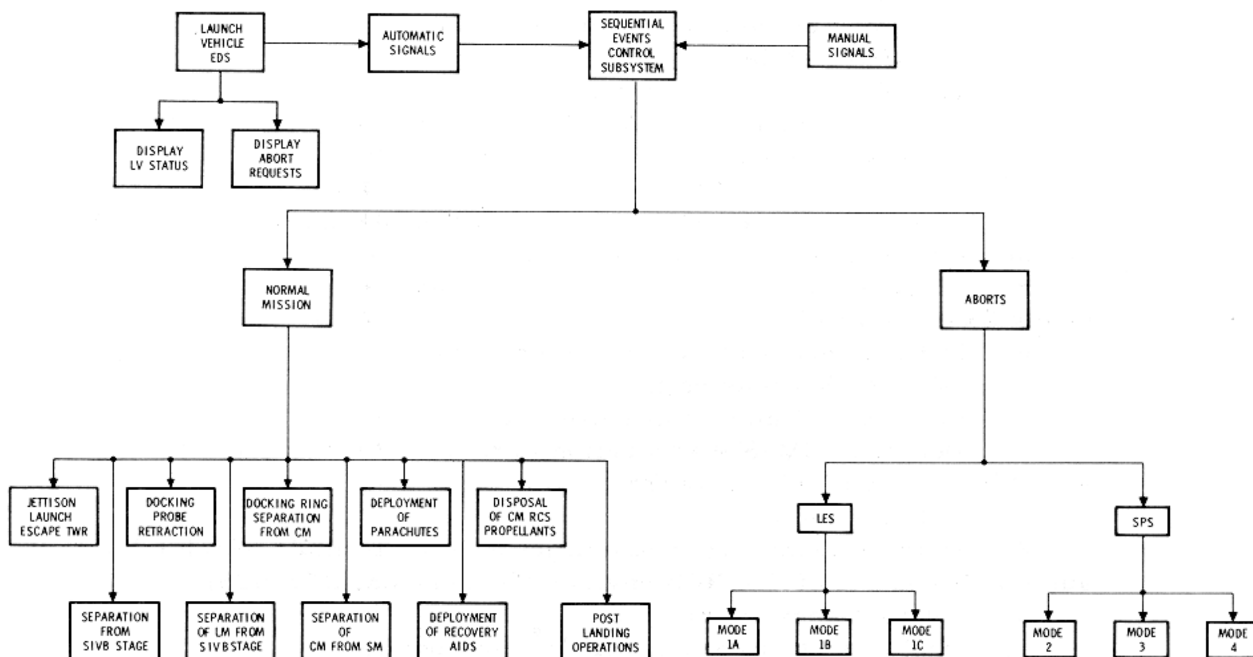
Figure 2.9-18. Circuit Concept
