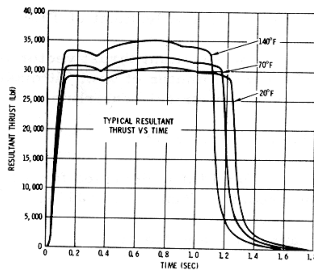
Figure 2.9-40. Tower Jettison Motor
