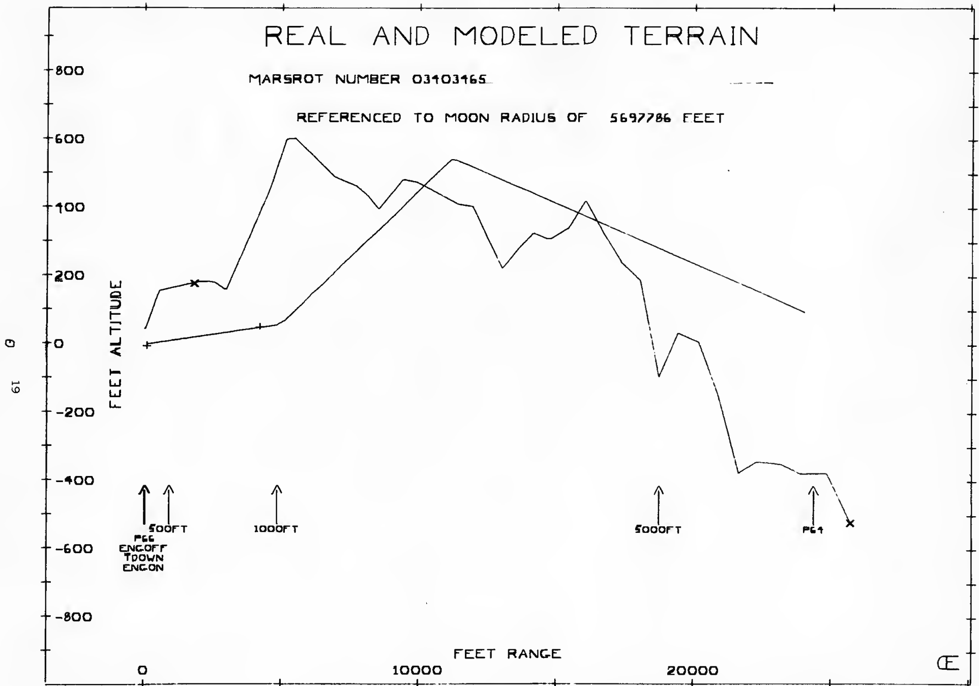
Figure 6C Land 4850 ft. Before Nominal Site
