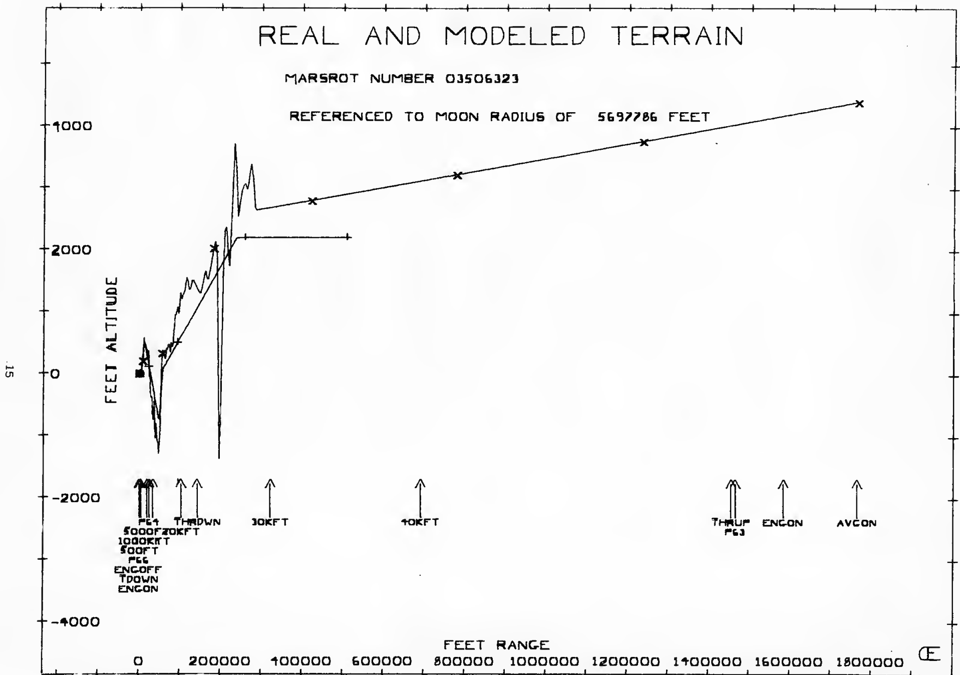
Figure 5B Land at Nominal Site
