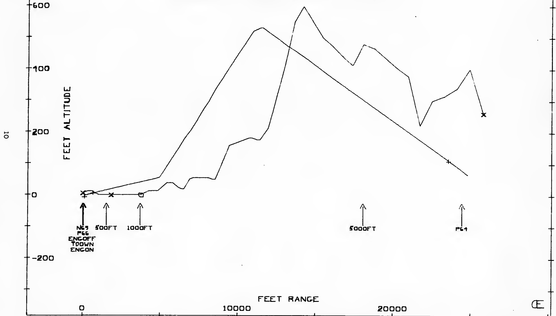
Figure 3C Land 3280 ft. Beyond Nominal Site
