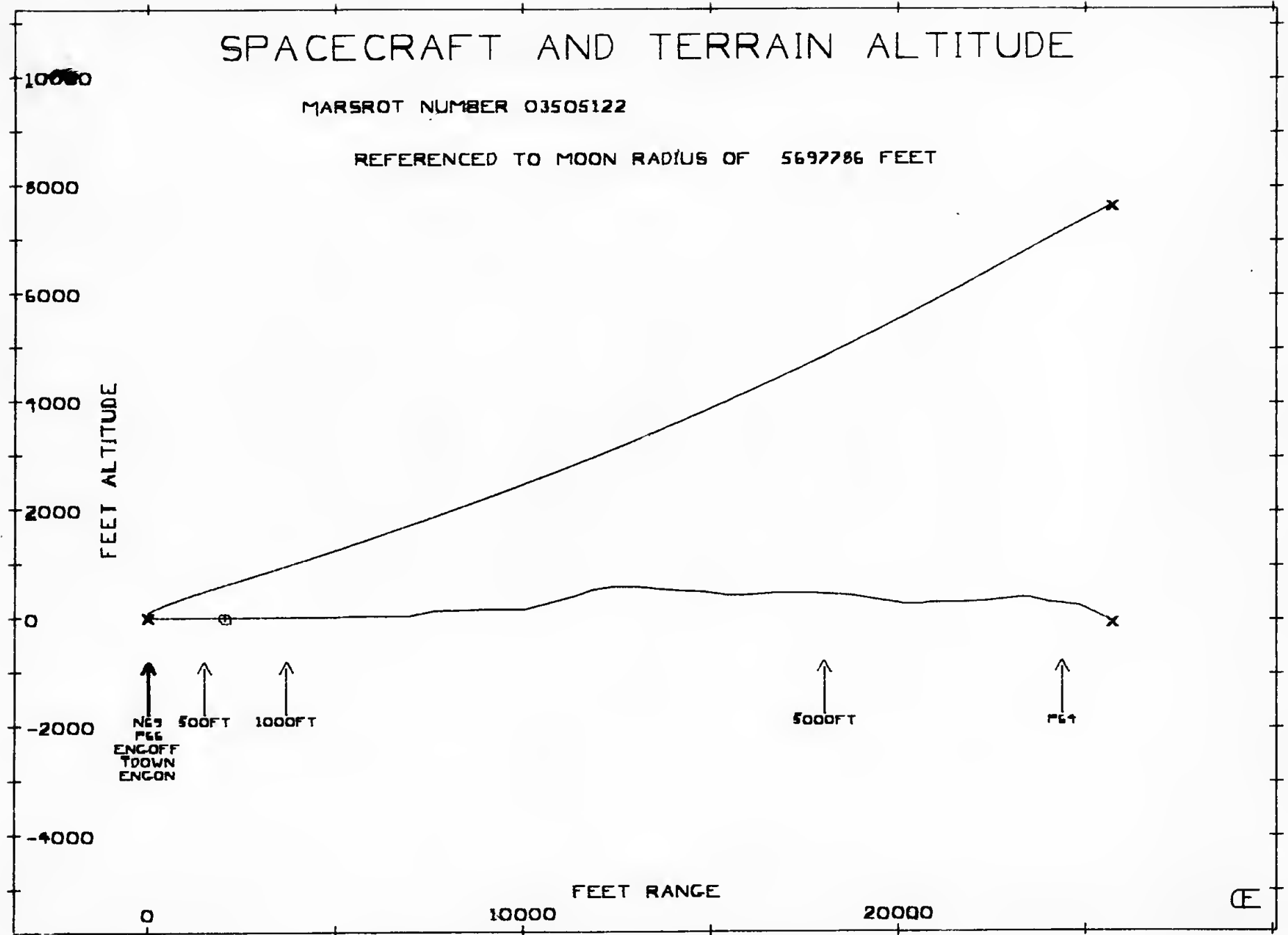
Figure 4A Land 1640 ft. Beyond Nominal Site
