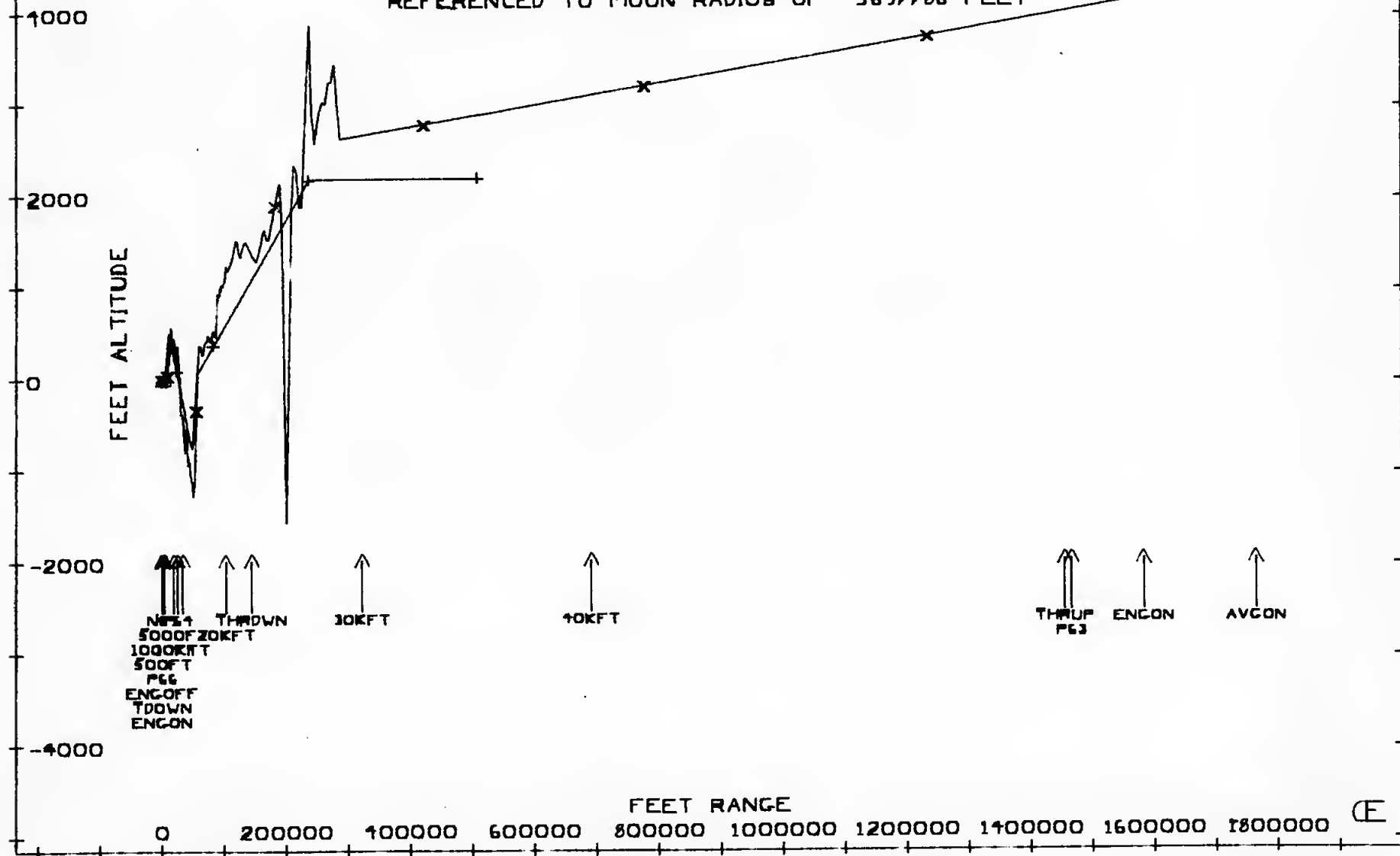
Figure 3B Land 3280 ft. Beyond Nominal Site
