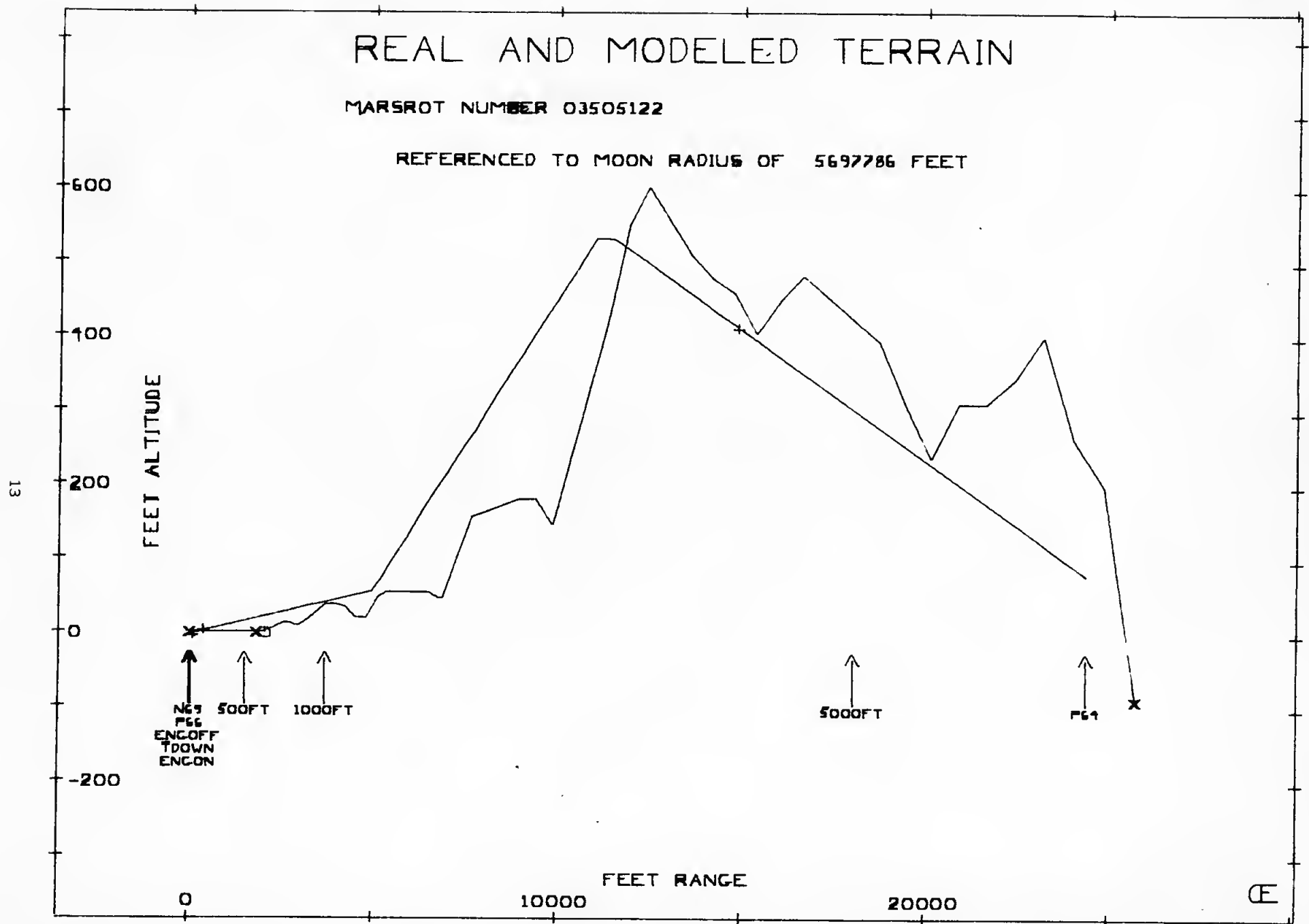
Figure 4C Land 1640 ft. Beyond Nominal Site
