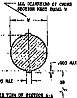
ENLARGED VIEW OF SECTION A-A
