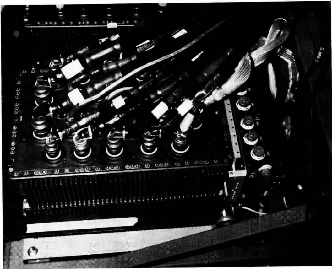
Figure 4-10. A Shuttle Main Engine Controller mounted in an engineering simulator at the Marshall Space Flight Center. (NASA photo)
