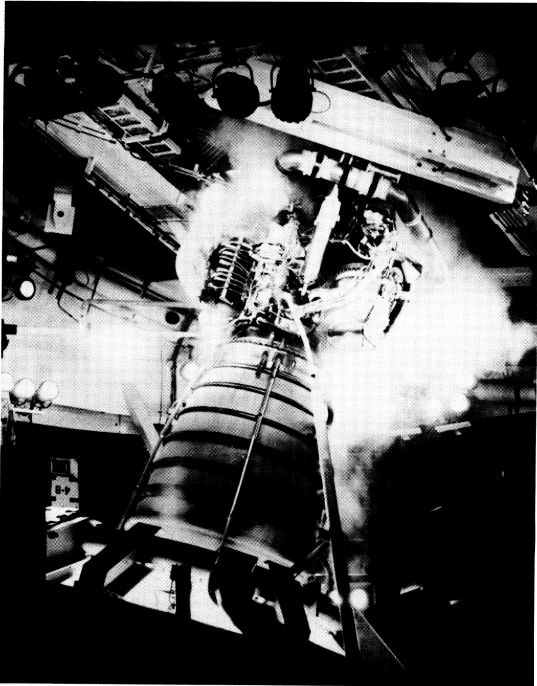
Figure 4-11. A Shuttle main engine in a ground test. The Controller can be seen mounted on the left side of the combustion chamber. (NASA photo 885338)
