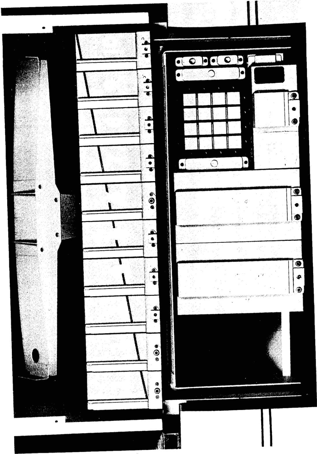
Fig. 10 Command Module Lower Equipment Bay
