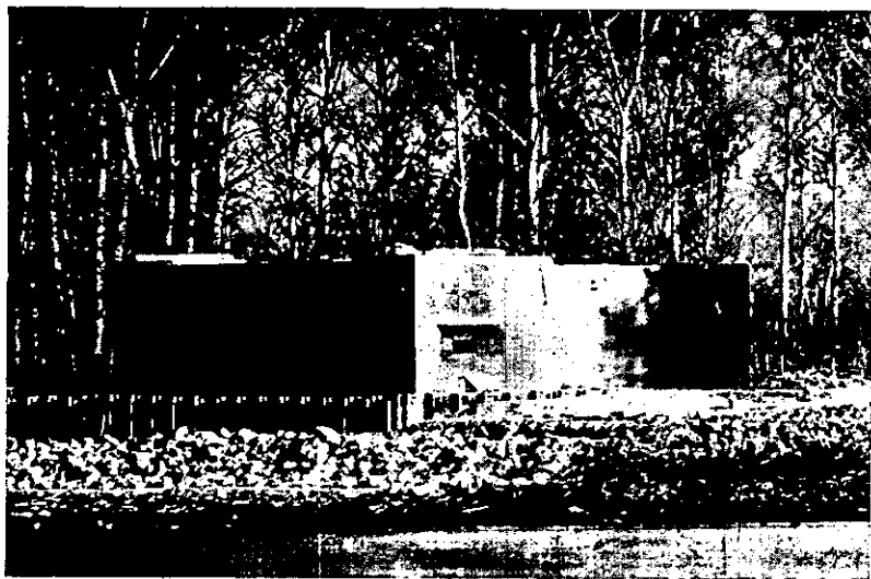
Figure 25.—Double flanking casemate, with wing-walls.
