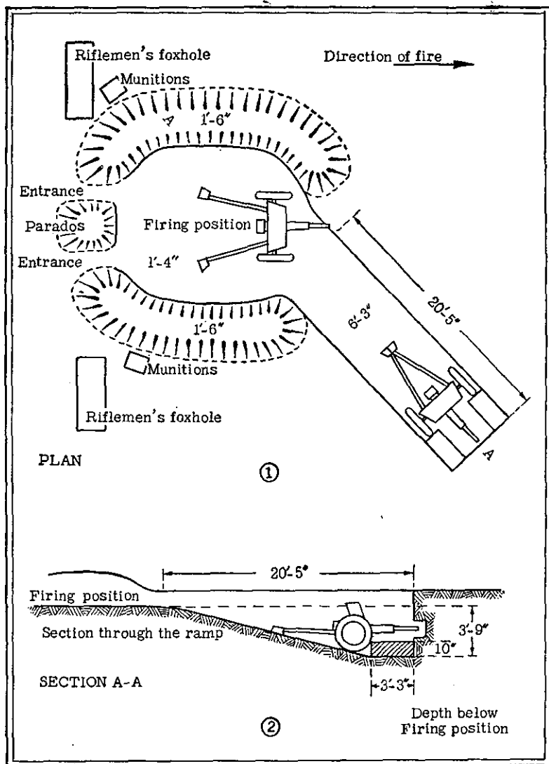
Figure 47.—Enplacement for antitank gun, with ramp.
