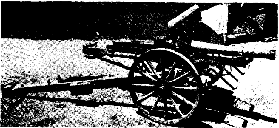
Figure 144.—Type 91 (1931) 105-mm howitzer.
