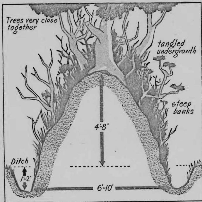
Cross Section of Typical Normandy Hedgerow.
