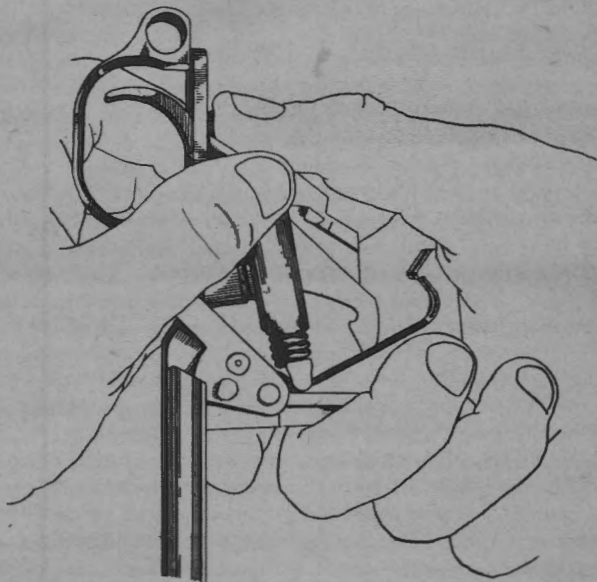
FIGURE 16.—Seating the trigger pin.
