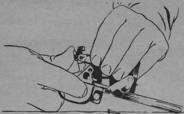
FIGURE 12.—Releasing hammer spring.
