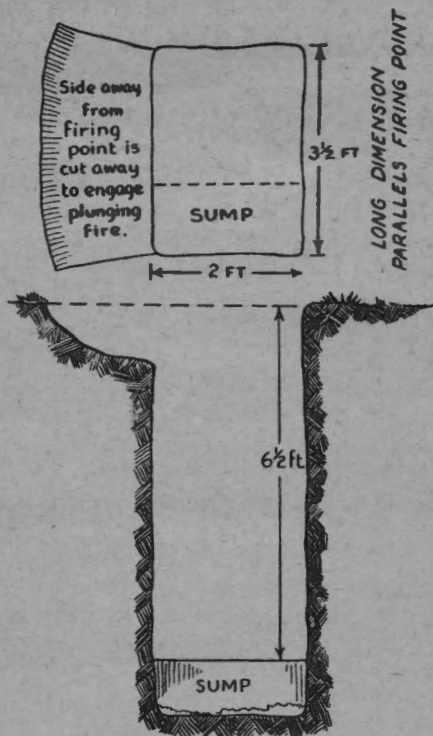
FIGURE 124.—Construction of open pit.
