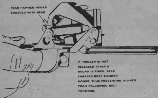
FIGURE 22.—Rear hammer hooks engaged with sear.
