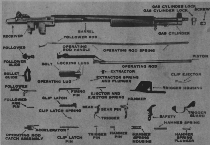
FIGURE 2.—Parts of U. S. rifle, caliber .30, M1.
