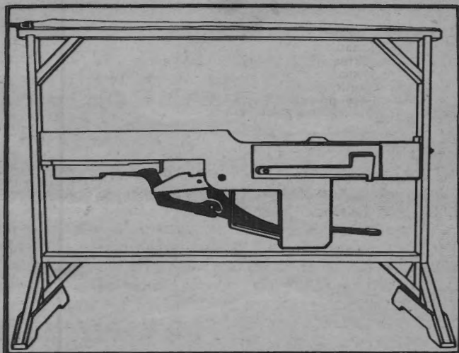
FIGURE 119.—Working model—M1 rifle.
