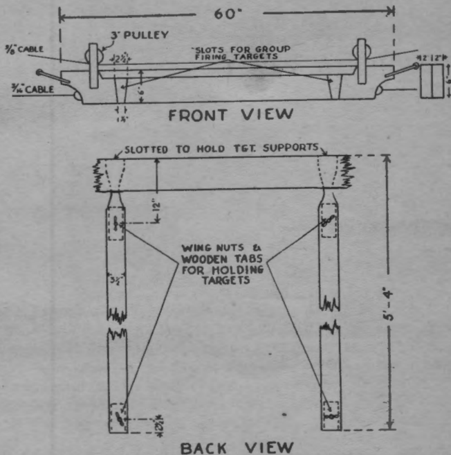
BACK VIEW SUPPORTS FOR INDIVIDUAL FIRING TARGETS FIGURE 73.—Nonoverhead target carrier.
