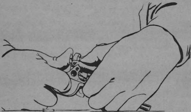
FIGURE 15.—Compressing the hammer spring.
