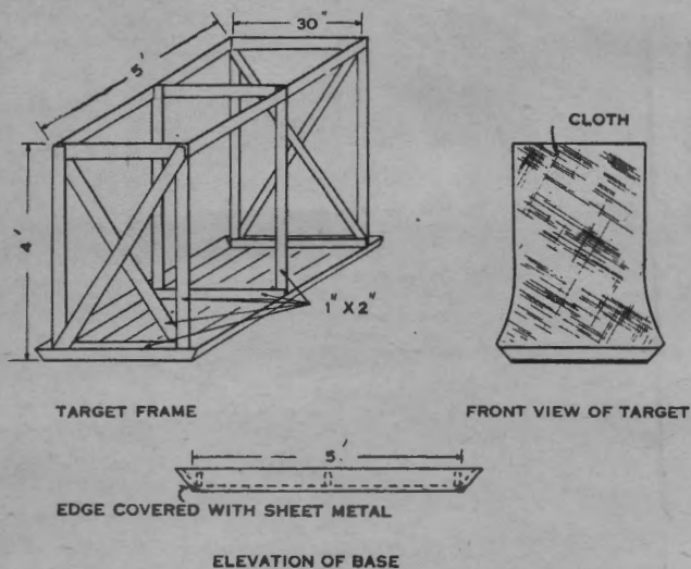
FIGURE 55.—Target frame for moving-target range.
