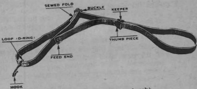
② Gun sling M1 (improved web)
