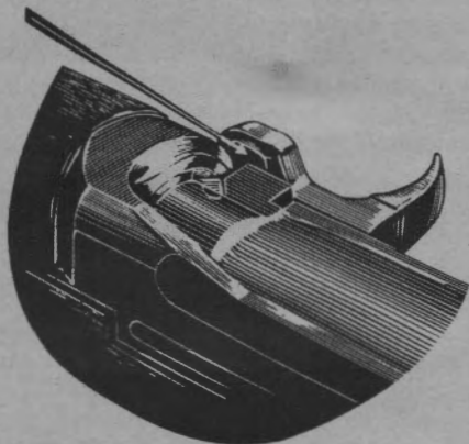
CAMMING SURFACE IN HUMP OF OPERATING ROD
