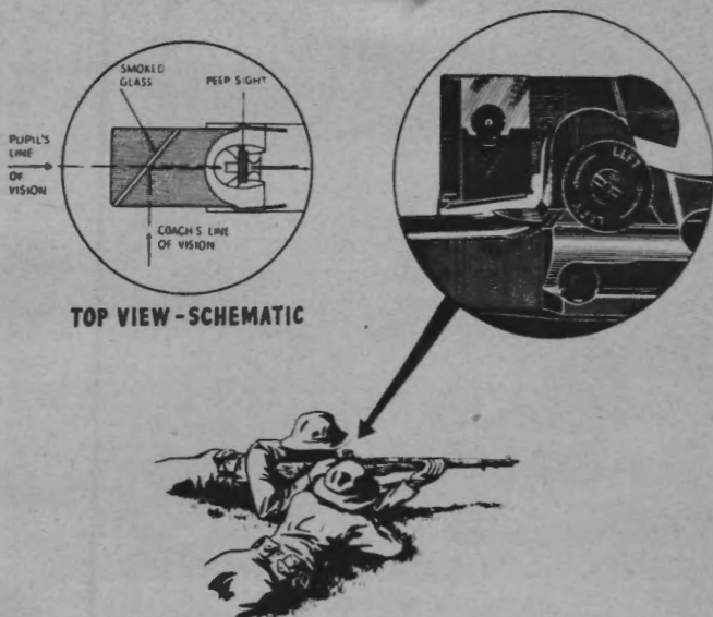
FIGURE 26.—Aiming device.
