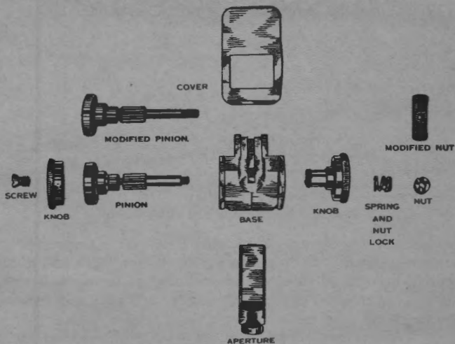
Ⓢ Parts disassembled.
