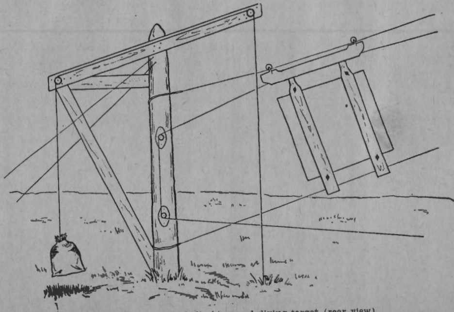
FIGURE 75.—Details of climbing and diving target (rear view).
