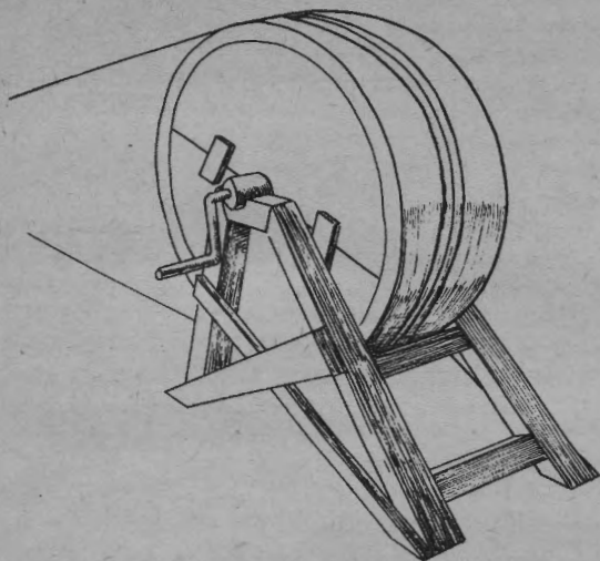
FIGURE 74.—Cable drum.
