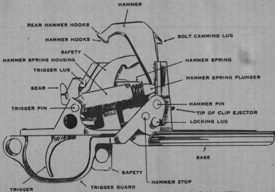
FIGURE 19—Trigger housing group with hammer in fired position.
