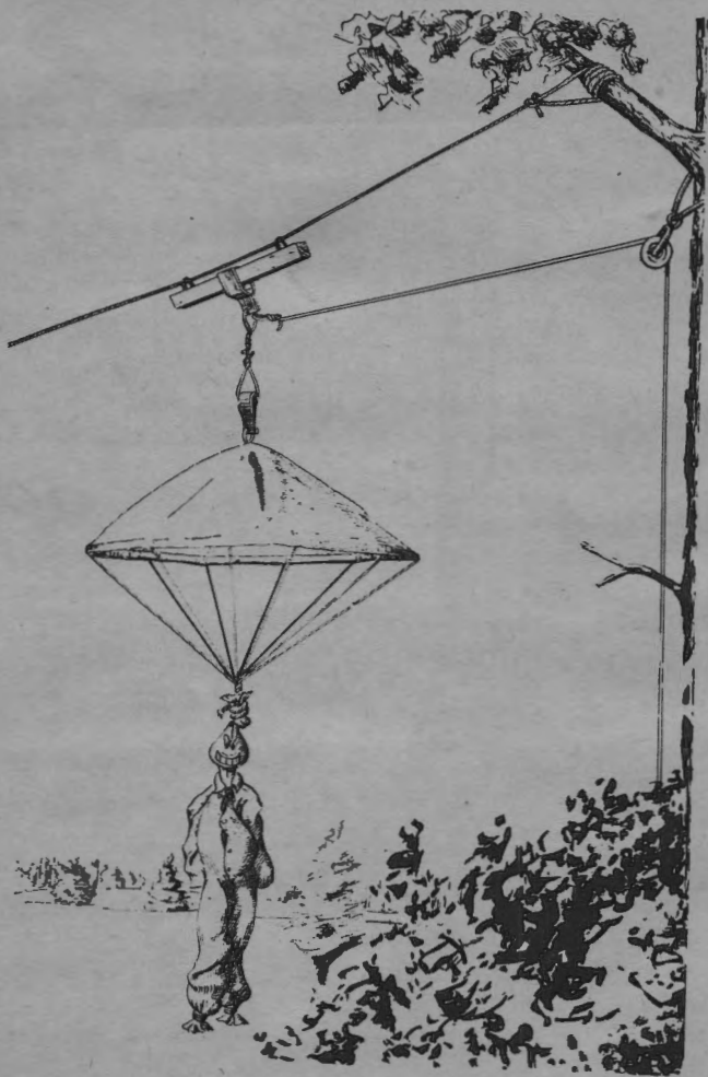
FIGURE 114.—Arrangement for raising and lowering surprise target (parachute). Note control rope leads to pit.
