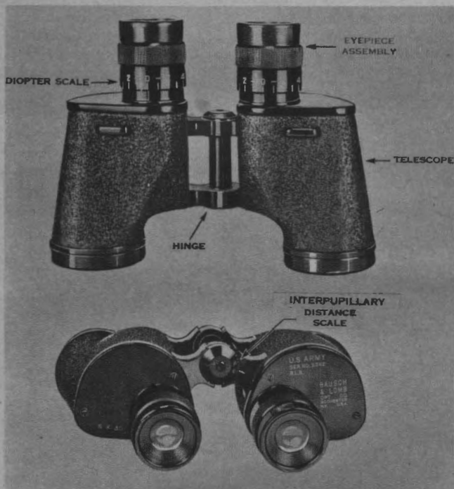
① Binocular, M3.
