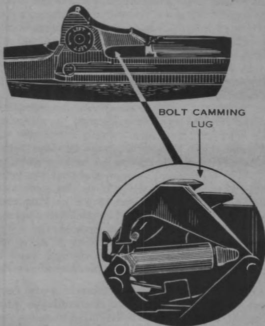
② FIGURE 18.—Points on which to apply rifle grease.
