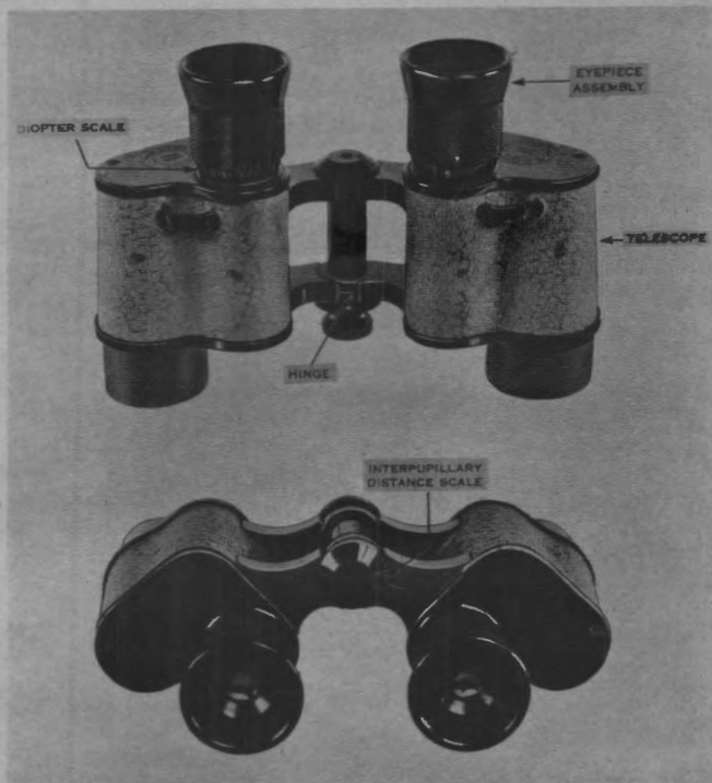
② Binocular, type EE.
