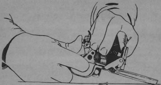
FIGURE 14.—Replacement of trigger assembly and hammer spring housing (note position of sear pin).
