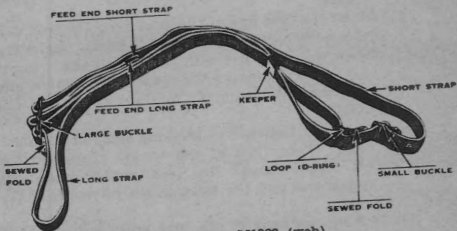
③ Gun sling M1923 (web).
