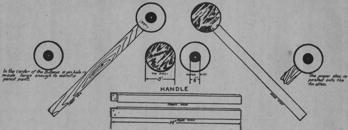
FIGURE 53.—Sighting disk
