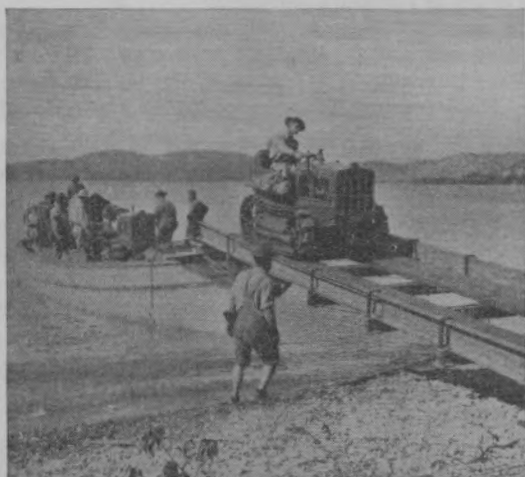
FIGURE 4.—Unloading tractors from 50-foot motor launch equipped with boat rig A and ramp.
