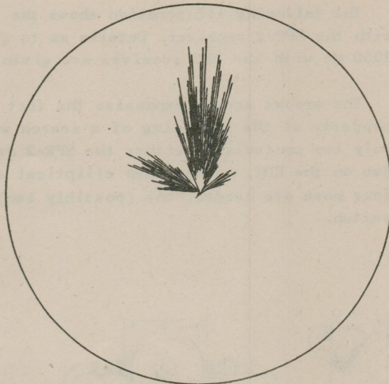
A typical picture of a pattern of a lobe switching radar on a DBM-1 shows that the pulses are of different lengths but do not appear to be arranged in groups.
