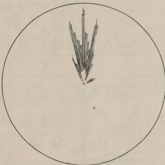
This drawing was made directly from a photograph of a response from a lobe-switching radar with a PRR of 1640 cycles at a time when the radar was searching.
