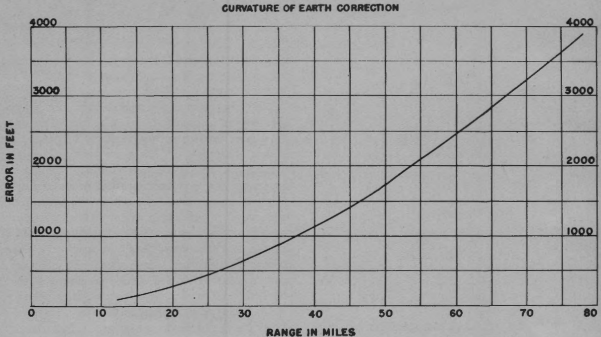
Figure 4 SP-7. Curvature of the earth correction.
