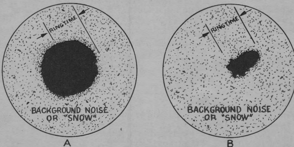
Figure 4 OBU-9. Measuring ringtime on PPI. A. When directional coupler is used. B. When pick-up dipole is used and is not mounted on antenna so as to rotate with it. Note that measurement is made at outermost fringe of echo.
