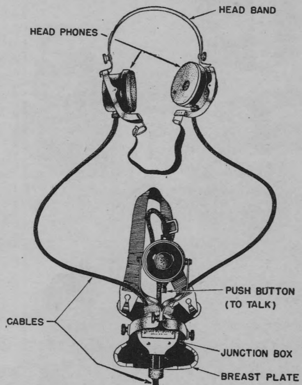
Figure 6-2. The headset.
