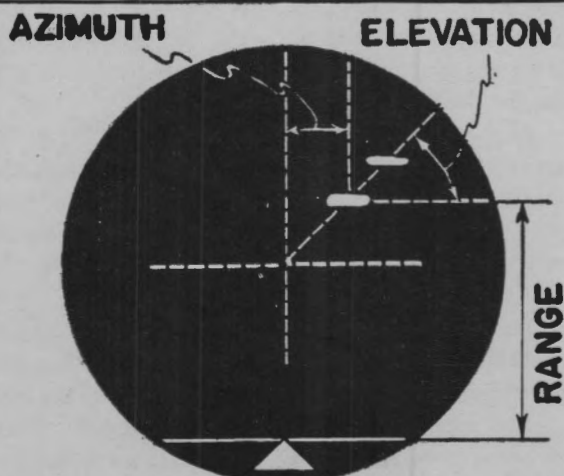
"H" SCOPE
