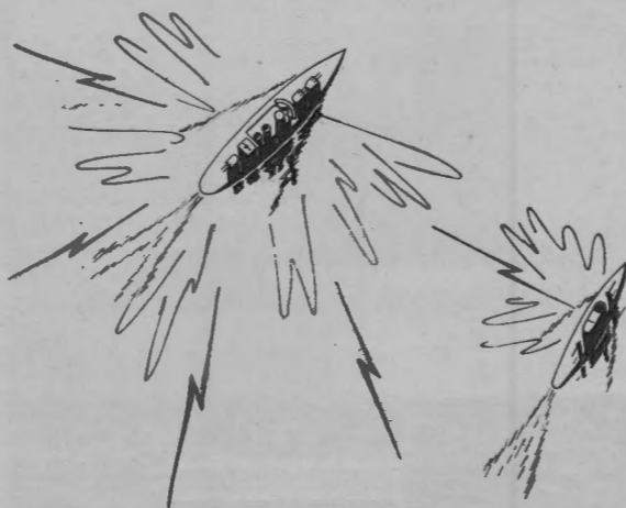
Figure 3-26. Antenna bearing 180° relative; target bearing 080° relative.
