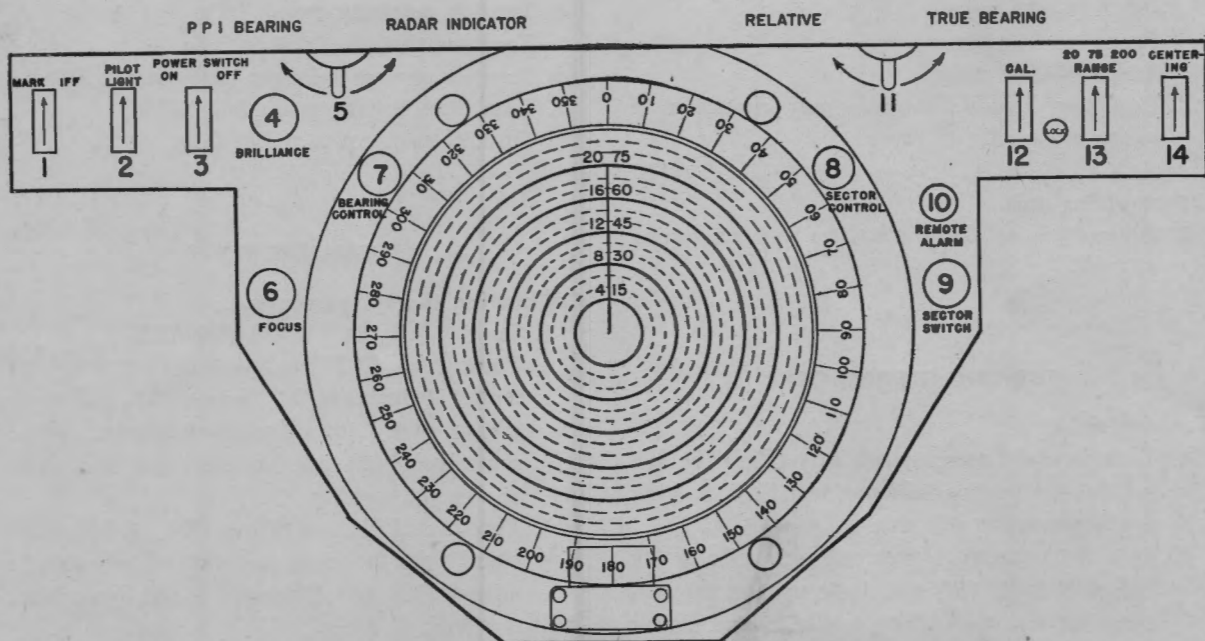
Figure 4 SC/SK-2. Plan position indicator.
