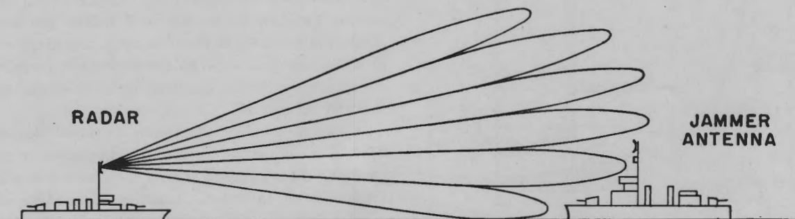
Figure 3-34. Jamming ineffective because the jammer antenna is in radar null.
