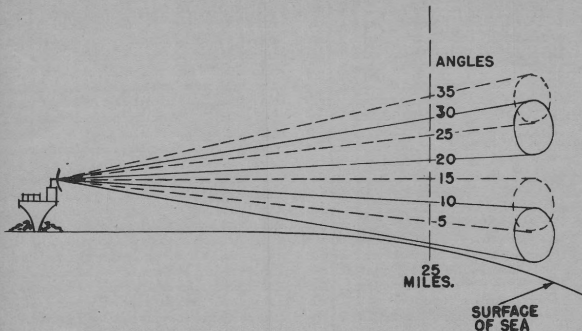
Figure 4 SP-3. "Overlap" of radar cone searching in elevation in 5,000 foot jumps at 25 miles.
