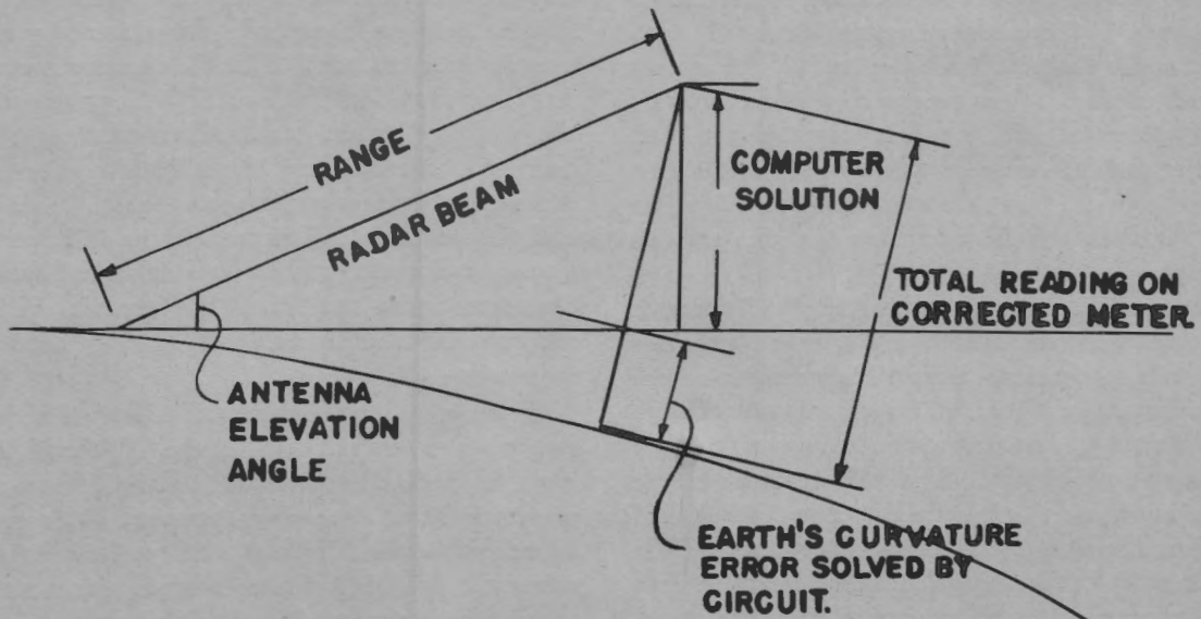
Figure 4 SP-6. Height meter reading.
