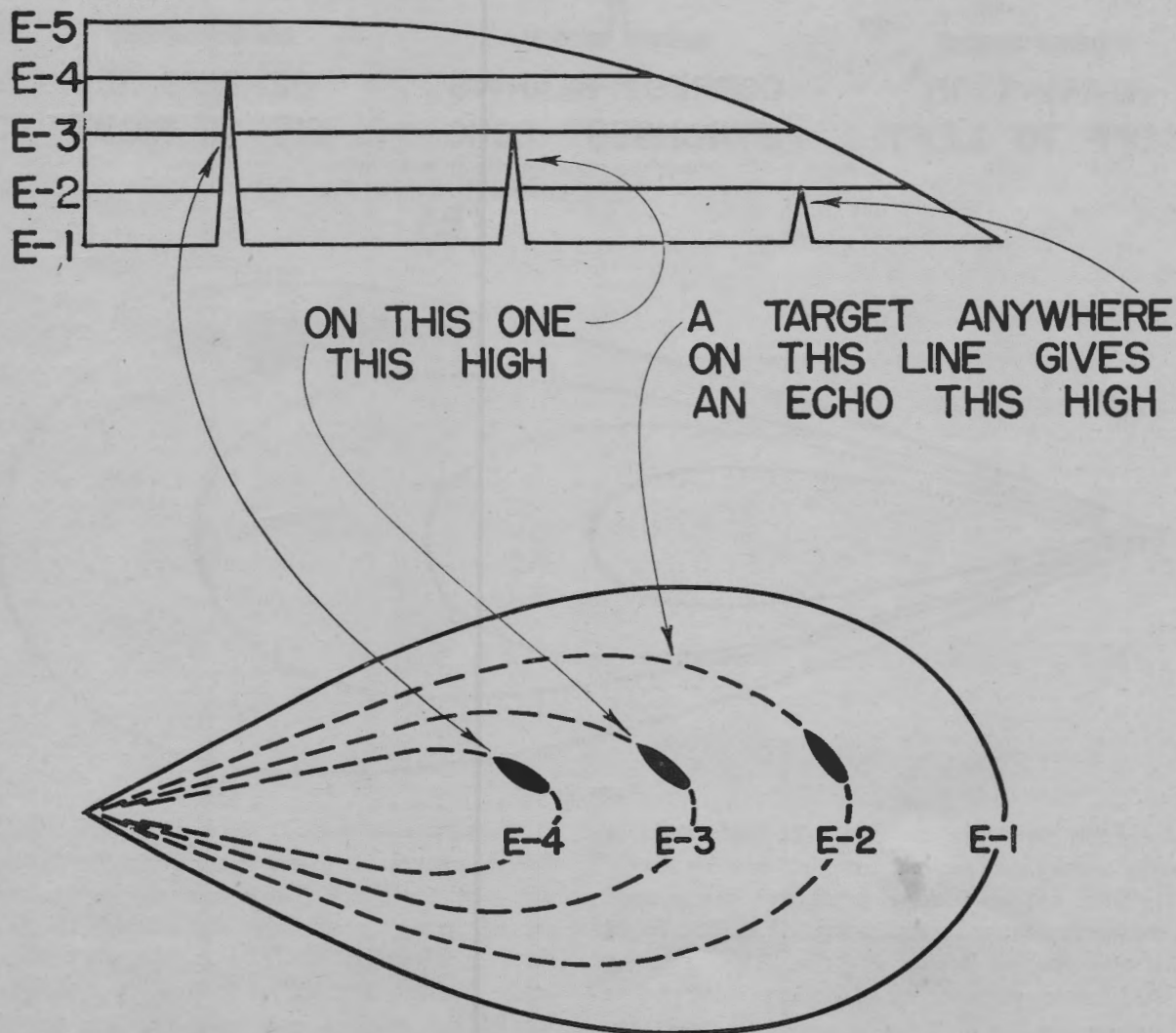
Figure 1-18. Lobe and corresponding echo height.
