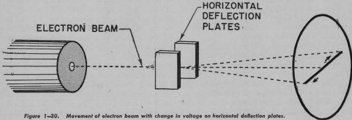
Figure 1-30. Movement of electron beam with change in voltage on horizontal deflection plates.
