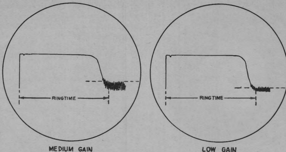
Figure 4 OBU-7. Measuring ringtime on "A" scope—receiver gain not a critical factor within reasonable limits.
