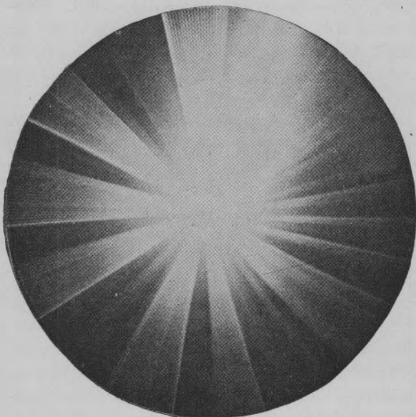
Figure 3-37. Interference produced by keying of radio transmitter on board ship. Note appearance of dots and dashes and non-directional effect produced. In this case the interference is not entering by means of the radar antenna, but directly into the radar receiver itself.
