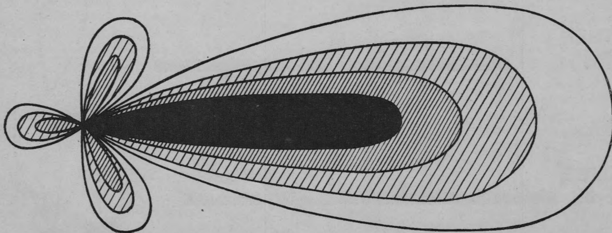
Figure 1-25. Main, minor, and back lobes. 1-28
