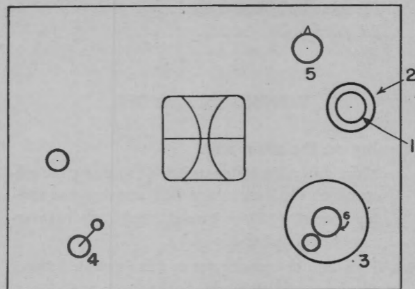
Figure 4 Mk. 3/Mk. 4-3. Range unit.
