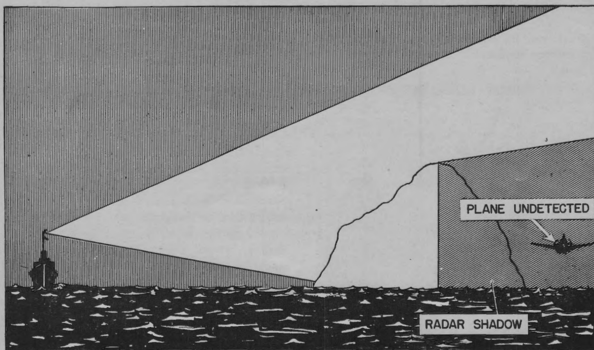
Figure 3-27. Radar shadow.
