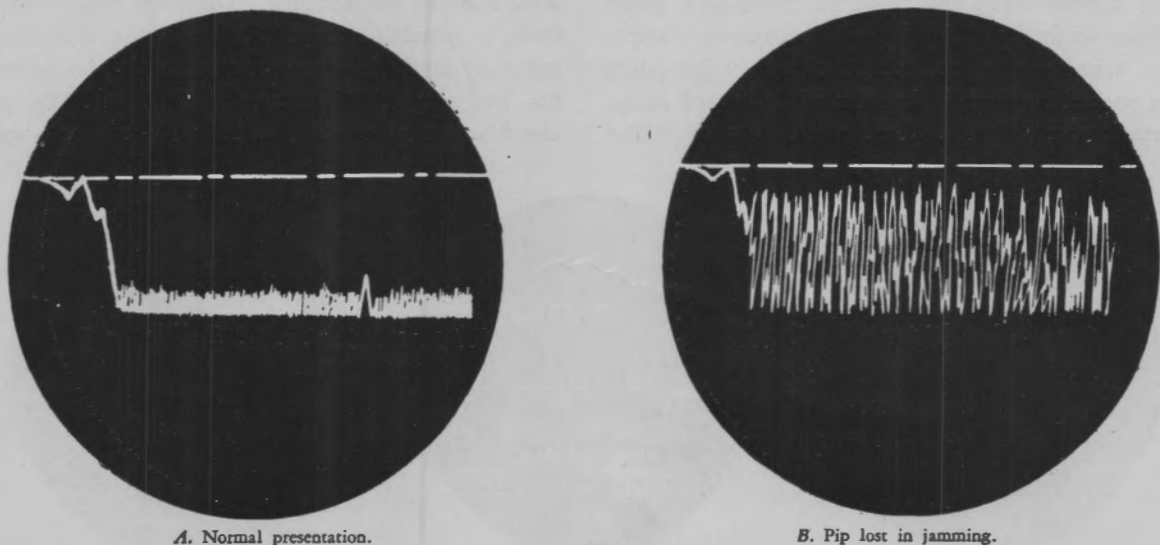
Figure 3-47. Random-noise modulated jamming.
