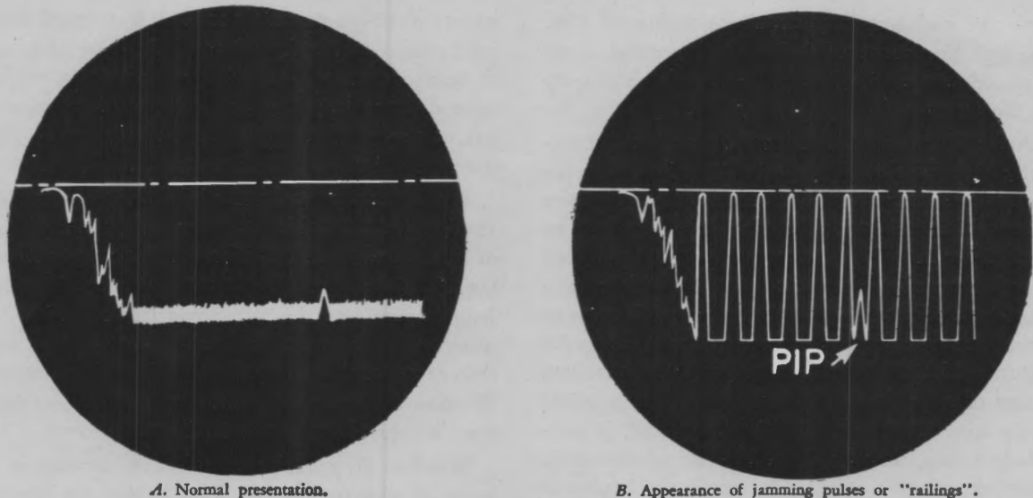
Figure 3-46. Pulse jamming.
