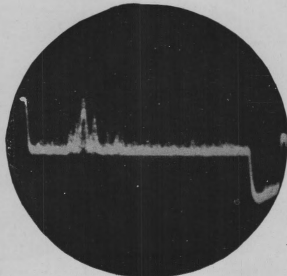
Figure 3-85. Window Echoes on Different Radars.
