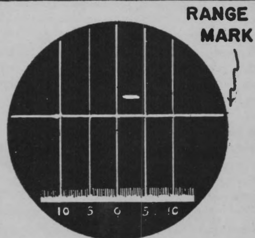
"B" SCOPE
