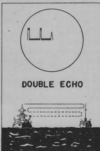
Figure 3-25. Multiple-range echoes.
