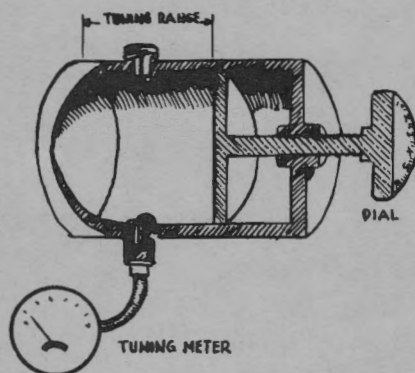
Figure 4 OBU-3. Simplified cross-section of echo box.
