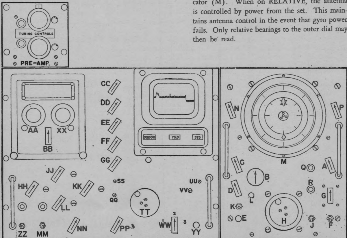
Figure 4 SC/SK-1. Receiver, indicator and control unit.
