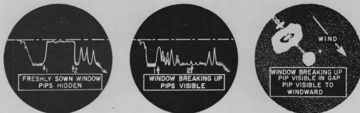
Figure 3-48. Typical Appearance of Window jamming.
