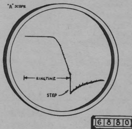
Figure 4 OBU-8. Setting the step.
