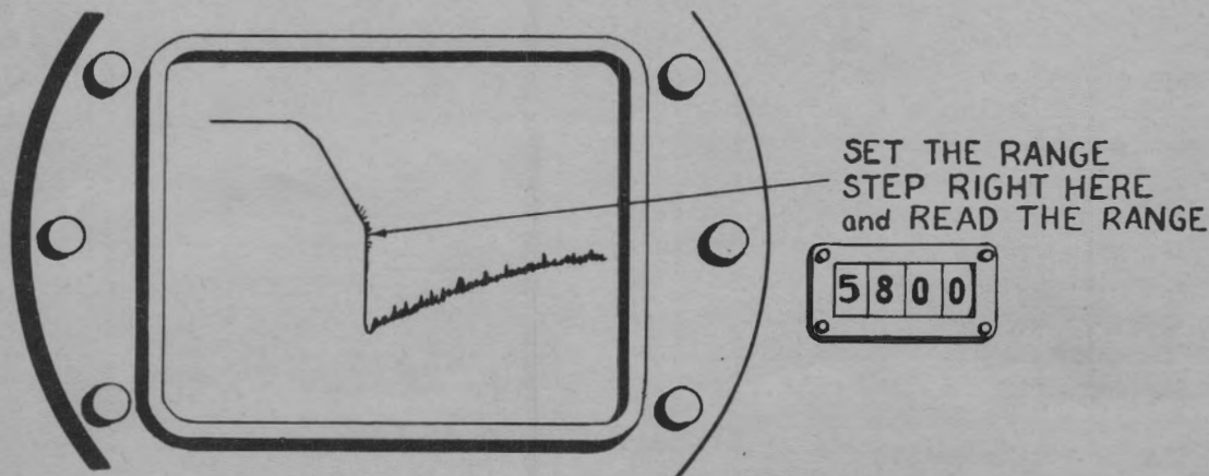
Figure 4 OBU-4. Echo box echo on "A" scope. Its duration is measured in yards and called "ringtime."
