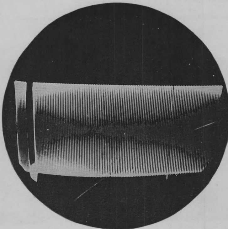
B. Similar to A, but on Army radar. Jamming has higher repetition rate or longer range scale is in use. Non-synchronous pulse jamming of high PRR is hard to distinguish from high-frequency AM jamming.
