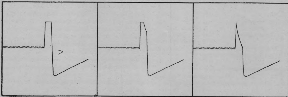
Figure 4 SG-4. Correct method for ranging on a saturated signal on the 15,000-yard range scale.
