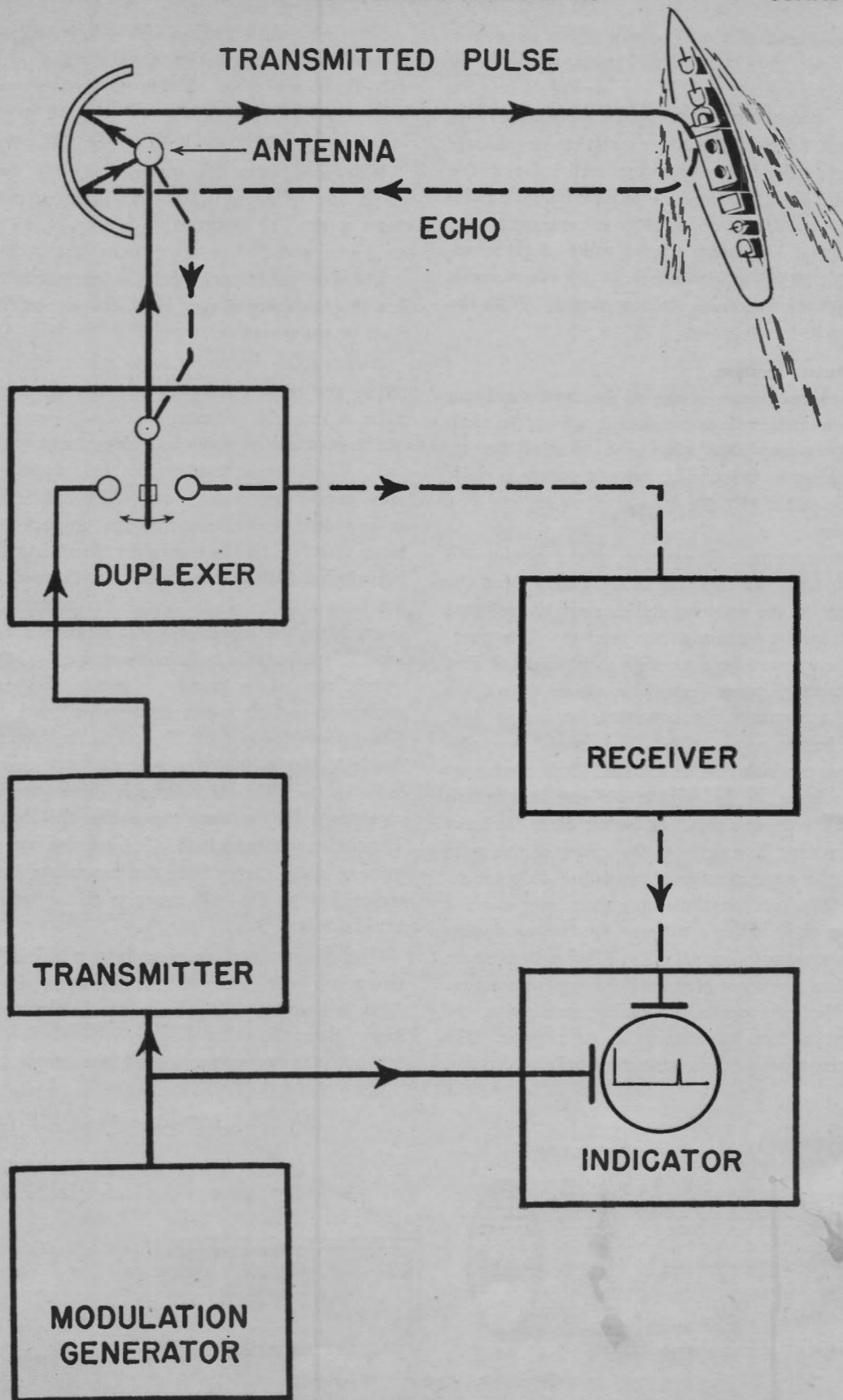
Figure 1-8. Block diagram of a typical radar system.
