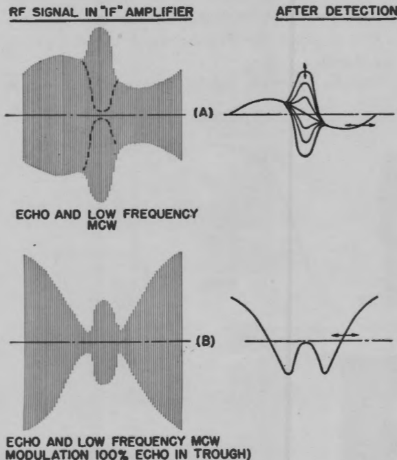
Figure 3-88. Echo in presence of Amplitude-modulated jamming.
