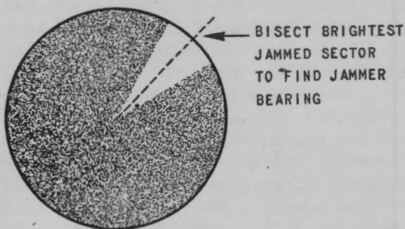
Figure 3-52. Taking bearing on Jammer on a PPI. Only the brightest sector is shown. Jamming will also appear at other bearings due to pick up in side lobes and because of reflection from parts of the ship.
