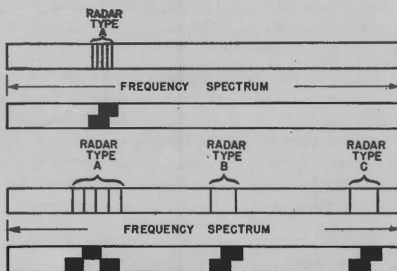
Figure 3-53. Shows the desirability of operating radars widely separated in frequency in each band, and of using several types to cover different frequency bands. Black areas indicate frequency coverage of individual jammers.
