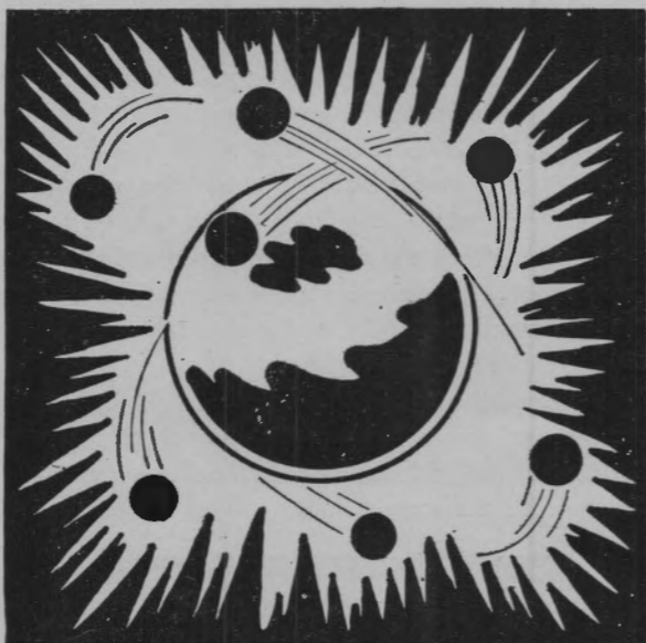
Figure 1-26. Structure of an atom showing electrons in their orbits.
