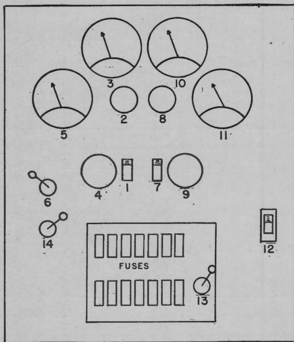
Figure 4 SJ-1. Main control unit.
