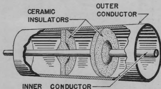
Figure 1-9. Coaxial. Wave-guide.
