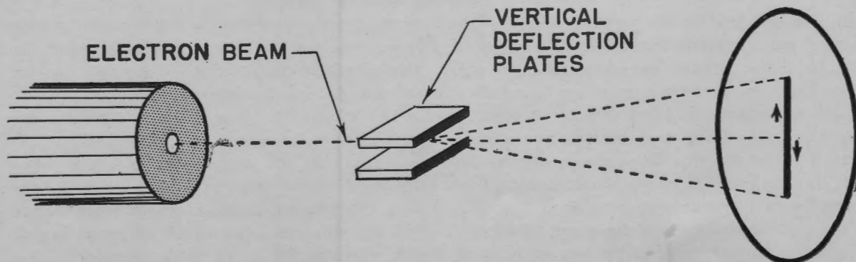
Figure 1-29. Movement of electron beam with change in voltage on vertical deflection plates.
