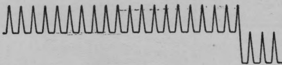
Figure 4 SF-6. Pattern for calibrating 40,000-yard range on 48,000-yard scale.
