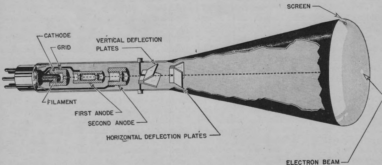
Figure 1-31. Electrostatic cathode-ray tube.
