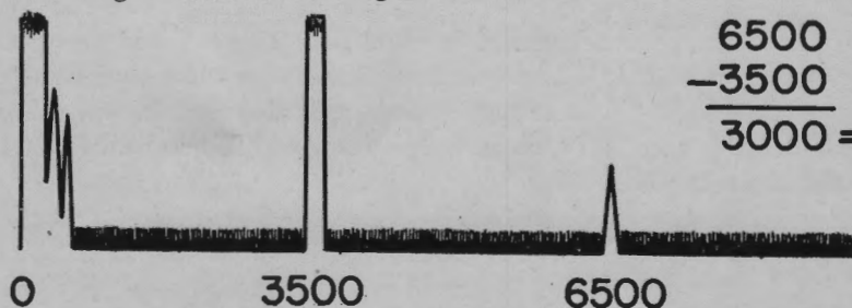
Figure 1-36. Zero set is off 500 yards.
