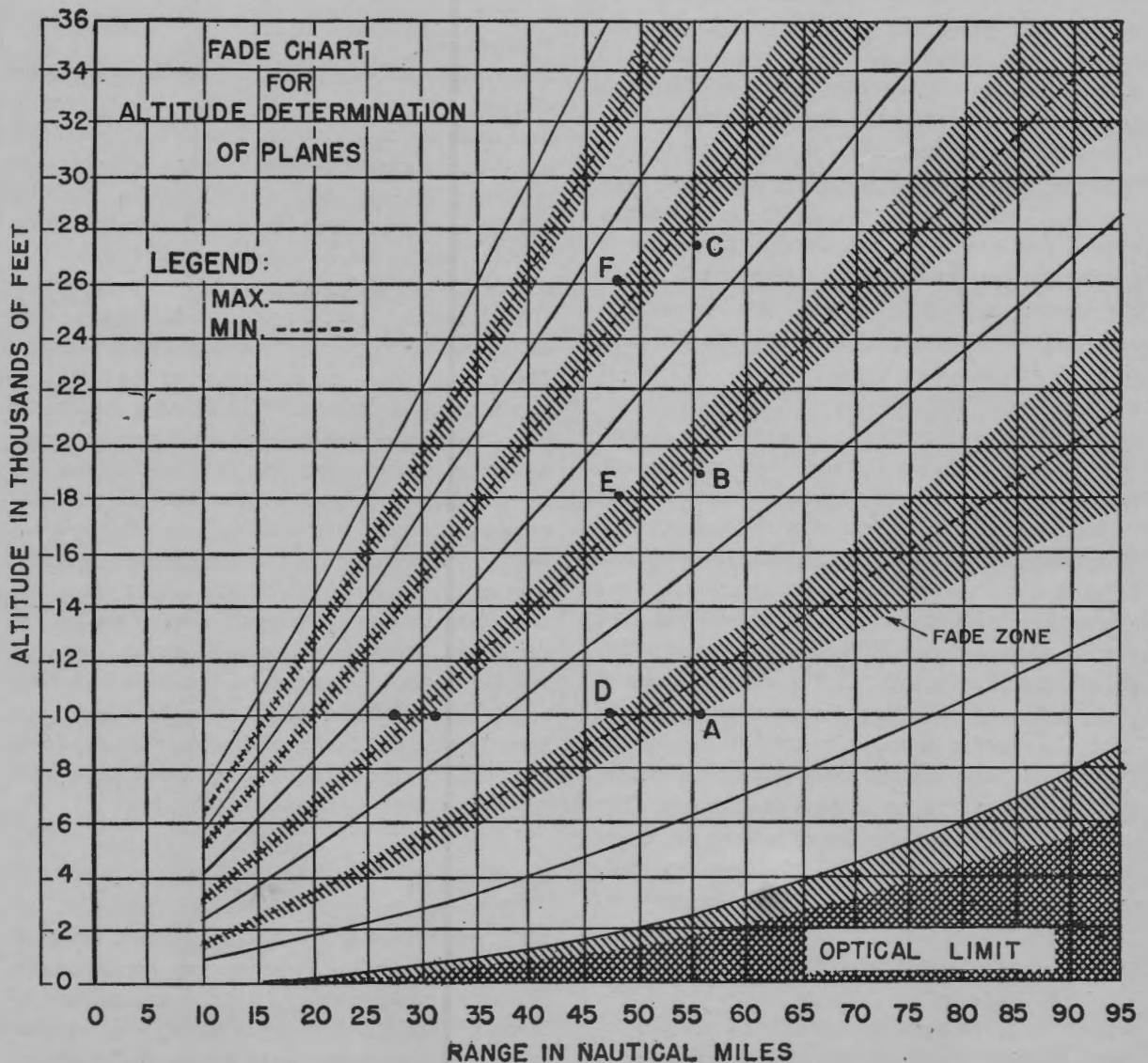
Figure 1-52. Fade chart.
