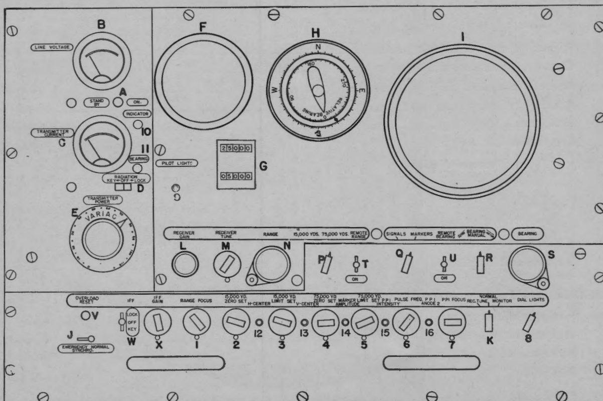
Figure 4 SG-1. Range and train indicator unit.
