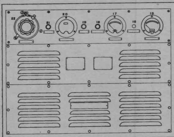
Figure 4 SU-2. Modulator unit.
