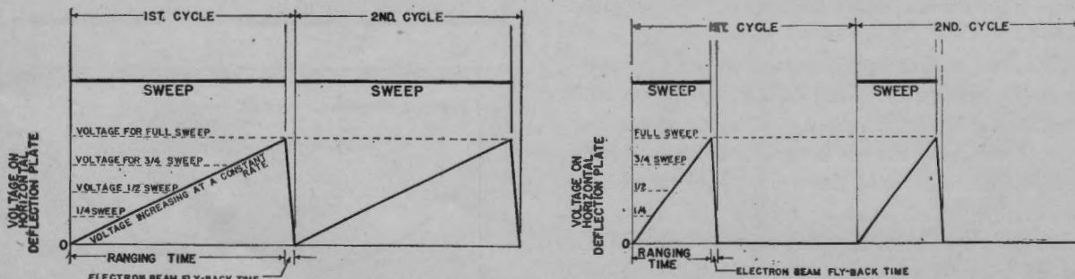
Figure 1-34. Continuous sweep.—Discontinuous sweep.
