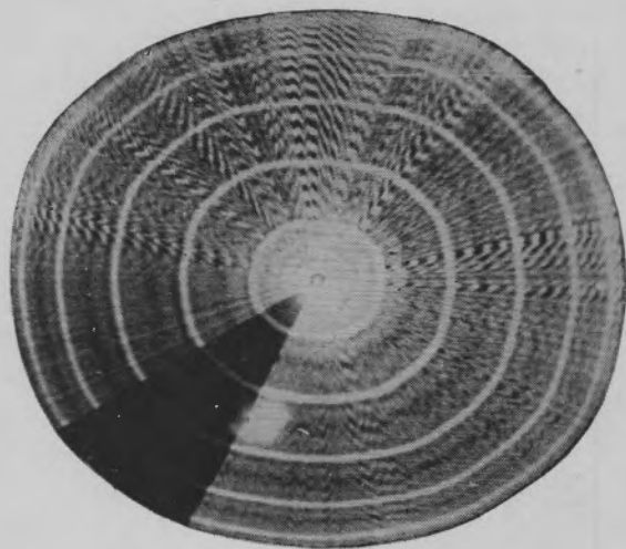
A. Airborne radar, 5-mile sweep. Strong jamming entering side lobes. Echo not visible. Note striations characteristic of semi-synchronous jamming. Dark sector caused by photography.
