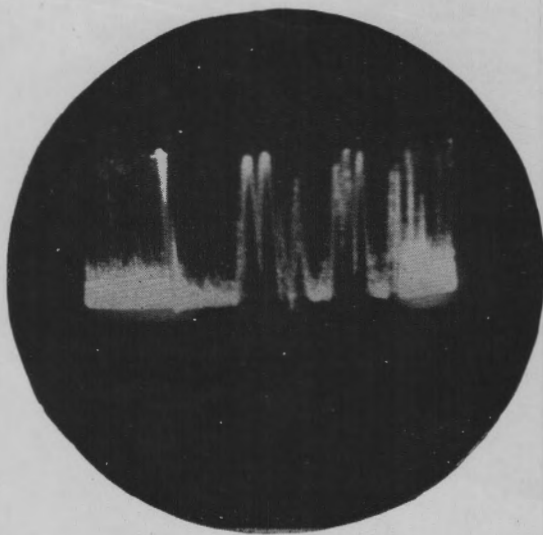
Figure 3-85. Window Echoes on Different Radars.
