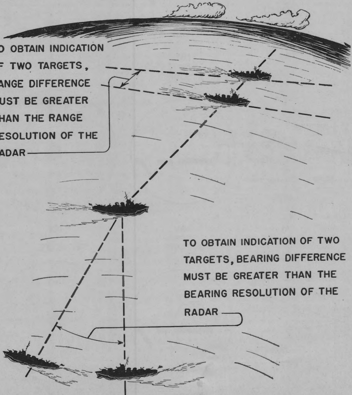
Figure 3-9. Bearing and range resolution.
