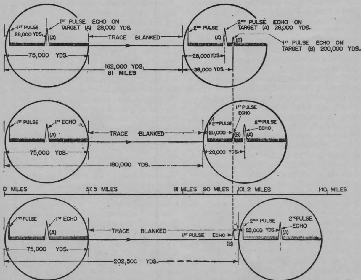
Figure 4 SG-5. Second-sweep echoes.
