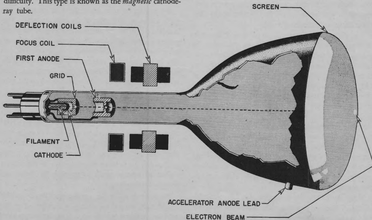
Figure 1-32. Magnetic cathode-ray tube.
