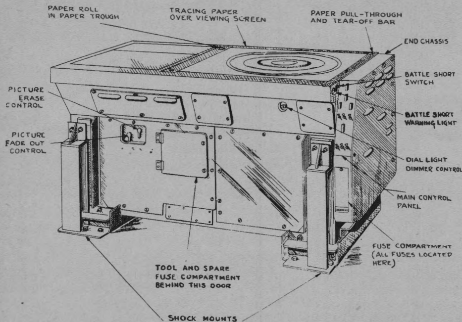
VG Projection PPI Repeater Unit
