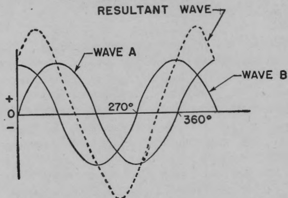
Figure 1-48. Two waves 270^\circ out of phase.
