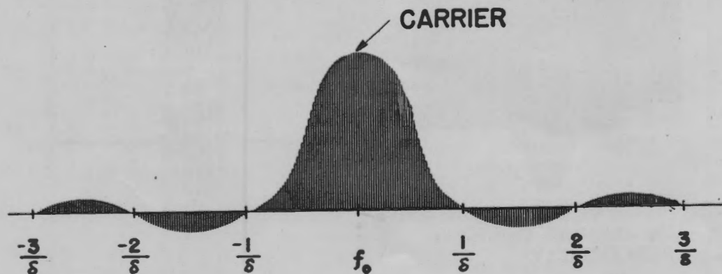
Figure 3-86. The Radio-Frequency spectrum of an echo pulse.
