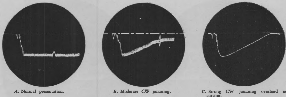
Figure 3-42. Unmodulated CW Jamming.
