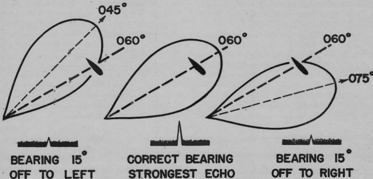
Figure 1-19. Determining correct bearing by echo's height.
