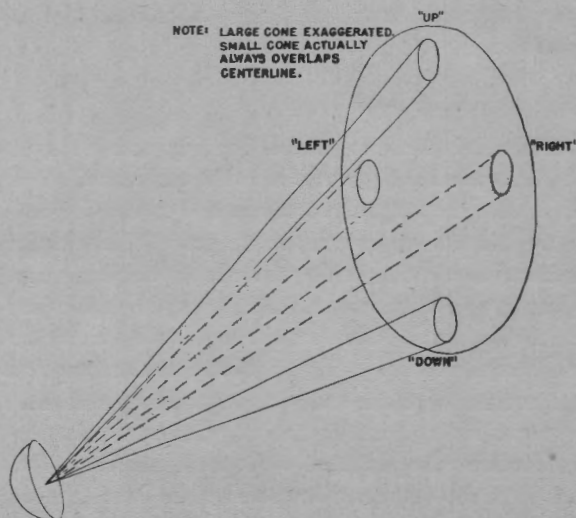
Figure 4 SP-4. 1. Precision circuit receives target only in four positions of cone. 2. Precision scope gets "net" signal from "up-down" and "right-left."
