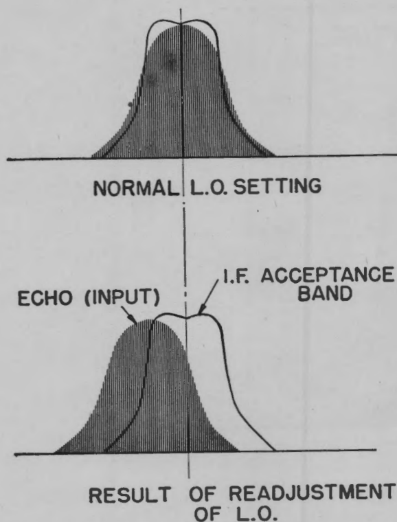
Figure 3-93. Effect of Adjusting Local Oscillator Tuning Control.
