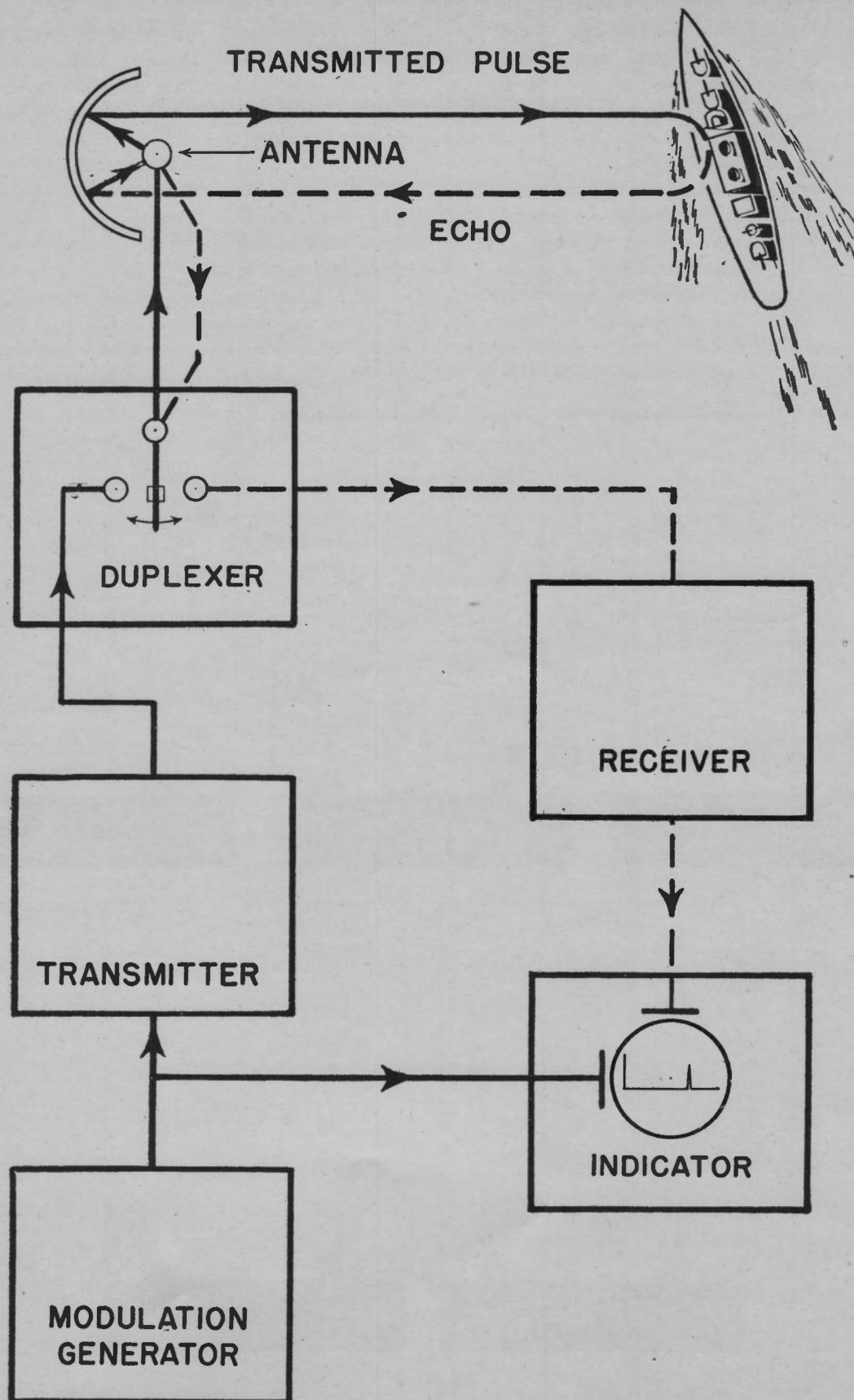
Figure 1-42. Block diagram of a typical radar system.
