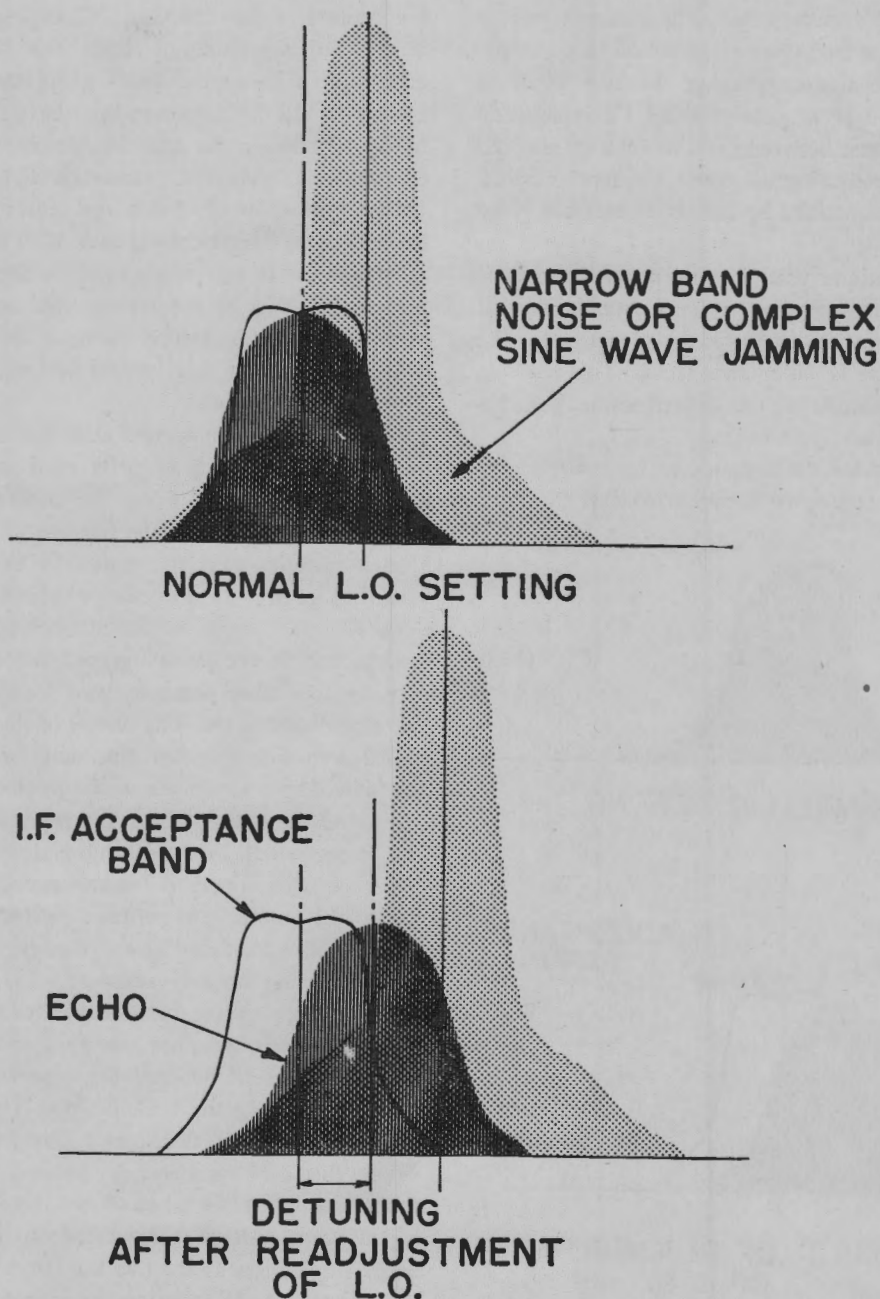
Figure 3-94. Using L.O. tuning to Discriminate Against Jamming.
