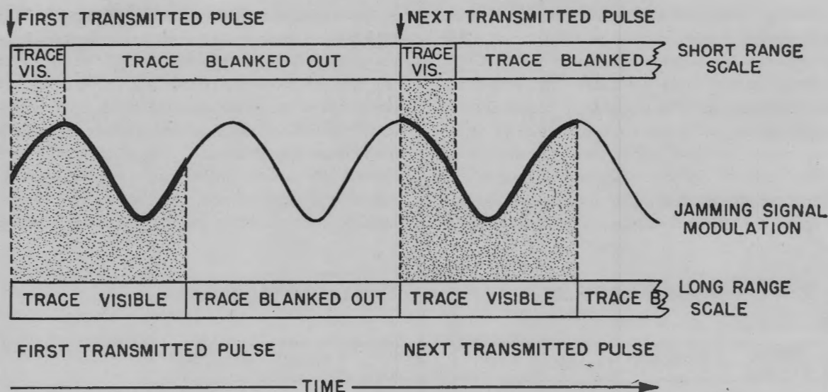
Figure 3-40. Effect of same jamming with different sweep times. The pattern in the long range will appear to be more complex, because a greater portion of the modulation cycle will appear.
