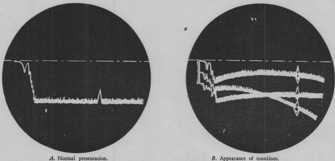
Figure 3-43. Low-frequency jamming.
