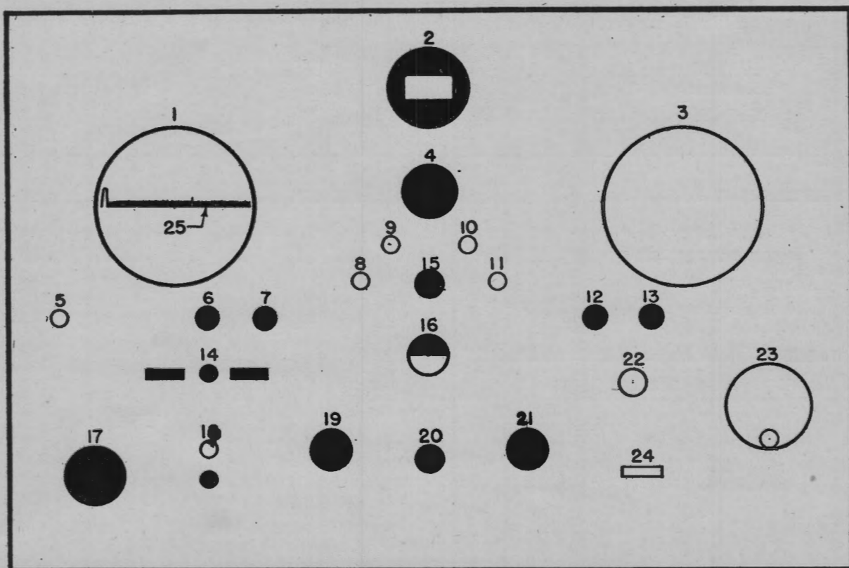
Figure 4 SF-1. Indicator unit.
