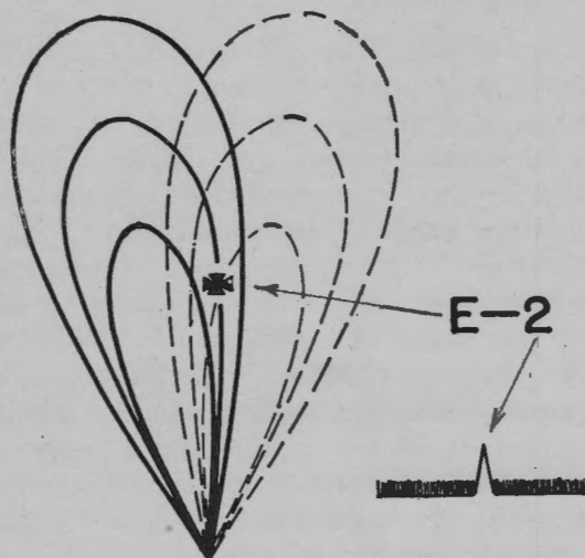
Figure 1-22. Lobe to port.
