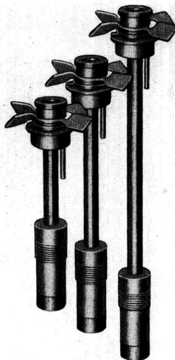
Figure 37.—Tail Fuzes AN-M100A2, AN-M101A2, AN-M102A2
