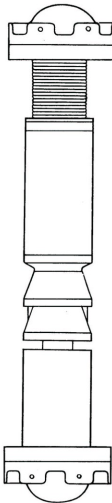
Figure 12.—Outline Drawing of Athwartship Hydrostatic Fuze Mk 224
