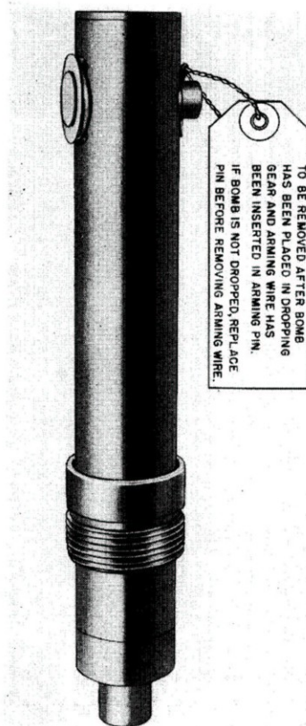
Figure 43.—Tail Fuze M106
