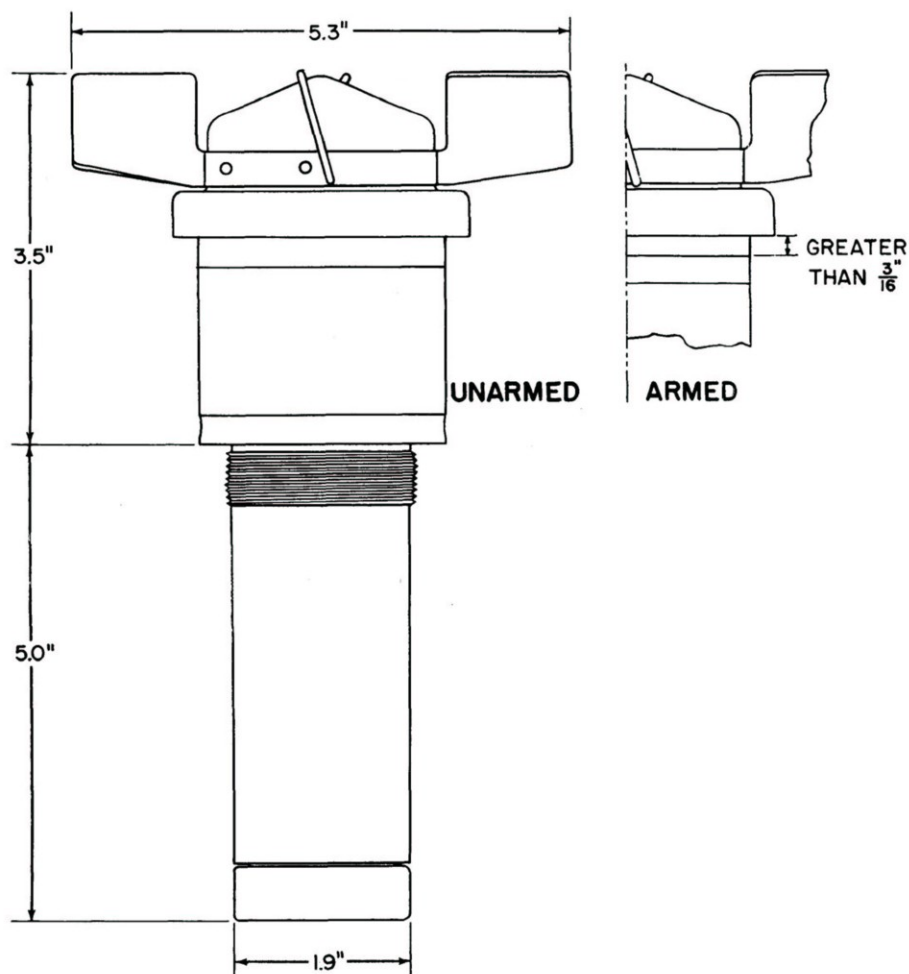
Figure 28.—Outline Drawing of Nose Fuze Mk 239
