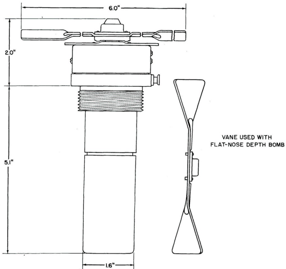
Figure 75.—Outline Drawing of Nose Fuze AN-M139A1
