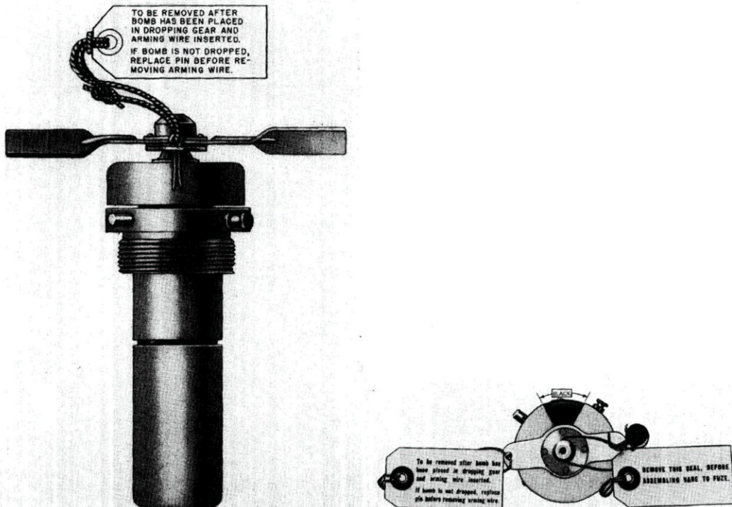
Figure 76.—Nose Fuze AN-M139A1
