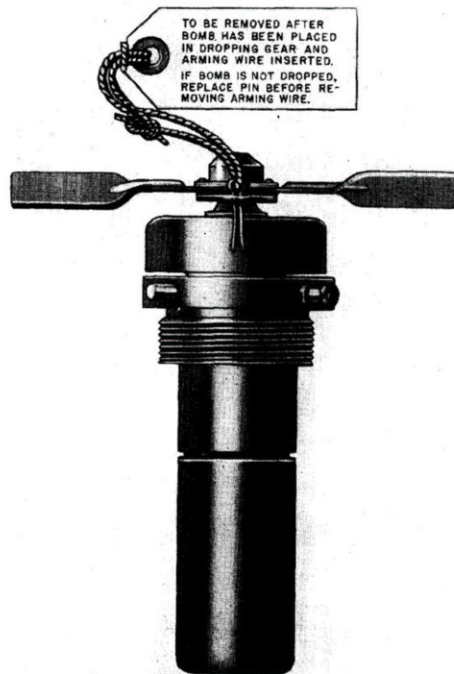
Figure 39.—Nose Fuze AN-M103A1
