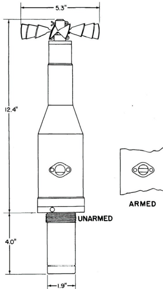
Figure 10.—Outline Drawing of Tail Fuze Mk 223
