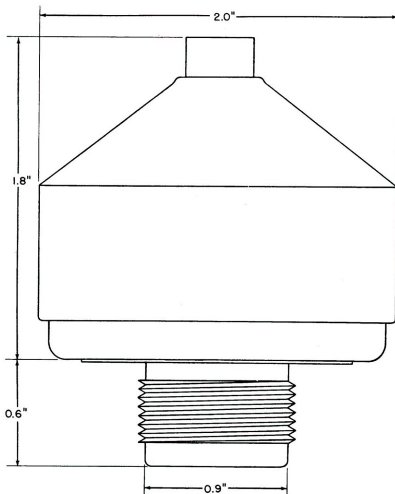
Figure 14.—Outline Drawing of Nose Fuze Mk 227
