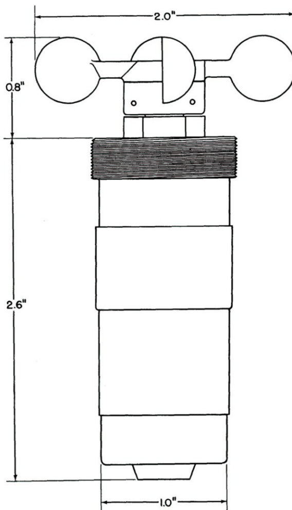
Figure 102.—Fuze M157
