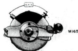
Figure 109.—Nose Fuzes M163, M164, M165
