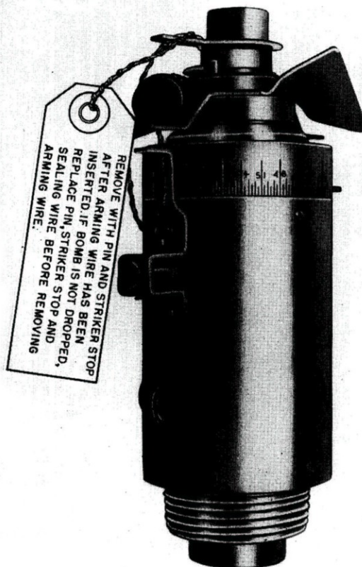
Figure 86.—Nose Fuze AN-M147
