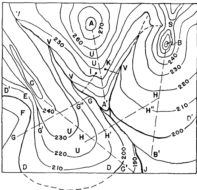
FIGURE 28.—Characteristics of contours.
