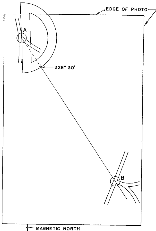
FIGURE 61.—Determining magnetic north on a photograph.
