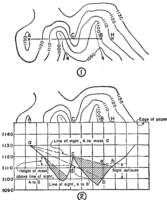
FIGURE 39.—Determination of visibility by profile method.
