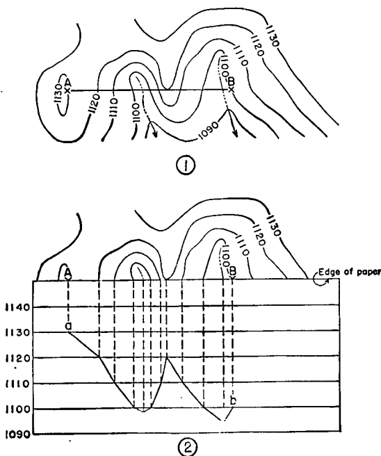
FIGURE 37.—Construction of a profile.
