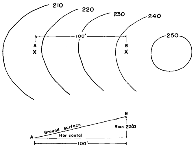
FIGURE 36.—Determination of slope.
