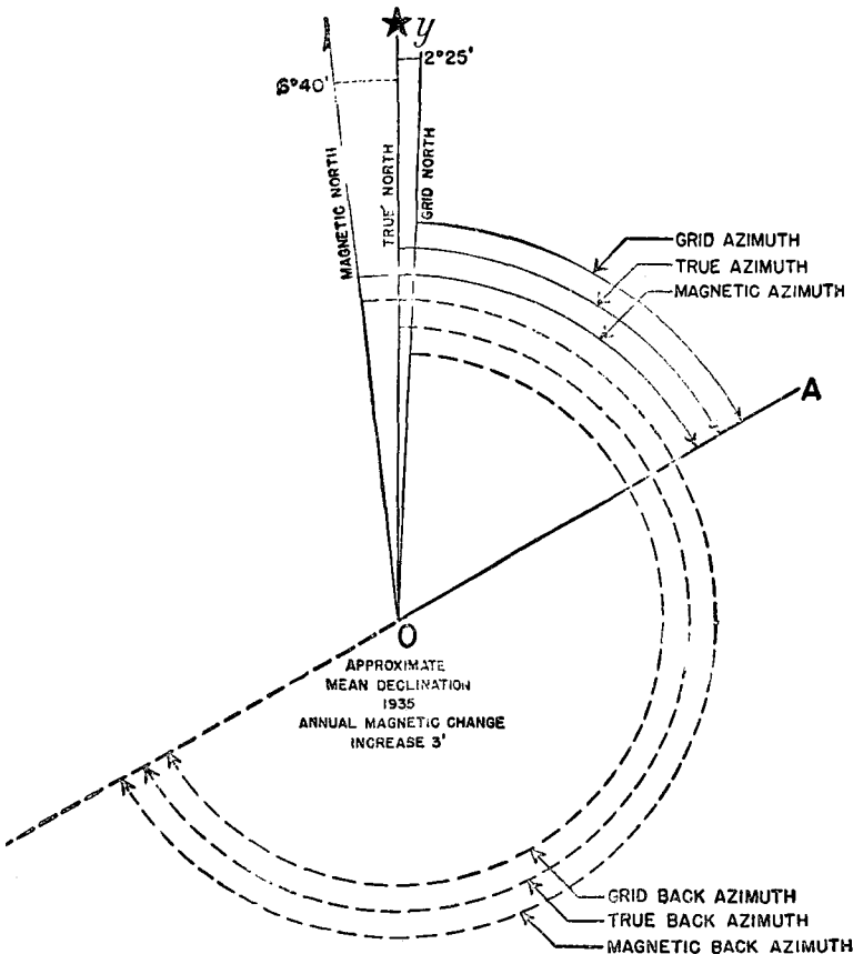
FIGURE 12.—Example of relationship between three base directions on a map, showing corresponding azimuths and back azimuths of line OA.
