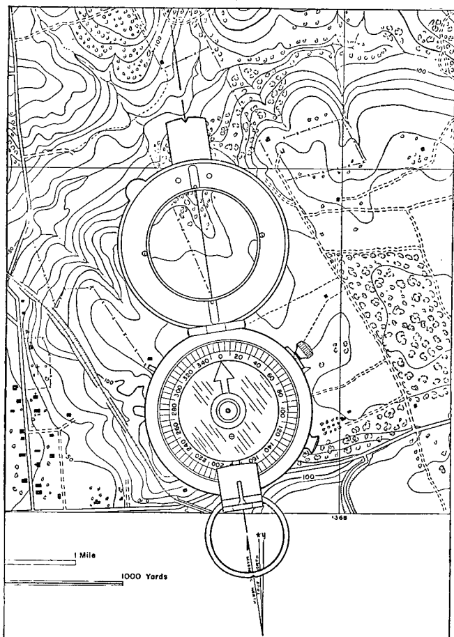
FIGURE 44.—Orientation of map by compass.
