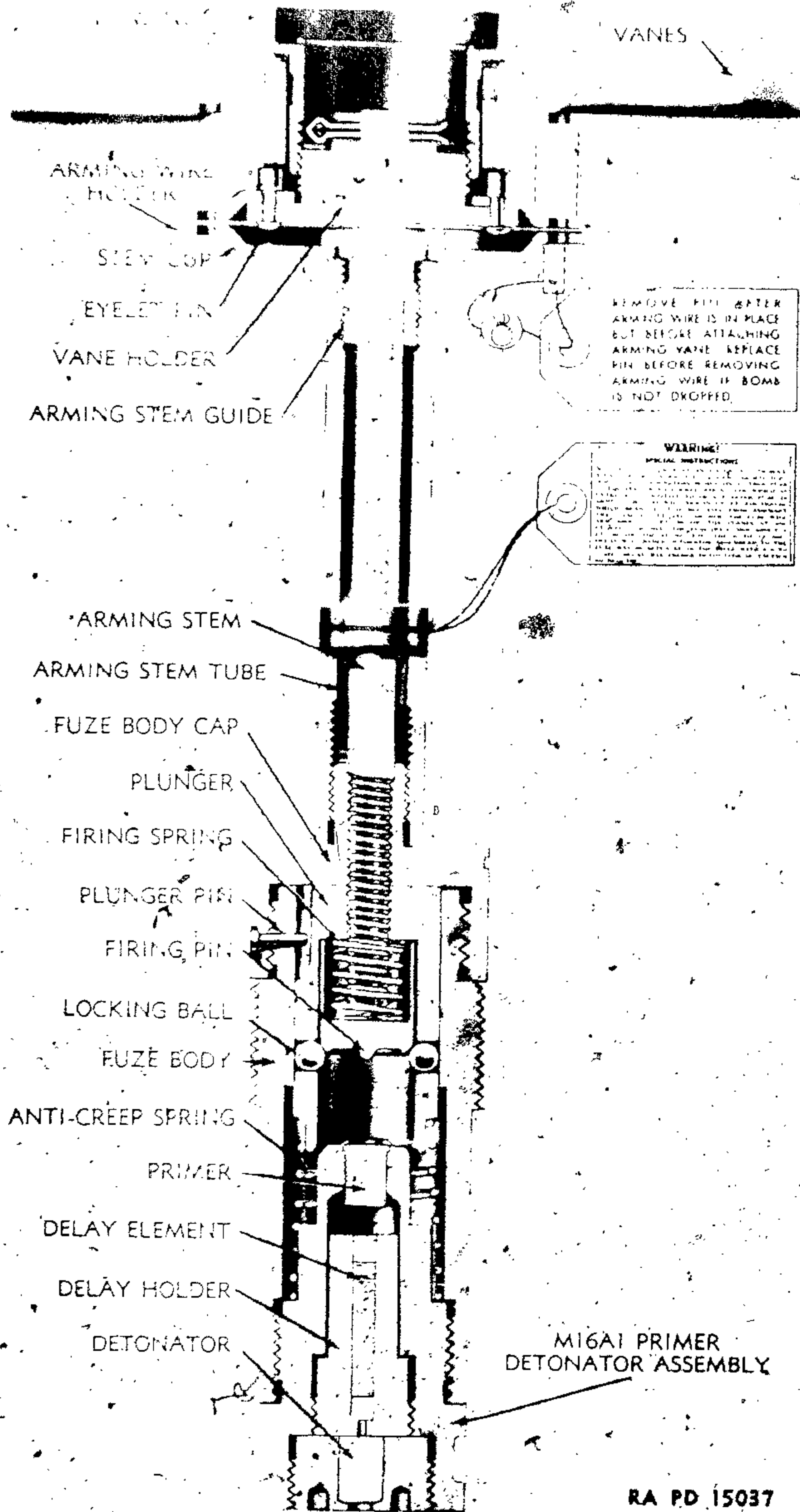
Figure 101 - Tail Fuze - Vane Arming Type (M112A1)
