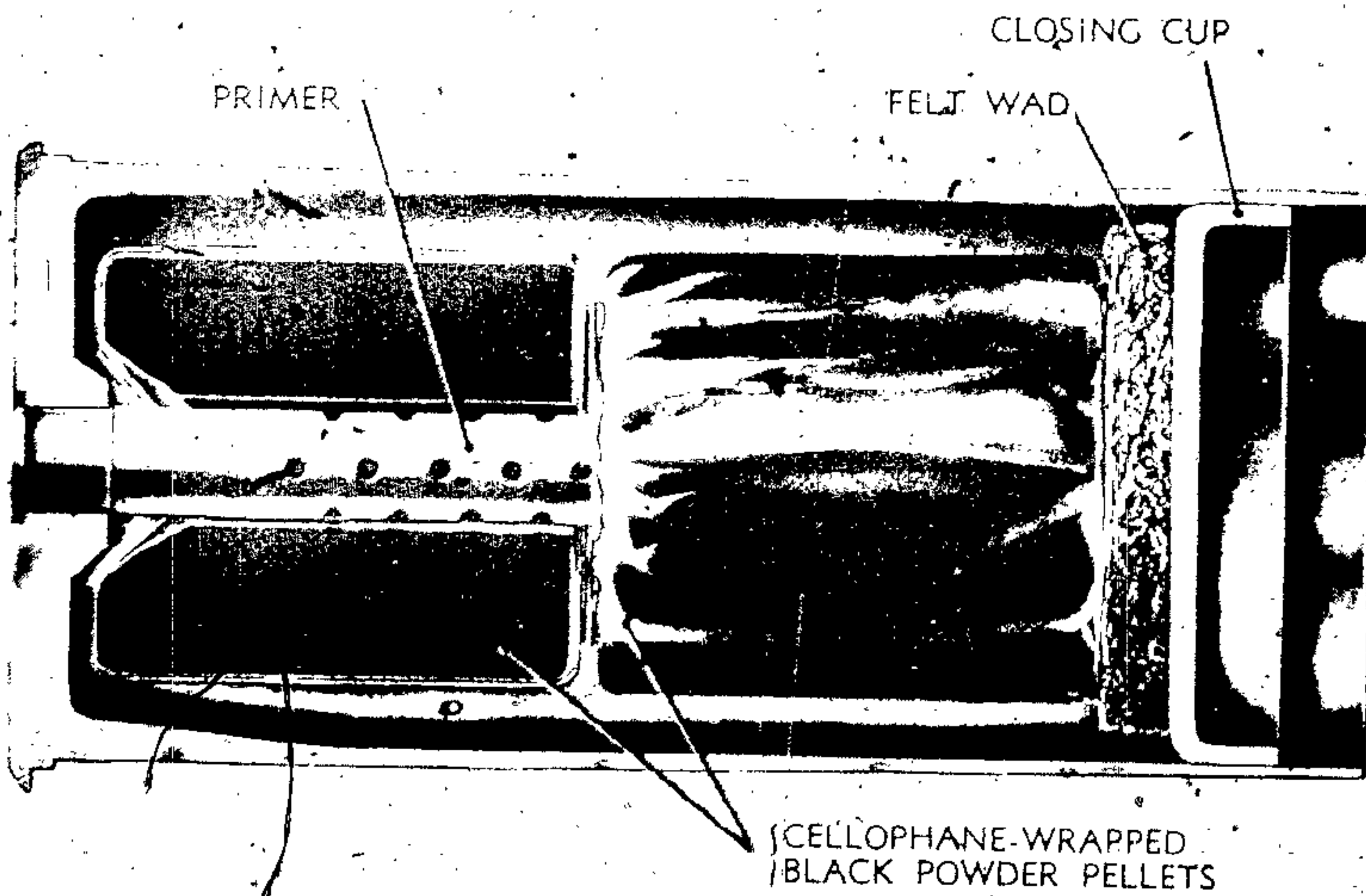
BLANK AMMUNITION (DOUBLE PELLET CHARGE), 75-MM GUN OR HOWITZER
