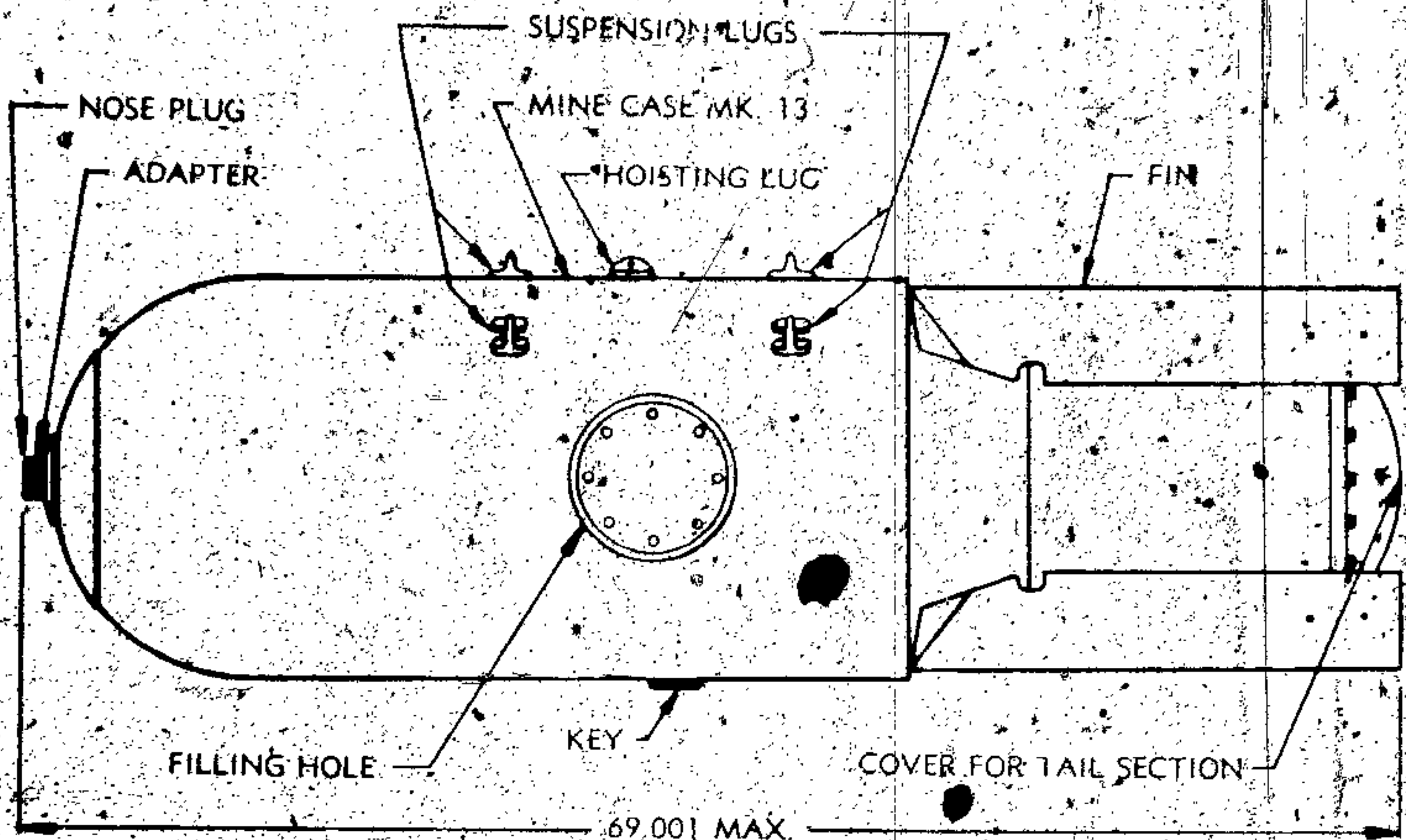
MINE, AIRCRAFT, MK. 13
