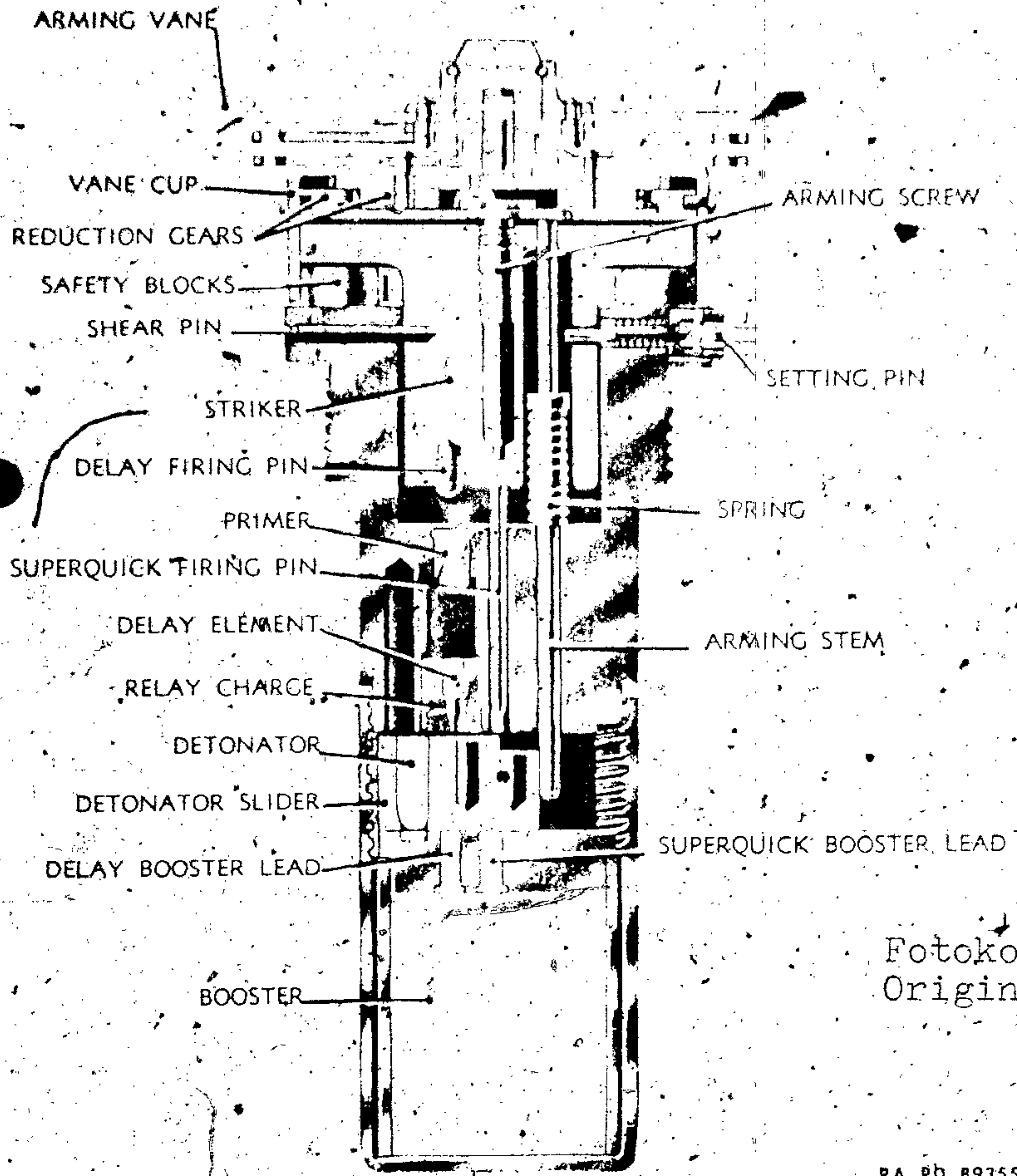
Figure 99 - Nose Fuze - Vane Arming Type
