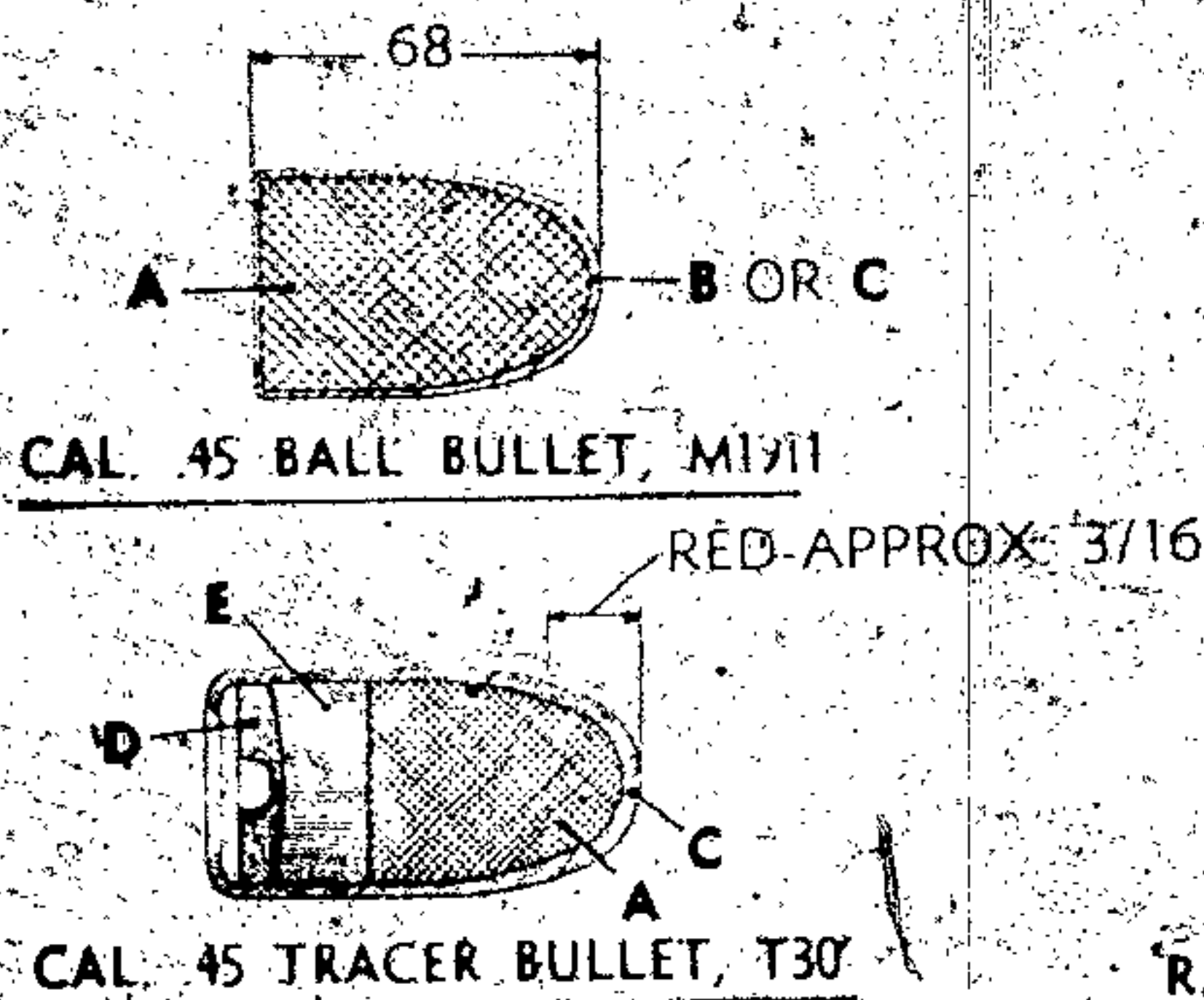
Figure 29 - Caliber .45 Bullets - Cross Section
