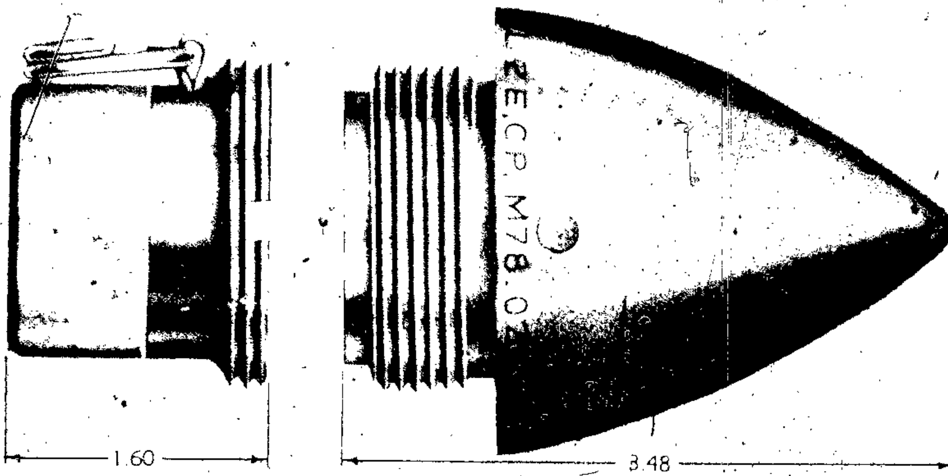
Figure 65 — Booster M25 and Concrete-piercing Fuze M78
