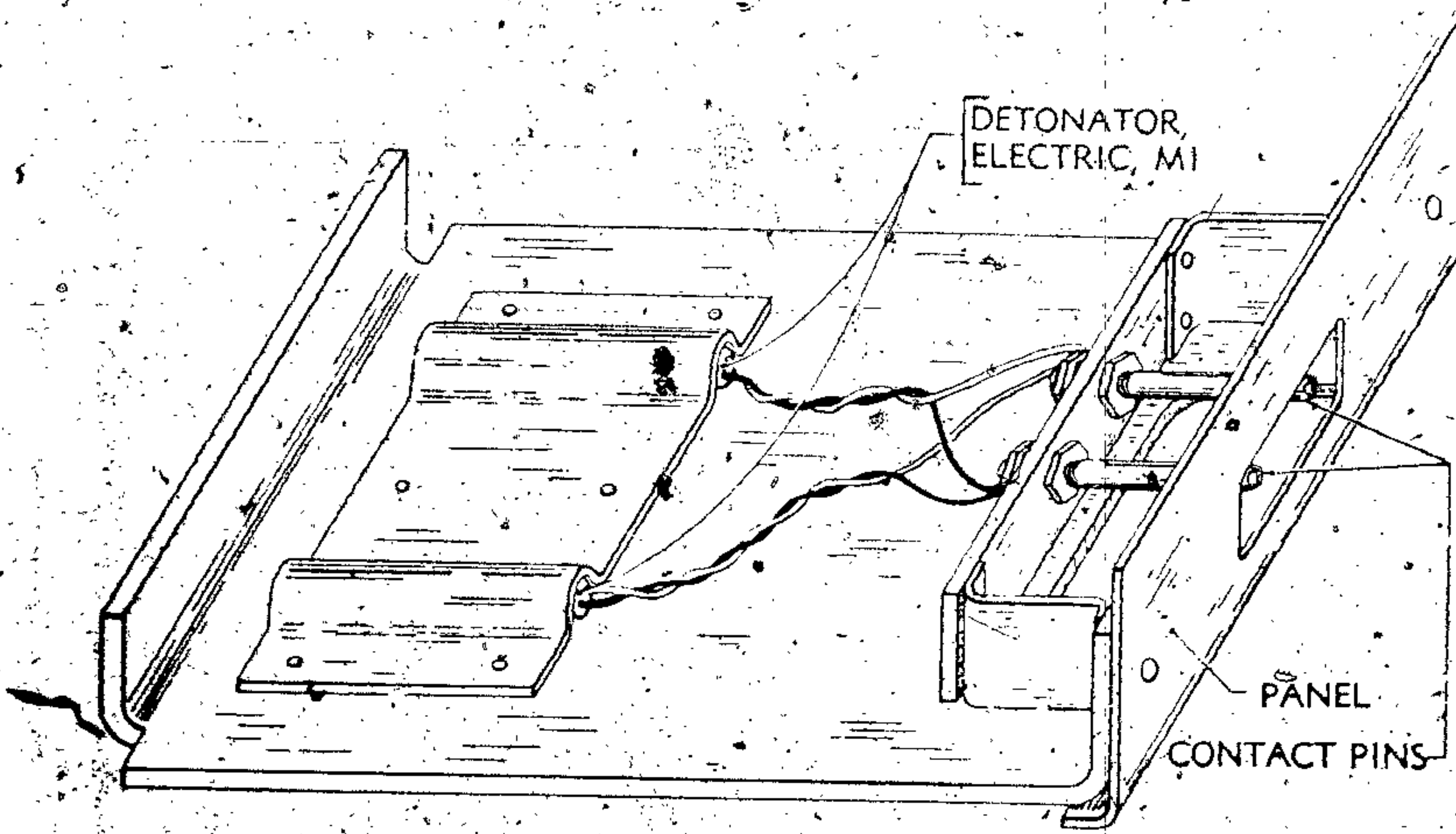
Figure 146 - Destructor AN-M2
