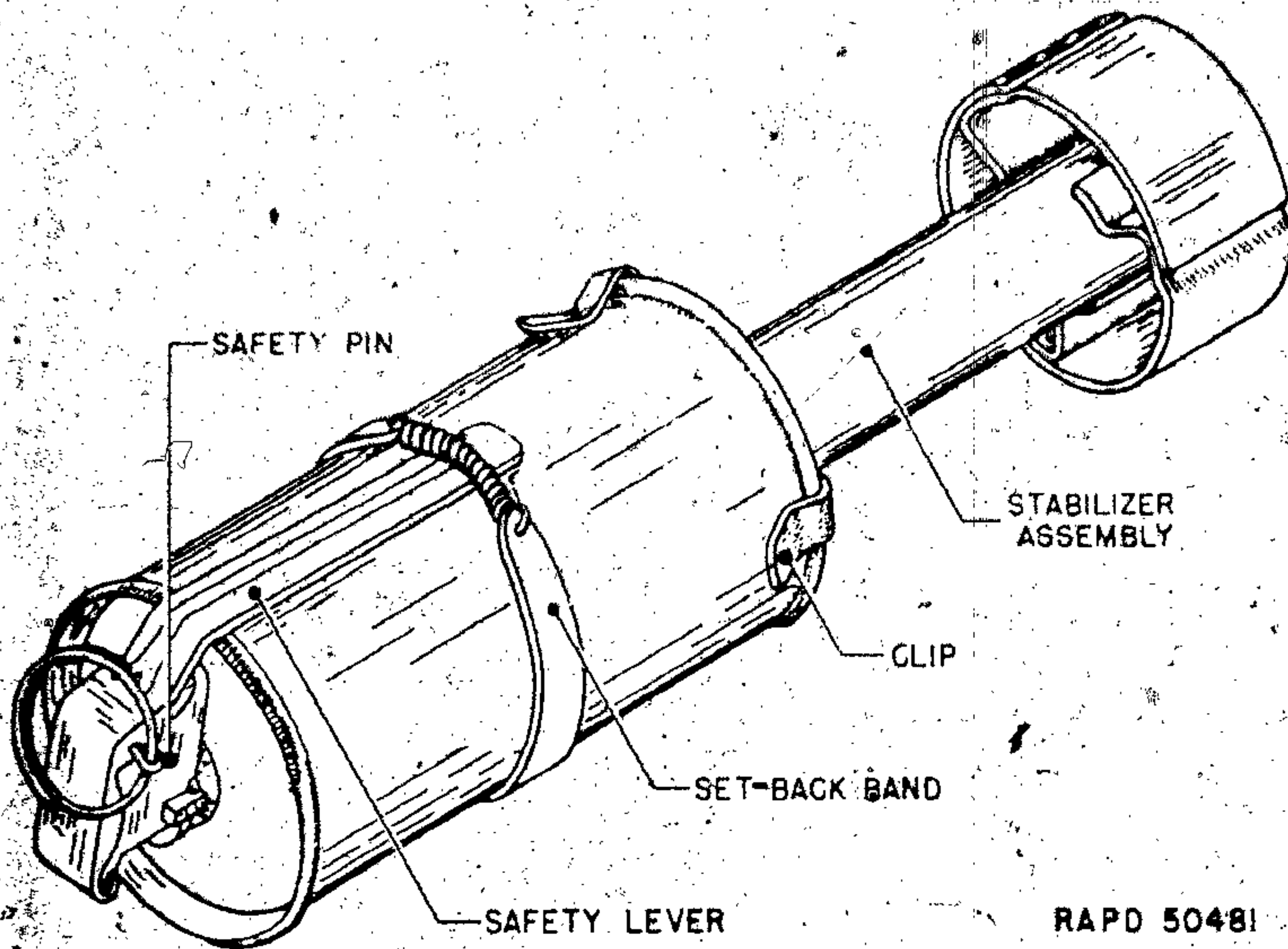
Figure 47 - Chemical Grenade Projection Adapter M2
