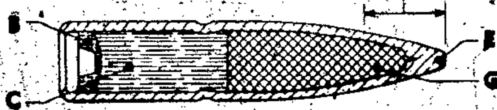
CAL. .30 TRACER BULLET, M1
