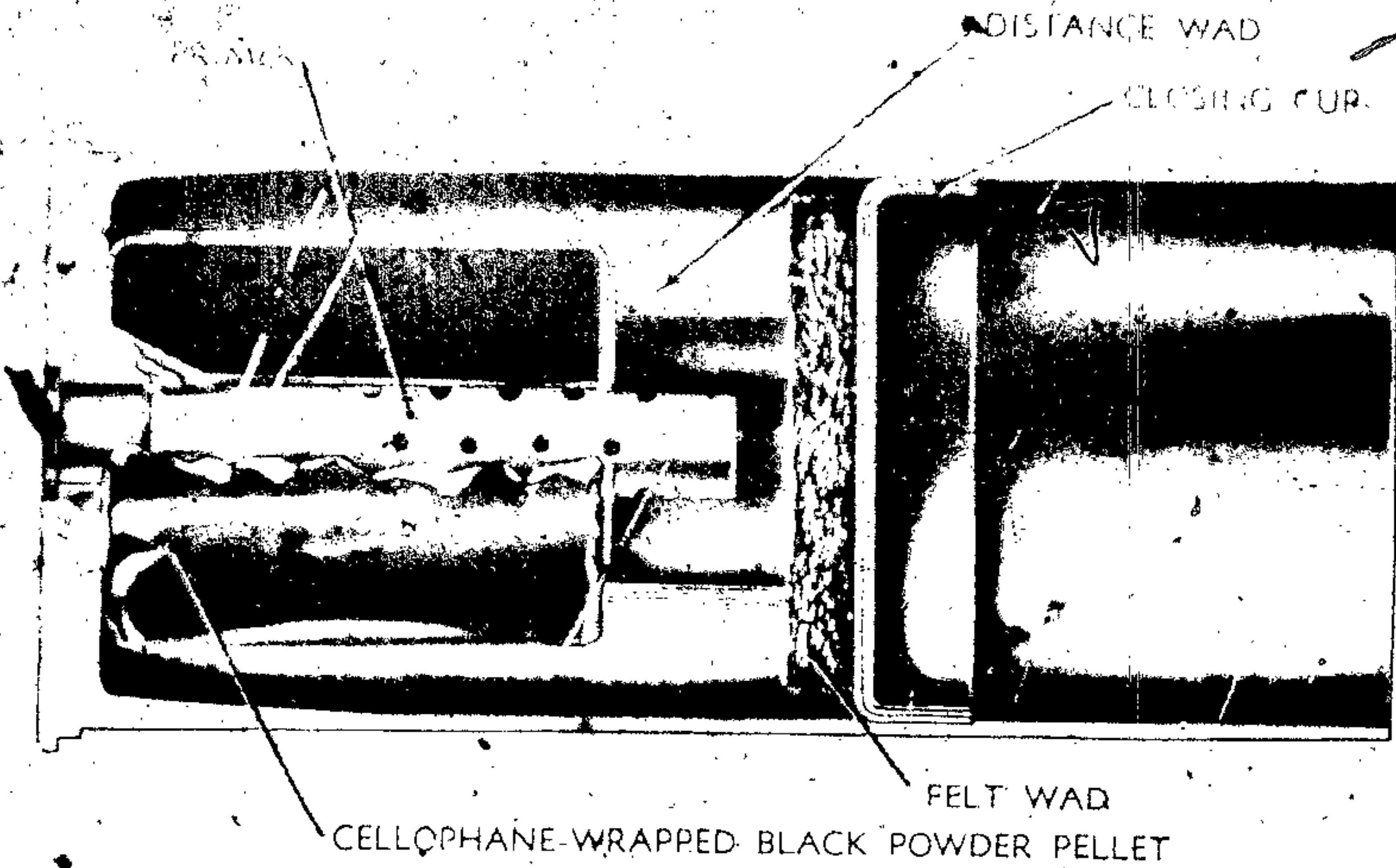
BLANK AMMUNITION (SINGLE PELLET CHARGE), 75-MM GUN OR HOWITZER
