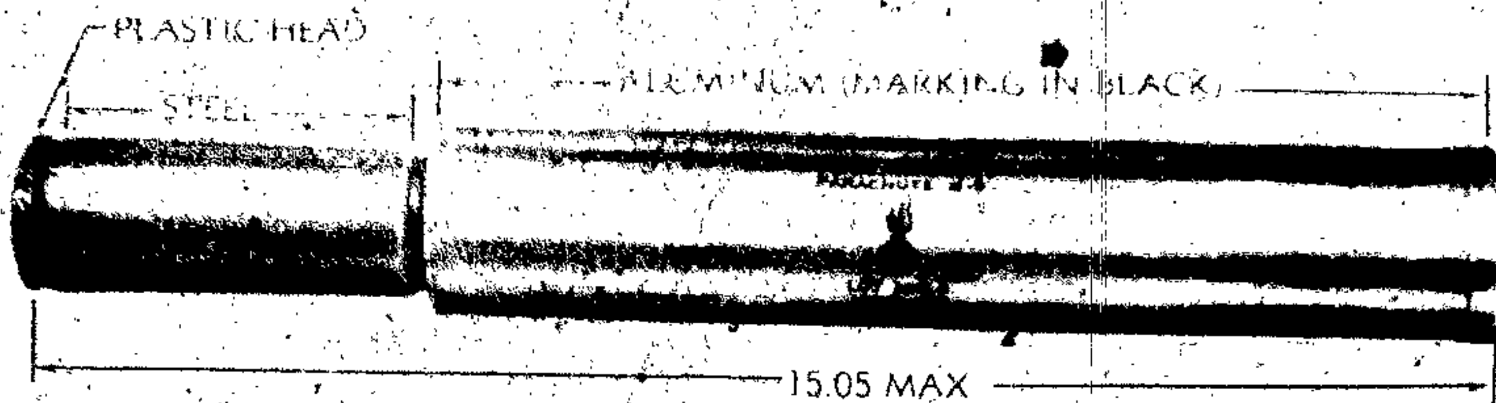
Figure 109 - Parachute Aircraft Flare M9A1
