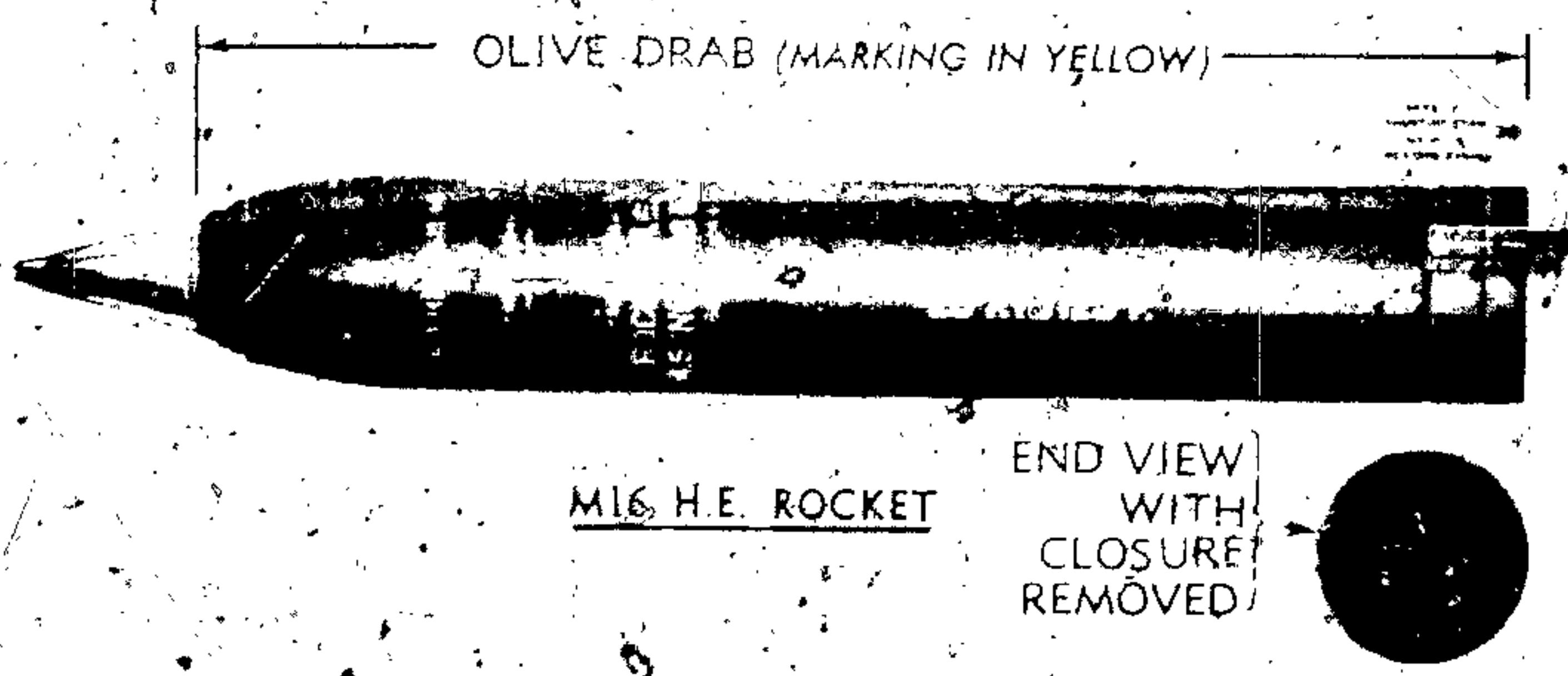
Figure 127 - 4.5-inch Rockets
