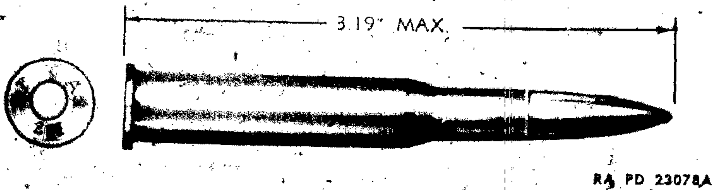
Figure 34 - Caliber .30 Subcaliber Cartridge M1925
