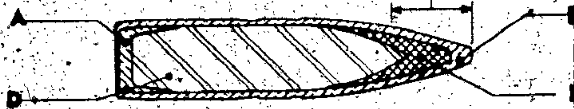
CAL. .30 ARMOR-PIERCING BULLET, M2
