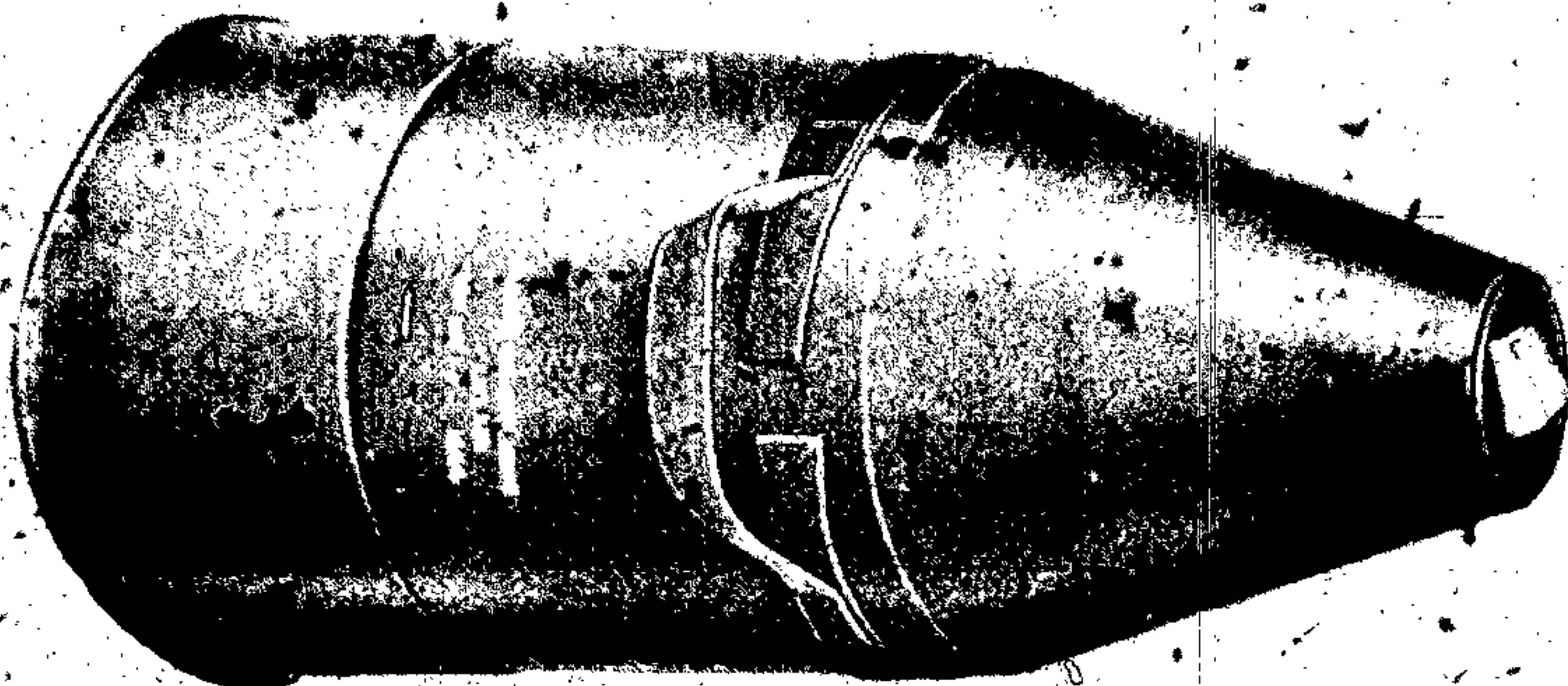
Figure 151 - Shaped Charge, 15-lb, M2A3
