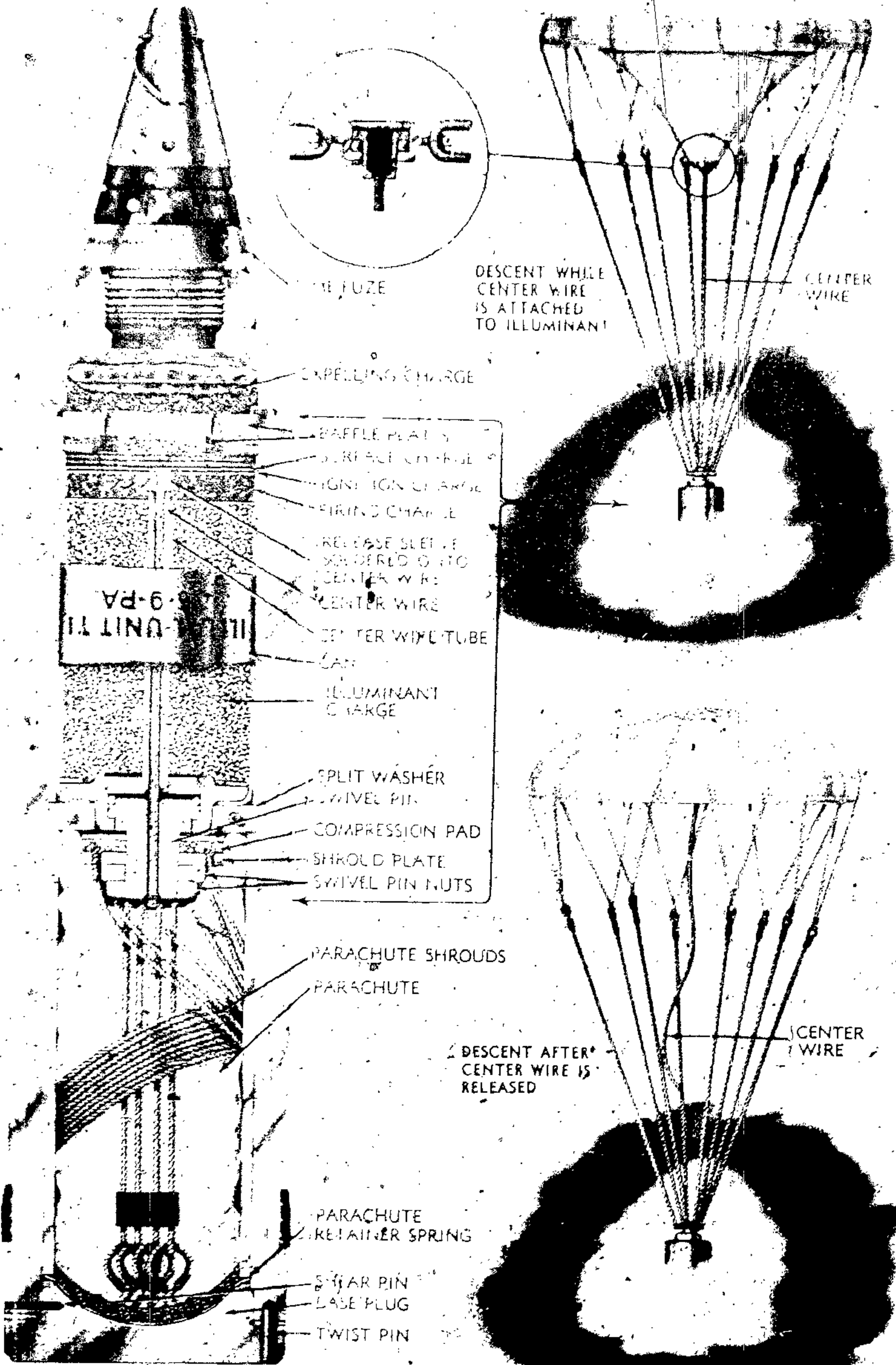
Figure 60 — Typical Illuminating Projectile
