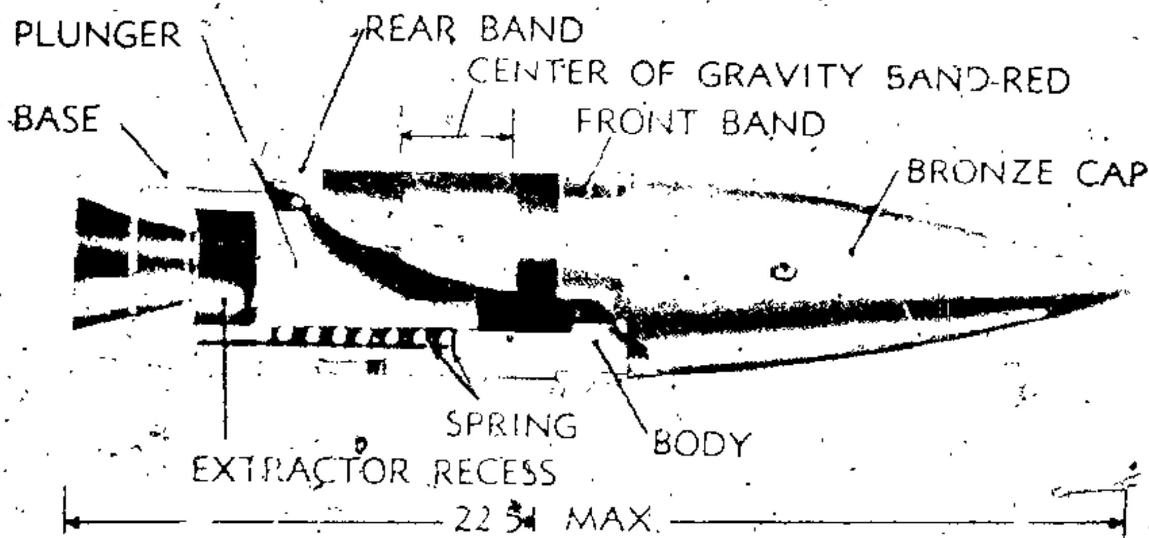
C - TYPICAL SEPARATE-LOADING DUMMY PROJECTILE
