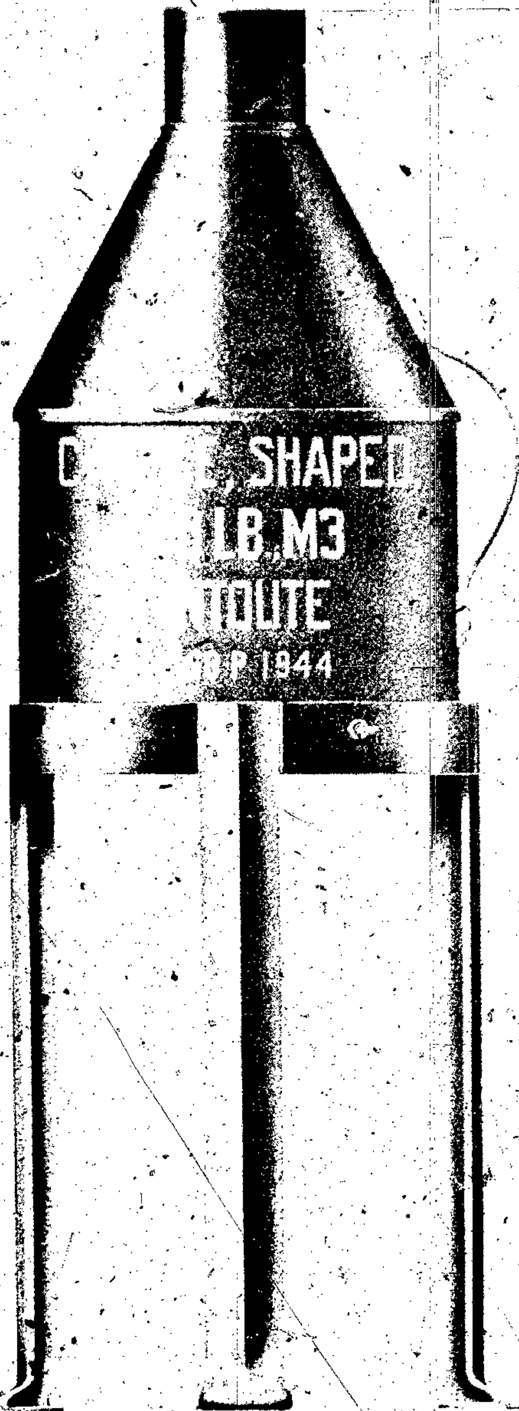
Figure 152.— Shaped Charge, 40-lb, M3
