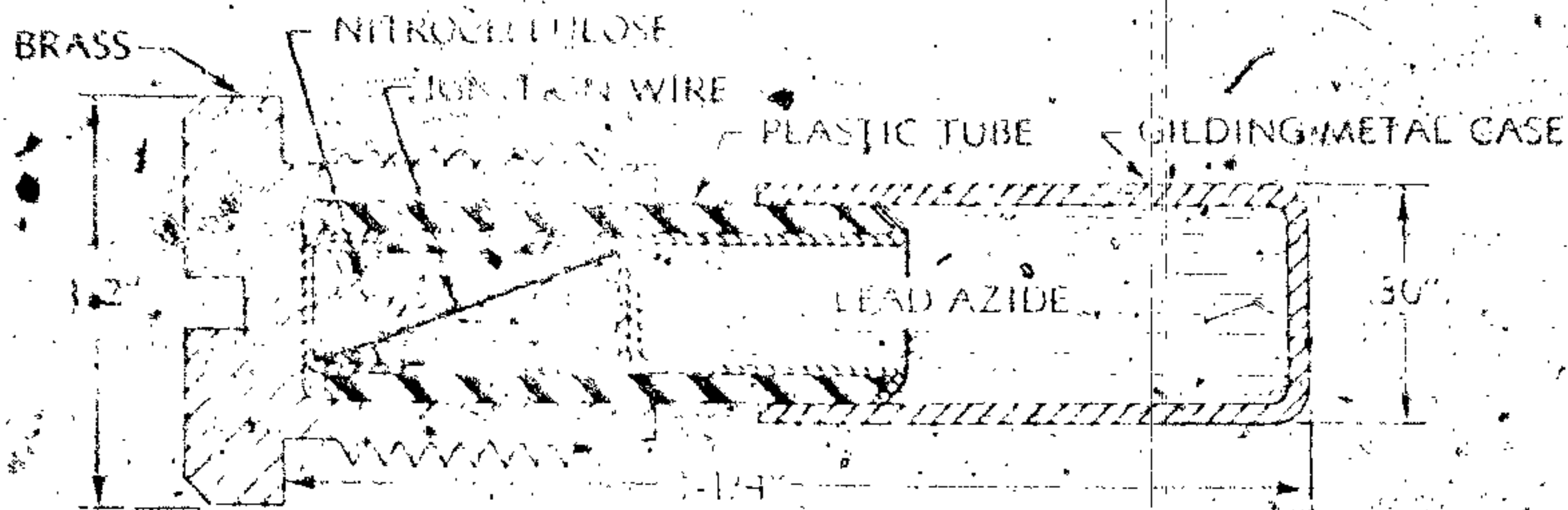
Figure 145 - Destructor AN-M1 - Sectioned
