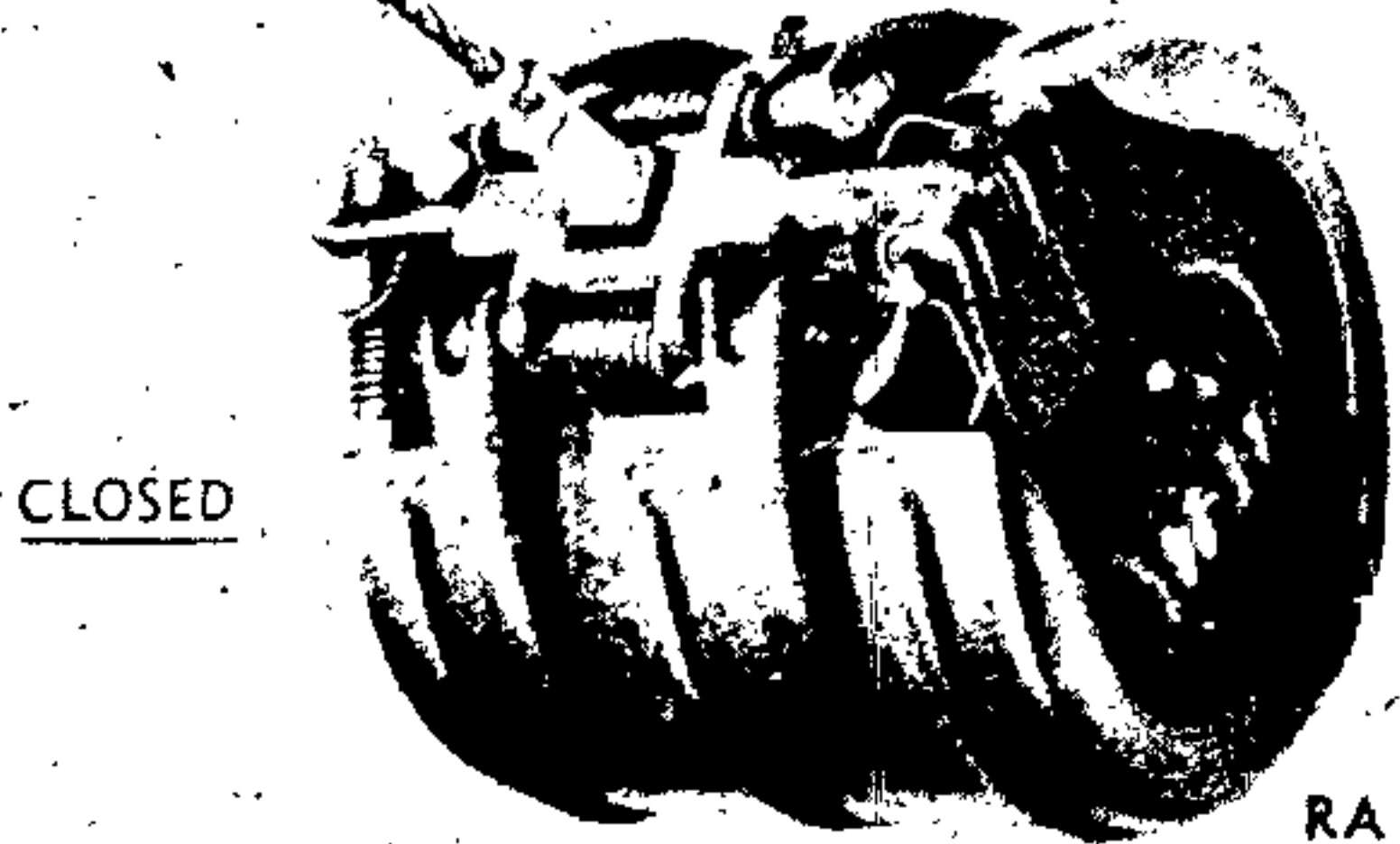
Figure 88 — 4-pound Fragmentation Bomb M83 (Butterfly Bomb)
