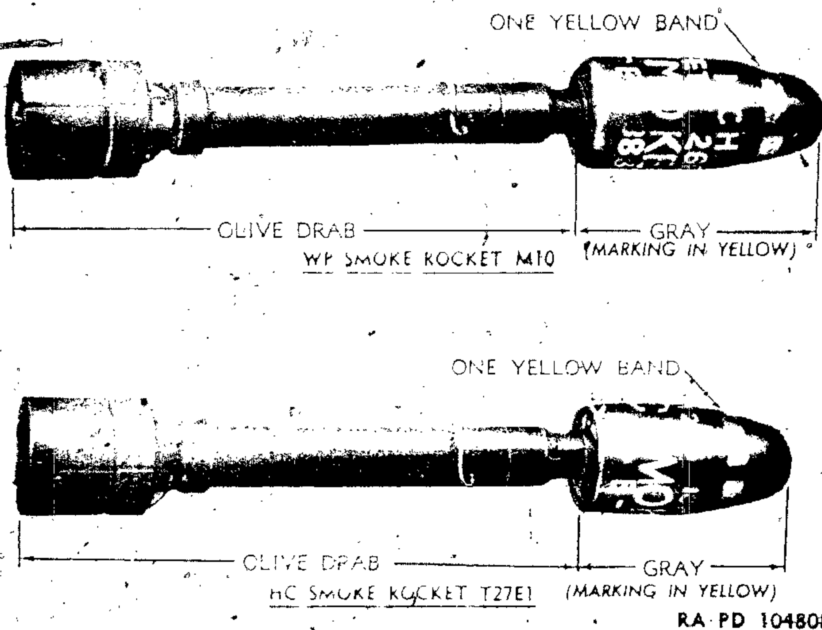
Figure 125 — 2 36-inch Smoke Rockets
