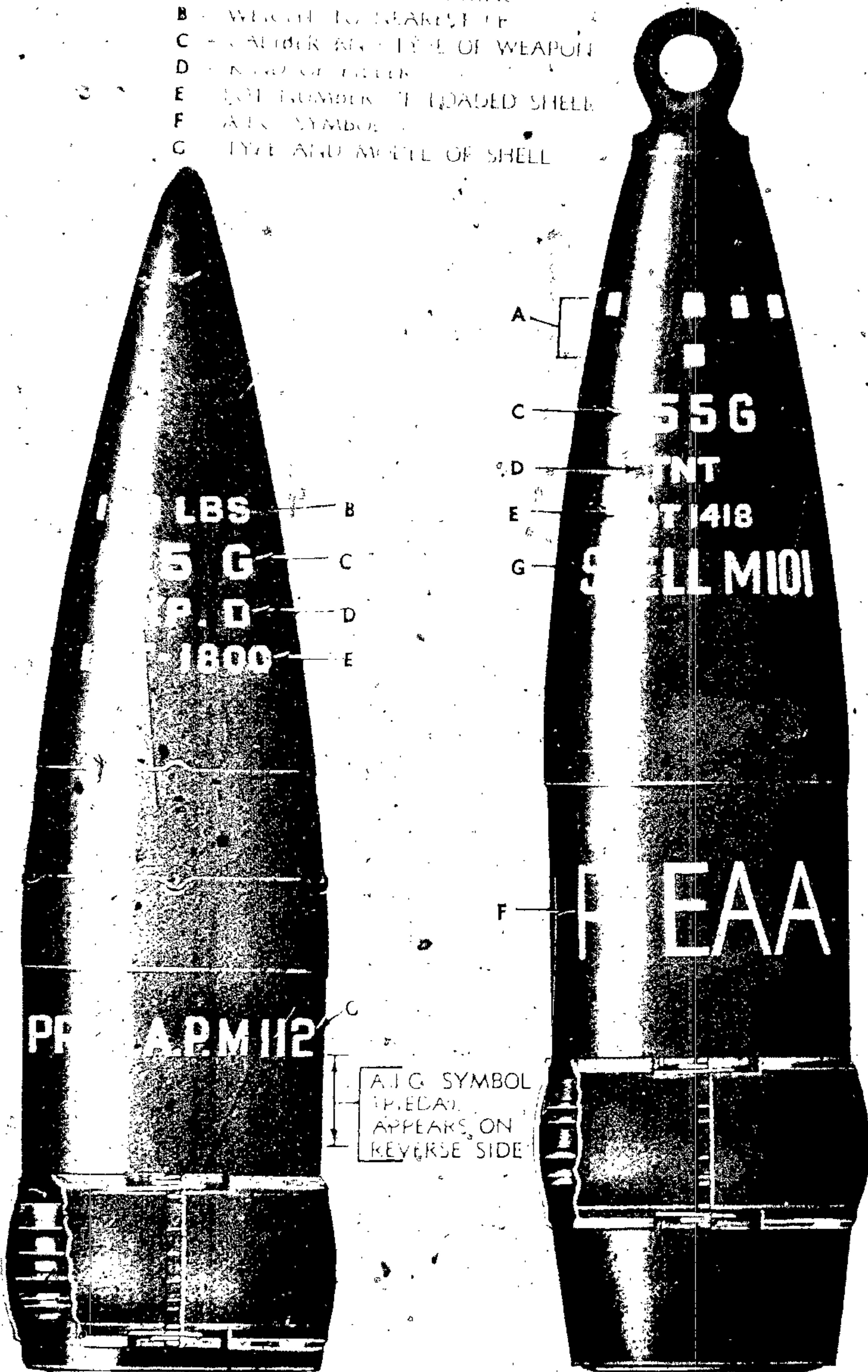
Figure 57 - Marking of Separate-loading Shell - As Shipped
