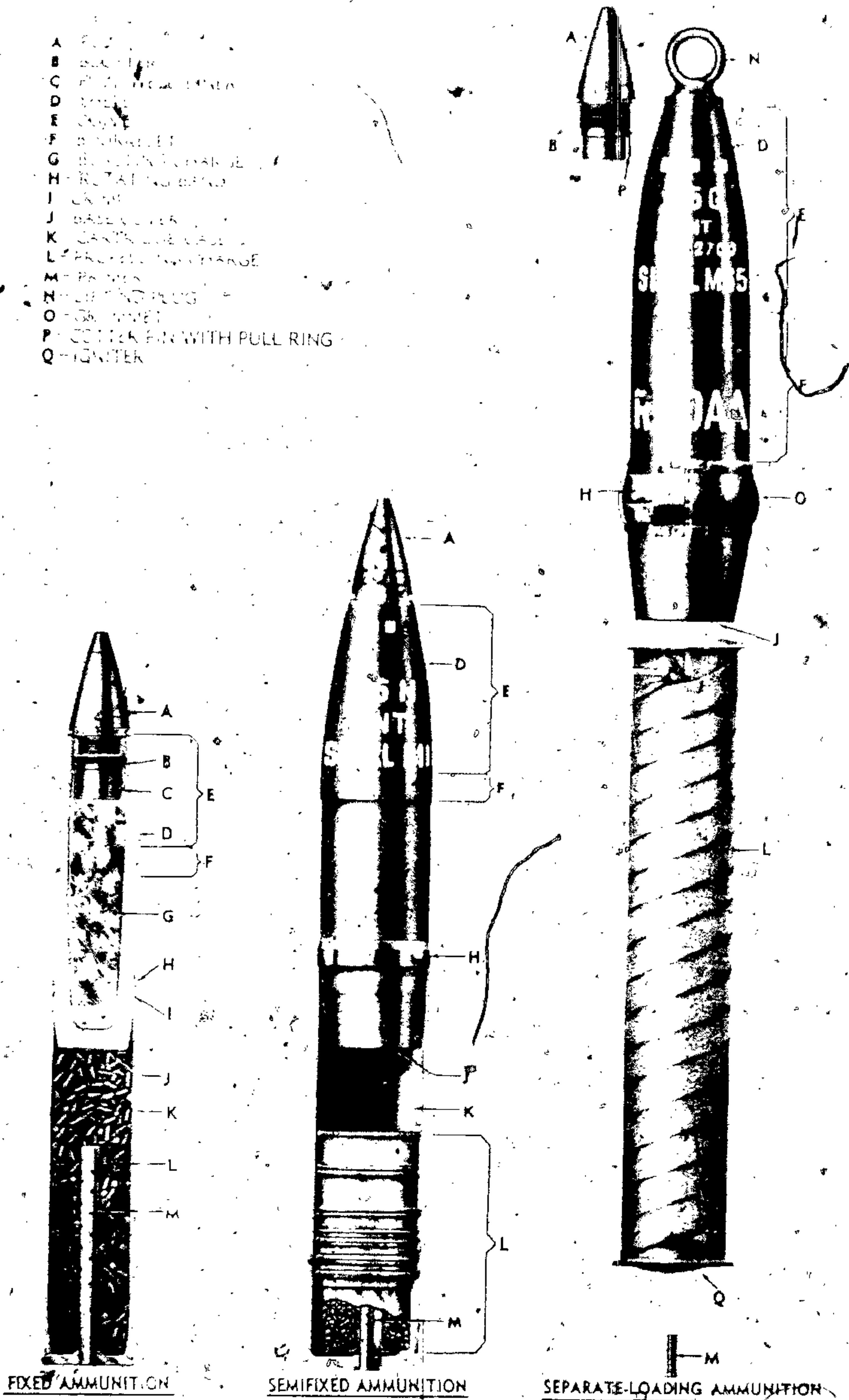
Figure 55 - Types of Complete Rounds of Artillery Ammunition
