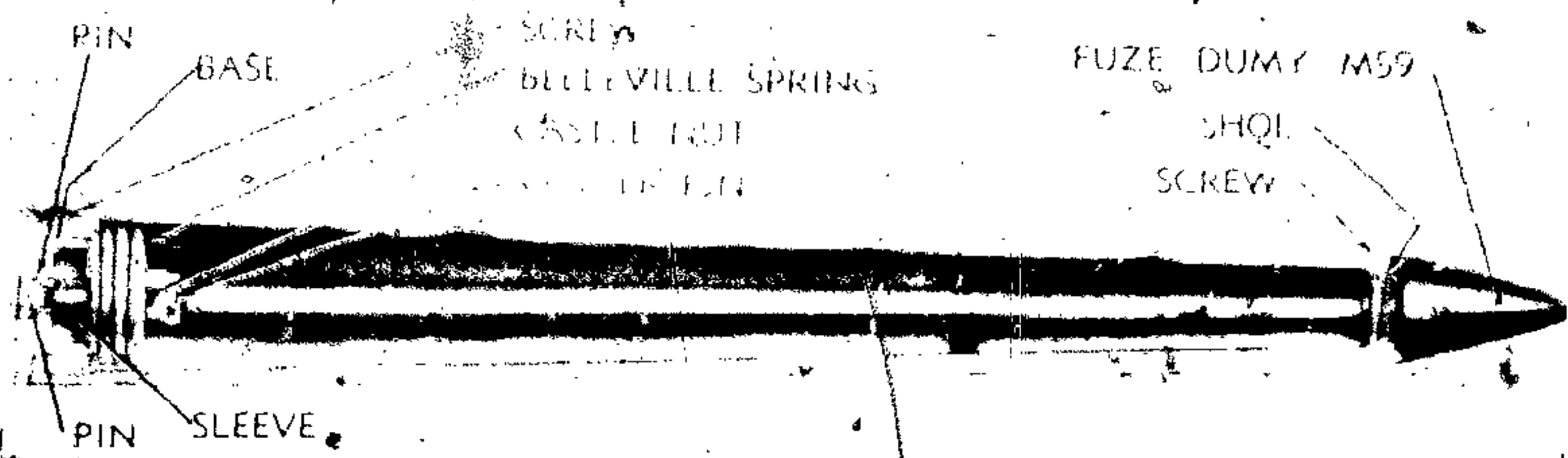
A - TYPICAL DRILL CARTRIDGE
