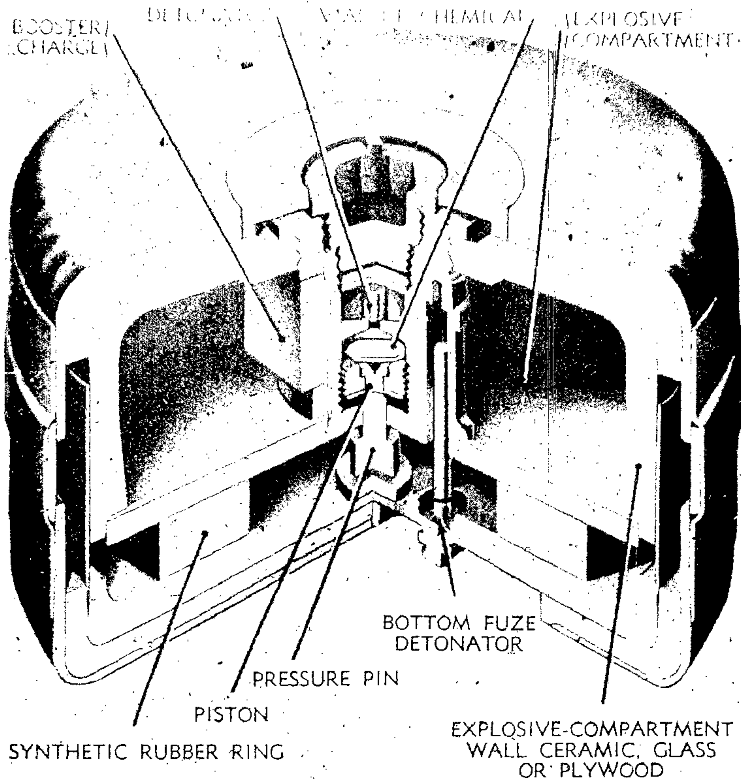
Figure 139 - Nonmetallic Antitank Mine M5
