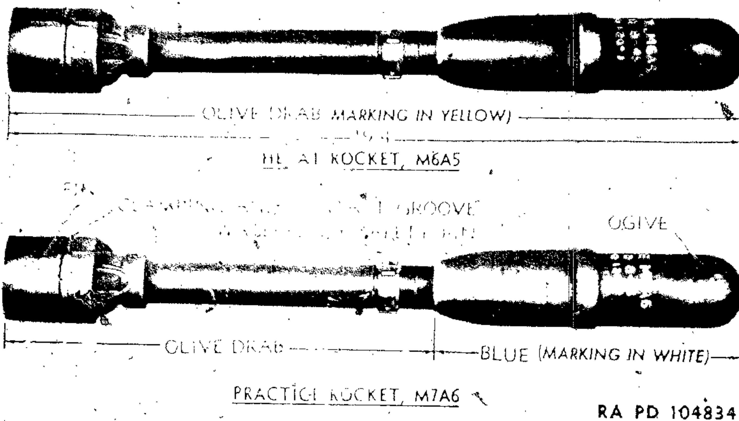
Figure 124 — Rocket M6A5 and Practice Rocket M7A6
