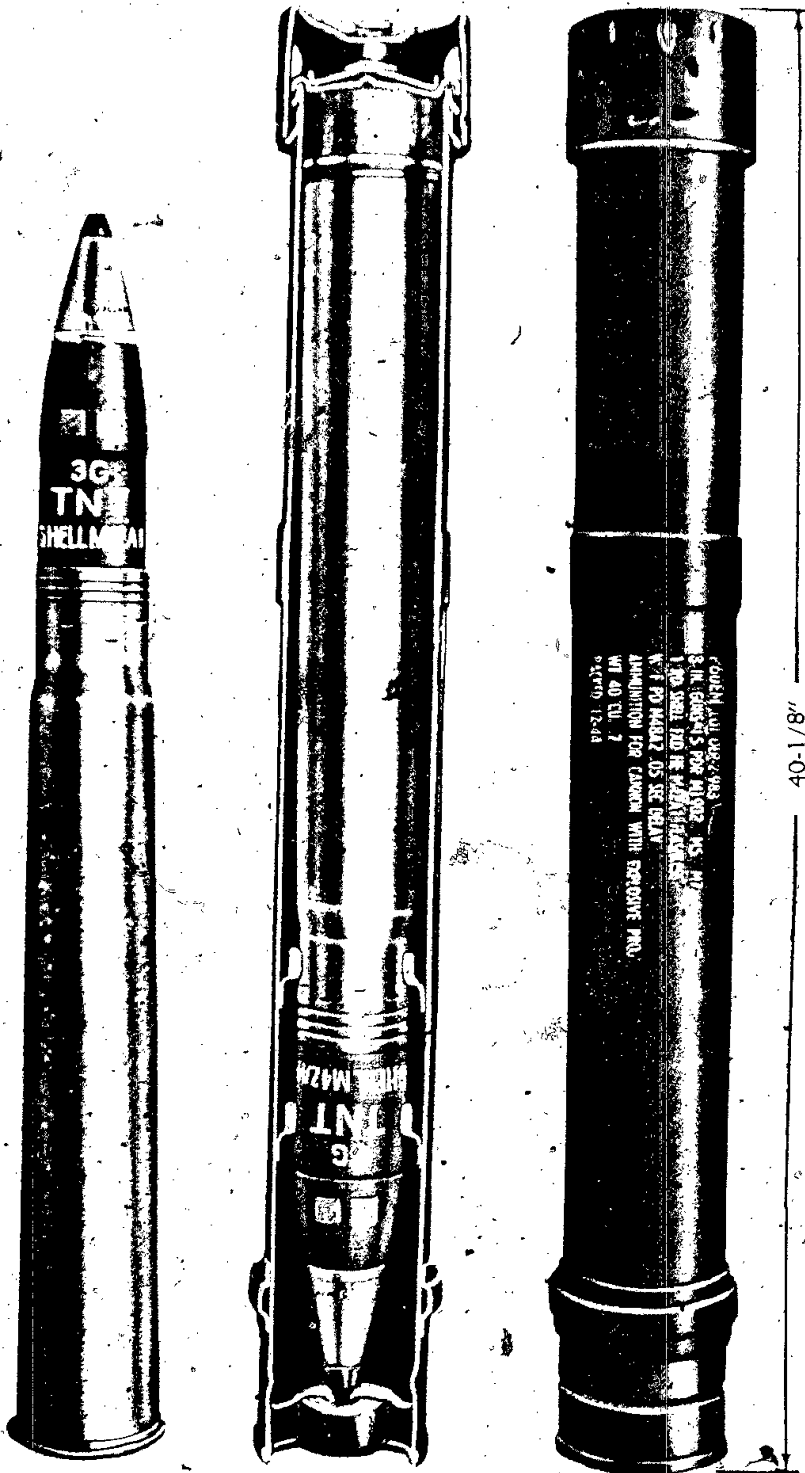
Figure 79 — Metal Container M158 for 3-inch Gun Rounds
