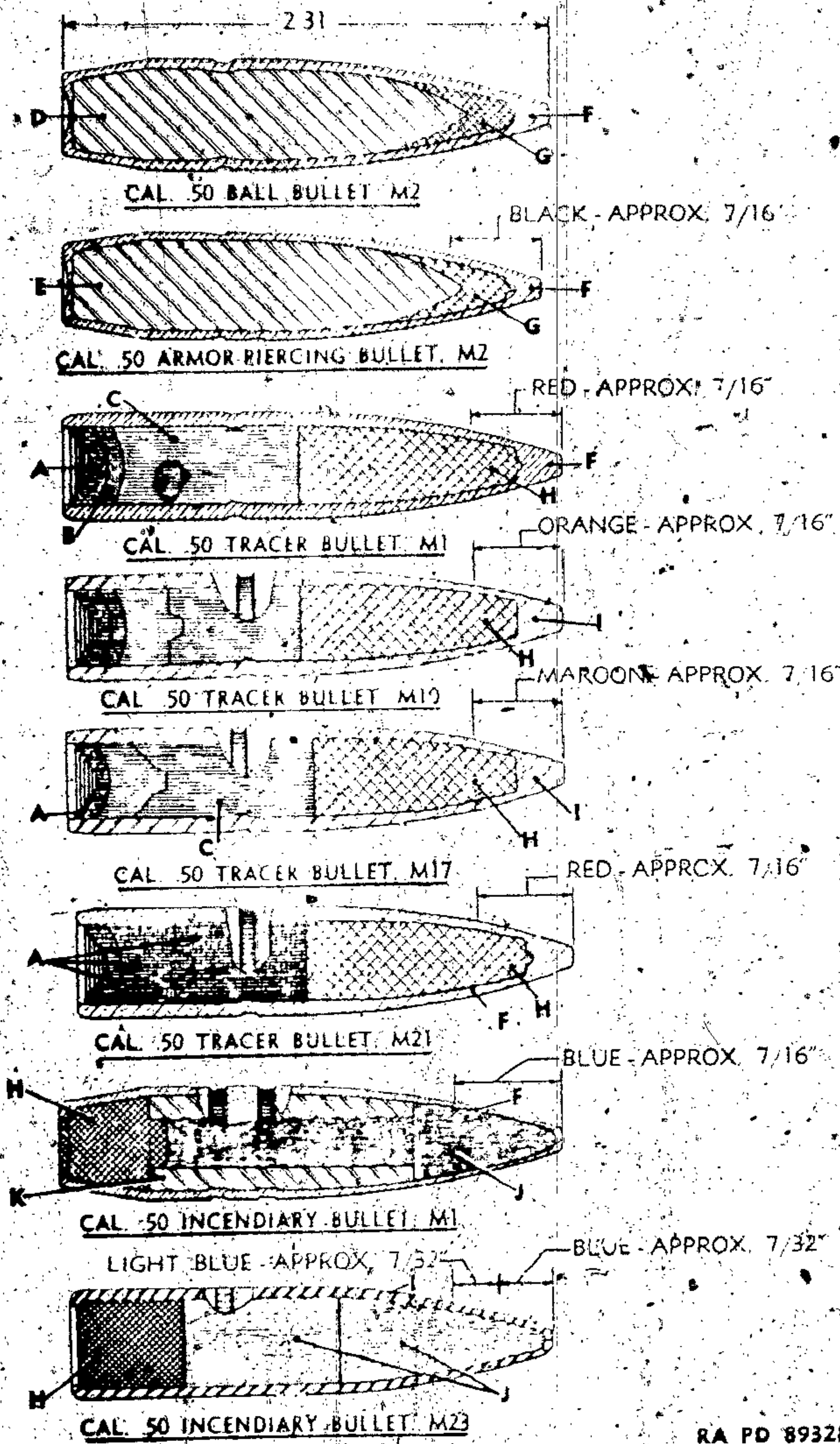
Figure 28 — Caliber .50 Bullets — Cross Section
