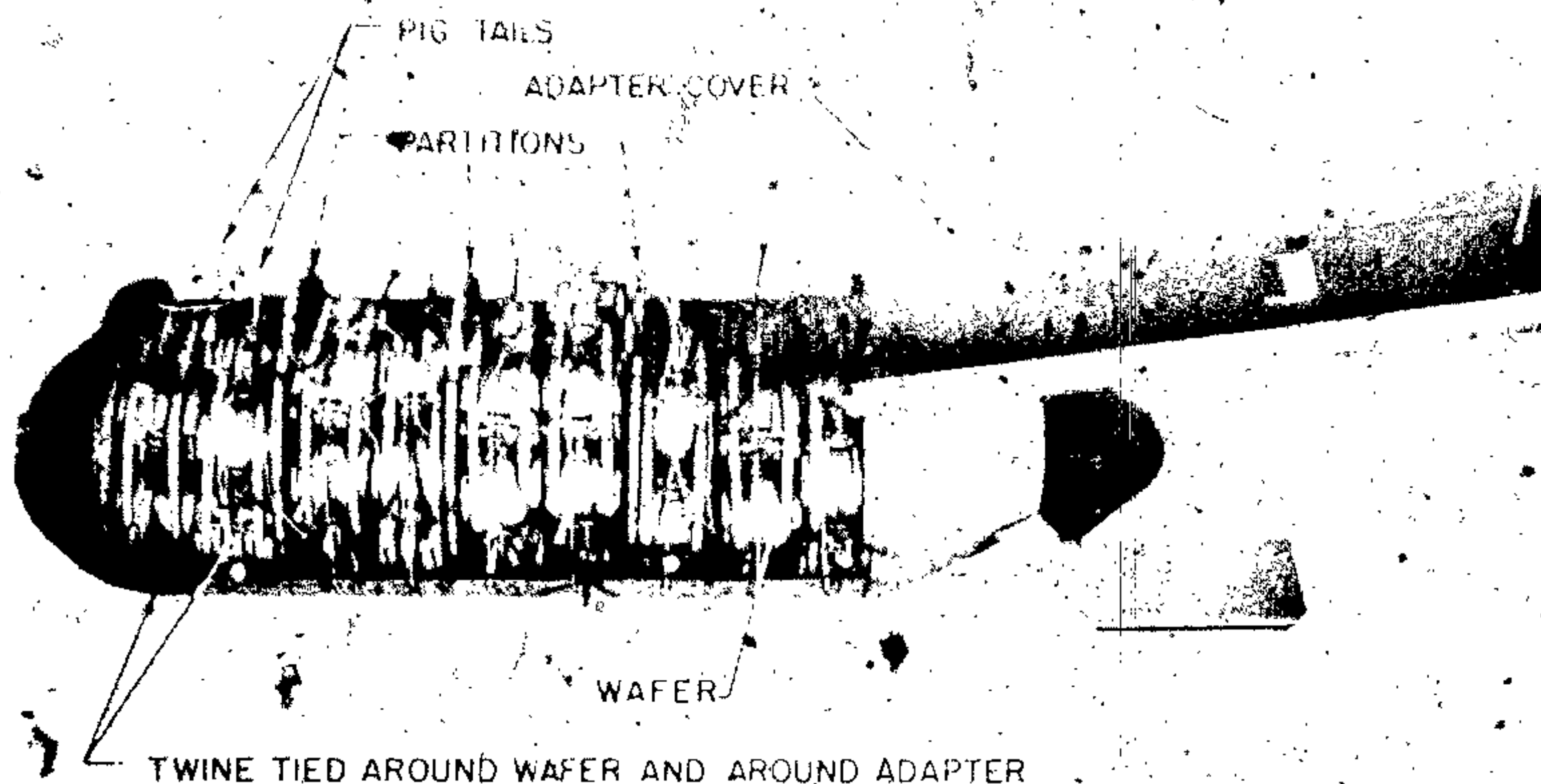
Figure 89 — Wafers in Place in Cluster Adapter
