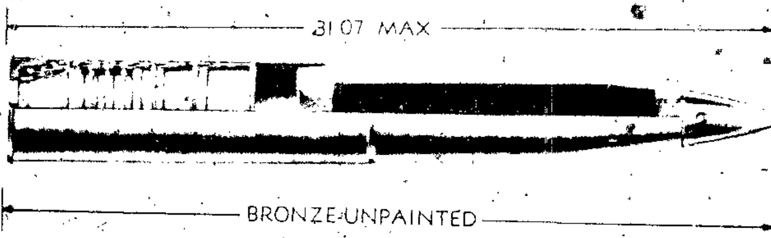
B - TYPICAL SEMIFIXED DRILL CARTRIDGE
