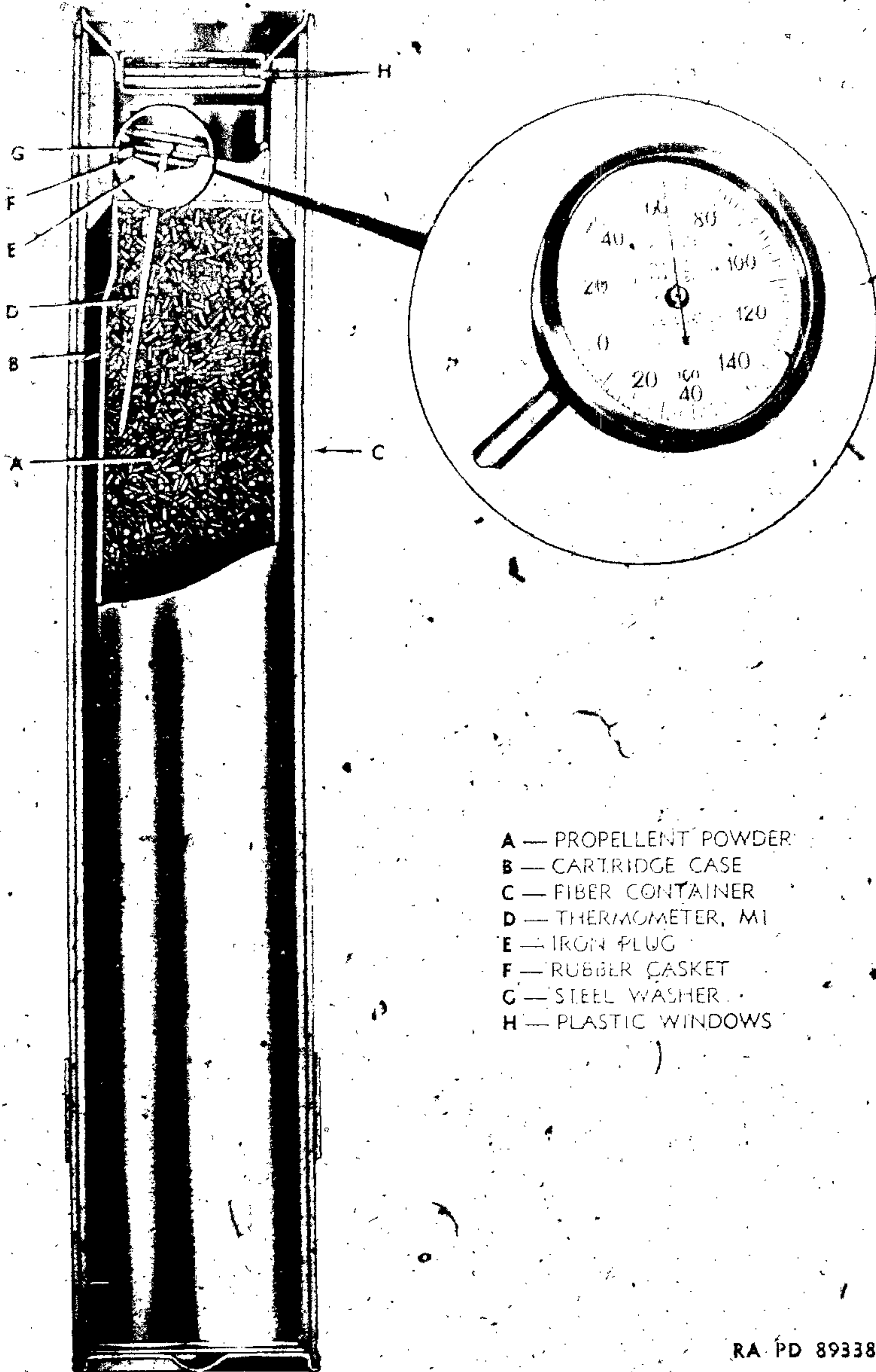
Figure 71 — Powder-temperature Indicator
