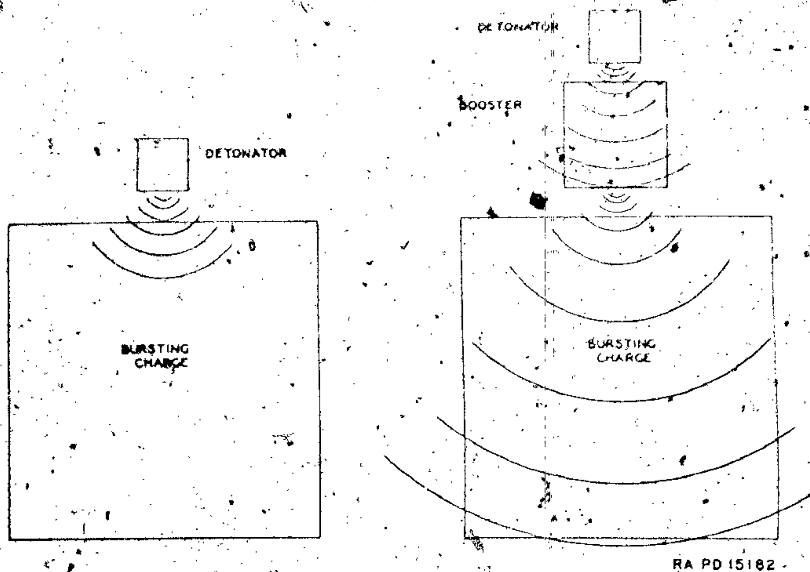
Figure 18 - Detonating Wave Amplified by Use of Booster
