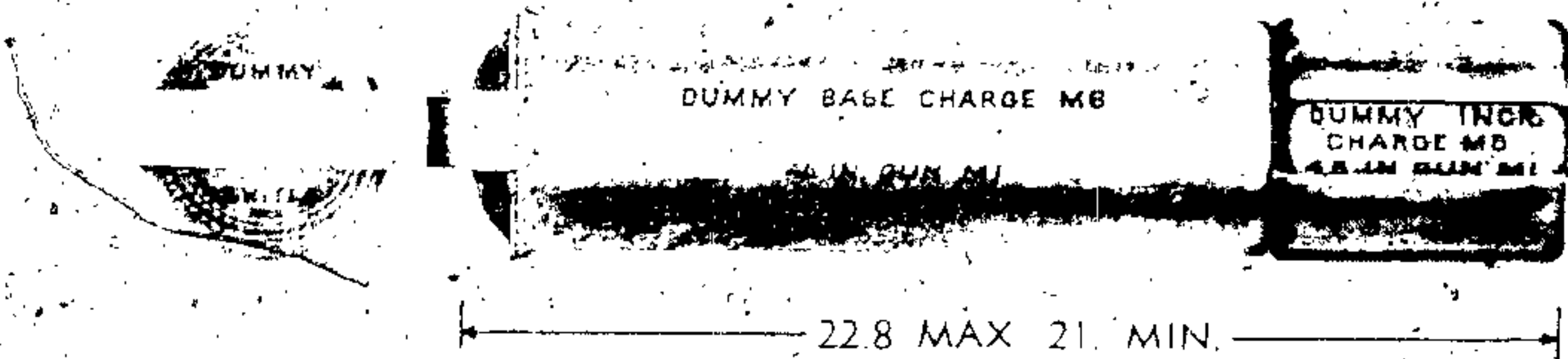
D - TYPICAL SEPARATE-LOADING DUMMY PROPELLING CHARGE
