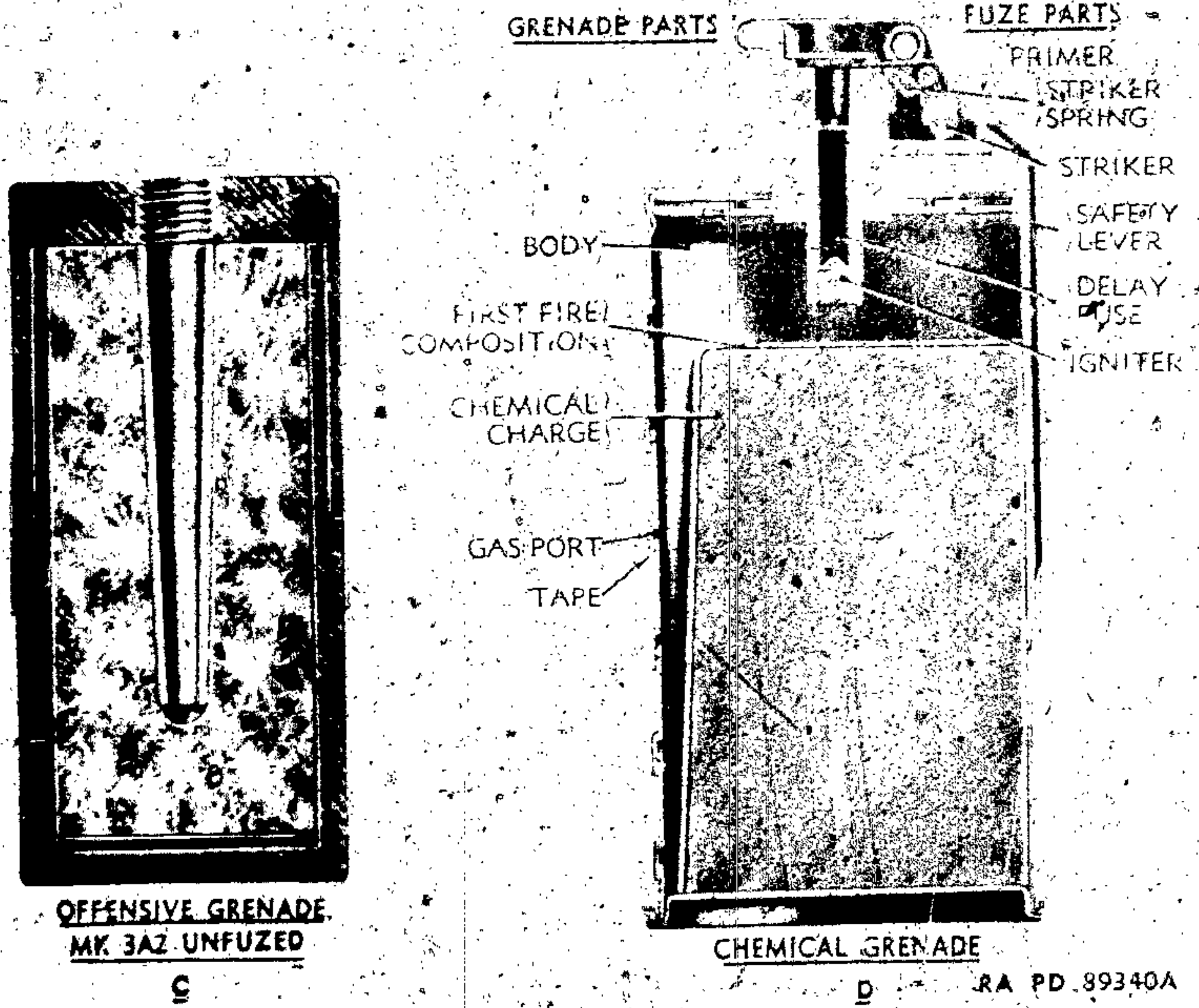
Figure 44 - Hand Grenades - Cross Section
