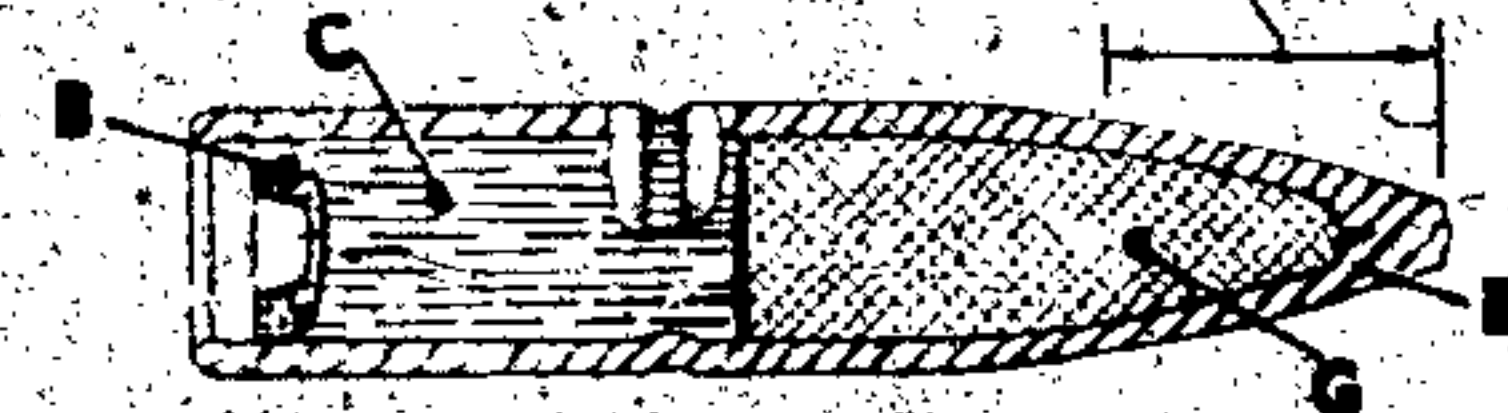
CAL. .30 TRACER BULLET, T10
