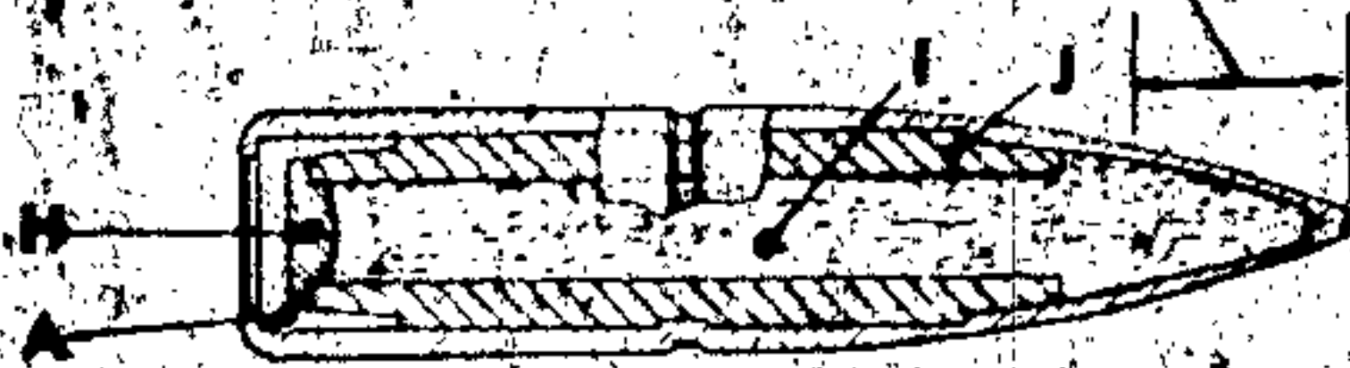
CAL. .30 INCENDIARY BULLET, M1
