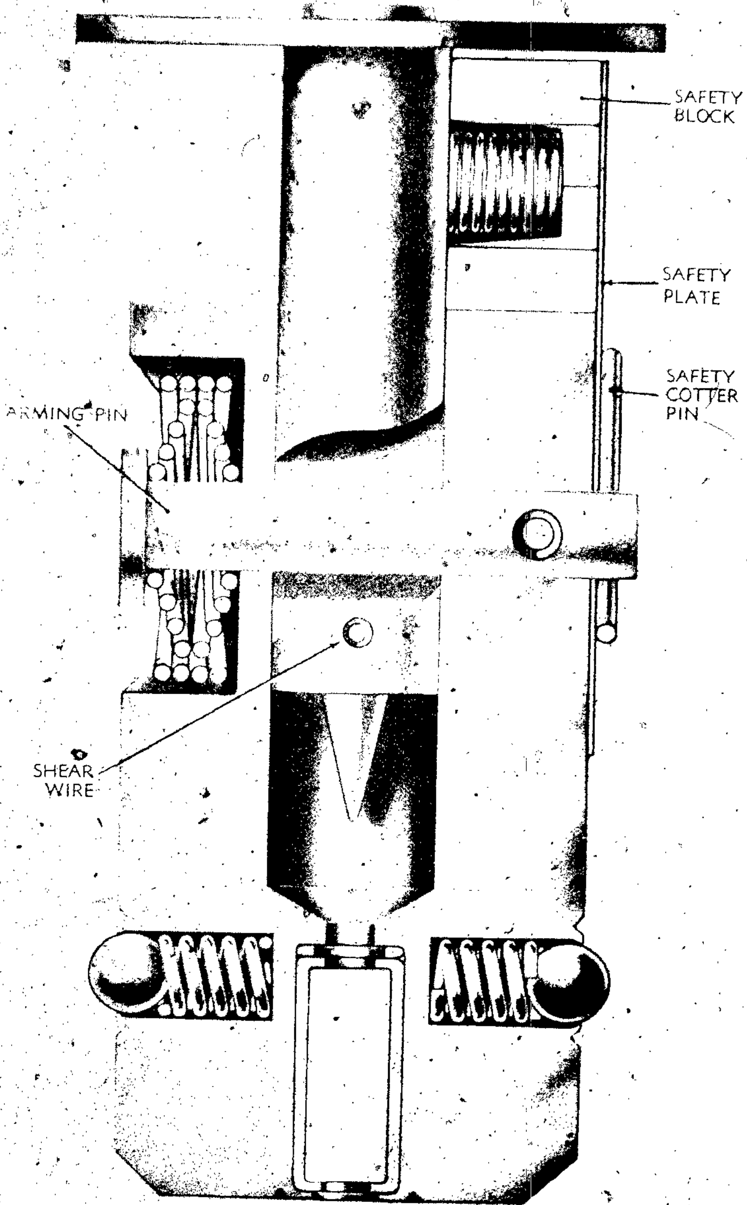
Figure 98 - Nose Fuze - Pin Arming Type (M108)
