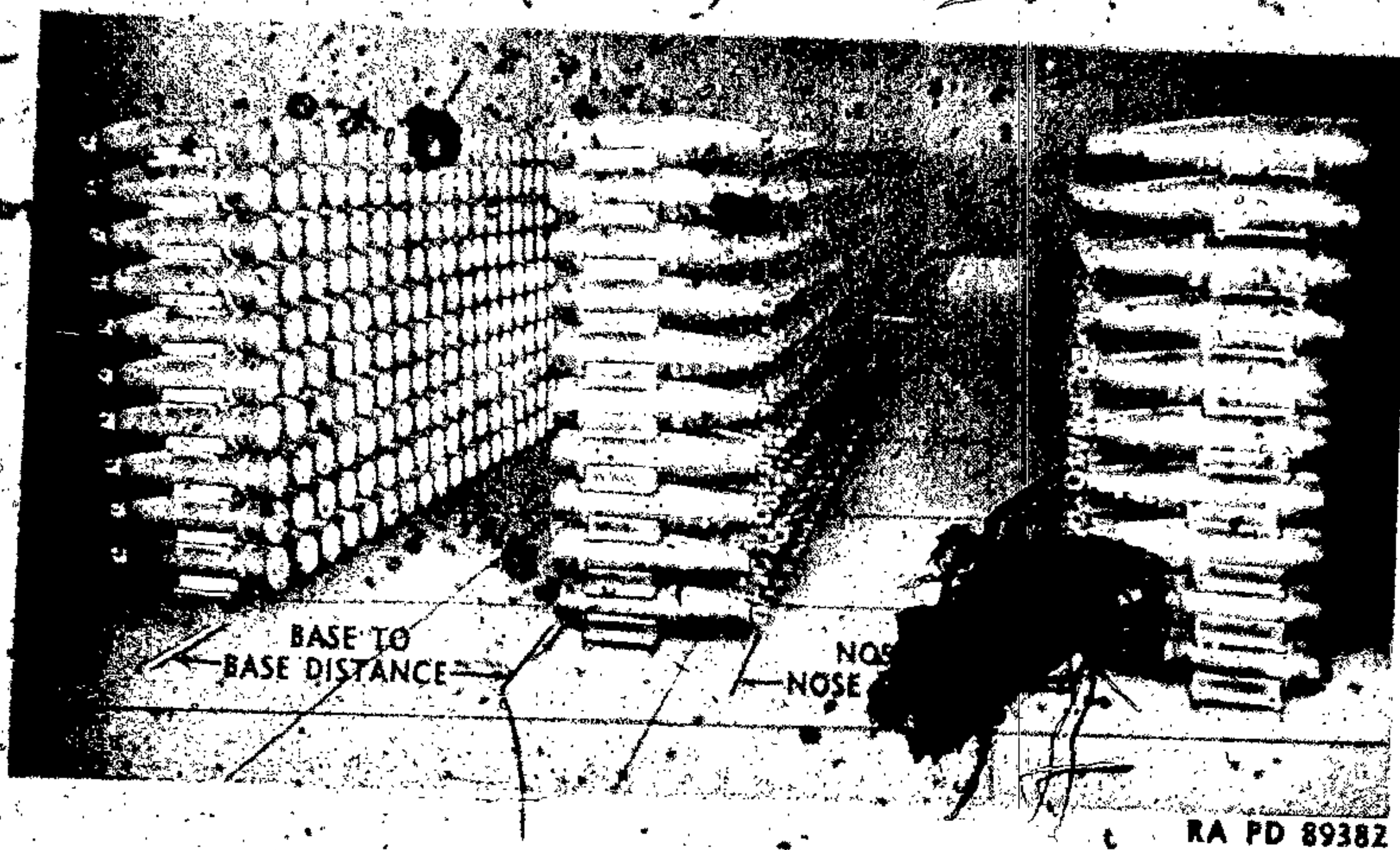
Figure 156 - Method of Stacking Shell in Above-ground Magazine Storage
