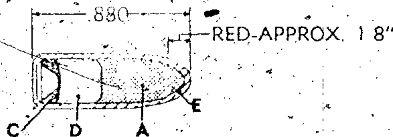
CAL. .30 CARBINE TRACER BULLET, M16
