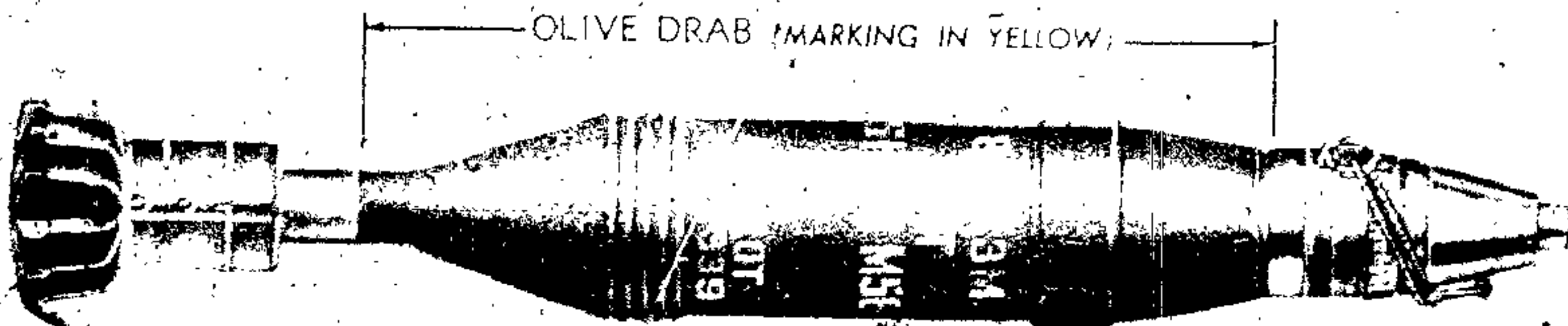
HE SHELL, M56, W, TSQ FUZE, M77
