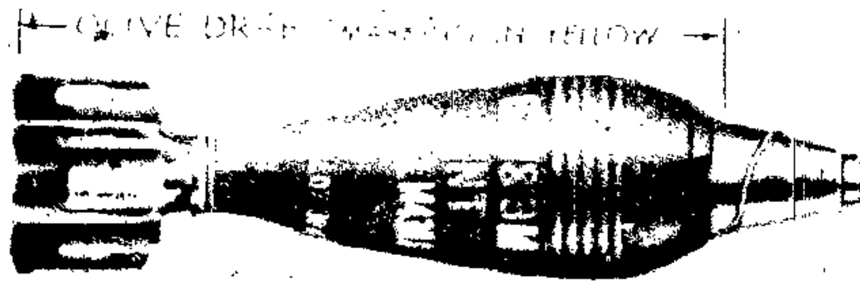
HE SHELL, M3A1, W PD FUZE, M52
