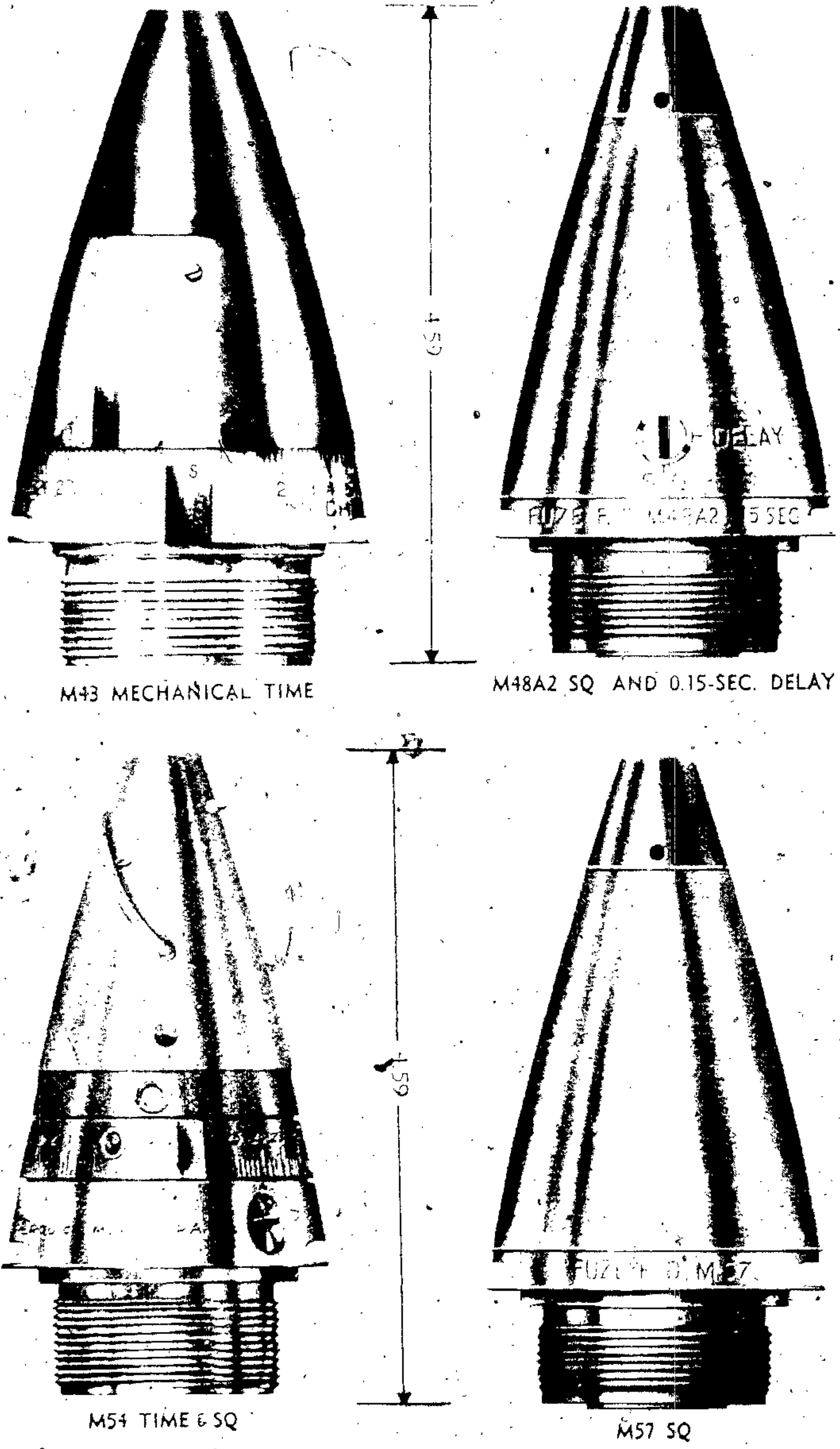
Figure 63 — Fuzes for Fixed and Semifixed Ammunition
