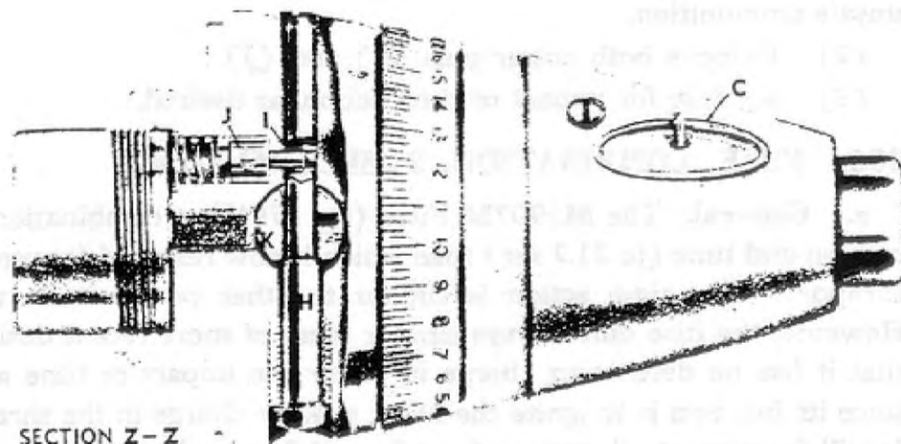
Figure 178 — FUZE, TSQ., M77 (T88)
