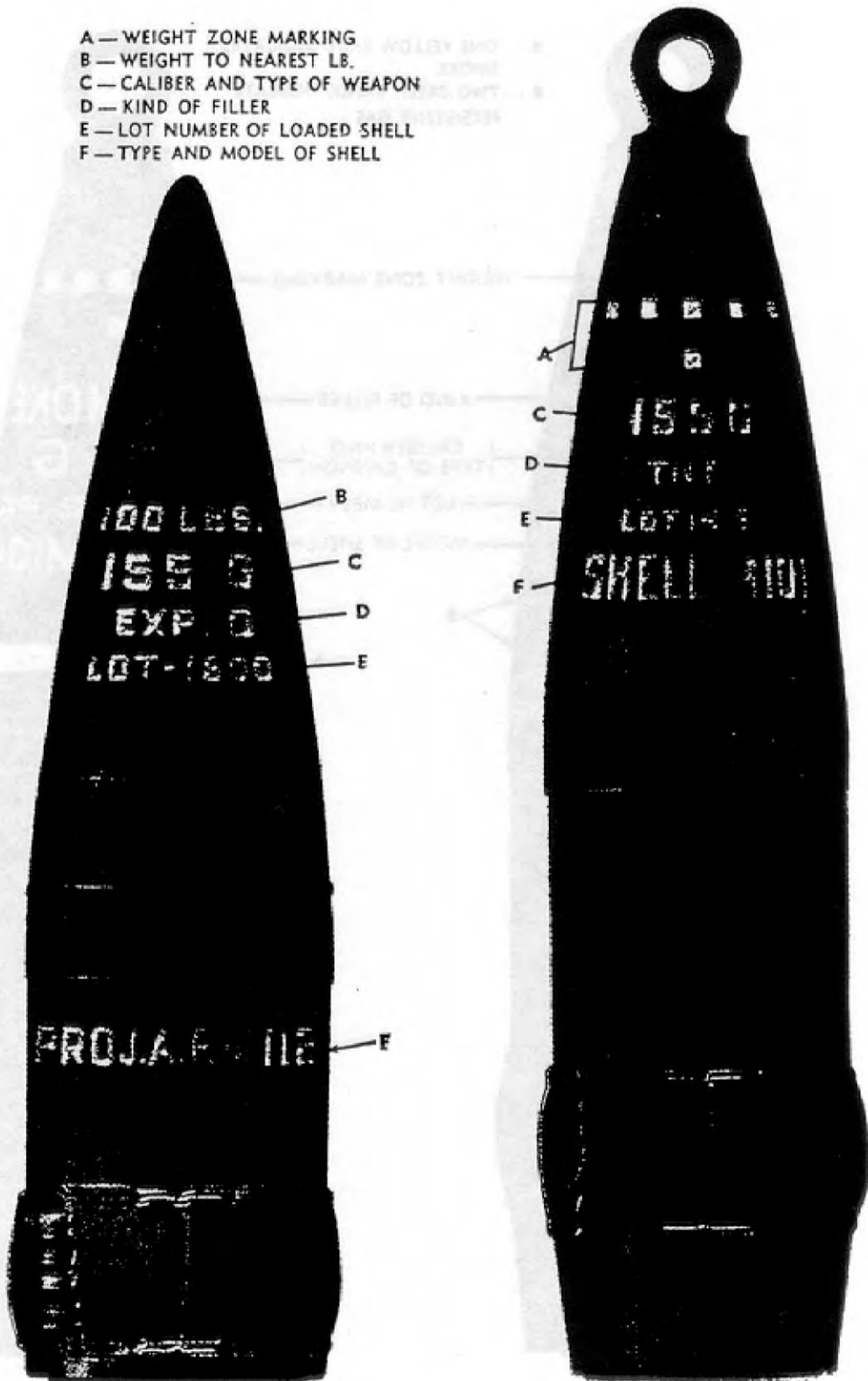
Figure 8 — Typical Marking of Separate-loading High-explosive and Armor-piercing Projectiles (Early Type Grommet Fastening Shown)
