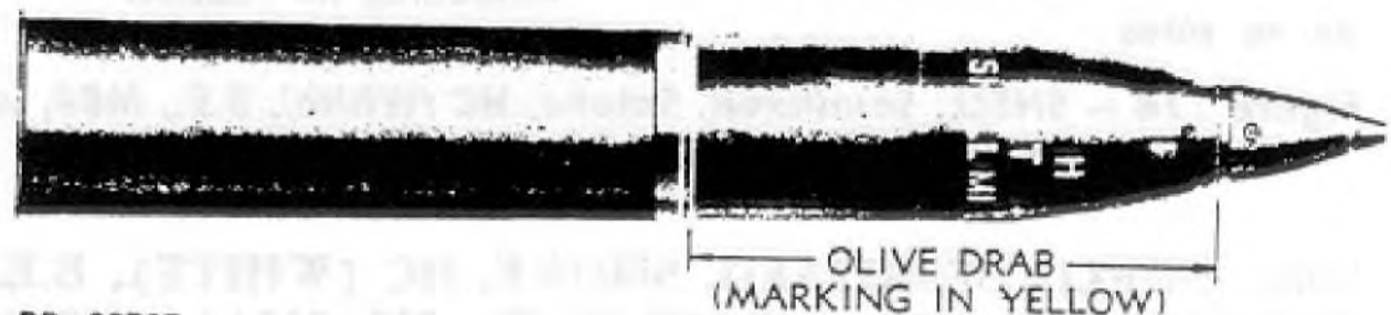
Figure 113 – SHELL, Semifixed, H.E., M1, w/FUZE, P.D., M48A2, SQ & 0.15-sec. Delay, 105-mm How., M2, M2A1, and M4
