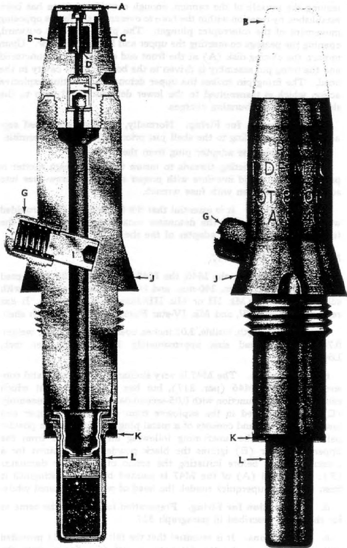
Figure 161 — FUZE, P.D., M46
