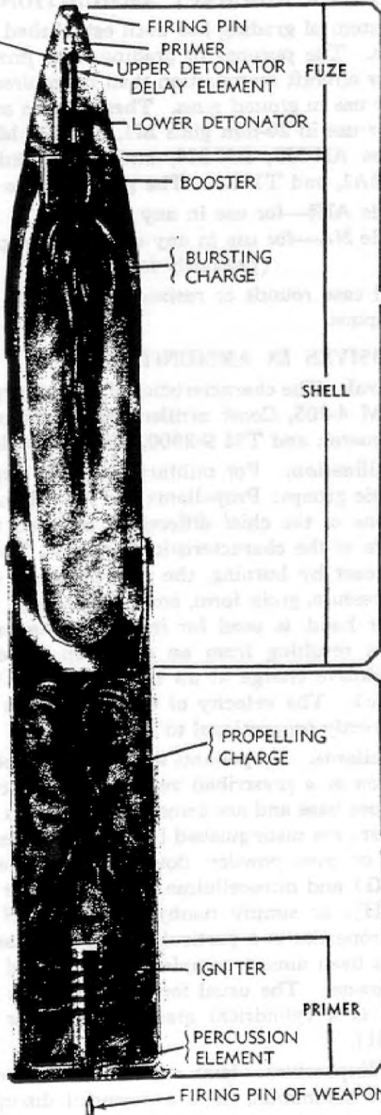
Figure 6 — Explosive Trains — Artillery Ammunition
