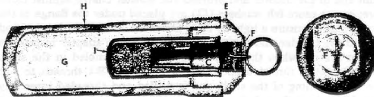
ADAPTER-BOOSTER, MK. VIB
