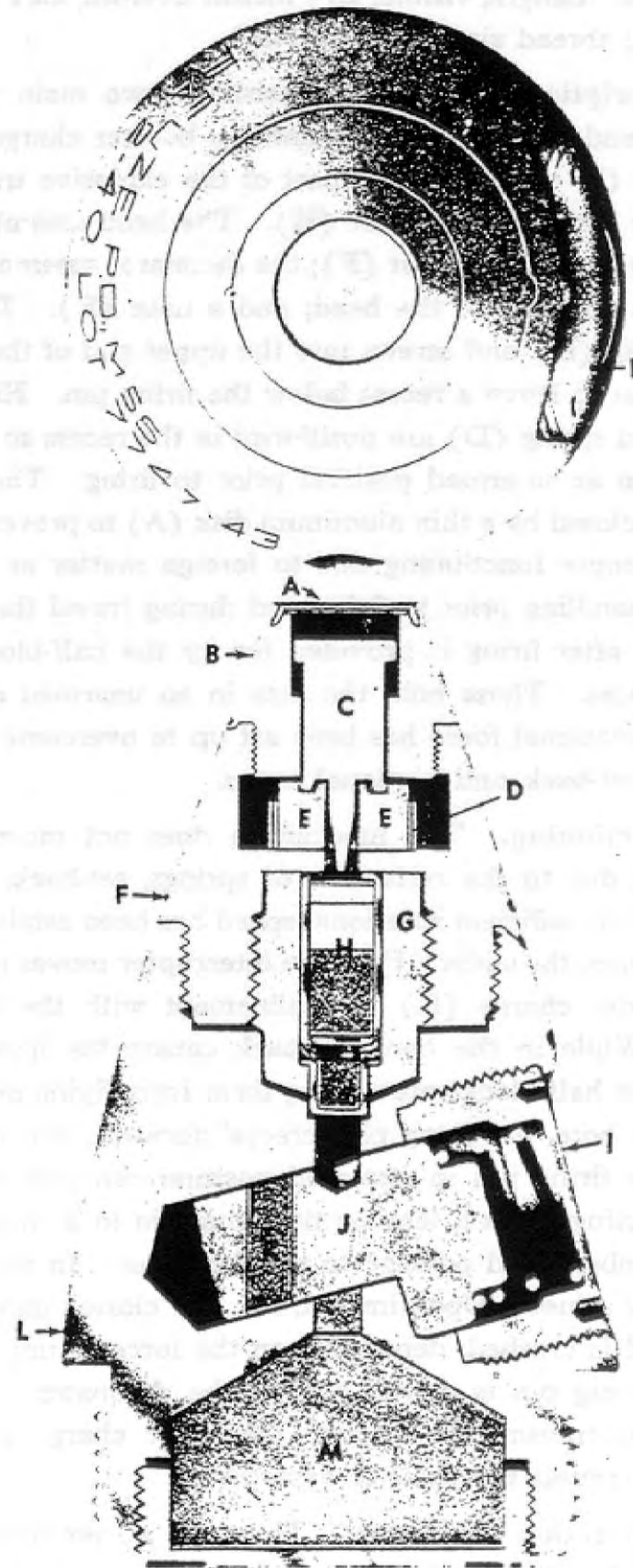
Figure 169 — FUZE, P.D., M56
