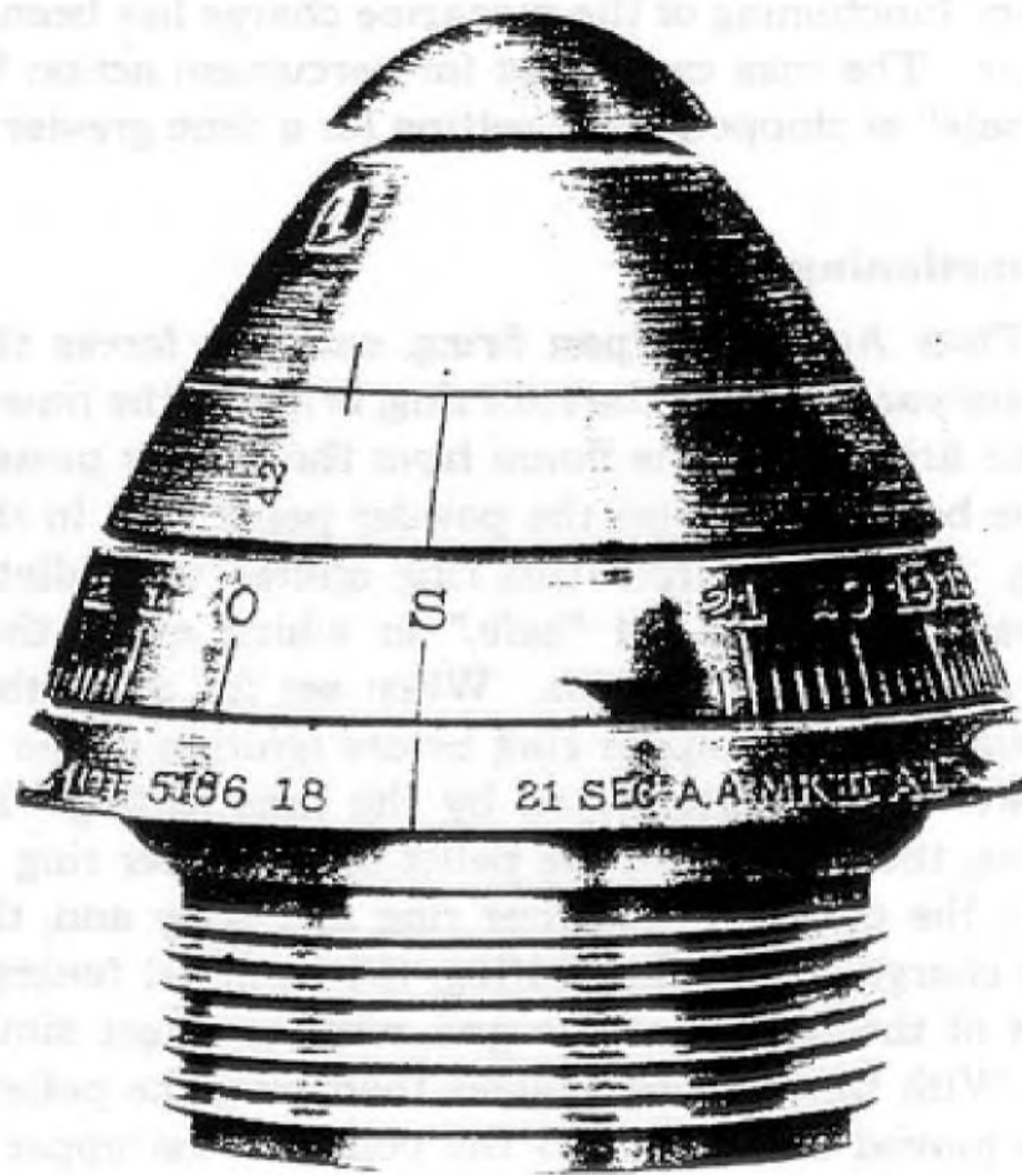
Figure 180 — FUZE, Time, 21-sec., AA., Mk. IIIA1
