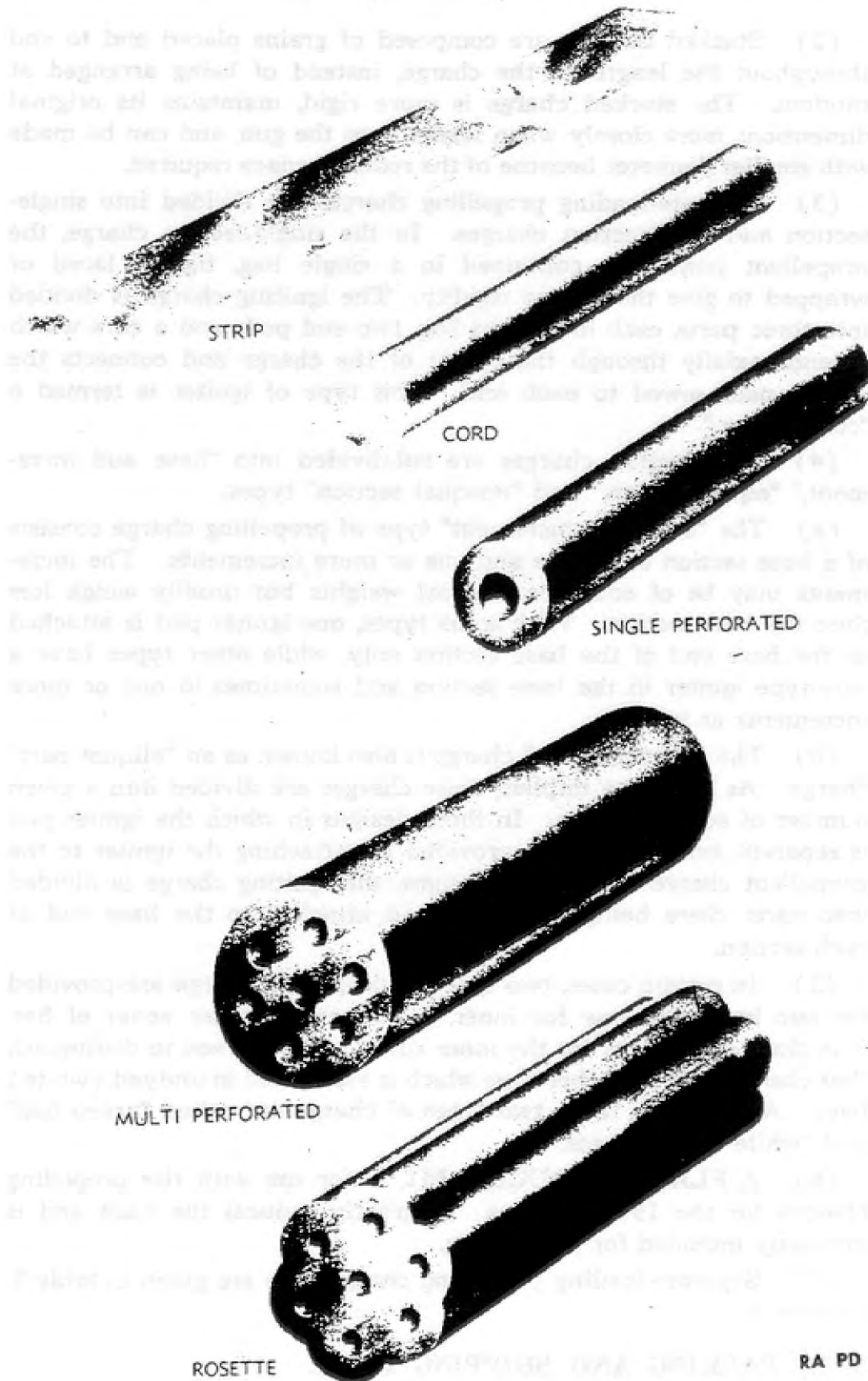
Figure 187 - Types of Powder Grains
