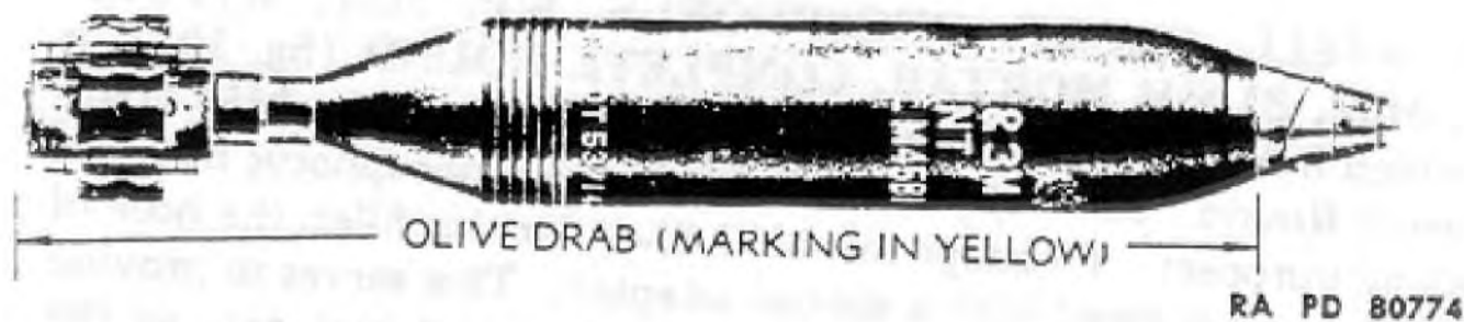
Figure 102 — SHELL, H.E., M45B1, w/FUZE, P.D., M53, 81-mm Mortar, Complete Round
