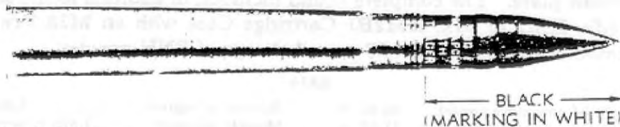
Figure 92 — PROJECTILE, Fixed, A.P.C., M62, w/TRACER, 3" Guns, M1918 (All Models), M3, M5, M6, and M7
