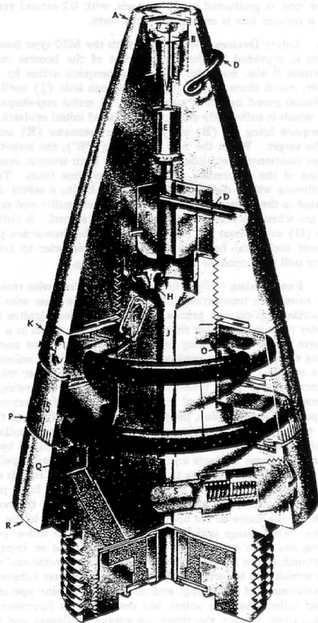
Figure 167 — FUZE, TSQ, M54
