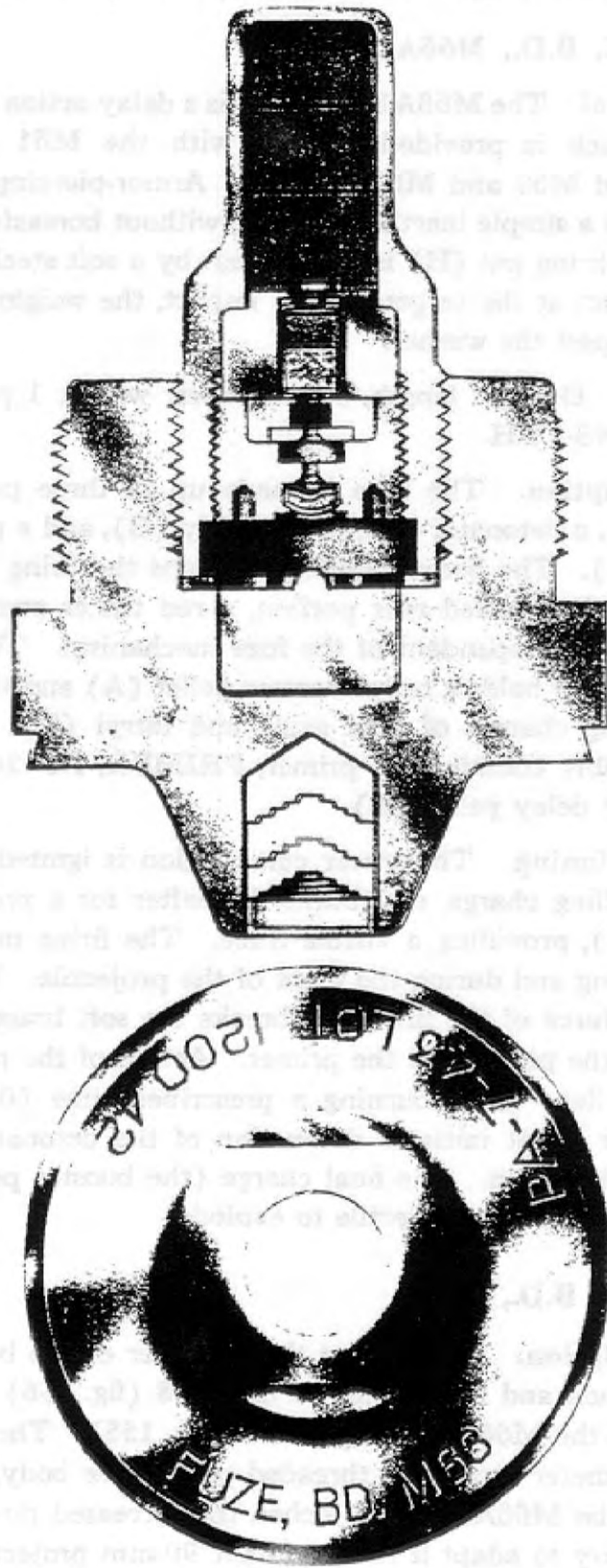
Figure 156 — FUZE, B.D., M68
