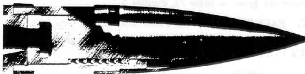
Figure 144 — PROJECTILE, Dummy, 240-lb., M13, 8" Gun
