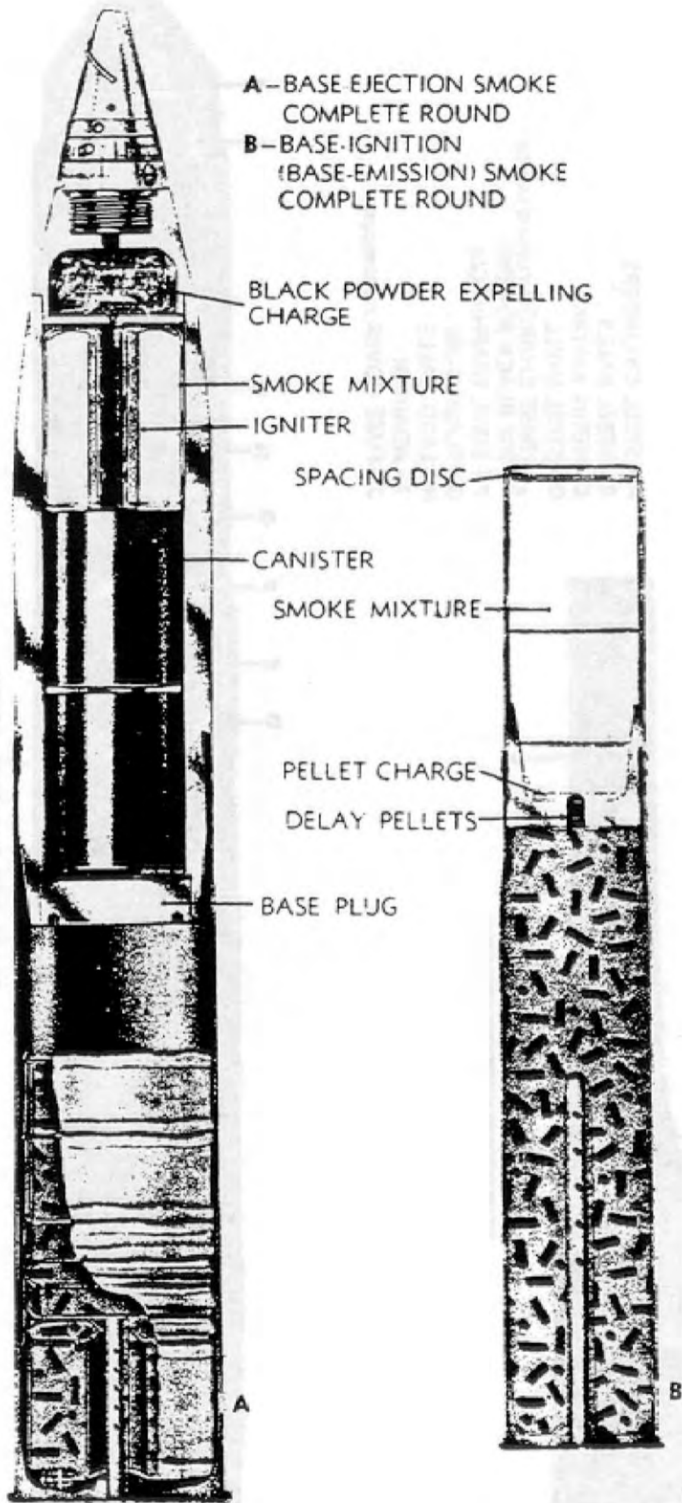
Figure 5 - Typical Base-ignition and Base-ejection Smoke Complete Rounds
