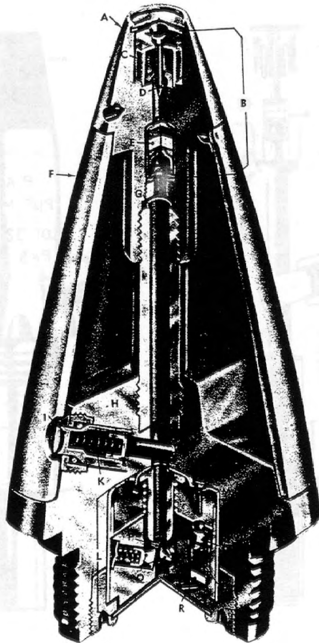
Figure 163 — FUZE, P.D., M48A2
