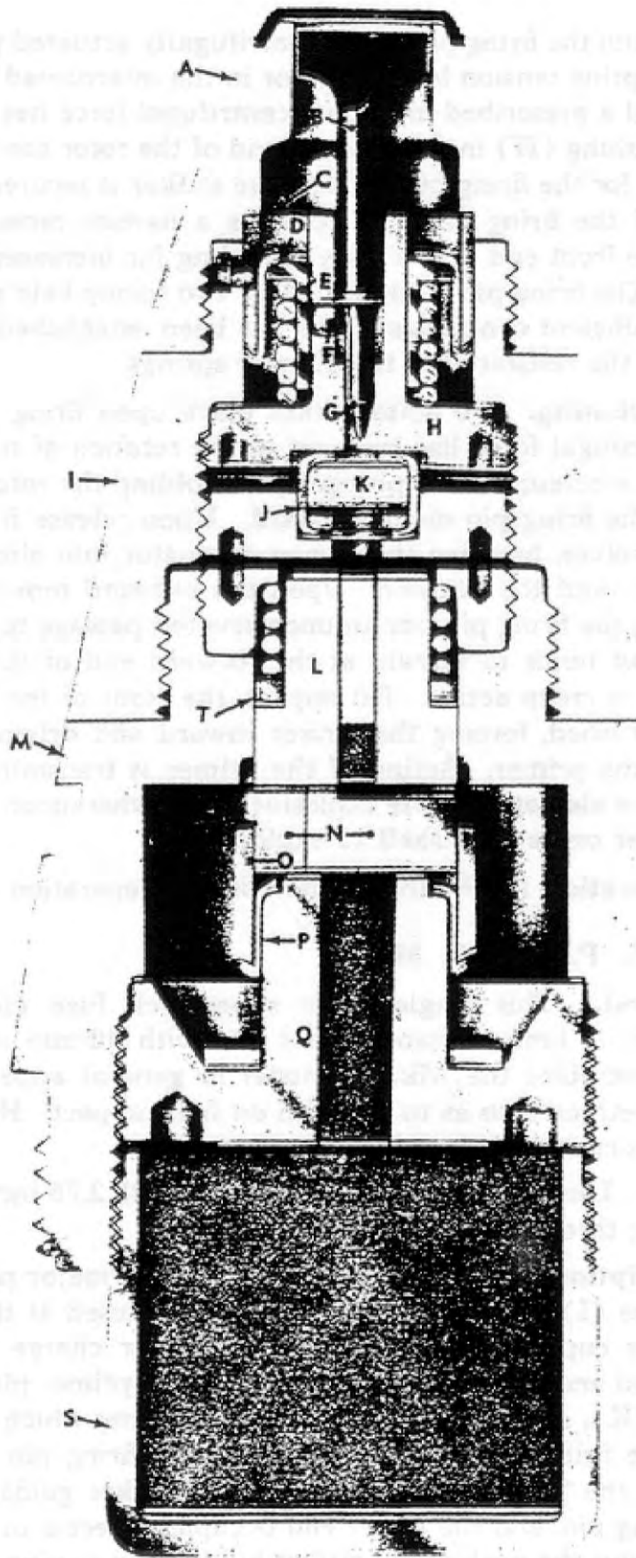
Figure 182 — FUZE, P.D., 251, Mk. I
