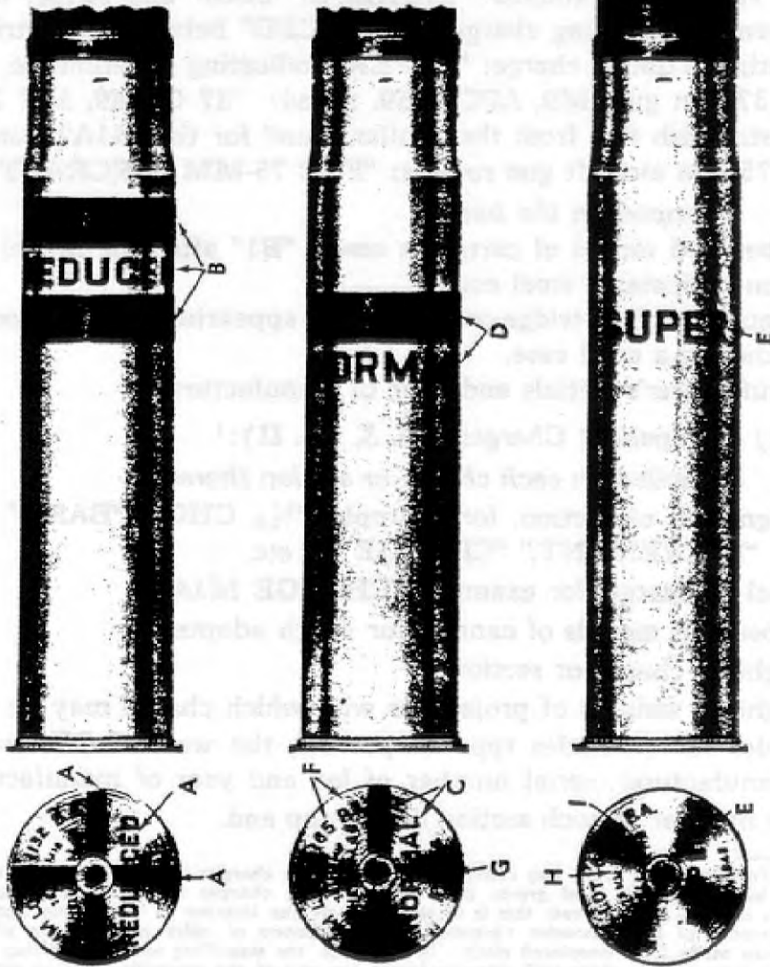
Figure 10 - Marking of 75-mm Complete Rounds Indicating Reduced, Normal, and Super Charges
