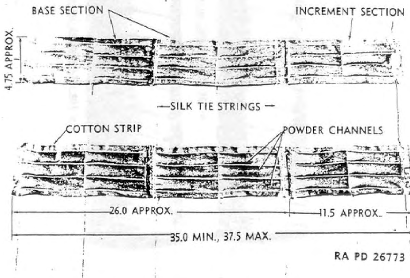
Figure 192 — Flash Reducer, M1
