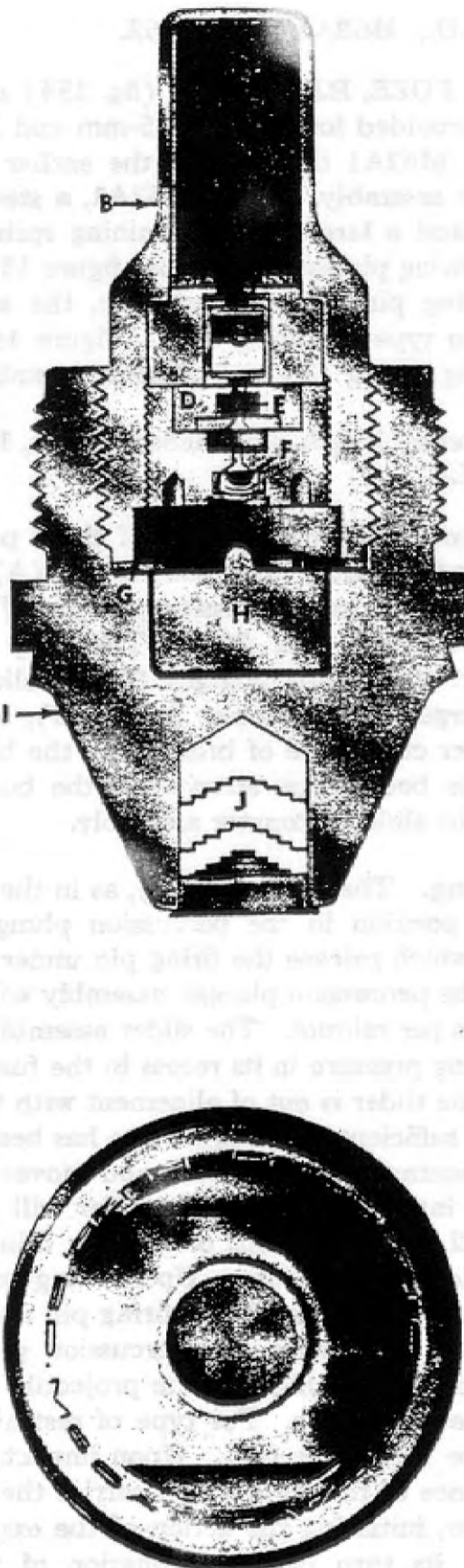
Figure 155 — FUZE, B.D., M66A1
