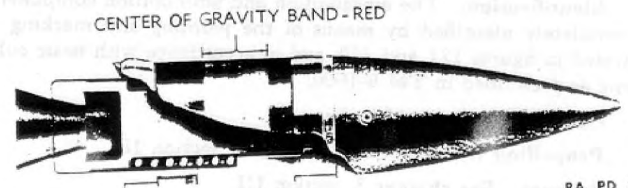
Figure 122 — PROJECTILE, Dummy, M8, 4.5" Gun, M1
