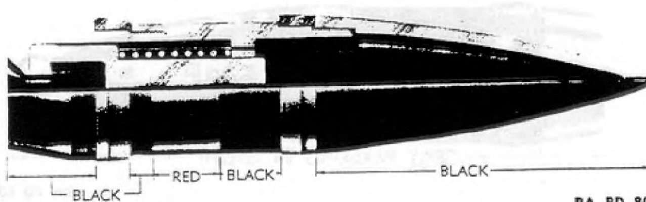
Figure 139 — PROJECTILE, Dummy, 95-lb., M7, 155-mm Gun or How.
