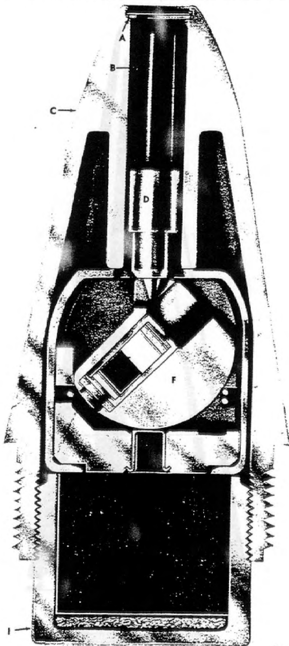
Figure 172 - FUZE, P.D., M64A1
