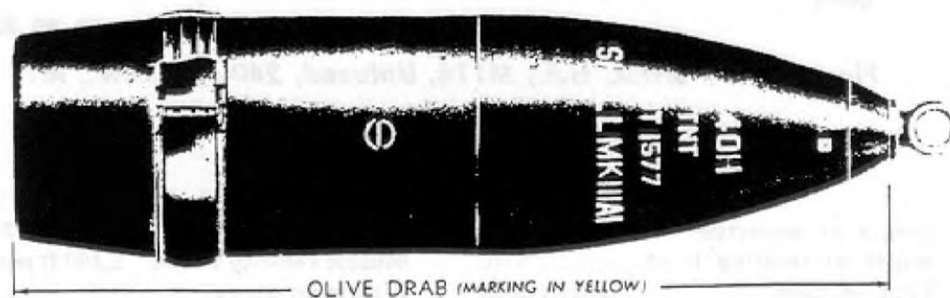
Figure 146 — SHELL, H.E., Mk. IIIA1, Unfuzed, 240-mm How., M1918-18A1-18MI-18MIA1
