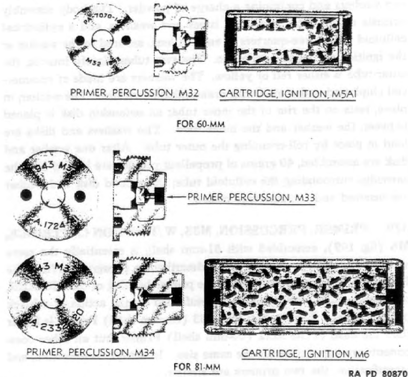
Figure 199 — Primers and Ignition Cartridges for Use With Mortar Ammunition
