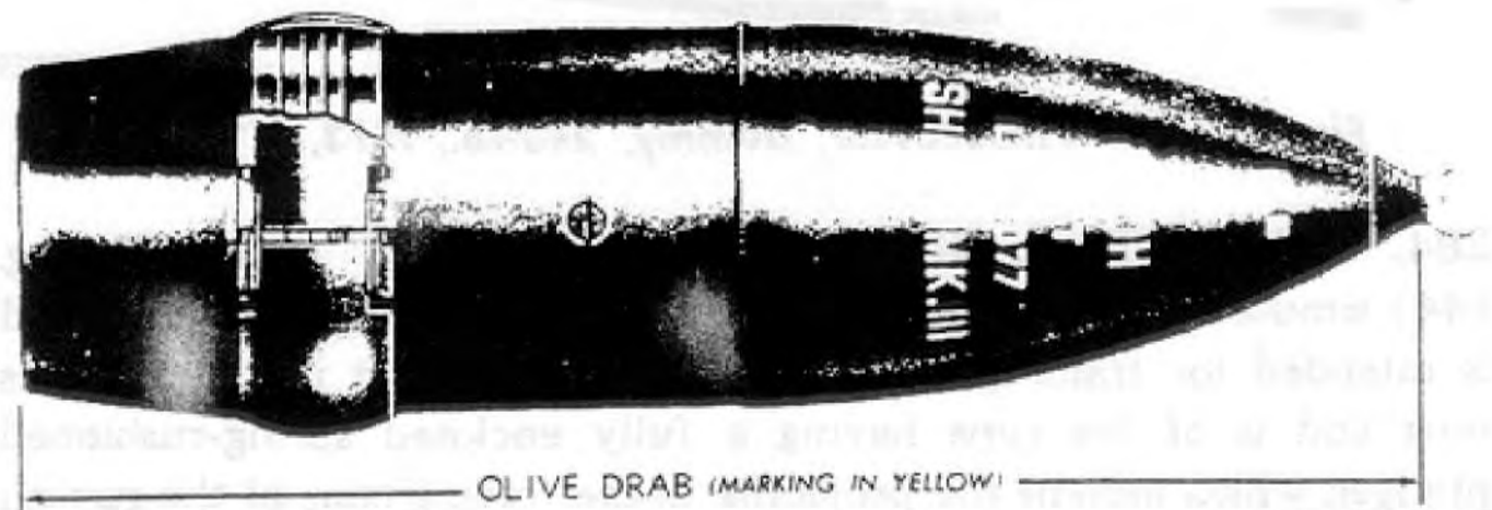
Figure 145 - SHELL, H.E., Mk. III, Unfuzed, 240-mm How., M1918-18A1-18MI-18MIA1
