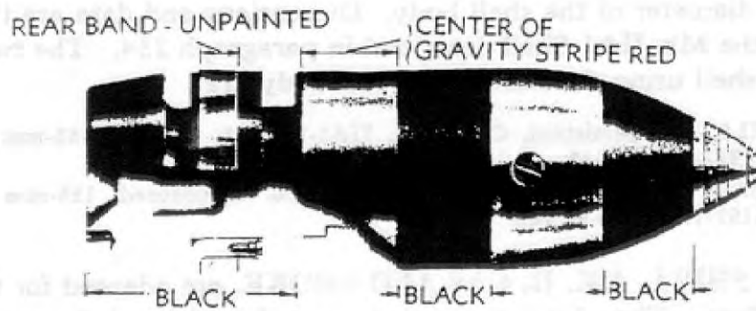
Figure 133 — PROJECTILE, Dummy, 95-lb., Mk. I, 155-mm How.
