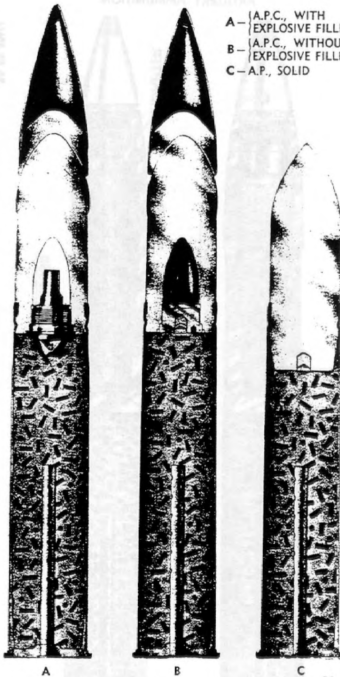
Figure 2—Typical Armor-piercing and Armor-piercing-capped Complete Rounds
