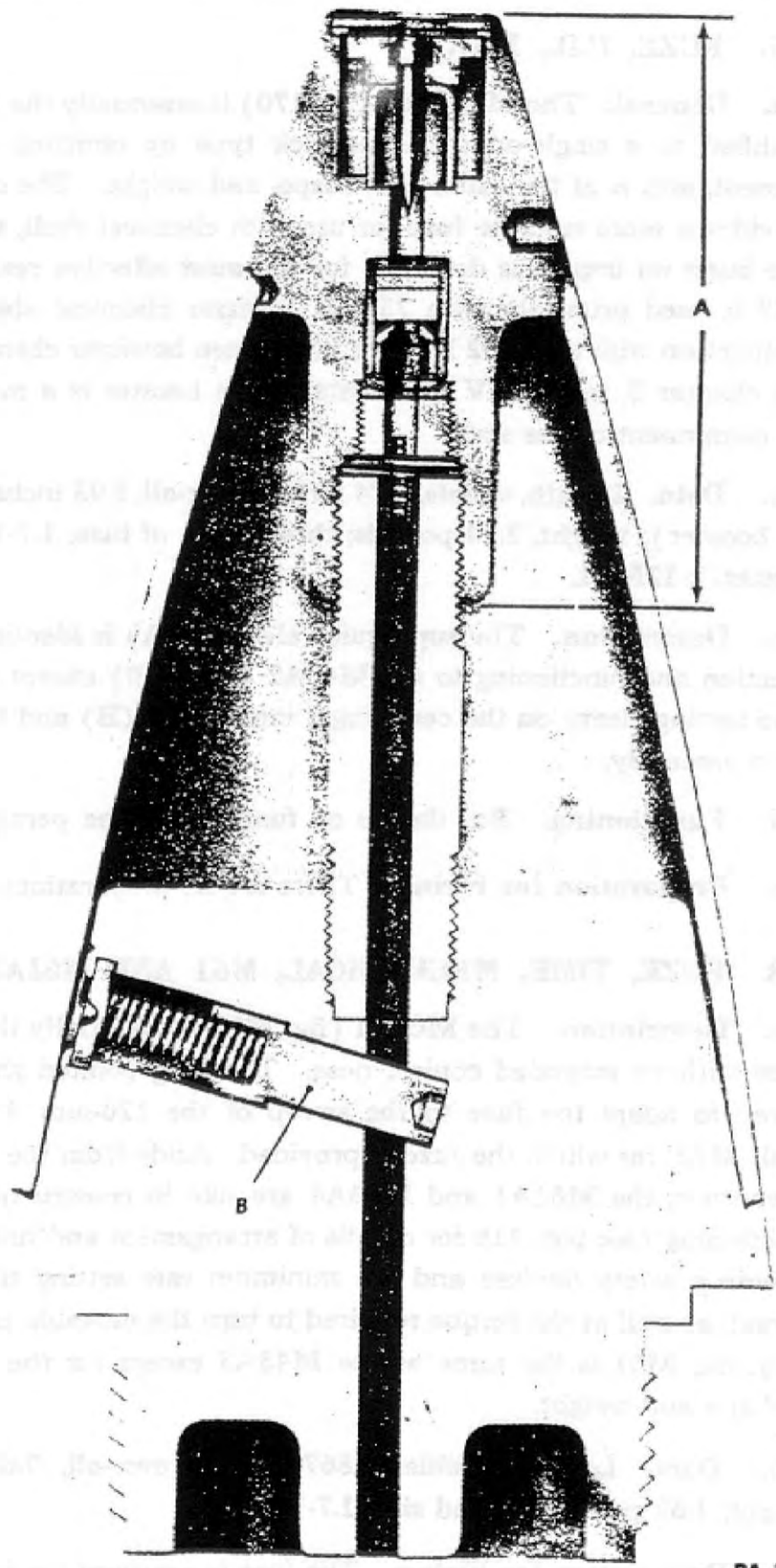
Figure 170 — FUZE, P.D., M57
