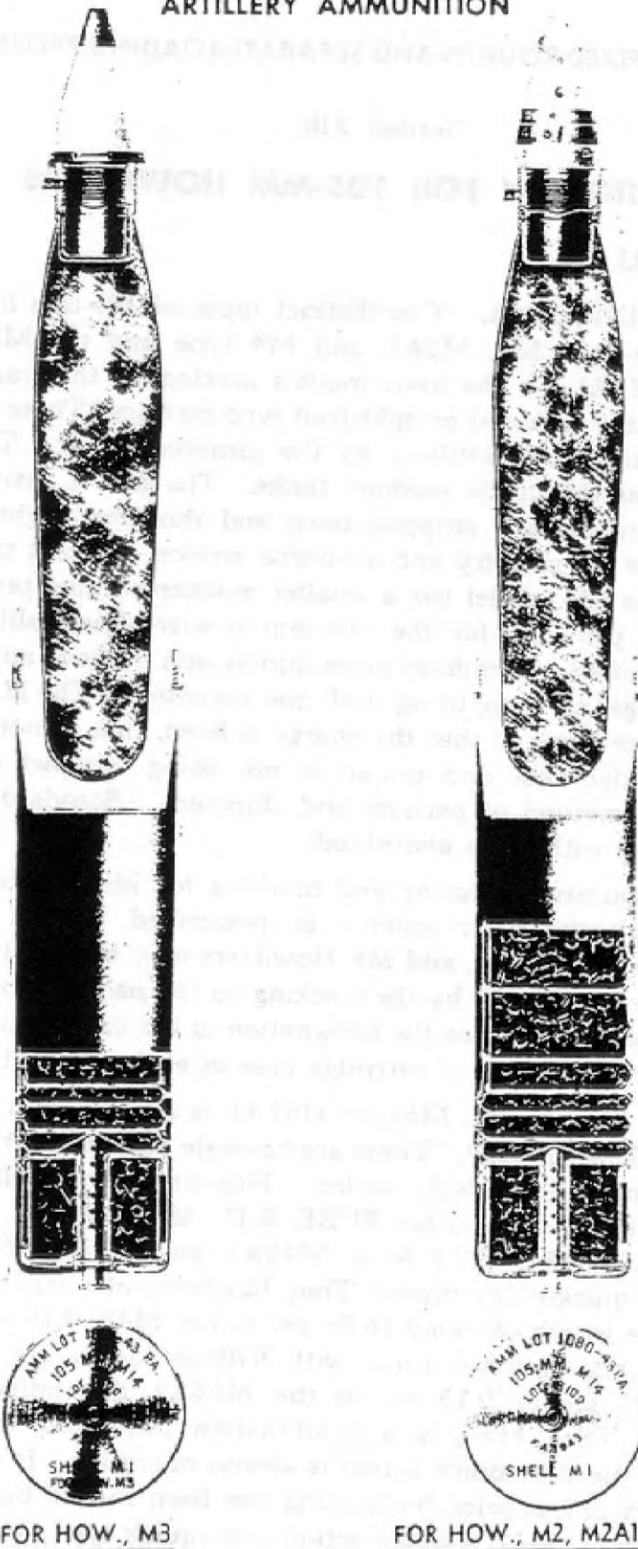
Figure 112 – Comparison of 105-mm Howitzer Complete Rounds
