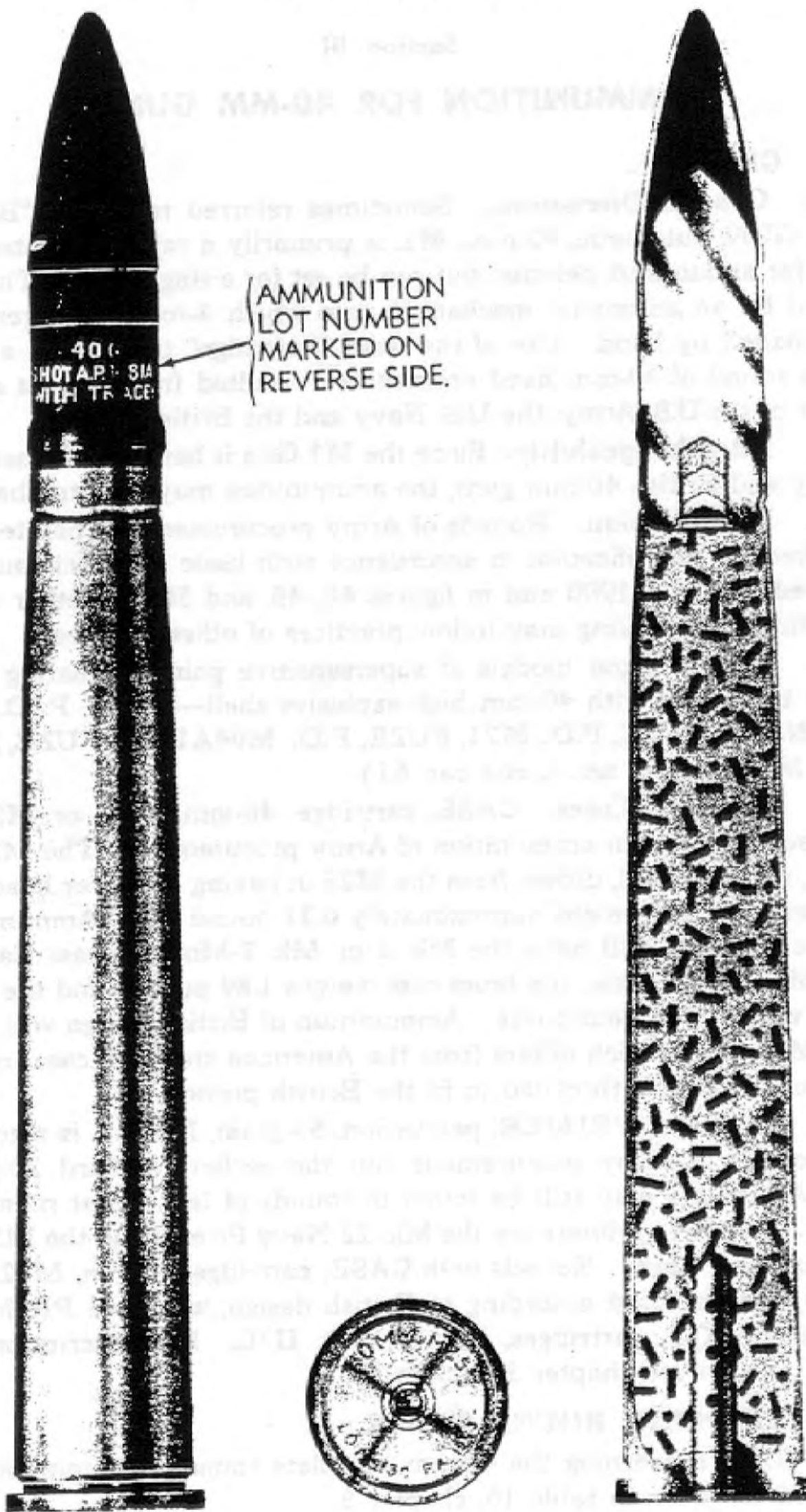
Figure 48 - CARTRIDGE, AP-T, M81A1, 40-mm AA. Guns
