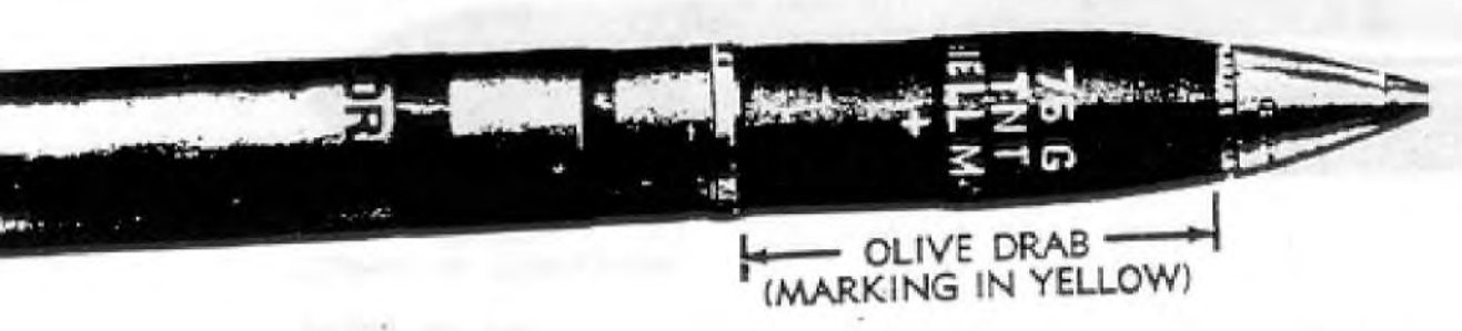
Figure 64 — SHELL, Fixed, H.E., M48, Normal Charge, w/FUZE, P.D., M48A2, SQ & 0.15-sec. Delay, 75-mm Gun
