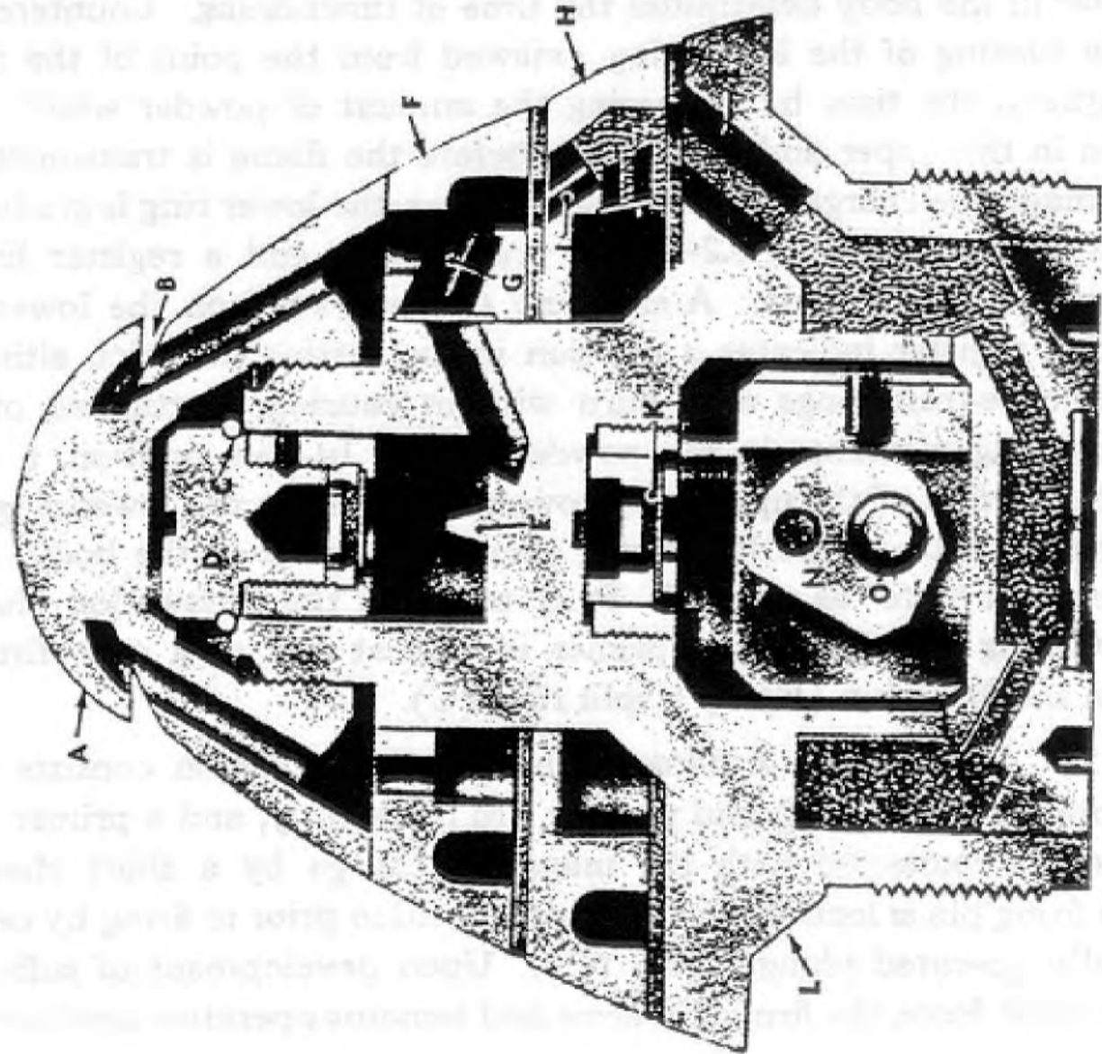
Figure 179 — FUZE, Combination, 21-sec., M1907M
