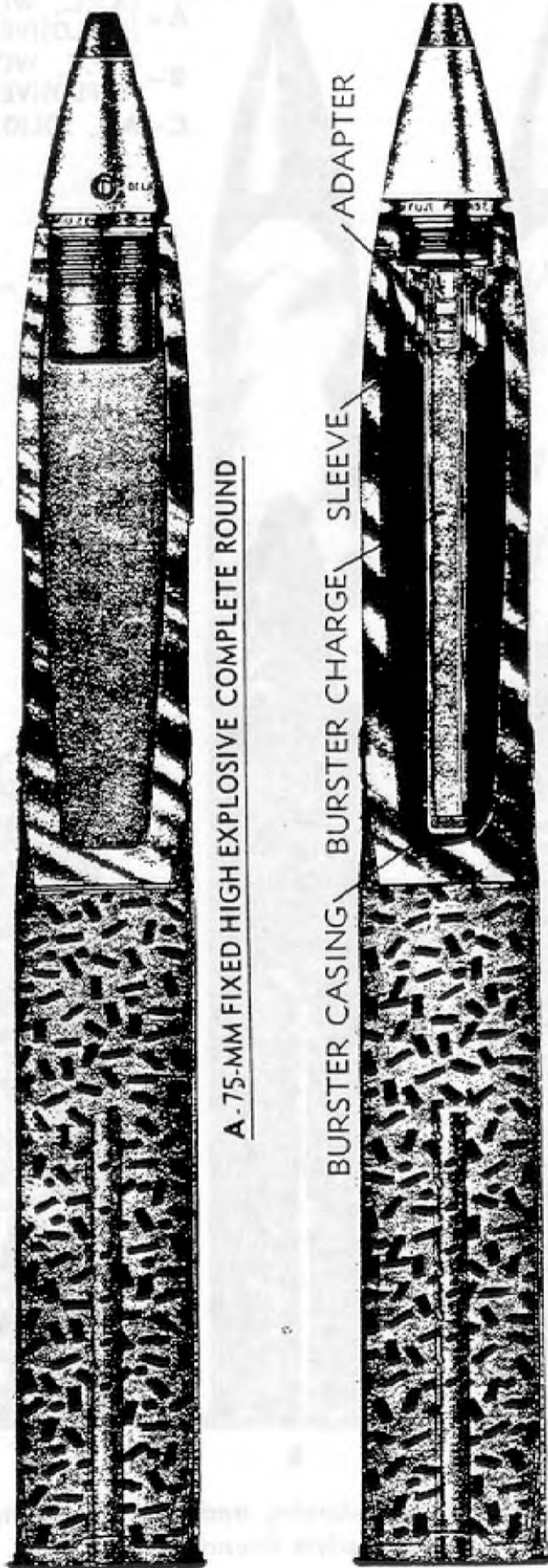
B. 75-MM FIXED CHEMICAL COMPLETE ROUND
