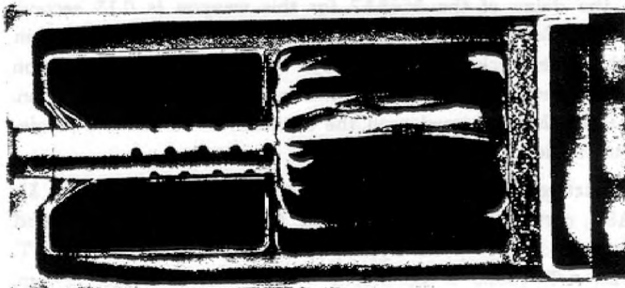
Figure 73 — AMMUNITION, Blank (Double Pellet Charge), 75-mm Guns, M1897-16-17, 75-mm How., M1 and M1A1, and 3" Field Guns, M1902-04-05
