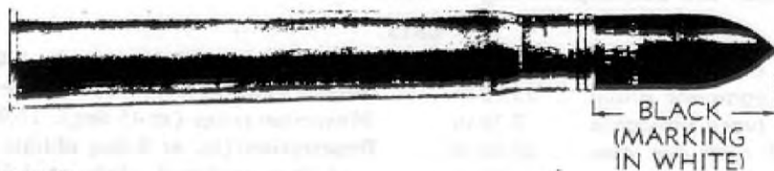
Figure 93 — SHOT, Fixed, A.P., M79, w/TRACER, 3" Guns, M1918 (All Models), M3, M5, M6, and M7
