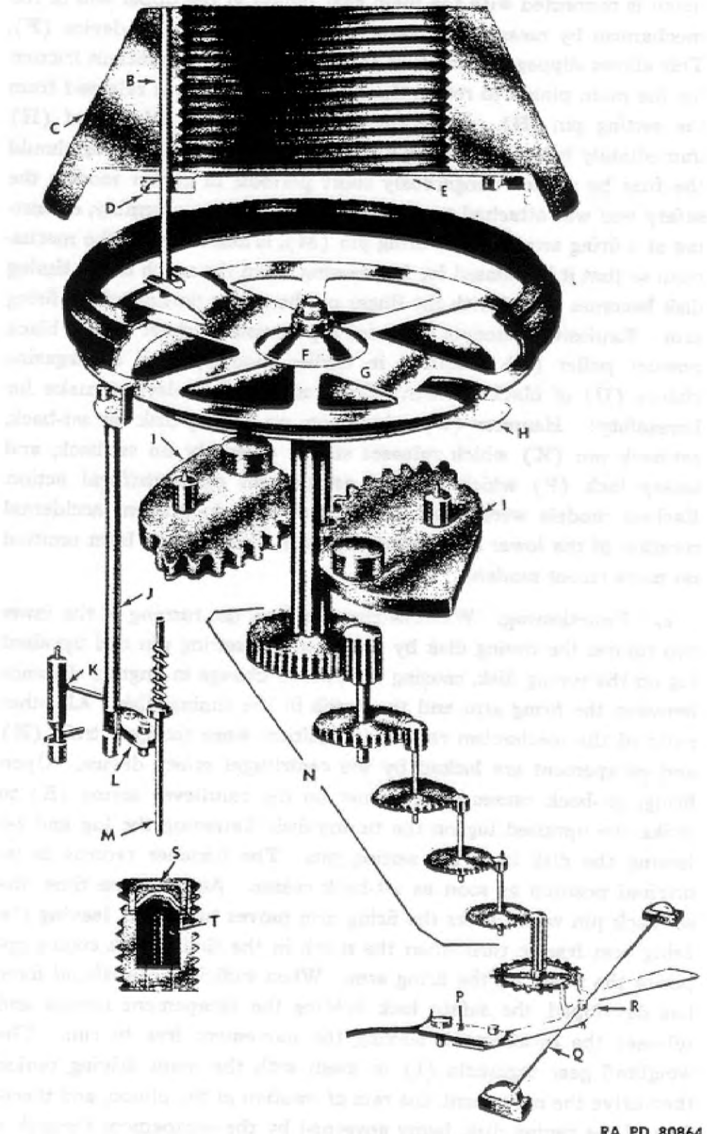
Figure 159 — Mechanism of FUZE, Time, Mechanical, M43A4
