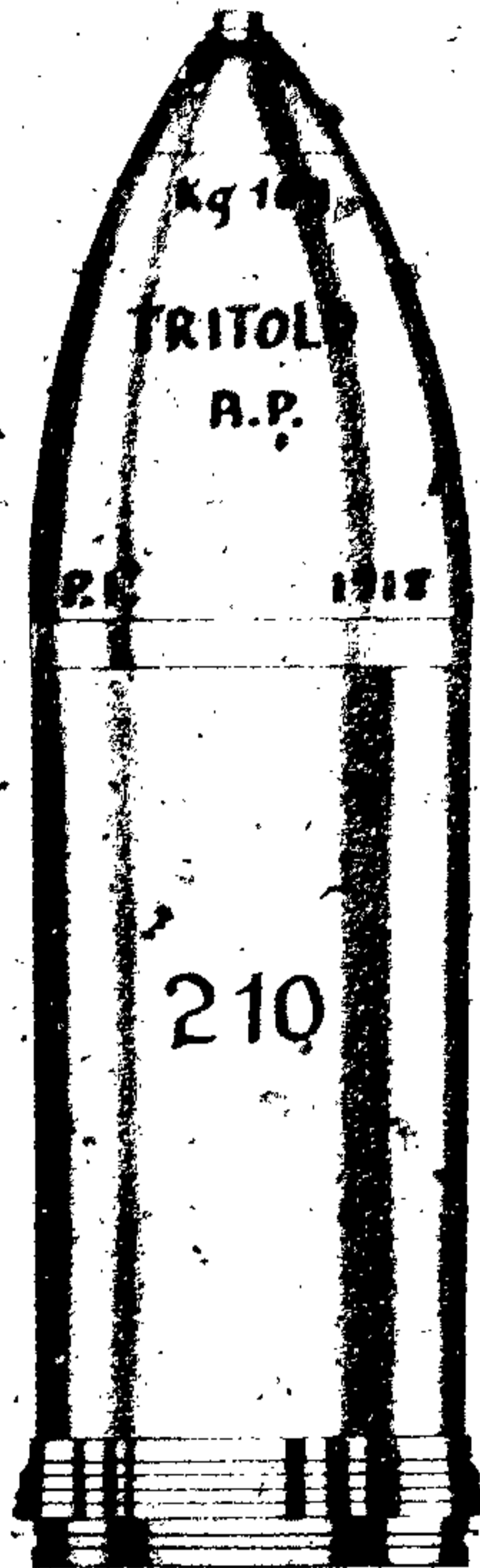
Figure 168 - 210-mm H.E.
