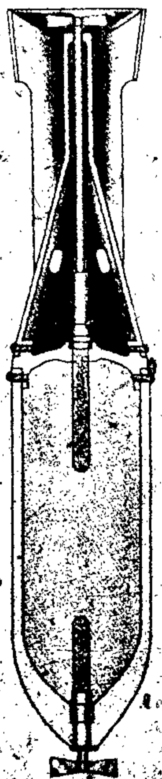
Figure 29 - 250-kg. and 500-kg. (500T) Gas Bombs
