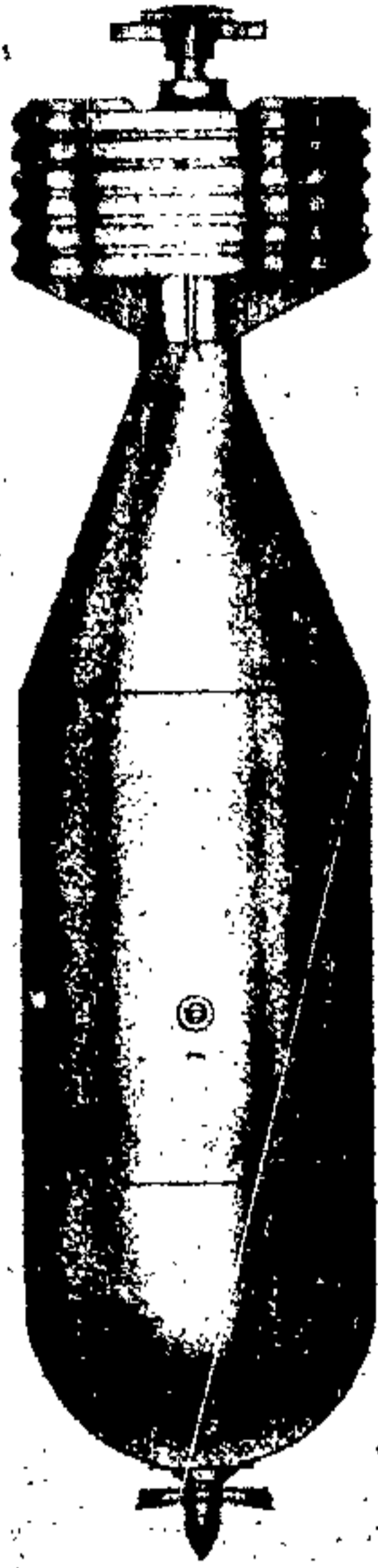
Figure 31 —160-kg. (CS) Antisubmarine Bomb
