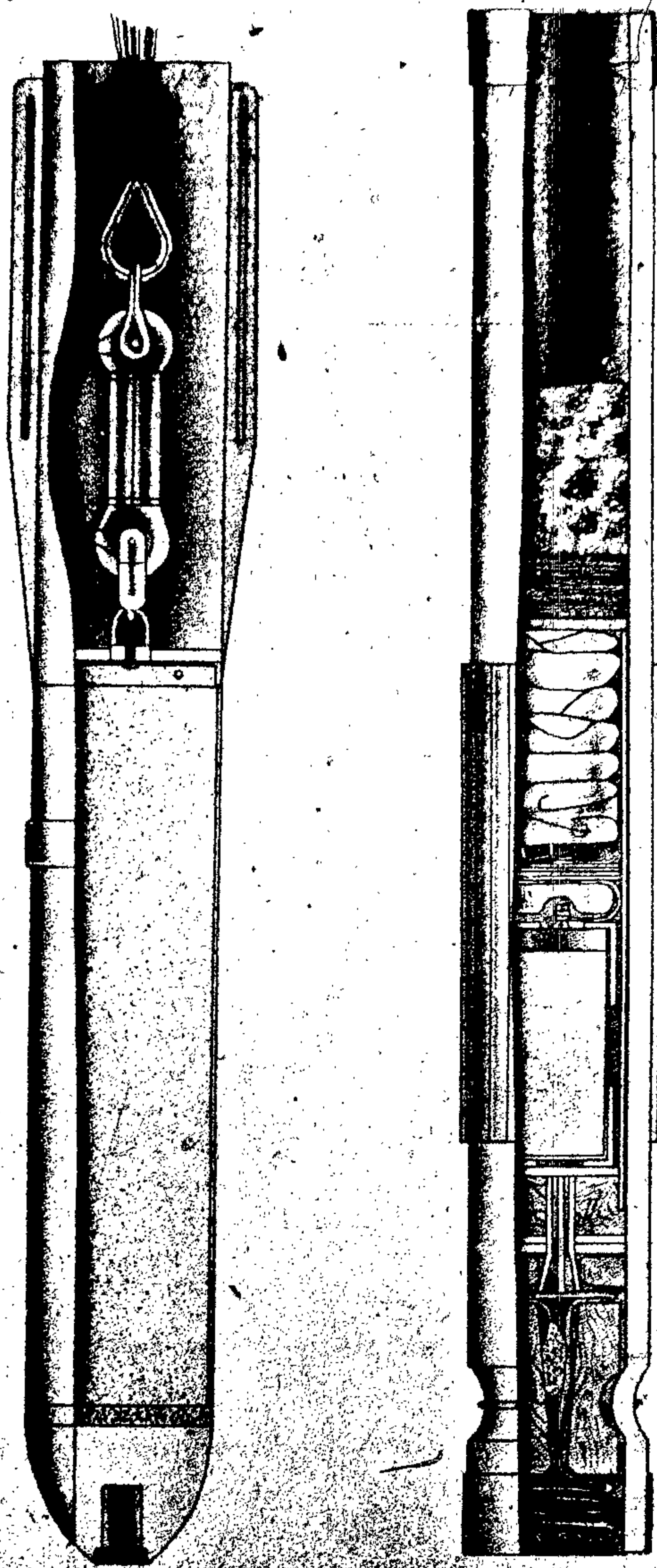
Figure 37 - Parachute Flares
