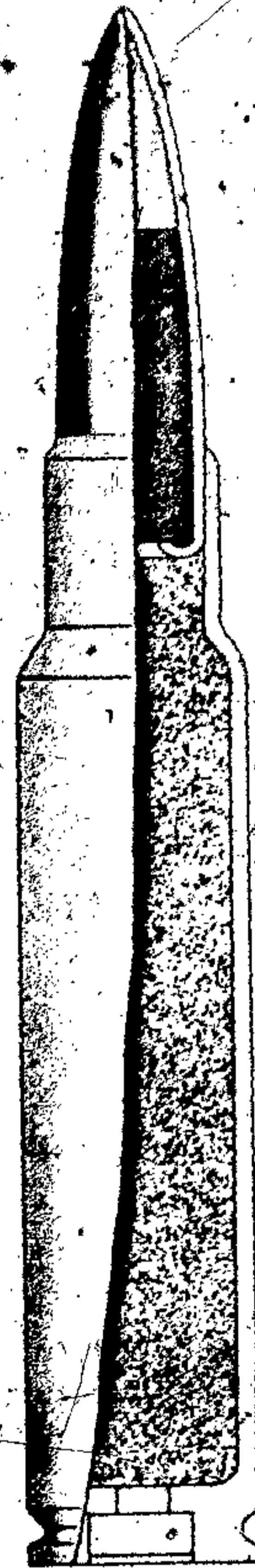
Figure 77 - 7.35-mm Ball
