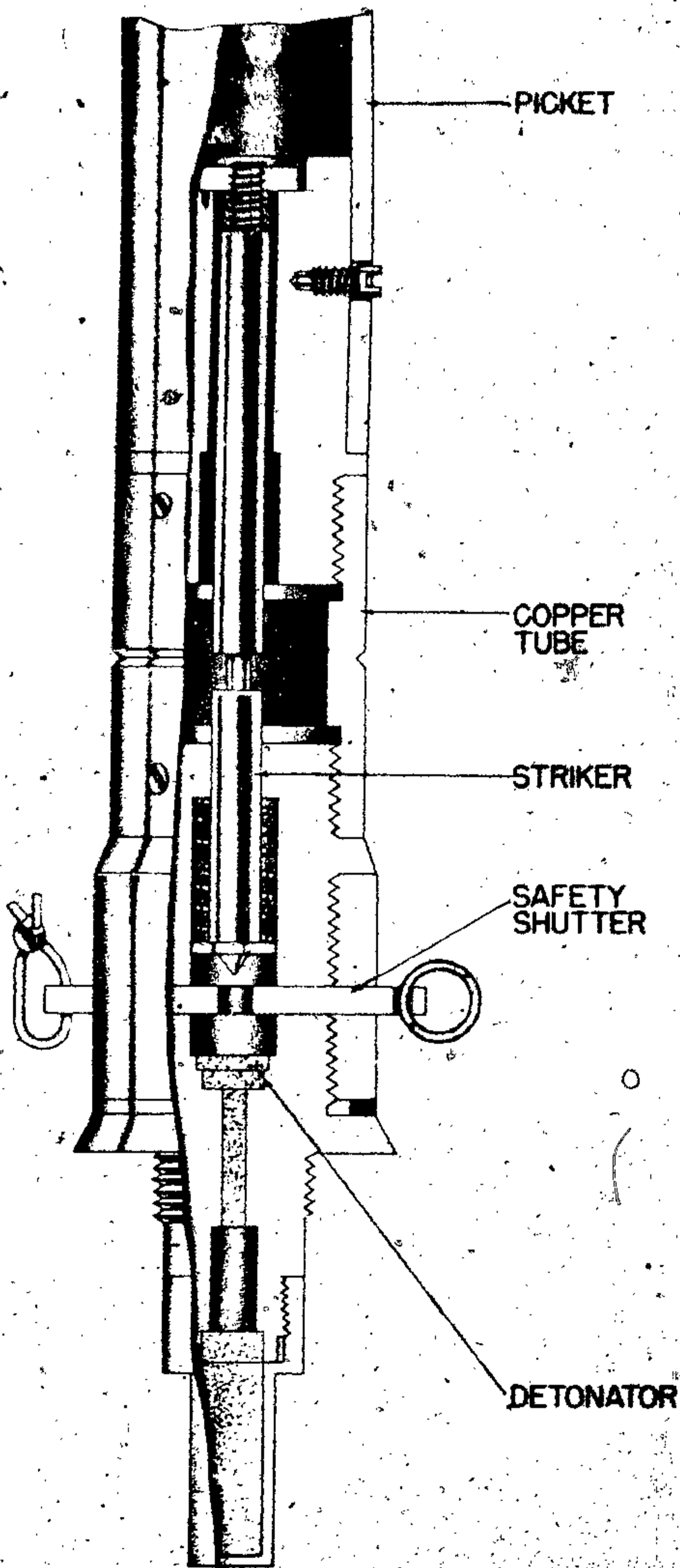
Figure 280 - Rupture Igniter
