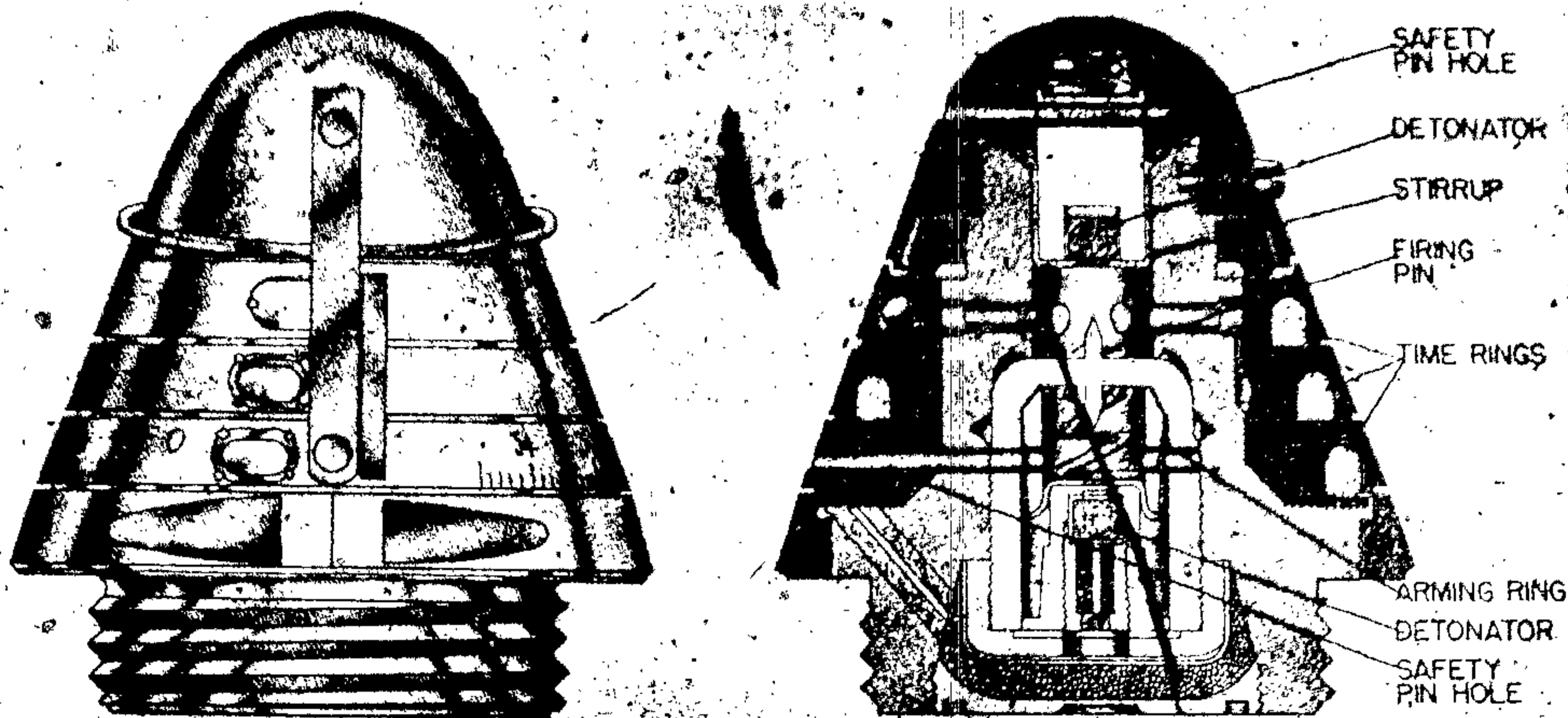
Figure 219 - Time and Percussion Nose Fuze A.D.E. M12
