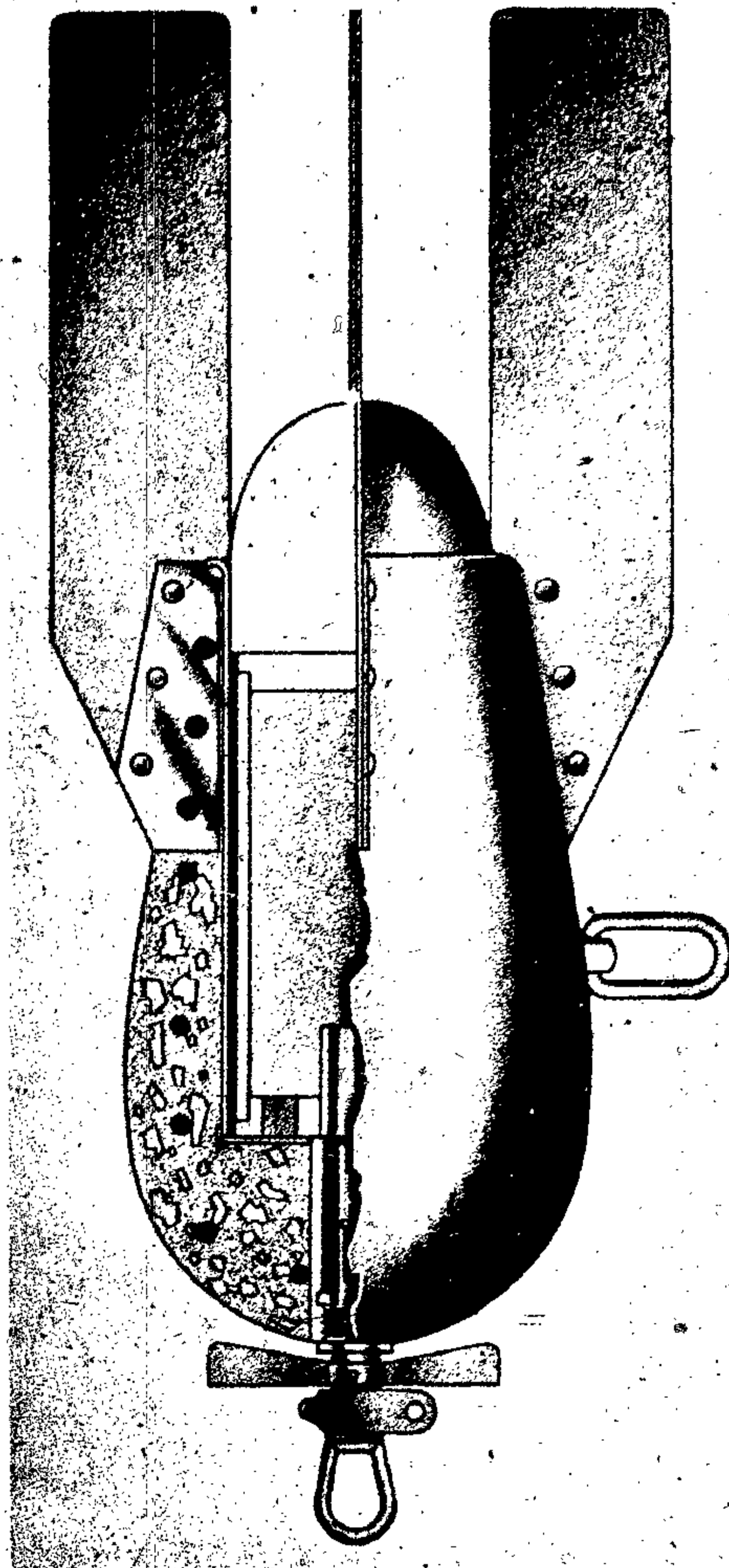
Figure 30 – 5-kg. Vento-Marker
