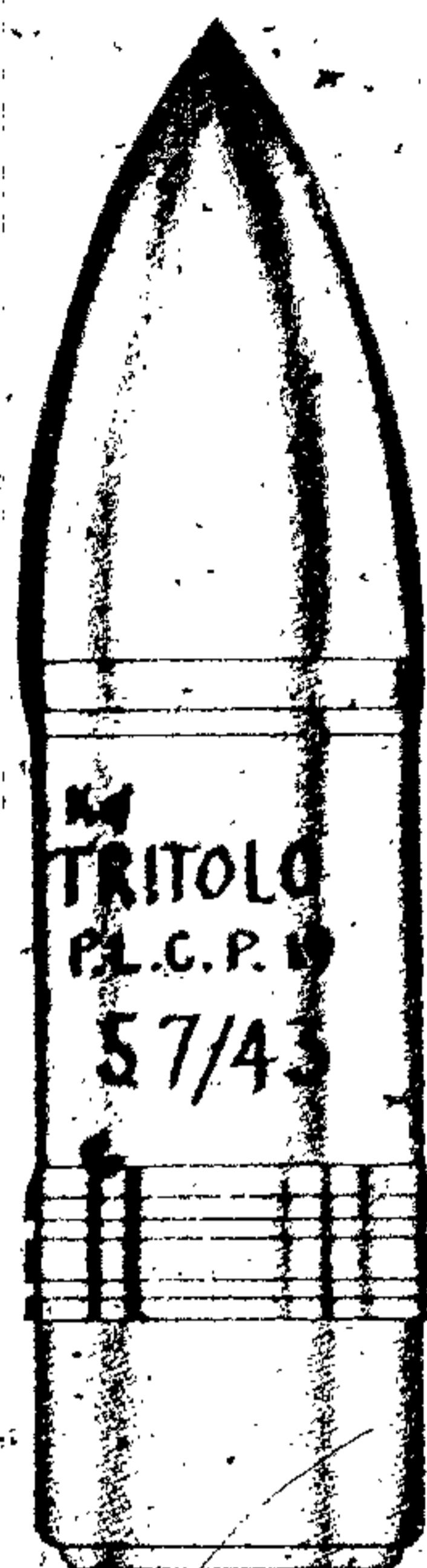
Figure 98.- 57/43-mm A.P. (Without Cap)
