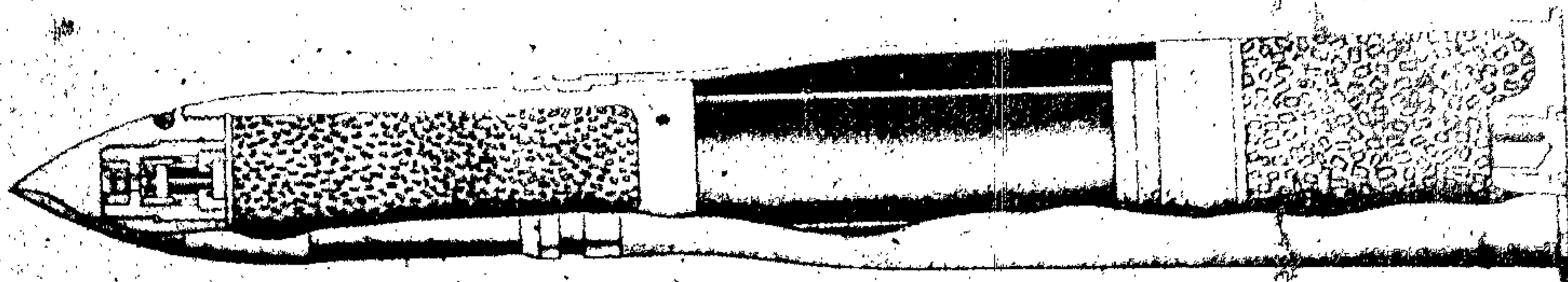
Figure 87 - 37/40-mm H.E.
