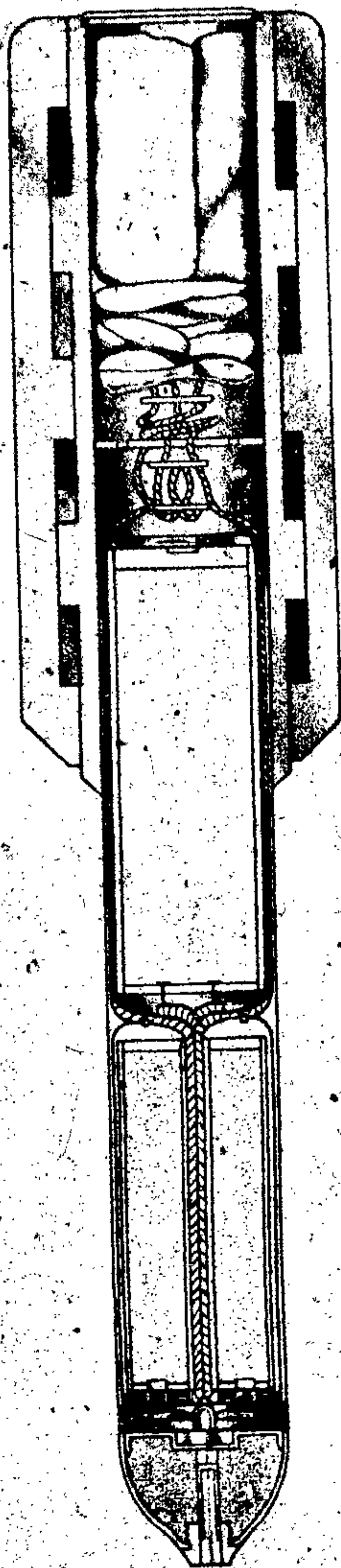
Figure 260 - 10-kg. Parachute Flare Type B
