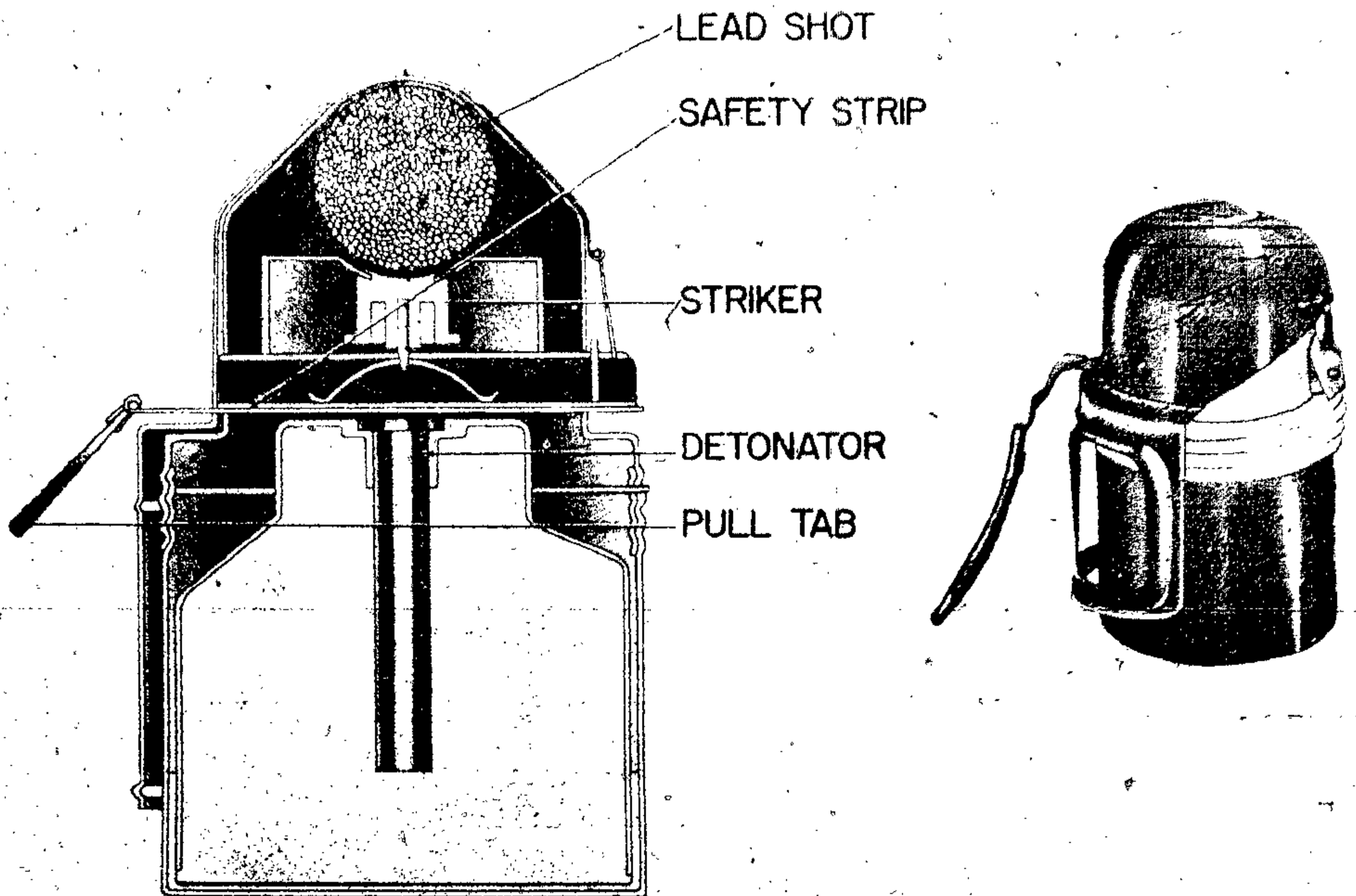
Figure 227 – Hand Grenade O.T.O. Mod 35
