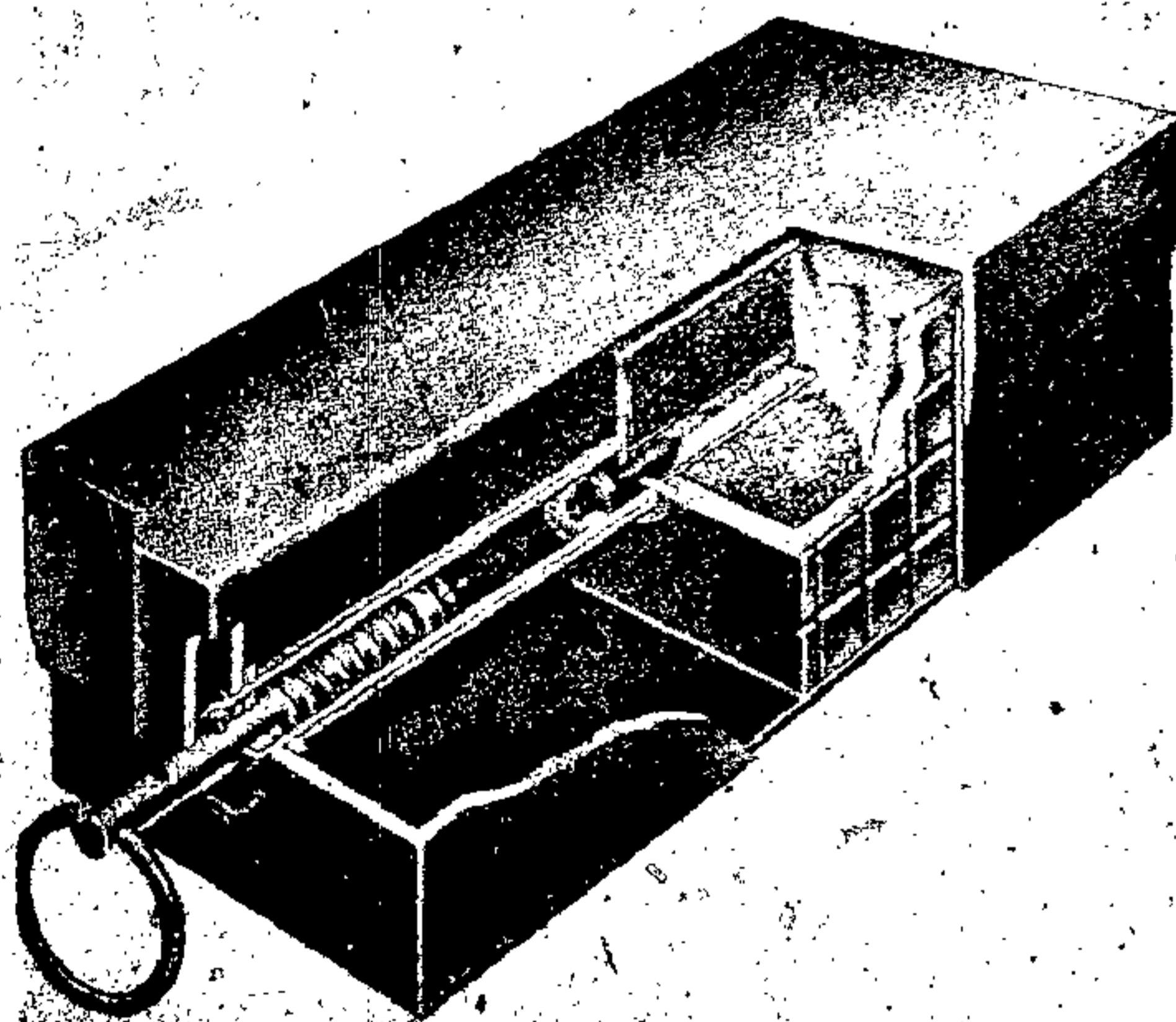
Figure 237 — Bakelite Mine — Anti-Personnel
