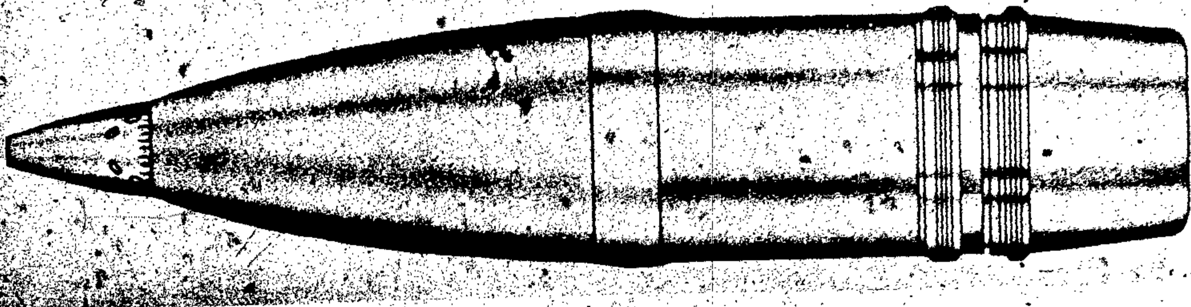
Figure 160 - 149/40-mm A.D.E.-H.E. M35
