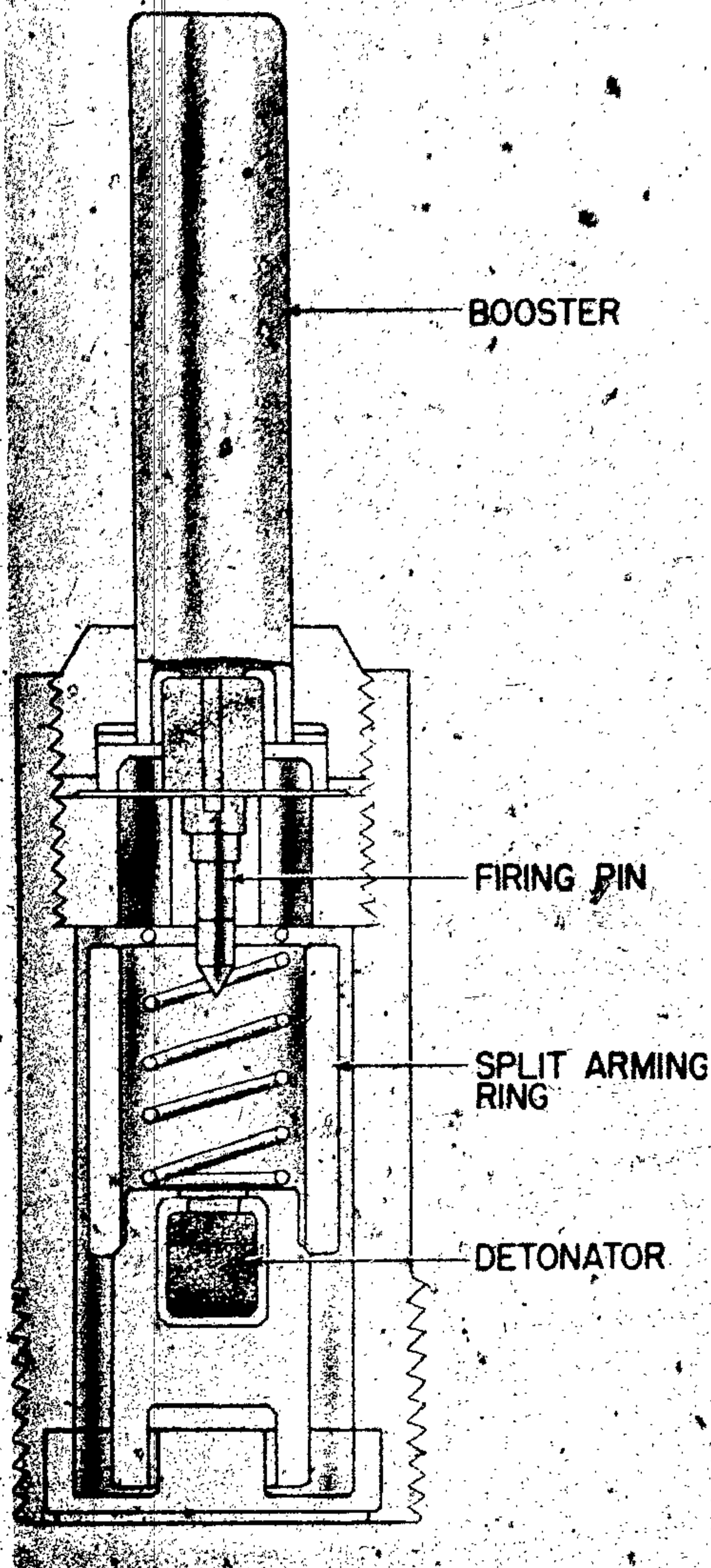
Figure 224 - Base Fuze for 47/32 A.P.
