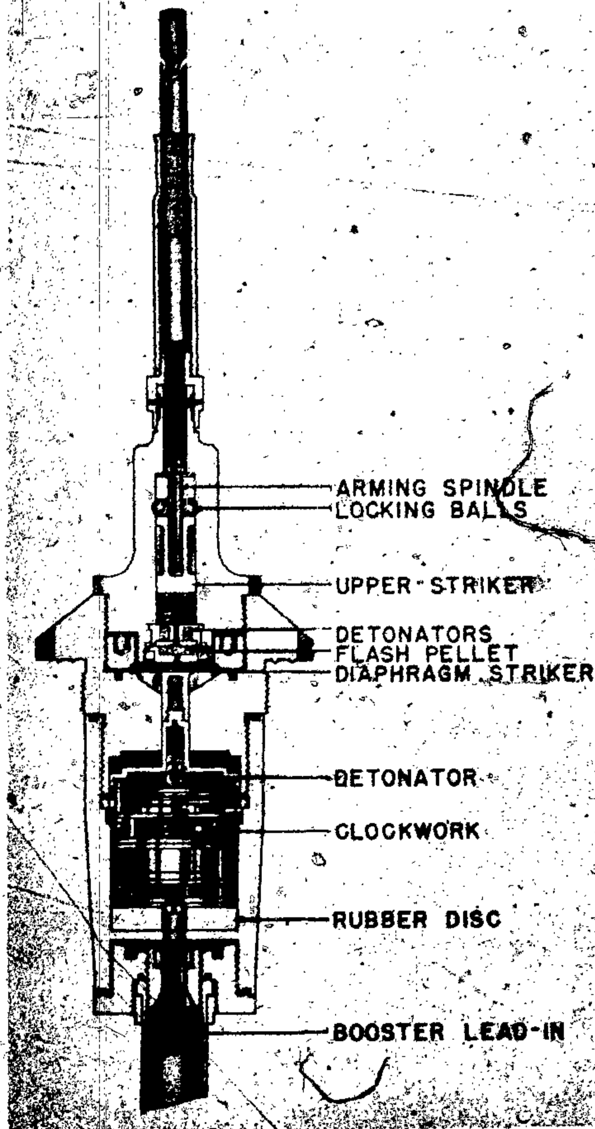
Figure 65 - Clockwork Long-Delay Tail Fuze
