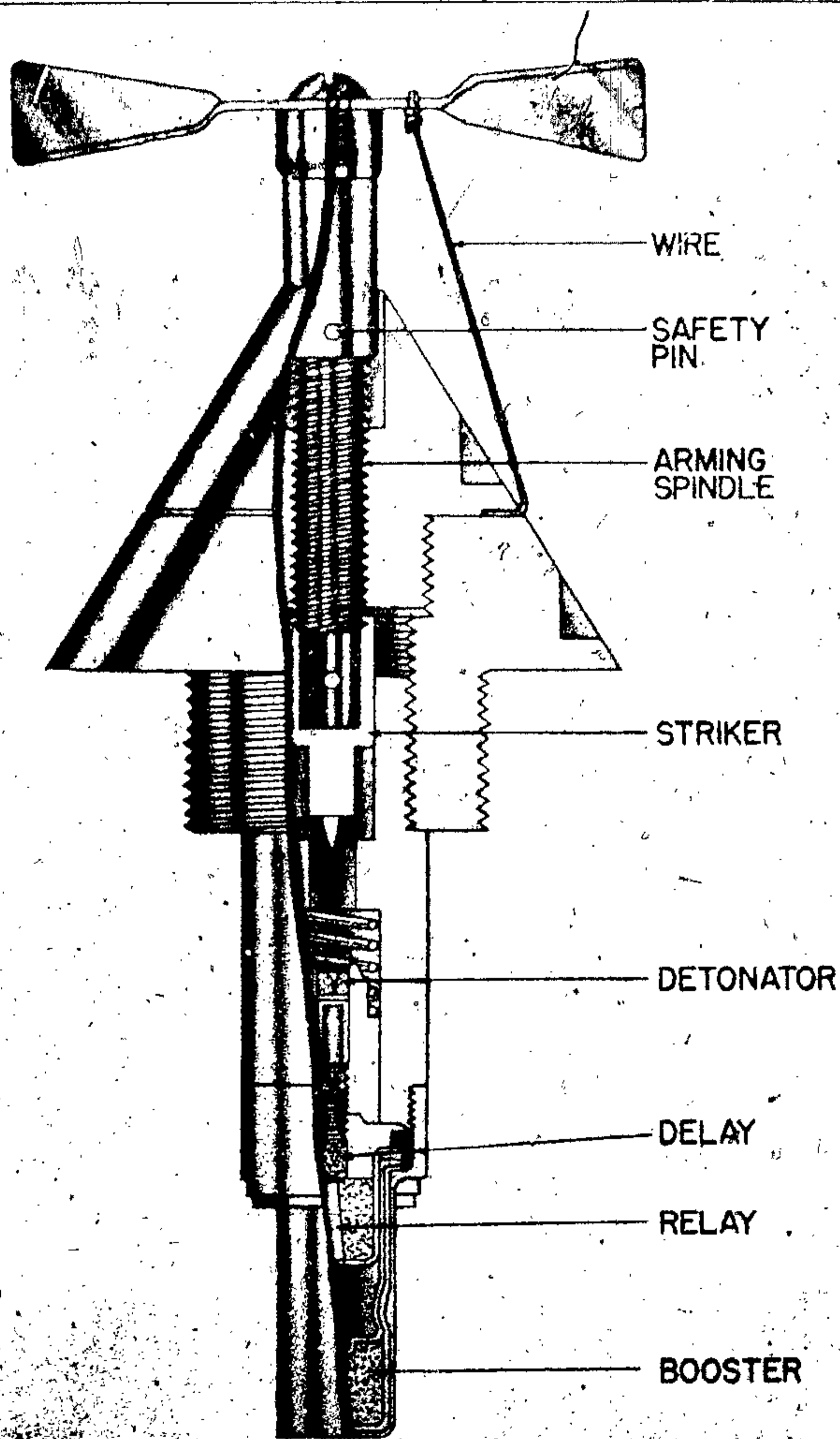
Figure 263 - Mechanical Impact Nose Fuze Type A
