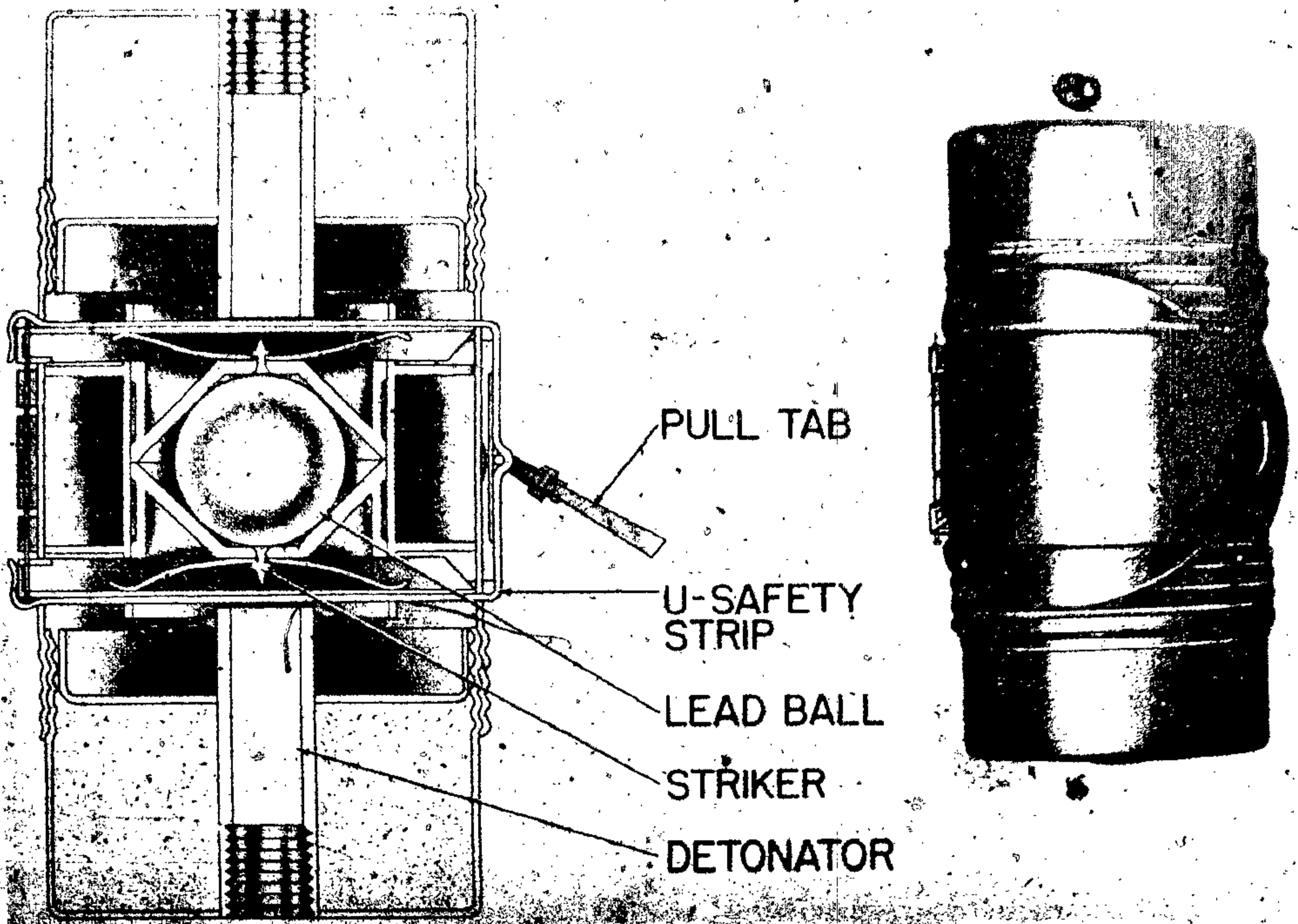
Figure 229 - P.C.R. Grenade
