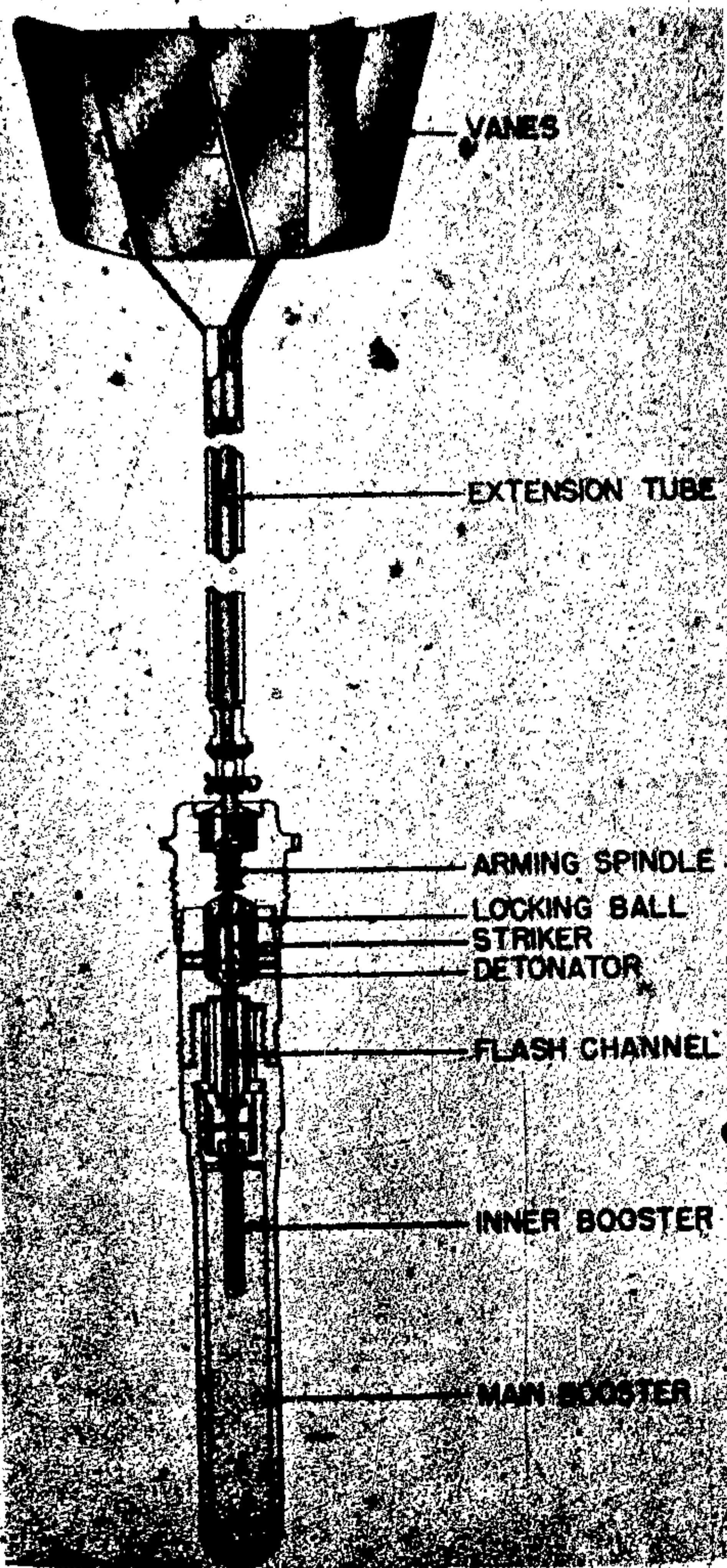
Figure 59 - Type P - Mechanical Impact Tail Fuze
