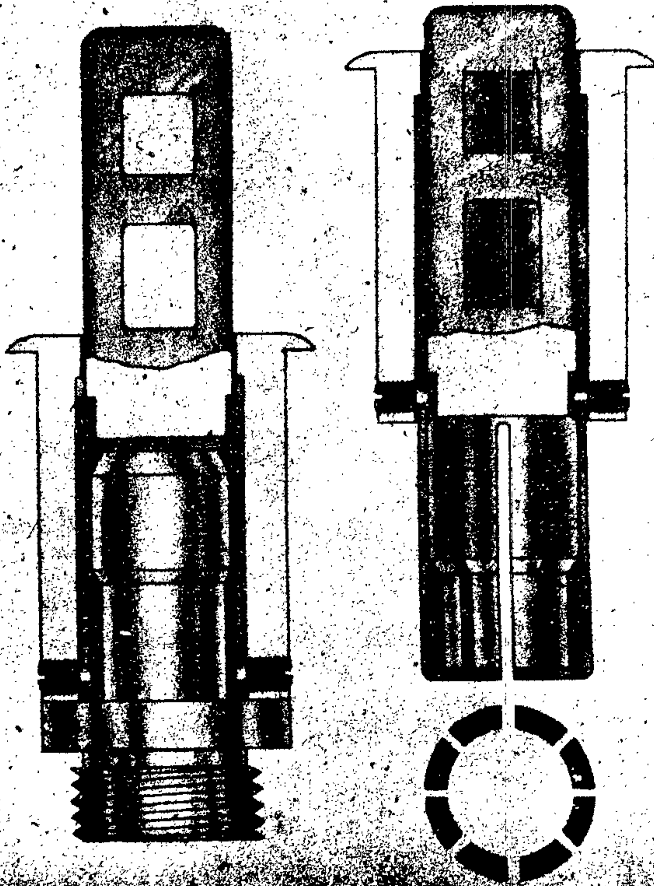
Figure 262 - Secondary Safety Devices
