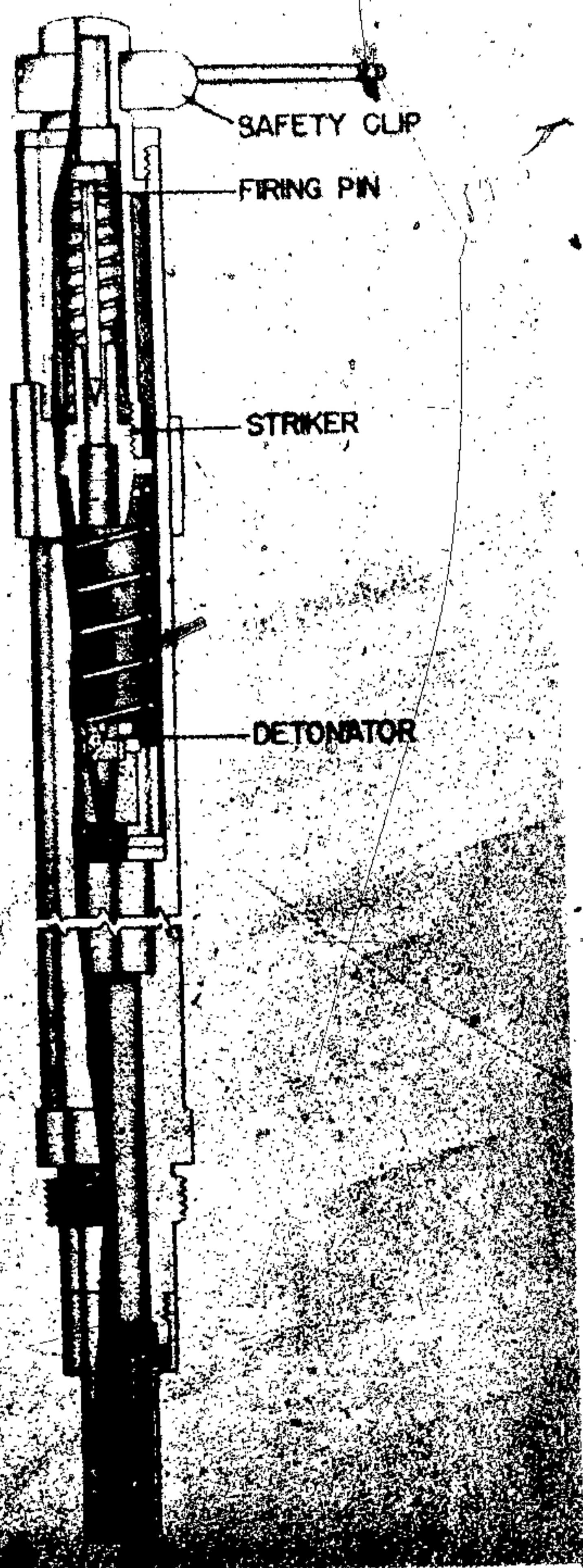
Figure 273—Mechanical Impact Tail Fuze Sch. R. Model 1938
