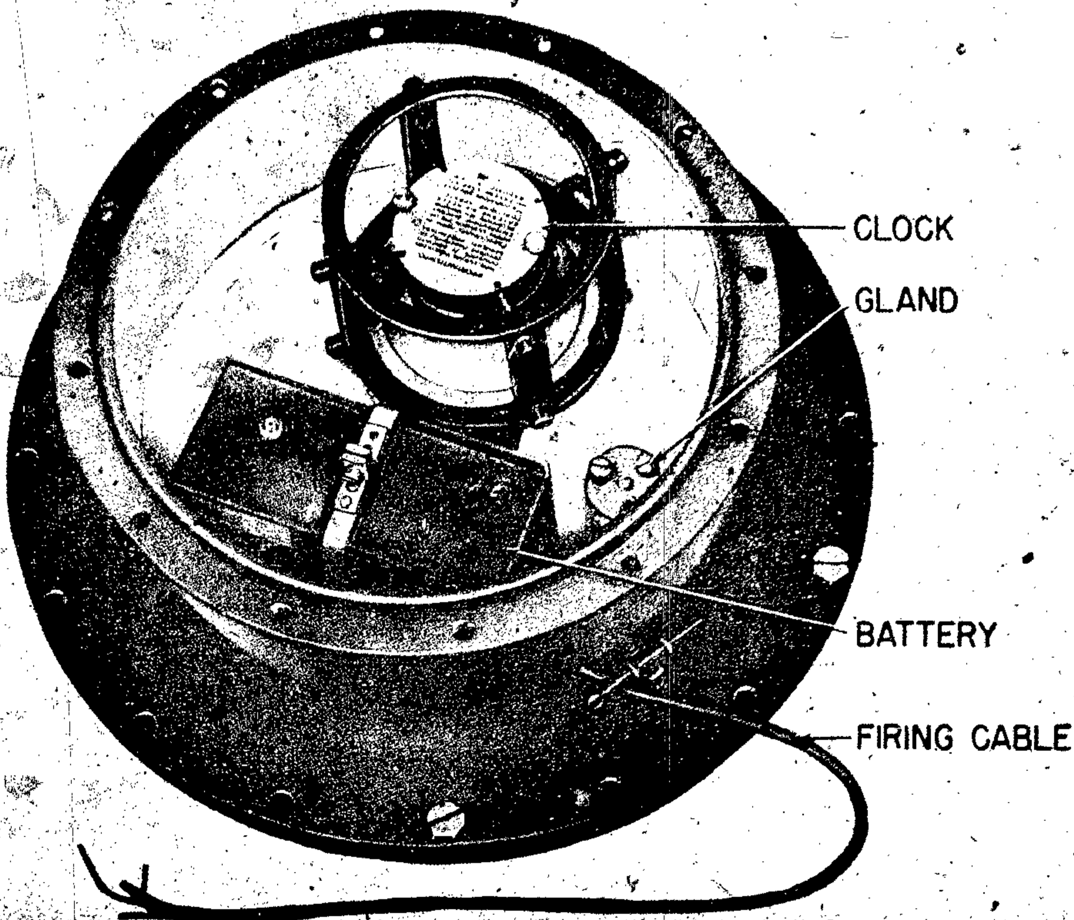
Figure 248 - 50-Day Clock
