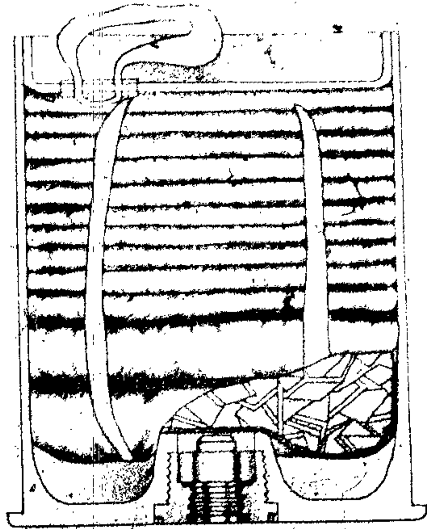
Figure 190 – 100/17-mm Light Field Howitzer Cartridge Case
