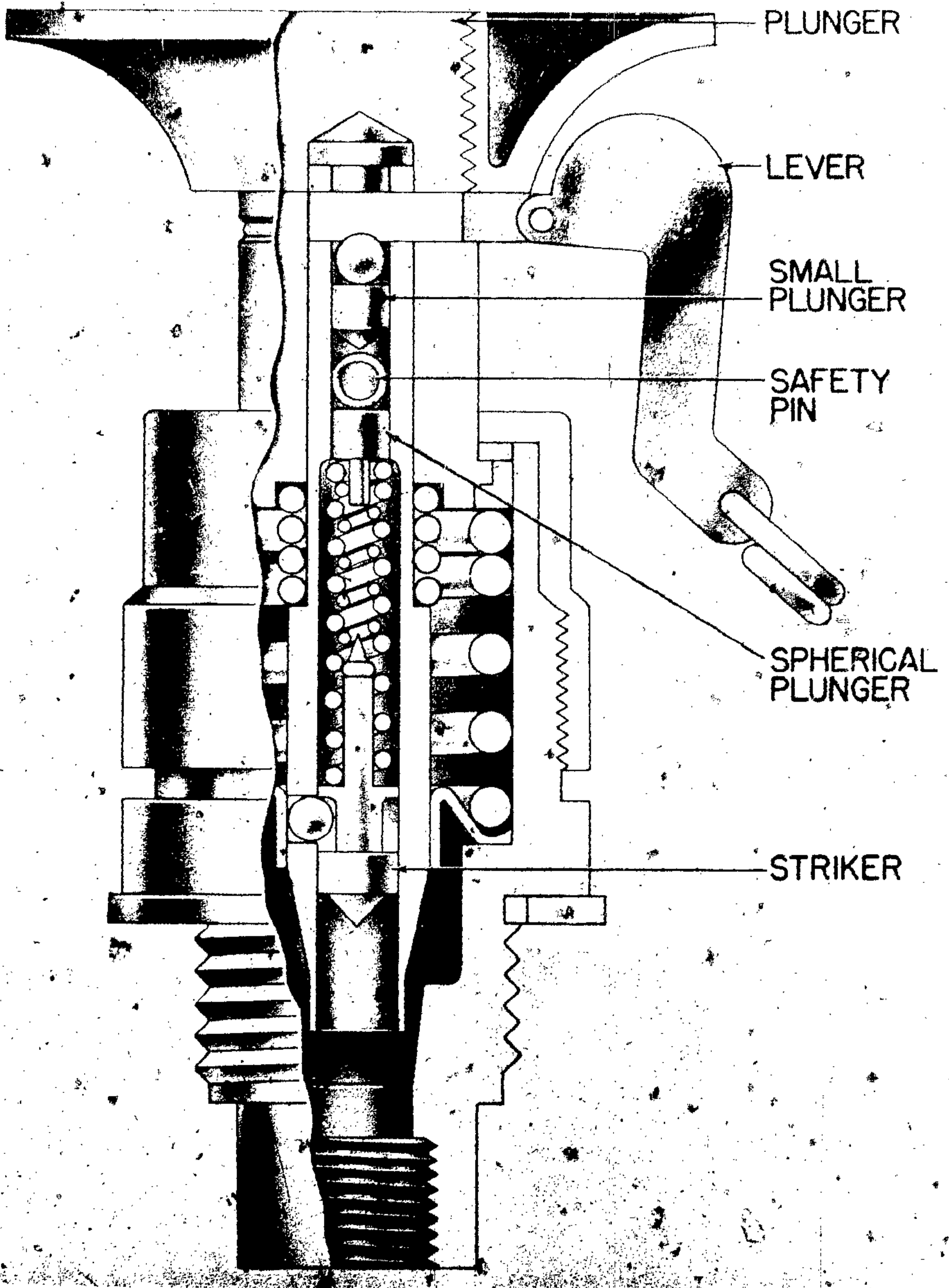
Figure 282 - Push-and-Pull Igniters
