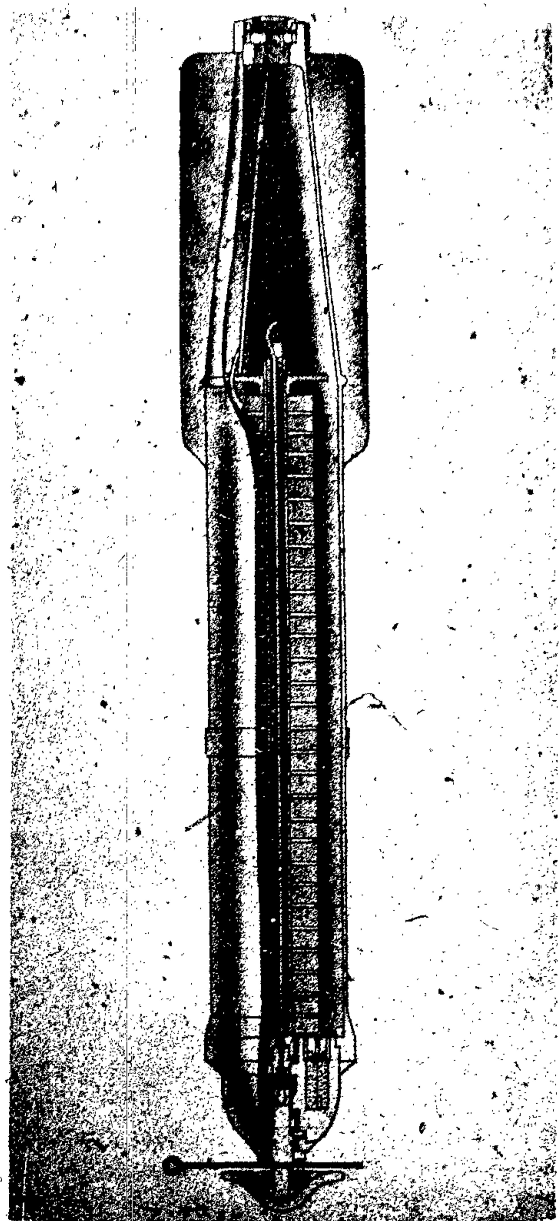
Figure 18 -- 12-kg. Smoke Bomb
