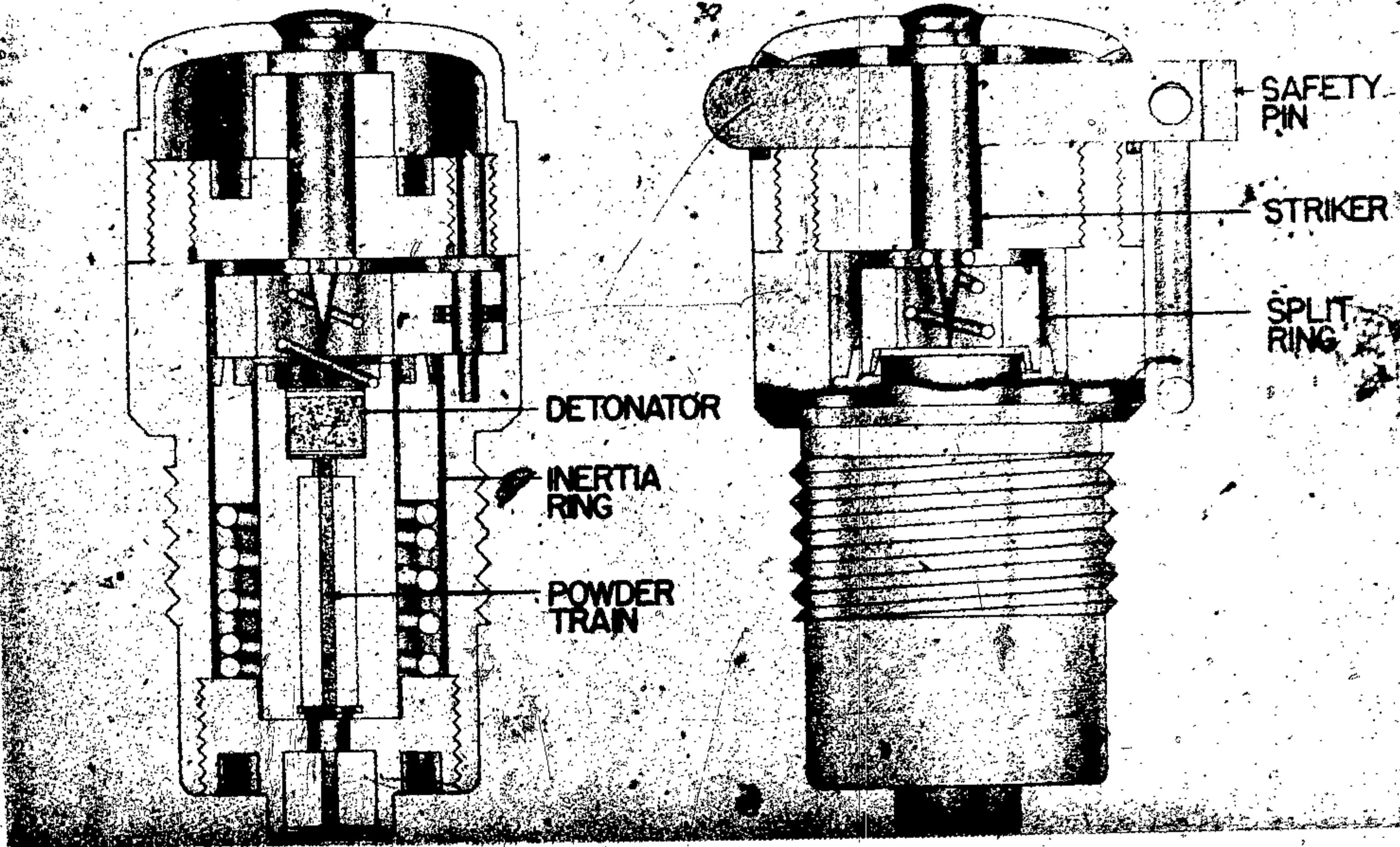
Figure 202 - Percussion Nose Fuze M10 (Guerritore) p.c.
