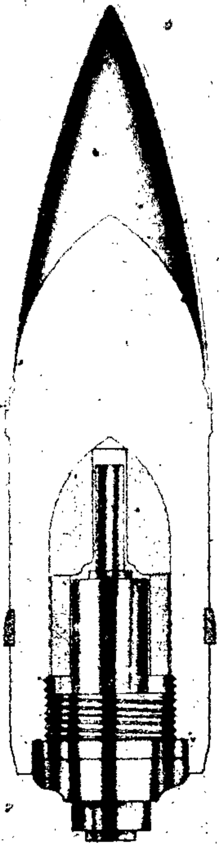
Figure 93 - 47/32-mm A.P. M35 (With Cap)
