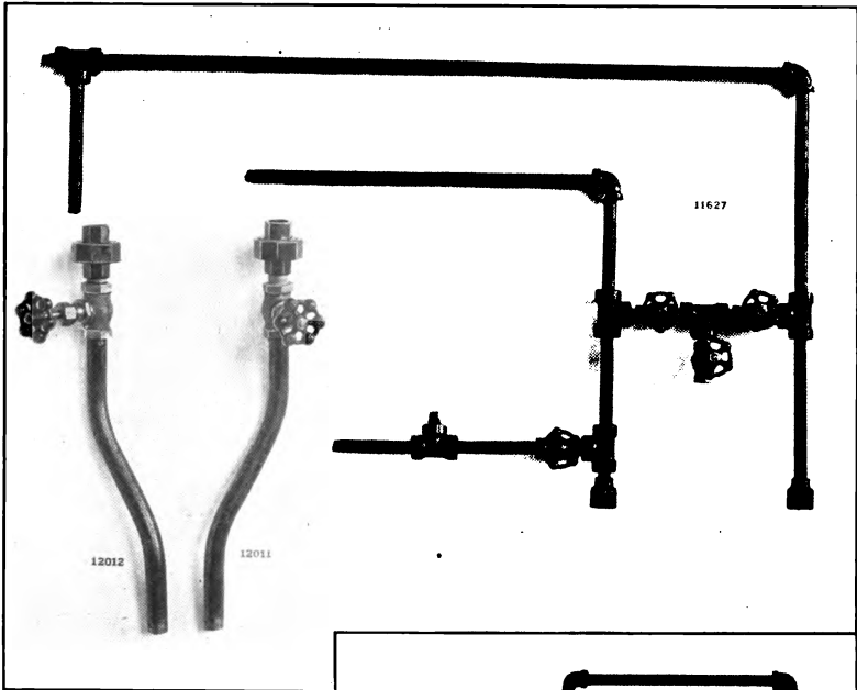
(above) FIG. 1590 TYPE C METER PIPING
