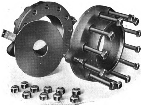
FIG. 1367 Orifice Plate and Flanges Patented
