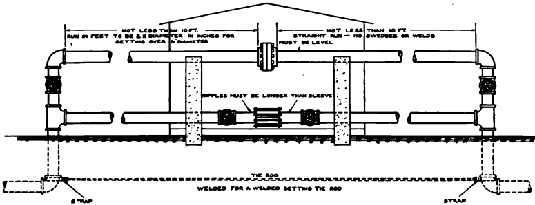
GOVERNMENT STANDARD ORIFICE METER SETTING IN THE OSAGE
